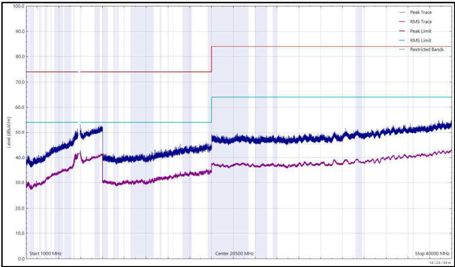
Figure 445 - U-NII-3 - 5825 MHz (CH165), 802.11a, Core 0, 1 GHz to 40 GHz, Horizontal
