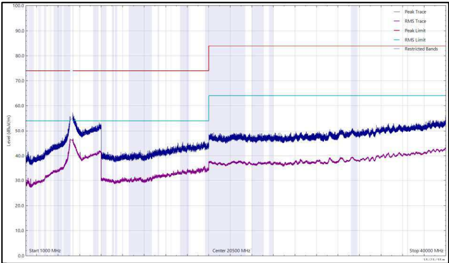
Figure 467 - U-NII-1 - 5180 MHz (CH36), VHT20, CDD, Core 0 + Core 1, 1 GHz to 40 GHz, Vertical
