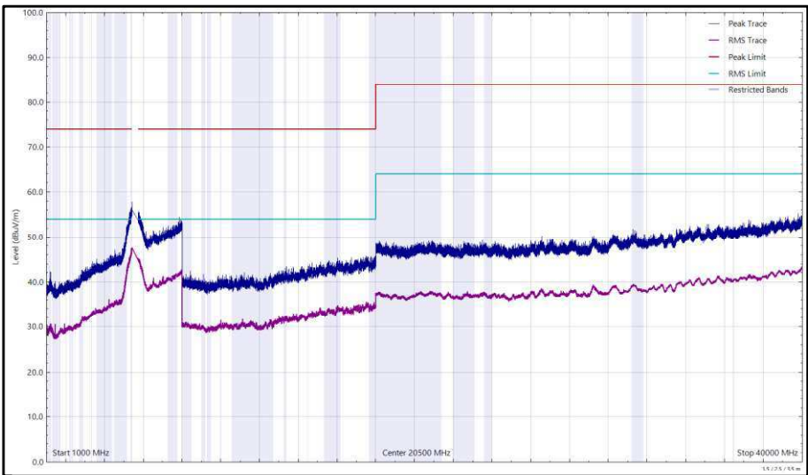
Figure 471 - U-NII-2C - 5500 MHz (CH100), VHT20, CDD, Core 0 + Core 1, 1 GHz to 40 GHz, Vertical
