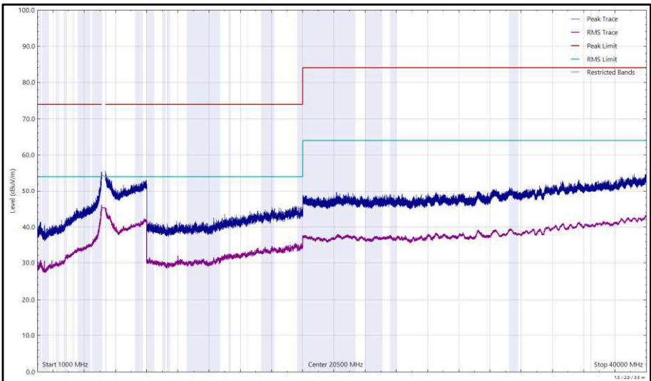
Figure 451 - U-NII-1 - 5180 MHz (CH36), 802.11a, Core 1, 1 GHz to 40 GHz, Vertical
