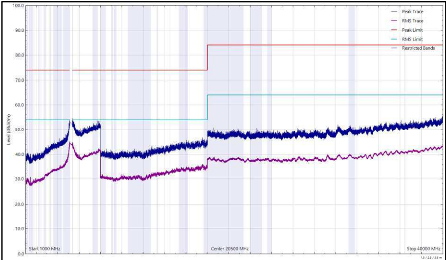
Figure 435 - U-NII-1 - 5180 MHz (CH36), 802.11a, Core 0, 1 GHz to 40 GHz, Vertical
