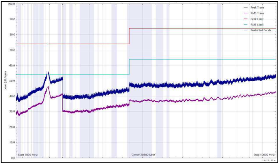
Figure 459 - U-NII-3 - 5745 MHz (CH149), 802.11a, Core 1, 1 GHz to 40 GHz, Vertical
