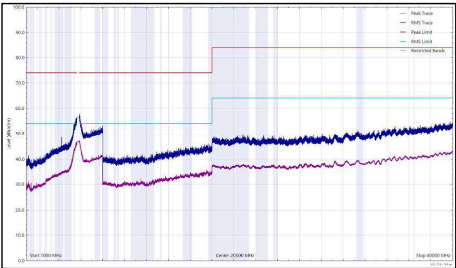
Figure 475 - U-NII-3 - 5745 MHz (CH149), VHT20, CDD, Core 0 + Core 1, 1 GHz to 40 GHz, Vertical
