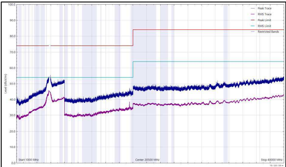
Figure 447 - U-NII-3 - 5825 MHz (CH165), 802.11a, Core 0, 1 GHz to 40 GHz, Vertical
