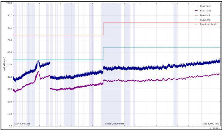
Figure 458 - U-NII-3 - 5745 MHz (CH149), 802.11a, Core 1, 1 GHz to 40 GHz, Horizontal
