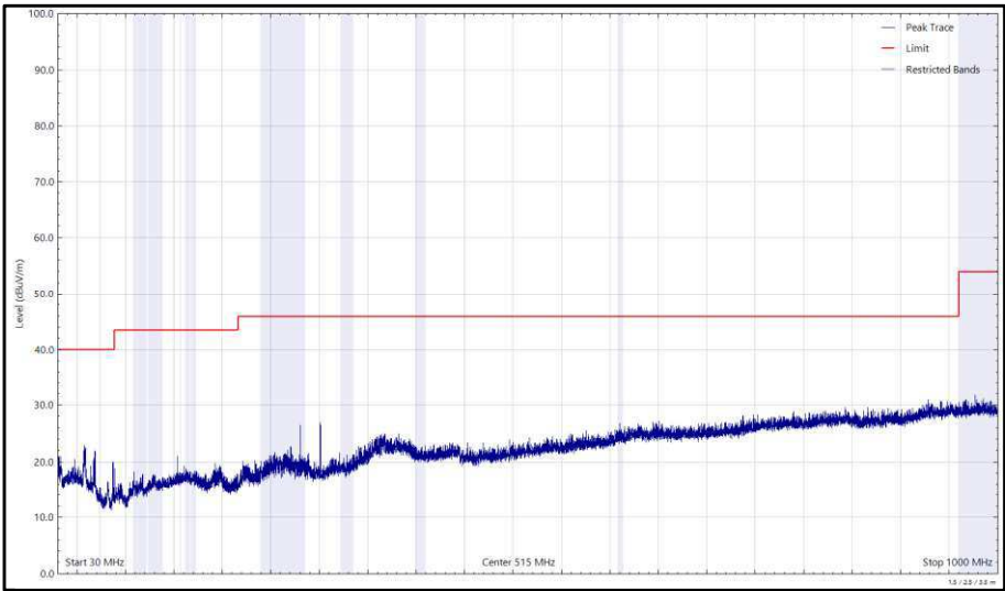
Figure 476 - U-NII-3 - 5825 MHz (CH165), VHT20, CDD, Core 0 + Core 1, 30 MHz to 1 GHz, Horizontal (Peak)
