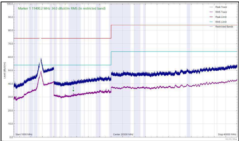
Figure 473 - U-NII-2C - 5700 MHz (CH140), VHT20, CDD, Core 0 + Core 1, 1 GHz to 40 GHz, Vertical
