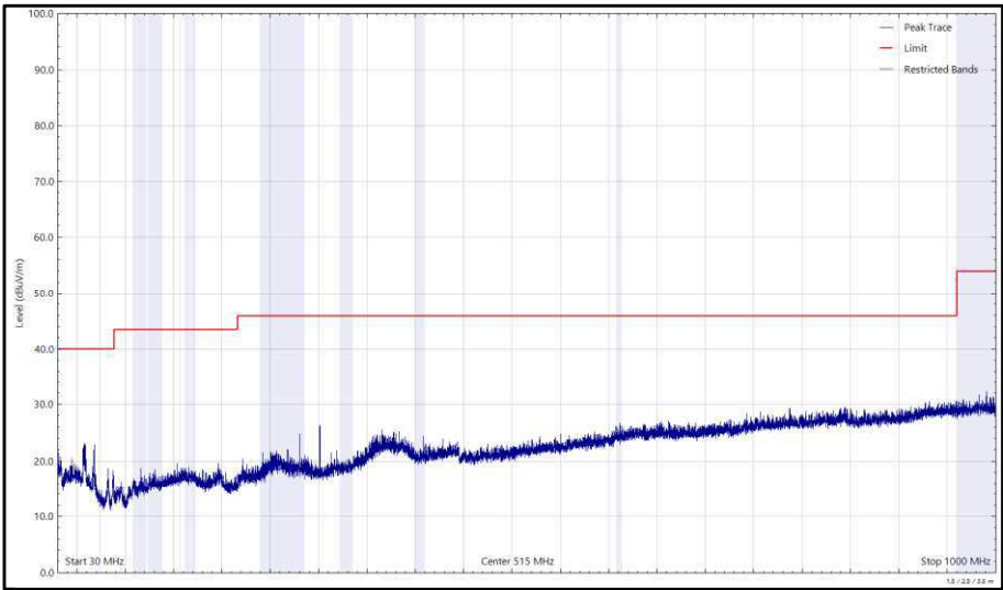
Figure 460 - U-NII-3 - 5825 MHz (CH165), 802.11a, Core 1, 30 MHz to 1 GHz, Horizontal (Peak)
