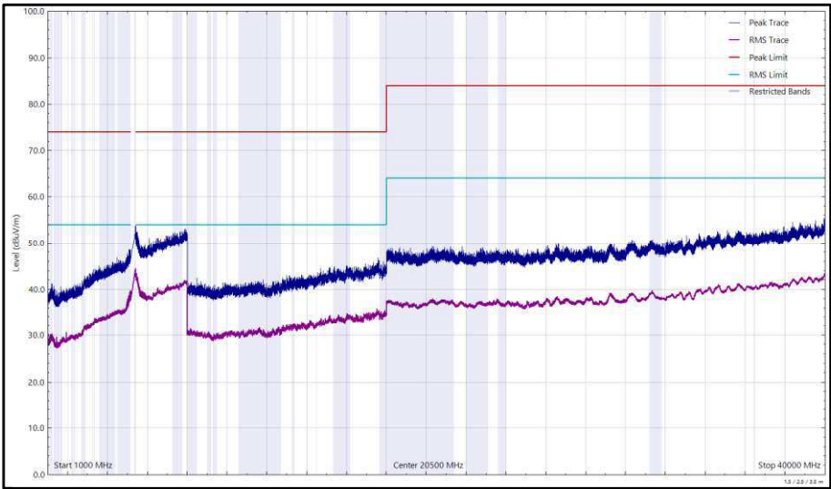
Figure 436 - U-NII-2A - 5320 MHz (CH64), 802.11a, Core 0, 1 GHz to 40 GHz, Horizontal
