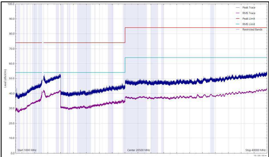
Figure 433 - U-NII-1 - 5180 MHz (CH36), 802.11a, Core 0, 1 GHz to 40 GHz, Horizontal
