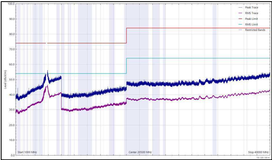
Figure 474 - U-NII-3 - 5745 MHz (CH149), VHT20, CDD, Core 0 + Core 1, 1 GHz to 40 GHz, Horizontal
