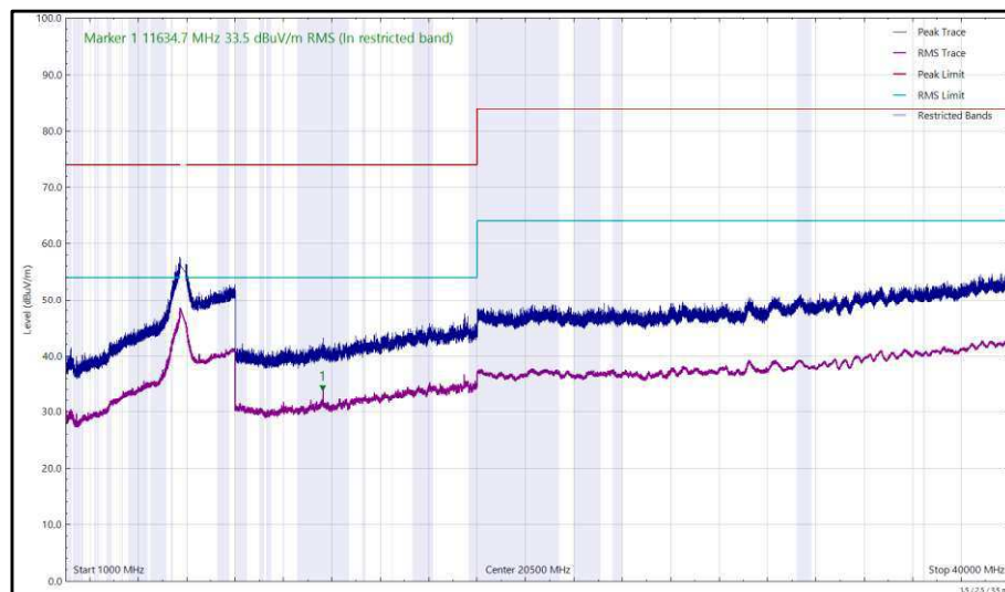
Figure 495 - U-NII-3 - 5825 MHz (CH165), HE20, RU26-0, CDD, Core 0 + Core 1, 1 GHz to 40 GHz, Vertical
