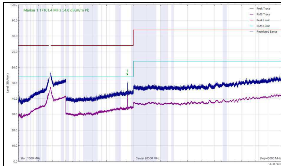
Figure 441 - U-NII-2C - 5700 MHz (CH140), 802.11a, Core 0, 1 GHz to 40 GHz, Vertical
