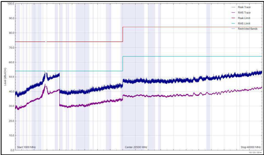
Figure 461 - U-NII-3 - 5825 MHz (CH165), 802.11a, Core 1, 1 GHz to 40 GHz, Horizontal
