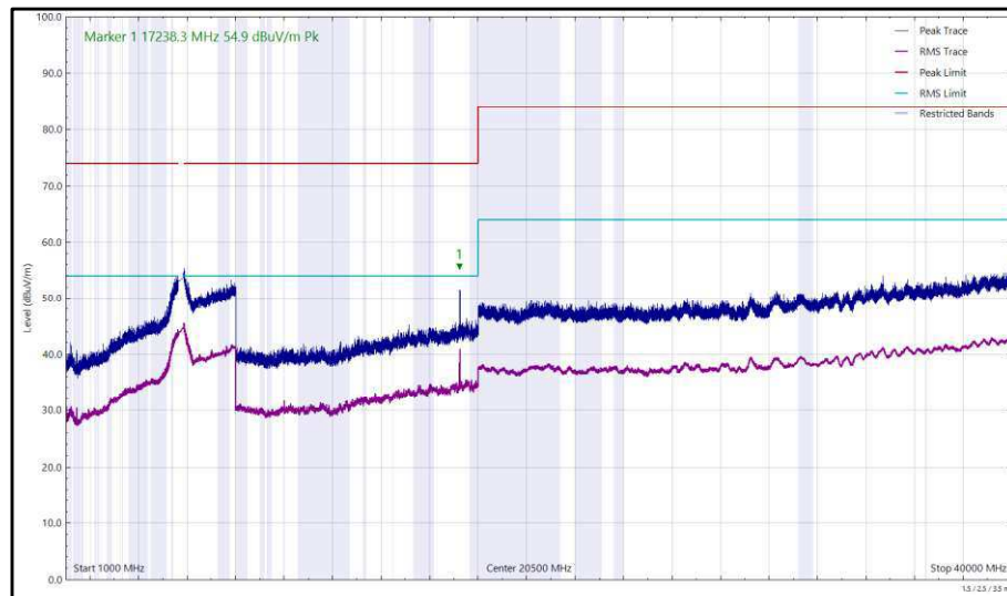
Figure 443 - U-NII-3 - 5745 MHz (CH149), 802.11a, Core 0, 1 GHz to 40 GHz, Vertical
