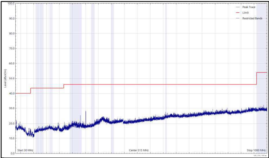
Figure 432 - U-NII-1 - 5180 MHz (CH36), 802.11a, Core 0, 30 MHz to 1 GHz, Horizontal (Peak)
