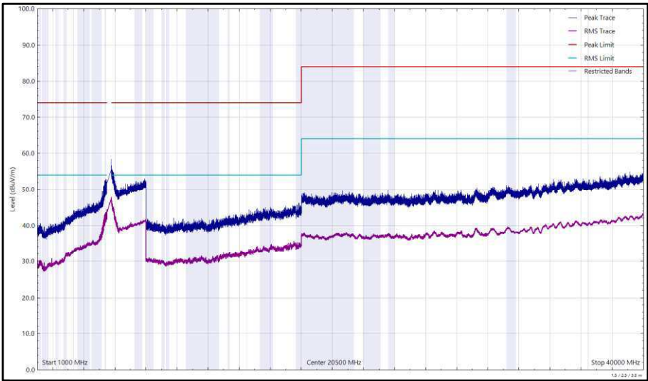
Figure 472 - U-NII-2C - 5700 MHz (CH140), VHT20, CDD, Core 0 + Core 1, 1 GHz to 40 GHz, Horizontal
