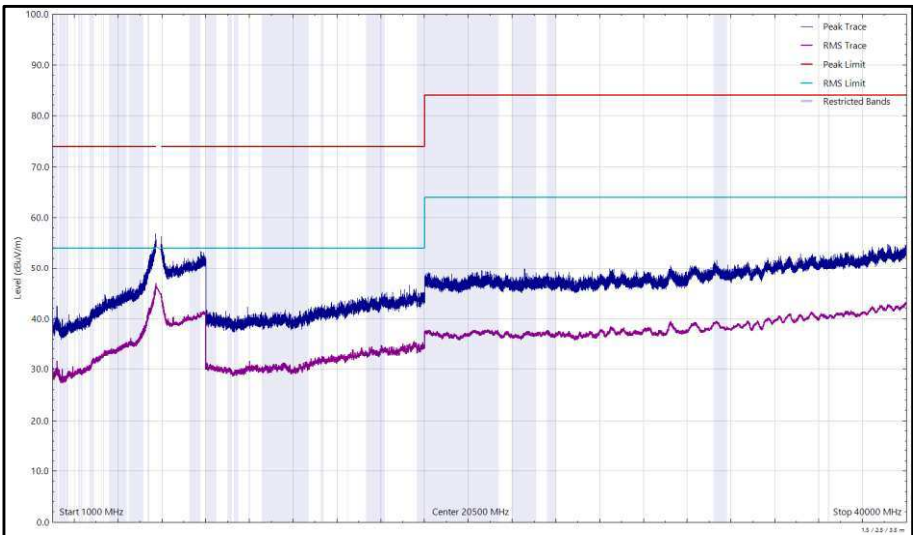
Figure 463 - U-NII-3 - 5825 MHz (CH165), 802.11a, Core 1, 1 GHz to 40 GHz, Vertical
