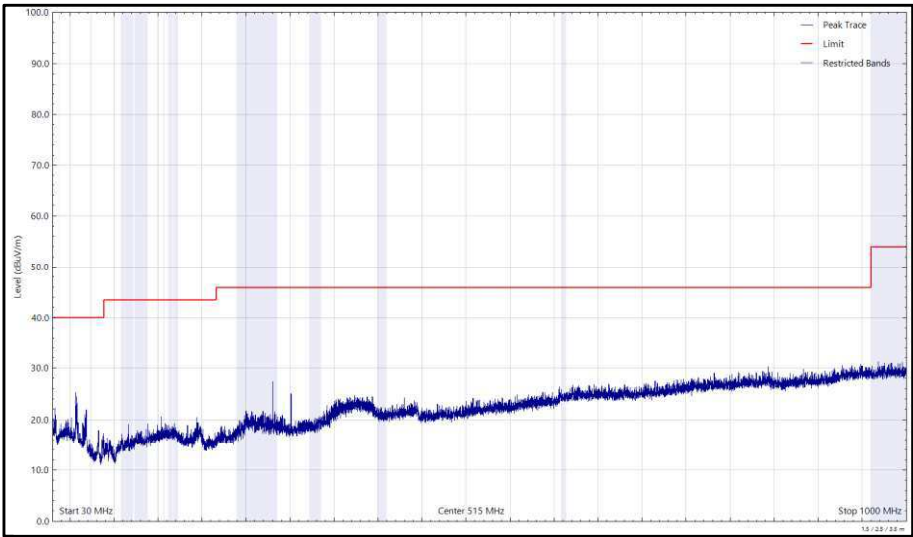
Figure 444 - U-NII-3 - 5825 MHz (CH165), 802.11a, Core 0, 30 MHz to 1 GHz, Horizontal (Peak)
