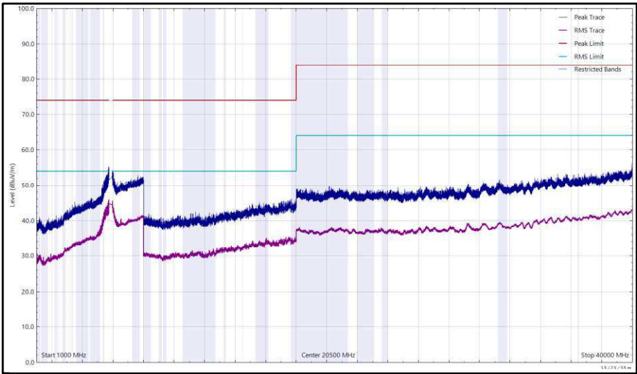
Figure 477 - U-NII-3 - 5825 MHz (CH165), VHT20, CDD, Core 0 + Core 1, 1 GHz to 40 GHz, Horizontal
