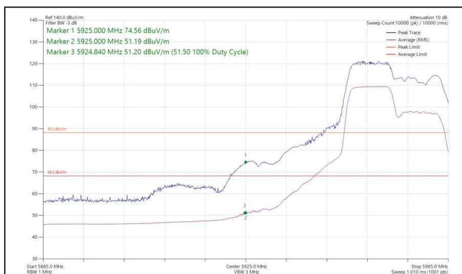
Figure 33 - 802.11ax, HE20, RU 106-53, SISO, Core 0 - 5955 MHz, Band Edge Frequency 5925 MHz
