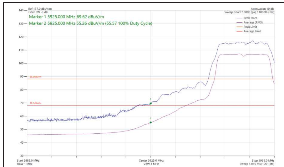
Figure 31 - 802.11a, SISO, Core 0 - 5955 MHz, Band Edge Frequency 5925 MHz
