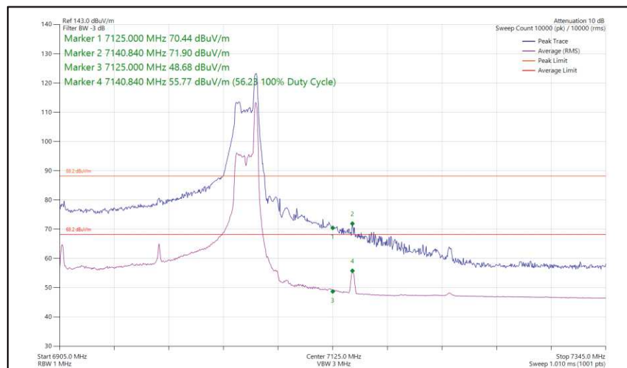
Figure 100 - 802.11ax, HE160, RU 26-36, SISO, Core 1 - 6985 MHz, Band Edge Frequency 7125 MHz
