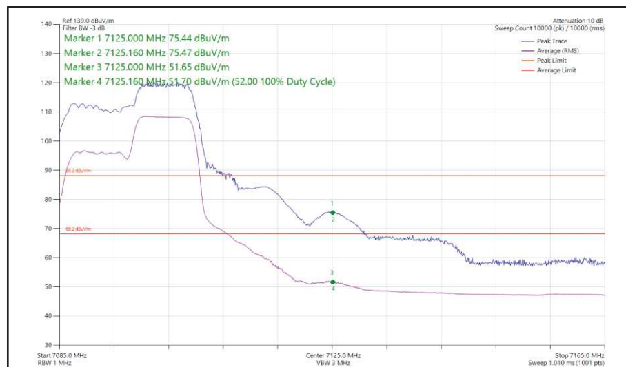
Figure 45 - 802.11ax, HE20, RU 106-54, SISO, Core 1 - 7095 MHz, Band Edge Frequency 7125 MHz
