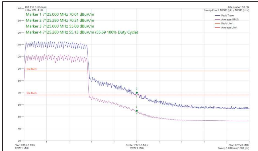
Figure 85 - 802.11ax, HE80, SU, CDD, Core 0-1 - 7025 MHz, Band Edge Frequency 7125 MHz
