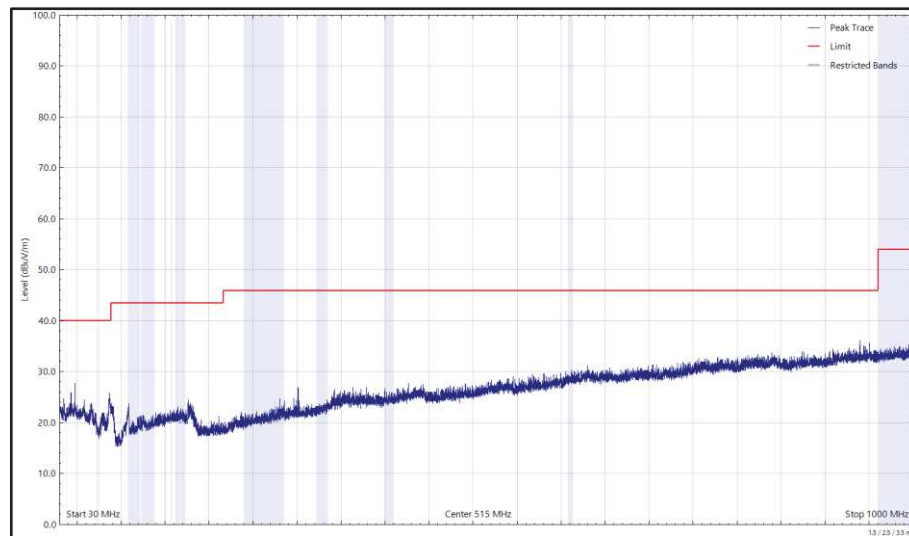
Figure 138 - U-NII-8 - 6995 MHz (CH209), HE20, SU, CDD, Core 0 + Core 1, 30 MHz to 1 GHz, Vertical (Peak)
