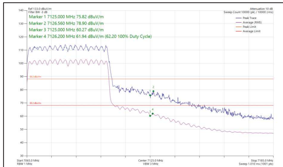
Figure 67 - 802.11ax, HE40, SU, CDD, Core 0-1 - 7085 MHz, Band Edge Frequency 7125 MHz
