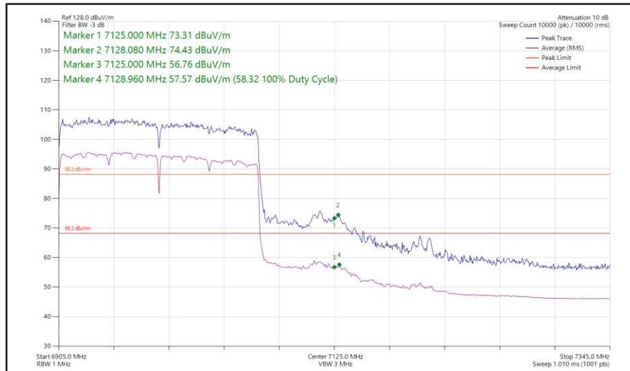
Figure 95 - 802.11ax, HE160, SU, SISO, Core 0 - 6985 MHz, Band Edge Frequency 7125 MHz
