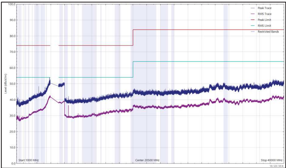
Figure 119 - U-NII-6 - 6435 MHz (CH97), HE20, SU, CDD, Core 0 + Core 1, 1 GHz to 40 GHz, Vertical
