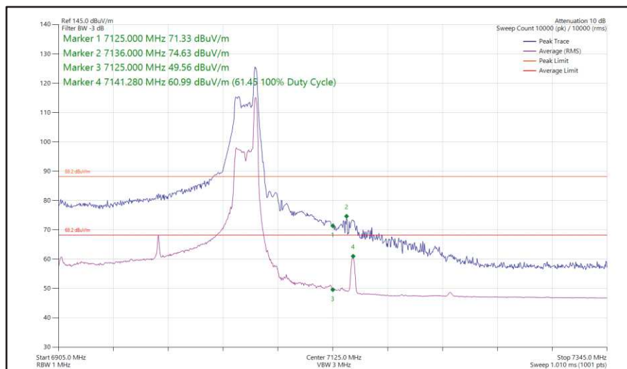
Figure 96 - 802.11ax, HE160, RU 26-36, SISO, Core 0 - 6985 MHz, Band Edge Frequency 7125 MHz
