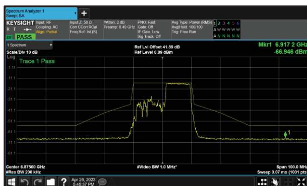
Figure 147 - A (Core 0) 802.11ax HE20 RU106 6875 MHz (CH185)
