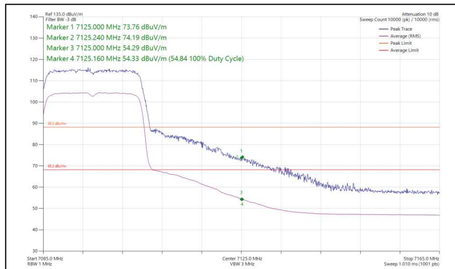
Figure 44 - 802.11ax, HE20, SU, SISO, Core 1 - 7095 MHz, Band Edge Frequency 7125 MHz
