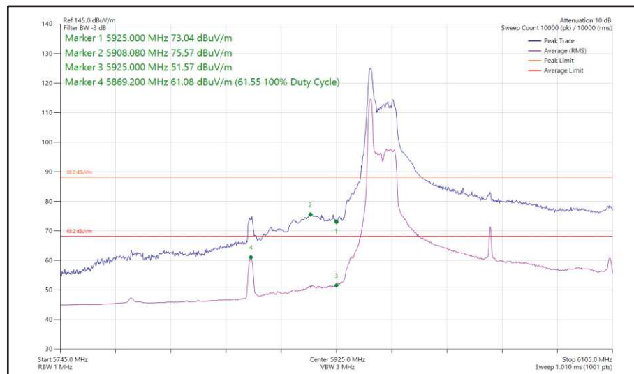
Figure 94 - 802.11ax, HE160, RU 26-0, SISO, Core 0 - 6025 MHz, Band Edge Frequency 5925 MHz
