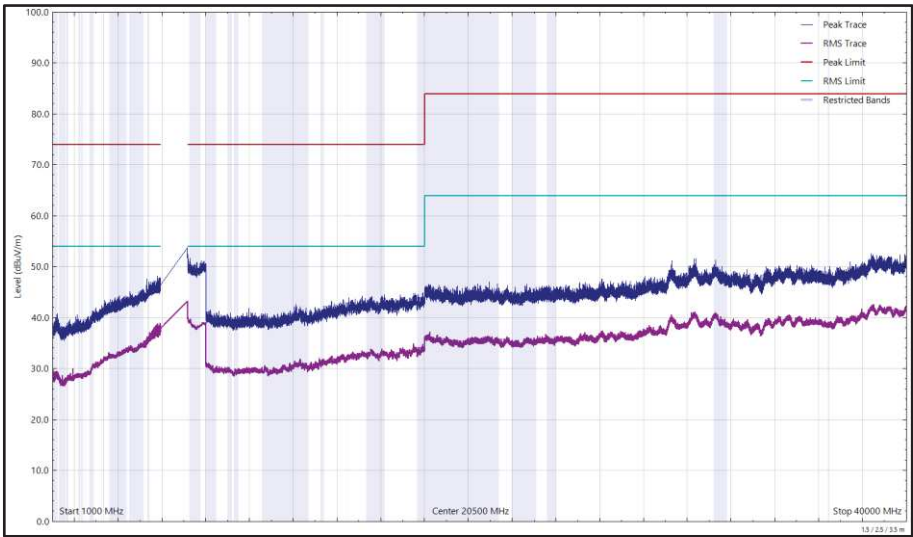
Figure 132 - U-NII-7 - 6855 MHz (CH181), HE20, SU, CDD, Core 0 + Core 1, 1 GHz to 40 GHz, Horizontal
