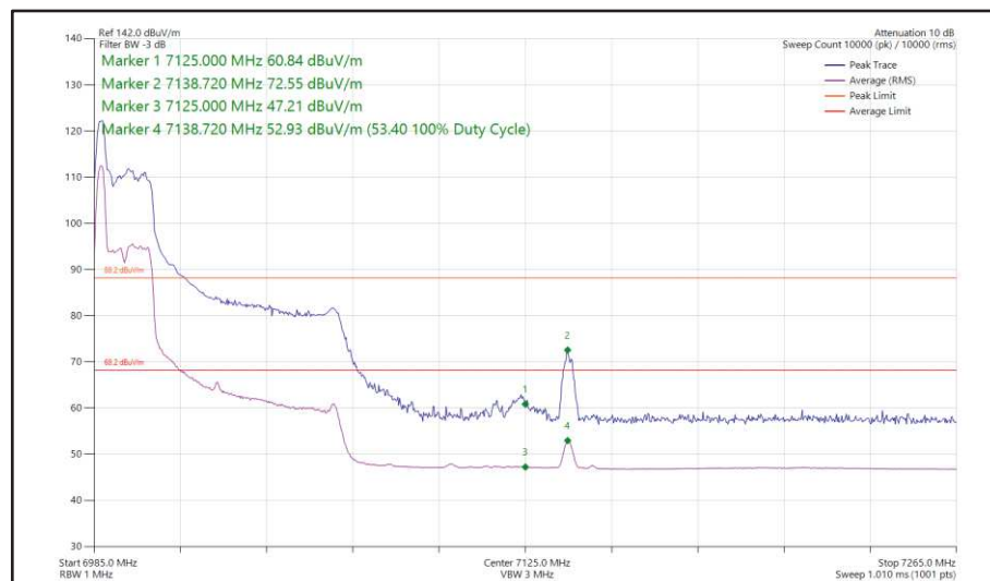
Figure 82 - 802.11ax, HE80, RU 26-0, SISO, Core 1 - 7025 MHz, Band Edge Frequency 7125 MHz
