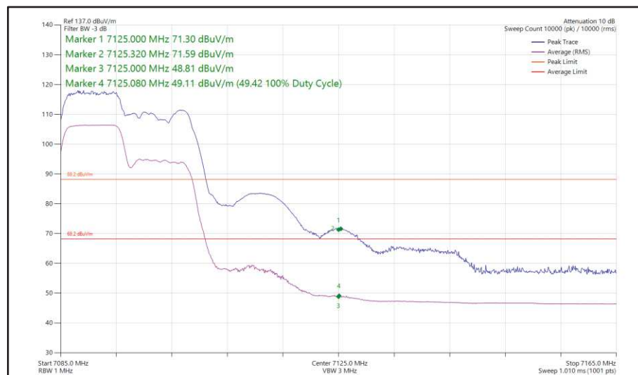
Figure 37 - 802.11ax, HE20, RU 106-53, SISO, Core 0 - 7095 MHz, Band Edge Frequency 7125 MHz
