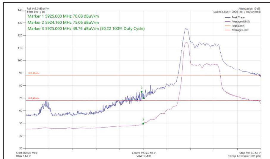
Figure 58 - 802.11ax, HE40, RU 26-0, SISO, Core 0 - 5965 MHz, Band Edge Frequency 5925 MHz
