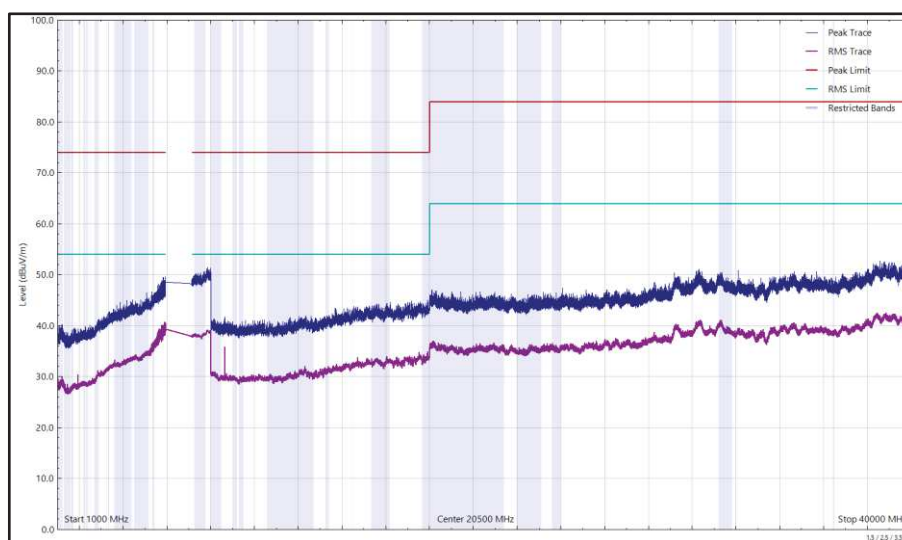
Figure 121 - U-NII-6 - 6475 MHz (CH105), HE20, SU, CDD, Core 0 + Core 1, 1 GHz to 40 GHz, Horizontal
