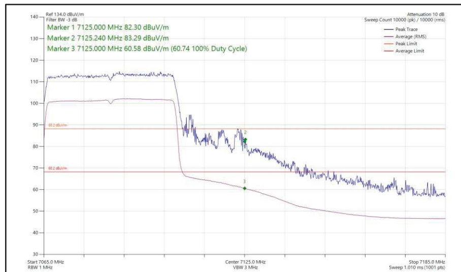
Figure 74 - 802.11ax, HE40, SU, TxBF, Core 0-1 - 7085 MHz, Band Edge Frequency 7125 MHz
