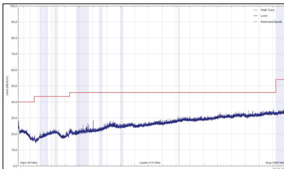
Figure 112 - U-NII-5 - 6175 MHz (CH45), HE20, SU, CDD, Core 0 + Core 1, 30 MHz to 1 GHz, Horizontal (Peak)
