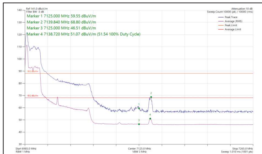
Figure 78 - 802.11ax, HE80, RU 26-0, SISO, Core 0 - 7025 MHz, Band Edge Frequency 7125 MHz
