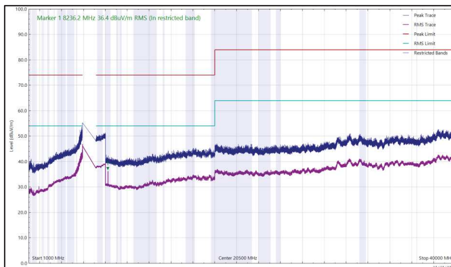
Figure 113 - U-NII-5 - 6175 MHz (CH45), HE20, SU, CDD, Core 0 + Core 1, 1 GHz to 40 GHz, Horizontal
