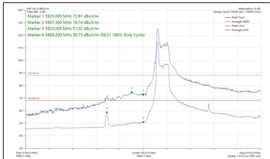
Figure 98 - 802.11ax, HE160, RU 26-0, SISO, Core 1 - 6025 MHz, Band Edge Frequency 5925 MHz
