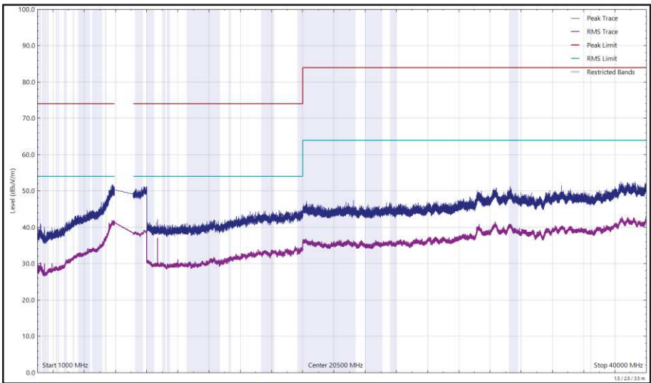
Figure 125 - U-NII-6 - 6515 MHz (CH113), HE20, SU, CDD, Core 0 + Core 1, 1 GHz to 40 GHz, Vertical
