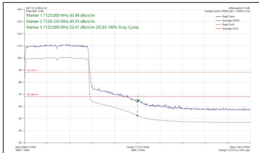
Figure 77 - 802.11ax, HE80, SU, SISO, Core 0 - 7025 MHz, Band Edge Frequency 7125 MHz
