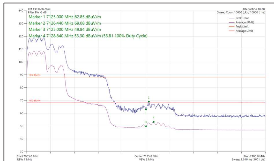
Figure 68 - 802.11ax, HE40, RU 103-53, CDD, Core 0-1 - 7085 MHz, Band Edge Frequency 7125 MHz
