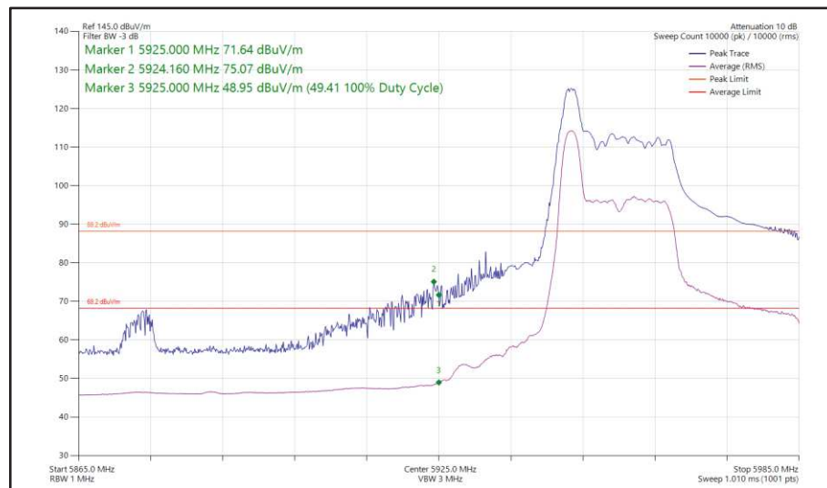
Figure 62 - 802.11ax, HE40, RU 26-0, SISO, Core 1 - 5965 MHz, Band Edge Frequency 5925 MHz
