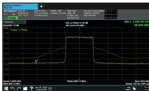
Figure 145 - A (Core 0) 802.11ax HE80 SU 5985 MHz (CH7)
