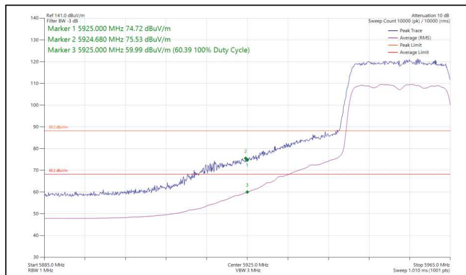
Figure 52 - 802.11ax, HE20, SU, SDM, Core 0-1 - 5955 MHz, Band Edge Frequency 5925 MHz
