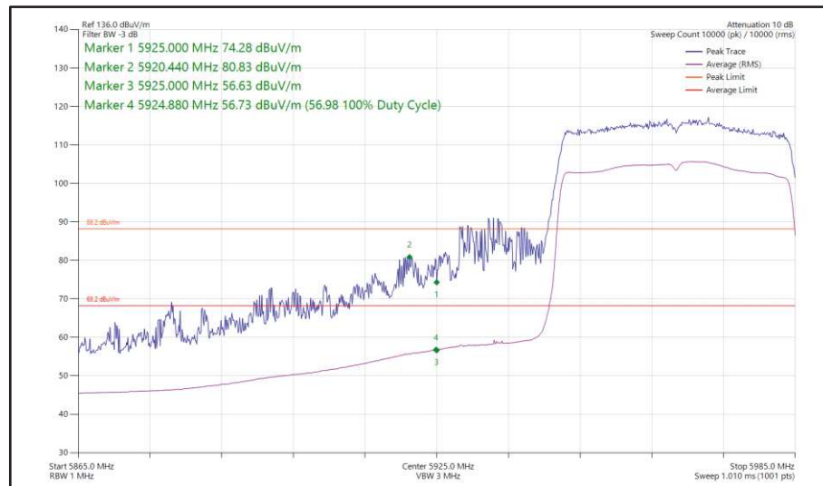
Figure 73 - 802.11ax, HE40, SU, TxBF, Core 0-1 - 5965 MHz, Band Edge Frequency 5925 MHz
