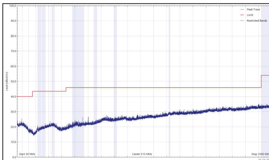
Figure 136 - U-NII-8 - 6995 MHz (CH209), HE20, SU, CDD, Core 0 + Core 1, 30 MHz to 1 GHz, Horizontal (Peak)
