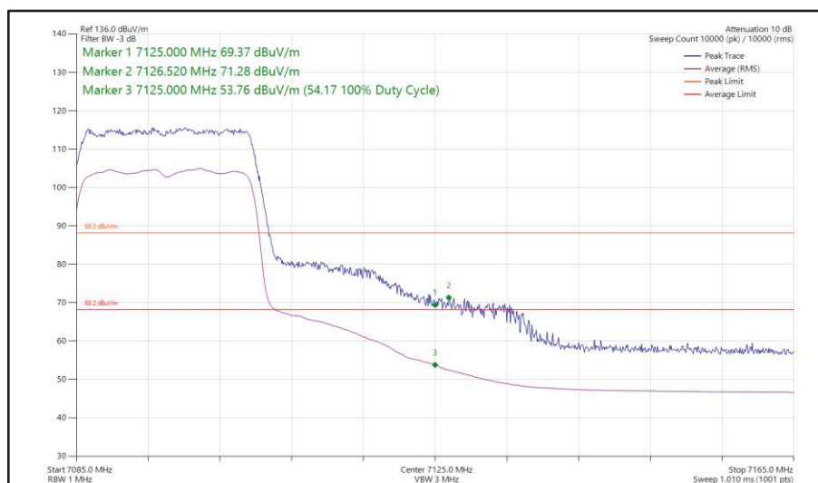
Figure 54 - 802.11ax, HE20, SU, SDM, Core 0-1 - 7095 MHz, Band Edge Frequency 7125 MHz
