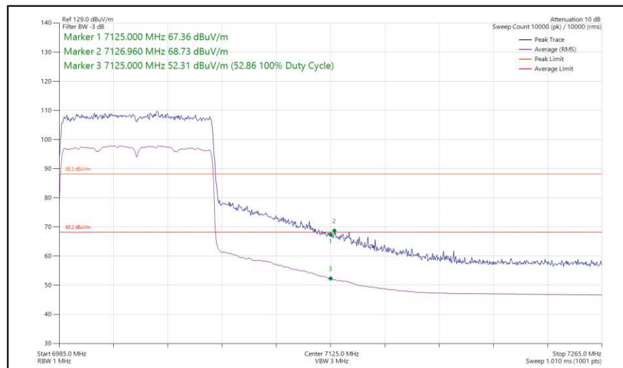
Figure 81 - 802.11ax, HE80, SU, SISO, Core 1 - 7025 MHz, Band Edge Frequency 7125 MHz
