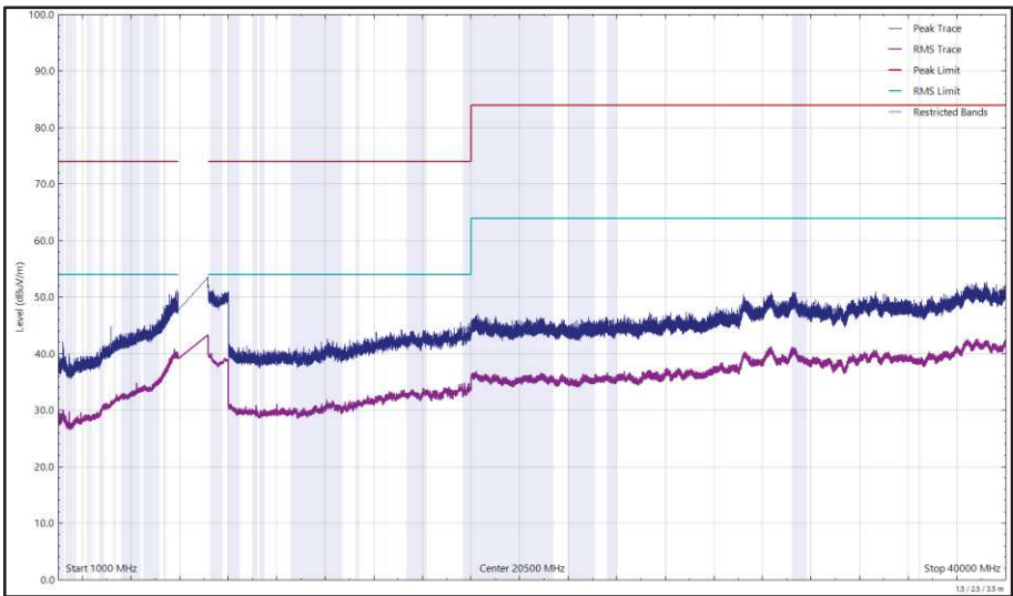
Figure 133 - U-NII-7 - 6855 MHz (CH181), HE20, SU, CDD, Core 0 + Core 1, 1 GHz to 40 GHz, Vertical
