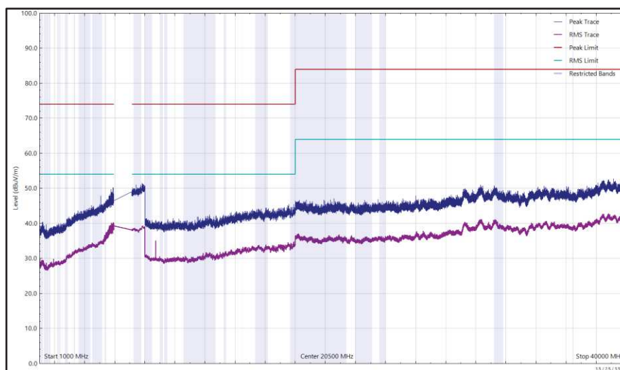
Figure 126 - U-NII-7 - 6535 MHz (CH117), HE20, SU, CDD, Core 0 + Core 1, 1 GHz to 40 GHz, Horizontal
