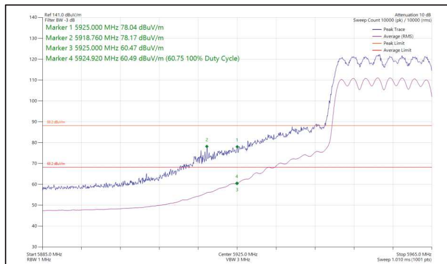
Figure 47 - 802.11ax, HE20, SU, CDD, Core 0-1 - 5955 MHz, Band Edge Frequency 5925 MHz
