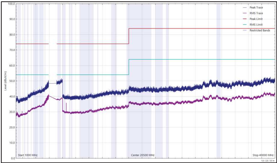
Figure 118 - U-NII-6 - 6435 MHz (CH97), HE20, SU, CDD, Core 0 + Core 1, 1 GHz to 40 GHz, Horizontal
