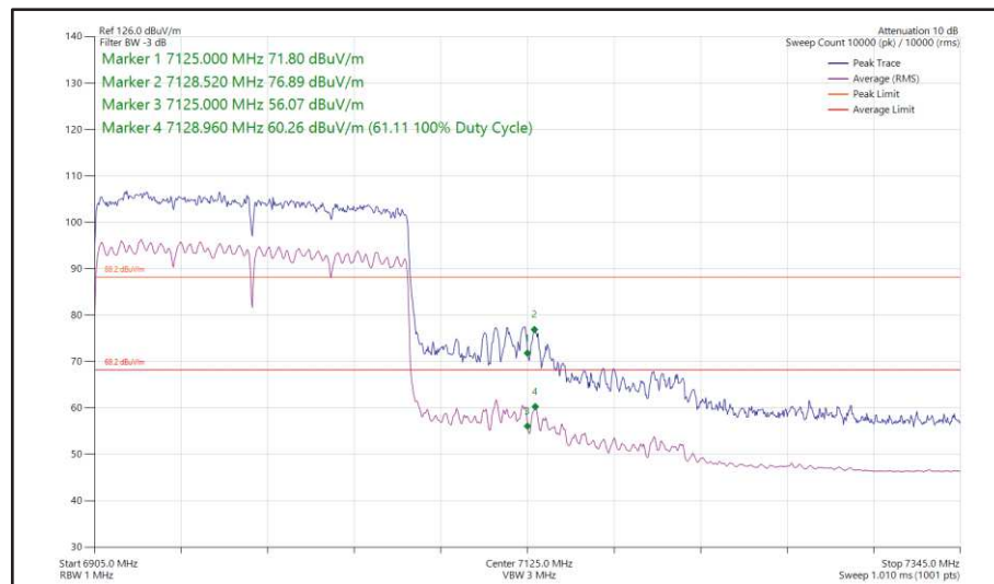
Figure 107 - 802.11ax, HE160, SU, SDM, Core 0-1 - 6985 MHz, Band Edge Frequency 7125 MHz
