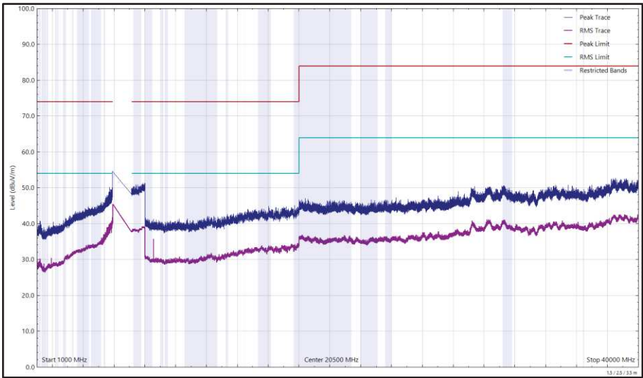
Figure 116 - U-NII-5 - 6415 MHz (CH93), HE20, SU, CDD, Core 0 + Core 1, 1 GHz to 40 GHz, Horizontal
