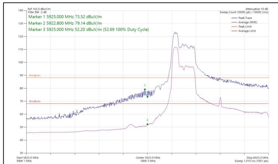
Figure 76 - 802.11ax, HE80, RU 52-37, SISO, Core 0 - 5985 MHz, Band Edge Frequency 5925 MHz
