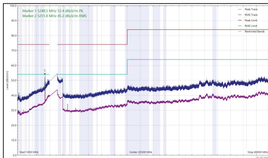
Figure 139 - U-NII-8 - 6995 MHz (CH209), HE20, SU, CDD, Core 0 + Core 1, 1 GHz to 40 GHz, Vertical
