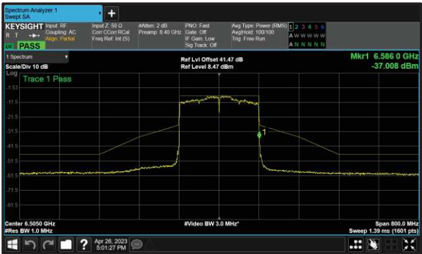
Figure 146 - A (Core 0) 802.11ax HE160 SU 6505 MHz (CH111)
