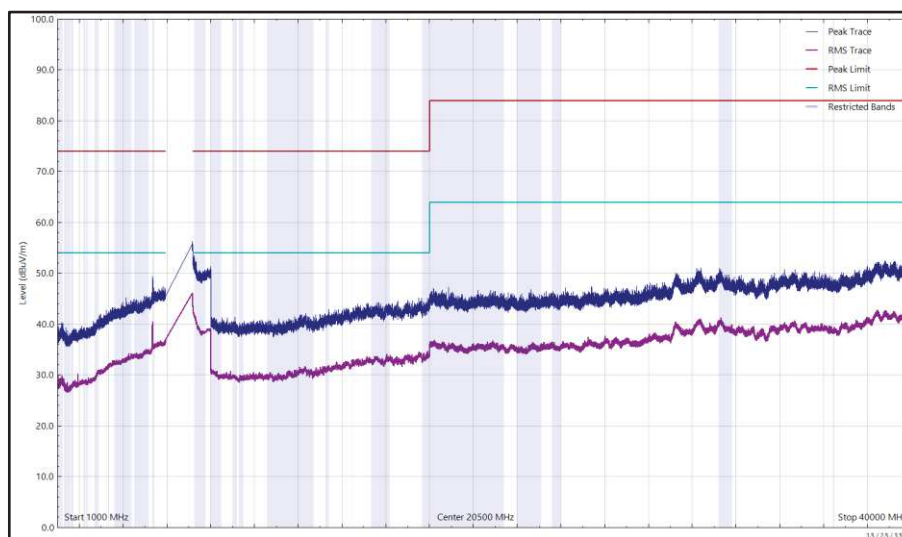
Figure 140 - U-NII-8 - 7115 MHz (CH233), HE20, SU, CDD, Core 0 + Core 1, 1 GHz to 40 GHz, Horizontal
