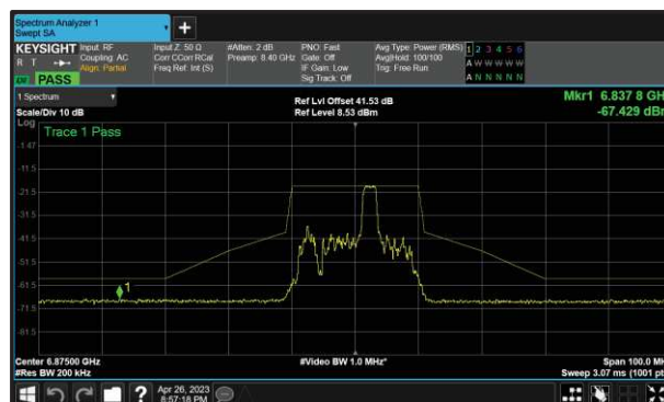
Figure 161 - B (Core 1) 802.11ax HE20 RU26 6875 MHz (CH185)
