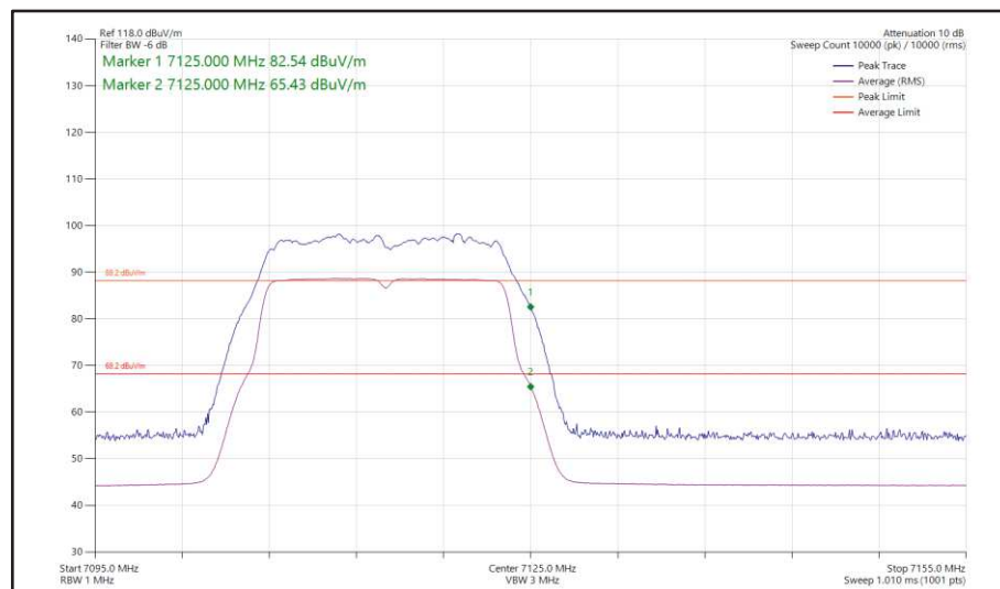
Figure 43 - 802.11a, SISO, Core 1 - 7115 MHz, Band Edge Frequency 7125 MHz
