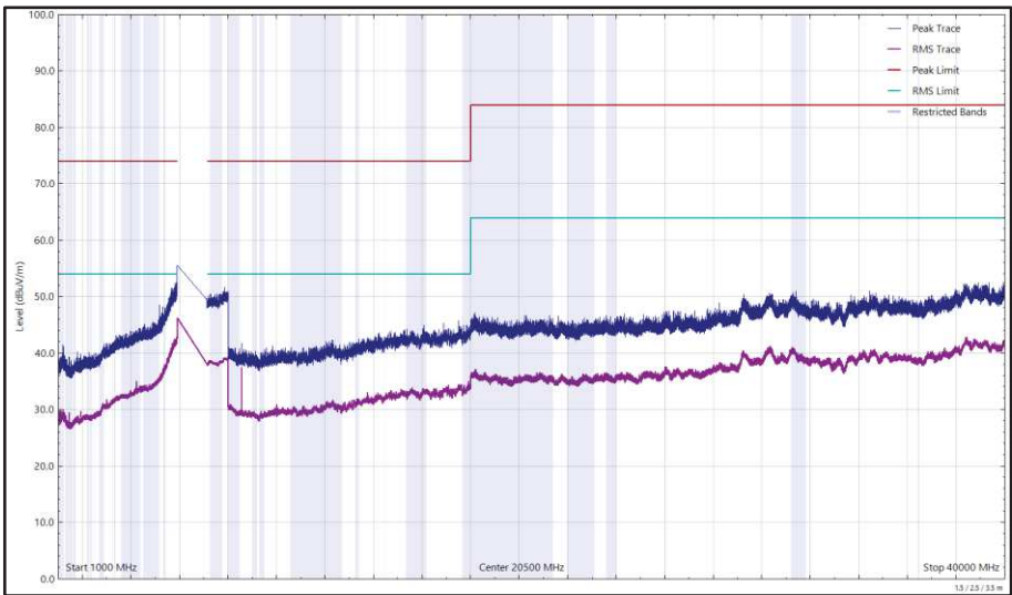
Figure 117 - U-NII-5 - 6415 MHz (CH93), HE20, SU, CDD, Core 0 + Core 1, 1 GHz to 40 GHz, Vertical
