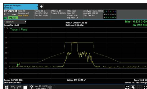
Figure 155 - A (Core 0) 802.11ax HE20 RU52 6875 MHz (CH185)
