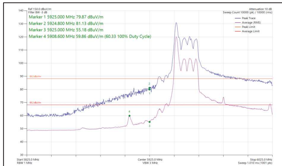
Figure 88 - 802.11ax, HE80, RU 26-0, SDM, Core 0-1 - 5985 MHz, Band Edge Frequency 5925 MHz
