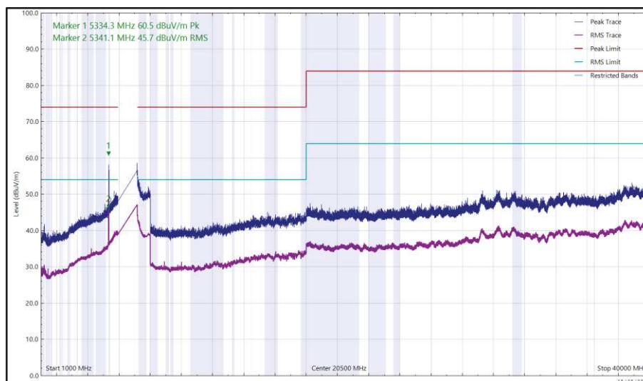
Figure 141 - U-NII-8 - 7115 MHz (CH233), HE20, SU, CDD, Core 0 + Core 1, 1 GHz to 40 GHz, Vertical
