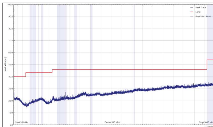
Figure 120 - U-NII-6 - 6475 MHz (CH105), HE20, SU, CDD, Core 0 + Core 1, 30 MHz to 1 GHz, Horizontal (Peak)
