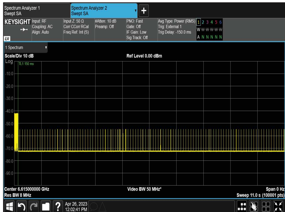
Figure 176 - U-NII-7, Minimum Bandwidth (AWGN Low)
