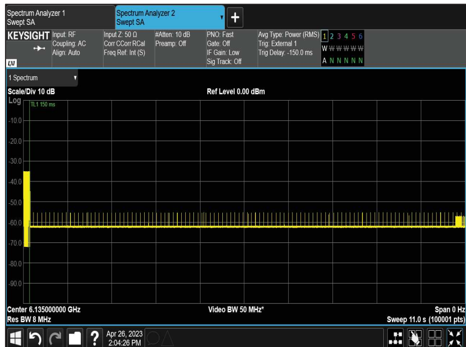
Figure 167 - U-NII-5, Minimum Bandwidth
