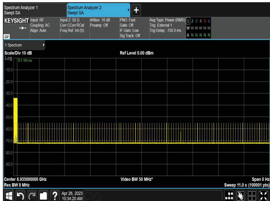
Figure 180 - U-NII-8, Minimum Bandwidth (AWGN Low)
