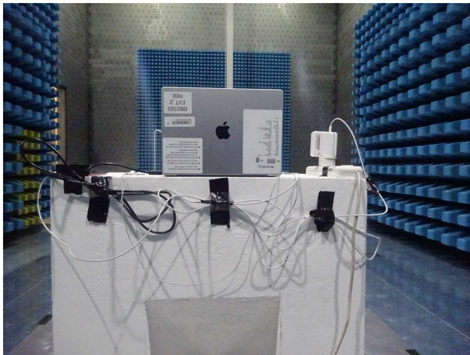
Figure 2 Radiated Disturbance - Above 1 GHz
