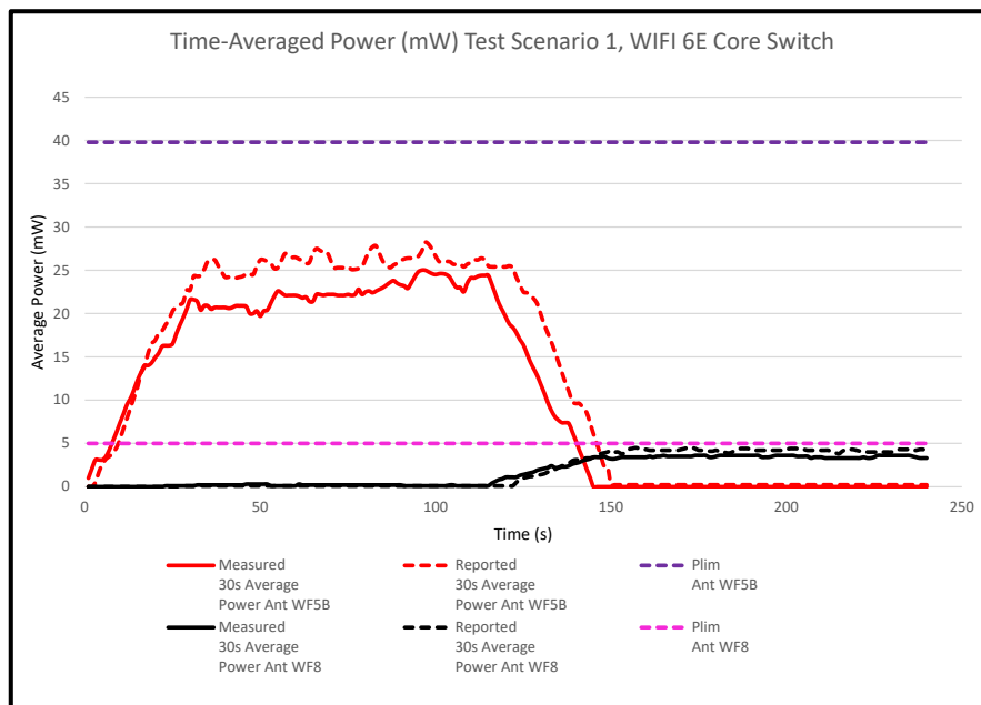
Figure H-6 30s Average Power vs. Time, 6 GHz
