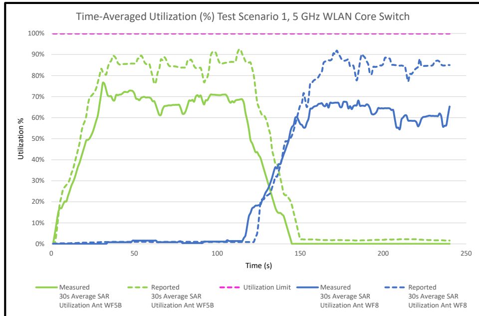
Figure H-3 30s Average SAR Utilization vs. Time, 5 GHz
