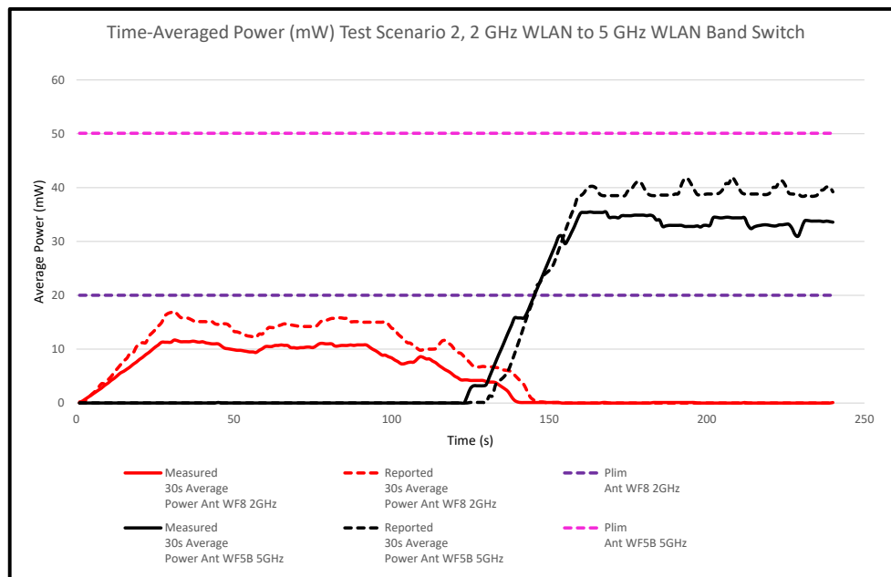
Figure H-8 30s Average Power vs. Time during Band Switch
