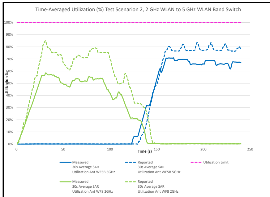
Figure H-7 30s Average Utilization vs. Time during Band Switch
