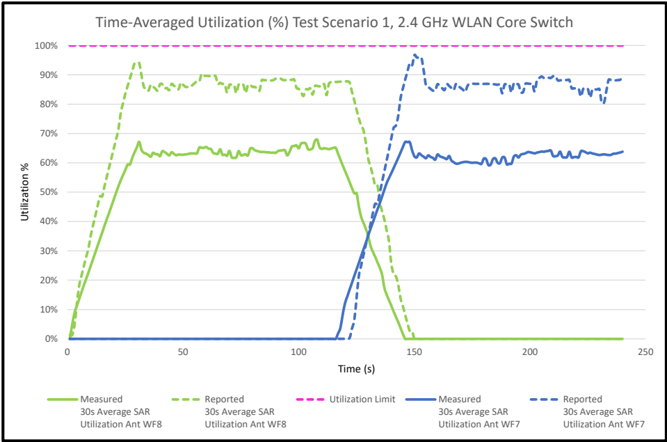
Figure H-1 30s Average SAR Utilization vs. Time, 2.4 GHz
