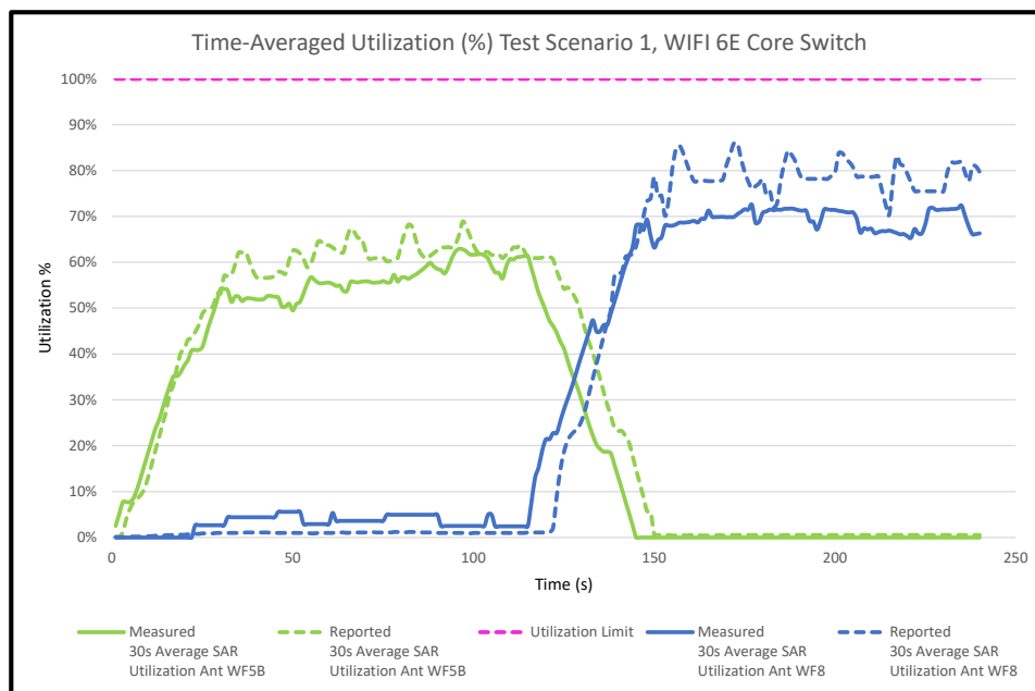
Figure H-5 30s Average SAR Utilization vs. Time, 6 GHz
