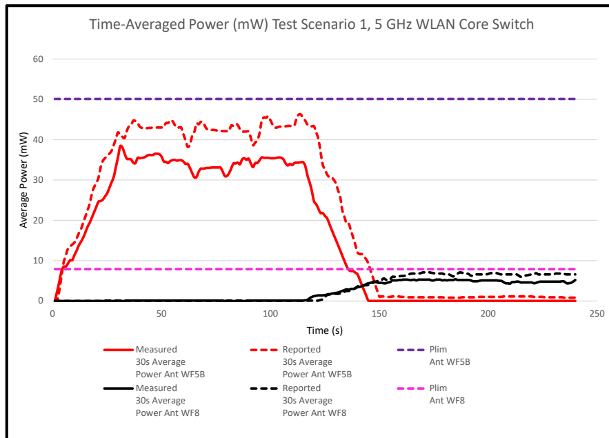
Figure H-4 30s Average Power vs. Time, 5 GHz
