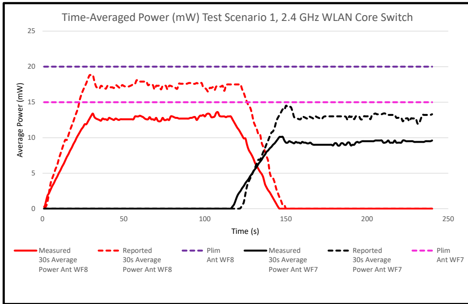
Figure H-2 30s Average Power vs. Time, 2.4 GHz
