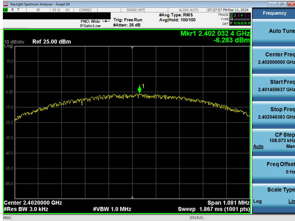
Plot 7-34. Power Spectral Density Plot Antenna WF7 (Bluetooth (LE), 1Mbps, iPA – Ch. 0)
