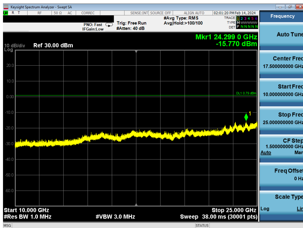
Plot 7-102. Conducted Spurious Plot Antenna WF7 (Bluetooth (LE), 1Mbps, ePA – Ch. 39)
