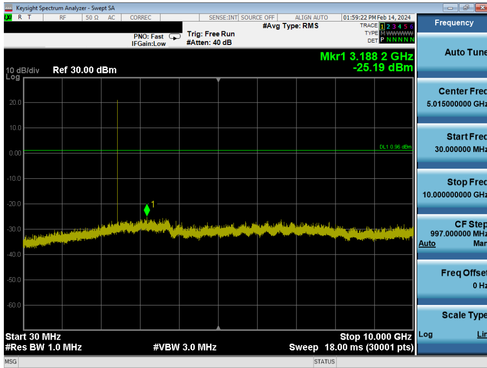
Plot 7-105. Conducted Spurious Plot Antenna WF9 (Bluetooth (LE), 1Mbps, ePA – Ch. 19)
