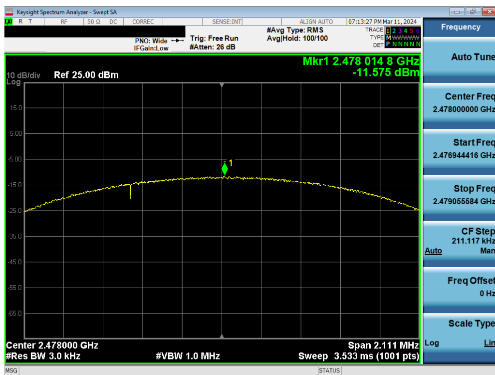
Plot 7-77. Power Spectral Density Plot Antenna WF8 (Bluetooth (LE), 2Mbps, iPA – Ch. 38)
