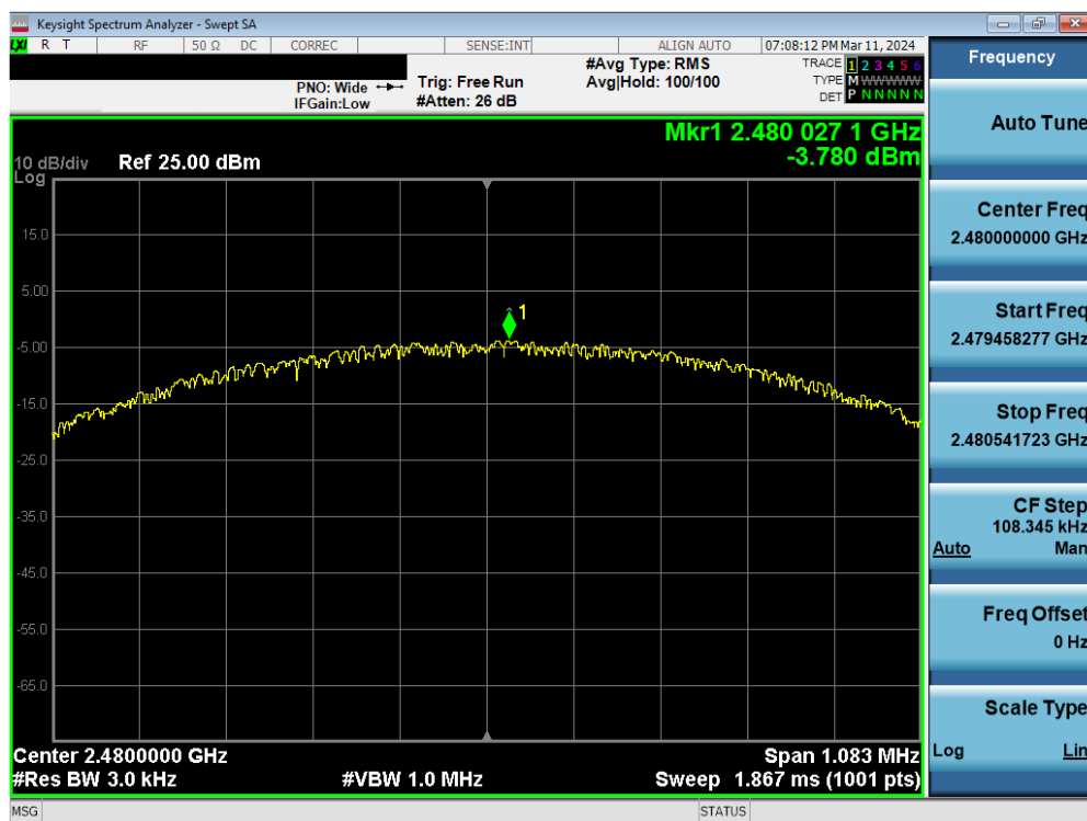
Plot 7-59. Power Spectral Density Plot Antenna WF8 (Bluetooth (LE), 1Mbps, ePA – Ch. 39)
