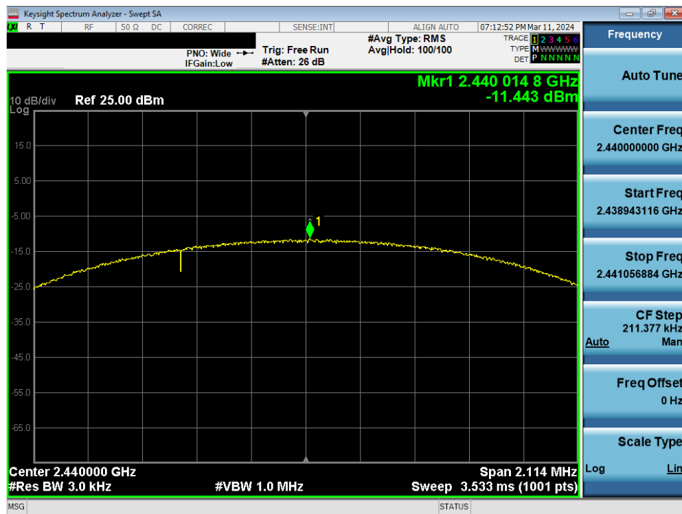
Plot 7-75. Power Spectral Density Plot Antenna WF8 (Bluetooth (LE), 2Mbps, iPA – Ch. 19)
