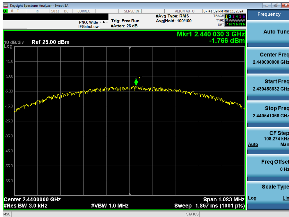
Plot 7-44. Power Spectral Density Plot Antenna WF9 (Bluetooth (LE), 1Mbps, ePA – Ch. 19)
