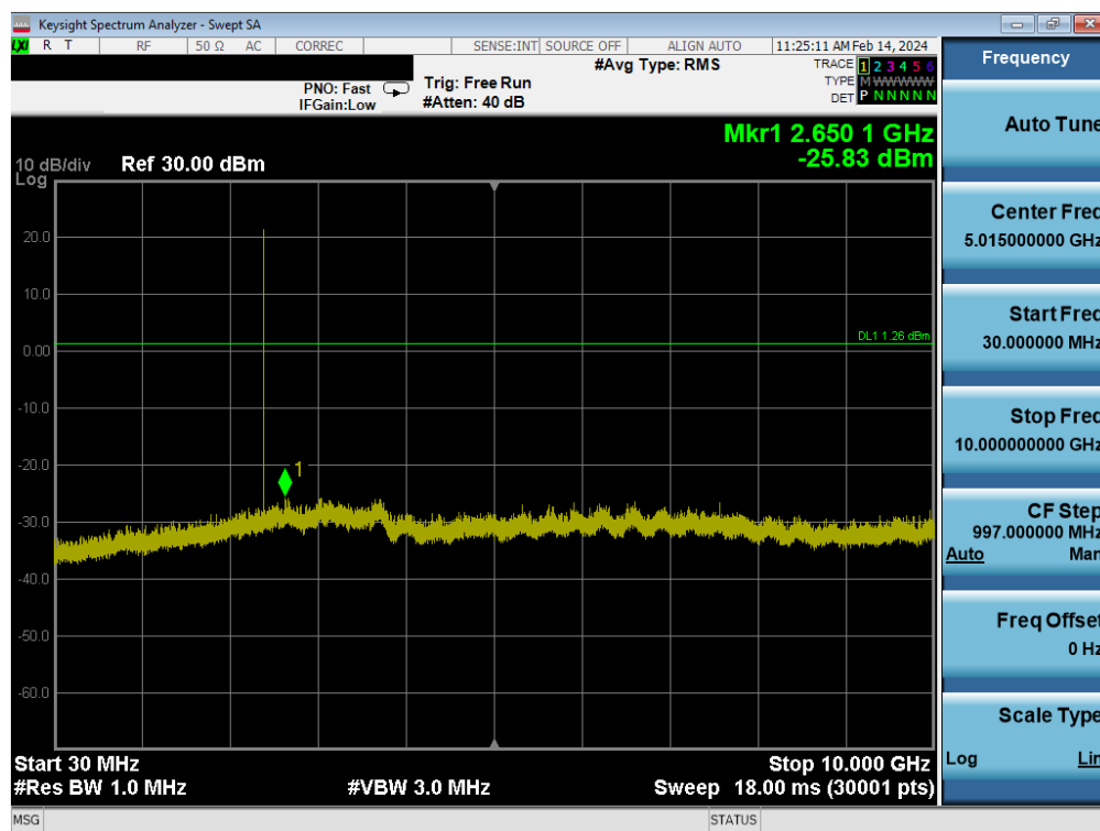
Plot 7-91. Conducted Spurious Plot Antenna WF8 (Bluetooth (LE), 1Mbps, ePA – Ch. 0)
