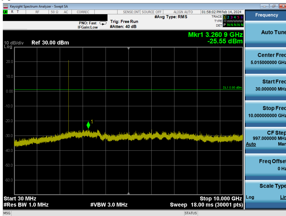
Plot 7-103. Conducted Spurious Plot Antenna WF9 (Bluetooth (LE), 1Mbps, ePA – Ch. 0)
