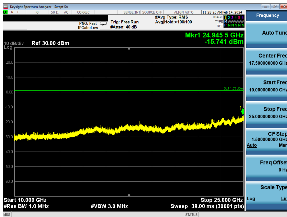
Plot 7-96. Conducted Spurious Plot Antenna WF8 (Bluetooth (LE), 1Mbps, ePA – Ch. 39)
