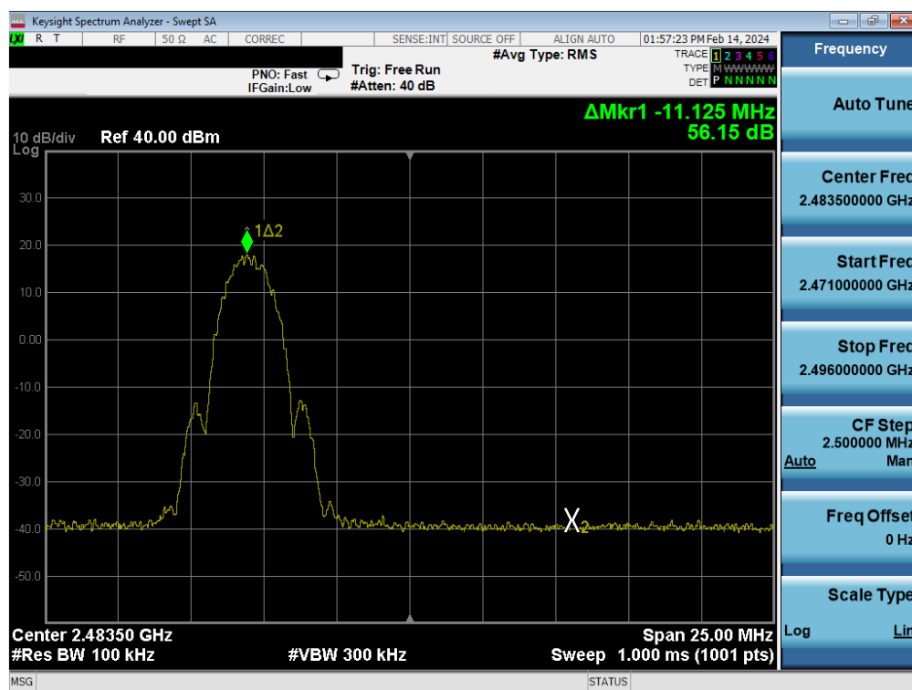
Plot 7-86. Band Edge Plot Antenna WF7 (Bluetooth (LE), 2Mbps, ePA – Ch. 38)
