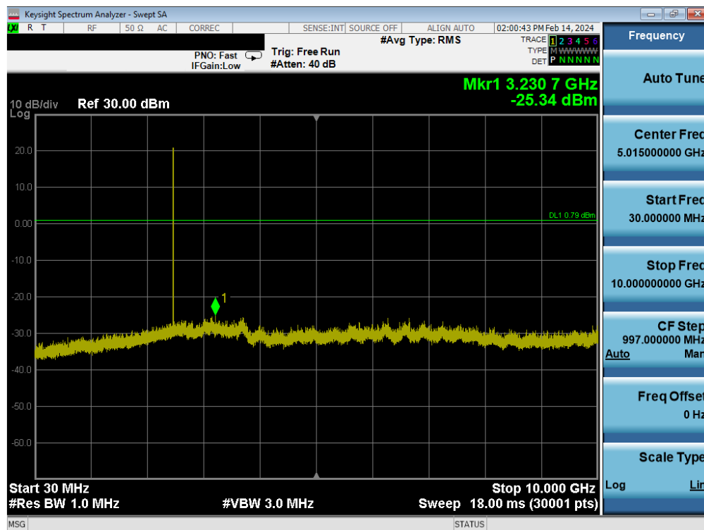
Plot 7-101. Conducted Spurious Plot Antenna WF7 (Bluetooth (LE), 1Mbps, ePA – Ch. 39)
