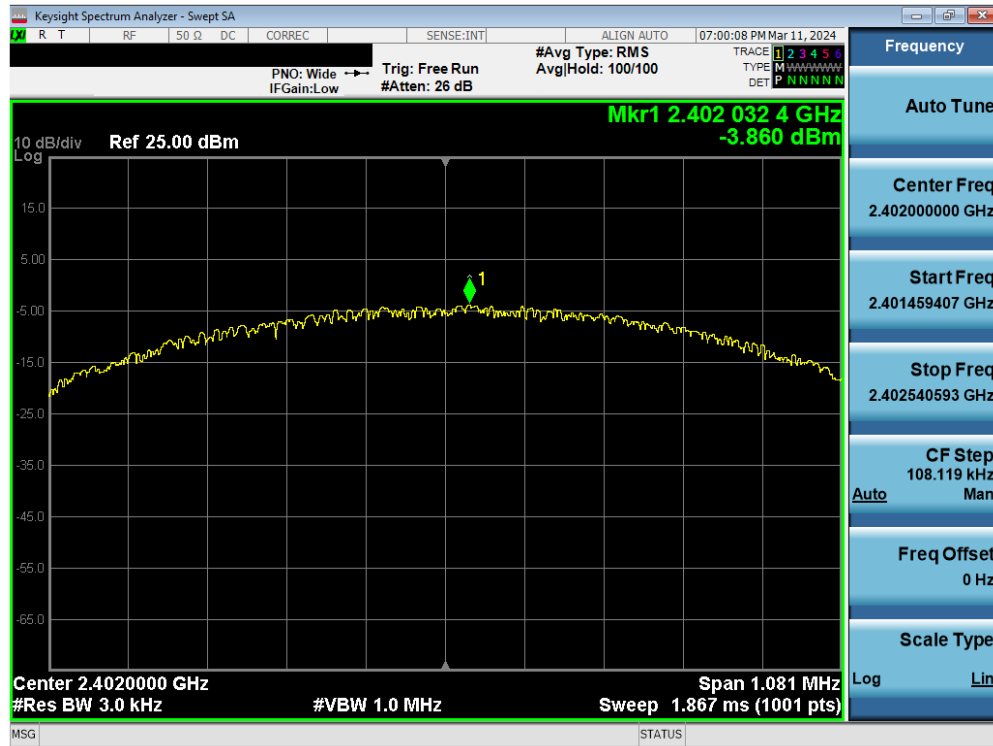
Plot 7-19. Power Spectral Density Plot Antenna WF8 (Bluetooth (LE), 1Mbps, ePA – Ch. 0)
