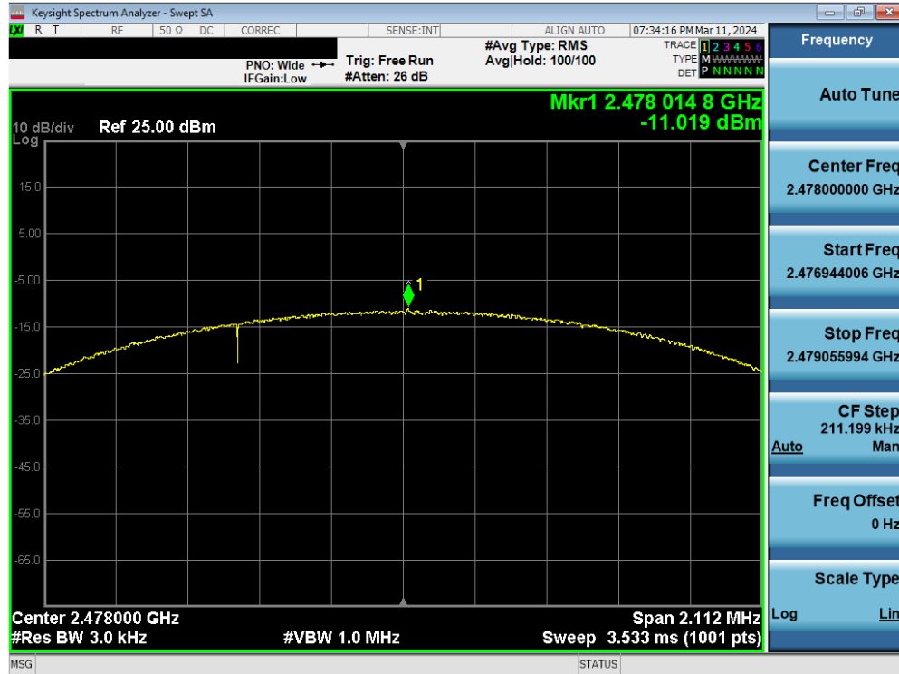
Plot 7-72. Power Spectral Density Plot Antenna WF7 (Bluetooth (LE), 2Mbps, ePA – Ch. 38)
