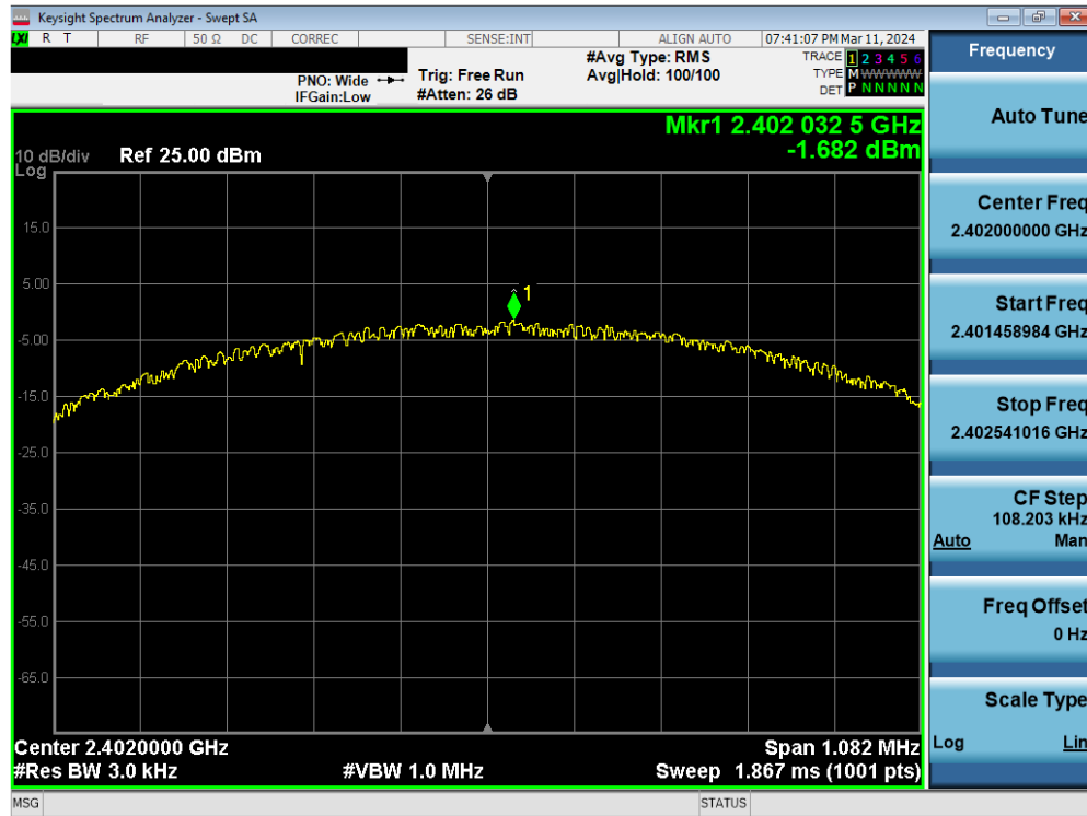
Plot 7-43. Power Spectral Density Plot Antenna WF9 (Bluetooth (LE), 1Mbps, ePA – Ch. 0)
