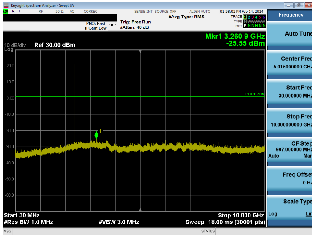
Plot 7-97. Conducted Spurious Plot Antenna WF7 (Bluetooth (LE), 1Mbps, ePA – Ch. 0)
