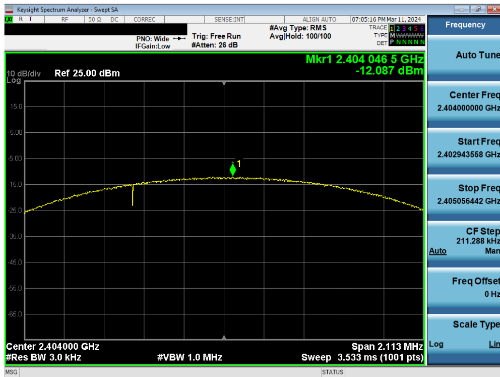
Plot 7-28. Power Spectral Density Plot Antenna WF8 (Bluetooth (LE), 2Mbps, iPA – Ch. 1)
