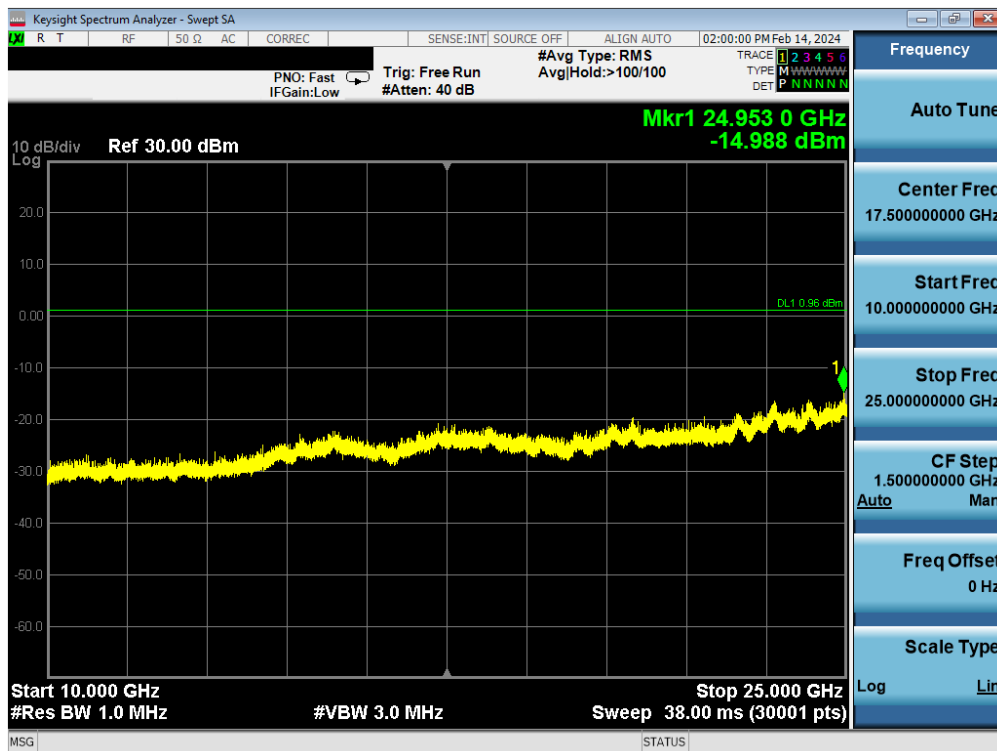
Plot 7-106. Conducted Spurious Plot Antenna WF9 (Bluetooth (LE), 1Mbps, ePA – Ch. 19)
