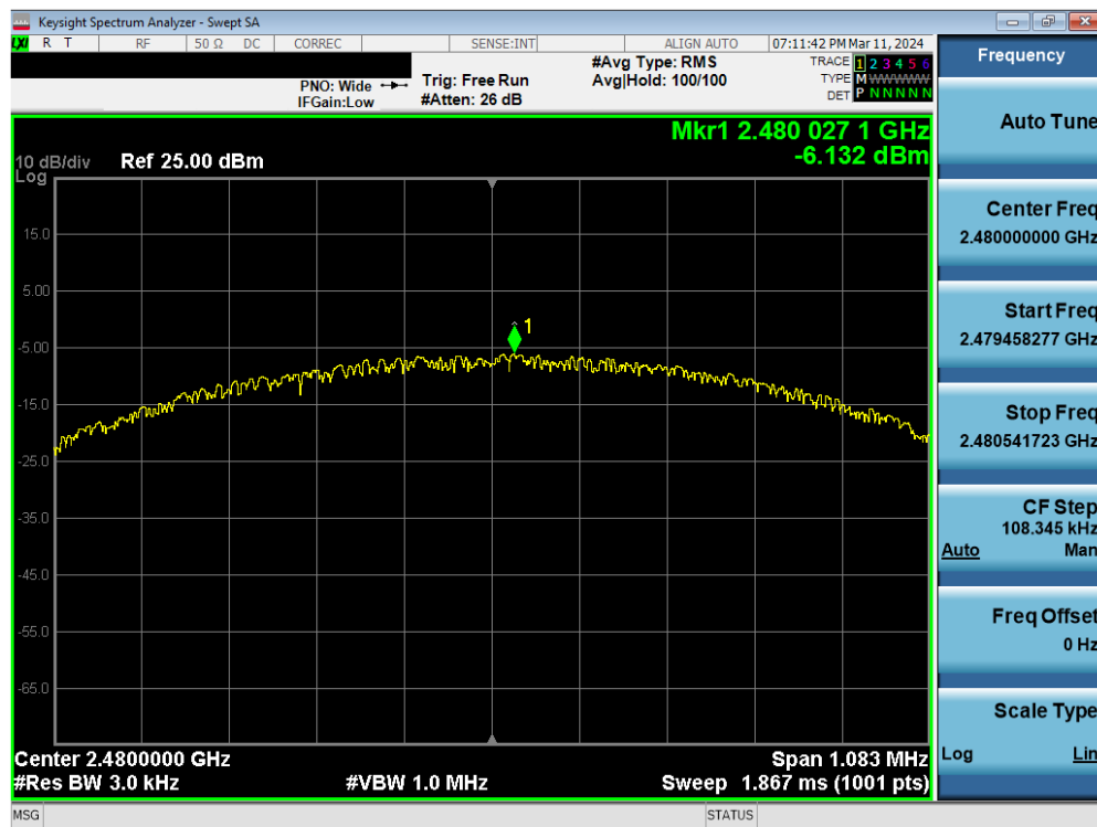
Plot 7-65. Power Spectral Density Plot Antenna WF8 (Bluetooth (LE), 1Mbps, iPA – Ch. 39)
