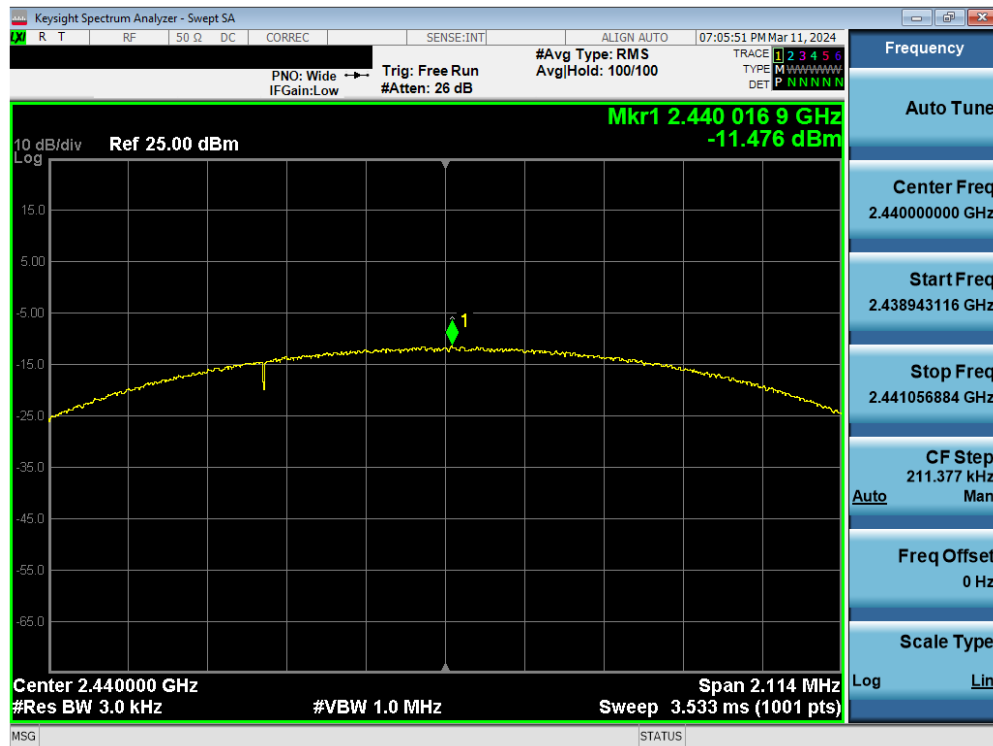
Plot 7-29. Power Spectral Density Plot Antenna WF8 (Bluetooth (LE), 2Mbps, iPA – Ch. 19)
