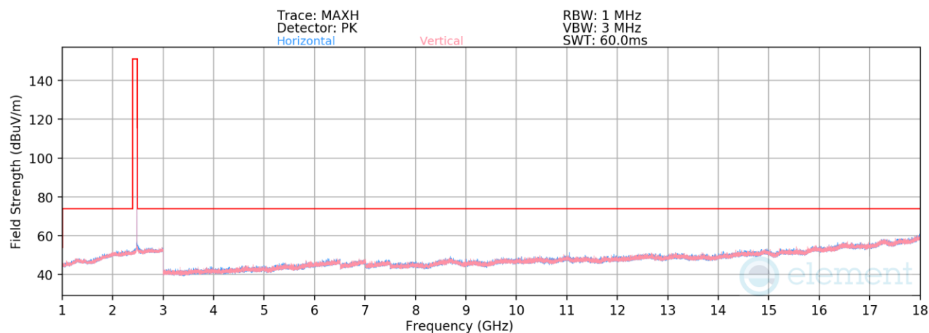
Plot 7-111. Radiated Spurious Emissions 1-18GHz Antenna WF8 (1Mbps ePA – Ch. 39)
