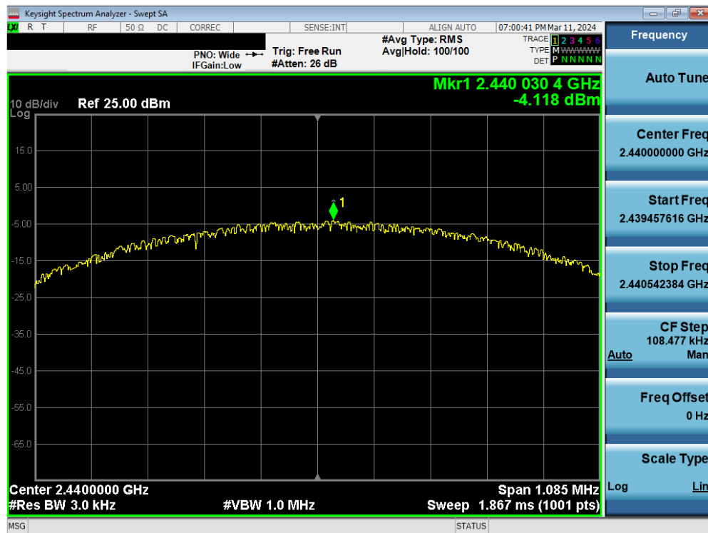
Plot 7-20. Power Spectral Density Plot Antenna WF8 (Bluetooth (LE), 1Mbps, ePA – Ch. 19)
