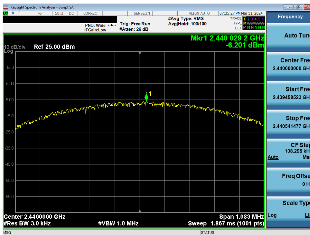
Plot 7-64. Power Spectral Density Plot Antenna WF7 (Bluetooth (LE), 1Mbps, iPA – Ch. 19)
