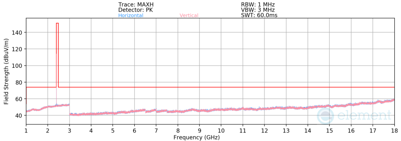
Plot 7-109. Radiated Spurious Emissions 1-18GHz Antenna WF8 (1Mbps, ePA – Ch. 0)
