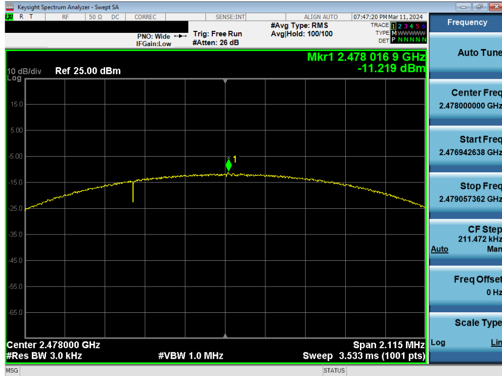
Plot 7-54. Power Spectral Density Plot Antenna WF9 (Bluetooth (LE), 2Mbps, iPA – Ch. 38)
