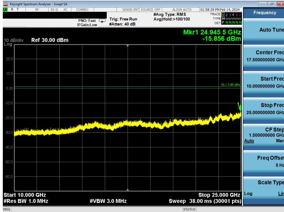
Plot 7-98. Conducted Spurious Plot Antenna WF7 (Bluetooth (LE), 1Mbps, ePA – Ch. 0)
