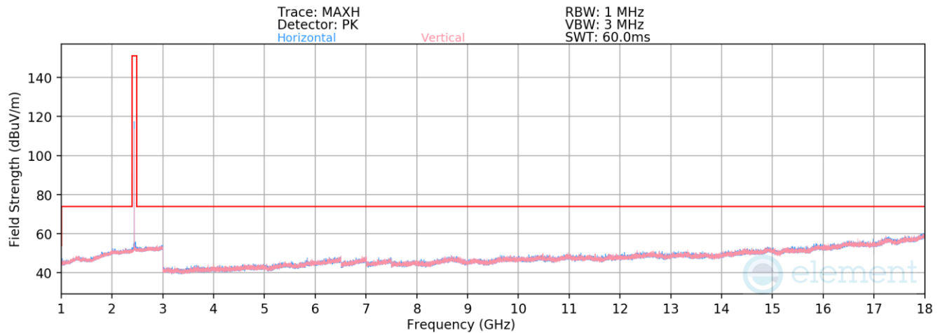
Plot 7-113. Radiated Spurious Emissions 1-18GHz Antenna WF7 (1Mbps, ePA – Ch. 19)
