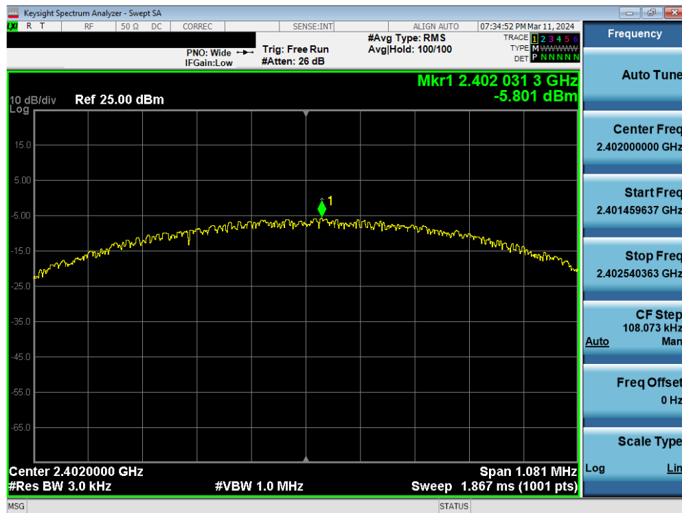
Plot 7-62. Power Spectral Density Plot Antenna WF7 (Bluetooth (LE), 1Mbps, iPA – Ch. 0)
