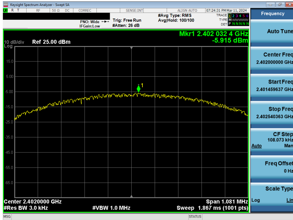
Plot 7-31. Power Spectral Density Plot Antenna WF7 (Bluetooth (LE), 1Mbps, ePA – Ch. 0)
