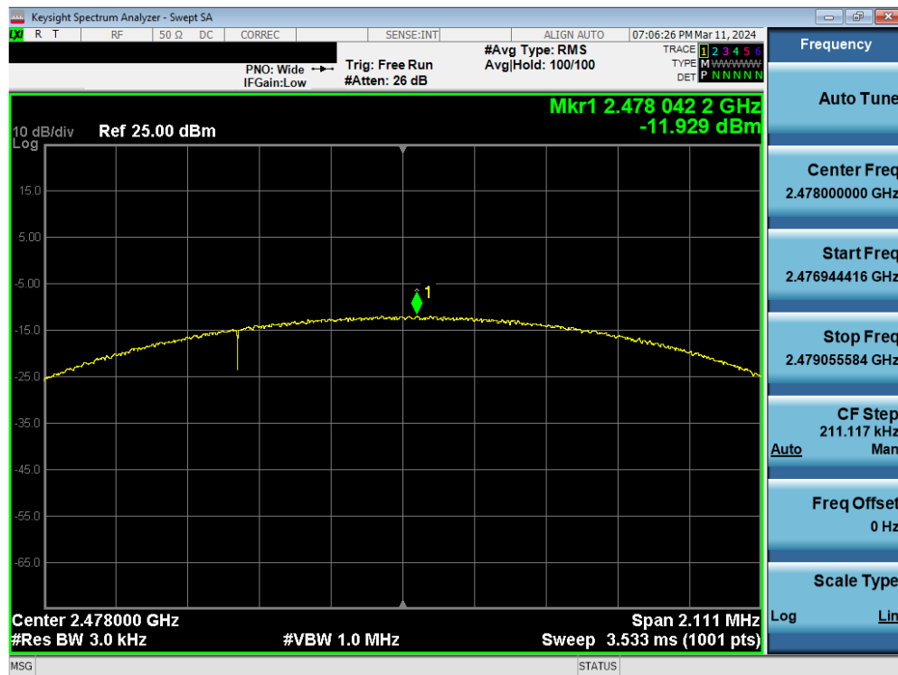
Plot 7-30. Power Spectral Density Plot Antenna WF8 (Bluetooth (LE), 2Mbps, iPA – Ch. 38)
