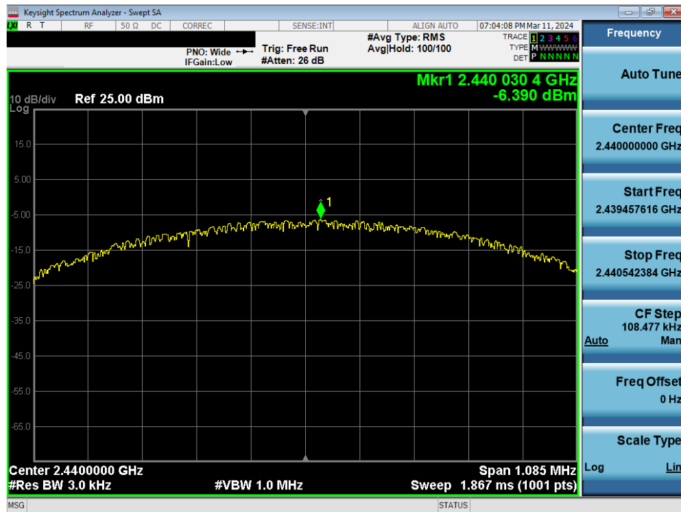
Plot 7-23. Power Spectral Density Plot Antenna WF8 (Bluetooth (LE), 1Mbps, iPA – Ch. 19)
