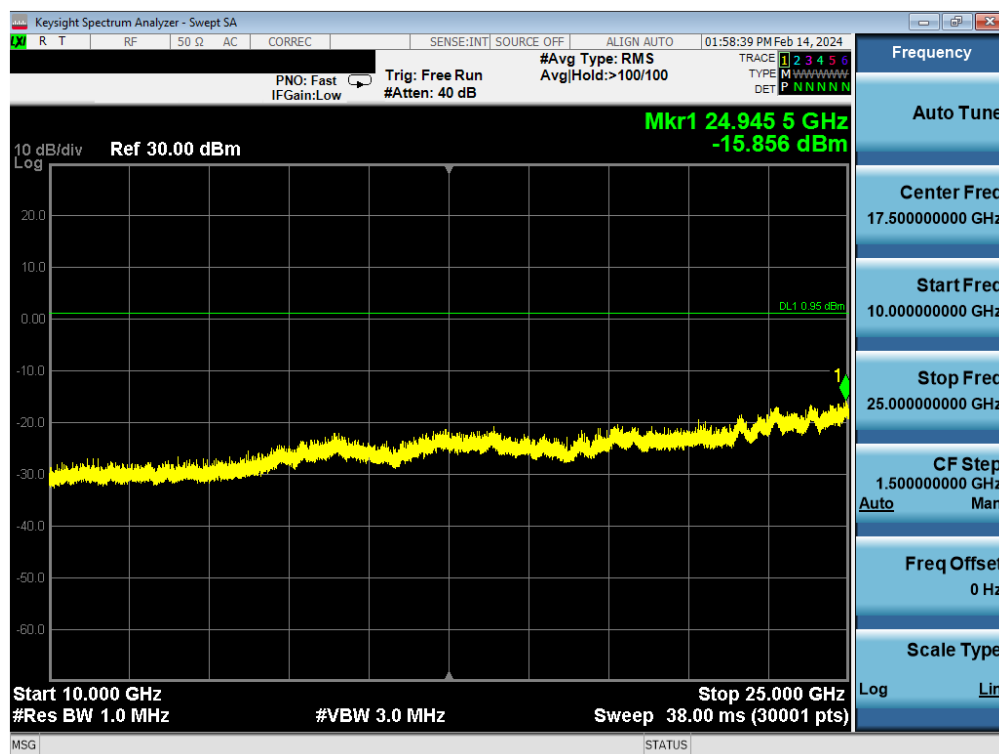
Plot 7-104. Conducted Spurious Plot Antenna WF9 (Bluetooth (LE), 1Mbps, ePA – Ch. 0)
