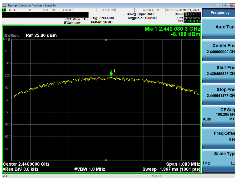
Plot 7-58. Power Spectral Density Plot Antenna WF7 (Bluetooth (LE), 1Mbps, ePA – Ch. 19)
