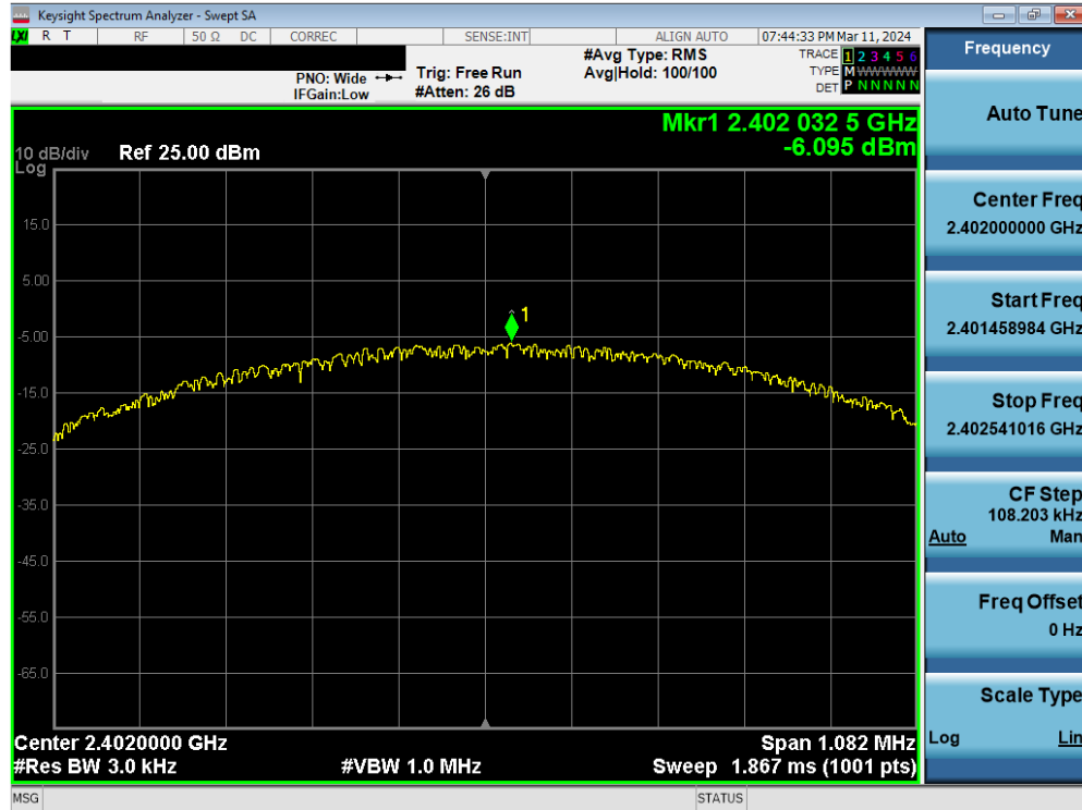
Plot 7-46. Power Spectral Density Plot Antenna WF9 (Bluetooth (LE), 1Mbps, iPA – Ch. 0)
