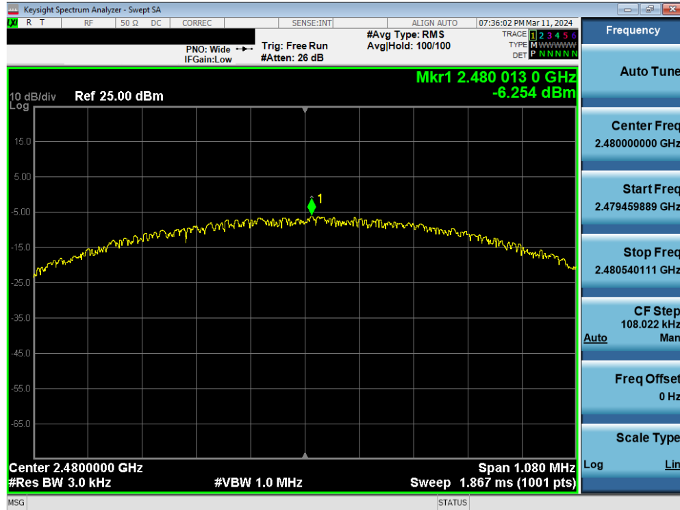
Plot 7-66. Power Spectral Density Plot Antenna WF7 (Bluetooth (LE), 1Mbps, iPA – Ch. 39)
