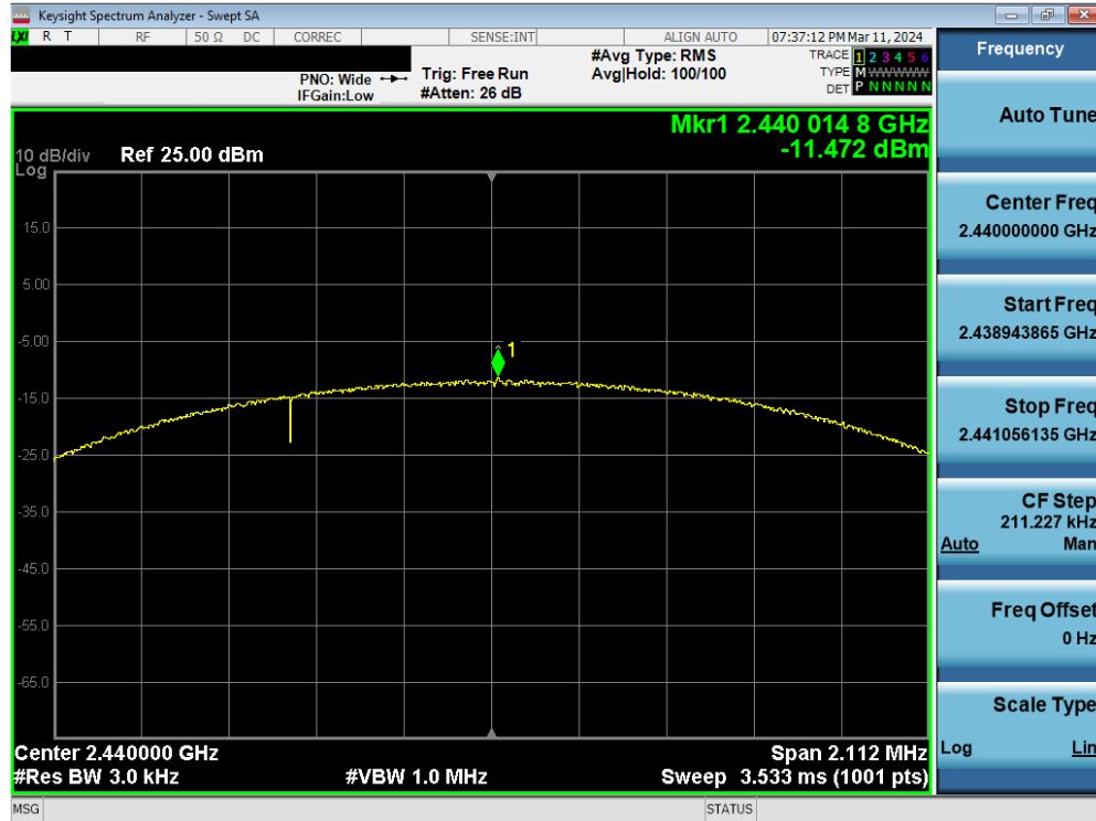
Plot 7-76. Power Spectral Density Plot Antenna WF7 (Bluetooth (LE), 2Mbps, iPA – Ch. 19)
