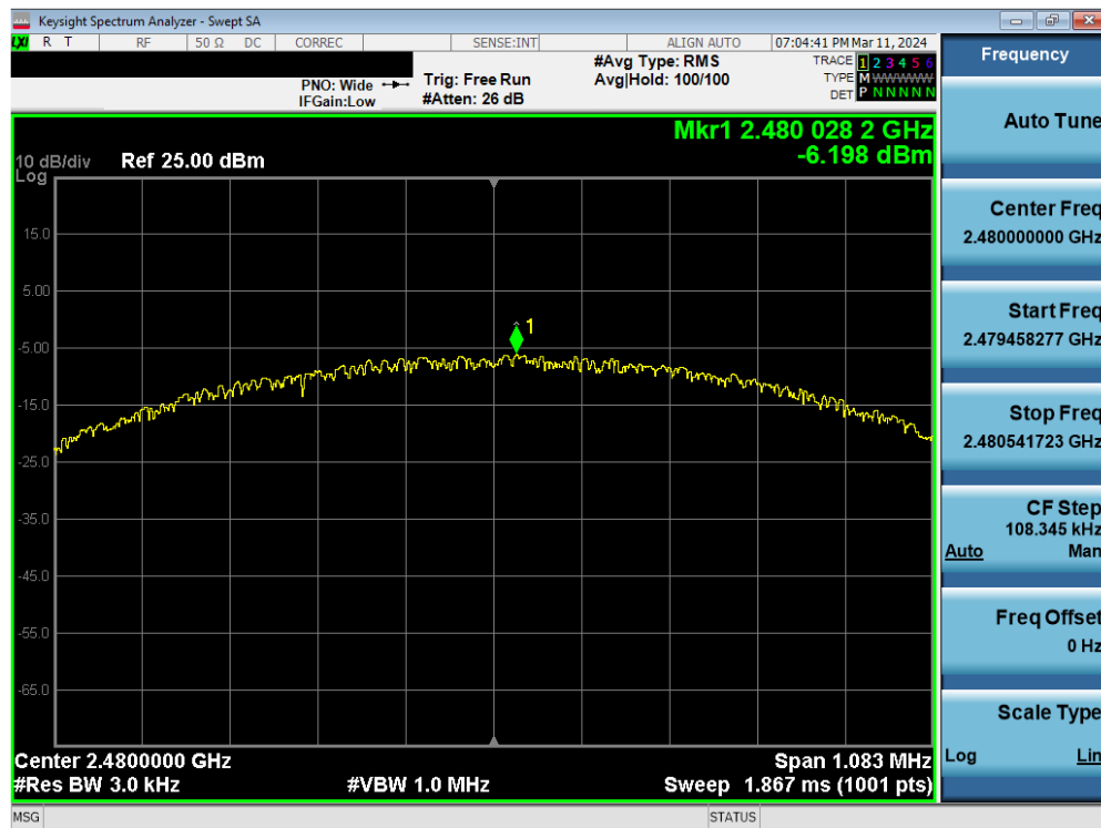
Plot 7-24. Power Spectral Density Plot Antenna WF8 (Bluetooth (LE), 1Mbps, iPA – Ch. 39)
