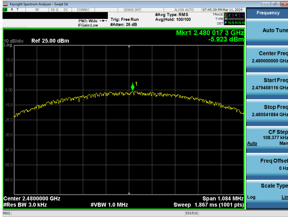
Plot 7-48. Power Spectral Density Plot Antenna WF9 (Bluetooth (LE), 1Mbps, iPA – Ch. 39)
