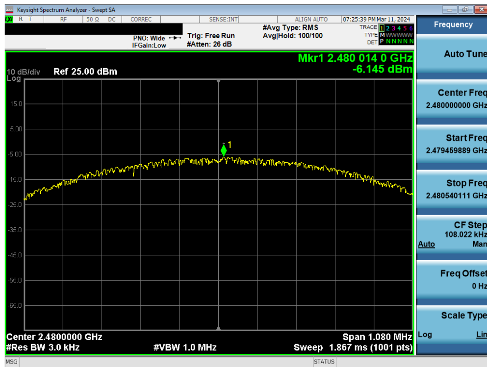
Plot 7-33. Power Spectral Density Plot Antenna WF7 (Bluetooth (LE), 1Mbps, ePA – Ch. 39)
