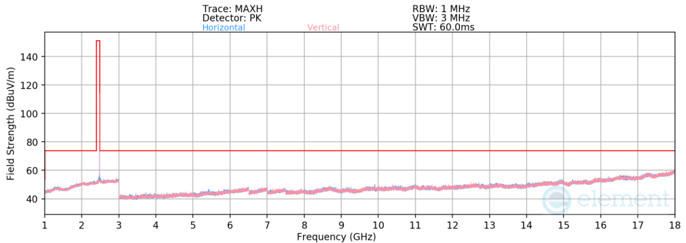
Plot 7-114. Radiated Spurious Emissions 1-18GHz Antenna WF7 (1Mbps ePA – Ch. 39)
