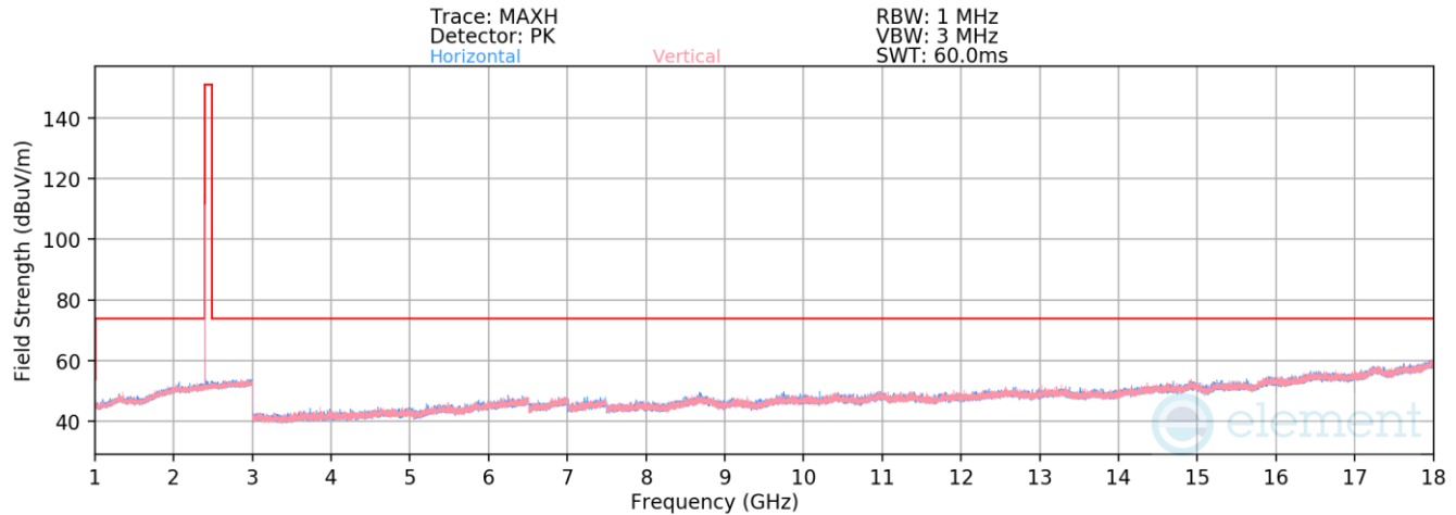
Plot 7-115. Radiated Spurious Emissions 1-18GHz Antenna WF9 (1Mbps, ePA – Ch. 0)
