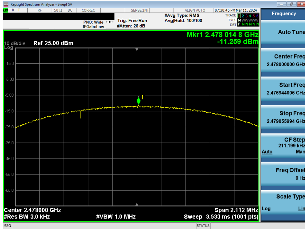
Plot 7-42. Power Spectral Density Plot Antenna WF7 (Bluetooth (LE), 2Mbps, iPA – Ch. 38)
