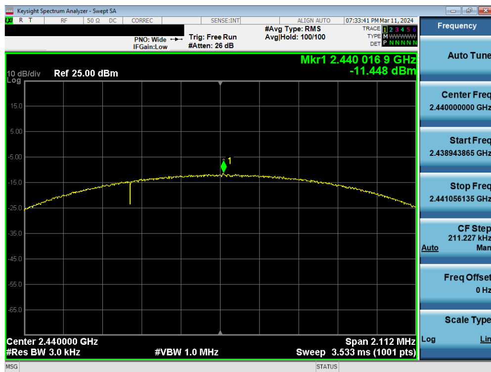
Plot 7-70. Power Spectral Density Plot Antenna WF7 (Bluetooth (LE), 2Mbps, ePA – Ch. 19)
