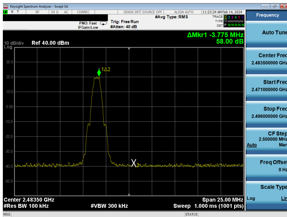
Plot 7-80. Band Edge Plot Antenna WF8 (Bluetooth (LE), 1Mbps, ePA – Ch. 39)
