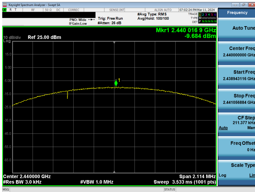
Plot 7-26. Power Spectral Density Plot Antenna WF8 (Bluetooth (LE), 2Mbps, ePA – Ch. 19)
