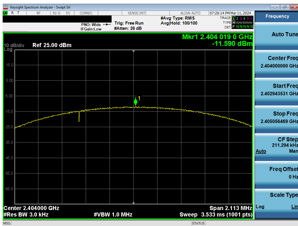
Plot 7-37. Power Spectral Density Plot Antenna WF7 (Bluetooth (LE), 2Mbps, ePA – Ch. 1)
