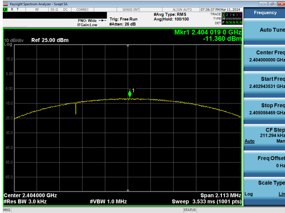
Plot 7-74. Power Spectral Density Plot Antenna WF7 (Bluetooth (LE), 2Mbps, iPA – Ch. 1)
