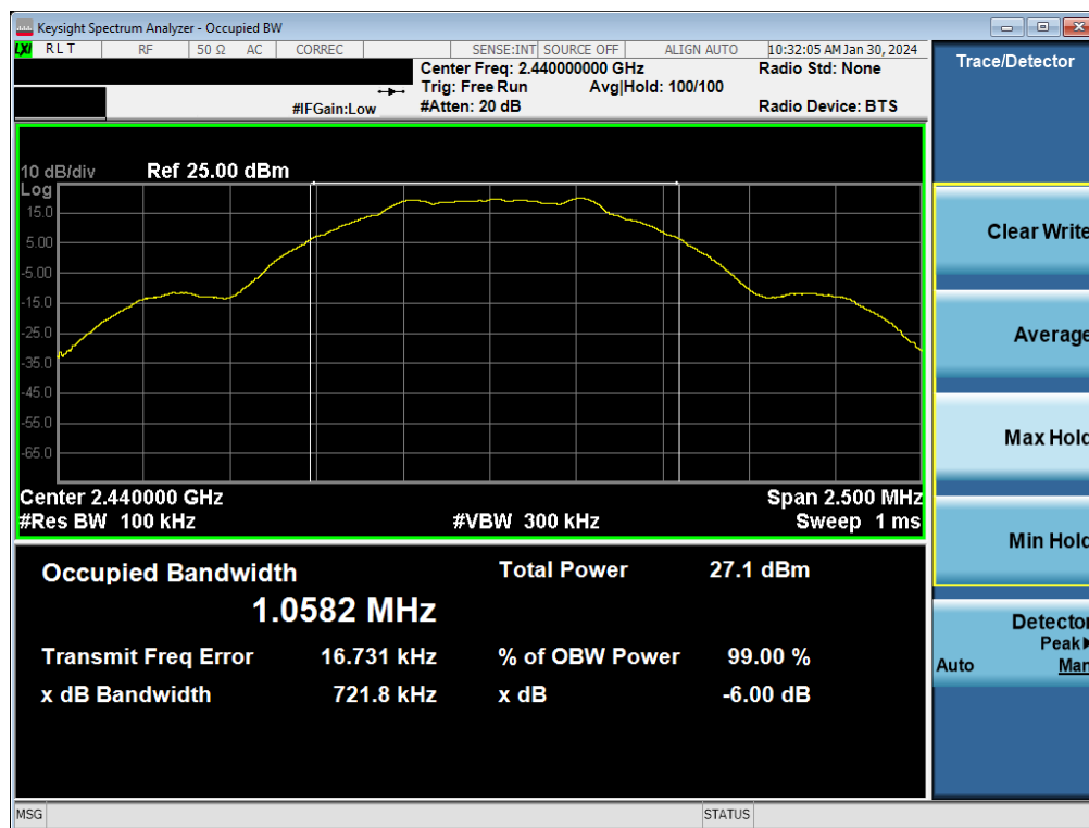
Plot 7-14. 6dB BW & 99% OBW Plot Antenna WF9 (Bluetooth (LE), 1Mbps, ePA – Ch. 19)
