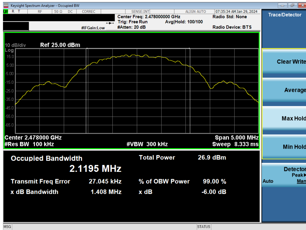
Plot 7-12. 6dB BW & 99% OBW Plot Antenna WF7 (Bluetooth (LE), 2Mbps, ePA – Ch. 38)
