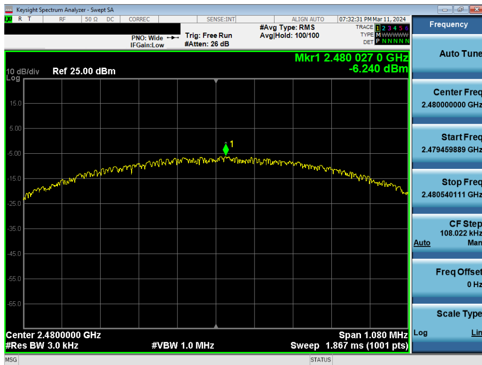
Plot 7-60. Power Spectral Density Plot Antenna WF7 (Bluetooth (LE), 1Mbps, ePA – Ch. 39)
