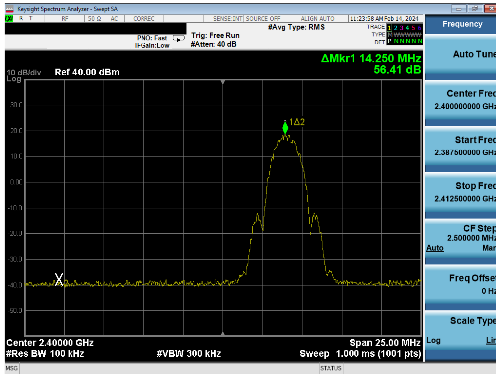
Plot 7-81. Band Edge Plot Antenna WF8 (Bluetooth (LE), 2Mbps, ePA – Ch. 1)
