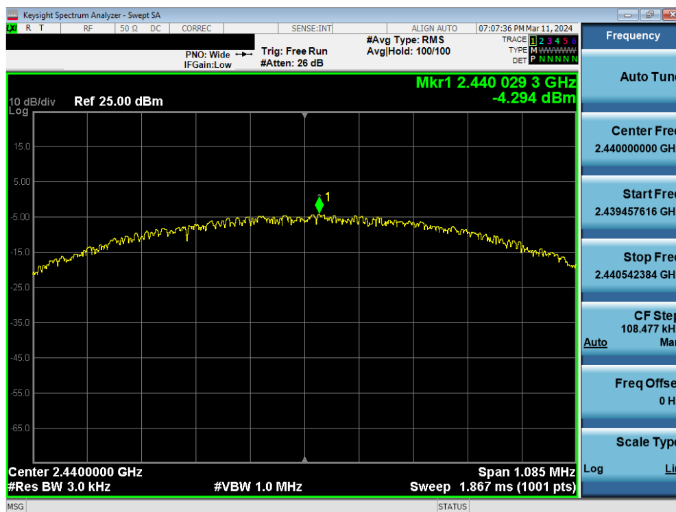
Plot 7-57. Power Spectral Density Plot Antenna WF8 (Bluetooth (LE), 1Mbps, ePA – Ch. 19)
