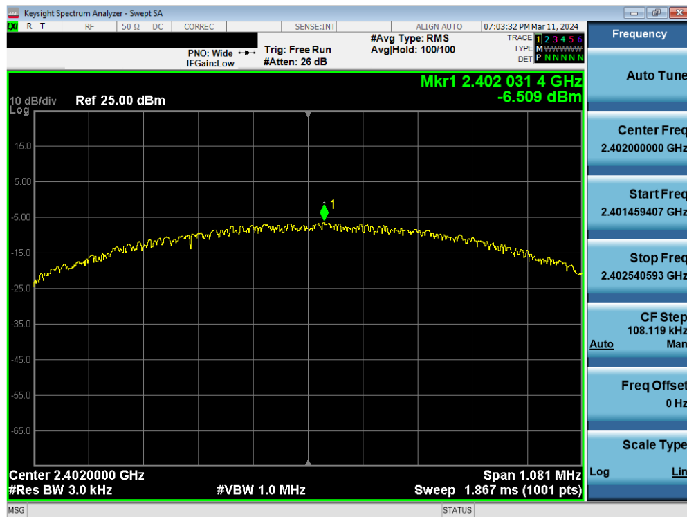
Plot 7-22. Power Spectral Density Plot Antenna WF8 (Bluetooth (LE), 1Mbps, iPA – Ch. 0)
