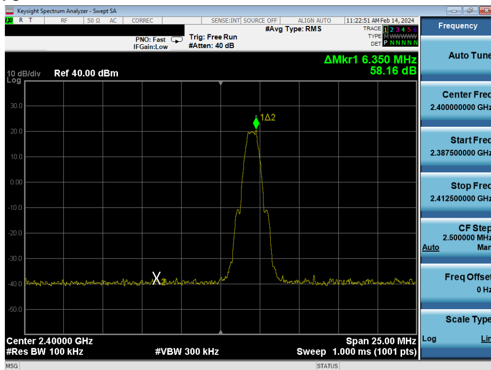
Plot 7-79. Band Edge Plot Antenna WF8 (Bluetooth (LE), 1Mbps, ePA – Ch.0)
