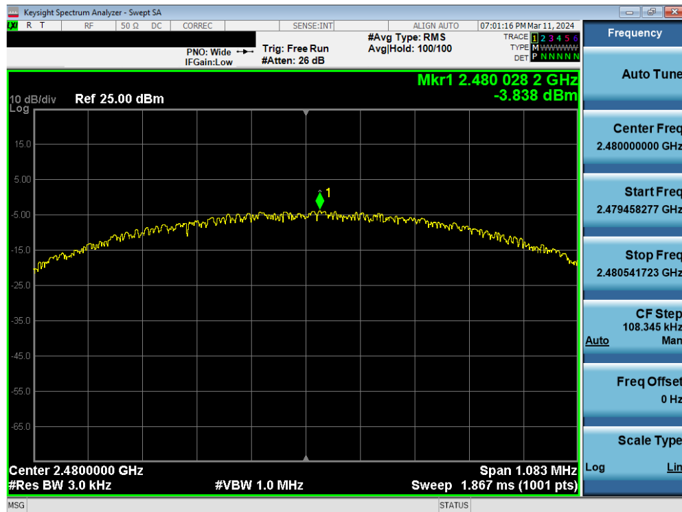
Plot 7-21. Power Spectral Density Plot Antenna WF8 (Bluetooth (LE), 1Mbps, ePA – Ch. 39)
