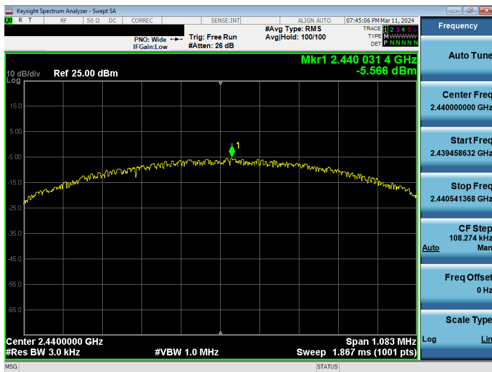
Plot 7-47. Power Spectral Density Plot Antenna WF9 (Bluetooth (LE), 1Mbps, iPA – Ch. 19)
