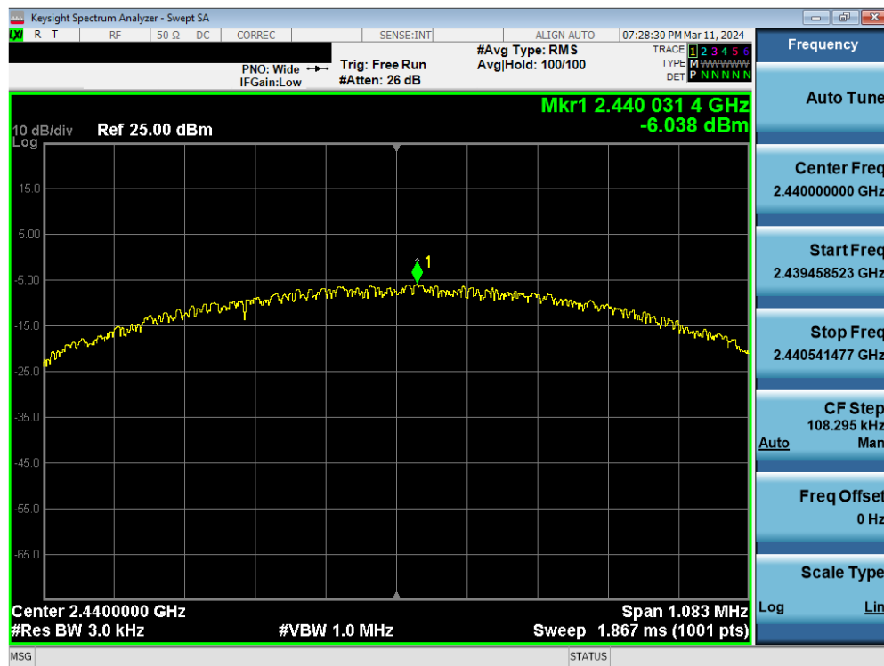
Plot 7-35. Power Spectral Density Plot Antenna WF7 (Bluetooth (LE), 1Mbps, iPA – Ch. 19)
