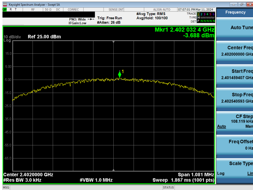
Plot 7-55. Power Spectral Density Plot Antenna WF8 (Bluetooth (LE), 1Mbps, ePA – Ch. 0)
