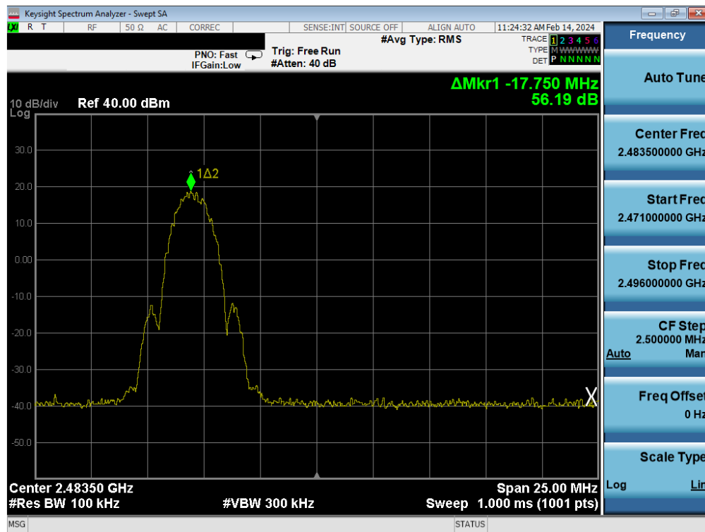
Plot 7-82. Band Edge Plot Antenna WF8 (Bluetooth (LE), 2Mbps, ePA – Ch. 38)
