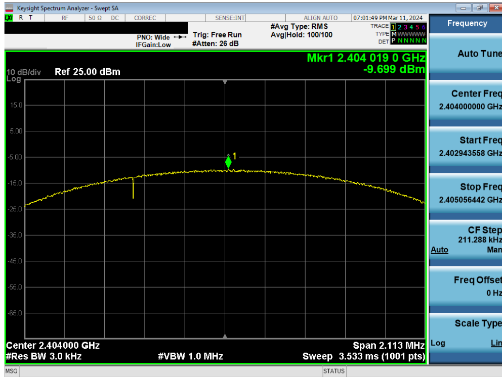
Plot 7-25. Power Spectral Density Plot Antenna WF8 (Bluetooth (LE), 2Mbps, ePA – Ch. 1)
