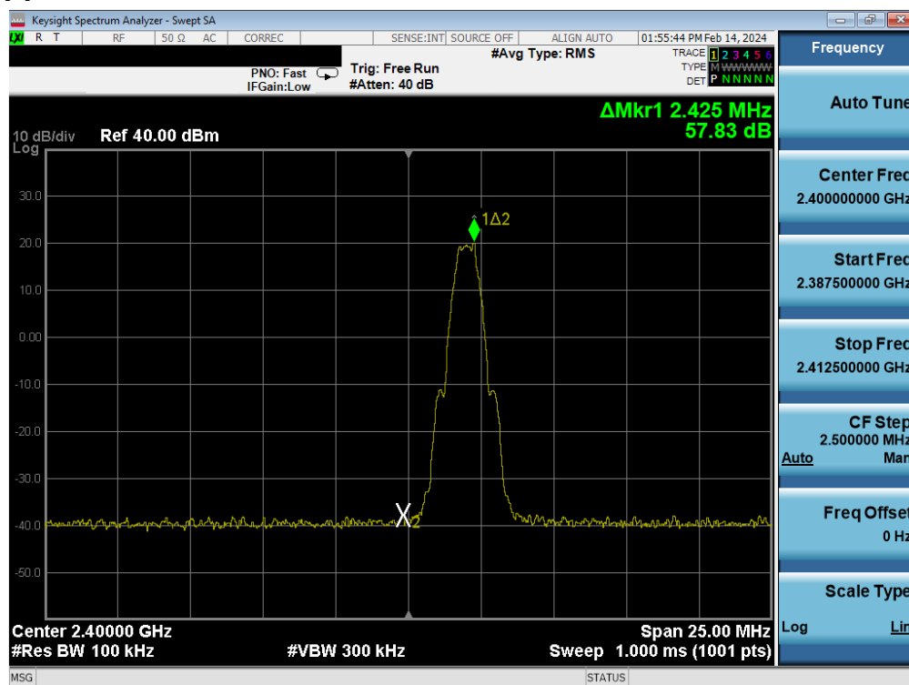
Plot 7-83. Band Edge Plot Antenna WF7 (Bluetooth (LE), 1Mbps, ePA – Ch.0)
