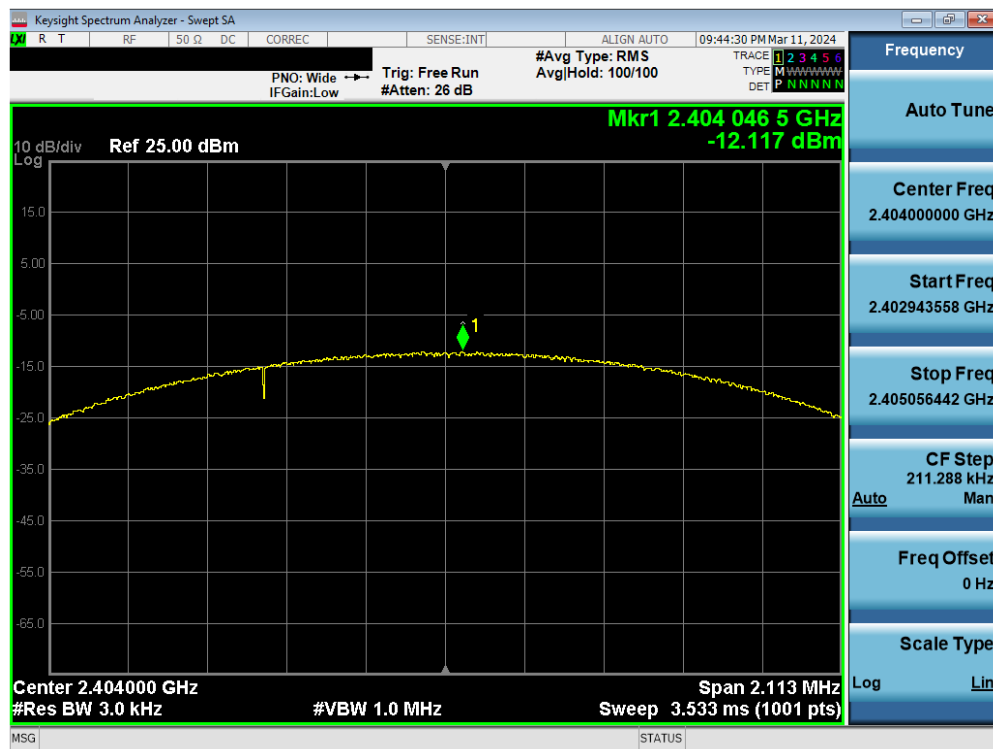
Plot 7-73. Power Spectral Density Plot Antenna WF8 (Bluetooth (LE), 2Mbps, iPA – Ch. 1)
