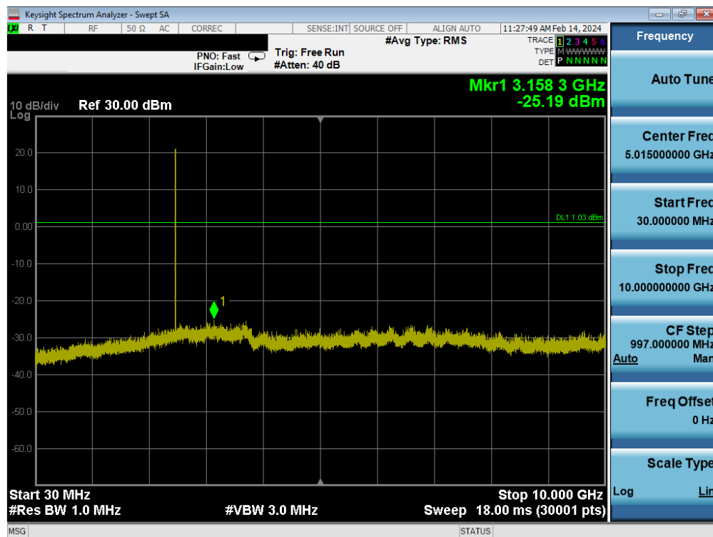
Plot 7-95. Conducted Spurious Plot Antenna WF8 (Bluetooth (LE), 1Mbps, ePA – Ch. 39)
