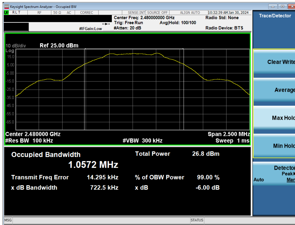
Plot 7-15. 6dB BW & 99% OBW Plot Antenna WF9 (Bluetooth (LE), 1Mbps, ePA – Ch. 39)
