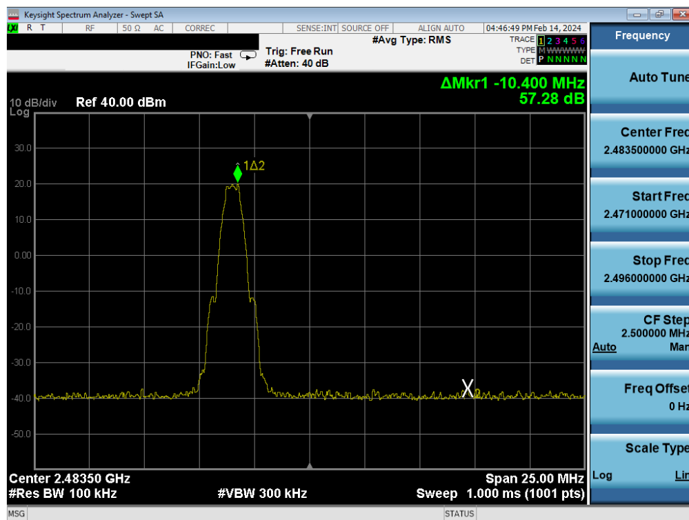
Plot 7-88. Band Edge Plot Antenna WF9 (Bluetooth (LE), 1Mbps, ePA – Ch. 39)
