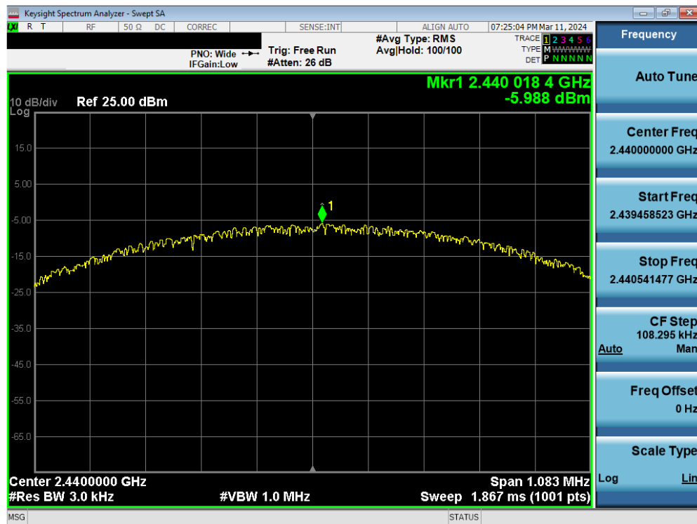
Plot 7-32. Power Spectral Density Plot Antenna WF7 (Bluetooth (LE), 1Mbps, ePA – Ch. 19)
