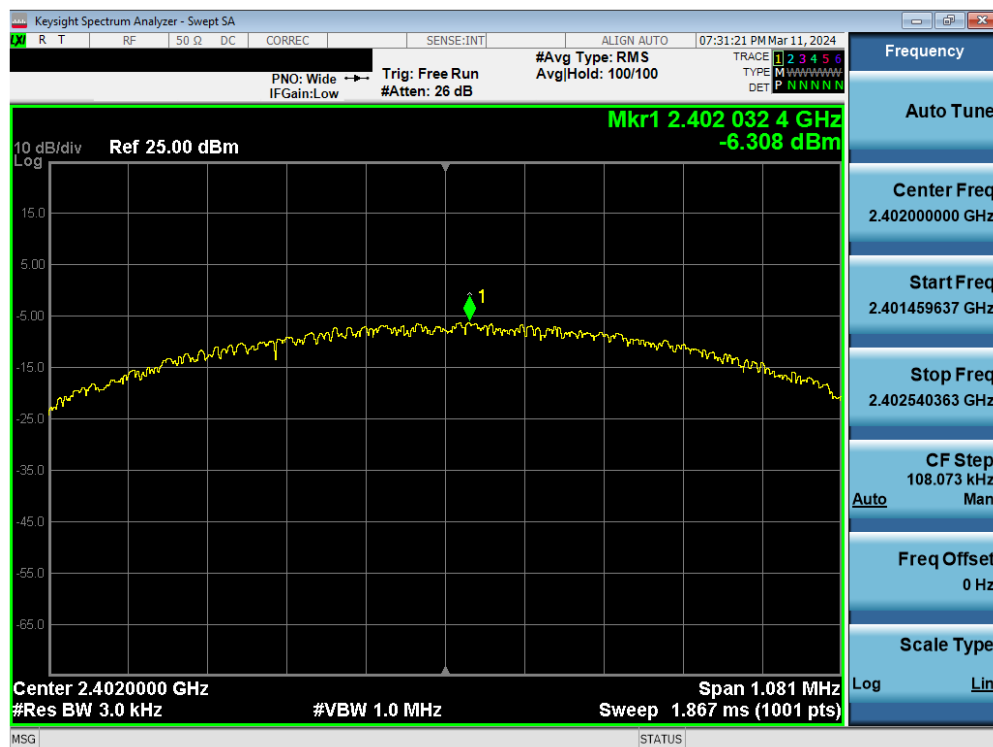
Plot 7-56. Power Spectral Density Plot Antenna WF7 (Bluetooth (LE), 1Mbps, ePA – Ch. 0)
