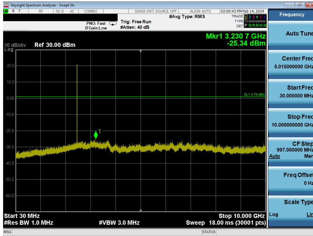
Plot 7-107. Conducted Spurious Plot Antenna WF9 (Bluetooth (LE), 1Mbps, ePA – Ch. 39)
