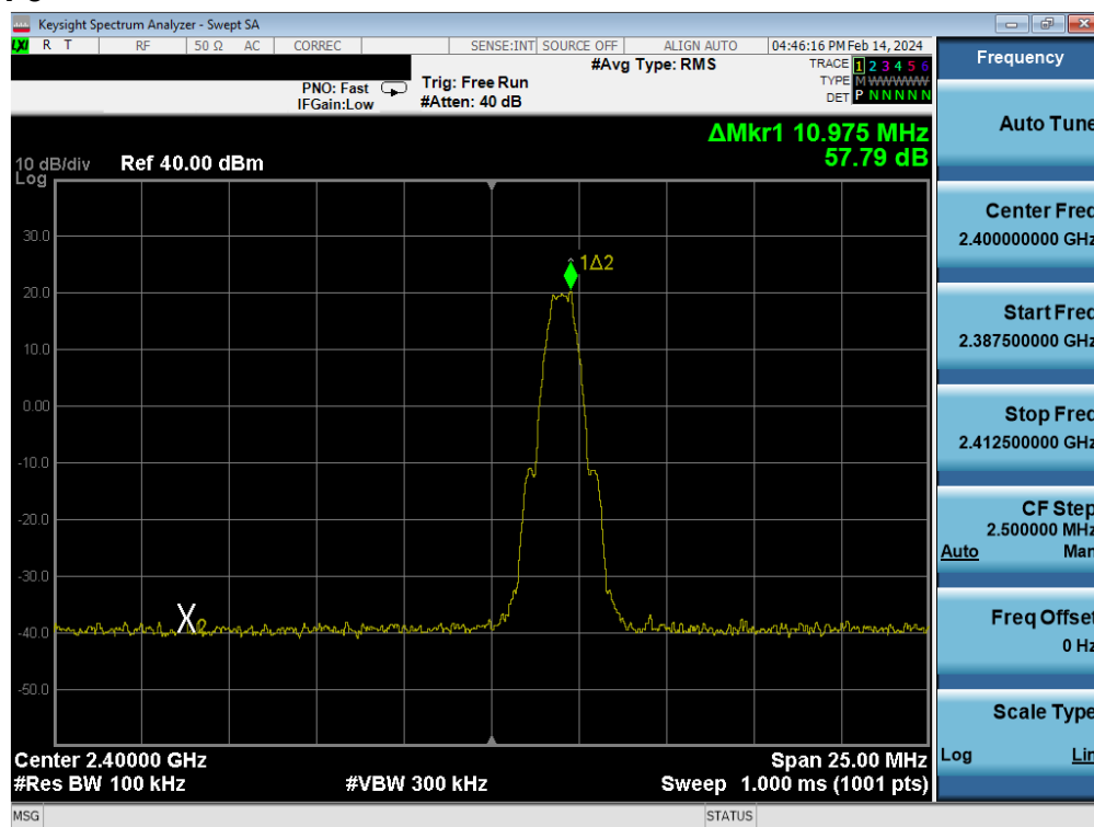
Plot 7-87. Band Edge Plot Antenna WF9 (Bluetooth (LE), 1Mbps, ePA – Ch.0)
