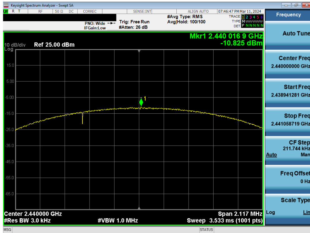
Plot 7-53. Power Spectral Density Plot Antenna WF9 (Bluetooth (LE), 2Mbps, iPA – Ch. 19)
