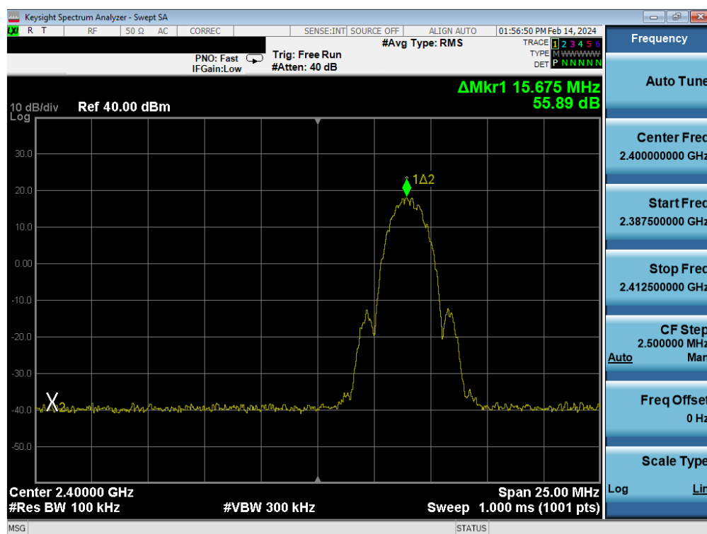
Plot 7-85. Band Edge Plot Antenna WF7 (Bluetooth (LE), 2Mbps, ePA – Ch. 1)
