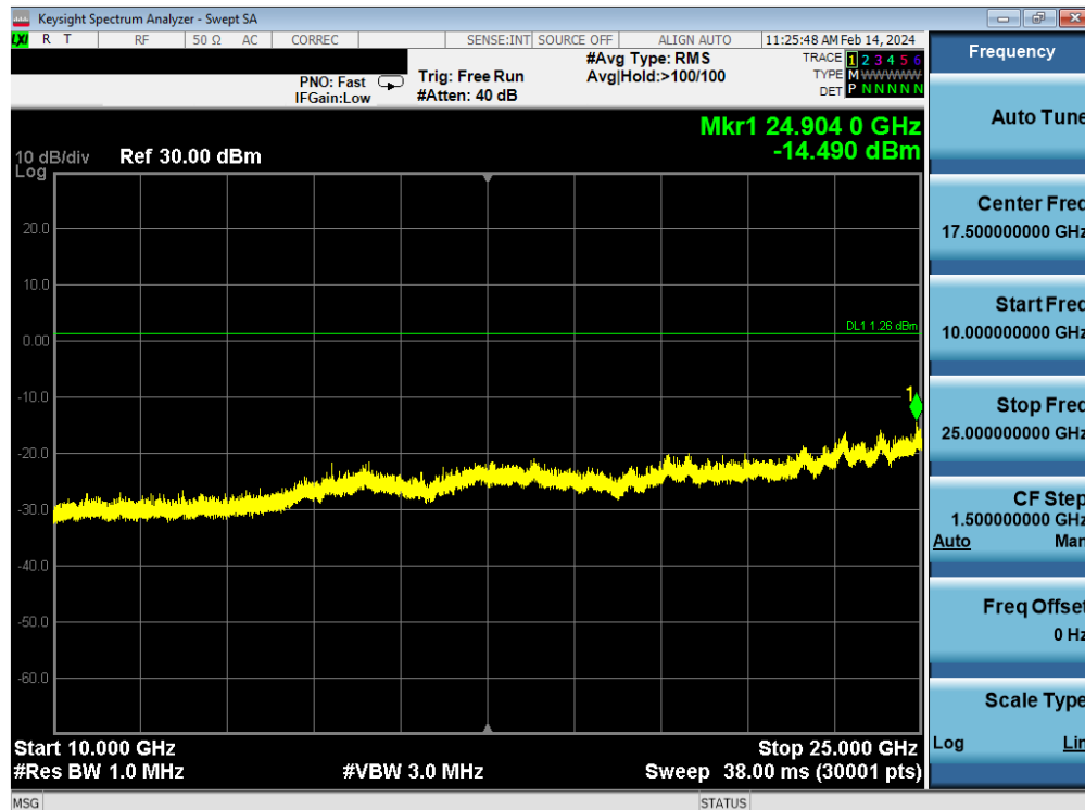
Plot 7-92. Conducted Spurious Plot Antenna WF8 (Bluetooth (LE), 1Mbps, ePA – Ch. 0)
