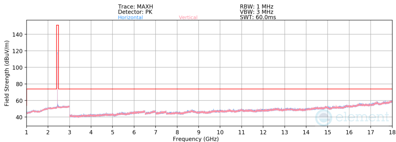
Plot 7-110. Radiated Spurious Emissions 1-18GHz Antenna WF8 (1Mbps, ePA – Ch. 19)
