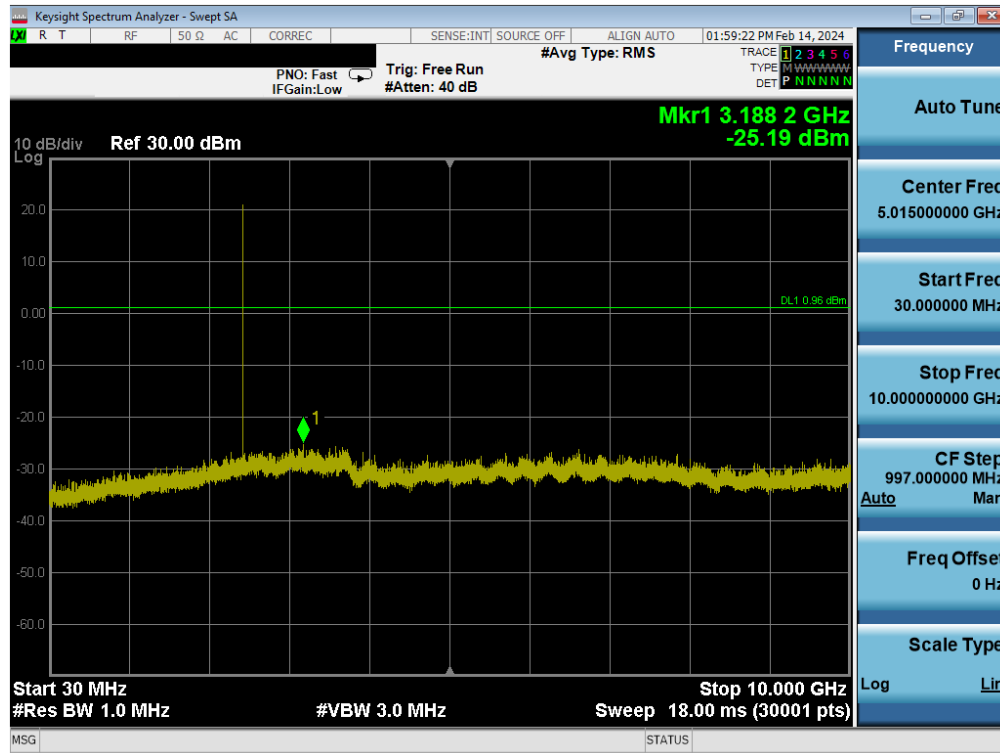
Plot 7-99. Conducted Spurious Plot Antenna WF7 (Bluetooth (LE), 1Mbps, ePA – Ch. 19)
