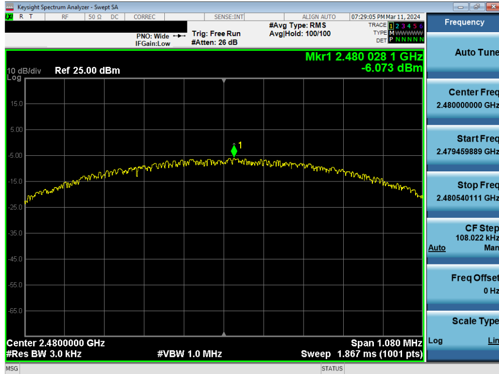
Plot 7-36. Power Spectral Density Plot Antenna WF7 (Bluetooth (LE), 1Mbps, iPA – Ch. 39)
