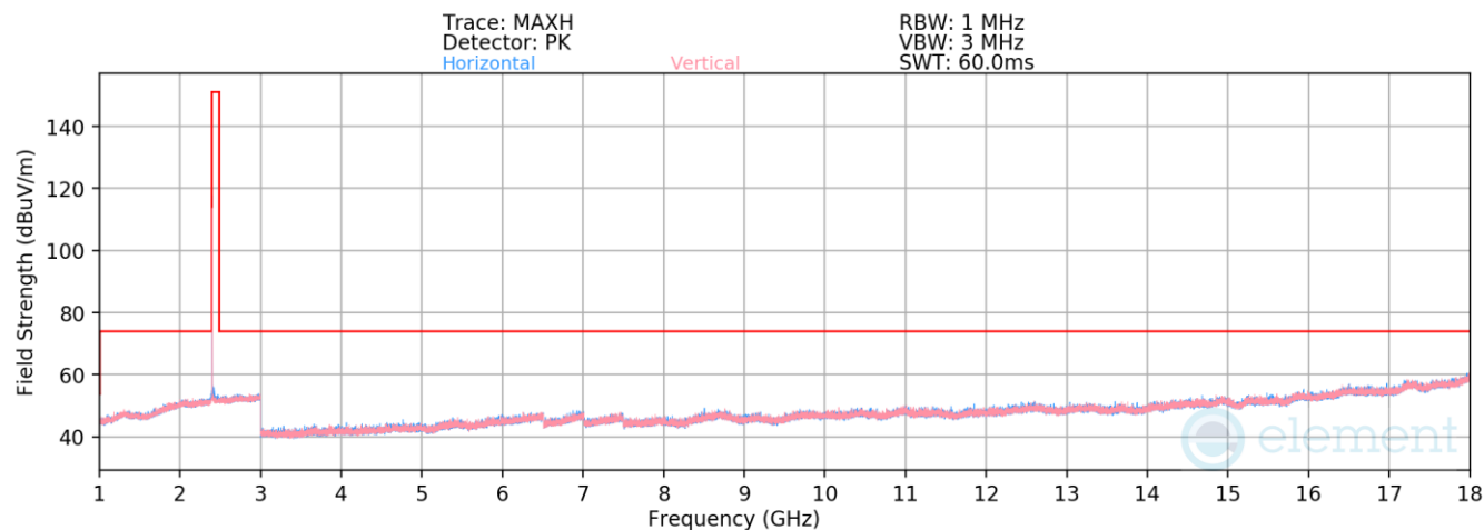
Plot 7-112. Radiated Spurious Emissions 1-18GHz Antenna WF7 (1Mbps, ePA – Ch. 0)
