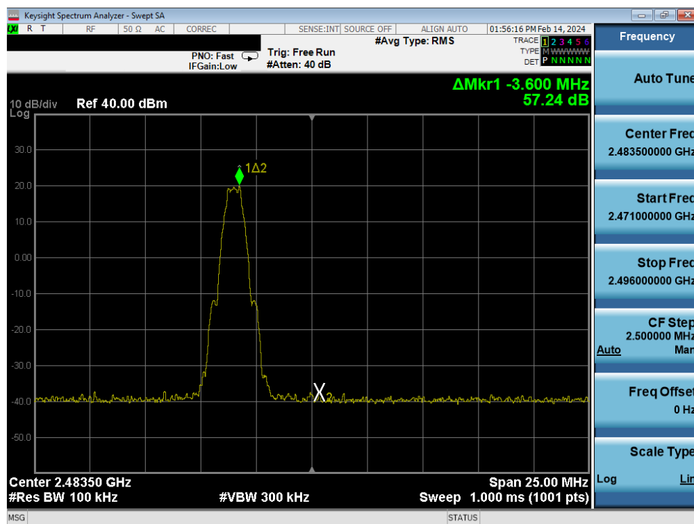
Plot 7-84. Band Edge Plot Antenna WF7 (Bluetooth (LE), 1Mbps, ePA – Ch. 39)
