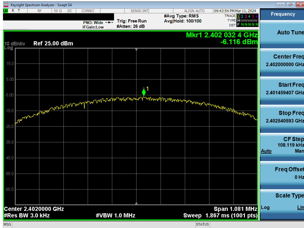
Plot 7-61. Power Spectral Density Plot Antenna WF8 (Bluetooth (LE), 1Mbps, iPA – Ch. 0)
