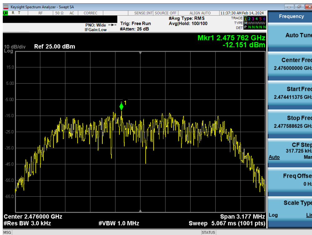
Plot 7-24. Power Spectral Density Plot Antenna WF8 (Bluetooth (HDR4), 4Mbps, iPA – Ch. 73)
