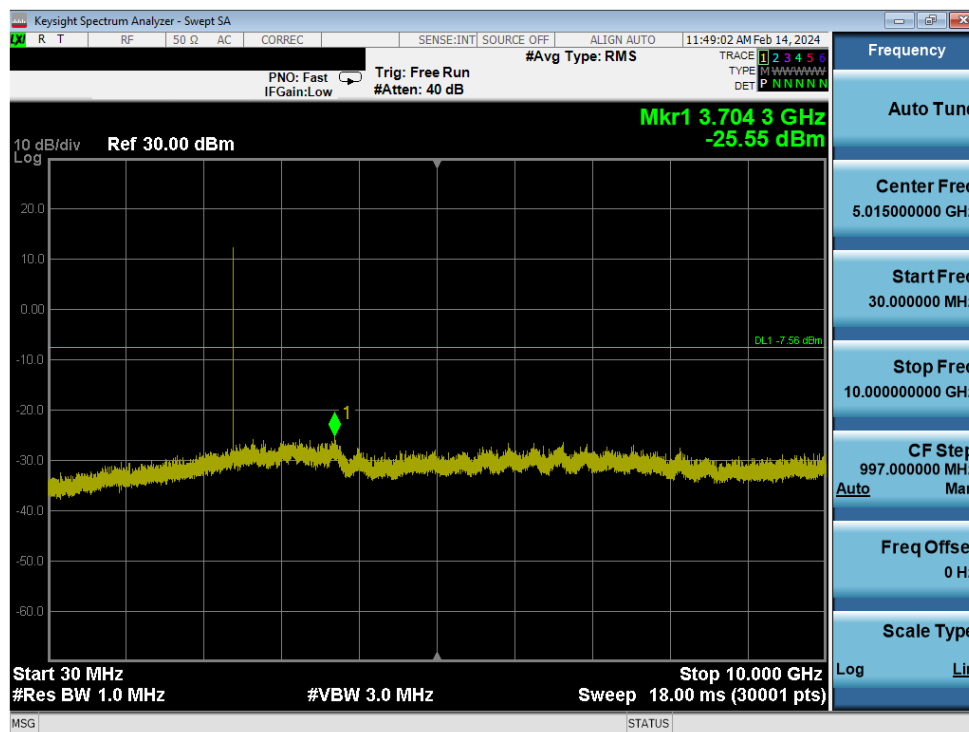
Plot 7-91. Conducted Spurious Plot Antenna WF8 (Bluetooth (HDR4), 4 Mbps, ePA – Ch. 1)
