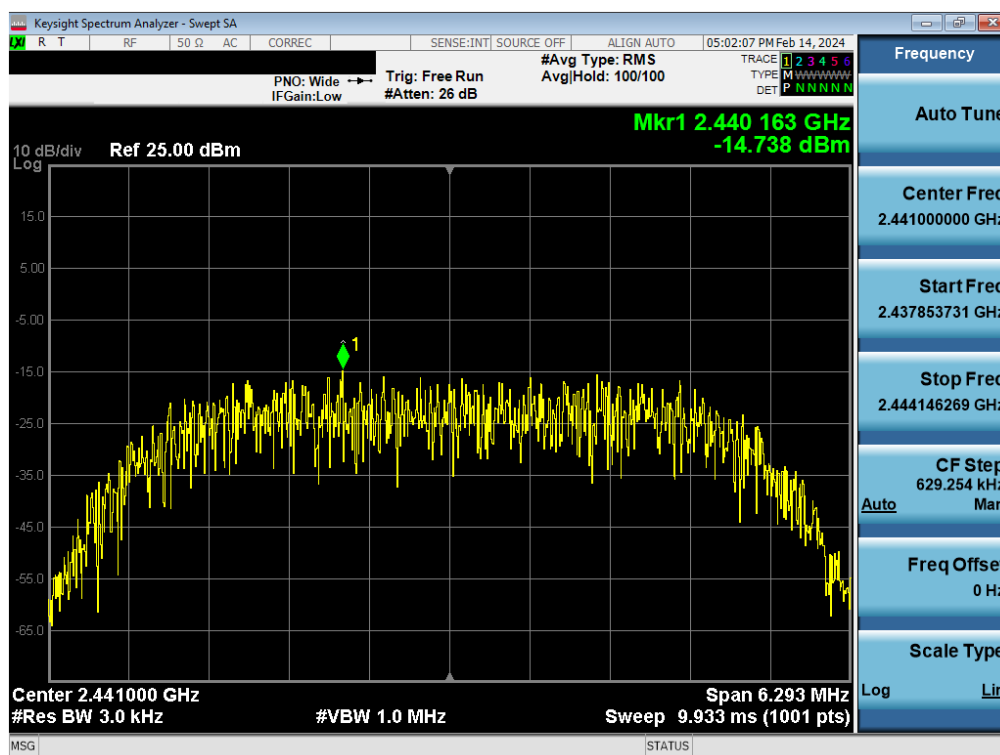
Plot 7-53. Power Spectral Density Plot Antenna WF9 (Bluetooth (HDR8), 8Mbps, iPA – Ch. 38)
