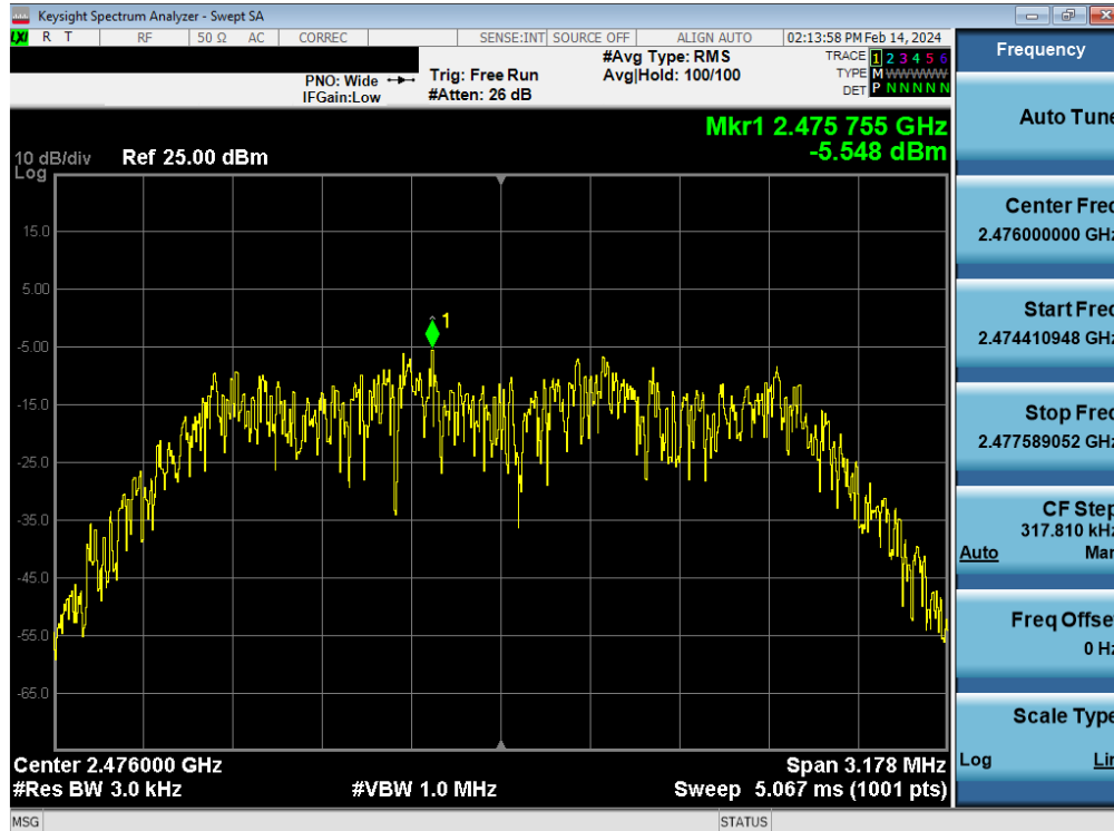
Plot 7-60. Power Spectral Density Plot Tx BF Antenna WF7 (Bluetooth (HDR4), 4Mbps, ePA – Ch. 73)
