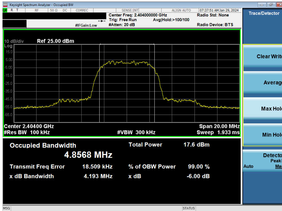
Plot 7-10. 6dB BW & 99% OBW Plot Antenna WF7 (Bluetooth (HDR8), 8Mbps, ePA – Ch. 1)
