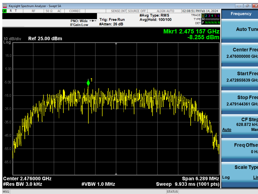
Plot 7-39. Power Spectral Density Plot Antenna WF7 (Bluetooth (HDR8), 8Mbps, ePA – Ch. 73)
