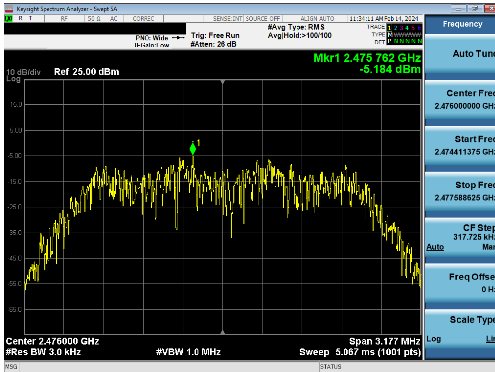
Plot 7-21. Power Spectral Density Plot Antenna WF8 (Bluetooth (HDR4), 4Mbps, ePA – Ch. 73)
