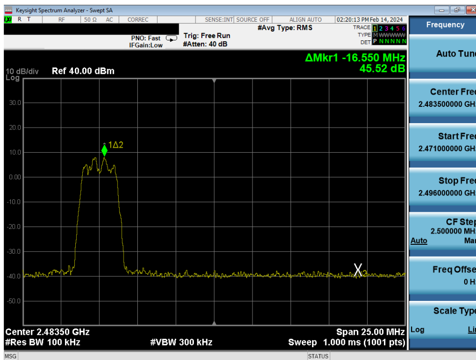
Plot 7-84. Band Edge Plot Antenna WF7 (Bluetooth (HDR4), ePA – Ch. 73)
