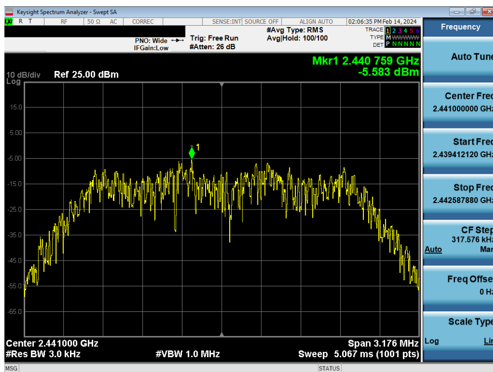
Plot 7-32. Power Spectral Density Plot Antenna WF7 (Bluetooth (HDR4), 4Mbps, ePA – Ch. 38)
