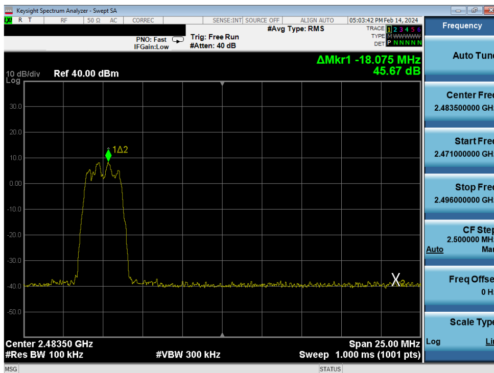
Plot 7-88. Band Edge Plot Antenna WF9 (Bluetooth (HDR4), ePA – Ch. 73)
