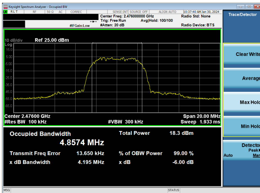
Plot 7-18. 6dB BW & 99% OBW Plot Antenna WF9 (Bluetooth (HDR8), 8Mbps, ePA – Ch. 73)
