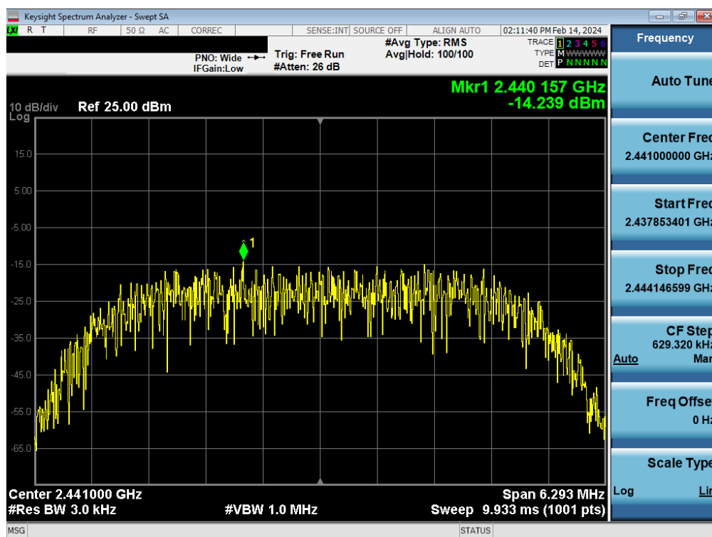
Plot 7-41. Power Spectral Density Plot Antenna WF7 (Bluetooth (HDR8), 8Mbps, iPA – Ch. 38)
