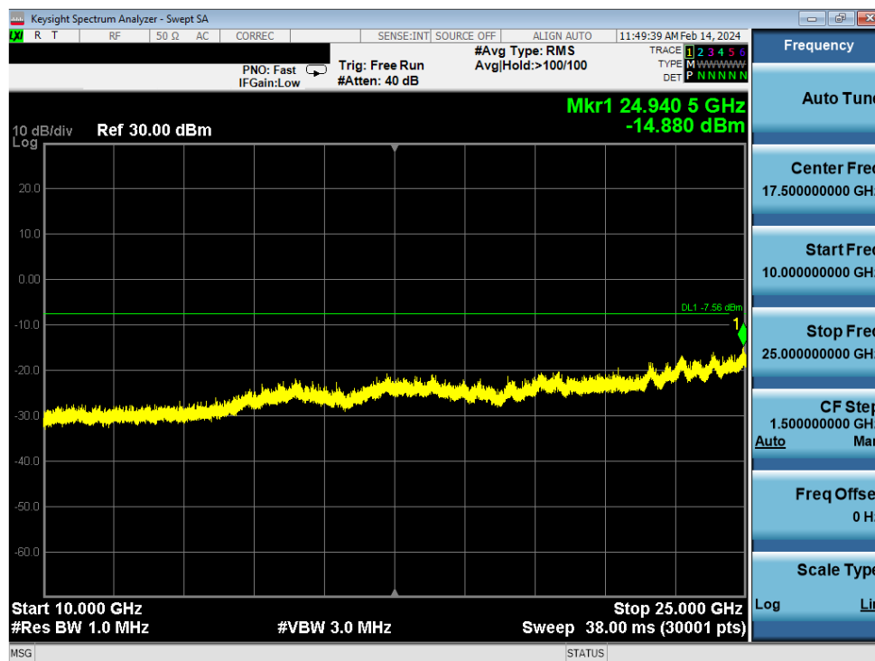
Plot 7-92. Conducted Spurious Plot Antenna WF8 (Bluetooth (HDR4), 4 Mbps, ePA – Ch. 1)
