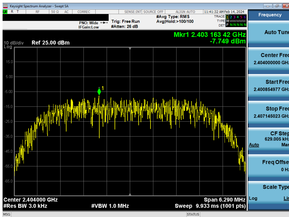
Plot 7-67. Power Spectral Density Plot Tx BF Antenna WF8 (Bluetooth (HDR8), 8Mbps, ePA – Ch. 1)
