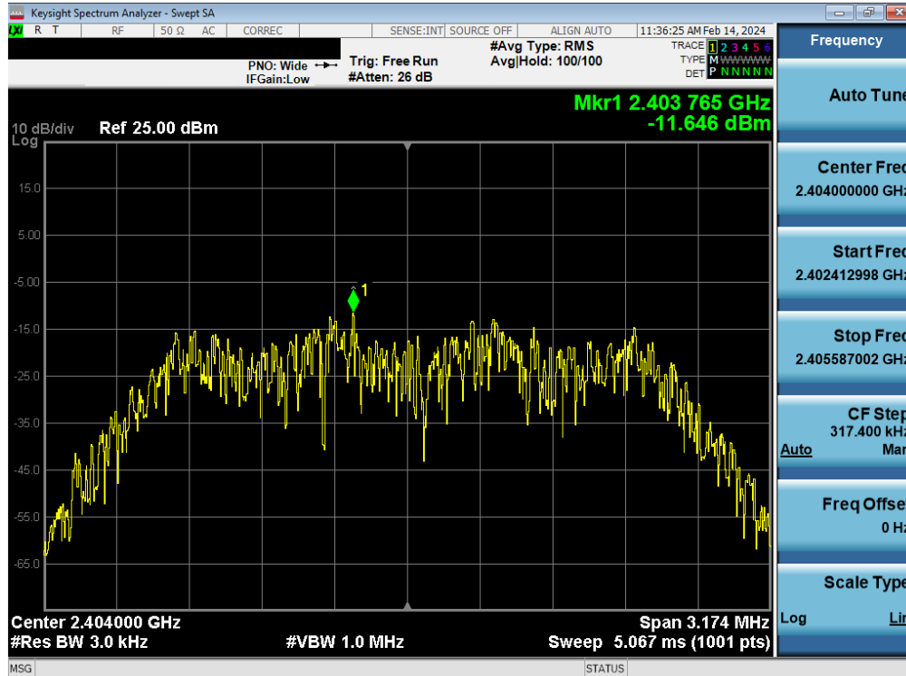
Plot 7-22. Power Spectral Density Plot Antenna WF8 (Bluetooth (HDR4), 4Mbps, iPA – Ch. 1)
