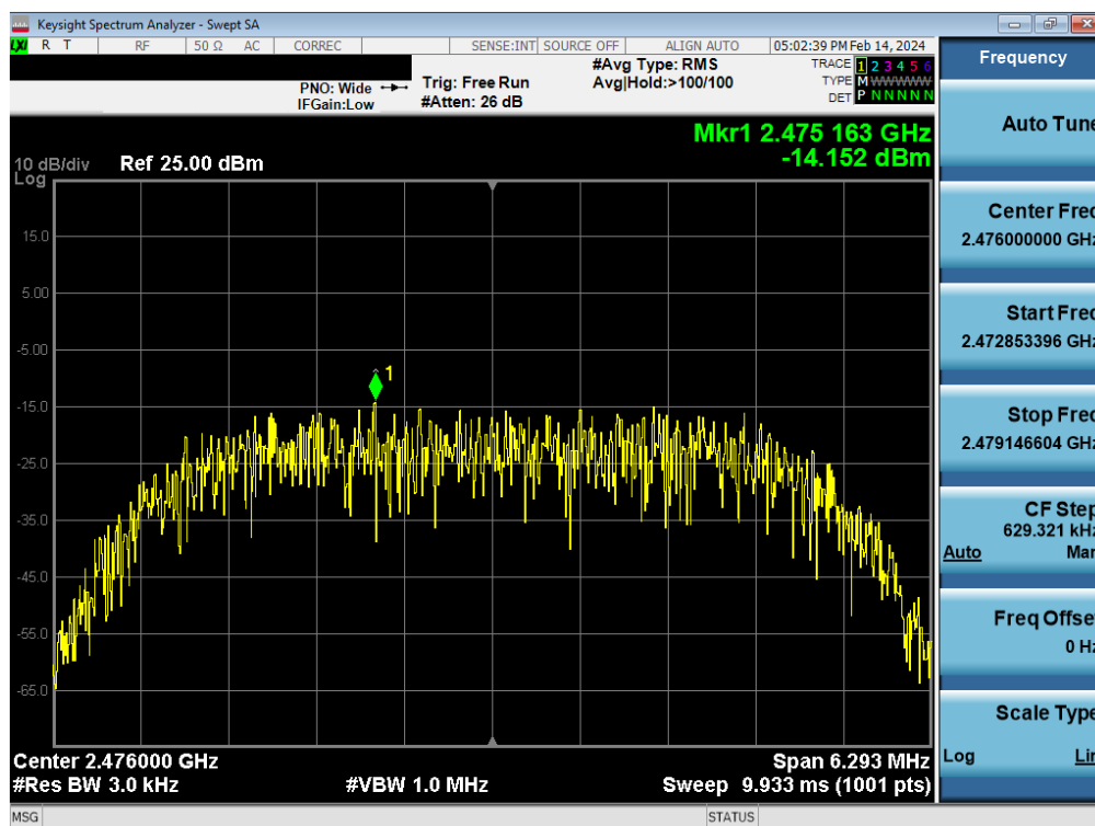
Plot 7-54. Power Spectral Density Plot Antenna WF9 (Bluetooth (HDR8), 8Mbps, iPA – Ch. 73)
