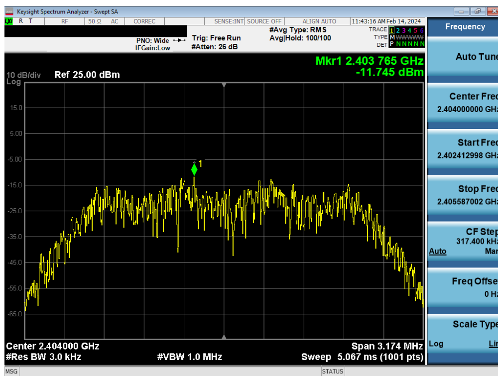
Plot 7-61. Power Spectral Density Plot Tx BF Antenna WF8 (Bluetooth (HDR4), 4Mbps, iPA – Ch. 1)
