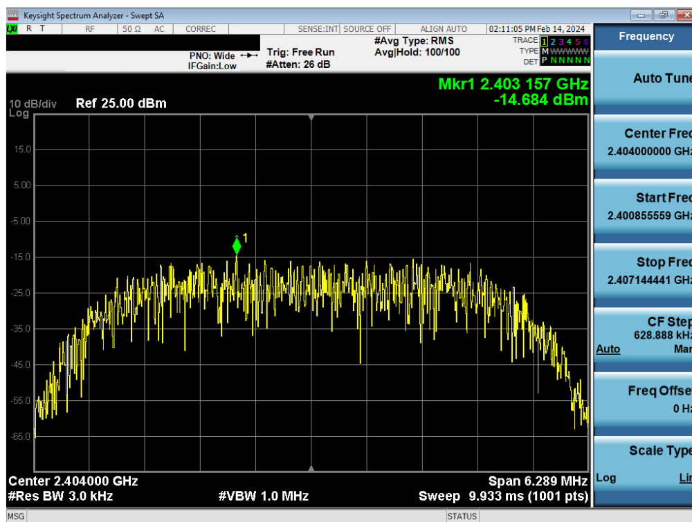
Plot 7-40. Power Spectral Density Plot Antenna WF7 (Bluetooth (HDR8), 8Mbps, iPA – Ch. 1)
