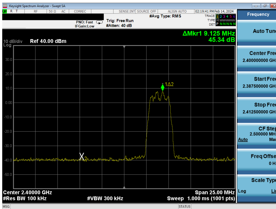
Plot 7-83. Band Edge Plot Antenna WF7 (Bluetooth (HDR4), ePA – Ch. 1)
