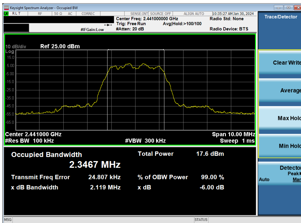
Plot 7-14. 6dB BW & 99% OBW Plot Antenna WF9 (Bluetooth (HDR4), 4Mbps, ePA – Ch. 38)
