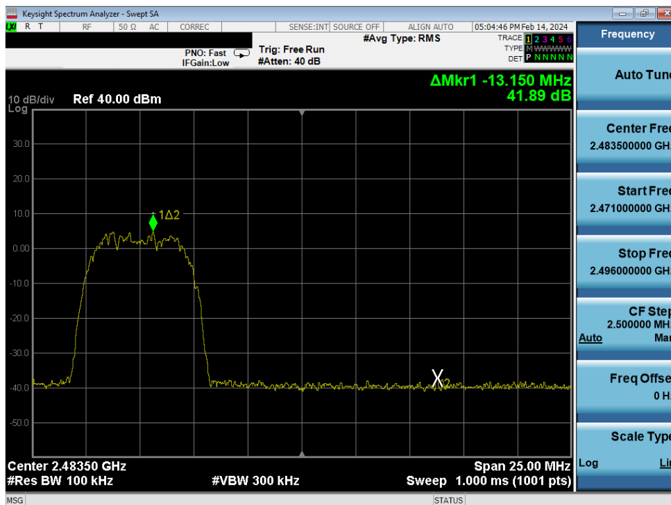
Plot 7-90. Band Edge Plot Antenna WF9 (Bluetooth (HDR8), ePA – Ch. 73)
