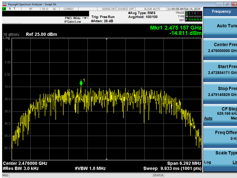
Plot 7-77. Power Spectral Density Plot Tx BF Antenna WF8 (Bluetooth (HDR8), 8Mbps, iPA – Ch. 73)
