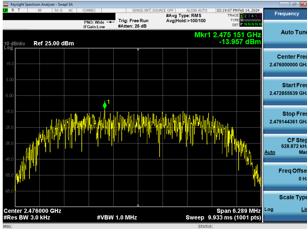
Plot 7-78. Power Spectral Density Plot Tx BF Antenna WF7 (Bluetooth (HDR8), 8Mbps, iPA – Ch. 73)
