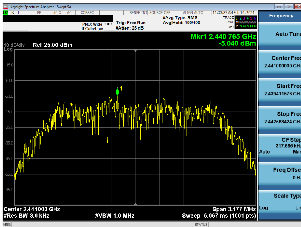
Plot 7-20. Power Spectral Density Plot Antenna WF8 (Bluetooth (HDR4), 4Mbps, ePA – Ch. 38)
