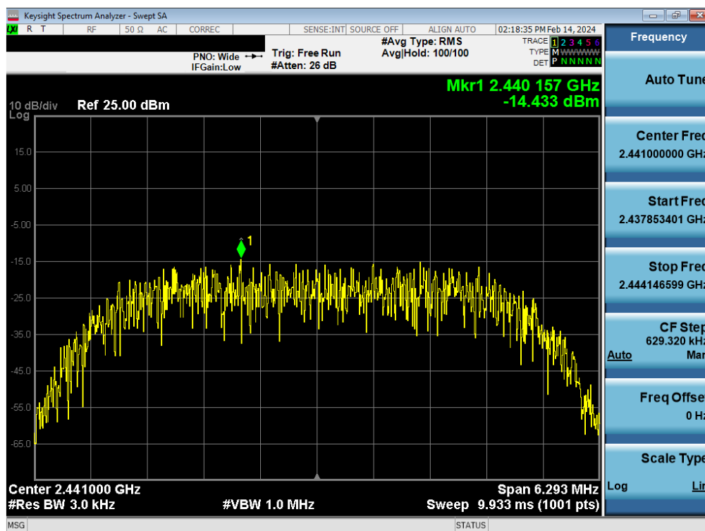
Plot 7-76. Power Spectral Density Plot Tx BF Antenna WF7 (Bluetooth (HDR8), 8Mbps, iPA – Ch. 38)
