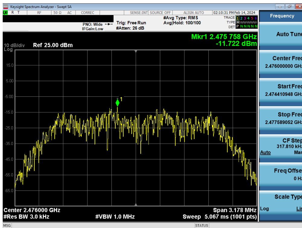
Plot 7-36. Power Spectral Density Plot Antenna WF7 (Bluetooth (HDR4), 4Mbps, iPA – Ch. 73)
