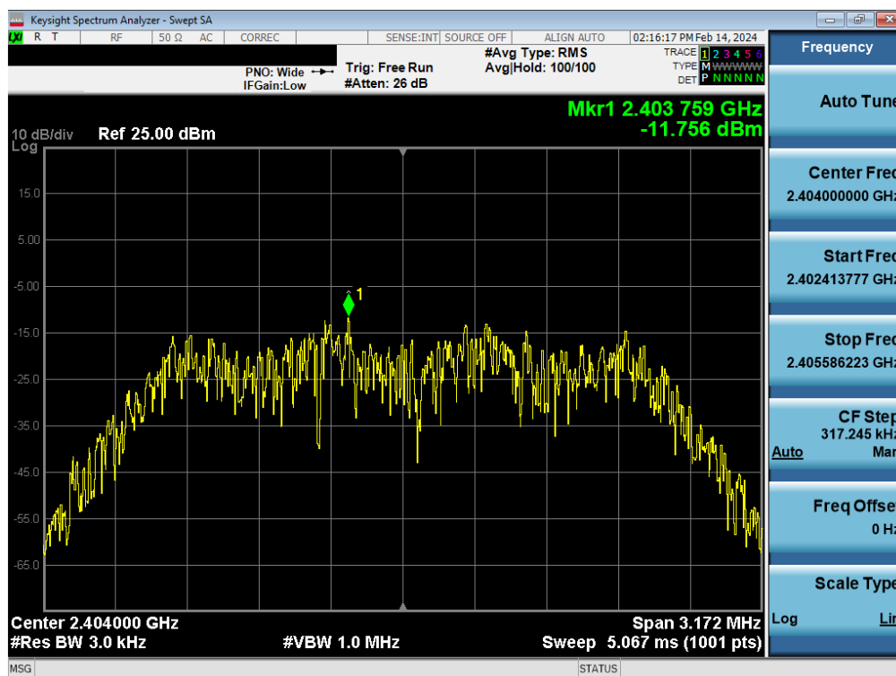
Plot 7-62. Power Spectral Density Plot Tx BF Antenna WF7 (Bluetooth (HDR4), 4Mbps, iPA – Ch. 1)
