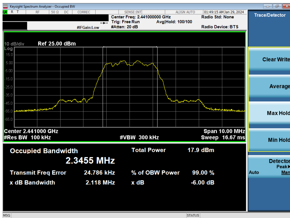
Plot 7-2. 6dB BW & 99% OBW Plot Antenna WF8 (Bluetooth (HDR4), 4Mbps, ePA – Ch. 38)
