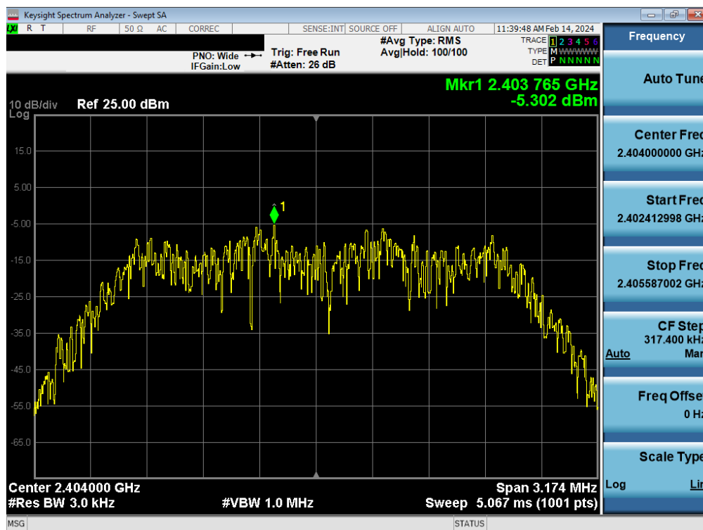
Plot 7-55. Power Spectral Density Plot Tx BF Antenna WF8 (Bluetooth (HDR4), 4Mbps, ePA – Ch. 1)
