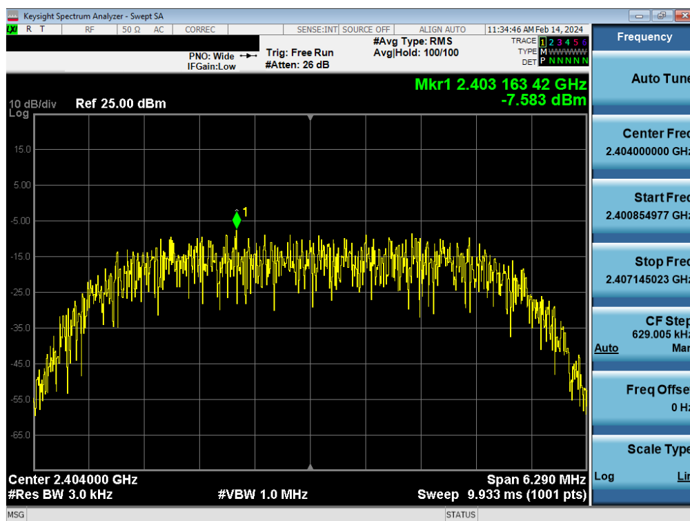
Plot 7-25. Power Spectral Density Plot Antenna WF8 (Bluetooth (HDR8), 8Mbps, ePA – Ch. 1)
