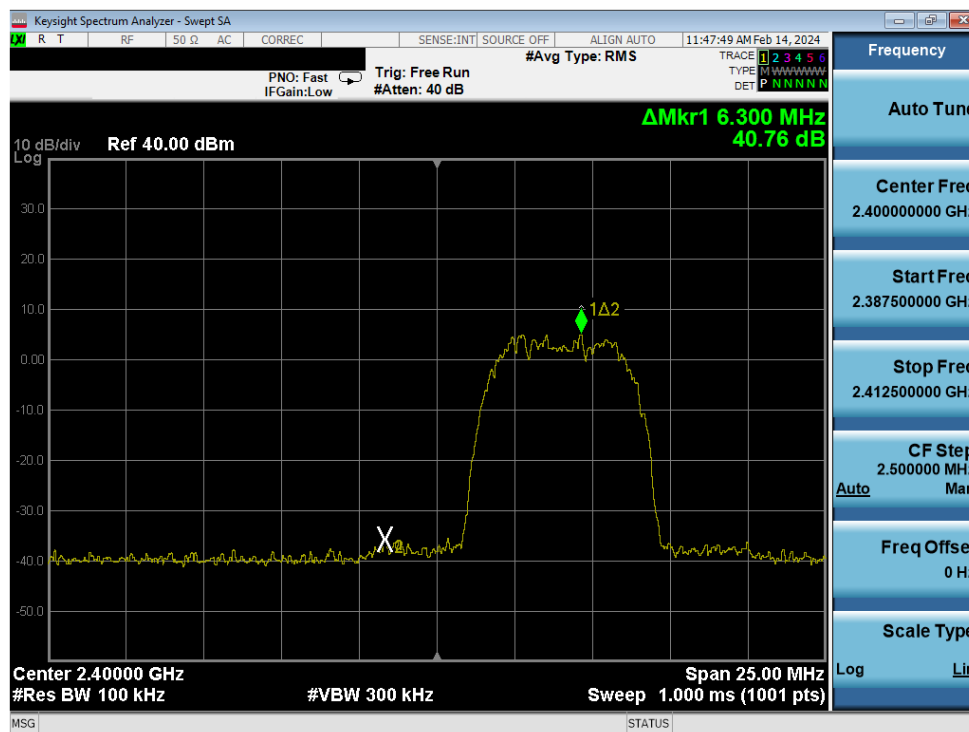
Plot 7-81. Band Edge Plot Antenna WF8 (Bluetooth (HDR8), ePA – Ch. 1)
