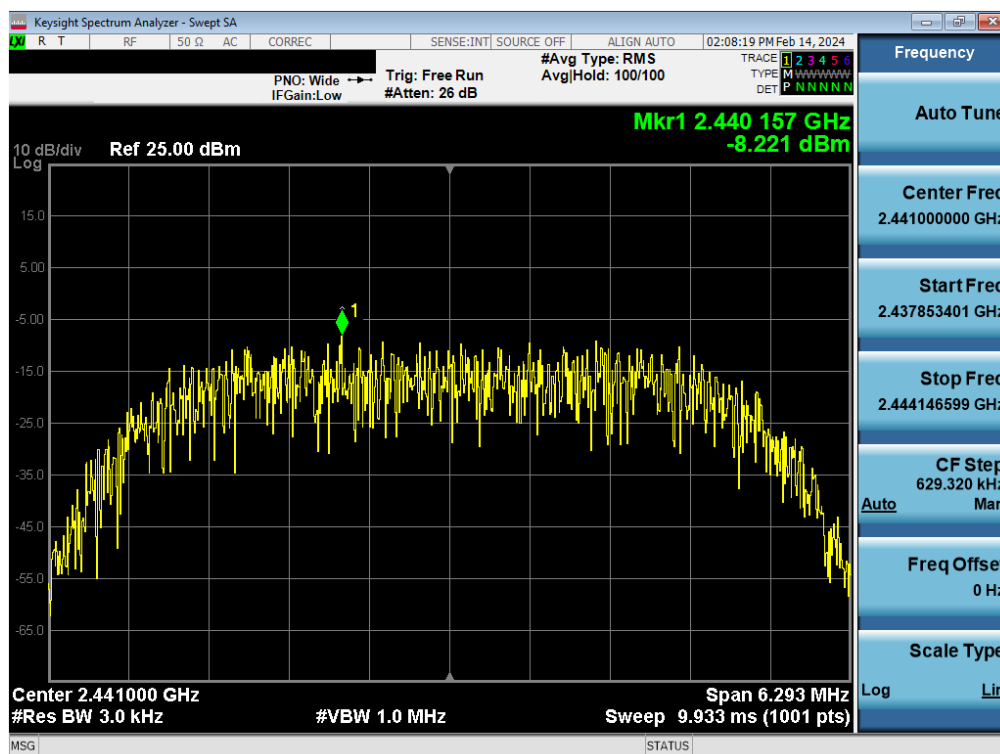
Plot 7-38. Power Spectral Density Plot Antenna WF7 (Bluetooth (HDR8), 8Mbps, ePA – Ch. 38)
