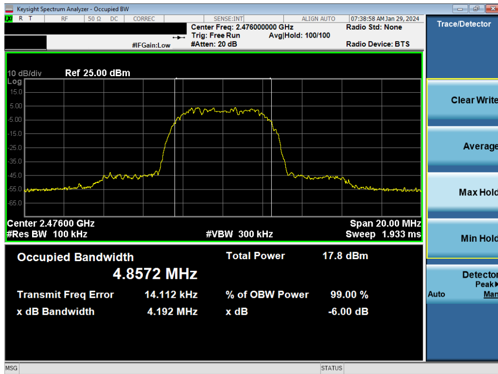
Plot 7-12. 6dB BW & 99% OBW Plot Antenna WF7 (Bluetooth (HDR8), 8Mbps, ePA – Ch. 73)
