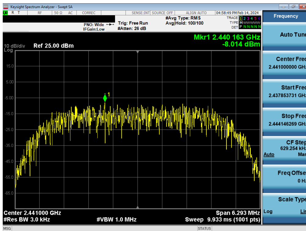
Plot 7-50. Power Spectral Density Plot Antenna WF9 (Bluetooth (HDR8), 8Mbps, ePA – Ch. 38)
