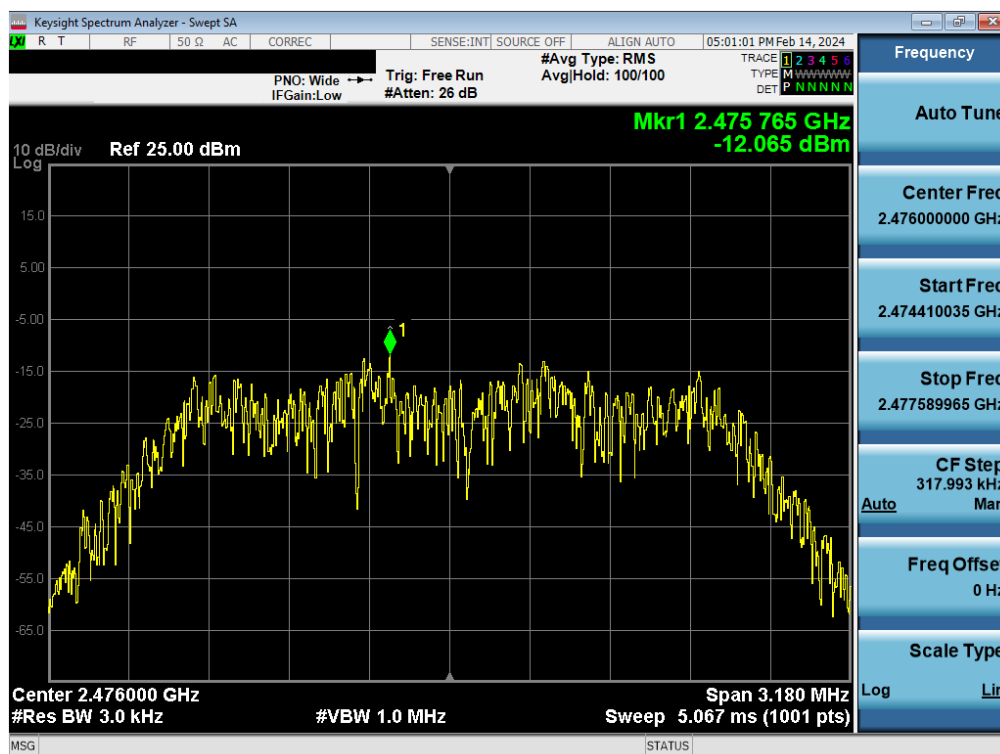
Plot 7-48. Power Spectral Density Plot Antenna WF9 (Bluetooth (HDR4), 4Mbps, iPA – Ch. 73)
