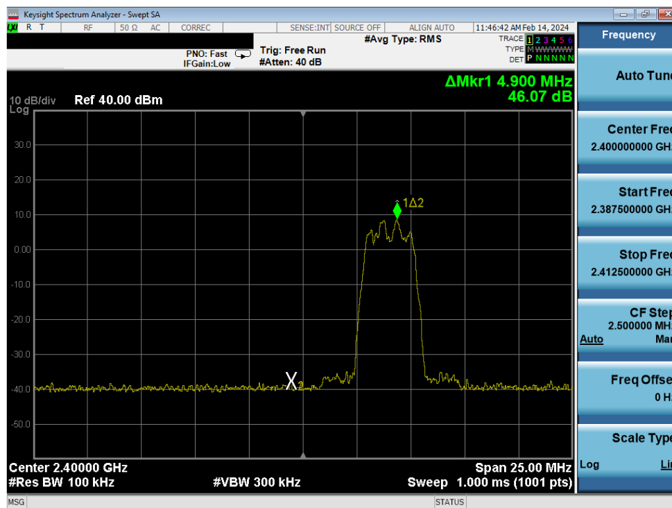
Plot 7-79. Band Edge Plot Antenna WF8 (Bluetooth (HDR4), ePA – Ch. 1)
