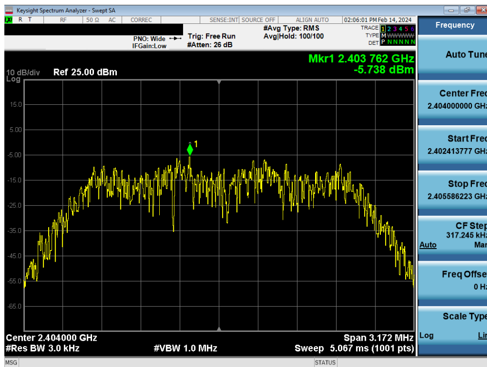
Plot 7-31. Power Spectral Density Plot Antenna WF7 (Bluetooth (HDR4), 4Mbps, ePA – Ch. 1)
