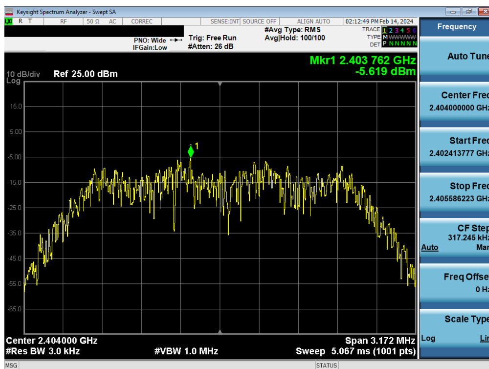
Plot 7-56. Power Spectral Density Plot Tx BF Antenna WF7 (Bluetooth (HDR4), 4Mbps, ePA – Ch. 1)
