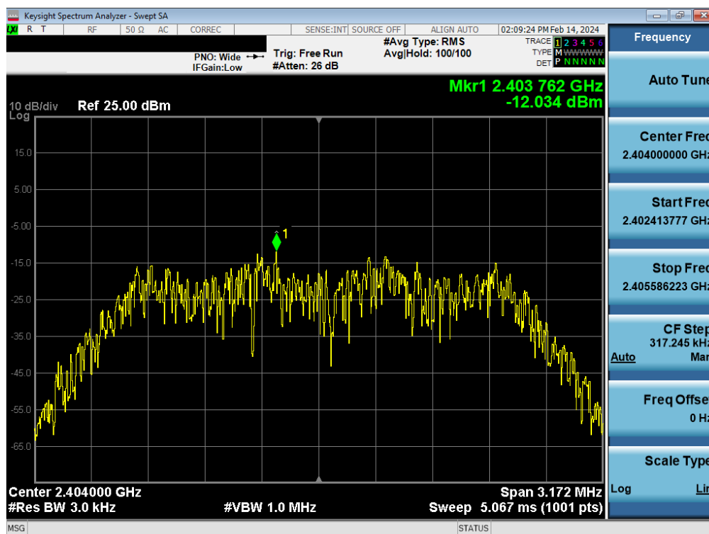
Plot 7-34. Power Spectral Density Plot Antenna WF7 (Bluetooth (HDR4), 4Mbps, iPA – Ch. 1)
