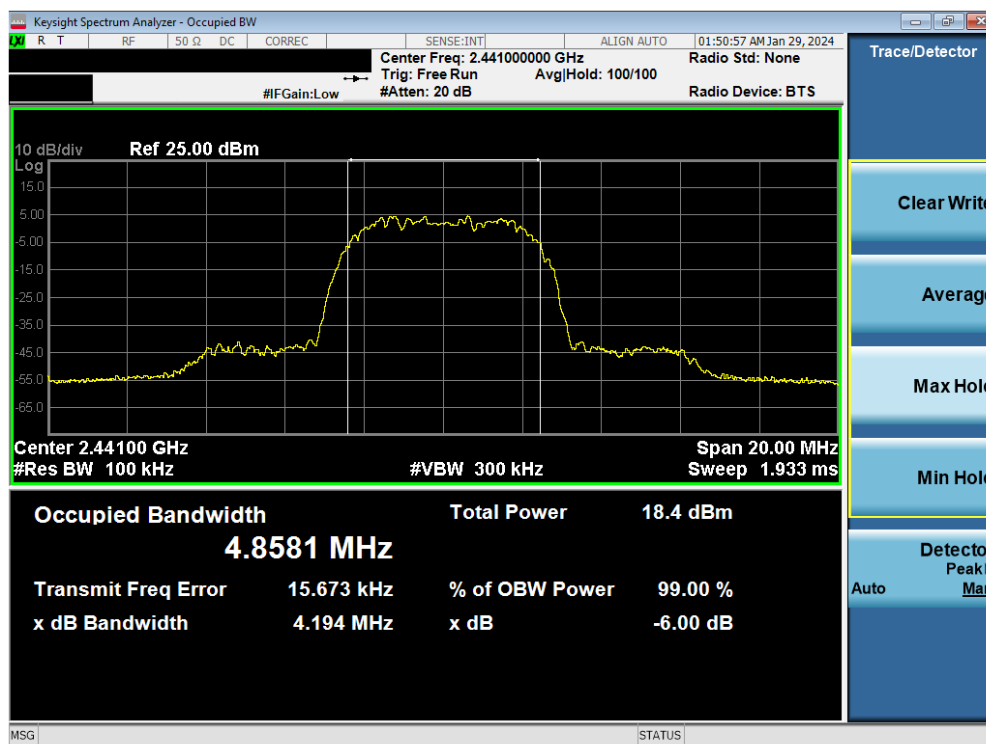
Plot 7-5. 6dB BW & 99% OBW Plot Antenna WF8 (Bluetooth (HDR8), 8Mbps, ePA – Ch. 38)
