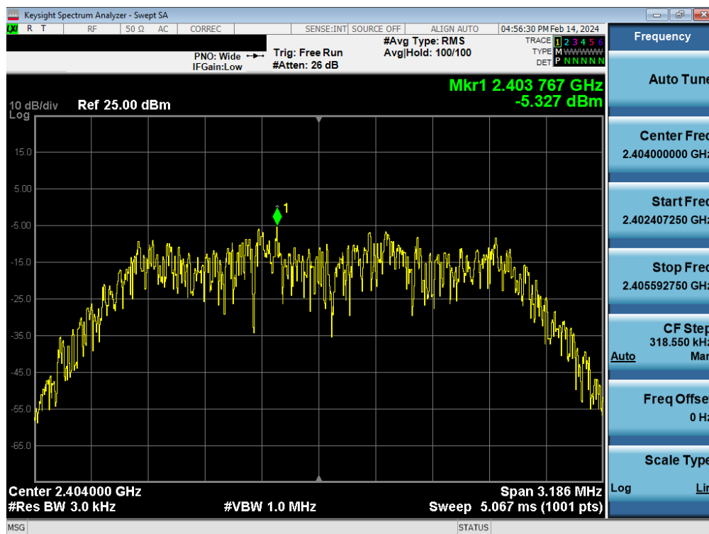
Plot 7-43. Power Spectral Density Plot Antenna WF9 (Bluetooth (HDR4), 4Mbps, ePA – Ch. 1)
