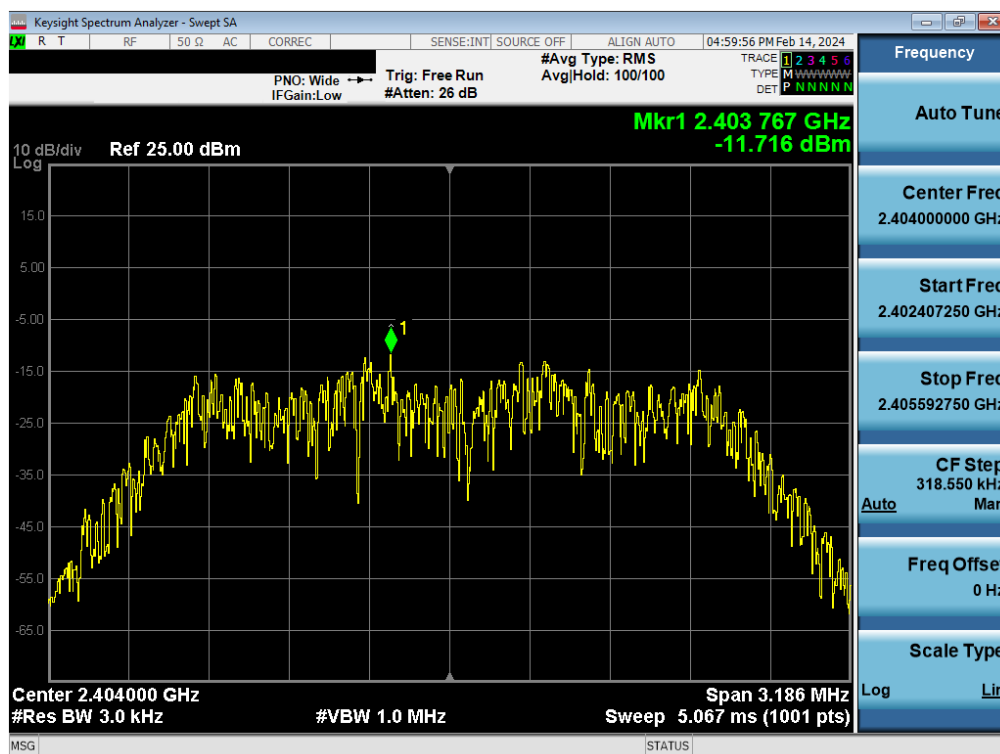
Plot 7-46. Power Spectral Density Plot Antenna WF9 (Bluetooth (HDR4), 4Mbps, iPA – Ch. 1)
