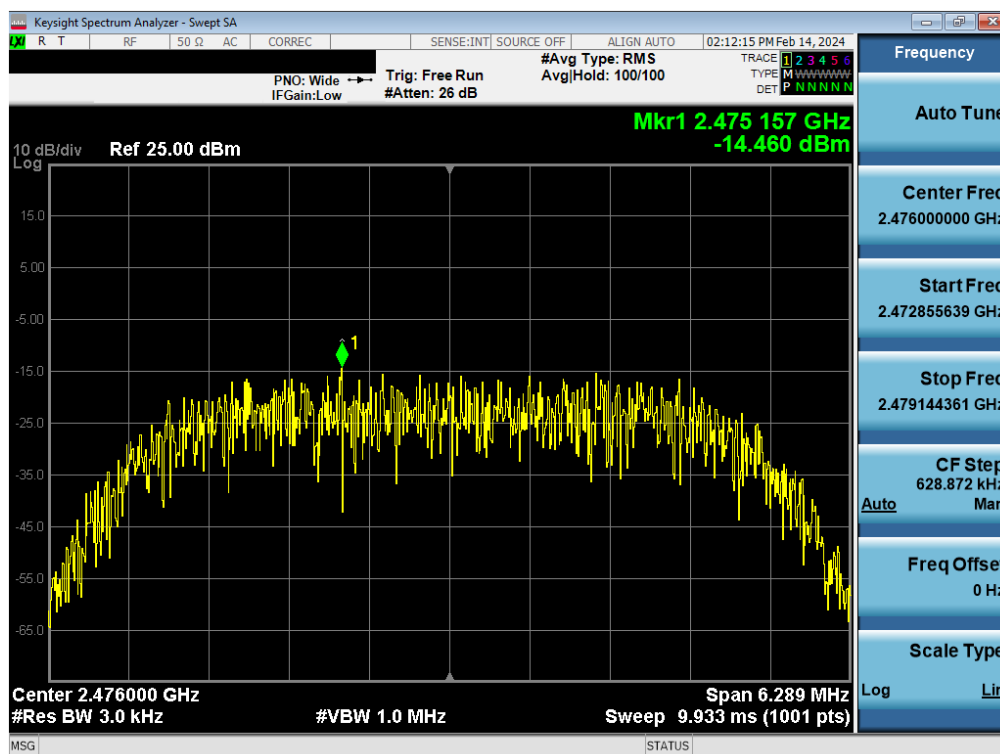
Plot 7-42. Power Spectral Density Plot Antenna WF7 (Bluetooth (HDR8), 8Mbps, iPA – Ch. 73)
