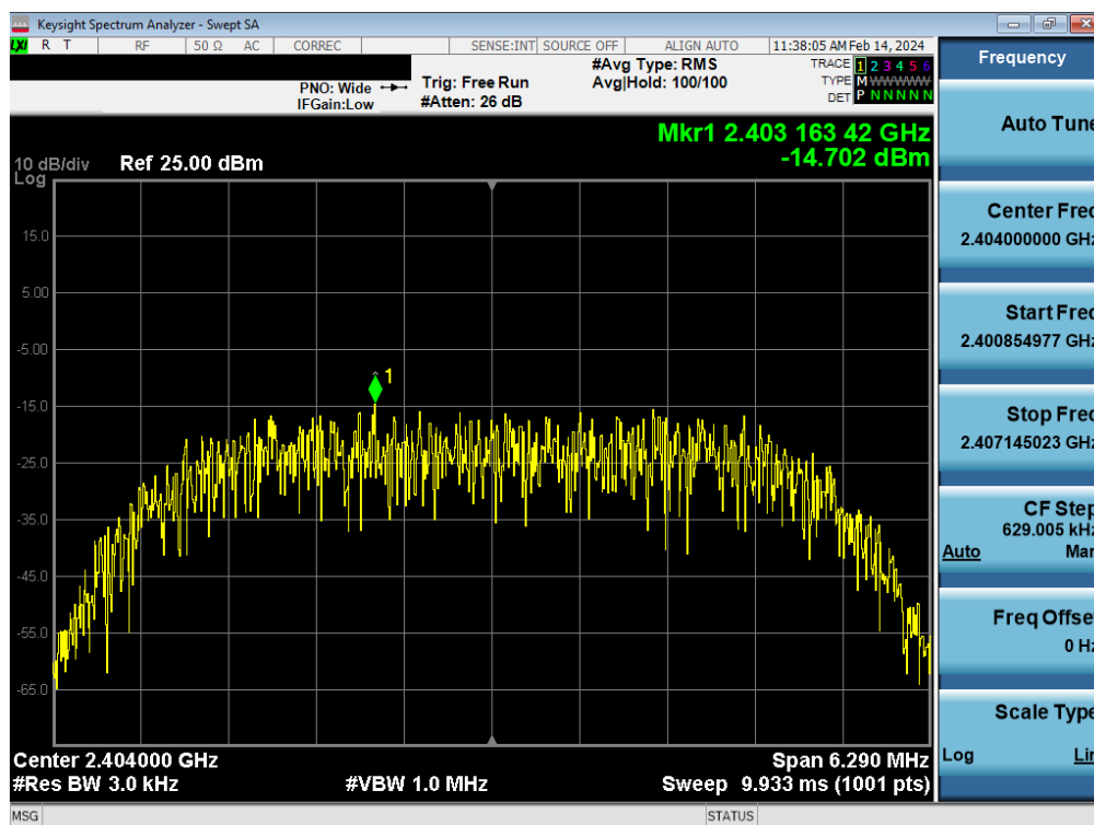
Plot 7-28. Power Spectral Density Plot Antenna WF8 (Bluetooth (HDR8), 8Mbps, iPA – Ch. 1)
