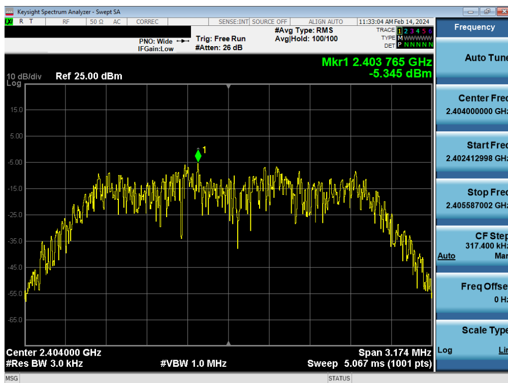
Plot 7-19. Power Spectral Density Plot Antenna WF8 (Bluetooth (HDR4), 4Mbps, ePA – Ch. 1)
