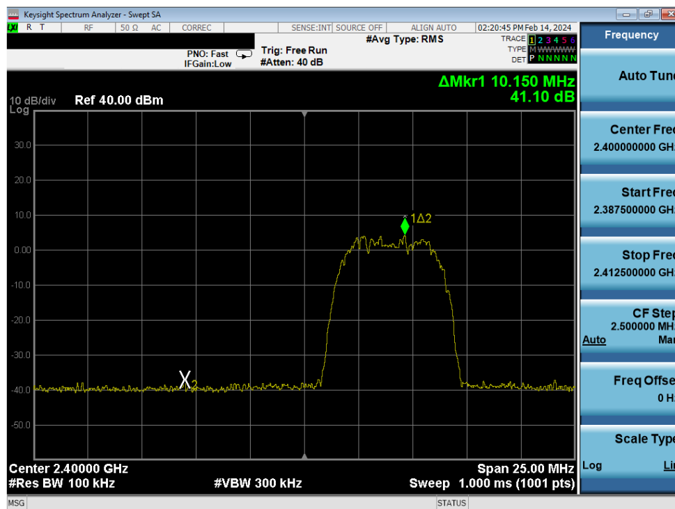
Plot 7-85. Band Edge Plot Antenna WF7 (Bluetooth (HDR8), ePA – Ch. 1)
