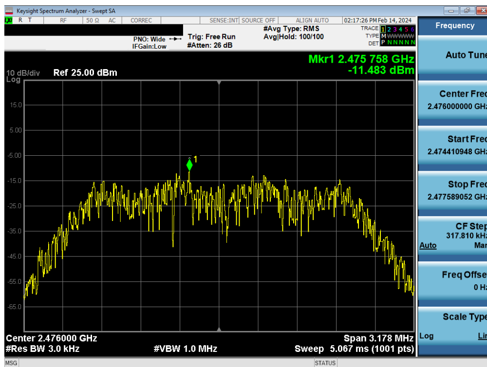
Plot 7-66. Power Spectral Density Plot Tx BF Antenna WF7 (Bluetooth (HDR4), 4Mbps, iPA – Ch. 73)
