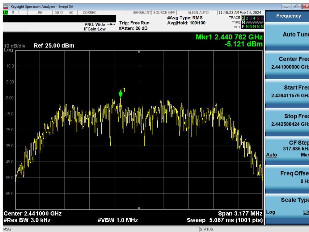
Plot 7-57. Power Spectral Density Plot Tx BF Antenna WF8 (Bluetooth (HDR4), 4Mbps, ePA – Ch. 38)
