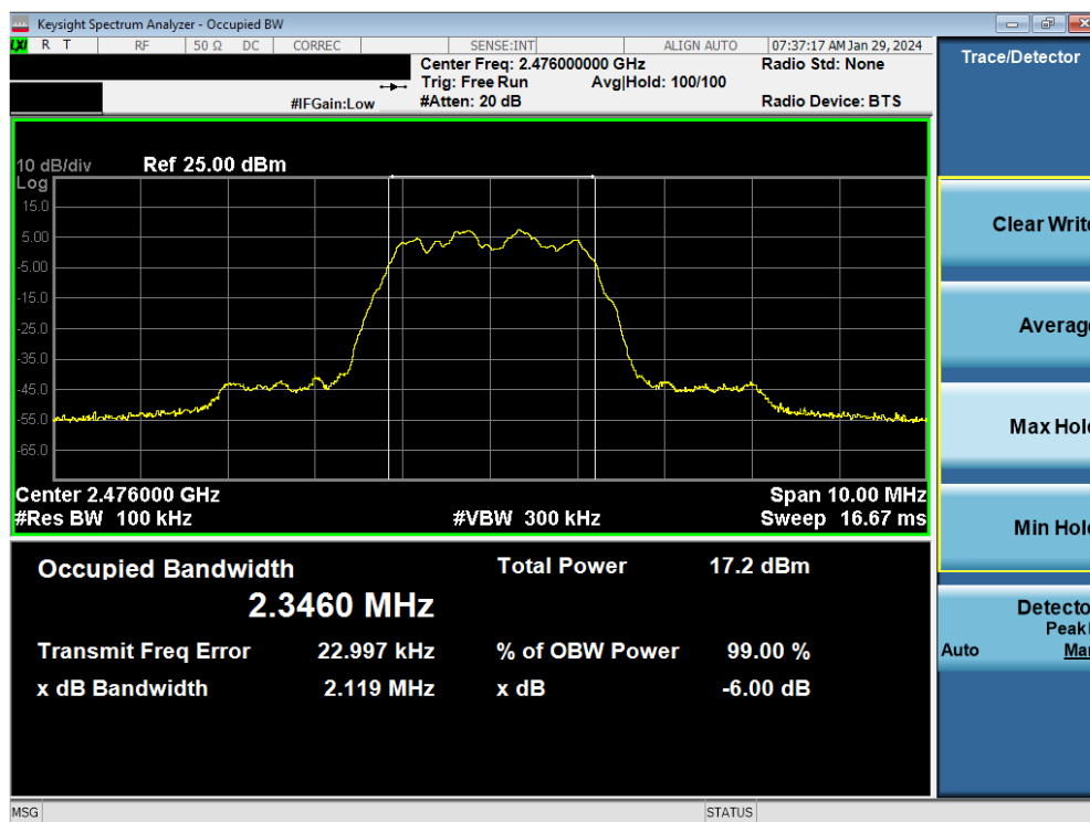
Plot 7-9. 6dB BW & 99% OBW Plot Antenna WF7 (Bluetooth (HDR4), 4Mbps, ePA – Ch. 73)
