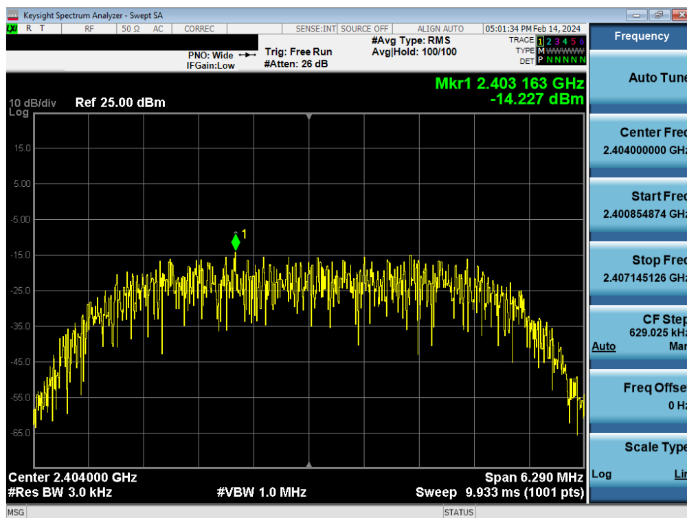
Plot 7-52. Power Spectral Density Plot Antenna WF9 (Bluetooth (HDR8), 8Mbps, iPA – Ch. 1)
