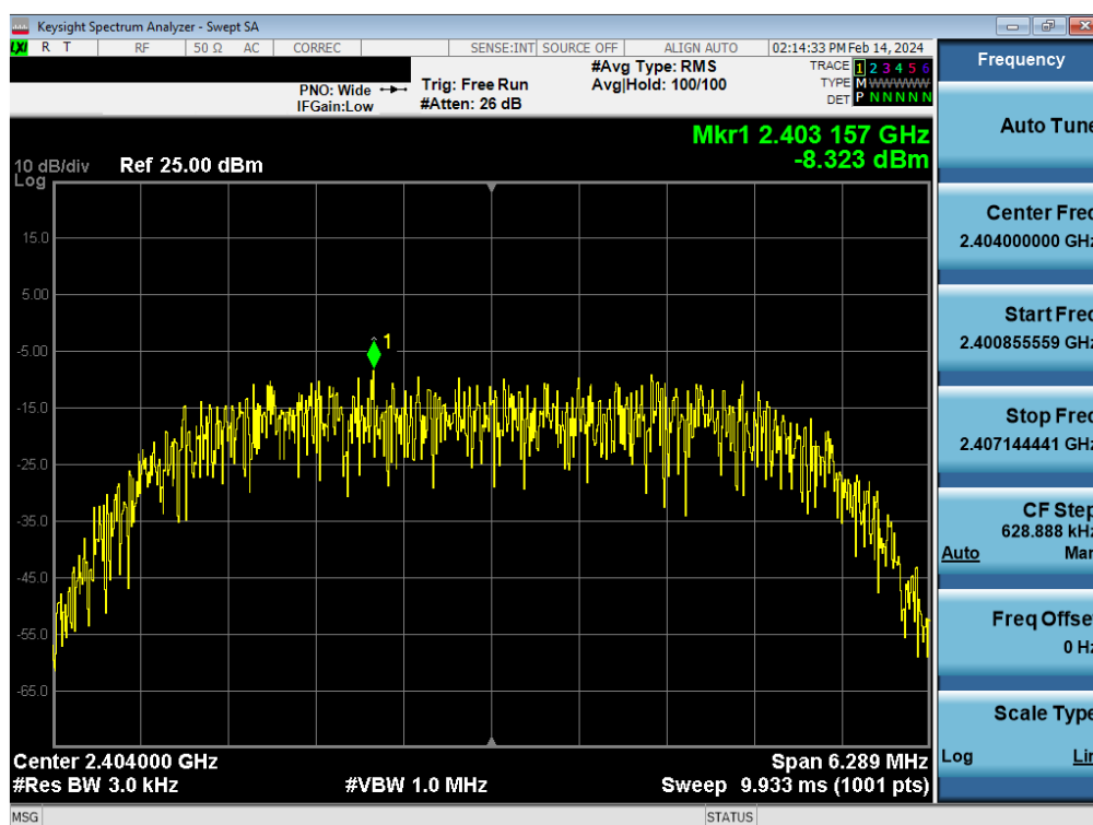
Plot 7-68. Power Spectral Density Plot Tx BF Antenna WF7 (Bluetooth (HDR8), 8Mbps, ePA – Ch. 1)
