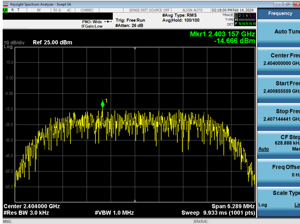
Plot 7-74. Power Spectral Density Plot Tx BF Antenna WF7 (Bluetooth (HDR8), 8Mbps, iPA – Ch. 1)
