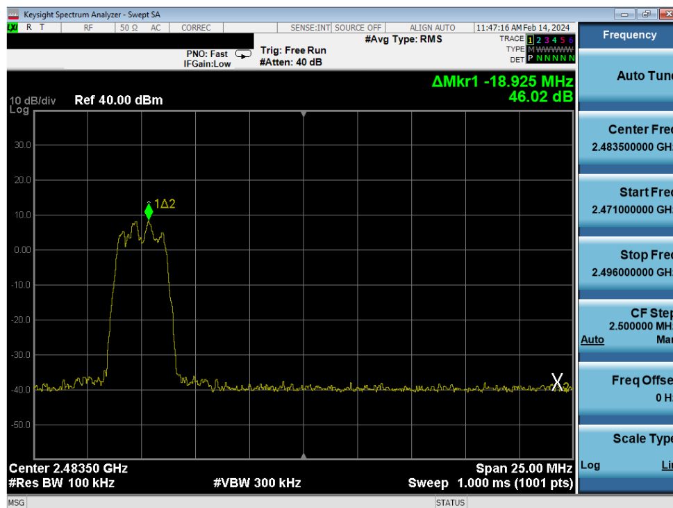
Plot 7-80. Band Edge Plot Antenna WF8 (Bluetooth (HDR4), ePA – Ch. 73)
