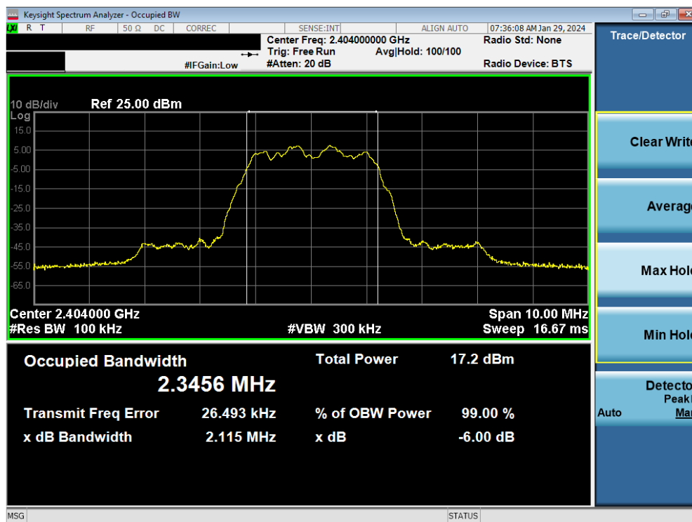
Plot 7-7. 6dB BW & 99% OBW Plot Antenna WF7 (Bluetooth (HDR4), 4Mbps, ePA – Ch. 1)
