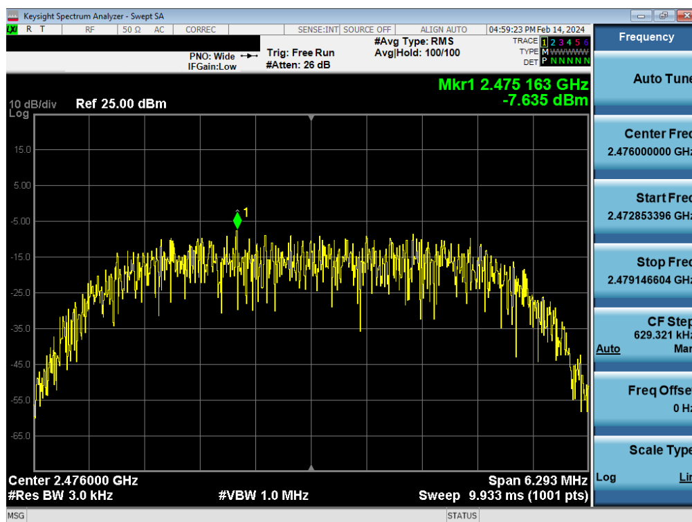
Plot 7-51. Power Spectral Density Plot Antenna WF9 (Bluetooth (HDR8), 8Mbps, ePA – Ch. 73)
