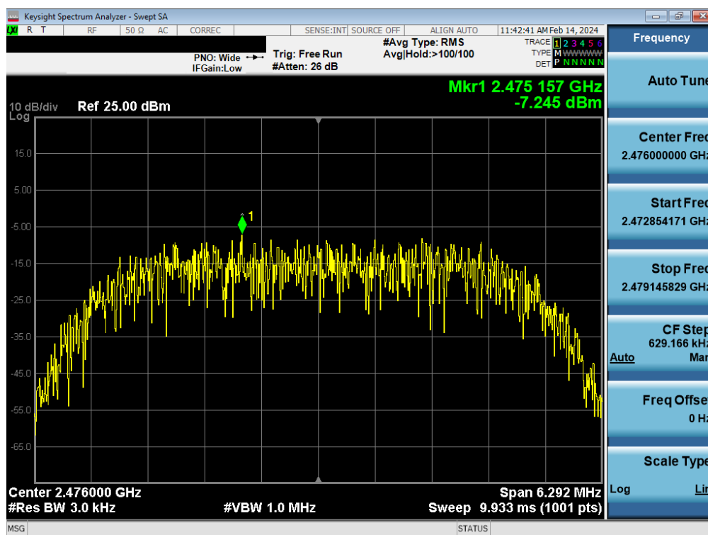
Plot 7-71. Power Spectral Density Plot Tx BF Antenna WF8 (Bluetooth (HDR8), 8Mbps, ePA – Ch. 73)
