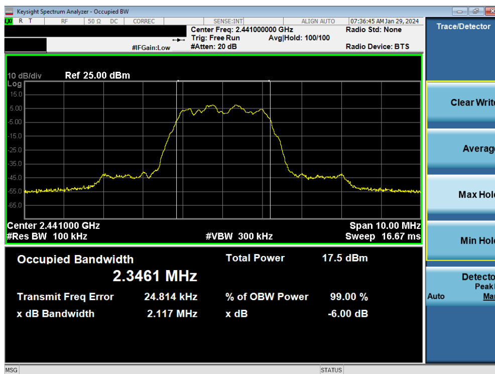
Plot 7-8. 6dB BW & 99% OBW Plot Antenna WF7 (Bluetooth (HDR4), 4Mbps, ePA – Ch. 38)
