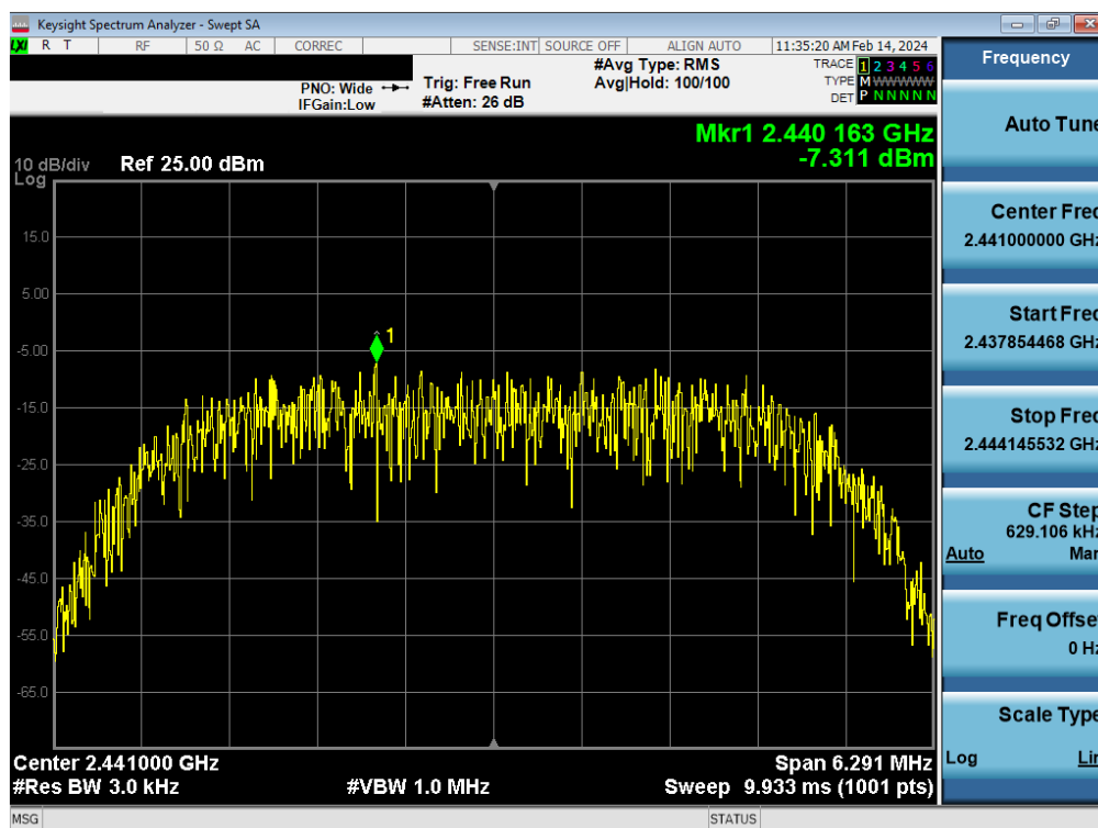
Plot 7-26. Power Spectral Density Plot Antenna WF8 (Bluetooth (HDR8), 8Mbps, ePA – Ch. 38)
