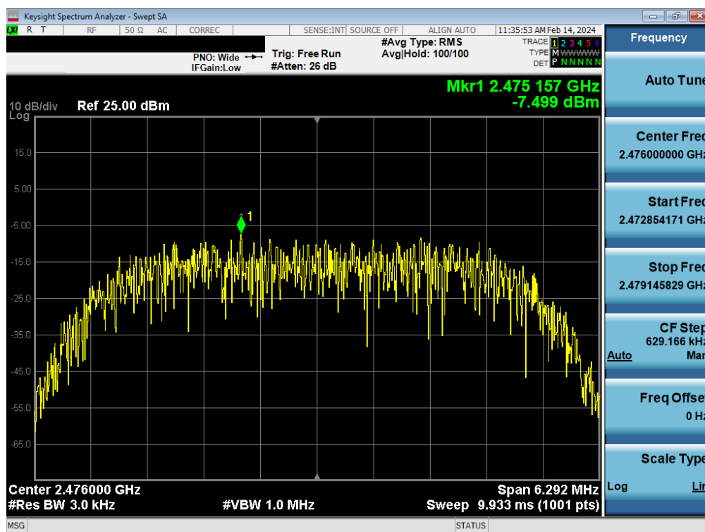
Plot 7-27. Power Spectral Density Plot Antenna WF8 (Bluetooth (HDR8), 8Mbps, ePA – Ch. 73)
