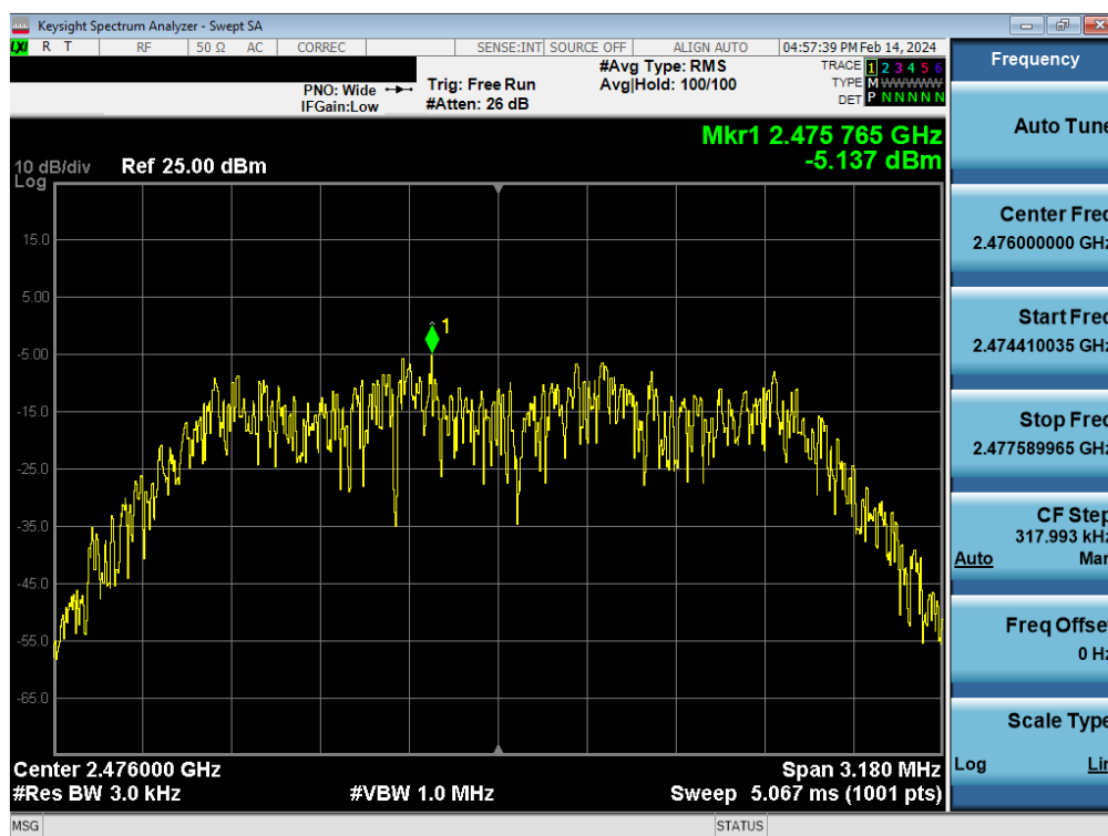
Plot 7-45. Power Spectral Density Plot Antenna WF9 (Bluetooth (HDR4), 4Mbps, ePA – Ch. 73)
