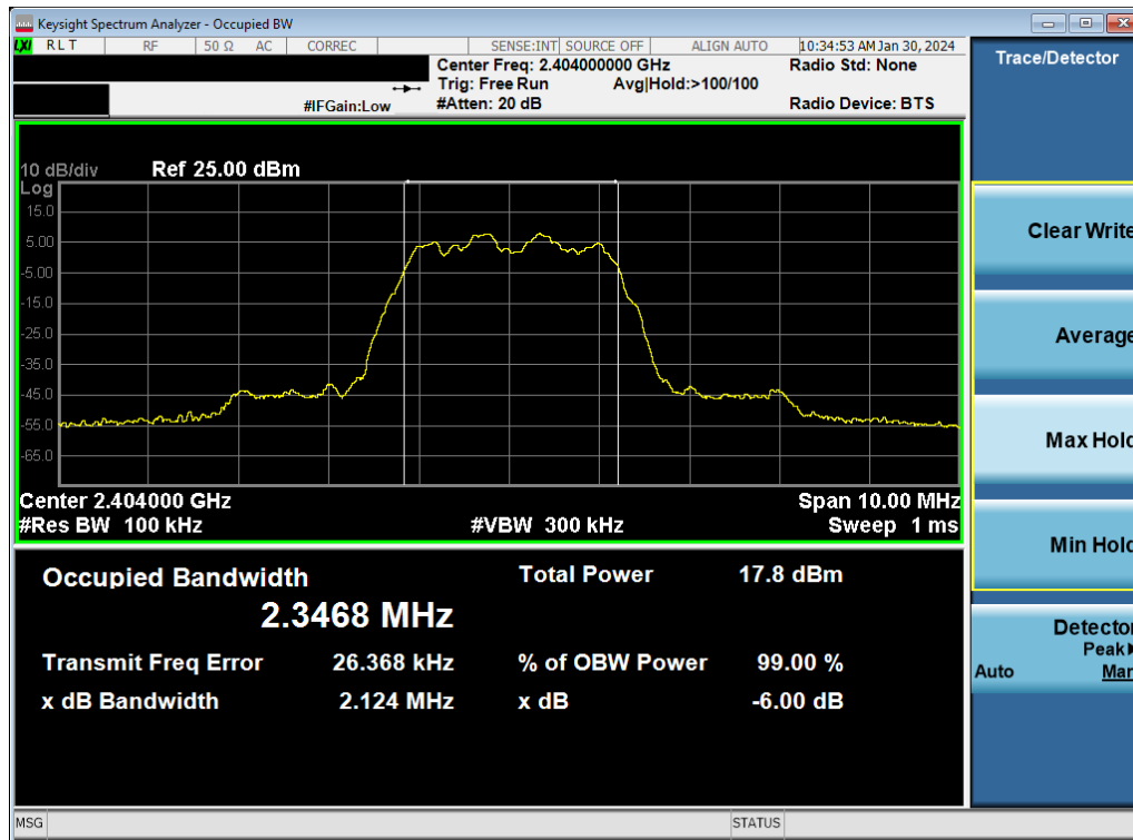
Plot 7-13. 6dB BW & 99% OBW Plot Antenna WF9 (Bluetooth (HDR4), 4Mbps, ePA – Ch. 1)
