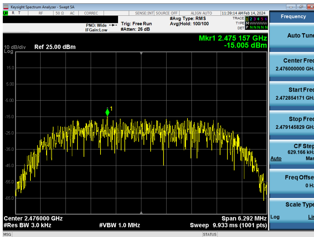
Plot 7-30. Power Spectral Density Plot Antenna WF8 (Bluetooth (HDR8), 8Mbps, iPA – Ch. 73)
