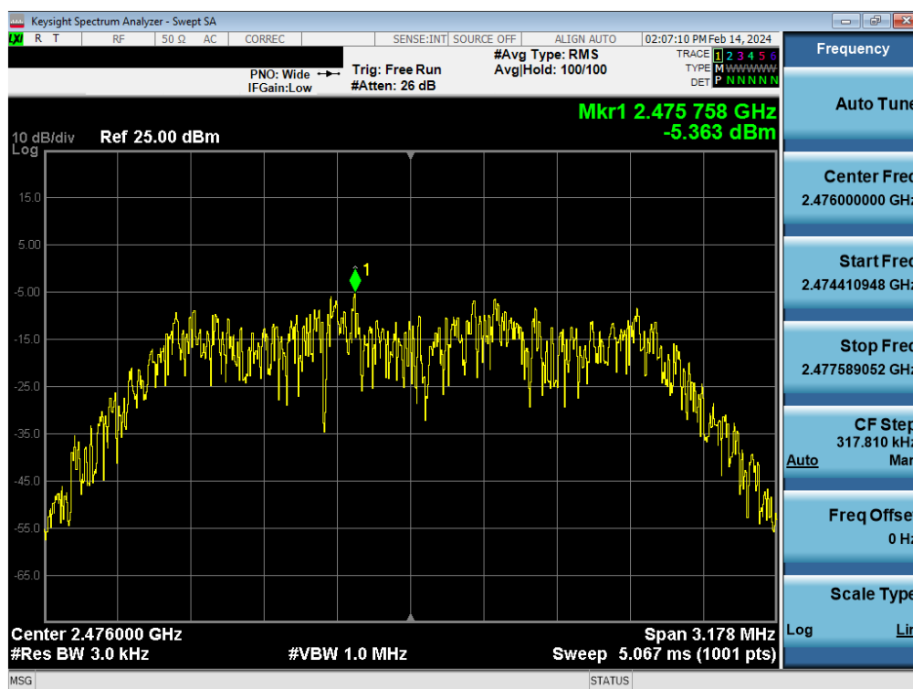
Plot 7-33. Power Spectral Density Plot Antenna WF7 (Bluetooth (HDR4), 4Mbps, ePA – Ch. 73)
