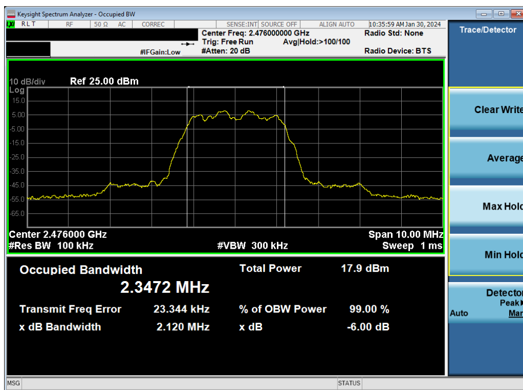
Plot 7-15. 6dB BW & 99% OBW Plot Antenna WF9 (Bluetooth (HDR4), 4Mbps, ePA – Ch. 73)
