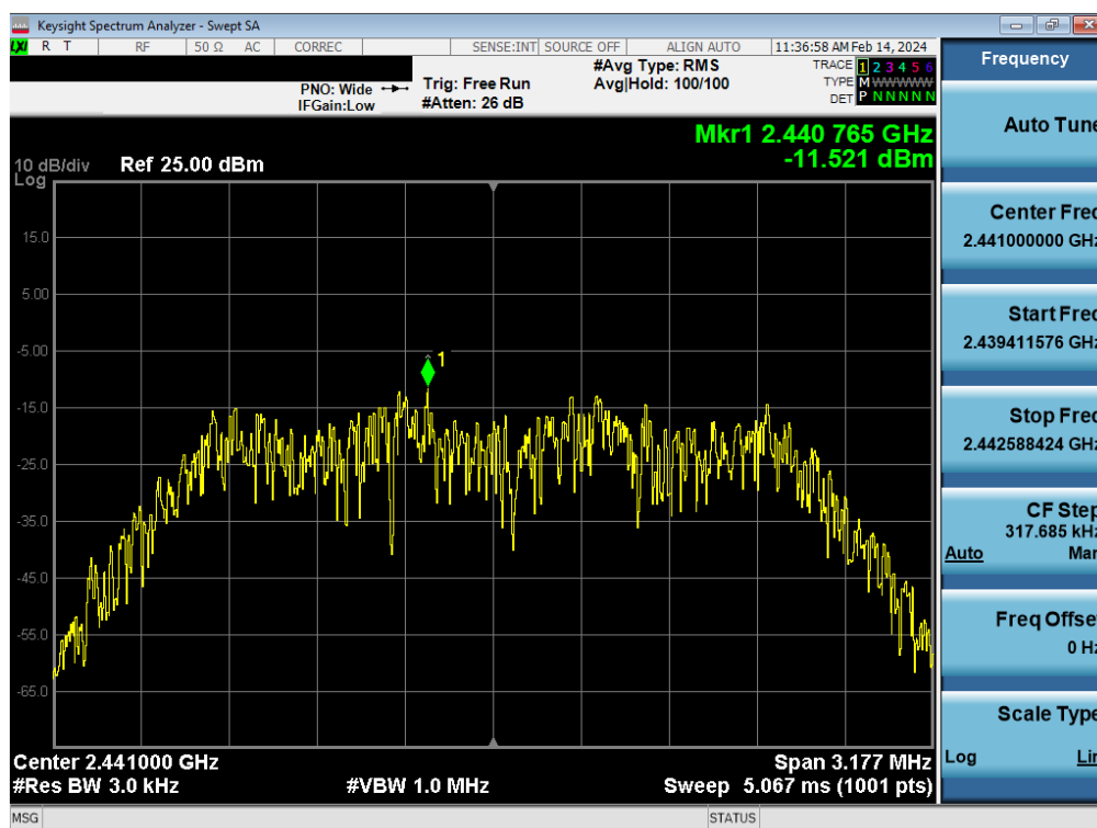
Plot 7-23. Power Spectral Density Plot Antenna WF8 (Bluetooth (HDR4), 4Mbps, iPA – Ch. 38)
