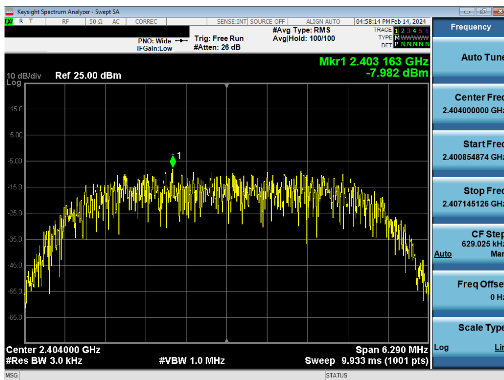
Plot 7-49. Power Spectral Density Plot Antenna WF9 (Bluetooth (HDR8), 8Mbps, ePA – Ch. 1)
