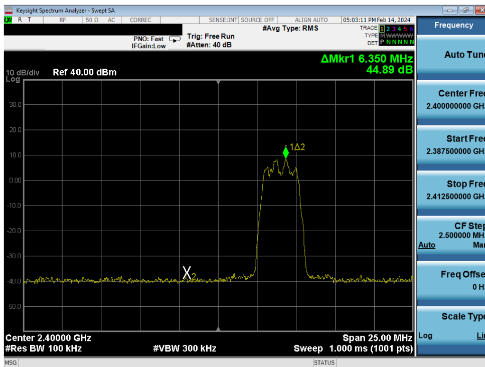
Plot 7-87. Band Edge Plot Antenna WF9 (Bluetooth (HDR4), ePA – Ch. 1)
