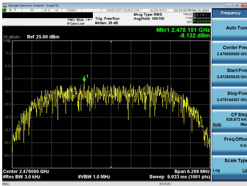
Plot 7-72. Power Spectral Density Plot Tx BF Antenna WF7 (Bluetooth (HDR8), 8Mbps, ePA – Ch. 73)
