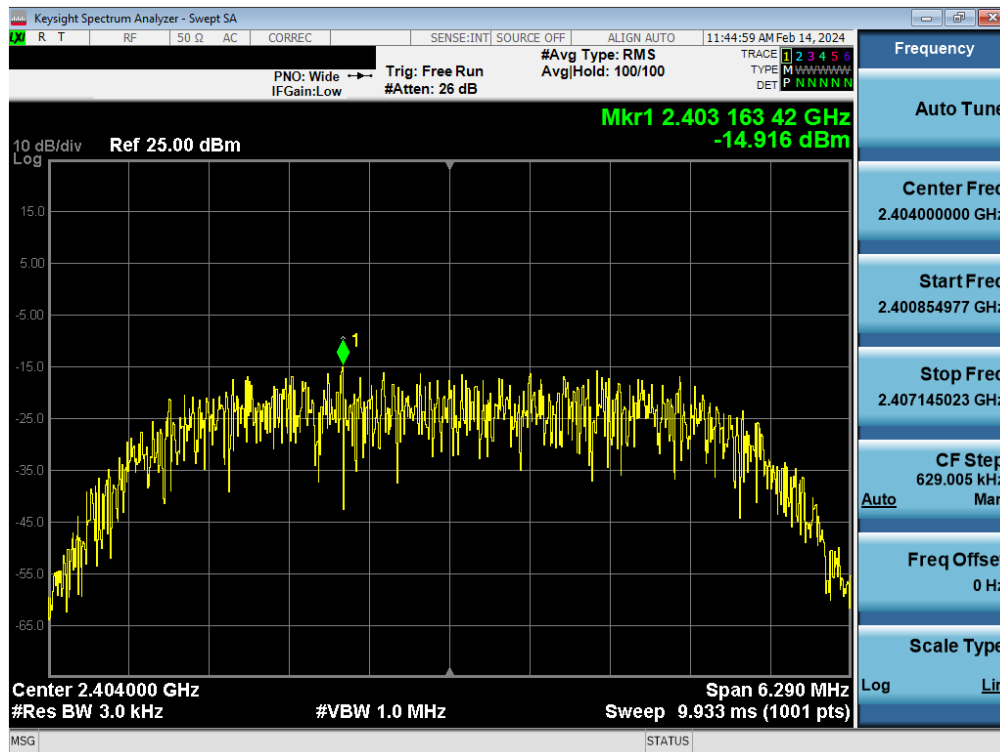
Plot 7-73. Power Spectral Density Plot Tx BF Antenna WF8 (Bluetooth (HDR8), 8Mbps, iPA – Ch. 1)
