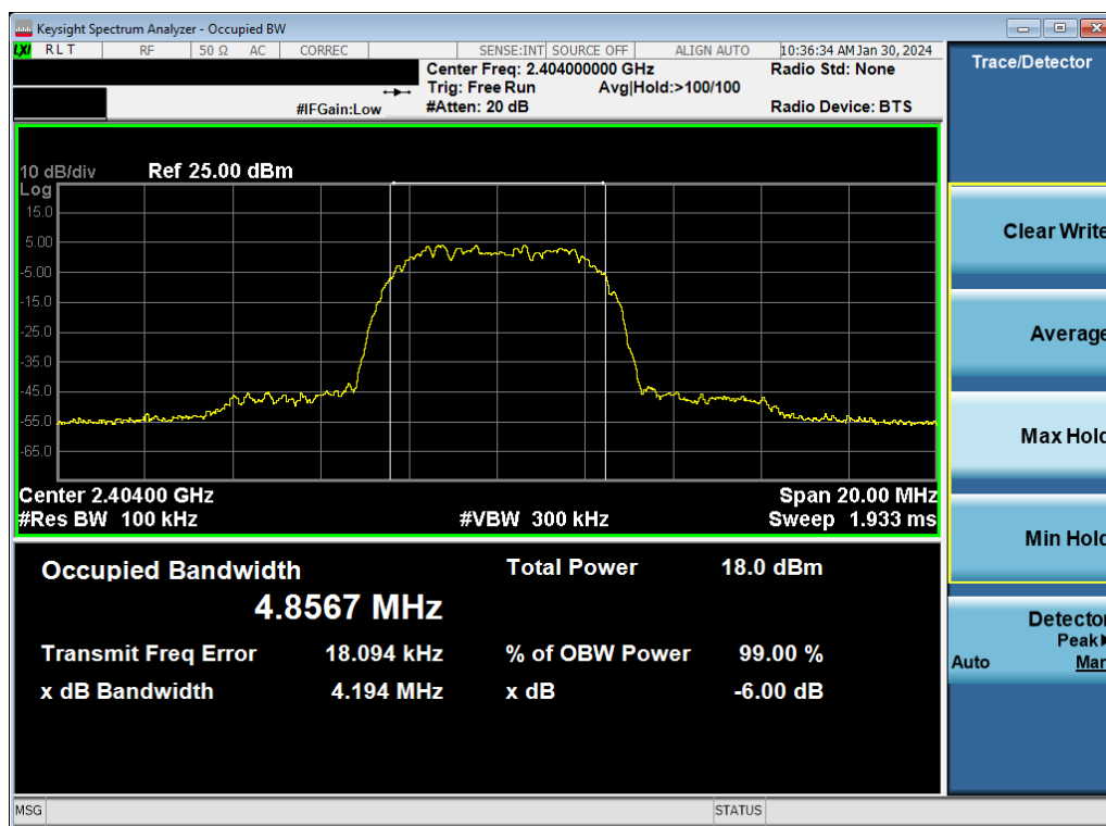
Plot 7-16. 6dB BW & 99% OBW Plot Antenna WF9 (Bluetooth (HDR8), 8Mbps, ePA – Ch. 1)
