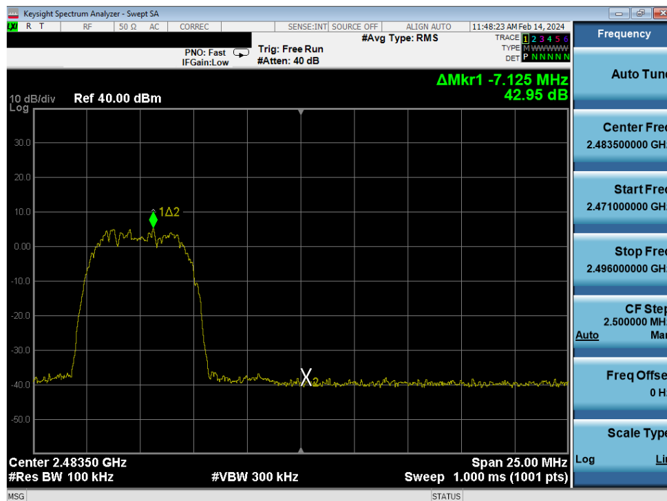
Plot 7-82. Band Edge Plot Antenna WF8 (Bluetooth (HDR8), ePA – Ch. 73)
