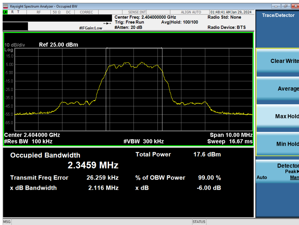
Plot 7-1. 6dB BW & 99% OBW Plot Antenna WF8 (Bluetooth (HDR4), 4Mbps, ePA – Ch. 1)
