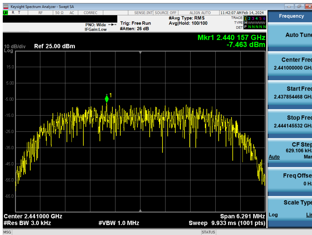
Plot 7-69. Power Spectral Density Plot Tx BF Antenna WF8 (Bluetooth (HDR8), 8Mbps, ePA – Ch. 38)
