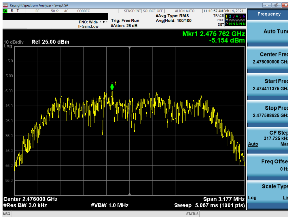
Plot 7-59. Power Spectral Density Plot Tx BF Antenna WF8 (Bluetooth (HDR4), 4Mbps, ePA – Ch. 73)
