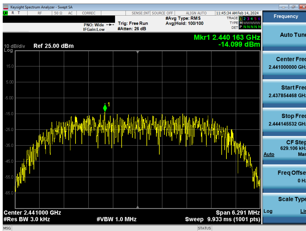
Plot 7-75. Power Spectral Density Plot Tx BF Antenna WF8 (Bluetooth (HDR8), 8Mbps, iPA – Ch. 38)
