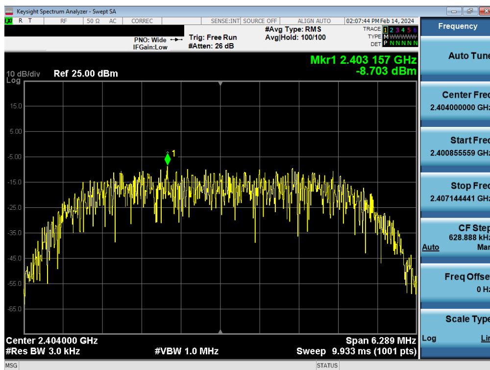
Plot 7-37. Power Spectral Density Plot Antenna WF7 (Bluetooth (HDR8), 8Mbps, ePA – Ch. 1)
