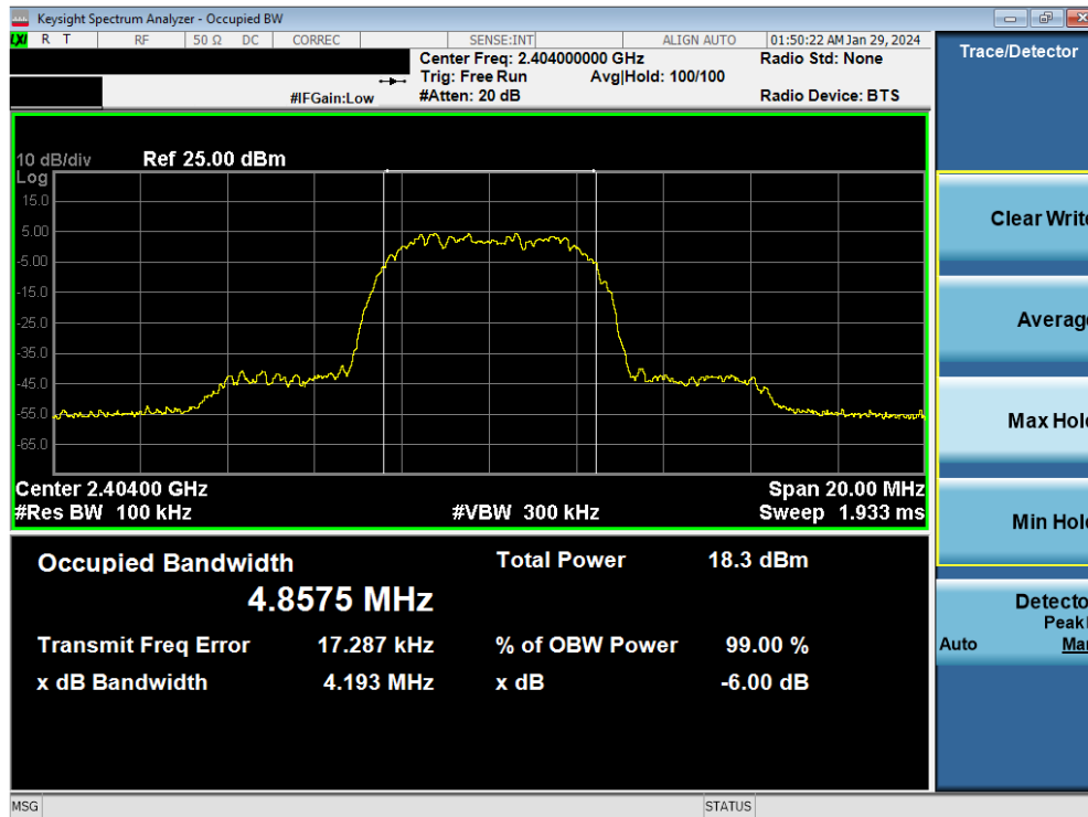
Plot 7-4. 6dB BW & 99% OBW Plot Antenna WF8 (Bluetooth (HDR8), 8Mbps, ePA – Ch. 1)
