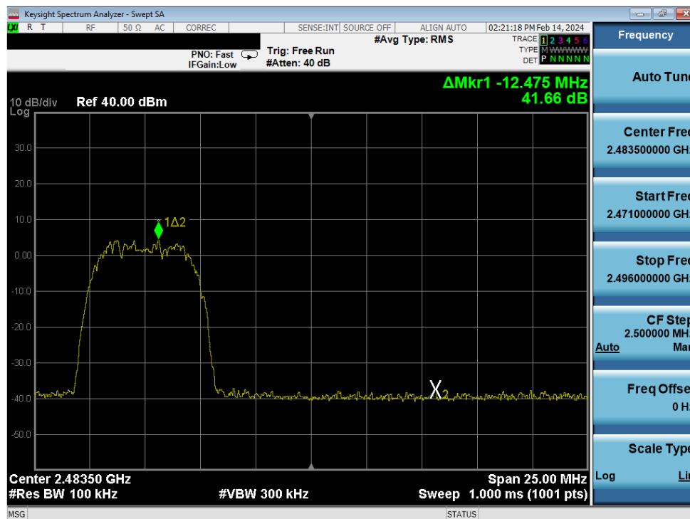
Plot 7-86. Band Edge Plot Antenna WF7 (Bluetooth (HDR8), ePA – Ch. 73)
