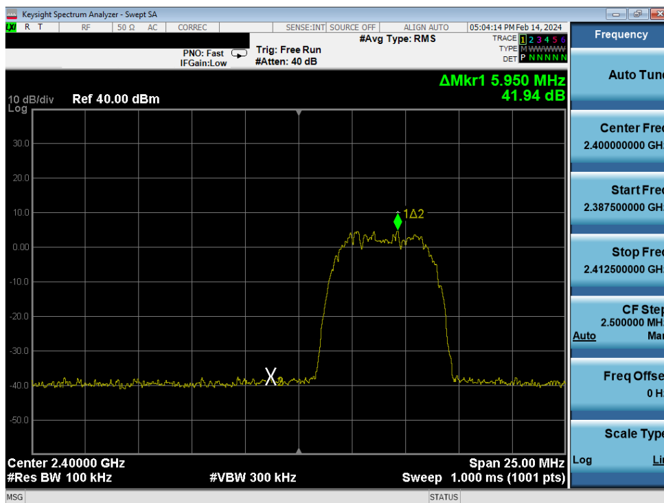
Plot 7-89. Band Edge Plot Antenna WF9 (Bluetooth (HDR8), ePA – Ch. 1)
