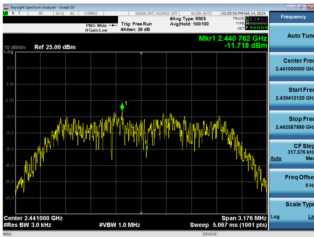
Plot 7-35. Power Spectral Density Plot Antenna WF7 (Bluetooth (HDR4), 4Mbps, iPA – Ch. 38)
