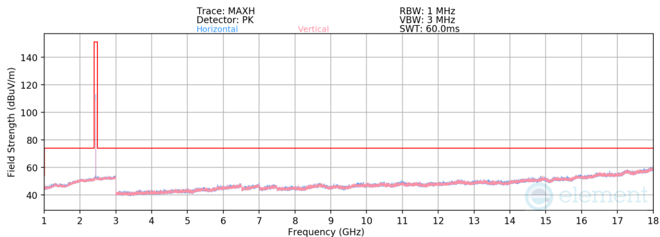
Plot 7-119. Radiated Spurious Emissions 1-18GHz TxBF (4Mbps, HDR4, ePA – Ch. 38)
