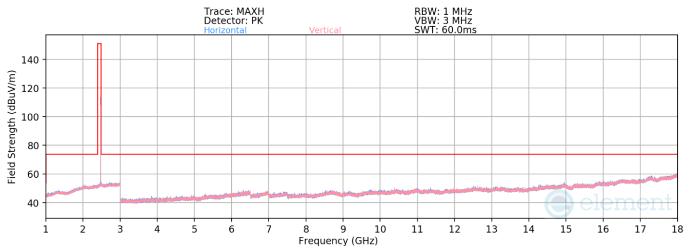
Plot 7-121. Radiated Spurious Emissions 1-18GHz TxBF (4Mbps, HDR4, ePA – Ch. 73)
