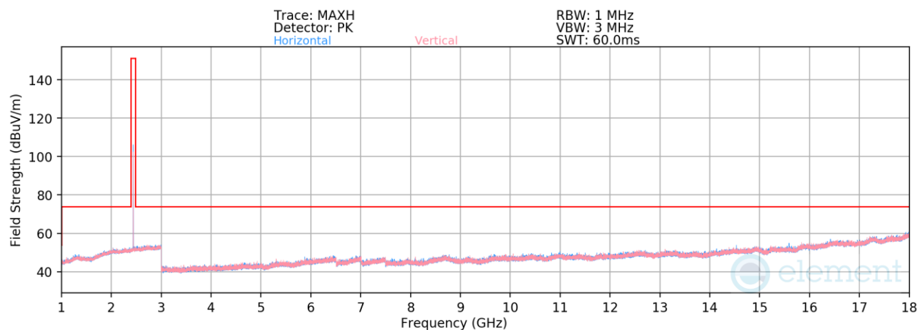
Plot 7-116. Radiated Spurious Emissions 1-18GHz Antenna WF9 (4Mbps, HDR4, ePA – Ch. 38)
