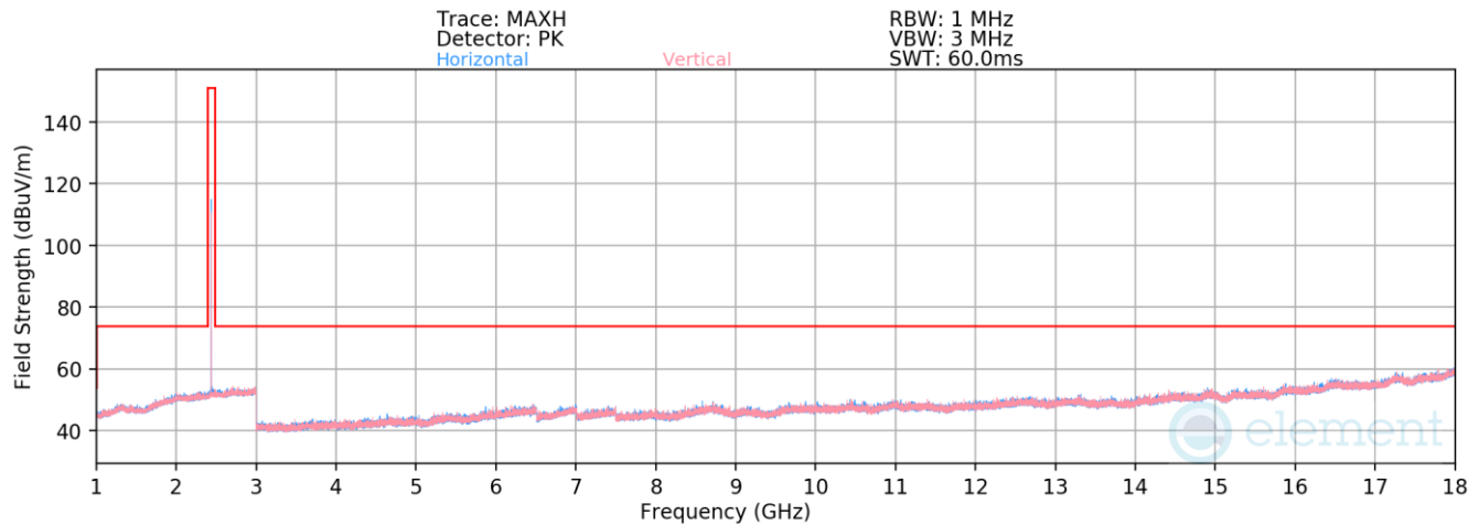
Plot 7-116. Radiated Spurious Emissions 1-18GHz Antenna WF9 (1Mbps, ePA – Ch. 19)
