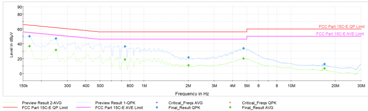
Plot 7-140. AC Line Conducted Plot with Bluetooth LE Tx BF (N, 1Mbps ePA – Ch.19, with AC/DC Adapter)
