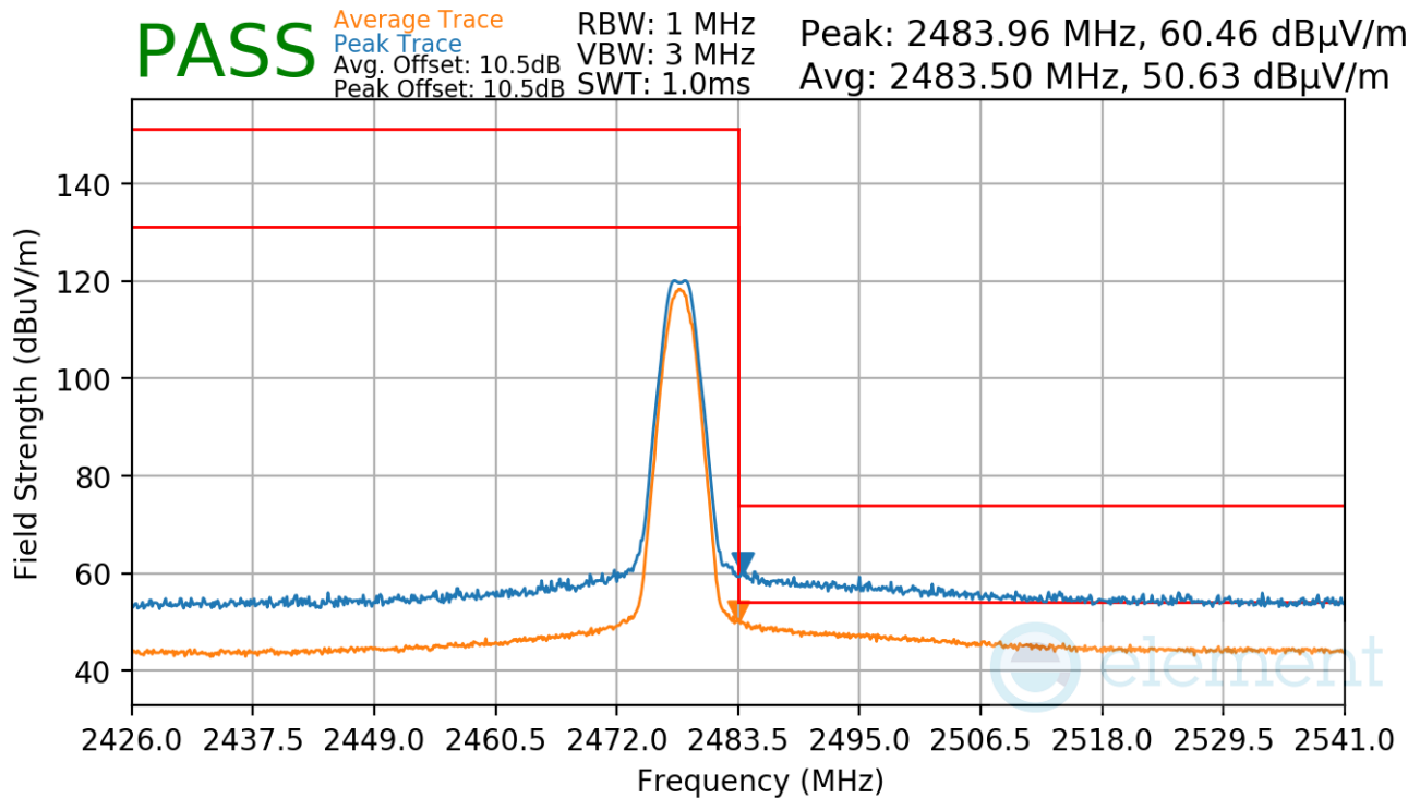
Plot 7-125. Radiated Restricted Upper Band Edge Measurement Antenna WF8 (Average & Peak)
