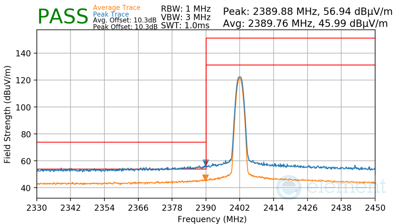
Plot 7-134. Radiated Restricted Lower Band Edge Measurement TxBF (Average & Peak)
