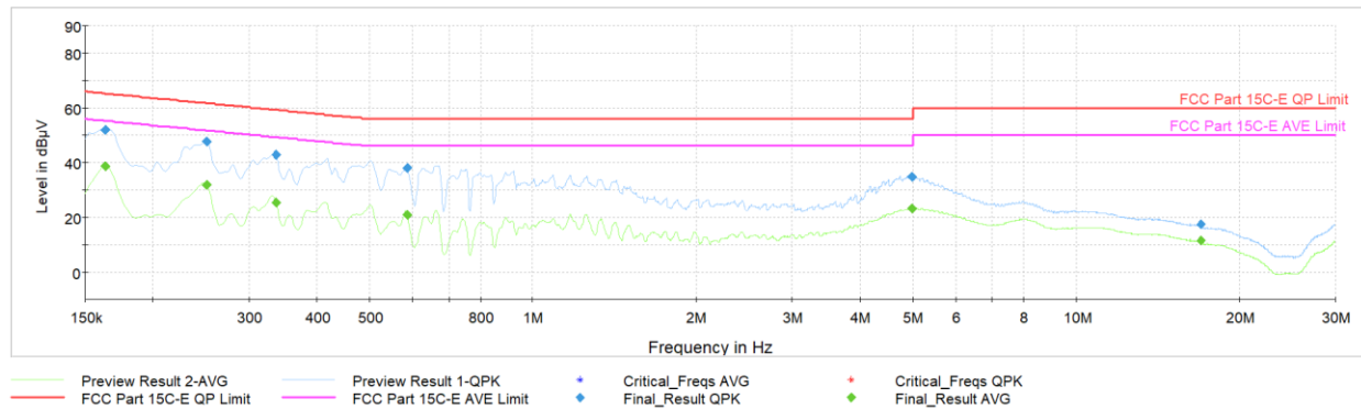
Plot 7-139. AC Line Conducted Plot with Bluetooth LE Tx BF (L1, 1Mbps ePA – Ch.19 with AC/DC Adapter)
