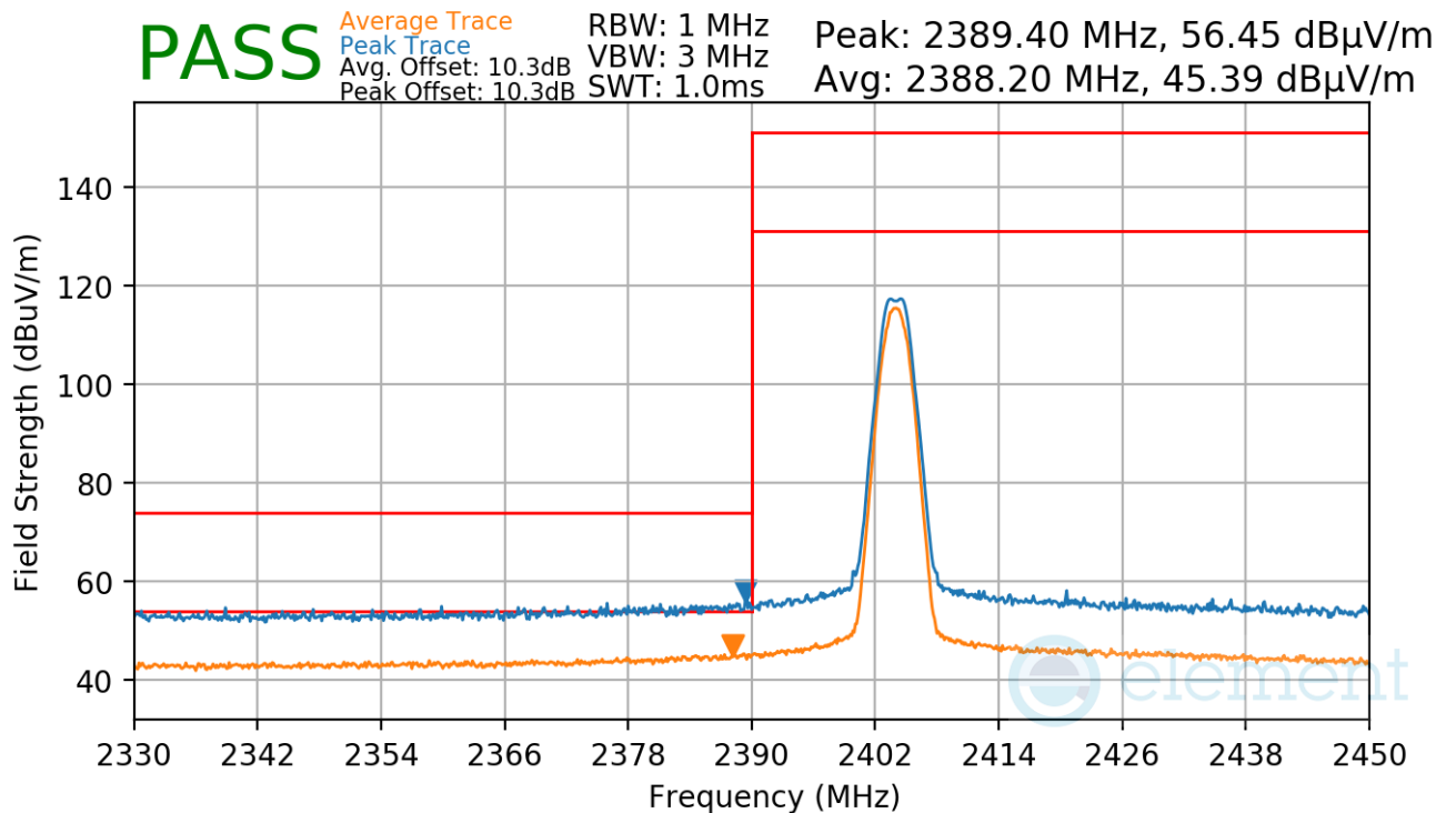
Plot 7-128. Radiated Restricted Lower Band Edge Measurement Antenna WF7 (Average & Peak)
