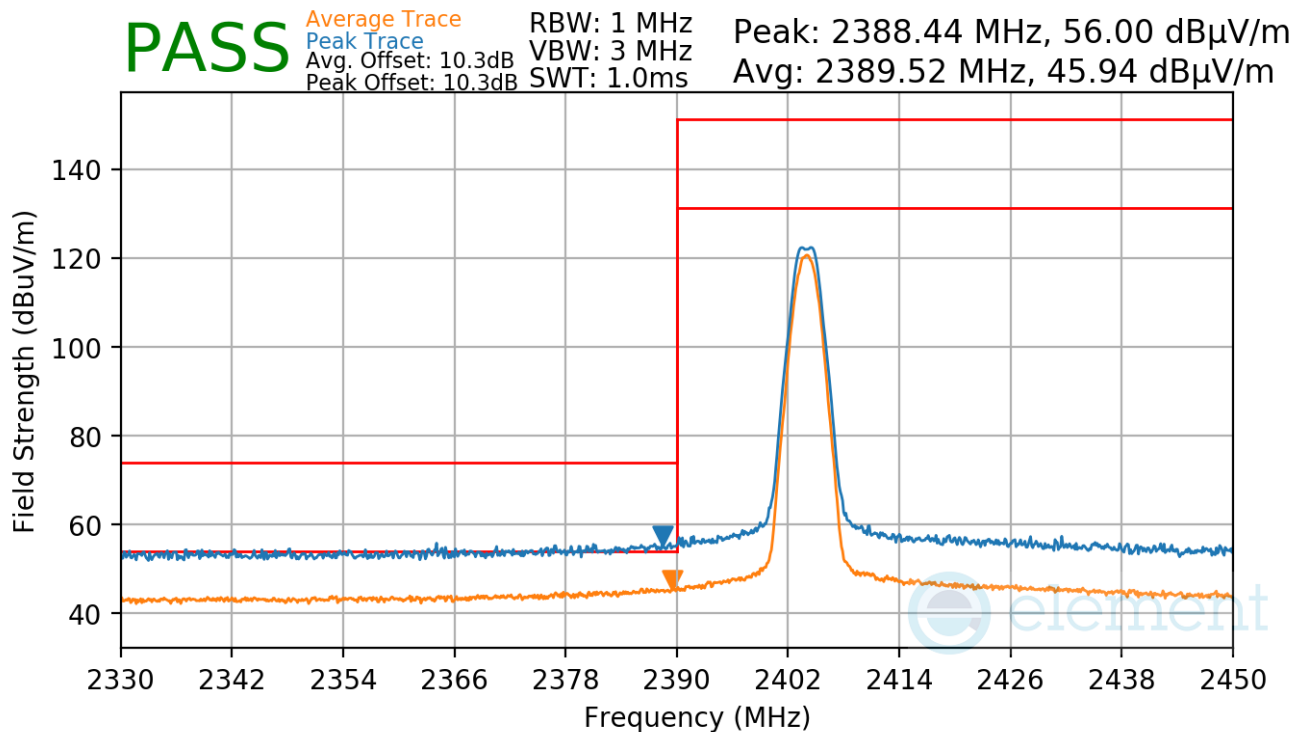
Plot 7-136. Radiated Restricted Lower Band Edge Measurement TxBF (Average & Peak)
