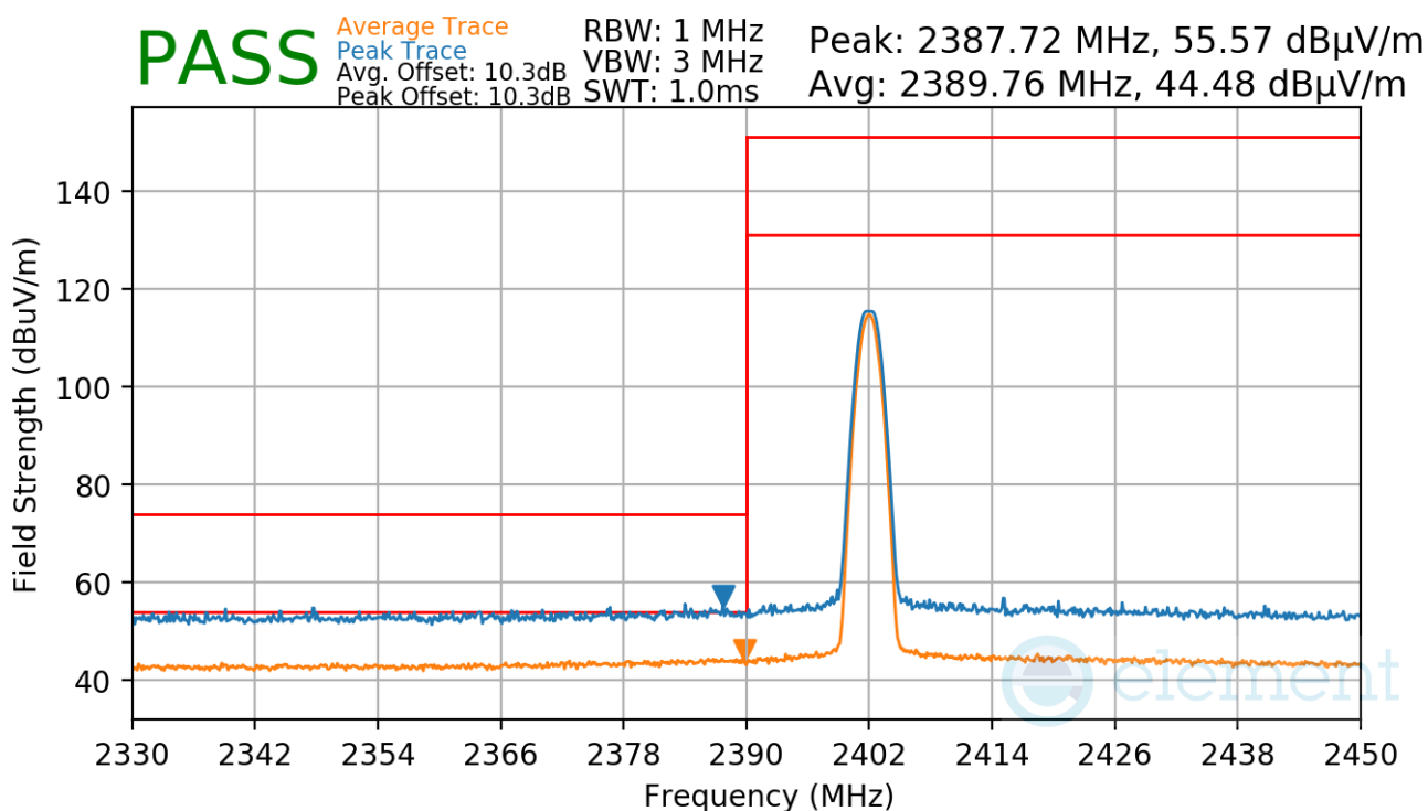
Plot 7-130. Radiated Restricted Lower Band Edge Measurement Antenna WF9 (Average & Peak)
