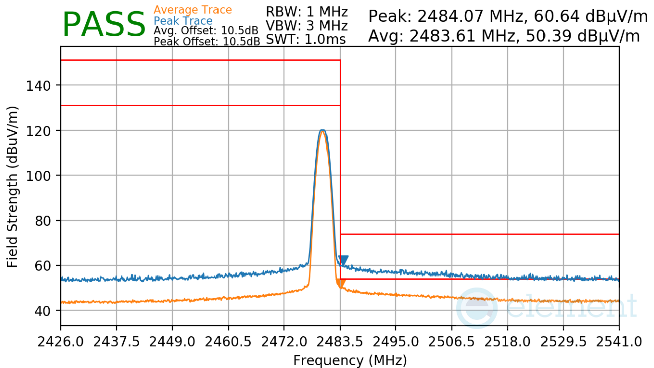
Plot 7-123. Radiated Restricted Upper Band Edge Measurement Antenna WF8 (Average & Peak)
