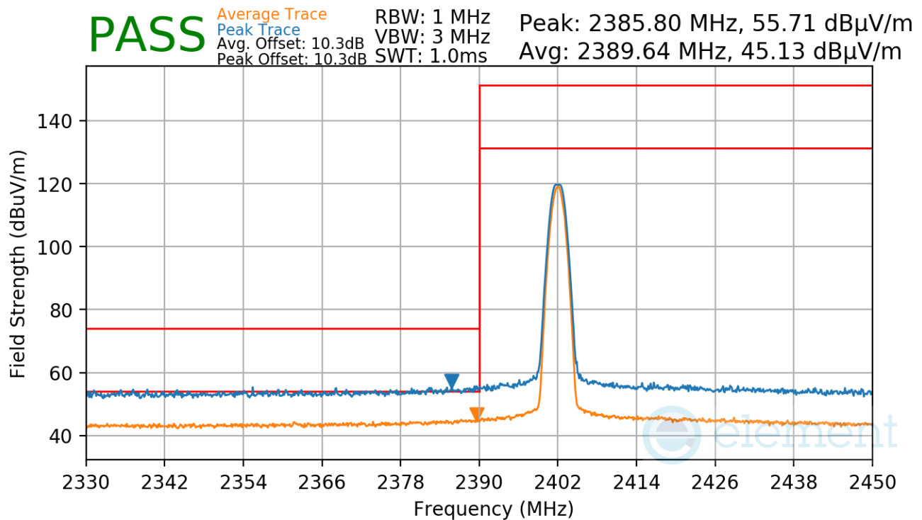
Plot 7-122. Radiated Restricted Lower Band Edge Measurement Antenna WF8 (Average & Peak)
