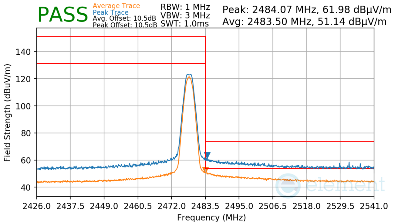
Plot 7-137. Radiated Restricted Upper Band Edge Measurement TxBF (Average & Peak)
