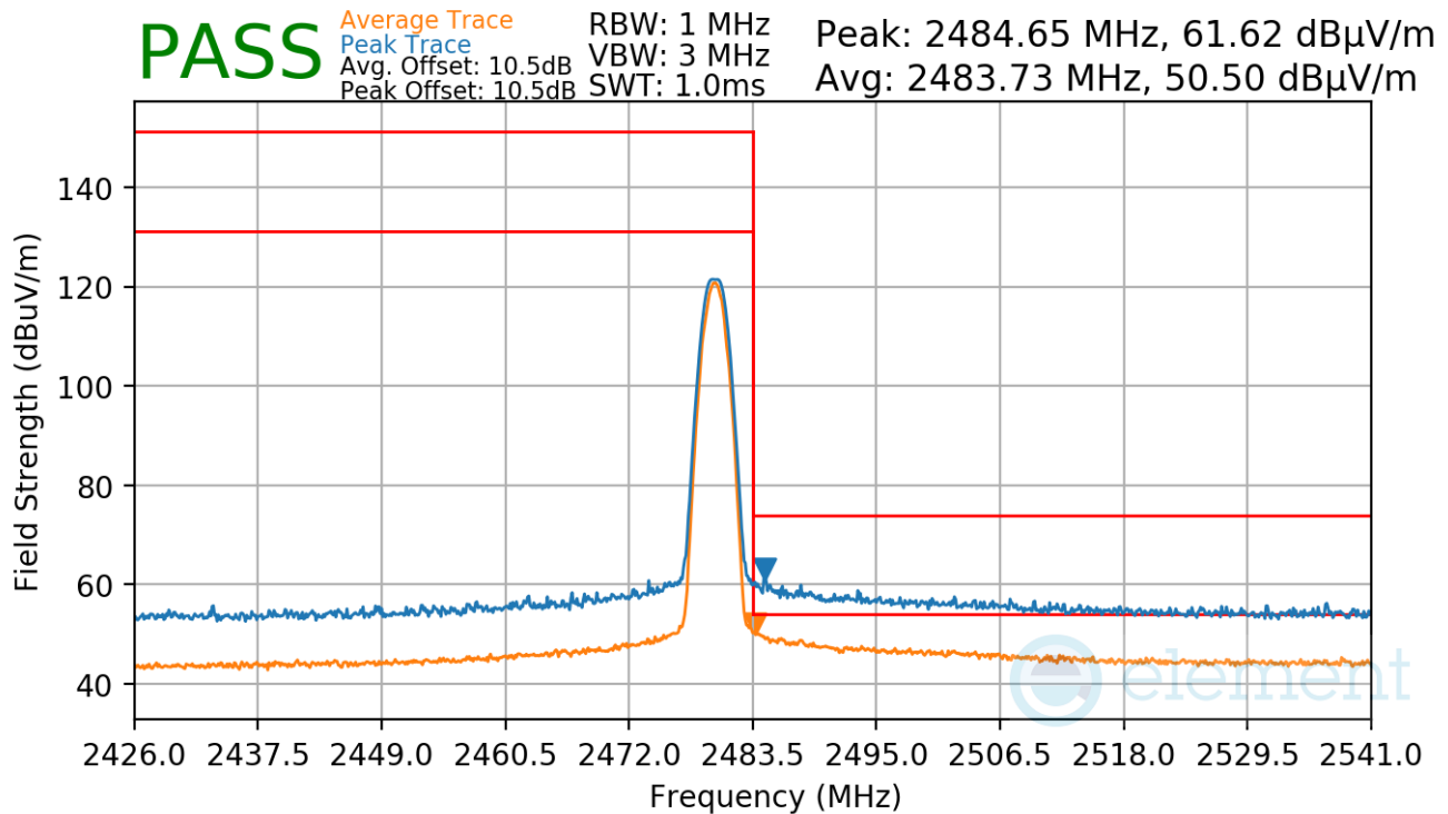
Plot 7-135. Radiated Restricted Upper Band Edge Measurement TxBF (Average & Peak)
