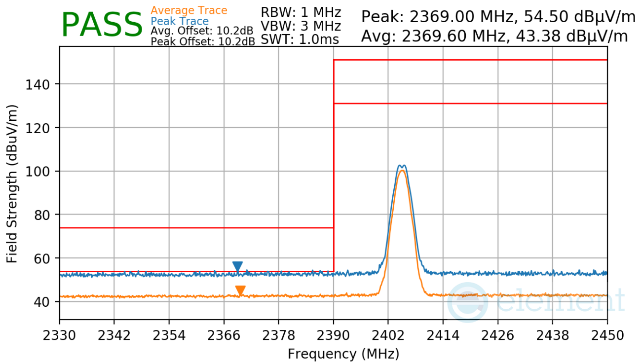
Plot 7-66. Radiated Restricted Lower Band Edge Measurement Antenna WF9
