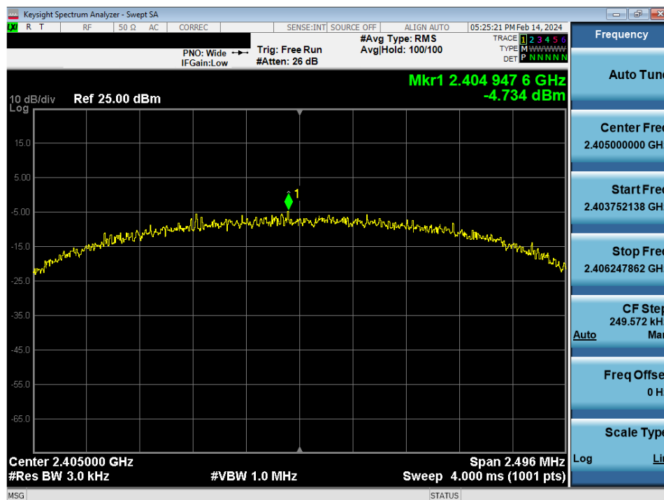
Plot 7-25. Power Spectral Density Antenna WF9 (802.15.4, iPA - Ch. 11)
