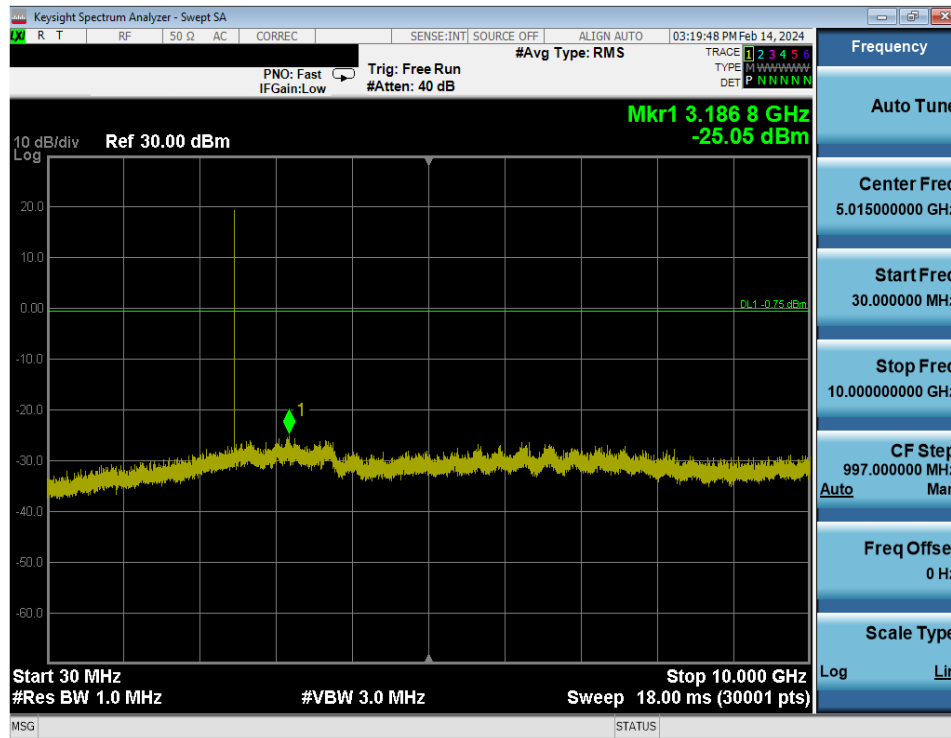
Plot 7-38. Conducted Spurious Antenna WF8 (802.15.4, ePA – Ch. 25)
