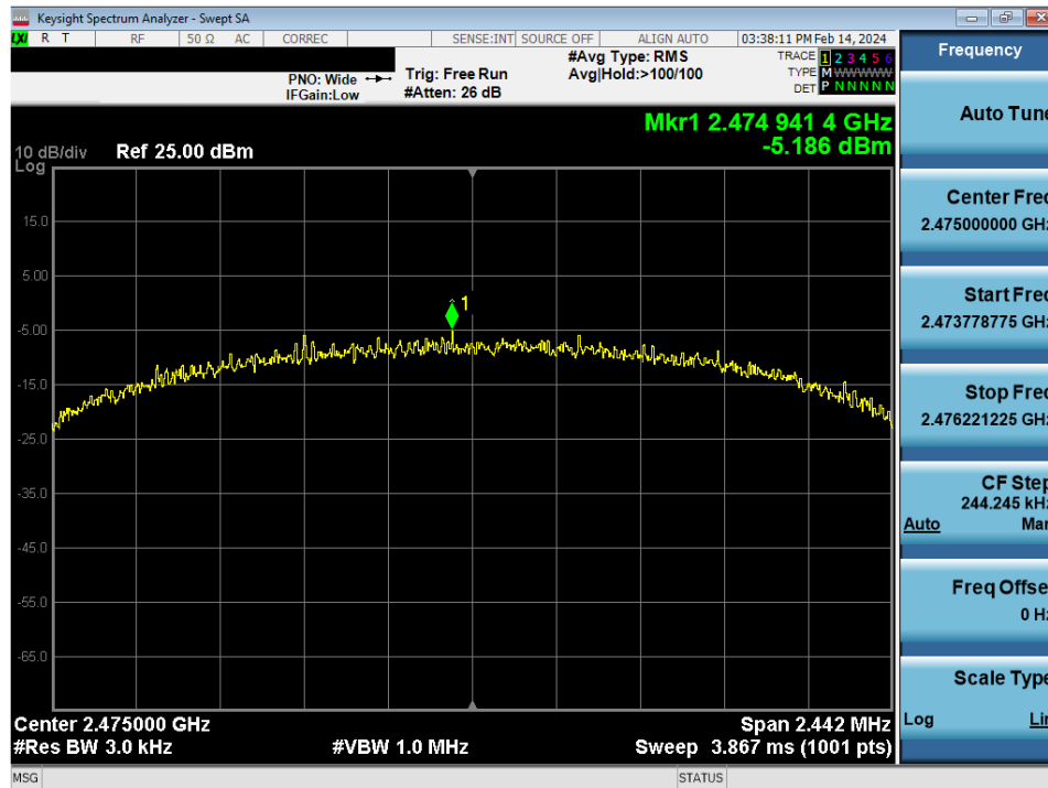
Plot 7-21. Power Spectral Density Antenna WF7 (802.15.4, iPA - Ch. 25)
