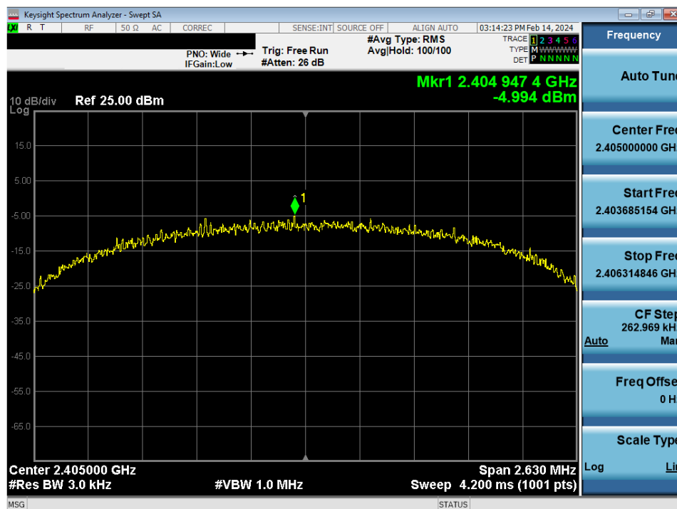
Plot 7-13. Power Spectral Density Antenna WF8 (802.15.4, iPA - Ch. 11)
