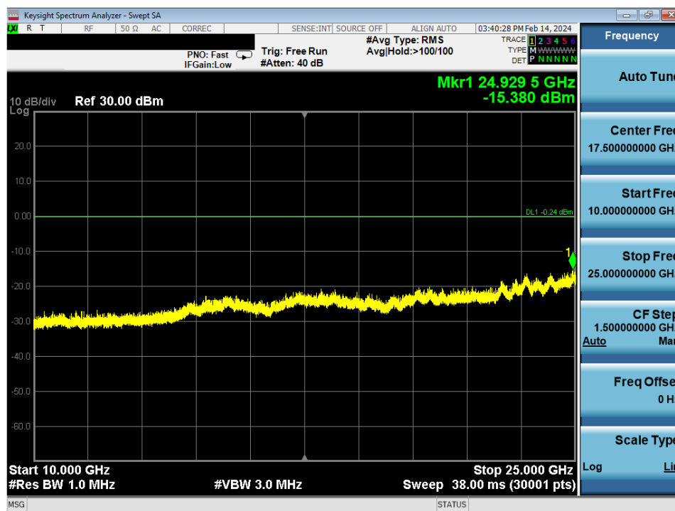
Plot 7-41. Conducted Spurious Antenna WF7 (802.15.4, ePA – Ch. 11)
