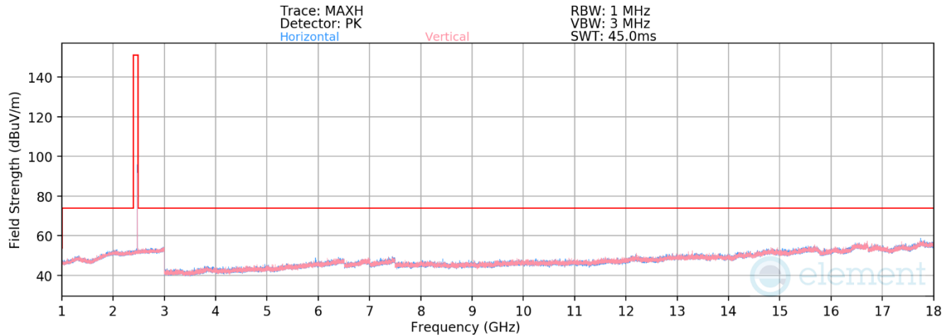
Plot 7-61. Radiated Spurious Emissions 1-18GHz Antenna WF9 (802.15.4 ePA – Ch. 25)
