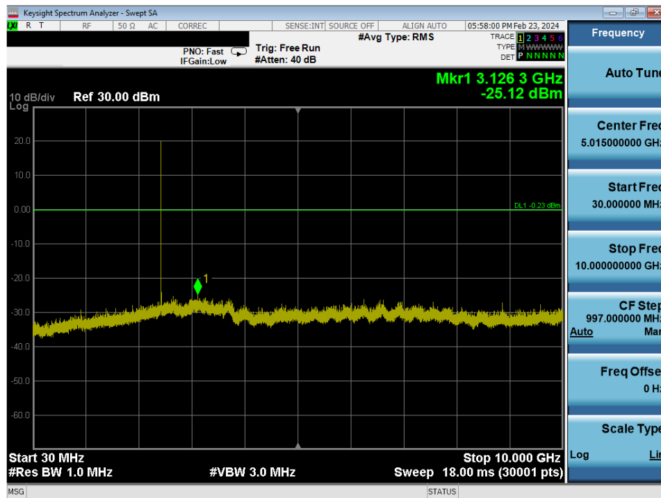
Plot 7-42. Conducted Spurious Antenna WF7 (802.15.4, ePA – Ch. 18)
