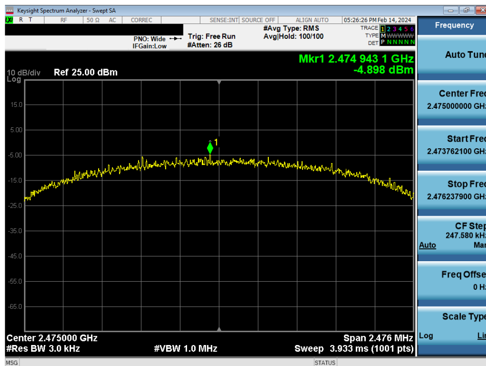
Plot 7-27. Power Spectral Density Antenna WF9 (802.15.4, iPA - Ch. 25)
