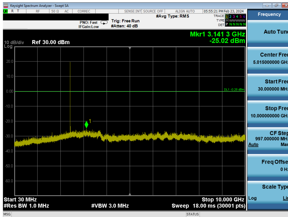
Plot 7-36. Conducted Spurious Antenna WF8 (802.15.4, ePA – Ch. 18)
