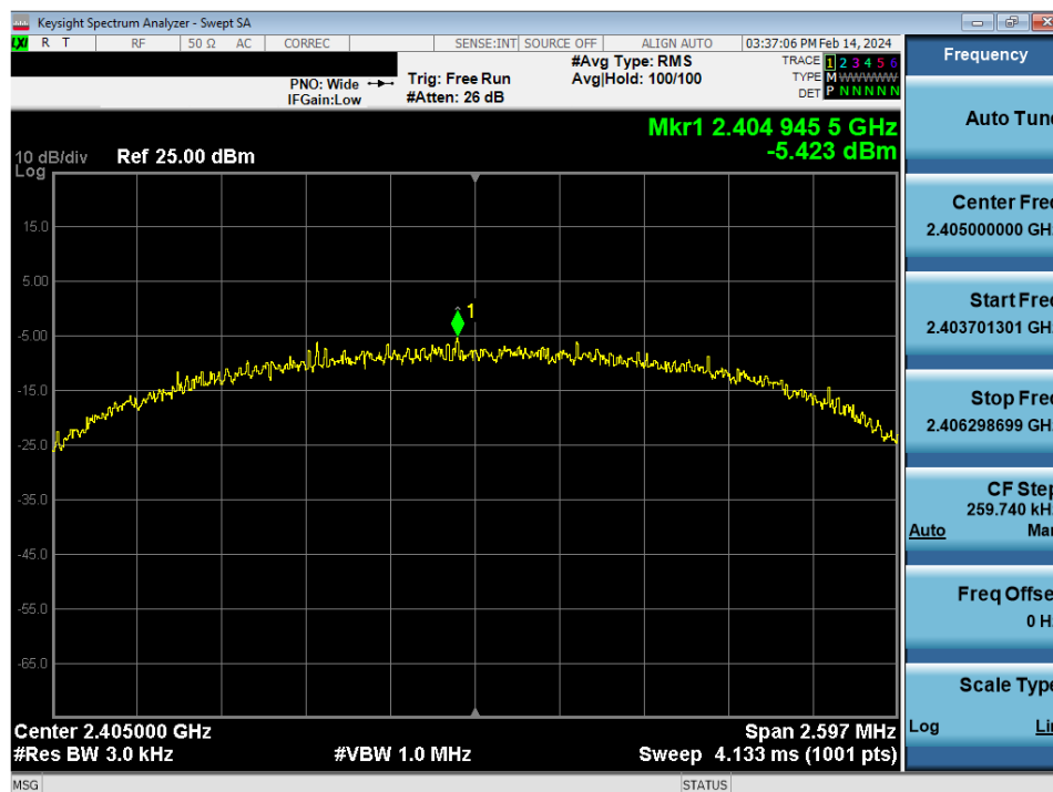
Plot 7-19. Power Spectral Density Antenna WF7 (802.15.4, iPA - Ch. 11)
