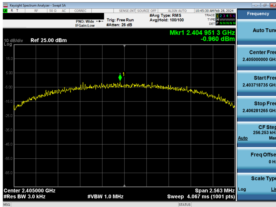
Plot 7-10. Power Spectral Density Antenna WF8 (802.15.4, ePA - Ch. 11)
