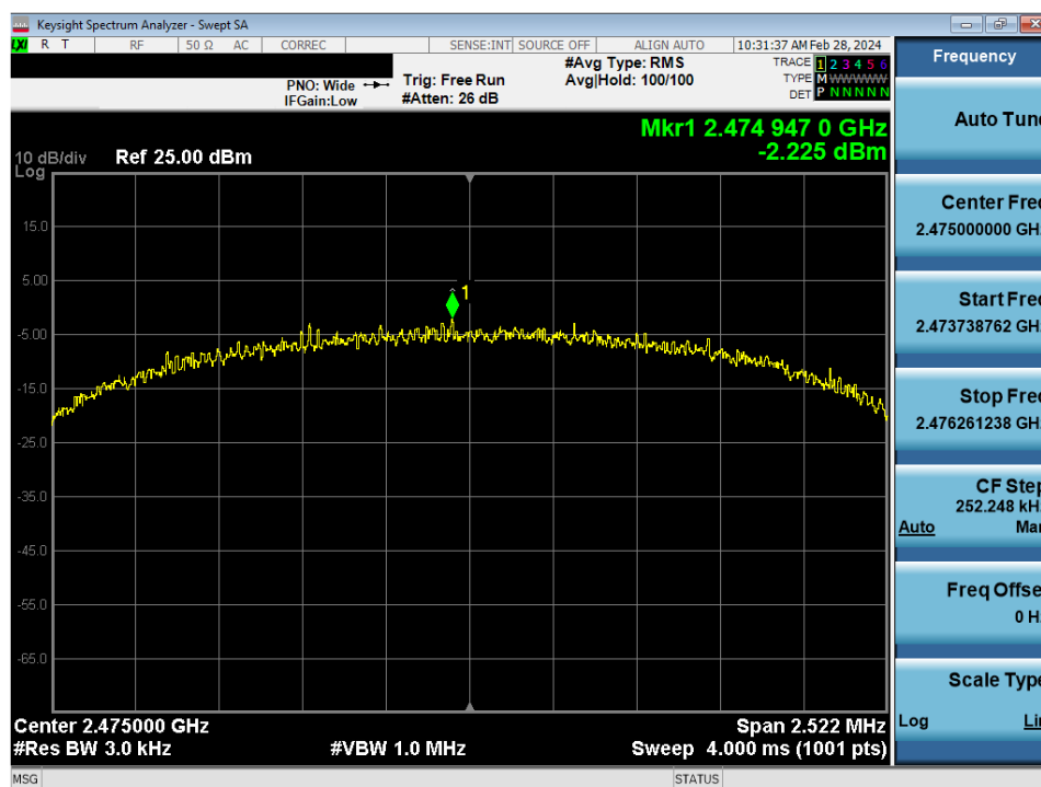
Plot 7-18. Power Spectral Density Antenna WF7 (802.15.4, ePA - Ch. 25)
