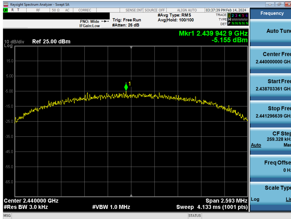
Plot 7-20. Power Spectral Density Antenna WF7 (802.15.4, iPA - Ch. 18)
