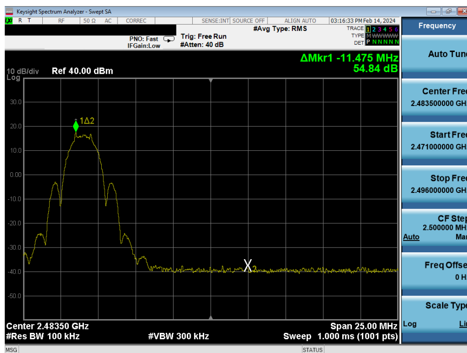
Plot 7-29. Band Edge Antenna WF8 (802.15.4, ePA – Ch. 25)
