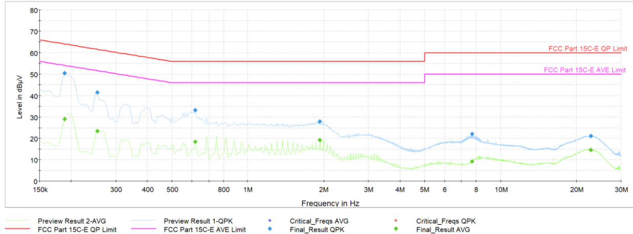
Plot 7-69. AC Line Conducted Emission with 802.15.4 Antenna WF8 (L1, Ch.11 - ePA, with Laptop)
