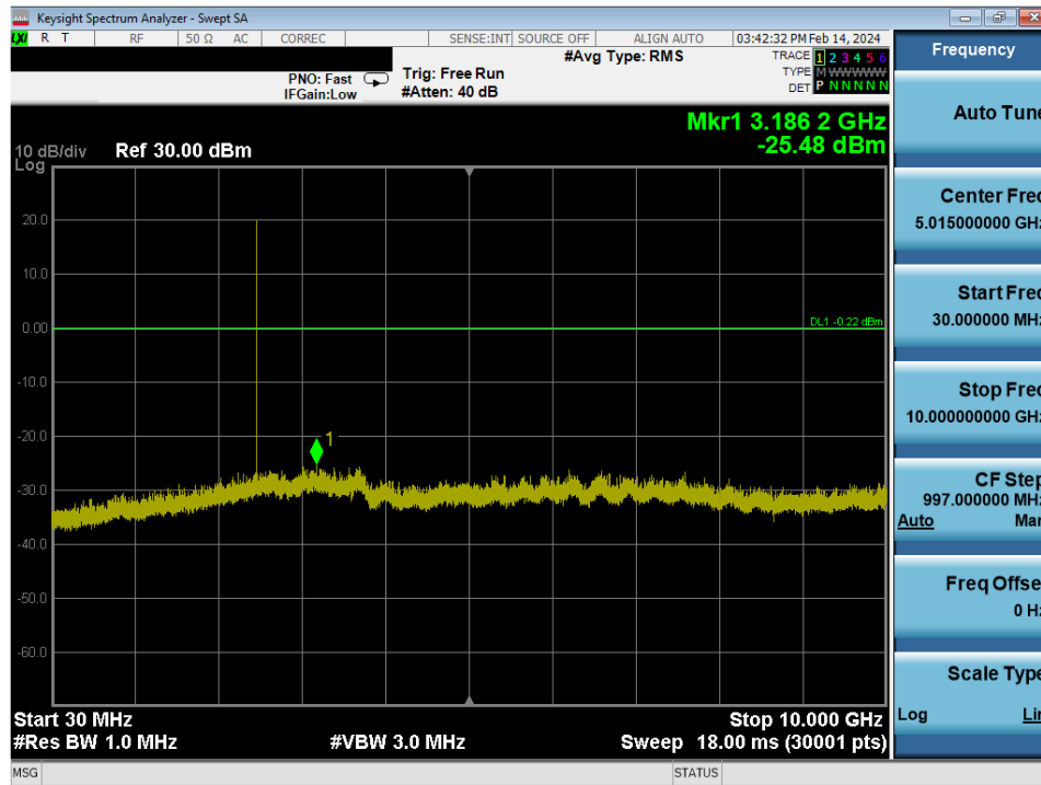
Plot 7-44. Conducted Spurious Antenna WF7 (802.15.4, ePA – Ch. 25)
