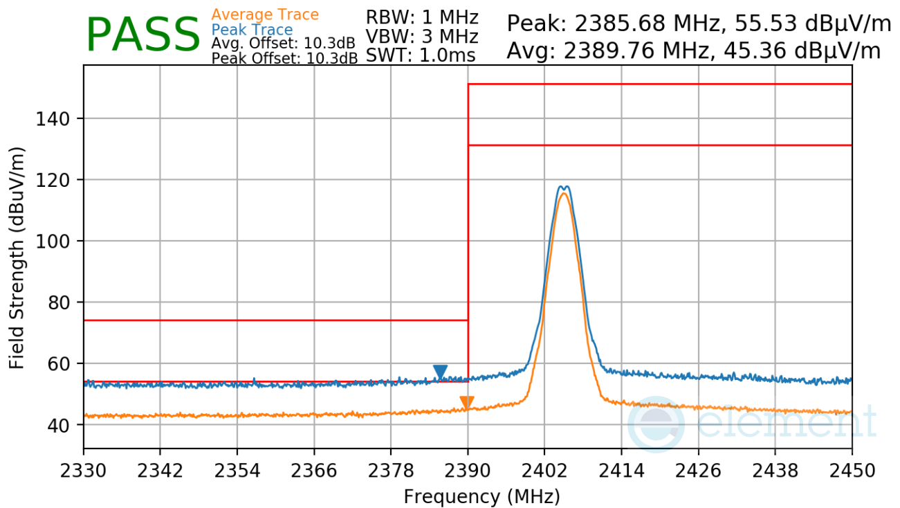
Plot 7-64. Radiated Restricted Lower Band Edge Measurement Antenna WF7
