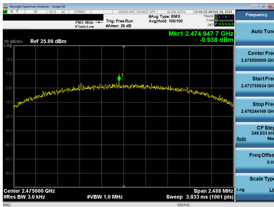
Plot 7-12. Power Spectral Density Antenna WF8 (802.15.4, ePA - Ch. 25)
