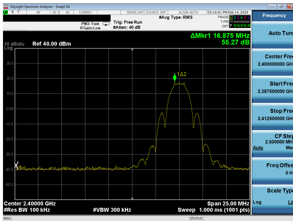
Plot 7-28. Band Edge Antenna WF8 (802.15.4, ePA – Ch. 11)
