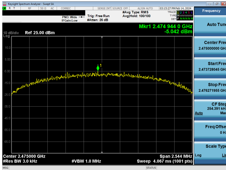
Plot 7-15. Power Spectral Density Antenna WF8 (802.15.4, iPA - Ch. 25)
