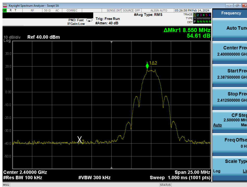
Plot 7-32. Band Edge Antenna WF9 (802.15.4, ePA – Ch. 11)
