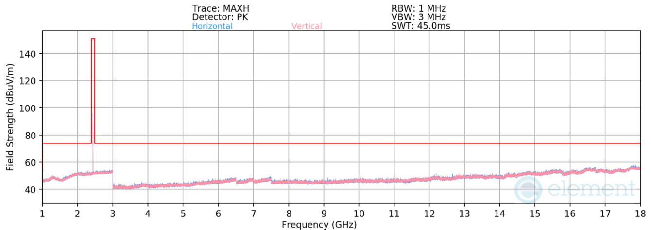
Plot 7-60. Radiated Spurious Emissions 1-18GHz Antenna WF9 (802.15.4 ePA – Ch. 18)
