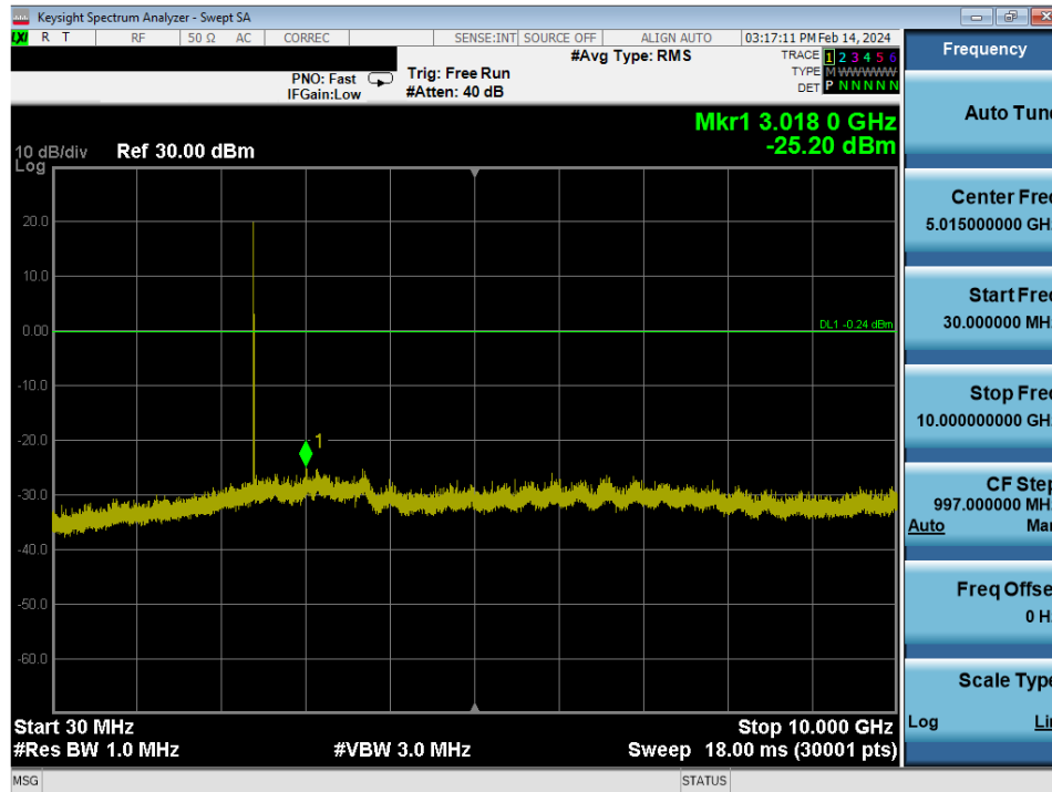
Plot 7-34. Conducted Spurious Antenna WF8 (802.15.4, ePA – Ch. 11)
