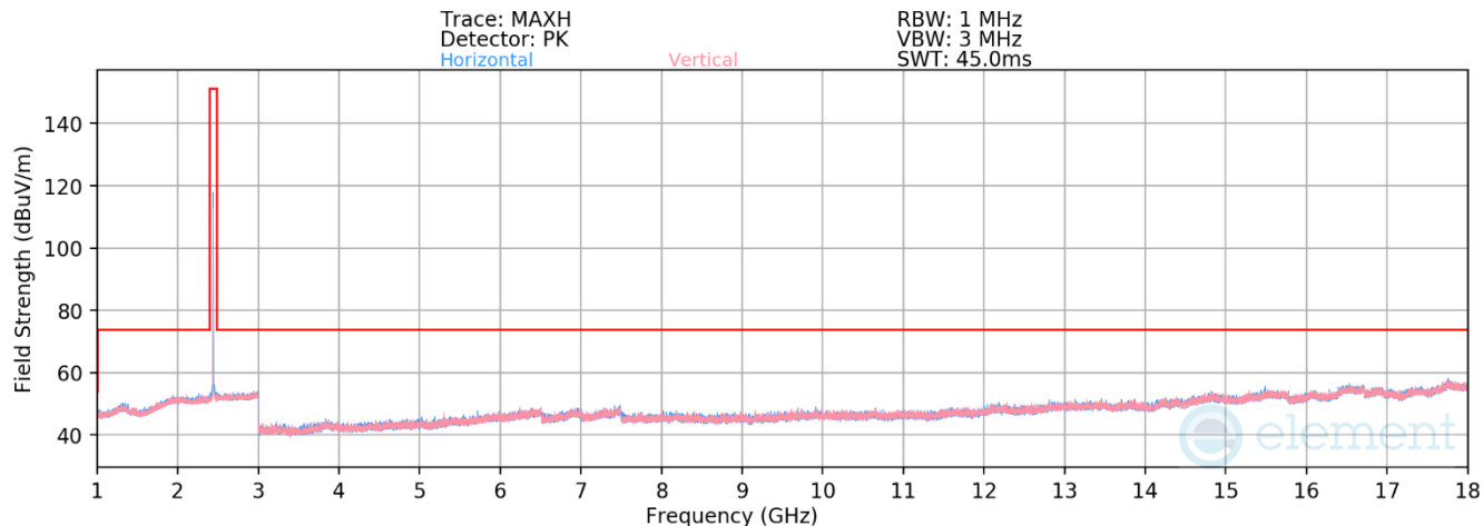
Plot 7-57. Radiated Spurious Emissions 1-18GHz Antenna WF7 (802.15.4 ePA – Ch. 18)
