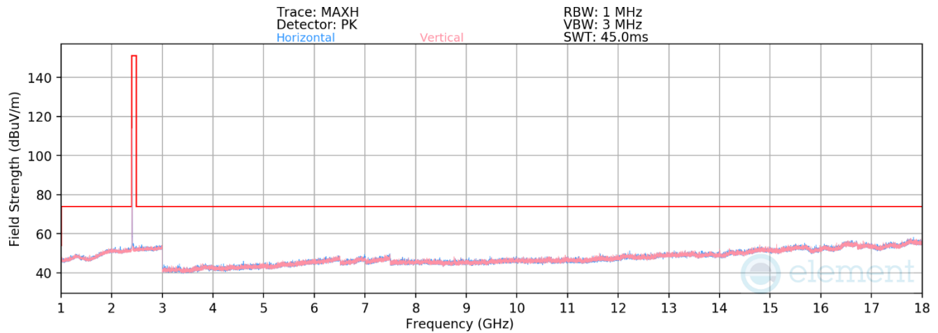
Plot 7-52. Radiated Spurious Emissions 1-18GHz Antenna WF8 (802.15.4 ePA – Ch. 11)
