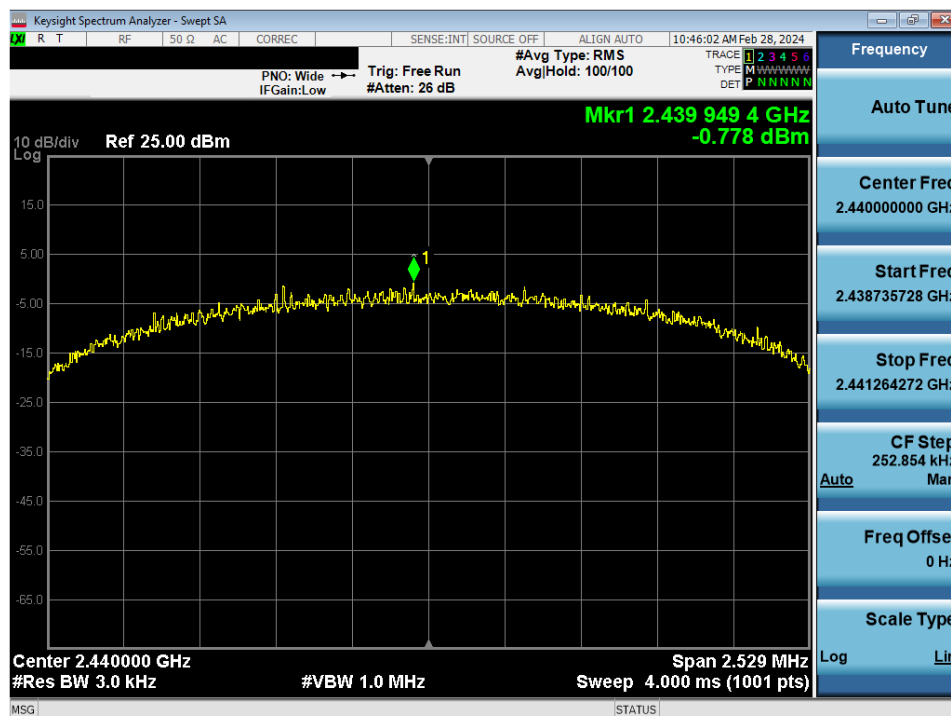
Plot 7-11. Power Spectral Density Antenna WF8 (802.15.4, ePA - Ch. 18)
