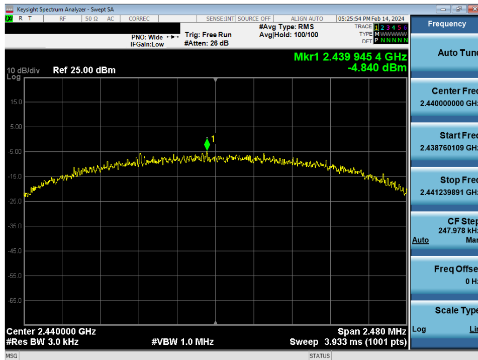
Plot 7-26. Power Spectral Density Antenna WF9 (802.15.4, iPA - Ch. 18)
