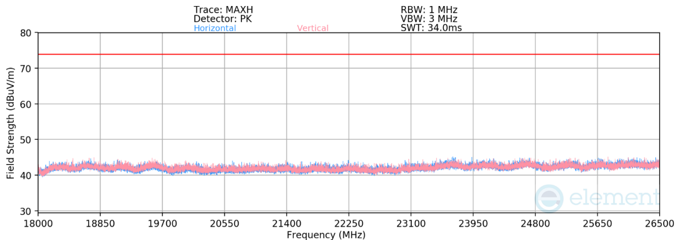
Plot 7-53. Radiated Spurious Emissions Above 18GHz Antenna WF8 (802.15.4 ePA – Ch. 11)
