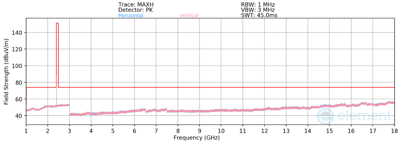
Plot 7-59. Radiated Spurious Emissions 1-18GHz Antenna WF9 (802.15.4 ePA – Ch. 11)
