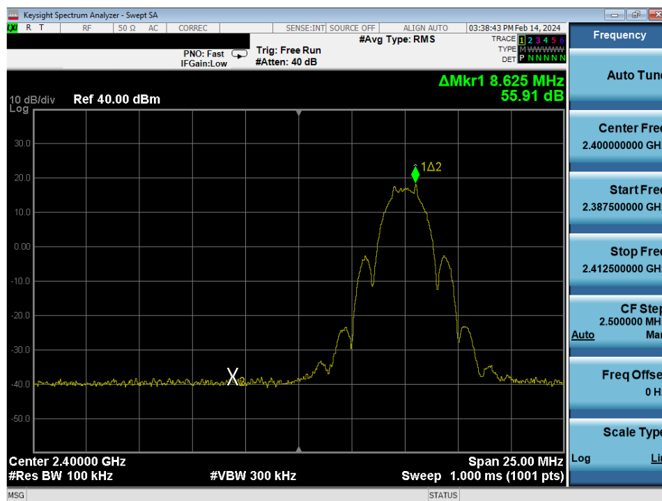
Plot 7-30. Band Edge Antenna WF7 (802.15.4, ePA – Ch. 11)
