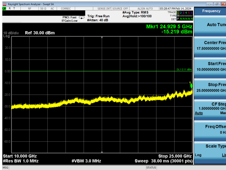
Plot 7-47. Conducted Spurious Antenna WF9 (802.15.4, ePA – Ch. 11)
