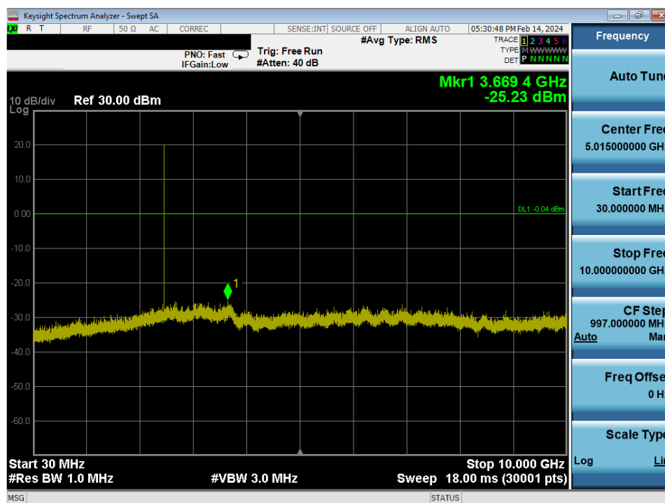
Plot 7-50. Conducted Spurious Antenna WF9 (802.15.4, ePA – Ch. 25)
