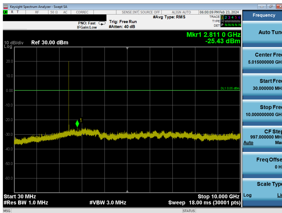
Plot 7-48. Conducted Spurious Antenna WF9 (802.15.4, ePA – Ch. 18)
