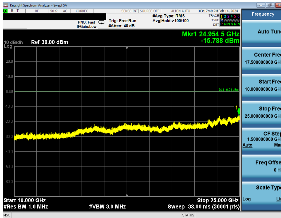
Plot 7-35. Conducted Spurious Antenna WF8 (802.15.4, ePA – Ch. 11)
