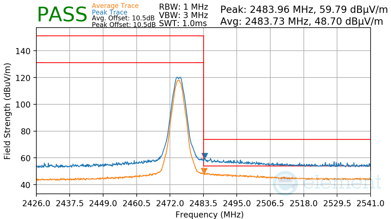
Plot 7-63. Radiated Restricted Upper Band Edge Measurement Antenna WF8
