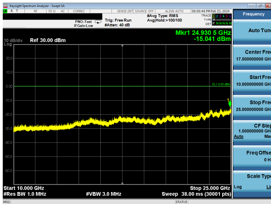
Plot 7-49. Conducted Spurious Antenna WF9 (802.15.4, ePA – Ch. 18)
