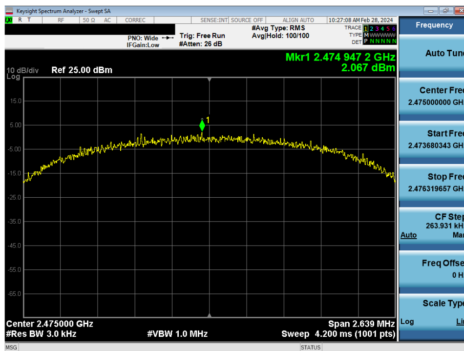
Plot 7-24. Power Spectral Density Antenna WF9 (802.15.4, ePA - Ch. 25)
