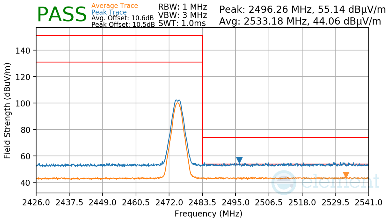
Plot 7-67. Radiated Restricted Upper Band Edge Measurement Antenna WF9
