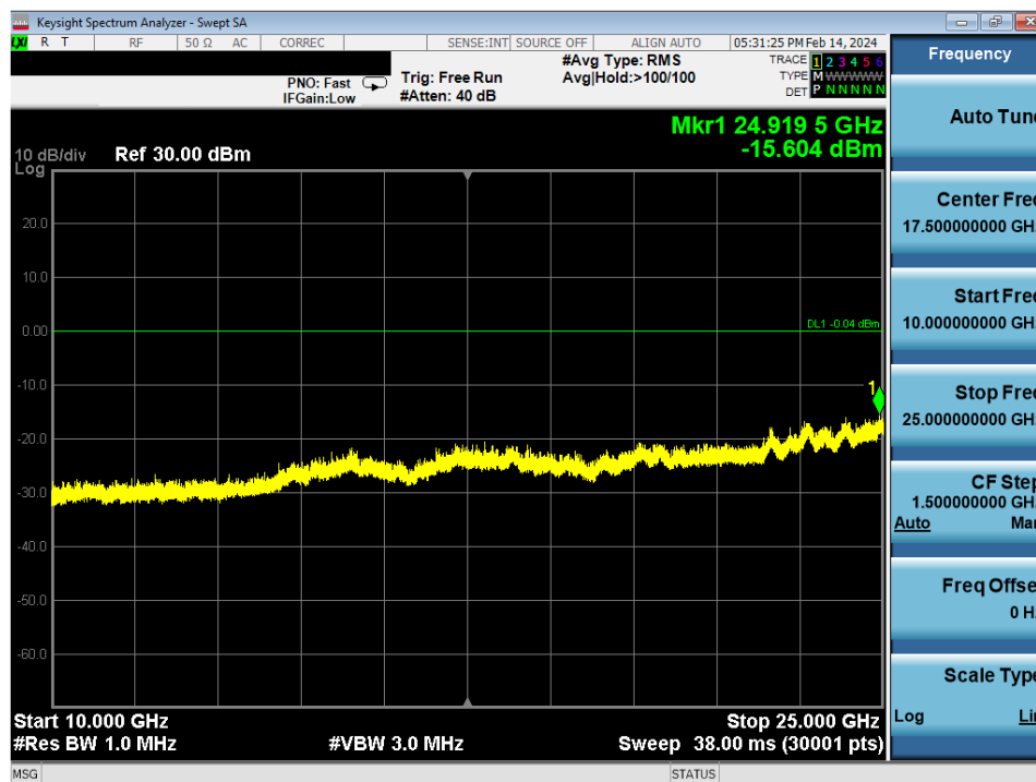
Plot 7-51. Conducted Spurious Antenna WF9 (802.15.4, ePA – Ch. 25)
