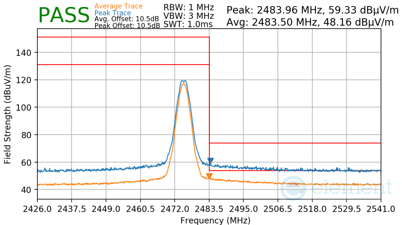
Plot 7-65. Radiated Restricted Upper Band Edge Measurement Antenna WF7
