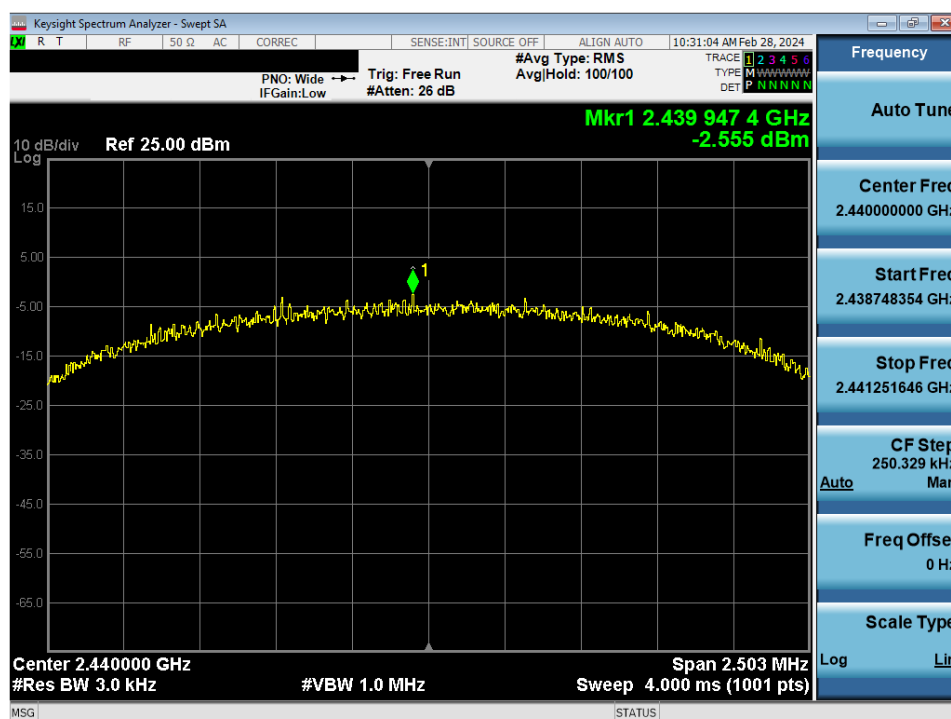
Plot 7-17. Power Spectral Density Antenna WF7 (802.15.4, ePA - Ch. 18)
