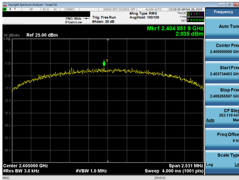
Plot 7-22. Power Spectral Density Antenna WF9 (802.15.4, ePA - Ch. 11)
