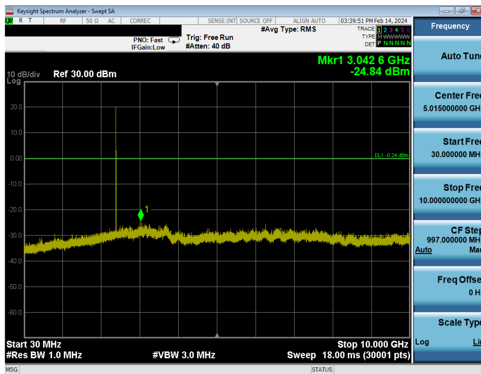
Plot 7-40. Conducted Spurious Antenna WF7 (802.15.4, ePA – Ch. 11)
