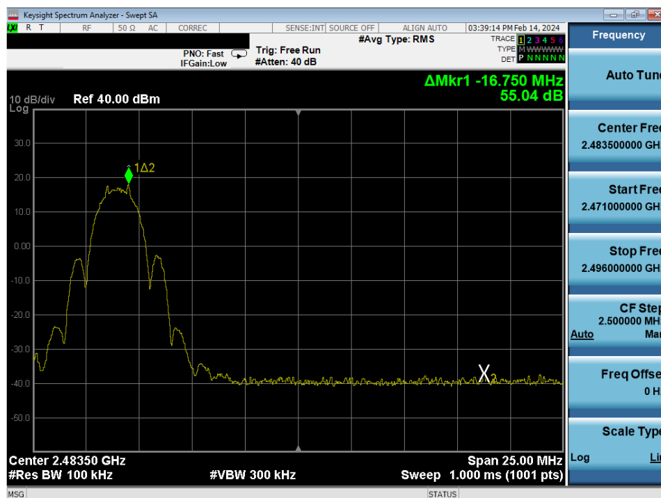
Plot 7-31. Band Edge Antenna WF7 (802.15.4, ePA – Ch. 25)
