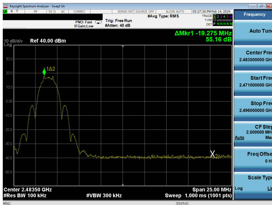
Plot 7-33. Band Edge Antenna WF9 (802.15.4, ePA – Ch. 25)
