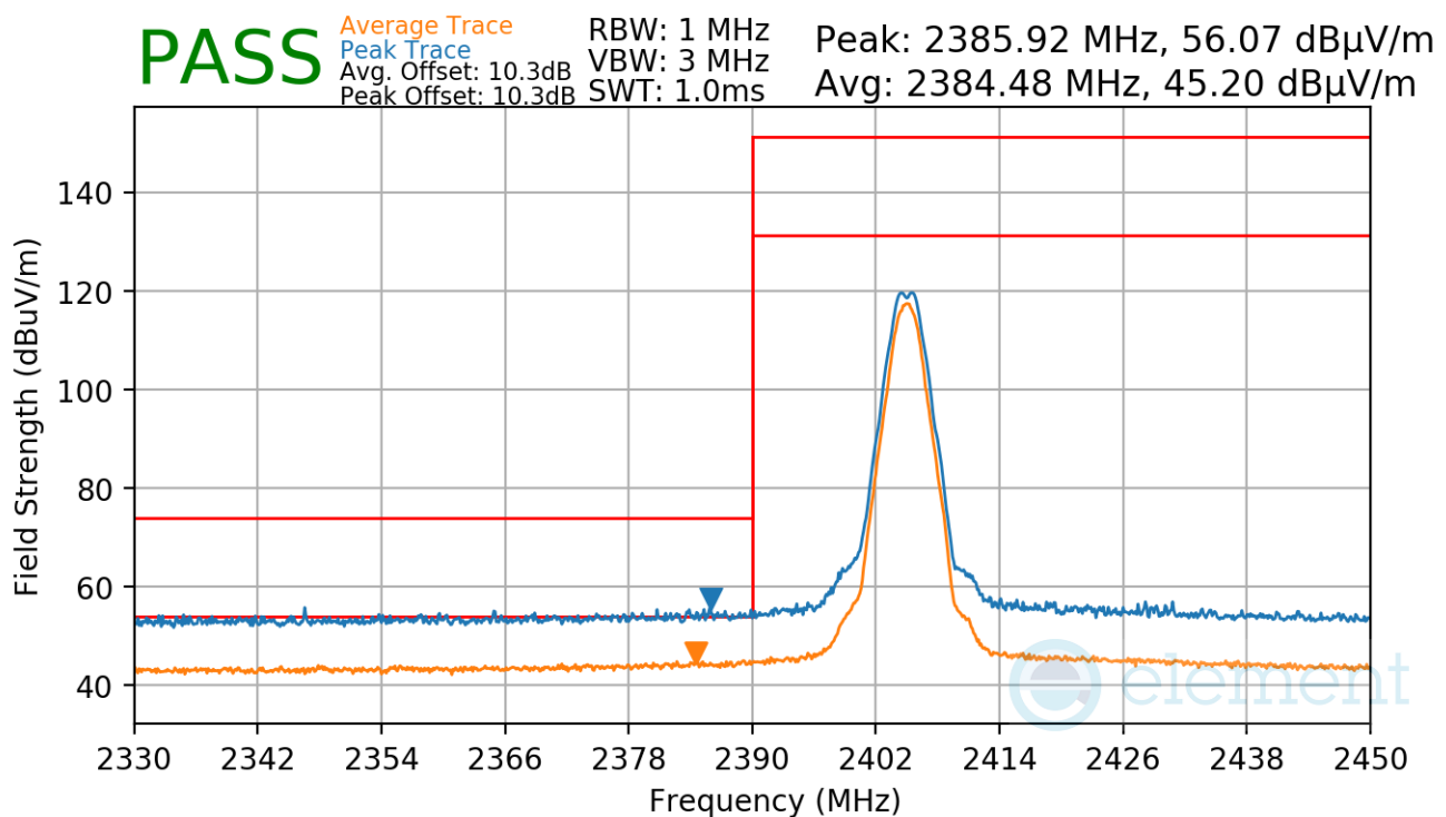
Plot 7-62. Radiated Restricted Lower Band Edge Measurement Antenna WF8
