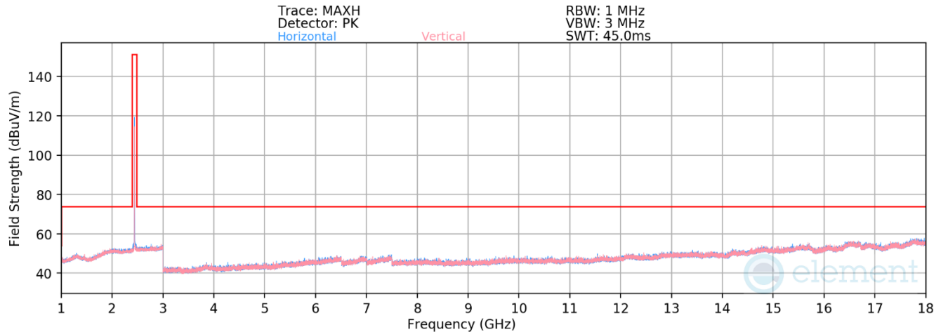
Plot 7-54. Radiated Spurious Emissions 1-18GHz Antenna WF8 (802.15.4 ePA – Ch. 18)
