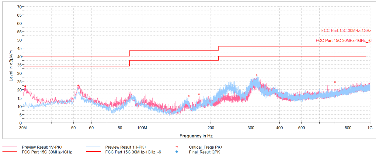
Plot 7-68. Radiated Spurious Emissions 30MHz-1GHz Antenna WF8 (ePA - Ch.11, with Laptop)
