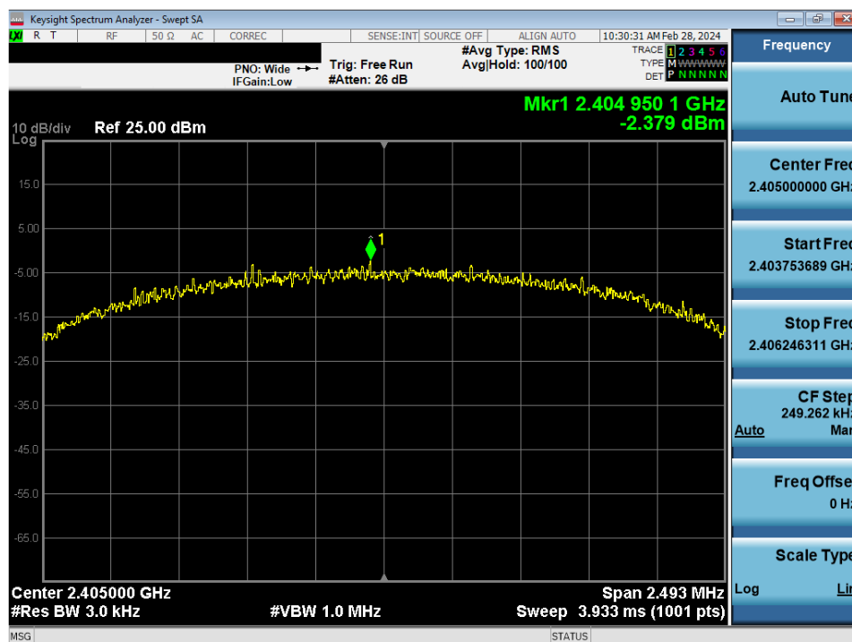
Plot 7-16. Power Spectral Density Antenna WF7 (802.15.4, ePA - Ch. 11)
