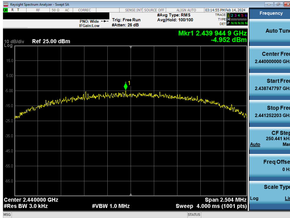
Plot 7-14. Power Spectral Density Antenna WF8 (802.15.4, iPA - Ch. 18)
