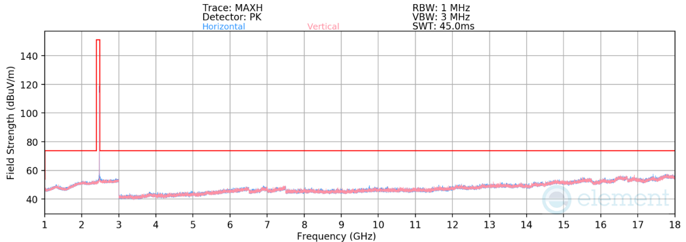
Plot 7-55. Radiated Spurious Emissions 1-18GHz Antenna WF8 (802.15.4 ePA – Ch. 25)
