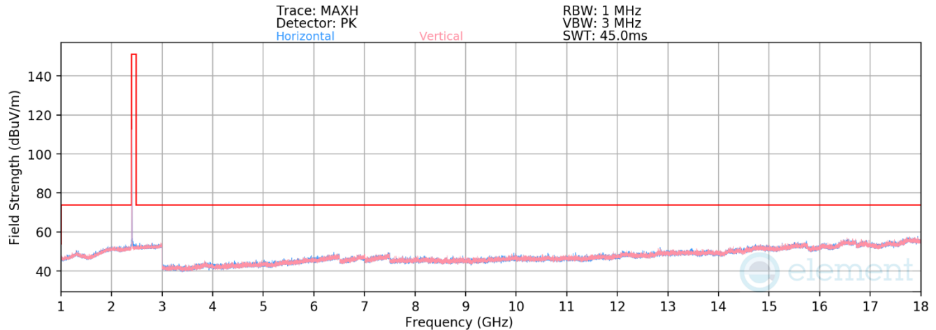
Plot 7-56. Radiated Spurious Emissions 1-18GHz Antenna WF7 (802.15.4 ePA – Ch. 11)
