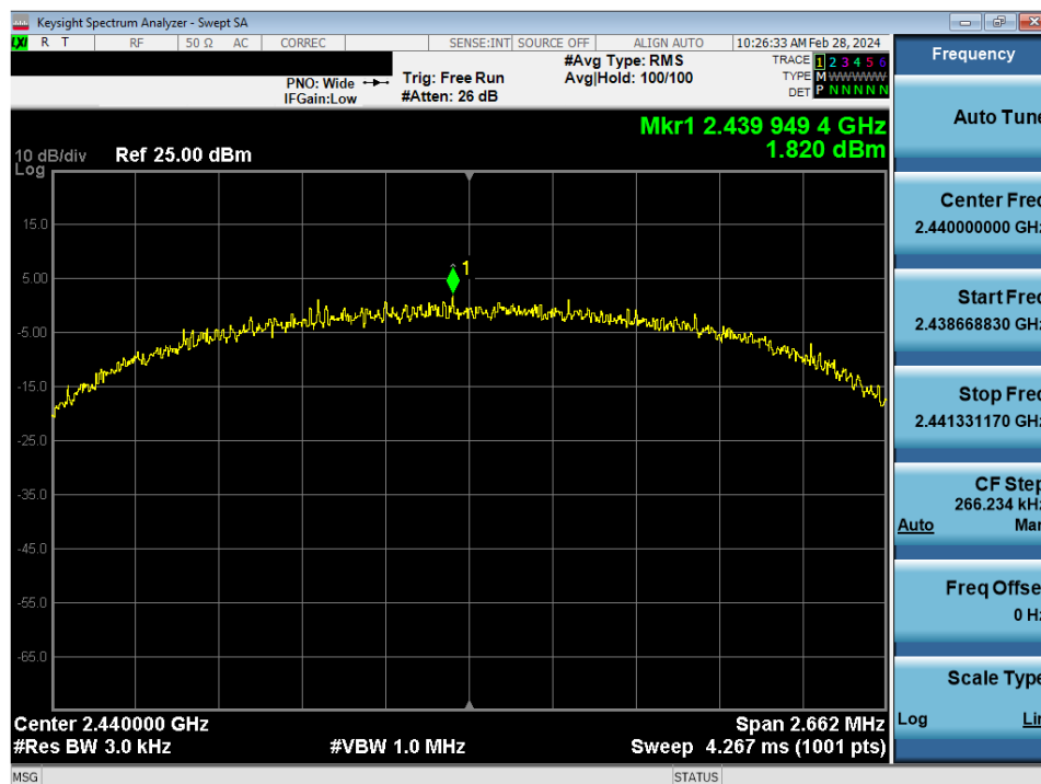
Plot 7-23. Power Spectral Density Antenna WF9 (802.15.4, ePA - Ch. 18)
