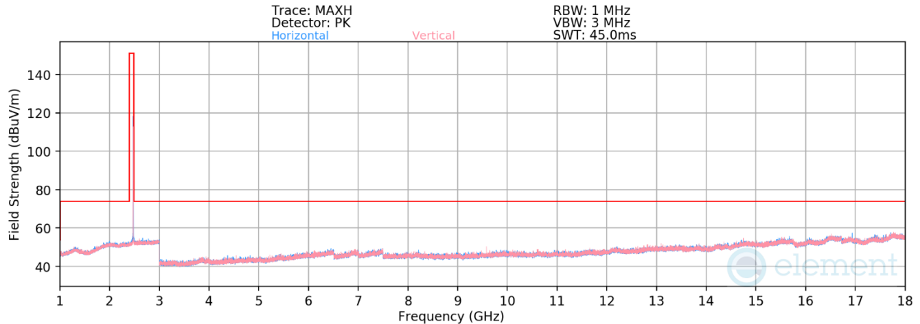
Plot 7-58. Radiated Spurious Emissions 1-18GHz Antenna WF7 (802.15.4 ePA – Ch. 25)
