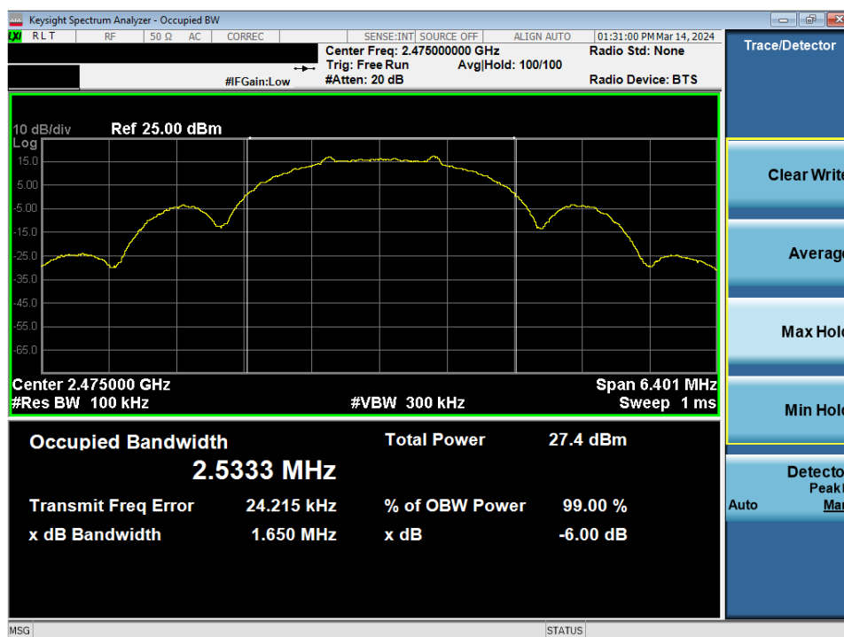
Plot 7-6. 6dB BW & 99% OBW Antenna WF7(802.15.4, Ch. 25)
