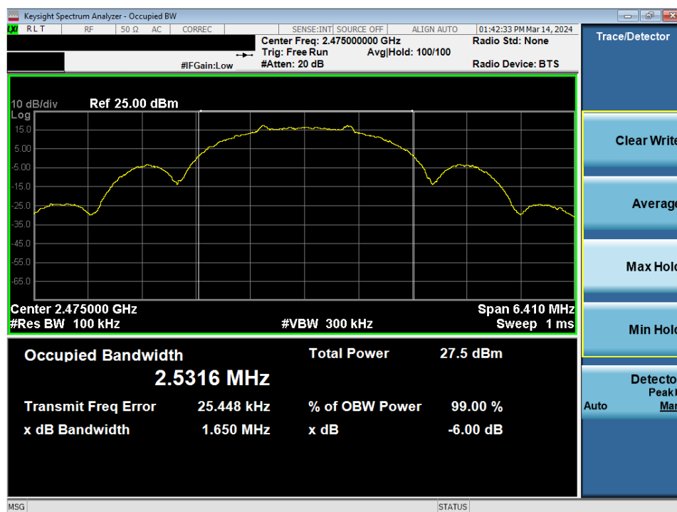
Plot 7-9. 6dB BW & 99% OBW Antenna WF9(802.15.4, Ch. 25)
