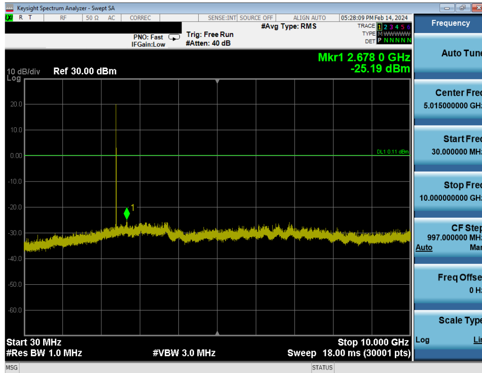
Plot 7-46. Conducted Spurious Antenna WF9 (802.15.4, ePA – Ch. 11)
