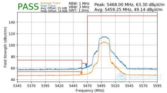
Plot 7-1223. Antenna WF8 (Peak & Average, Ch.100, 802.11n, MCS4)
