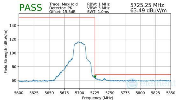
Plot 7-1230. Antenna WF8 (Peak, Ch.140, 802.11n, MCS4)
