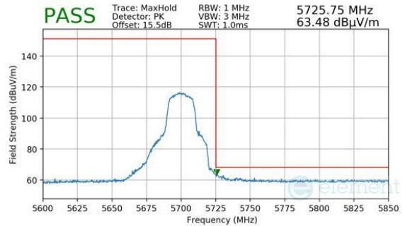
Plot 7-1229. Antenna WF8 (Peak, Ch.140, 802.11n, MCS2)
