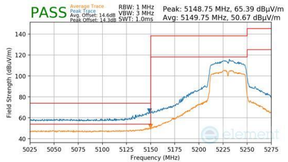
Plot 7-1269. Antenna WF8 (Peak & Average, Ch.46, 802.11n, MCS4)
