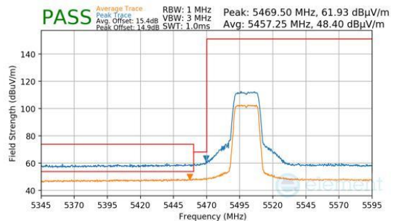
Plot 7-1224. Antenna WF8 (Peak & Average, Ch.100, 802.11n, MCS7)
