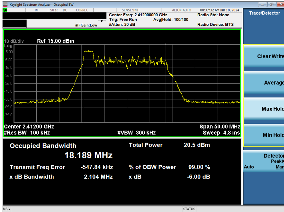
Plot 7-13. 6dB BW & 99% OBW Plot Antenna WF7 (802.11ax OFDMA – RU26 Index 0 – Ch. 1)
