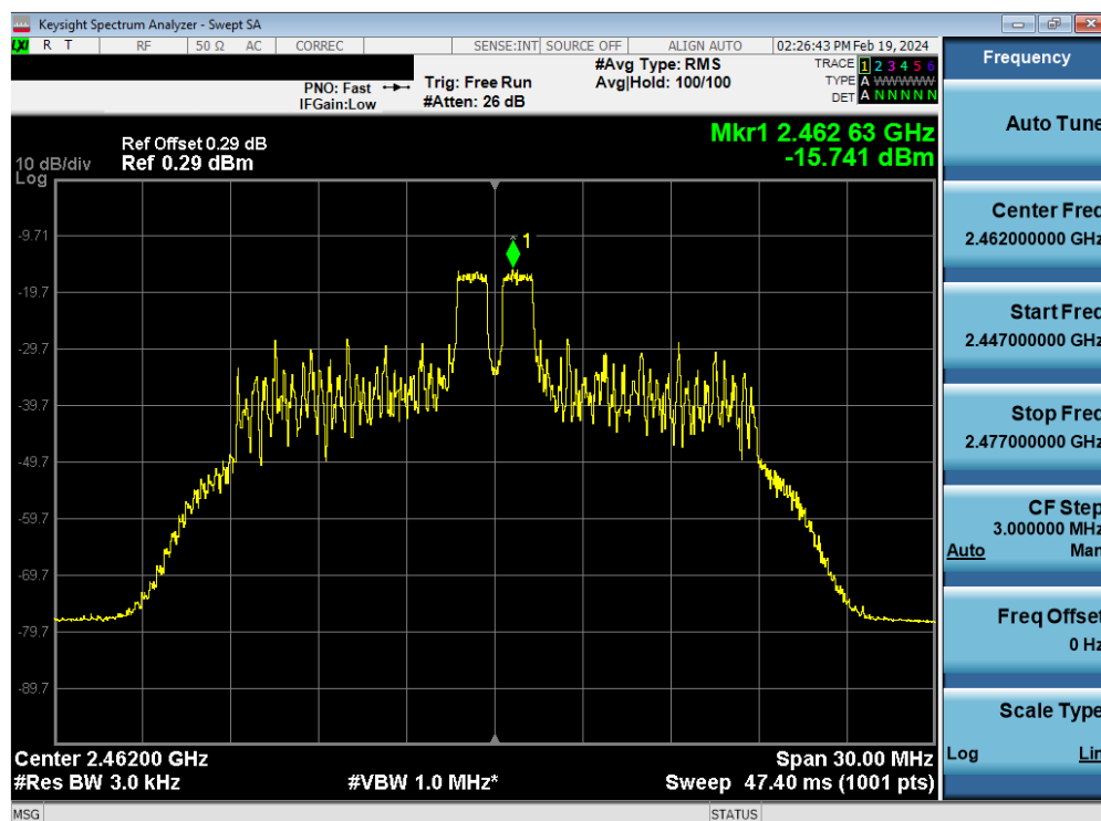
Plot 7-87. Power Spectral Density Plot Antenna WF8 (802.11ax OFDMA – RU26 Index 4 – Ch. 11)
