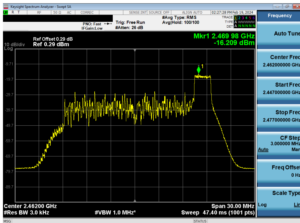
Plot 7-89. Power Spectral Density Plot Antenna WF8 (802.11ax OFDMA – RU26 Index 8 – Ch. 11)
