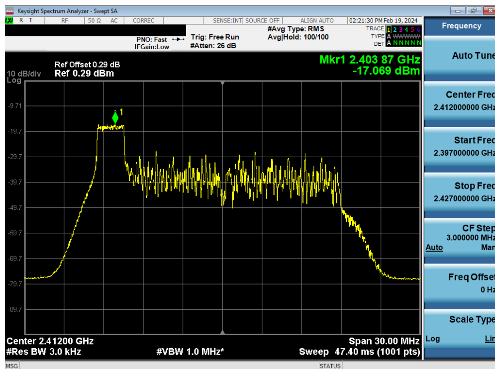
Plot 7-73. Power Spectral Density Plot Antenna WF8 (802.11ax OFDMA – RU26 Index 0 – Ch. 1)
