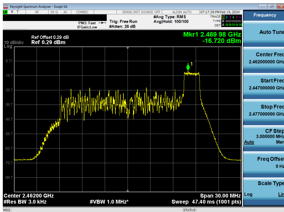
Plot 7-90. Power Spectral Density Plot Antenna WF7 (802.11ax OFDMA – RU26 Index 8 – Ch. 11)
