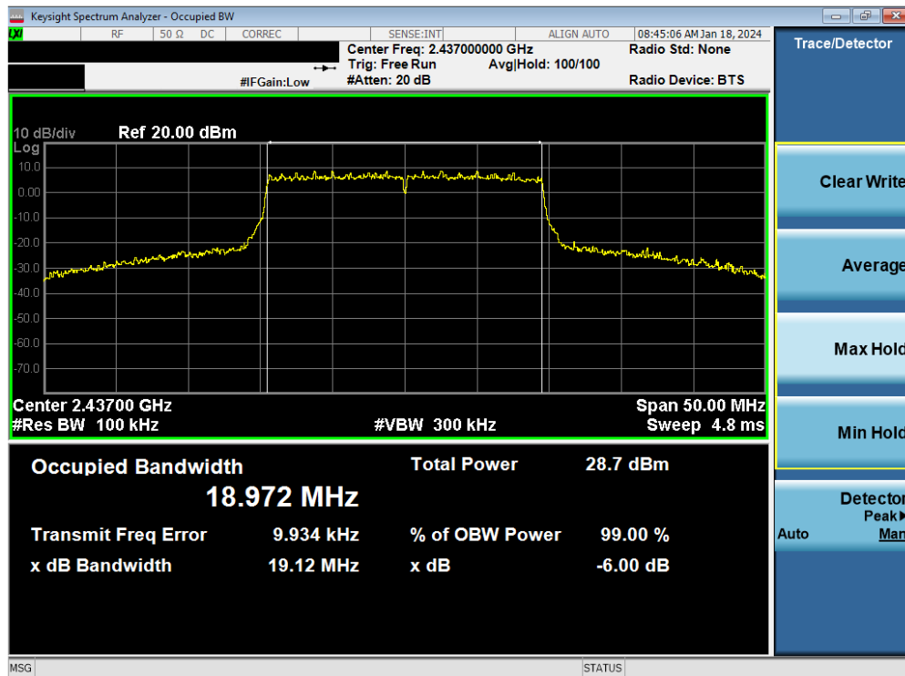
Plot 7-23. 6dB BW & 99% OBW Plot Antenna WF7 (802.11ax OFDMA – RU242 – Ch. 6)
