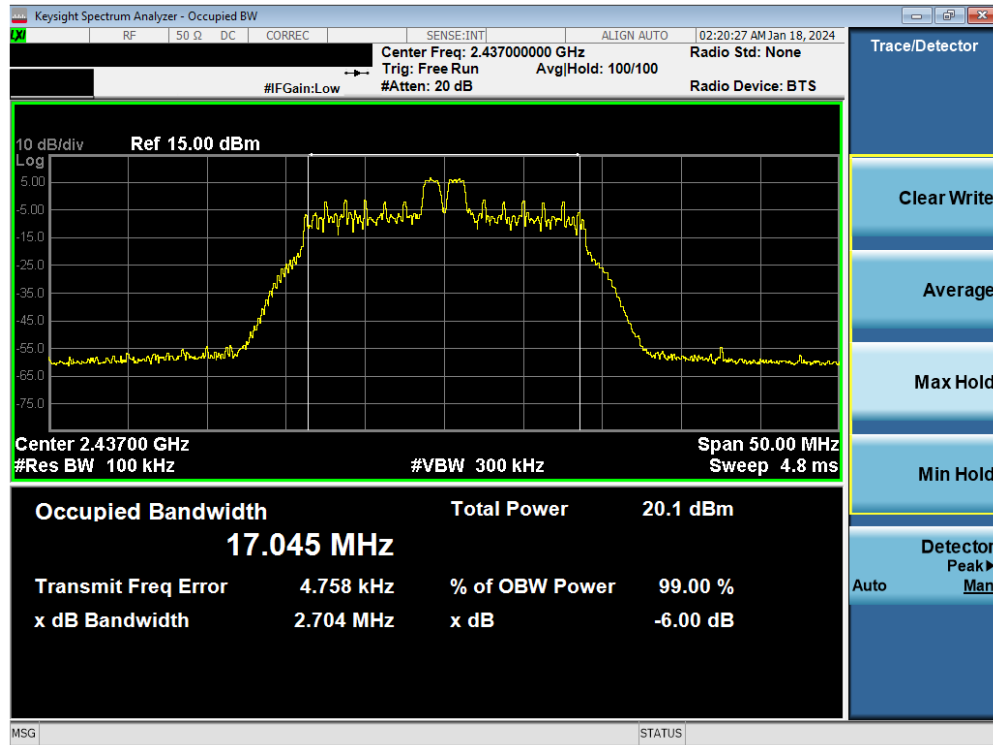
Plot 7-5. 6dB BW & 99% OBW Plot Antenna WF8 (802.11ax OFDMA – RU26 Index 4 – Ch. 6)
