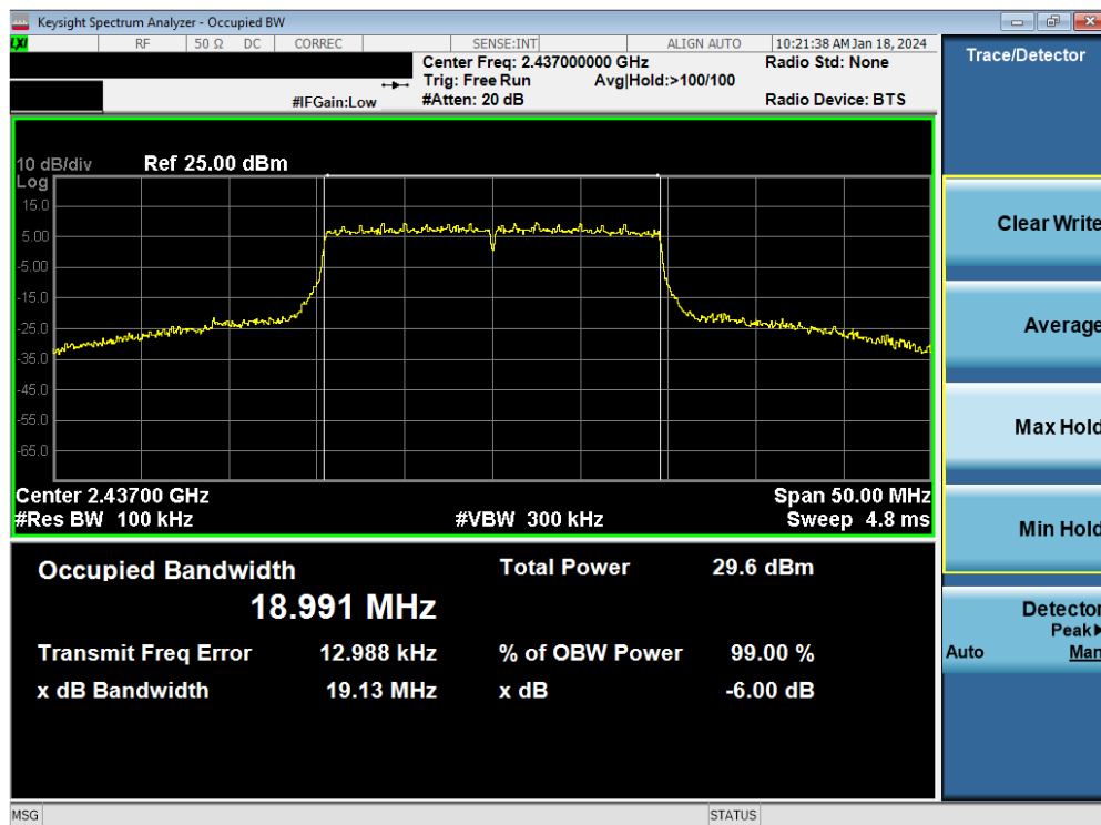
Plot 7-35. 6dB BW & 99% OBW Plot Antenna WF9 (802.11ax OFDMA – RU242 – Ch. 6)
