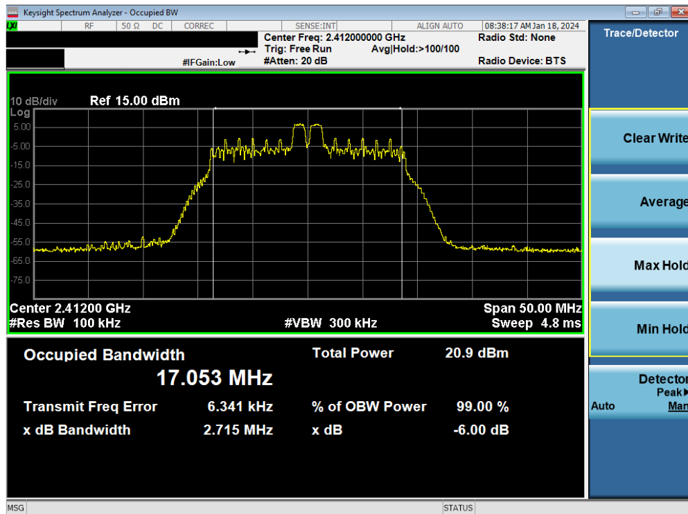
Plot 7-14. 6dB BW & 99% OBW Plot Antenna WF7 (802.11ax OFDMA – RU26 Index 4 – Ch. 1)
