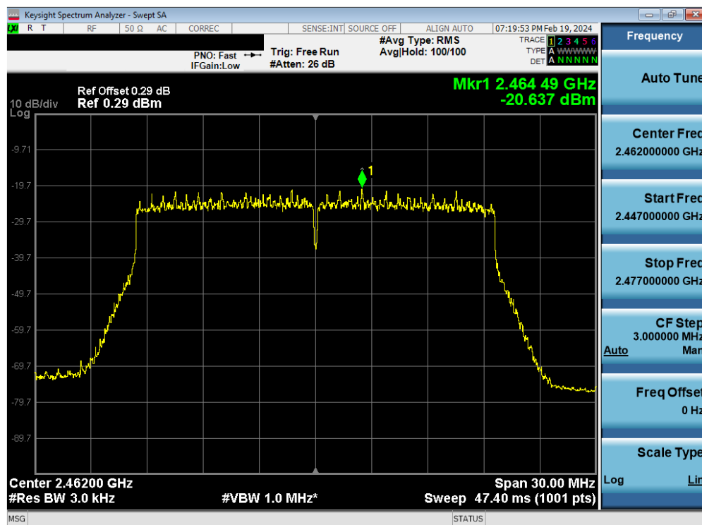
Plot 7-96. Power Spectral Density Plot Antenna WF7 (802.11ax OFDMA – RU242 – Ch. 11)
