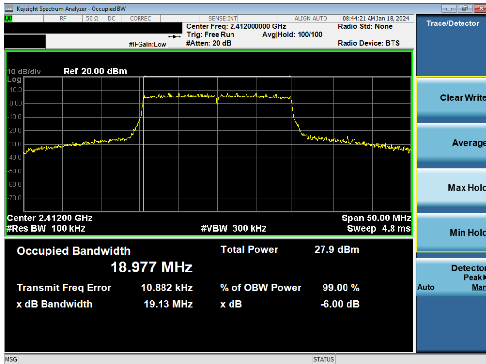
Plot 7-22. 6dB BW & 99% OBW Plot Antenna WF7 (802.11ax OFDMA – RU242 – Ch. 1)
