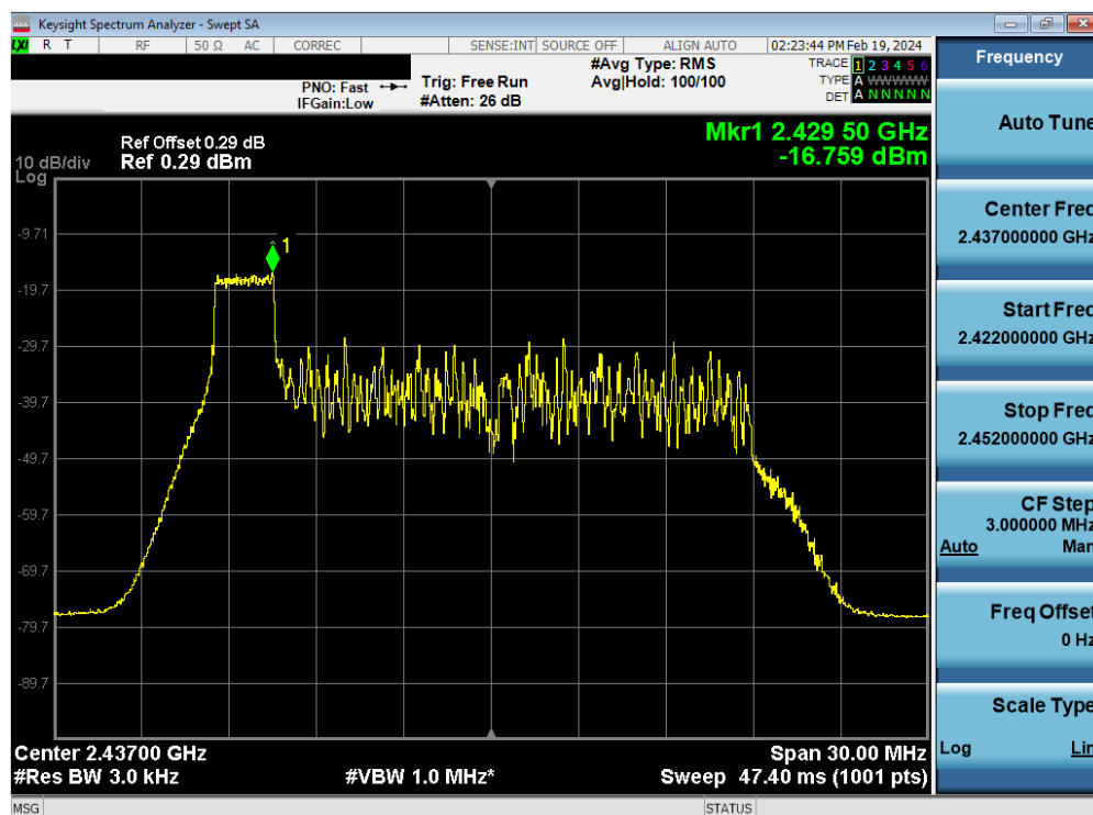
Plot 7-79. Power Spectral Density Plot Antenna WF8 (802.11ax OFDMA – RU26 Index 0 – Ch. 6)
