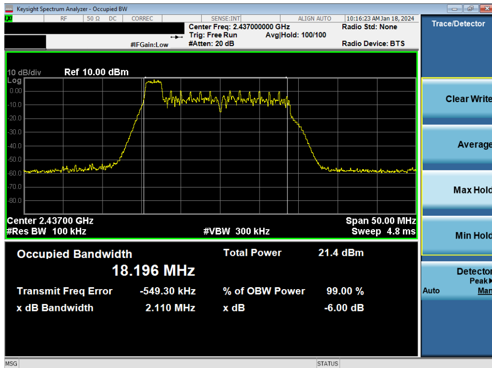
Plot 7-28. 6dB BW & 99% OBW Plot Antenna WF9 (802.11ax OFDMA – RU26 Index 0 – Ch. 6)
