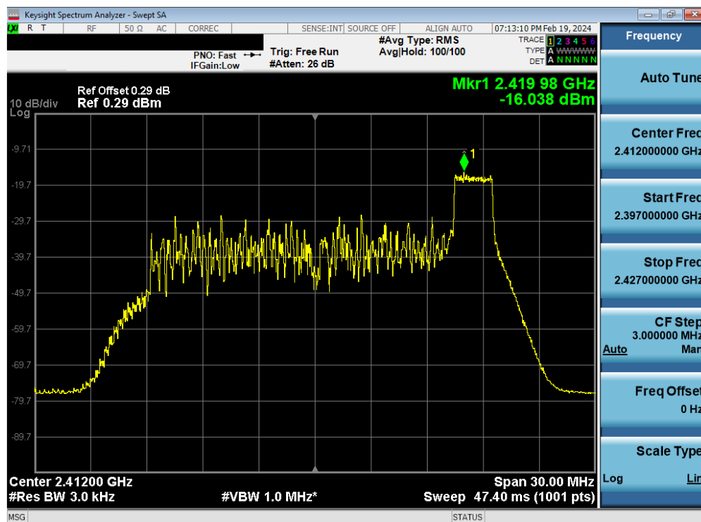
Plot 7-78. Power Spectral Density Plot Antenna WF7 (802.11ax OFDMA – RU26 Index 8 – Ch. 1)
