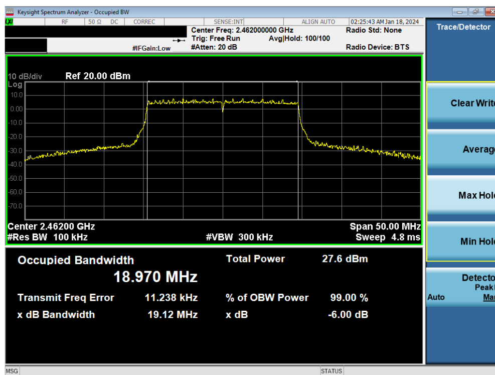
Plot 7-12. 6dB BW & 99% OBW Plot Antenna WF8 (802.11ax OFDMA – RU242 – Ch. 11)
