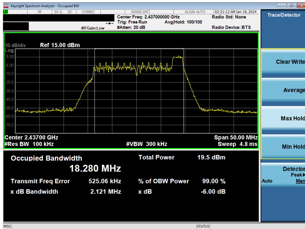
Plot 7-6. 6dB BW & 99% OBW Antenna WF8 (802.11ax OFDMA – RU26 Index 8 – Ch. 6)
