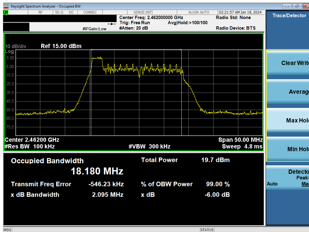
Plot 7-7. 6dB BW & 99% OBW Antenna WF8 (802.11ax OFDMA – RU26 Index 0 – Ch. 11)
