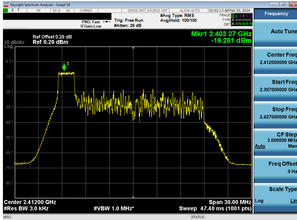
Plot 7-97. Power Spectral Density Plot Antenna WF9 (802.11ax OFDMA – RU26 Index 0 – Ch. 1)
