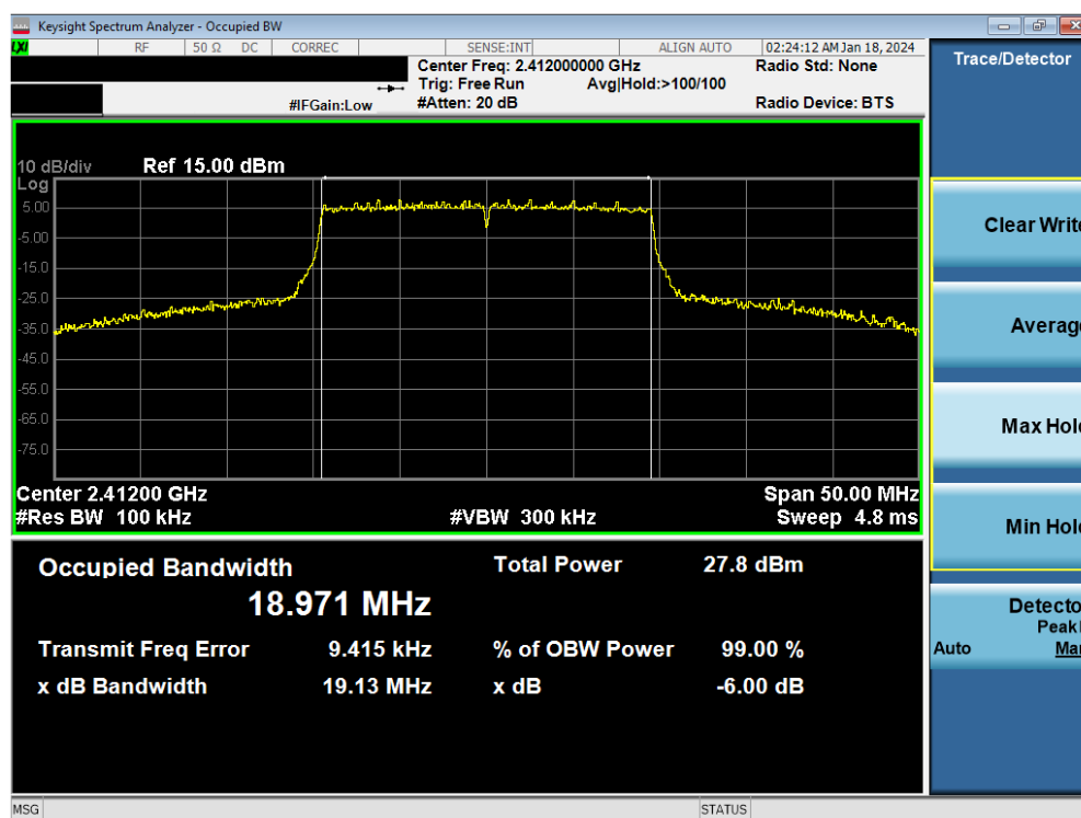
Plot 7-10. 6dB BW & 99% OBW Plot Antenna WF8 (802.11ax OFDMA – RU242 – Ch. 1)
