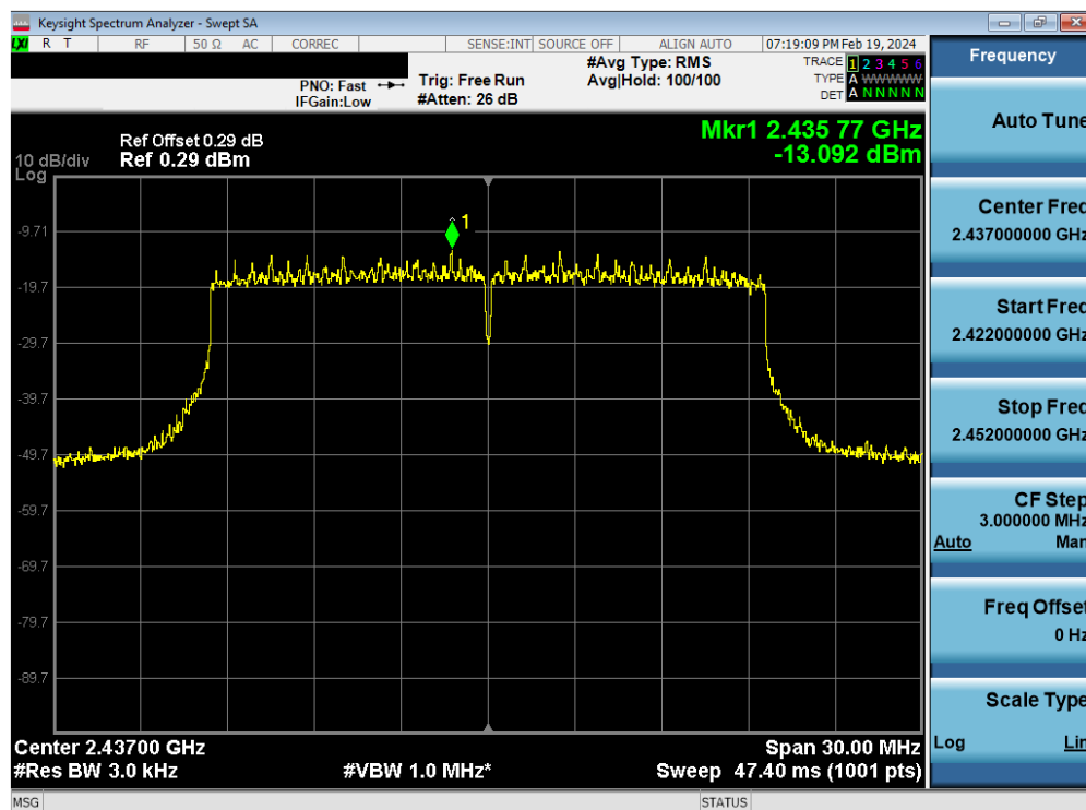
Plot 7-94. Power Spectral Density Plot Antenna WF7 (802.11ax OFDMA – RU242 – Ch. 6)
