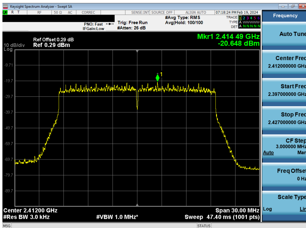
Plot 7-92. Power Spectral Density Plot Antenna WF7 (802.11ax OFDMA – RU242 – Ch. 1)
