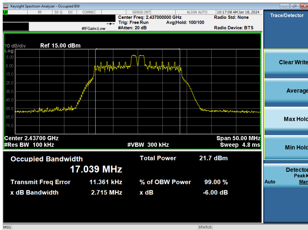
Plot 7-29. 6dB BW & 99% OBW Plot Antenna WF9 (802.11ax OFDMA – RU26 Index 4 – Ch. 6)
