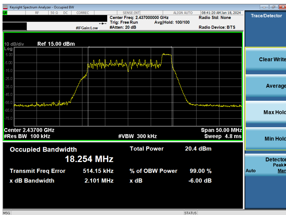
Plot 7-18. 6dB BW & 99% OBW Antenna WF7 (802.11ax OFDMA – RU26 Index 8 – Ch. 6)
