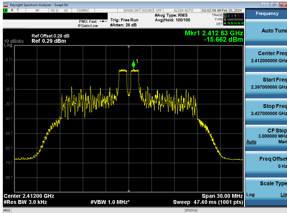
Plot 7-98. Power Spectral Density Plot Antenna WF9 (802.11ax OFDMA – RU26 Index 4 – Ch. 1)
