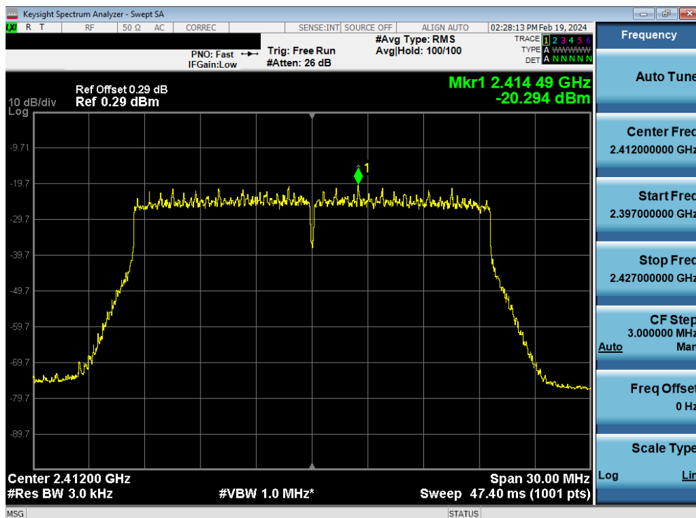
Plot 7-91. Power Spectral Density Plot Antenna WF8 (802.11ax OFDMA – RU242 – Ch. 1)
