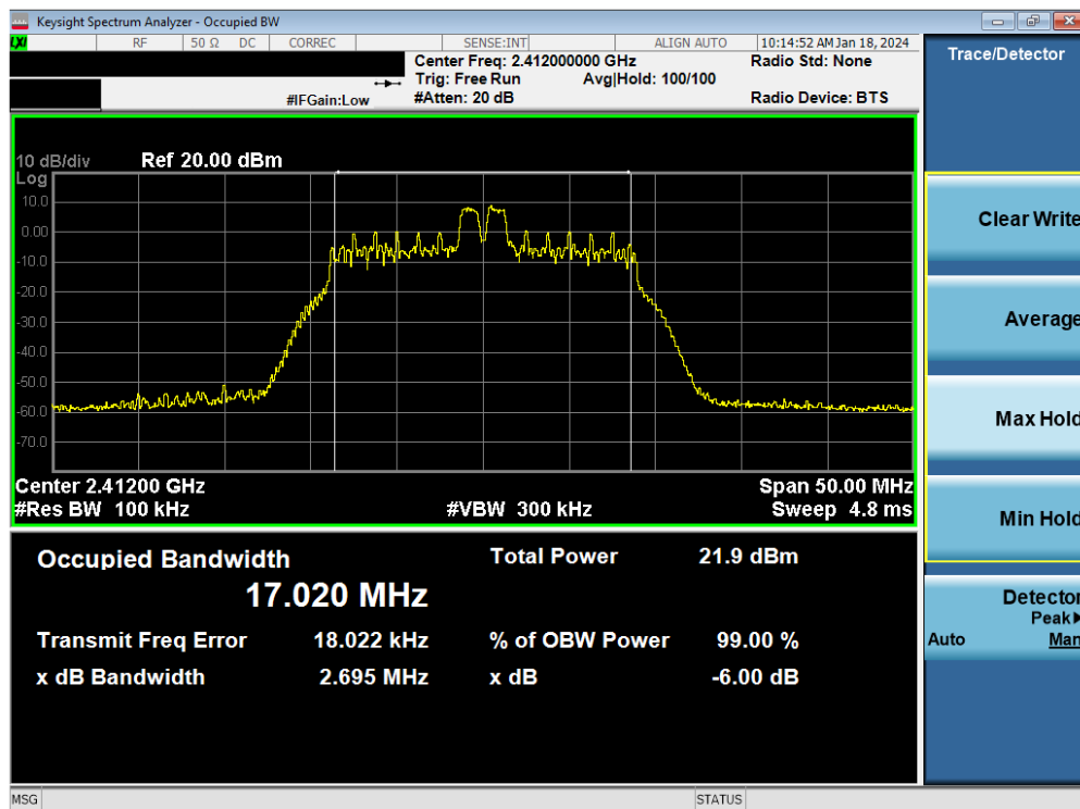
Plot 7-26. 6dB BW & 99% OBW Plot Antenna WF9 (802.11ax OFDMA – RU26 Index 4 – Ch. 1)
