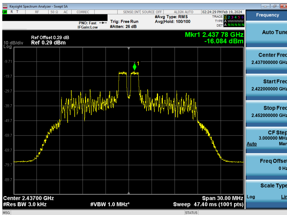
Plot 7-81. Power Spectral Density Plot Antenna WF8 (802.11ax OFDMA – RU26 Index 4 – Ch. 6)
