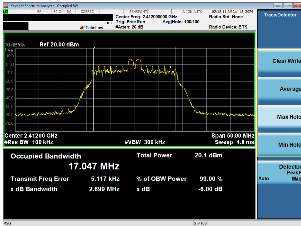
Plot 7-2. 6dB BW & 99% OBW Plot Antenna WF8 (802.11ax OFDMA – RU26 Index 4 – Ch. 1)
