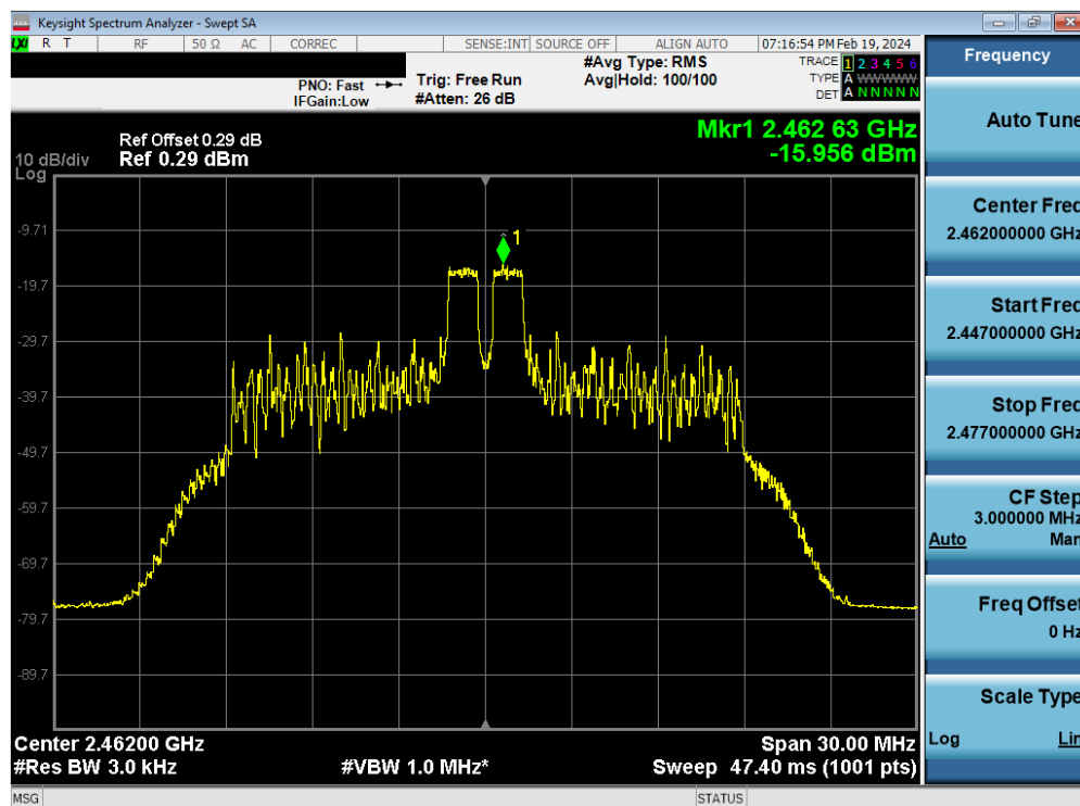
Plot 7-88. Power Spectral Density Plot Antenna WF7 (802.11ax OFDMA – RU26 Index 4 – Ch. 11)
