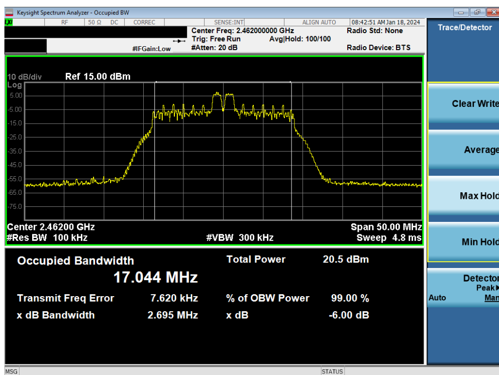
Plot 7-20. 6dB BW & 99% OBW Antenna WF7 (802.11ax OFDMA – RU26 Index 4 – Ch. 11)
