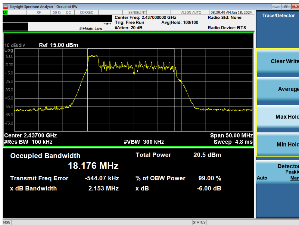
Plot 7-16. 6dB BW & 99% OBW Plot Antenna WF7 (802.11ax OFDMA – RU26 Index 0 – Ch. 6)
