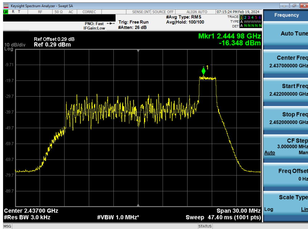
Plot 7-84. Power Spectral Density Plot Antenna WF7 (802.11ax OFDMA – RU26 Index 8 – Ch. 6)
