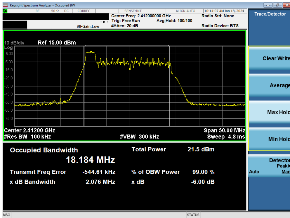
Plot 7-25. 6dB BW & 99% OBW Plot Antenna WF9 (802.11ax OFDMA – RU26 Index 0 – Ch. 1)
