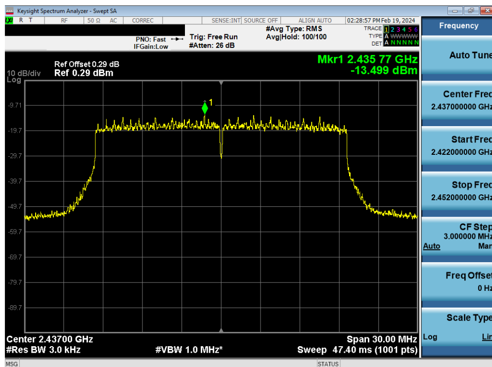
Plot 7-93. Power Spectral Density Plot Antenna WF8 (802.11ax OFDMA – RU242 – Ch. 6)
