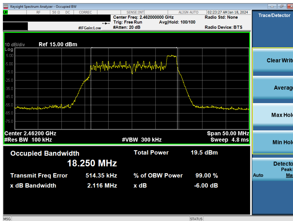
Plot 7-9. 6dB BW & 99% OBW Plot Antenna WF8 (802.11ax OFDMA – RU26 Index 8 – Ch. 11)
