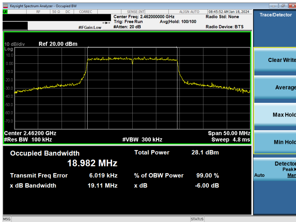
Plot 7-24. 6dB BW & 99% OBW Plot Antenna WF7 (802.11ax OFDMA – RU242 – Ch. 11)
