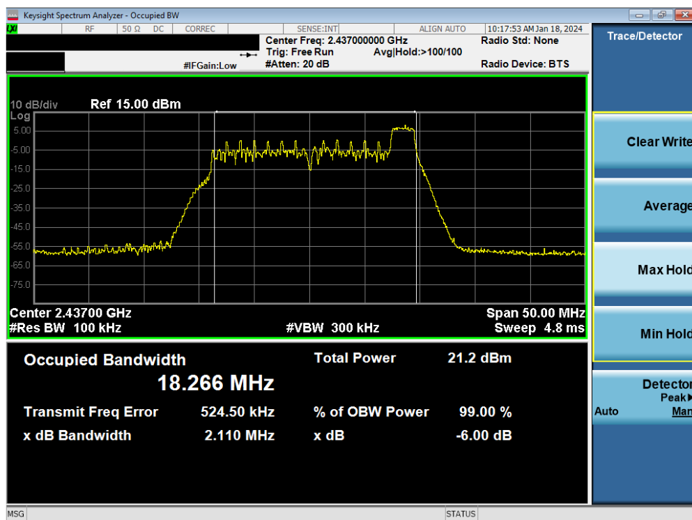
Plot 7-30. 6dB BW & 99% OBW Antenna WF9 (802.11ax OFDMA – RU26 Index 8 – Ch. 6)
