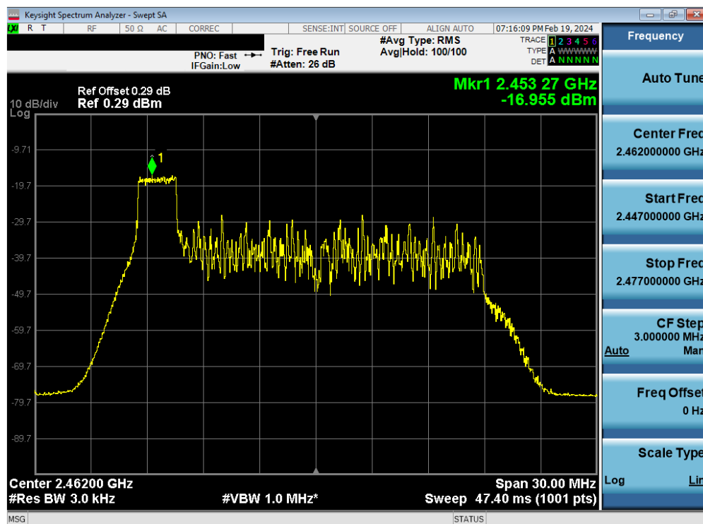
Plot 7-86. Power Spectral Density Plot Antenna WF7 (802.11ax OFDMA – RU26 Index 0 – Ch. 11)
