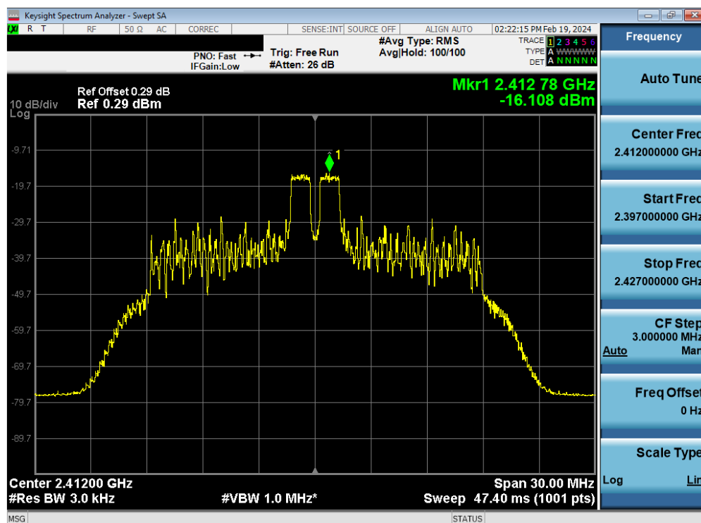
Plot 7-75. Power Spectral Density Plot Antenna WF8 (802.11ax OFDMA – RU26 Index 4 – Ch. 1)
