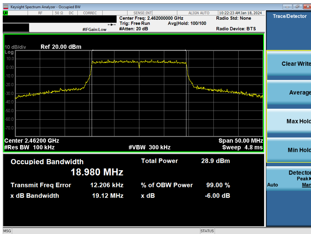
Plot 7-36. 6dB BW & 99% OBW Plot Antenna WF9 (802.11ax OFDMA – RU242 – Ch. 11)
