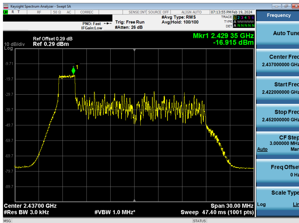
Plot 7-80. Power Spectral Density Plot Antenna WF7 (802.11ax OFDMA – RU26 Index 0 – Ch. 6)
