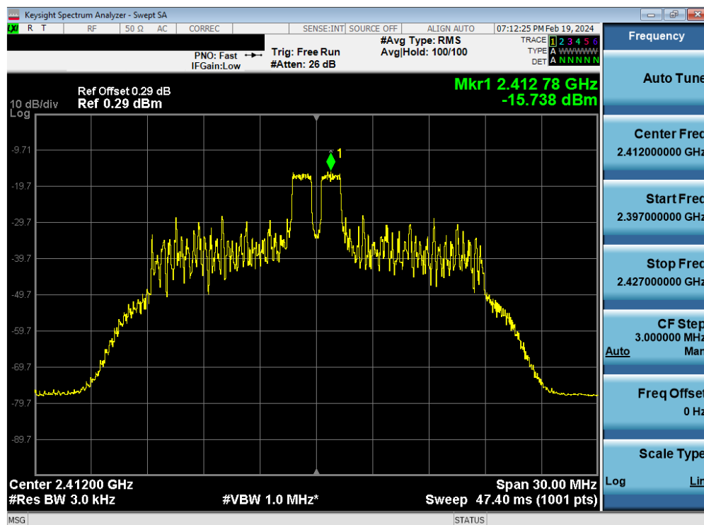
Plot 7-76. Power Spectral Density Plot Antenna WF7 (802.11ax OFDMA – RU26 Index 4 – Ch. 1)
