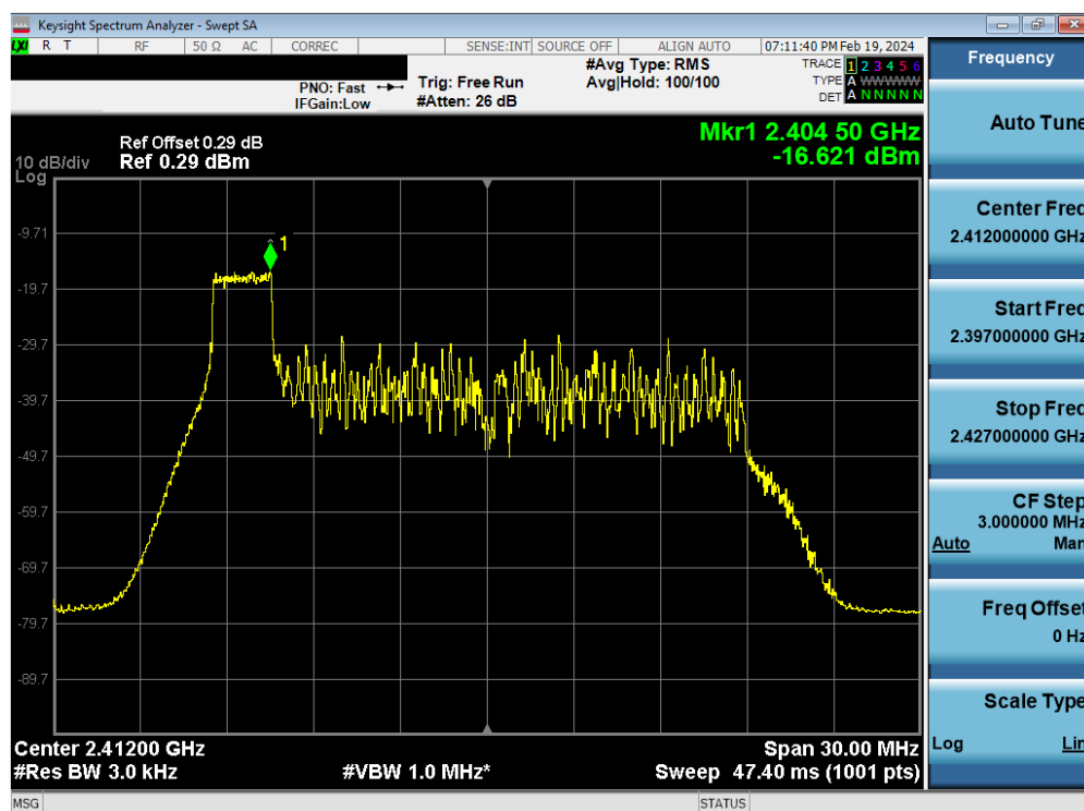
Plot 7-74. Power Spectral Density Plot Antenna WF7 (802.11ax OFDMA – RU26 Index 0 – Ch. 1)
