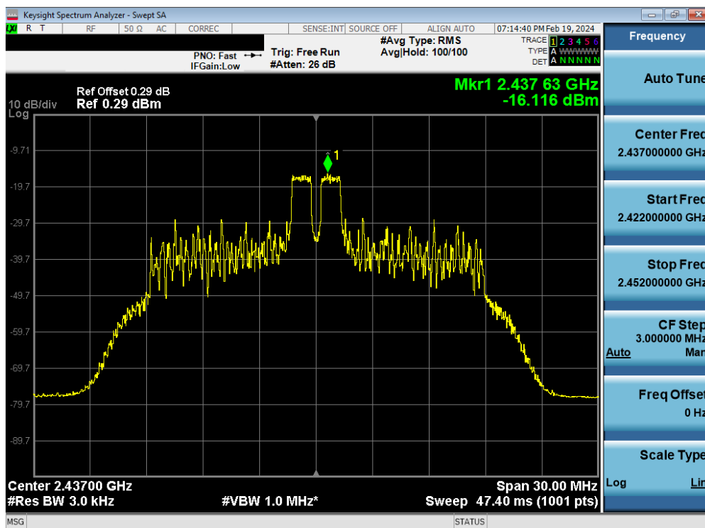
Plot 7-82. Power Spectral Density Plot Antenna WF7 (802.11ax OFDMA – RU26 Index 4 – Ch. 6)
