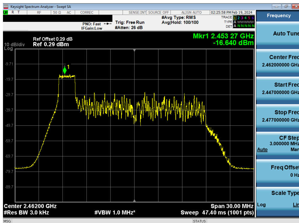
Plot 7-85. Power Spectral Density Plot Antenna WF8 (802.11ax OFDMA – RU26 Index 0 – Ch. 11)
