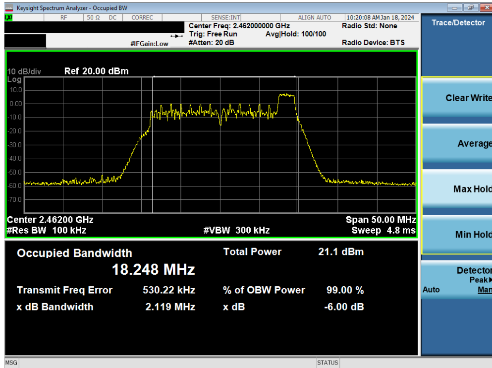
Plot 7-33. 6dB BW & 99% OBW Plot Antenna WF9 (802.11ax OFDMA – RU26 Index 8 – Ch. 11)
