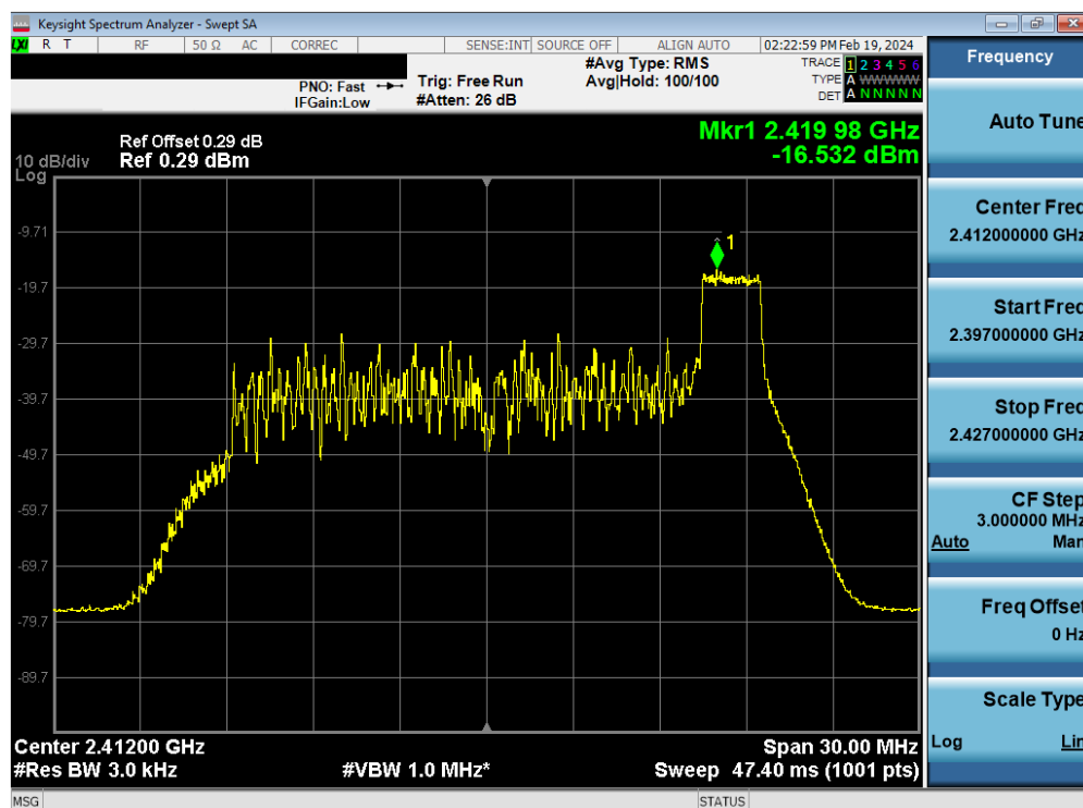
Plot 7-77. Power Spectral Density Plot Antenna WF8 (802.11ax OFDMA – RU26 Index 8 – Ch. 1)
