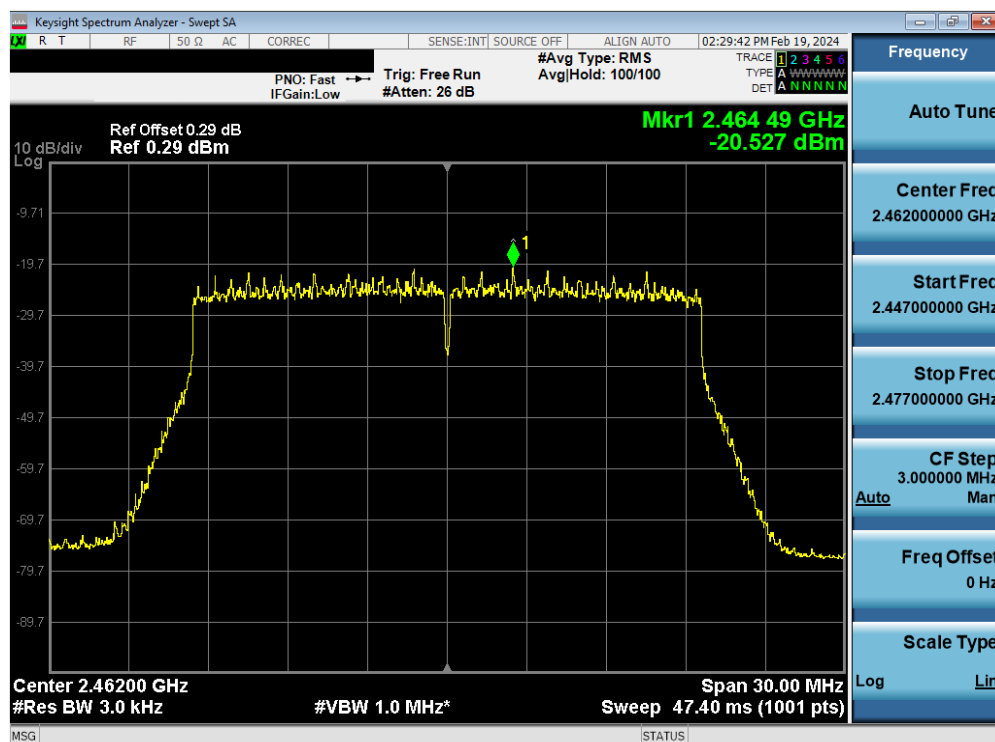
Plot 7-95. Power Spectral Density Plot Antenna WF8 (802.11ax OFDMA – RU242 – Ch. 11)
