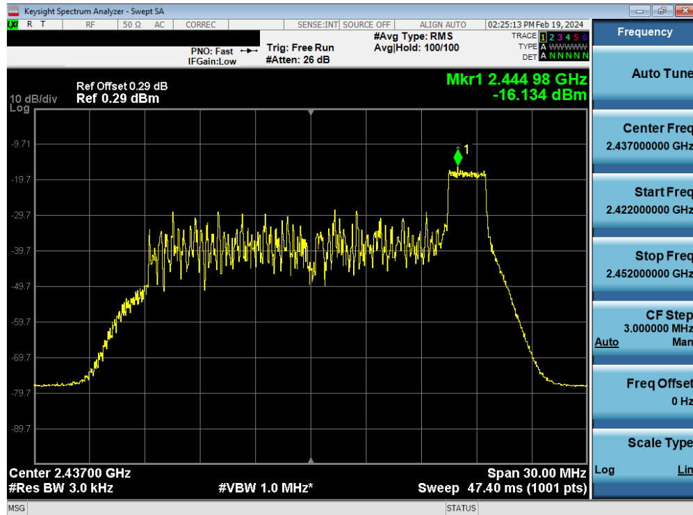
Plot 7-83. Power Spectral Density Plot Antenna WF8 (802.11ax OFDMA – RU26 Index 8 – Ch. 6)
