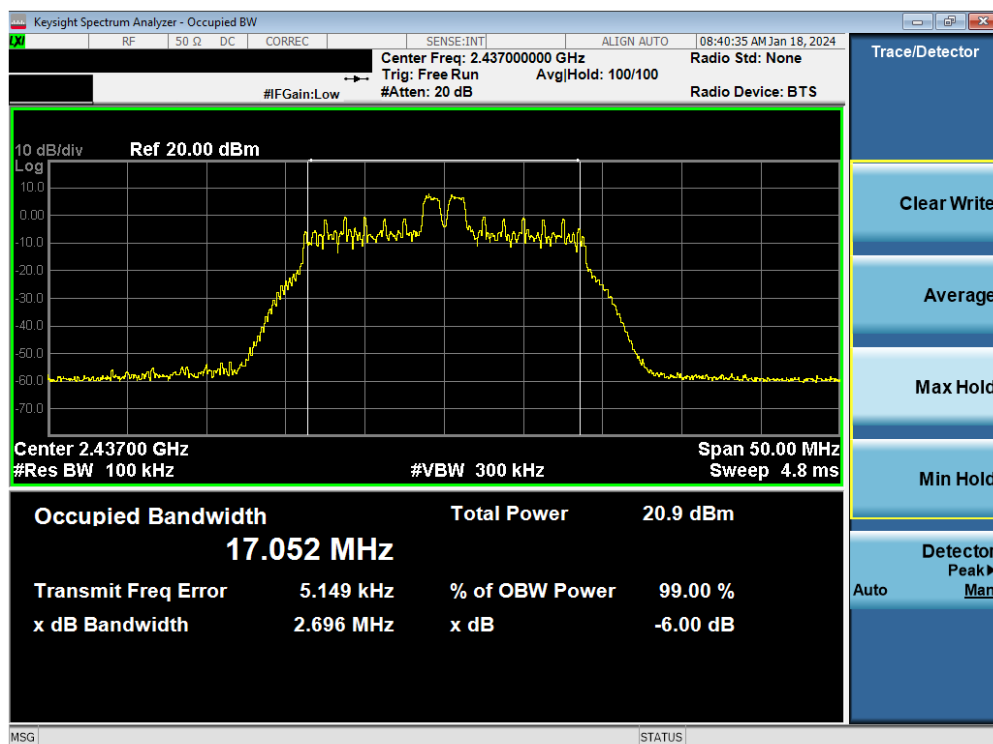
Plot 7-17. 6dB BW & 99% OBW Plot Antenna WF7 (802.11ax OFDMA – RU26 Index 4 – Ch. 6)
