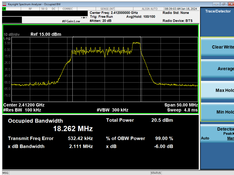
Plot 7-15. 6dB BW & 99% OBW Plot Antenna WF7 (802.11ax OFDMA – RU26 Index 8 – Ch. 1)
