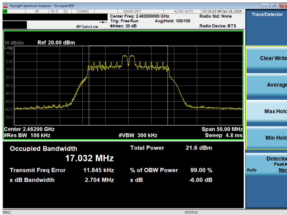
Plot 7-32. 6dB BW & 99% OBW Antenna WF9 (802.11ax OFDMA – RU26 Index 4 – Ch. 11)
