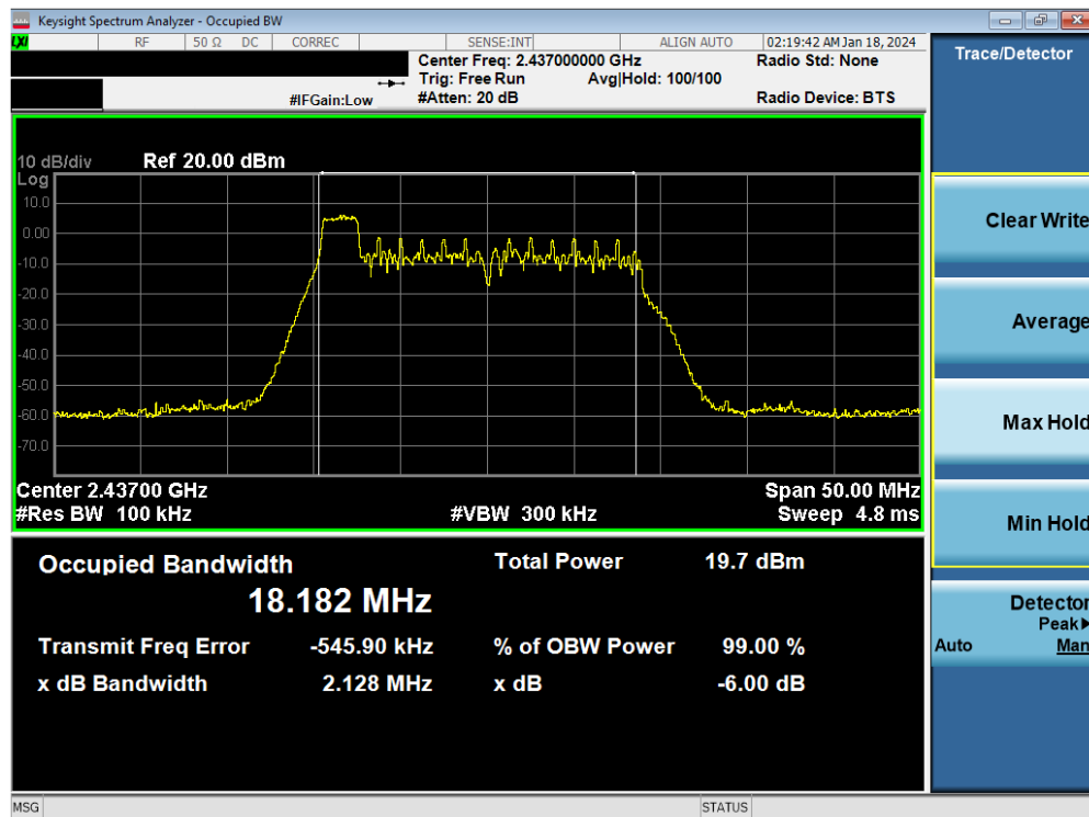
Plot 7-4. 6dB BW & 99% OBW Plot Antenna WF8 (802.11ax OFDMA – RU26 Index 0 – Ch. 6)
