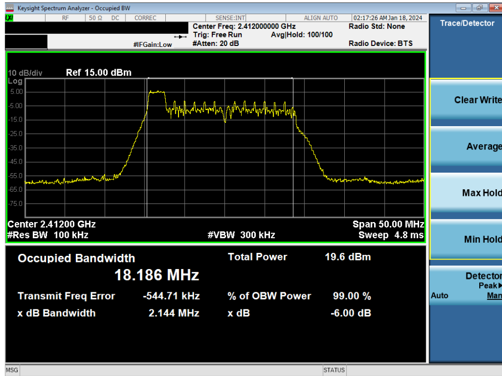
Plot 7-1. 6dB BW & 99% OBW Plot Antenna WF8 (802.11ax OFDMA – RU26 Index 0 – Ch. 1)
