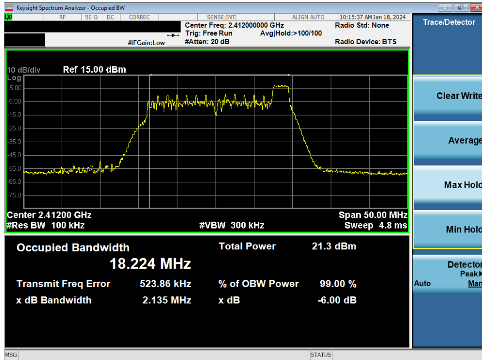
Plot 7-27. 6dB BW & 99% OBW Plot Antenna WF9 (802.11ax OFDMA – RU26 Index 8 – Ch. 1)
