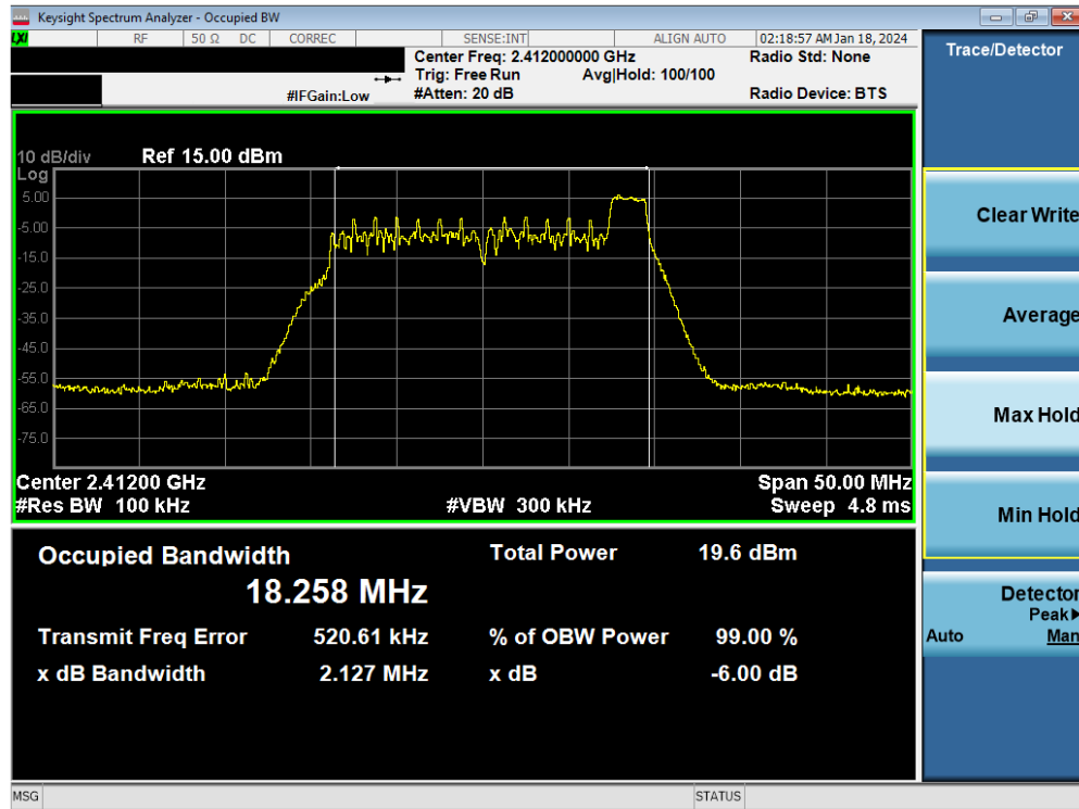
Plot 7-3. 6dB BW & 99% OBW Plot Antenna WF8 (802.11ax OFDMA – RU26 Index 8 – Ch. 1)
