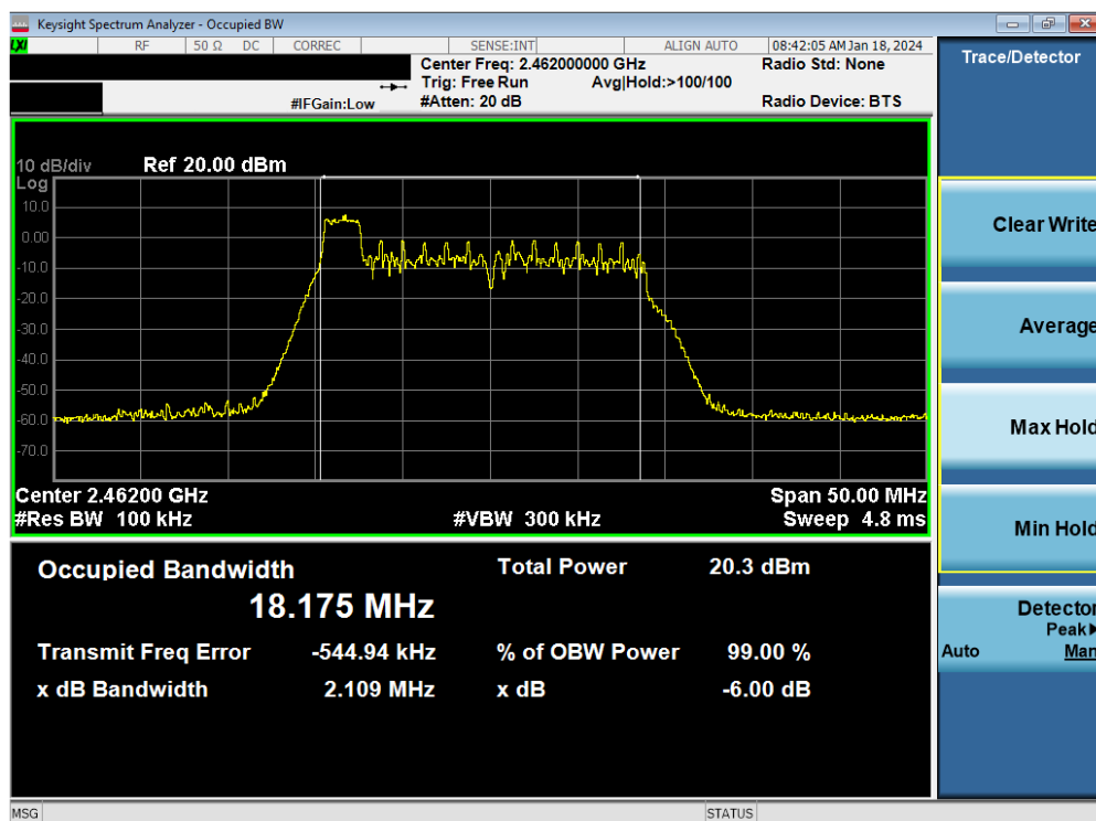
Plot 7-19. 6dB BW & 99% OBW Antenna WF7 (802.11ax OFDMA – RU26 Index 0 – Ch. 11)
