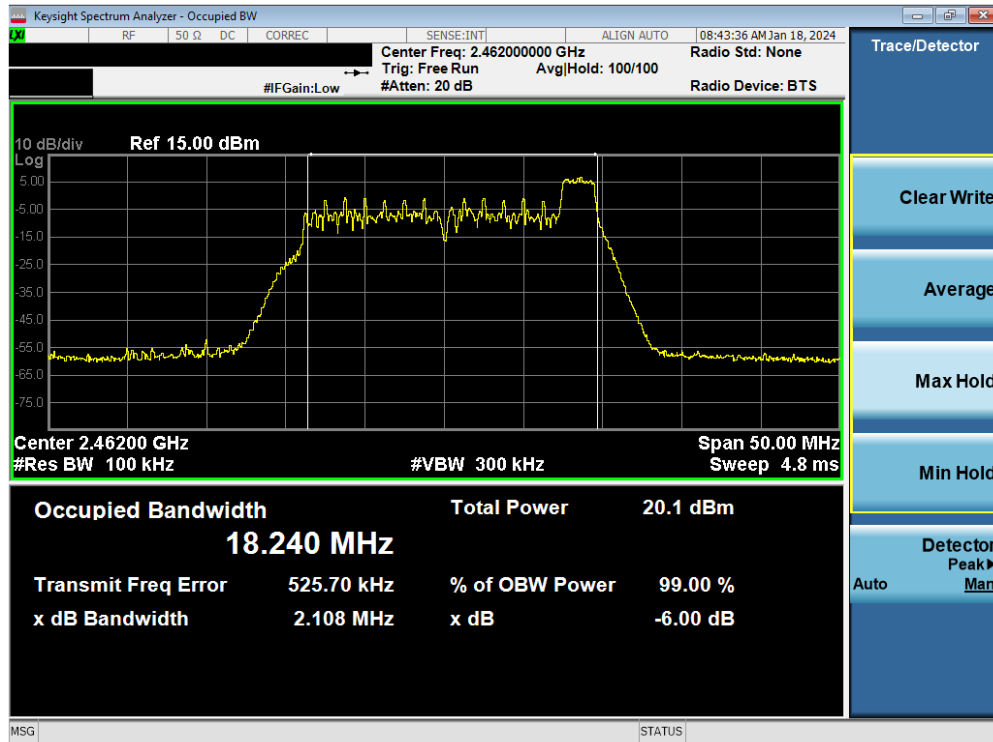
Plot 7-21. 6dB BW & 99% OBW Plot Antenna WF7 (802.11ax OFDMA – RU26 Index 8 – Ch. 11)
