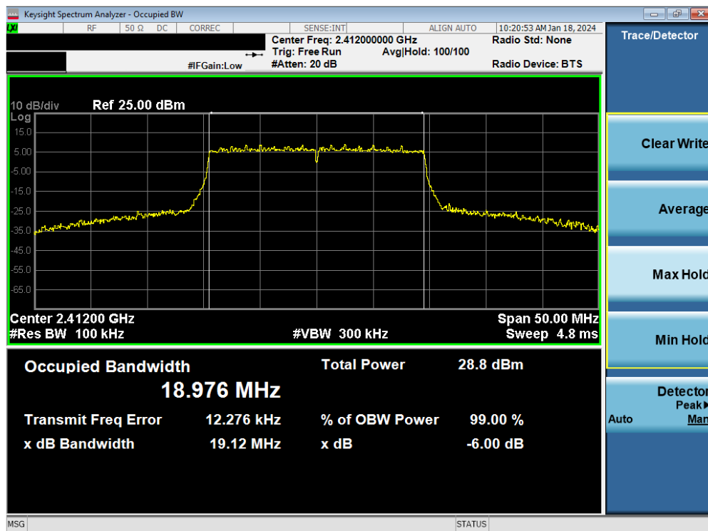
Plot 7-34. 6dB BW & 99% OBW Plot Antenna WF9 (802.11ax OFDMA – RU242 – Ch. 1)
