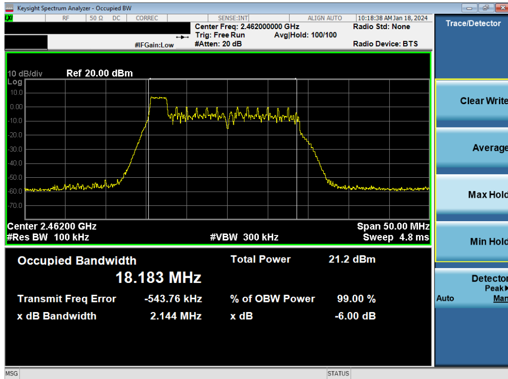
Plot 7-31. 6dB BW & 99% OBW Antenna WF9 (802.11ax OFDMA – RU26 Index 0 – Ch. 11)
