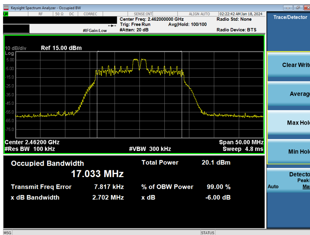
Plot 7-8. 6dB BW & 99% OBW Antenna WF8 (802.11ax OFDMA – RU26 Index 4 – Ch. 11)
