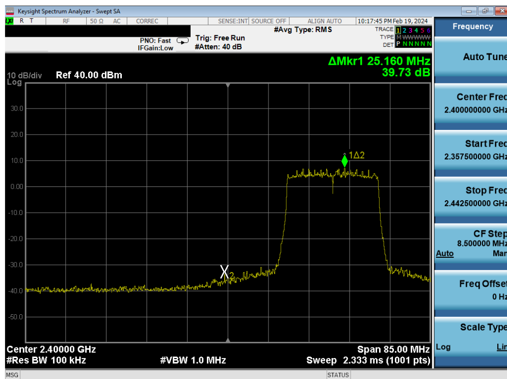
Plot 7-128. Band Edge Antenna WF7 (802.11ax OFDMA – RU242 – Ch. 3)
