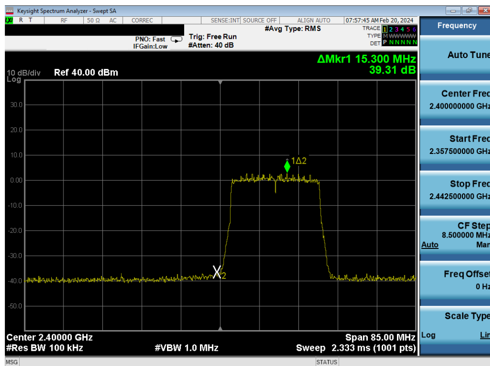
Plot 7-141. Band Edge Antenna WF9 (802.11ax OFDMA – RU242 – Ch. 1)
