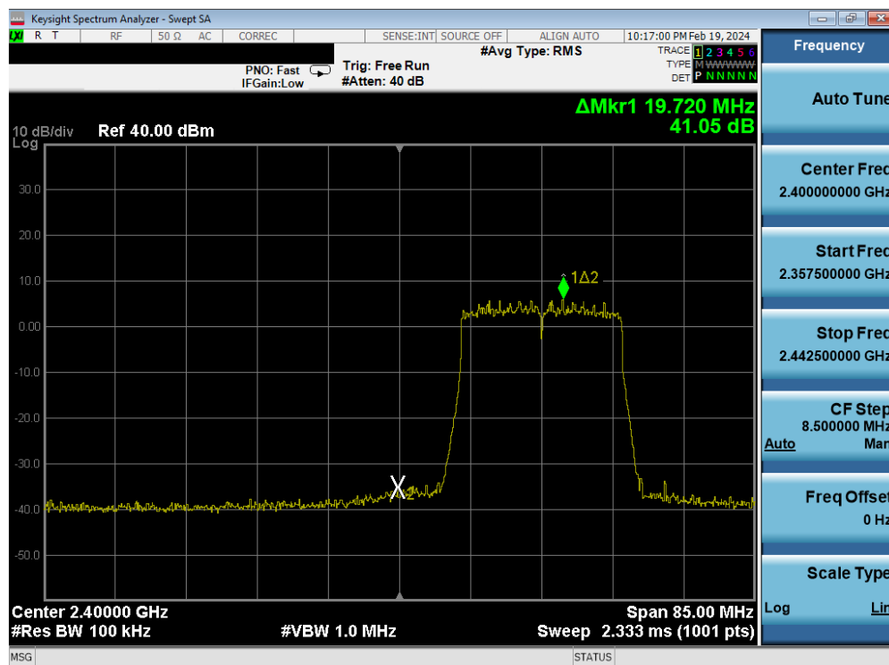
Plot 7-127. Band Edge Antenna WF7 (802.11ax OFDMA – RU242 – Ch. 2)
