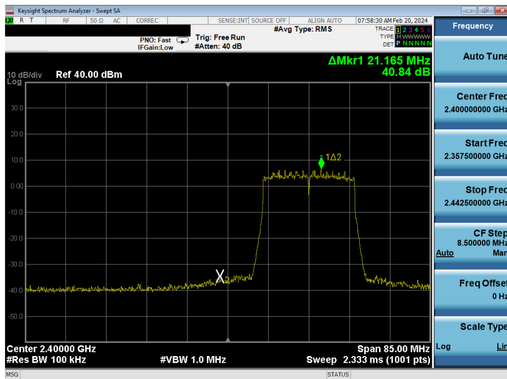
Plot 7-142. Band Edge Antenna WF9 (802.11ax OFDMA – RU242 – Ch. 2)
