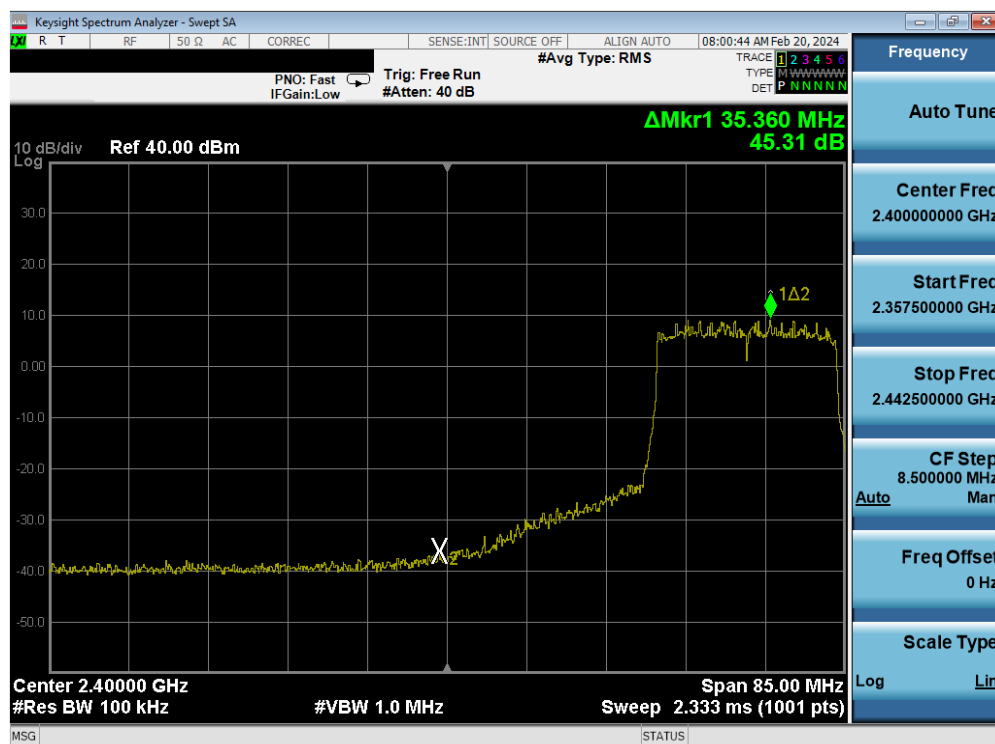
Plot 7-145. Band Edge Antenna WF9 (802.11ax OFDMA – RU242 – Ch. 5)
