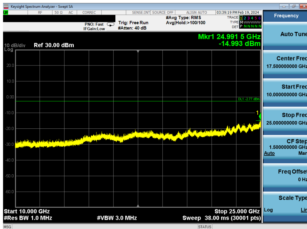
Plot 7-159. Conducted Spurious Plot Antenna WF8 (802.11ax OFDMA – RU26 – Ch. 11)
