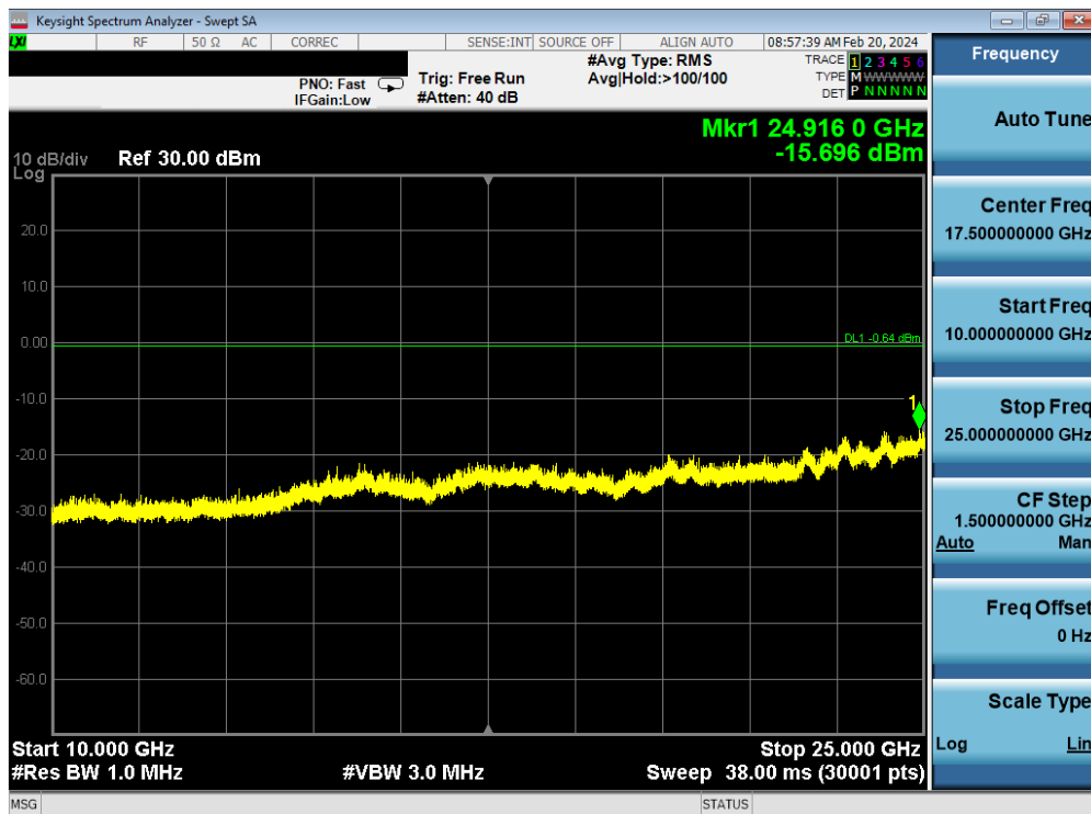
Plot 7-187. Conducted Spurious Plot Antenna WF9 (802.11ax OFDMA – RU242 – Ch. 6)
