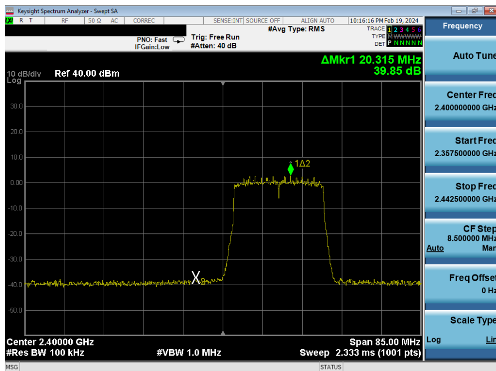
Plot 7-126. Band Edge Antenna WF7 (802.11ax OFDMA – RU242 – Ch. 1)
