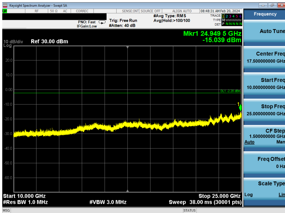
Plot 7-181. Conducted Spurious Plot Antenna WF9 (802.11ax OFDMA – RU26 – Ch. 6)
