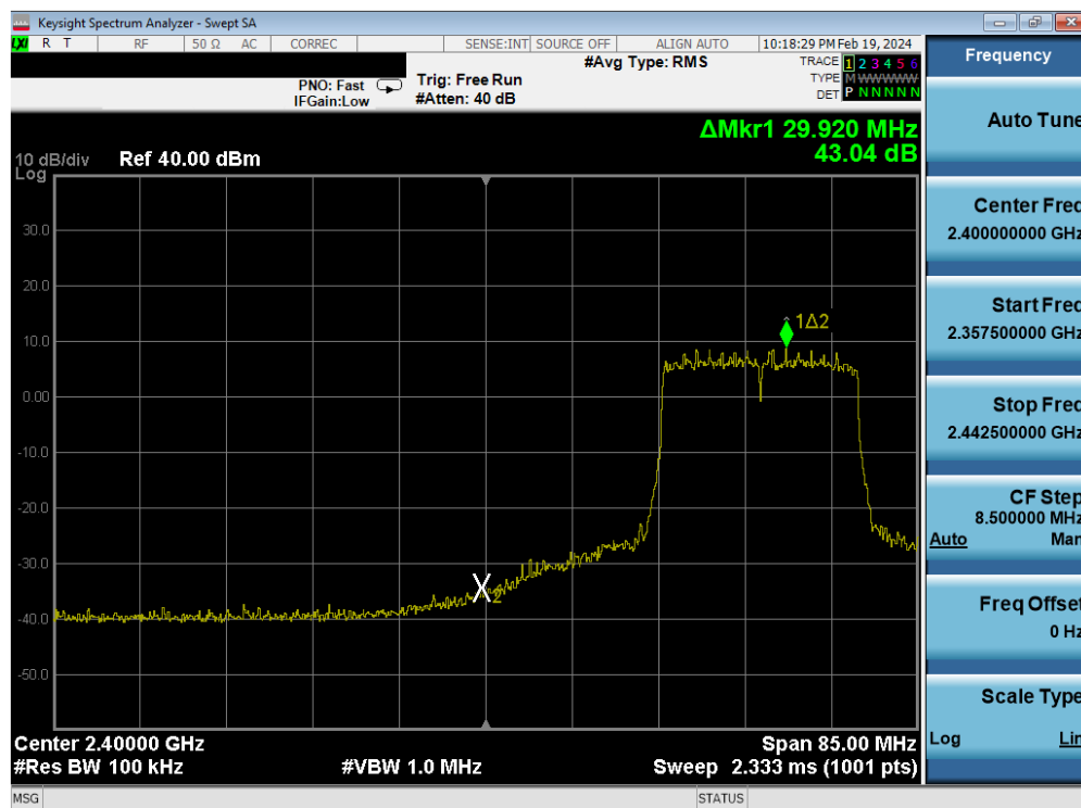
Plot 7-129. Band Edge Antenna WF7 (802.11ax OFDMA – RU242 – Ch. 4)
