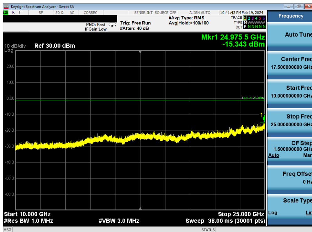
Plot 7-175. Conducted Spurious Plot Antenna WF7 (802.11ax OFDMA – RU242 – Ch. 6)
