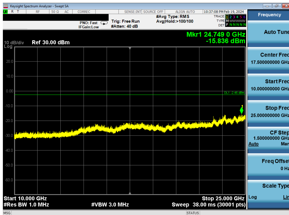
Plot 7-171. Conducted Spurious Plot Antenna WF7 (802.11ax OFDMA – RU26 – Ch. 11)
