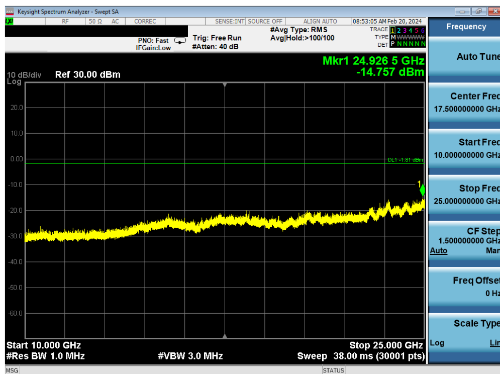
Plot 7-183. Conducted Spurious Plot Antenna WF9 (802.11ax OFDMA – RU26 – Ch. 11)
