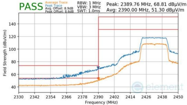
Plot 7-230 Radiated Restricted Lower Band Edge Measurement Antenna WF8 (Peak & Average – RU242)
