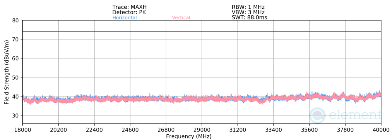
Plot 7-215. Radiated Spurious Emissions above 18GHz CDD Primary (802.11ax OFDMA – RU242 – Ch. 6)
