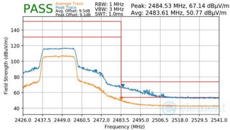
Plot 7-234 Radiated Restricted Upper Band Edge Measurement Antenna WF8 (Peak & Average – RU242)
