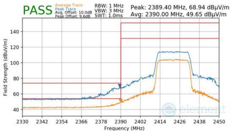
Plot 7-243 Radiated Restricted Lower Band Edge Measurement Antenna WF7 (Peak & Average – RU242)
