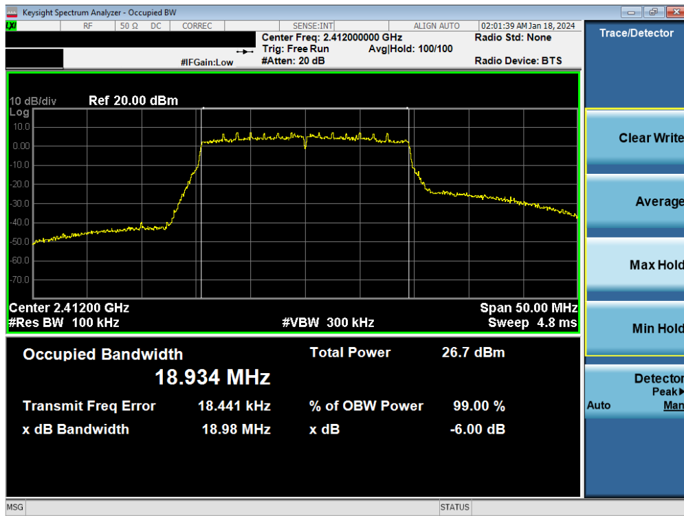
Plot 7-7. 6 dB BW and 99% OBW Plot Antenna WF8 (802.11ax (SU - 2.4GHz) – Ch. 1) – MCS2
