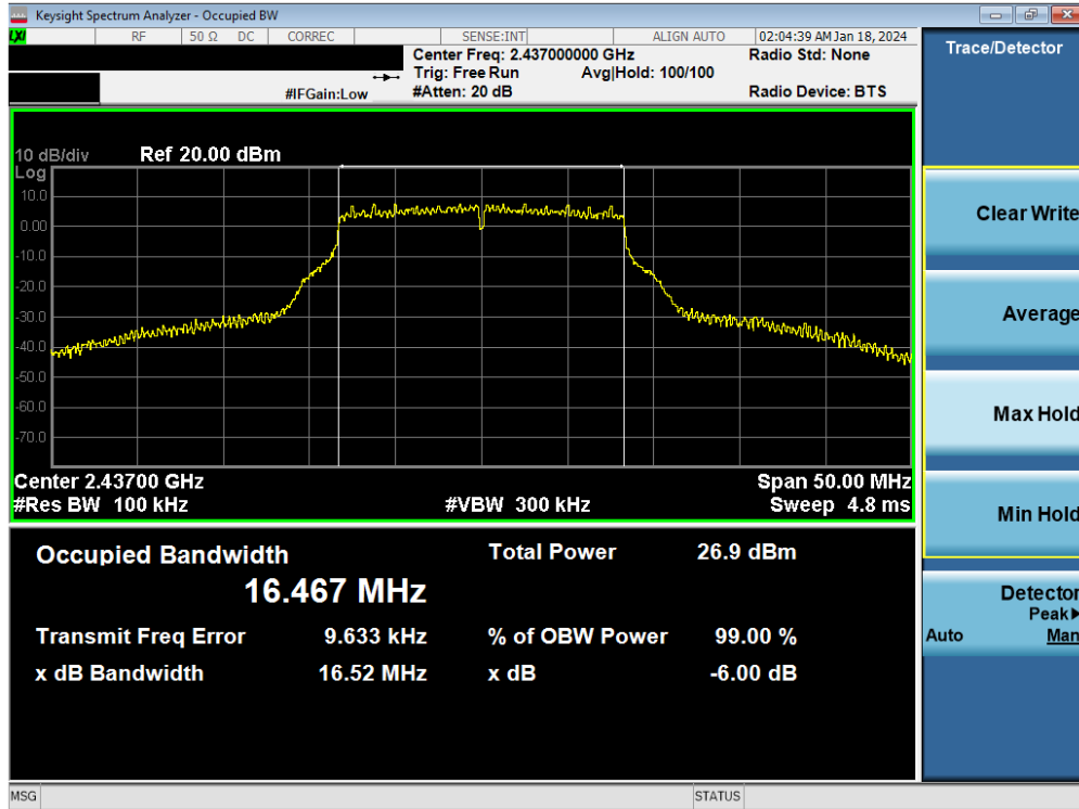
Plot 7-11. 6 dB BW and 99% OBW Plot Antenna WF8 (802.11g – Ch. 6) – 24Mbps
