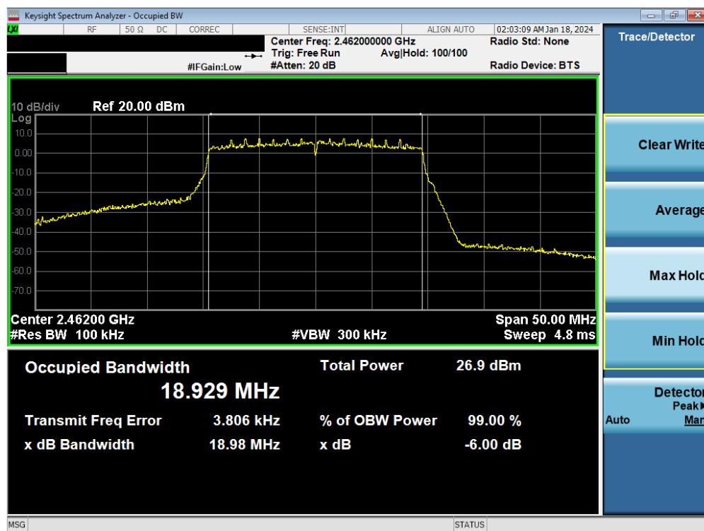
Plot 7-9. 6 dB BW and 99% OBW Plot Antenna WF8 (802.11ax (SU - 2.4GHz) – Ch. 11) – MCS2
