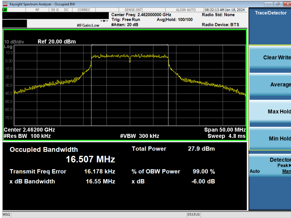
Plot 7-54. 6 dB BW and 99% OBW Plot Antenna WF7 (802.11g – Ch. 11) – 54Mbps
