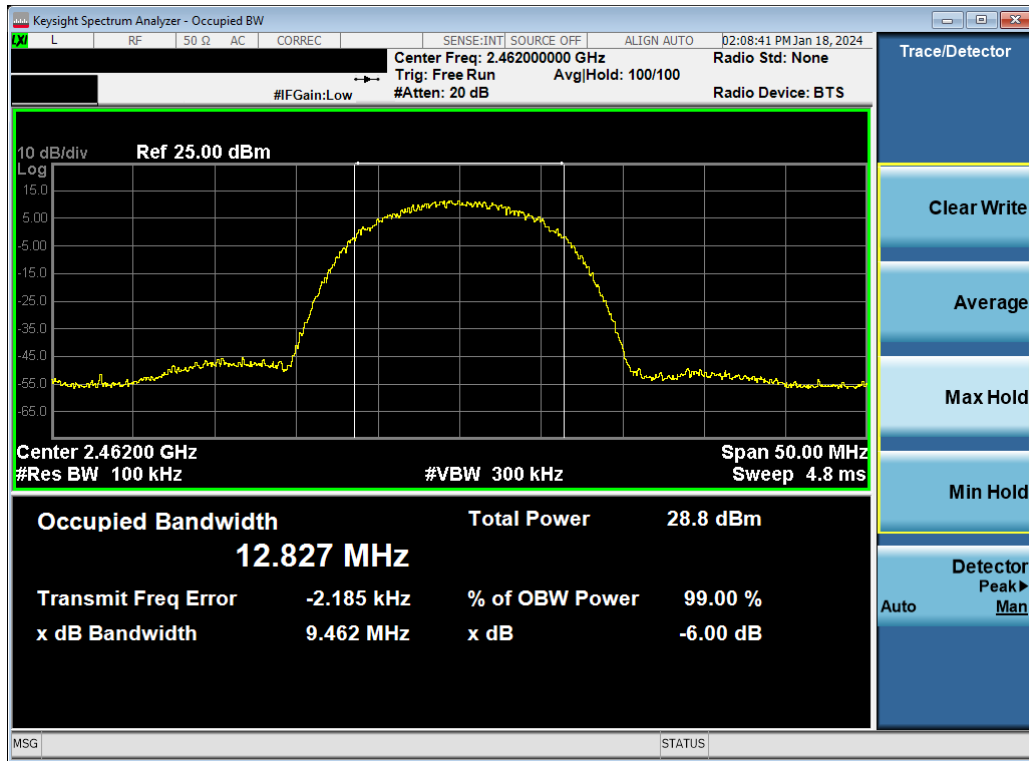
Plot 7-21. 6 dB BW and 99% OBW Plot Antenna WF8 (802.11b – Ch. 11) – 11Mbps
