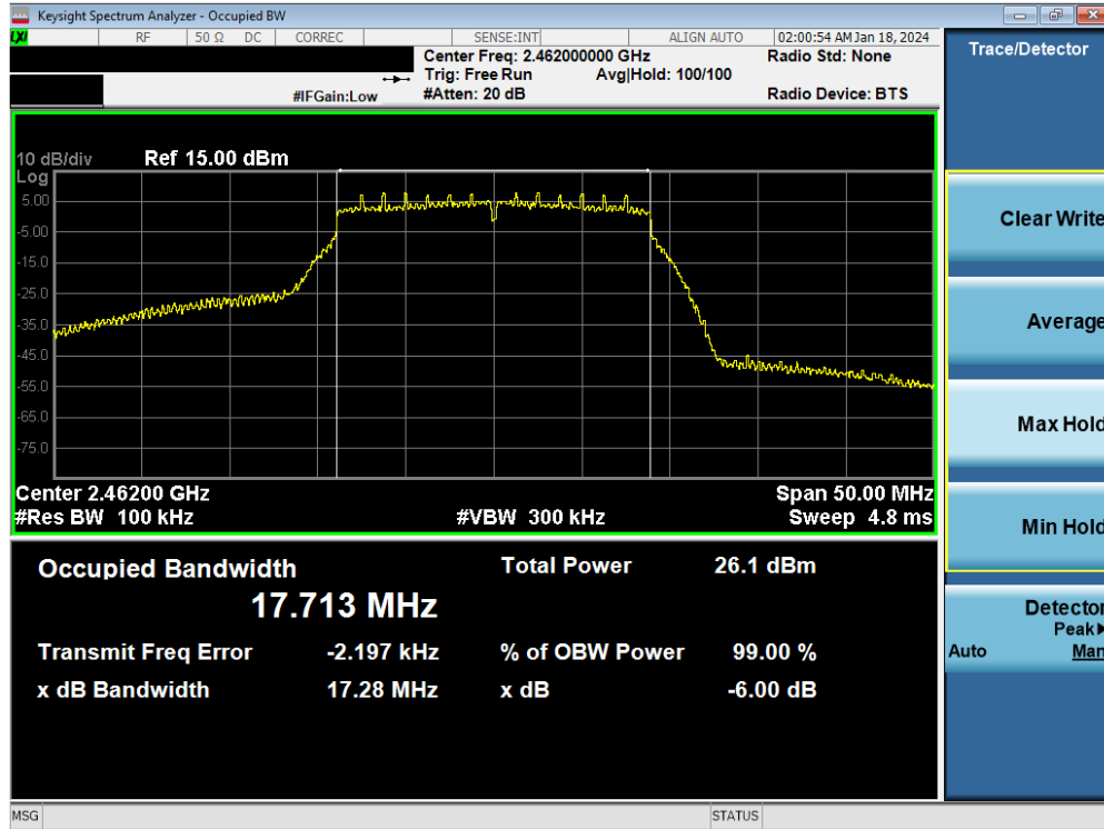
Plot 7-6. 6 dB BW and 99% OBW Plot Antenna WF8 (802.11n (2.4GHz) – Ch. 11) – MCS2
