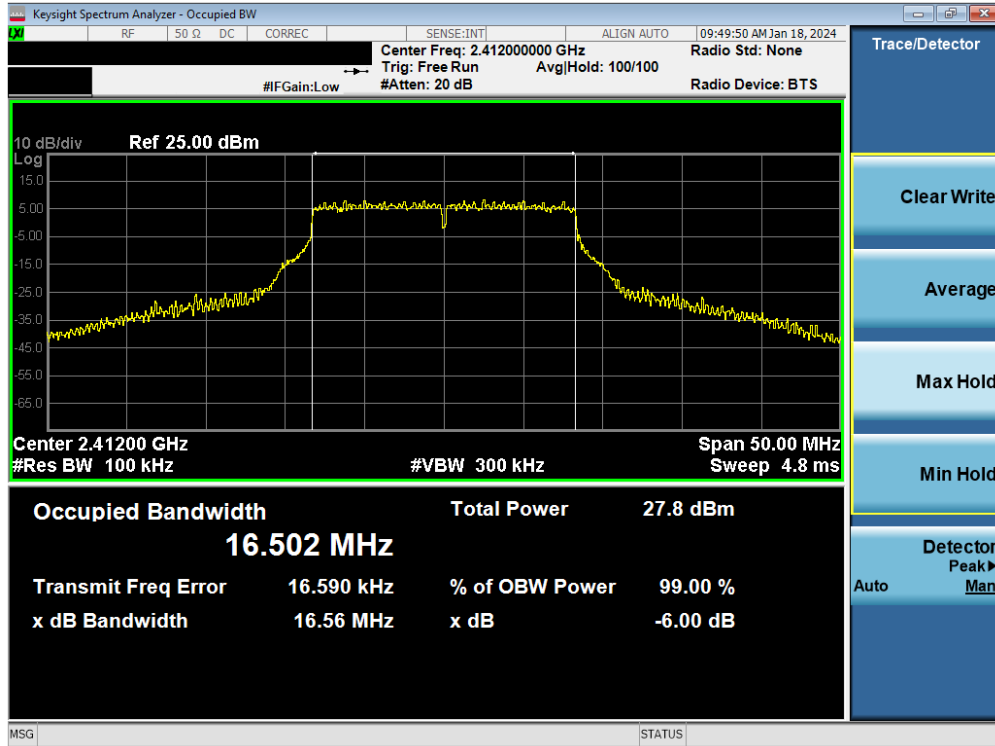
Plot 7-82. 6 dB BW and 99% OBW Plot Antenna WF9 (802.11g – Ch. 1) – 54Mbps
