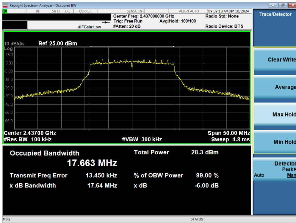
Plot 7-65. 6 dB BW and 99% OBW Plot Antenna WF9 (802.11n (2.4GHz) – Ch. 6) – MCS2
