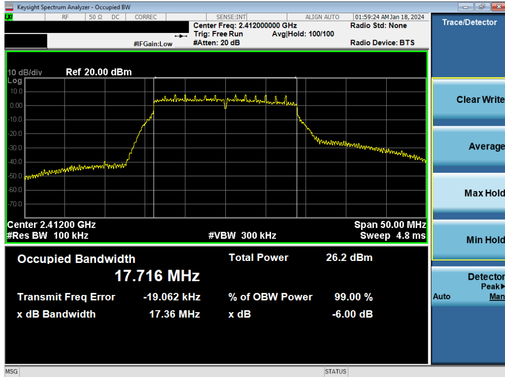
Plot 7-4. 6 dB BW and 99% OBW Plot Antenna WF8 (802.11n (2.4GHz) – Ch. 1) – MCS2
