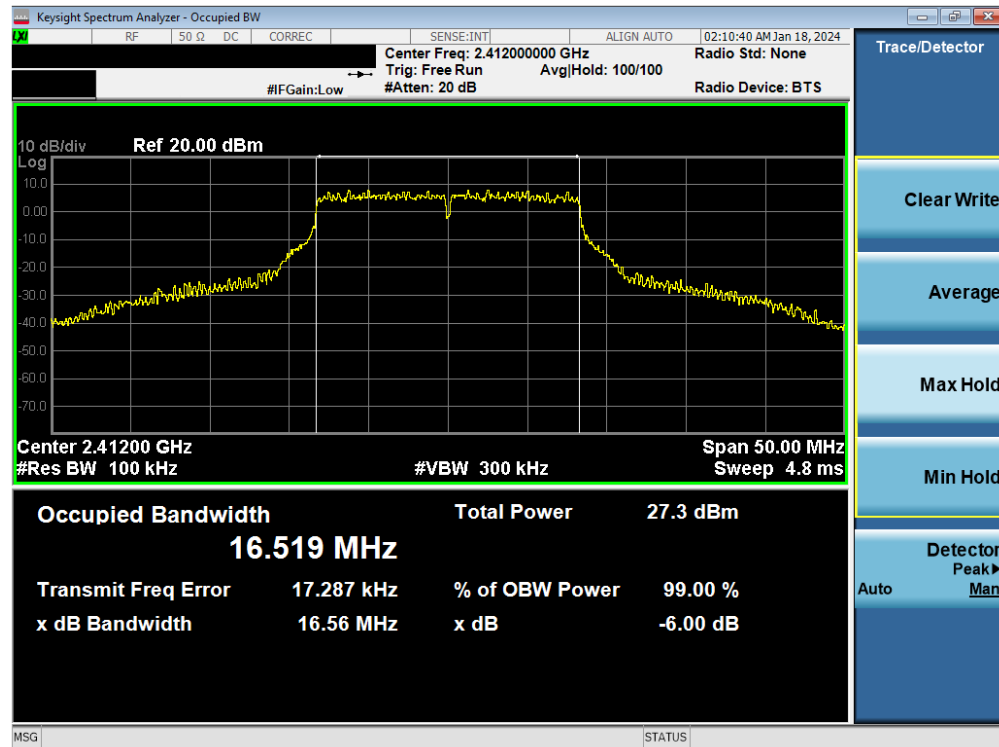
Plot 7-22. 6 dB BW and 99% OBW Plot Antenna WF8 (802.11g – Ch. 1) – 54Mbps
