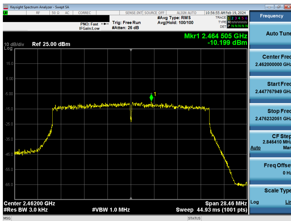
Plot 7-99. Power Spectral Density Plot Antenna WF8 (802.11ax (SU - 2.4GHz) – Ch. 11) – MCS2
