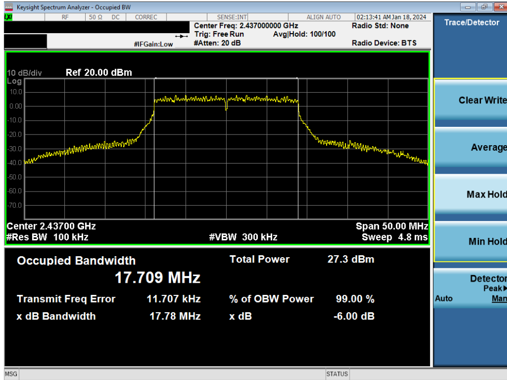
Plot 7-26. 6 dB BW and 99% OBW Plot Antenna WF8 (802.11n (2.4GHz) – Ch. 6) – MCS7
