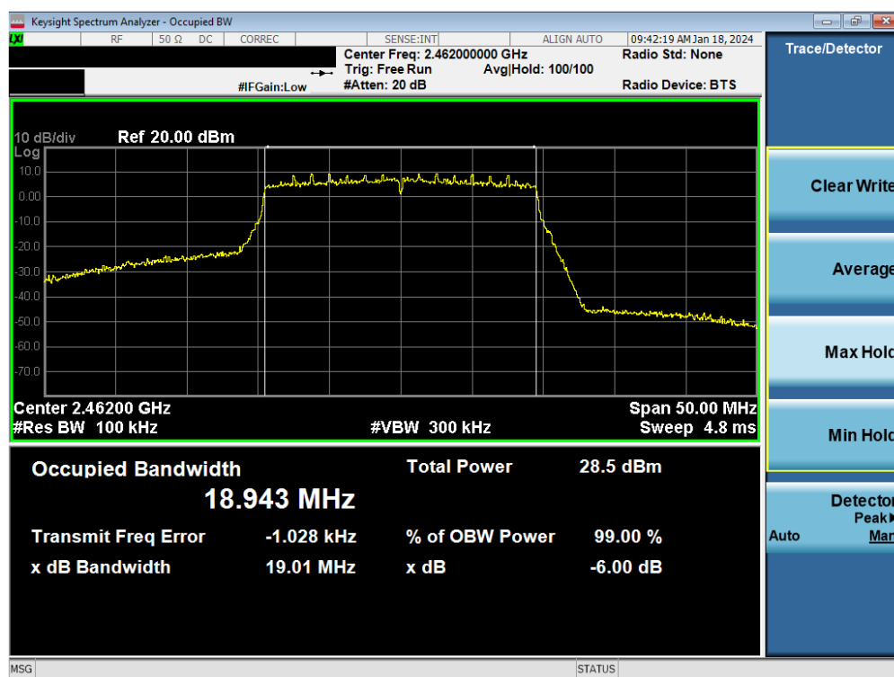
Plot 7-69. 6 dB BW and 99% OBW Plot Antenna WF9 (802.11ax (SU - 2.4GHz) – Ch. 11) – MCS2
