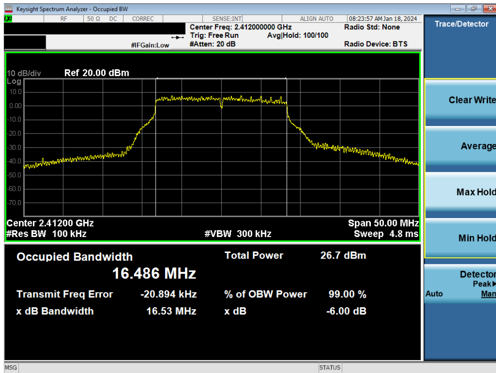
Plot 7-40. 6 dB BW and 99% OBW Plot Antenna WF7 (802.11g – Ch. 1) – 24Mbps
