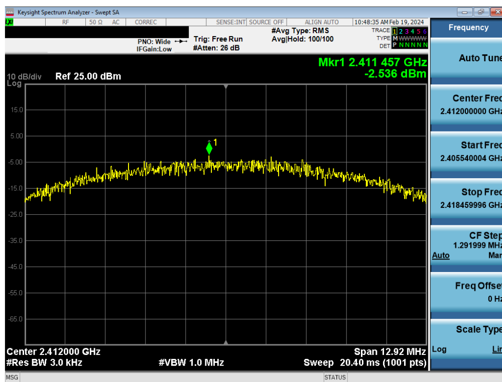
Plot 7-109. Power Spectral Density Plot Antenna WF8 (802.11b – Ch. 1) – 11Mbps
