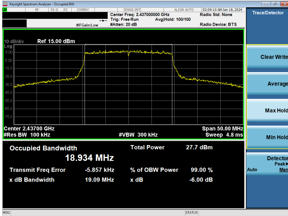
Plot 7-17. 6 dB BW and 99% OBW Plot Antenna WF8 (802.11ax (SU - 2.4GHz) – Ch. 6) – MCS4
