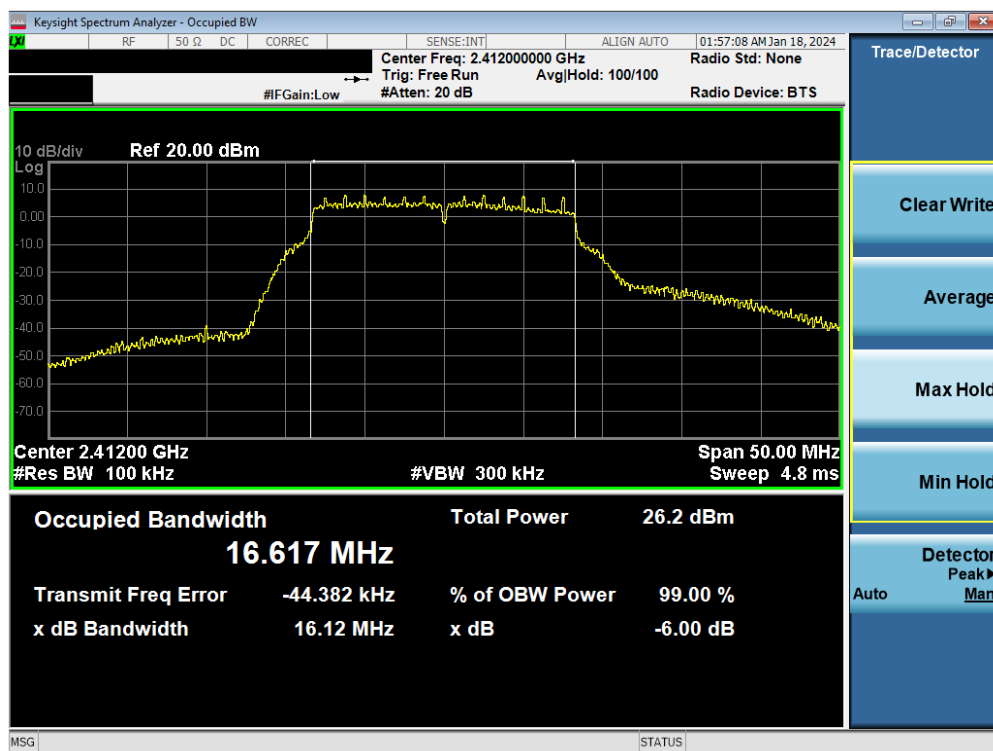
Plot 7-1. 6 dB BW and 99% OBW Plot Antenna WF8 (802.11g – Ch. 1) – 12Mbps
