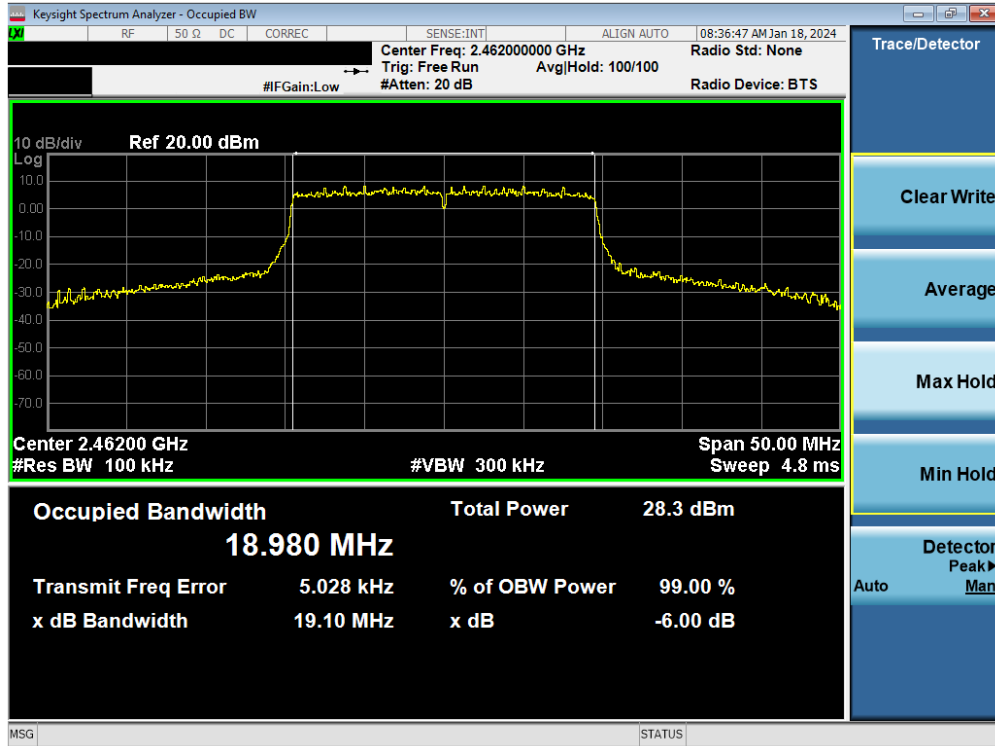
Plot 7-60. 6 dB BW and 99% OBW Plot Antenna WF7 (802.11ax (SU - 2.4GHz) – Ch. 11) – MCS9
