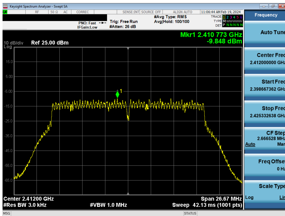
Plot 7-115. Power Spectral Density Plot Antenna WF8 (802.11n (2.4GHz) – Ch. 1) – MCS7
