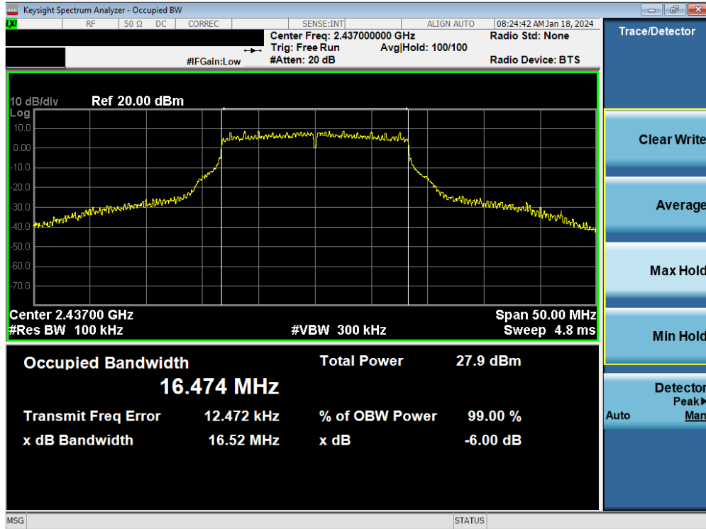
Plot 7-41. 6 dB BW and 99% OBW Plot Antenna WF7 (802.11g – Ch. 6) – 24Mbps
