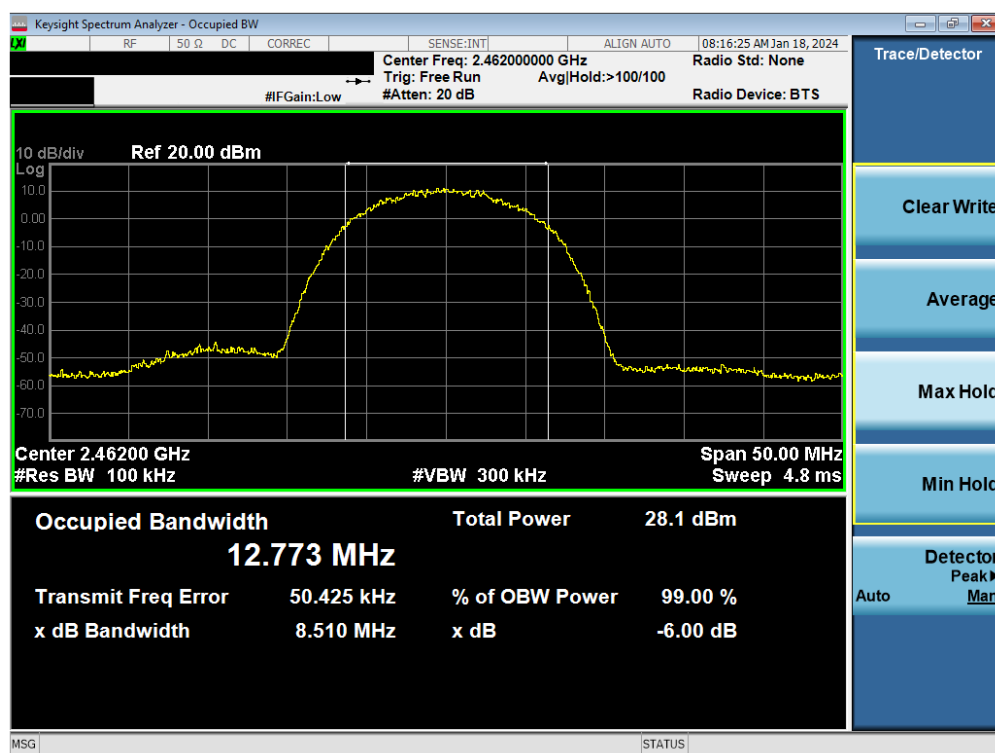
Plot 7-51. 6 dB BW and 99% OBW Plot Antenna WF7 (802.11b – Ch. 11) – 11Mbps
