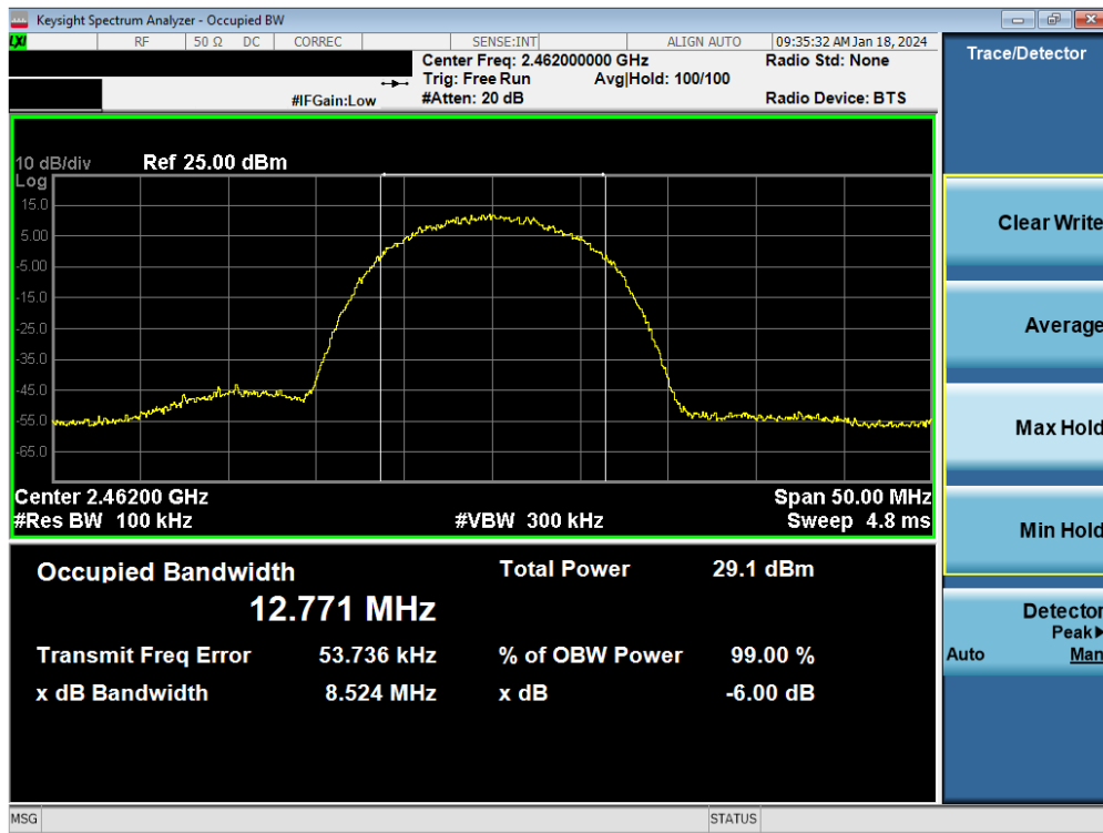
Plot 7-81. 6 dB BW and 99% OBW Plot Antenna WF9 (802.11b – Ch. 11) – 11Mbps
