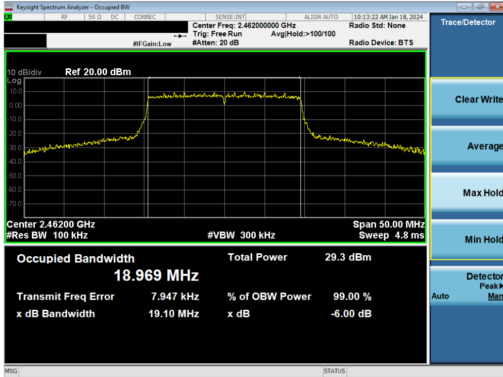
Plot 7-90. 6 dB BW and 99% OBW Plot Antenna WF9 (802.11ax (SU - 2.4GHz) – Ch. 11) – MCS9
