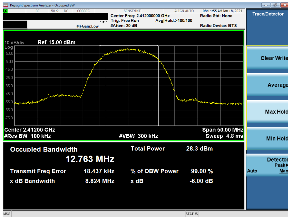
Plot 7-49. 6 dB BW and 99% OBW Plot Antenna WF7 (802.11b – Ch. 1) – 11Mbps
