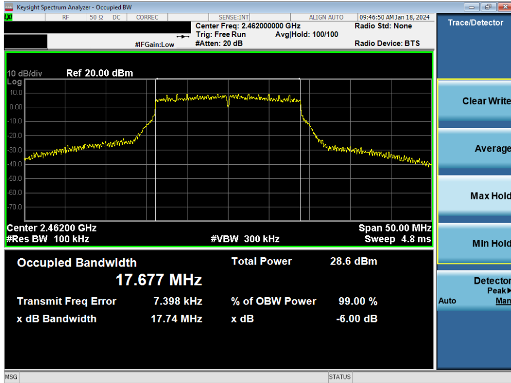
Plot 7-75. 6 dB BW and 99% OBW Plot Antenna WF9 (802.11n (2.4GHz) – Ch. 11) – MCS4
