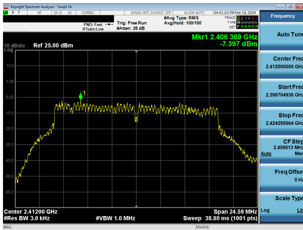
Plot 7-121. Power Spectral Density Plot Antenna WF7 (802.11g – Ch. 1) – 6Mbps
