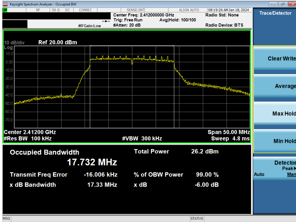
Plot 7-34. 6 dB BW and 99% OBW Plot Antenna WF7 (802.11n (2.4GHz) – Ch. 1) – MCS2
