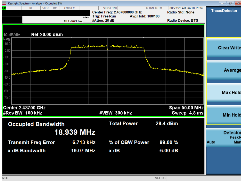
Plot 7-38. 6 dB BW and 99% OBW Plot Antenna WF7 (802.11ax (SU - 2.4GHz) – Ch. 6) – MCS2
