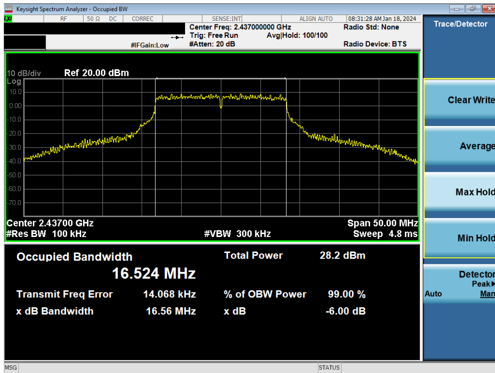
Plot 7-53. 6 dB BW and 99% OBW Plot Antenna WF7 (802.11g – Ch. 6) – 54Mbps
