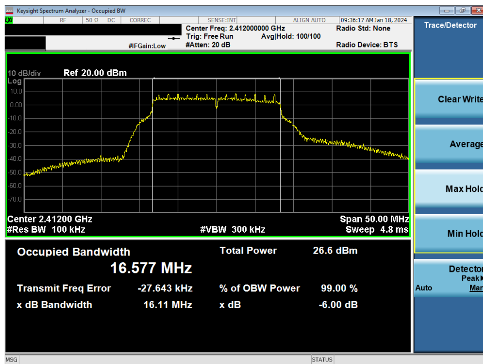
Plot 7-61. 6 dB BW and 99% OBW Plot Antenna WF9 (802.11g – Ch. 1) – 12Mbps
