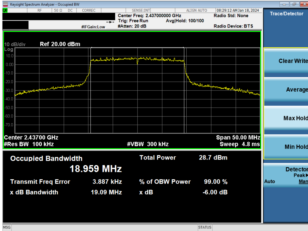
Plot 7-47. 6 dB BW and 99% OBW Plot Antenna WF7 (802.11ax (SU - 2.4GHz) – Ch. 6) – MCS4
