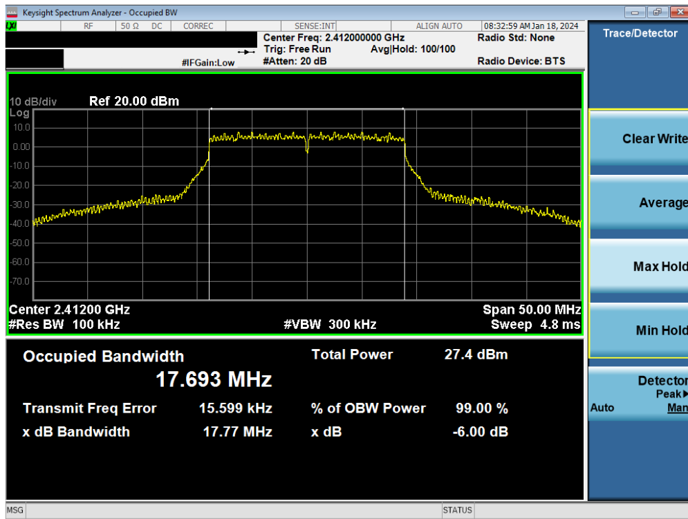
Plot 7-55. 6 dB BW and 99% OBW Plot Antenna WF7 (802.11n (2.4GHz) – Ch. 1) – MCS7
