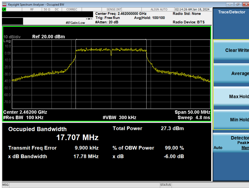
Plot 7-27. 6 dB BW and 99% OBW Plot Antenna WF8 (802.11n (2.4GHz) – Ch. 11) – MCS7
