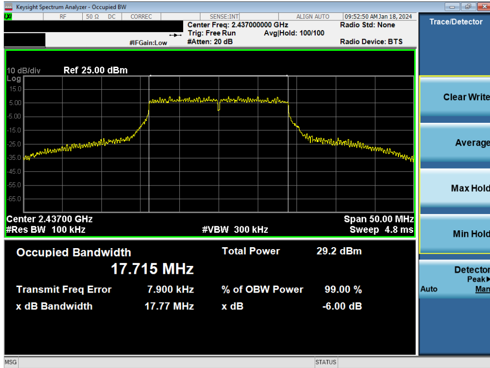
Plot 7-86. 6 dB BW and 99% OBW Plot Antenna WF9 (802.11n (2.4GHz) – Ch. 6) – MCS7
