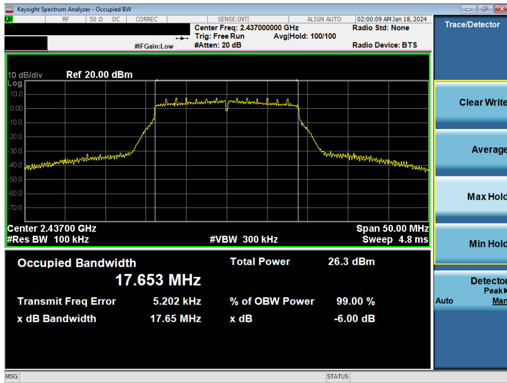
Plot 7-5. 6 dB BW and 99% OBW Plot Antenna WF8 (802.11n (2.4GHz) – Ch. 6) – MCS2
