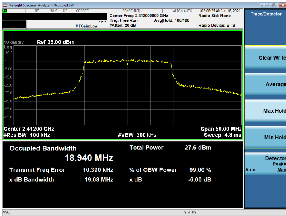
Plot 7-16. 6 dB BW and 99% OBW Plot Antenna WF8 (802.11ax (SU - 2.4GHz) – Ch. 1) – MCS4
