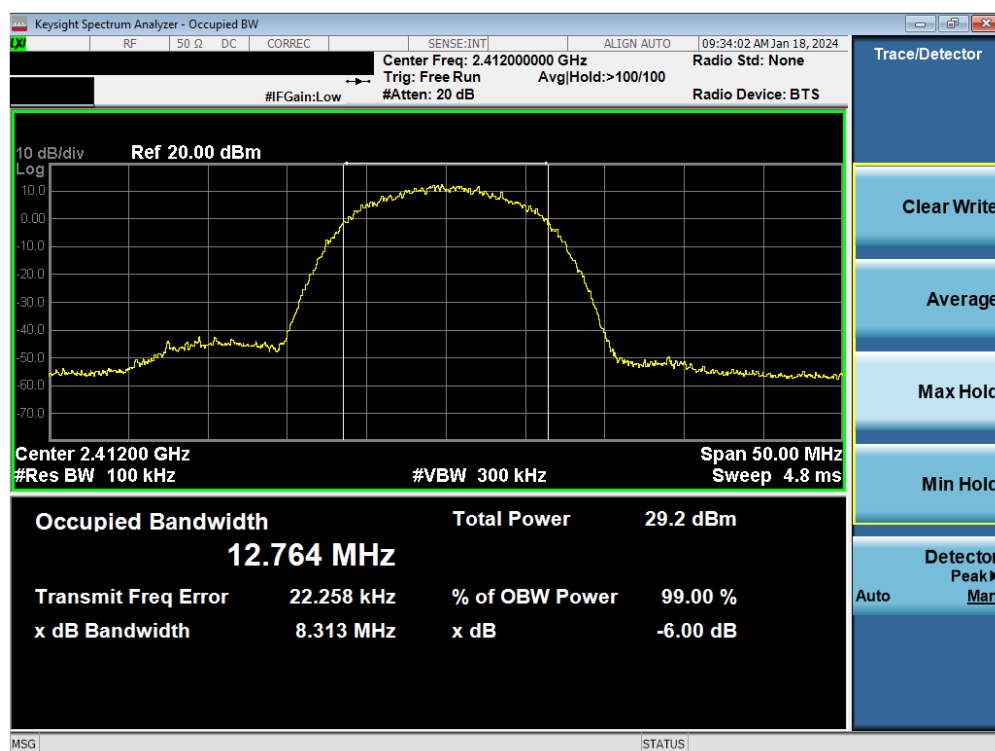
Plot 7-79. 6 dB BW and 99% OBW Plot Antenna WF9 (802.11b – Ch. 1) – 11Mbps
