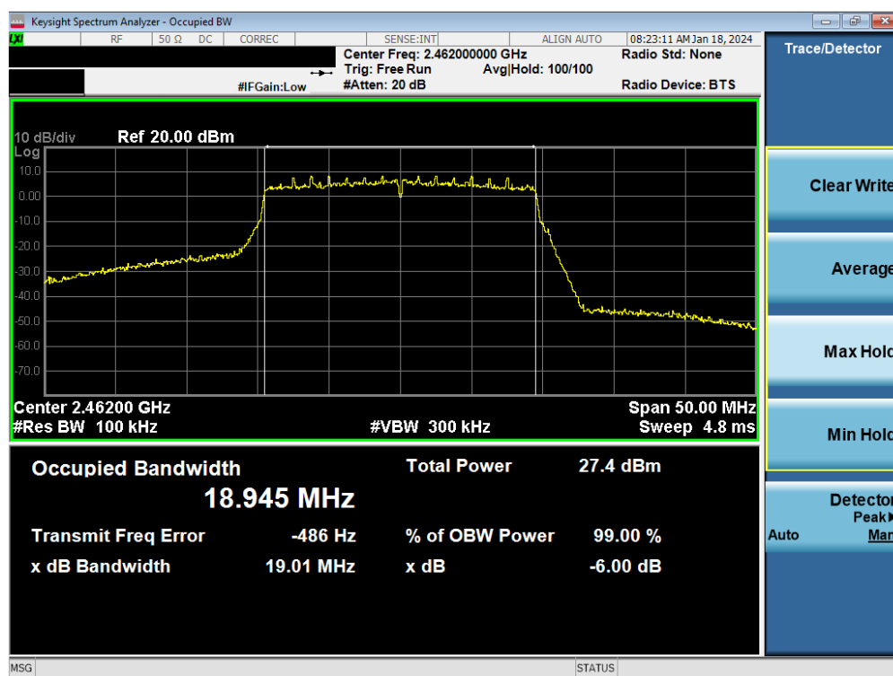
Plot 7-39. 6 dB BW and 99% OBW Plot Antenna WF7 (802.11ax (SU - 2.4GHz) – Ch. 11) – MCS2
