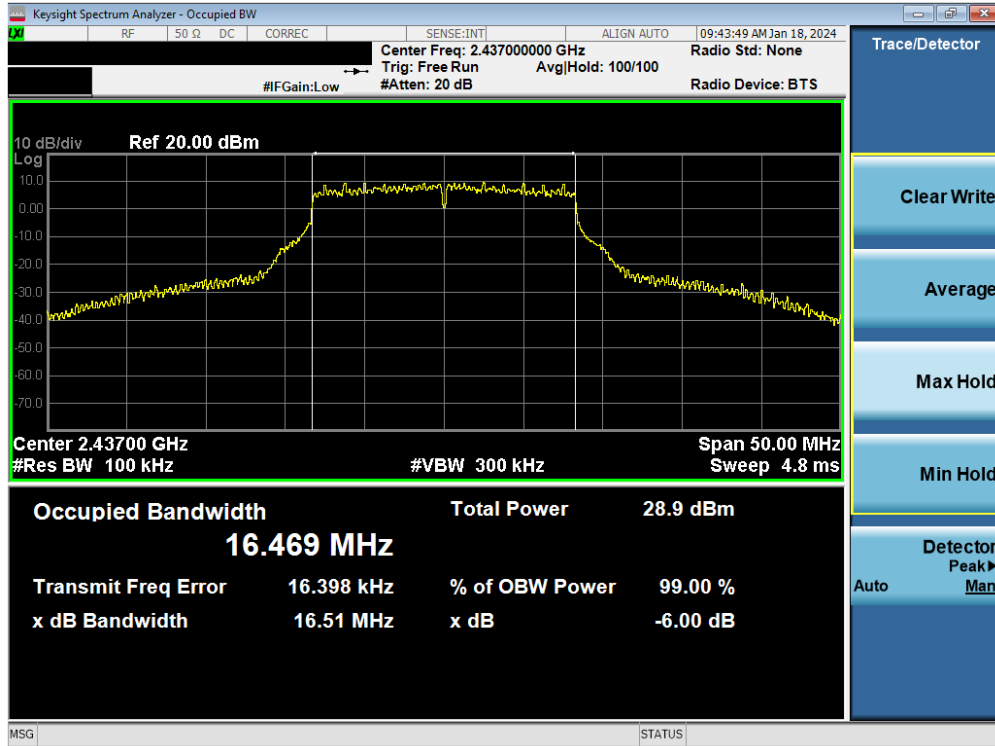
Plot 7-71. 6 dB BW and 99% OBW Plot Antenna WF9 (802.11g – Ch. 6) – 24Mbps
