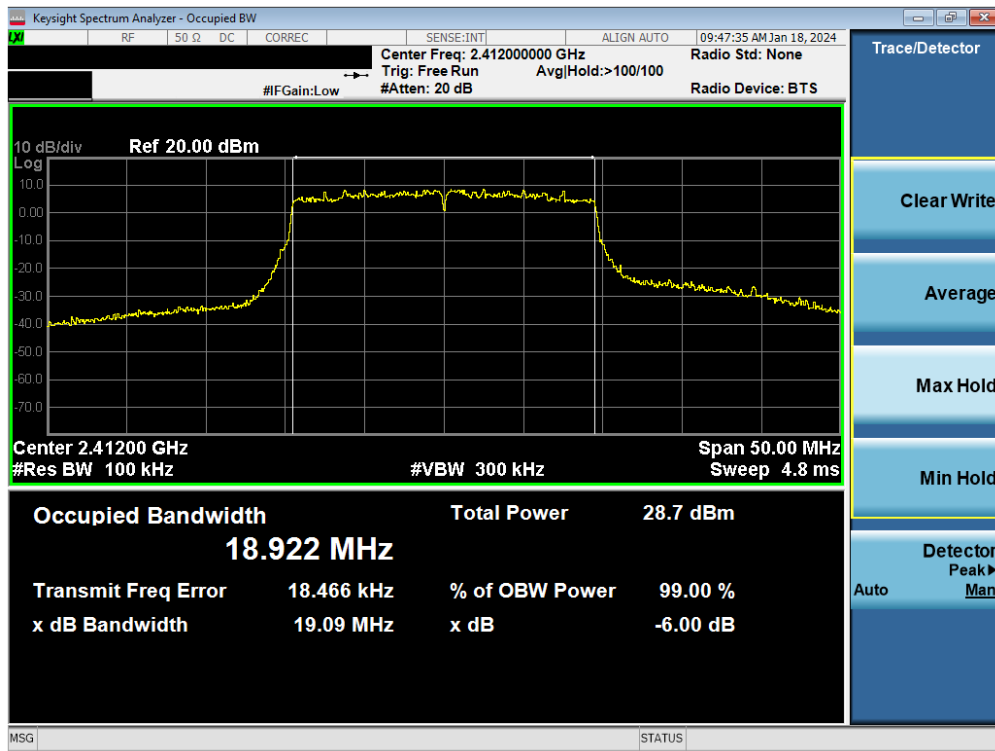
Plot 7-76. 6 dB BW and 99% OBW Plot Antenna WF9 (802.11ax (SU - 2.4GHz) – Ch. 1) – MCS4
