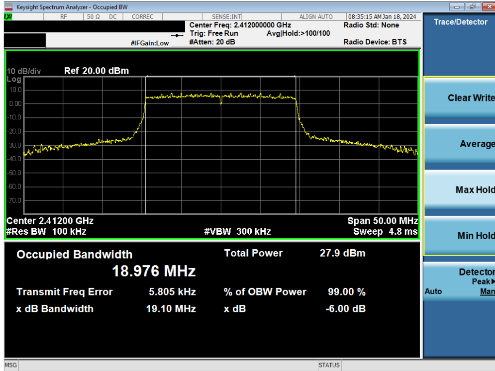
Plot 7-58. 6 dB BW and 99% OBW Plot Antenna WF7 (802.11ax (SU - 2.4GHz) – Ch. 1) – MCS9
