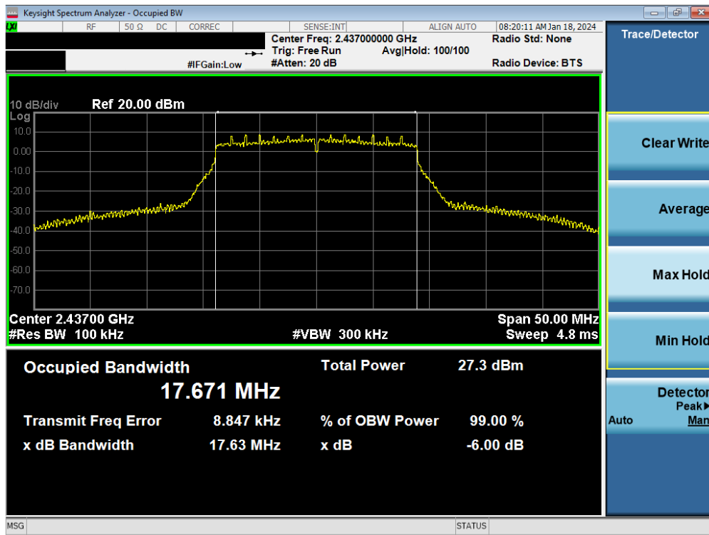
Plot 7-35. 6 dB BW and 99% OBW Plot Antenna WF7 (802.11n (2.4GHz) – Ch. 6) – MCS2
