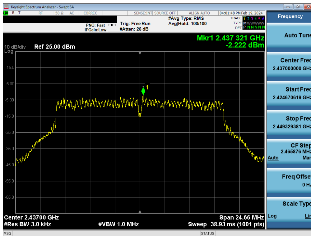
Plot 7-122. Power Spectral Density Plot Antenna WF7 (802.11g – Ch. 6) – 6Mbps
