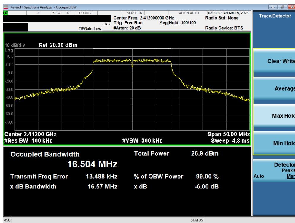
Plot 7-52. 6 dB BW and 99% OBW Plot Antenna WF7 (802.11g – Ch. 1) – 54Mbps
