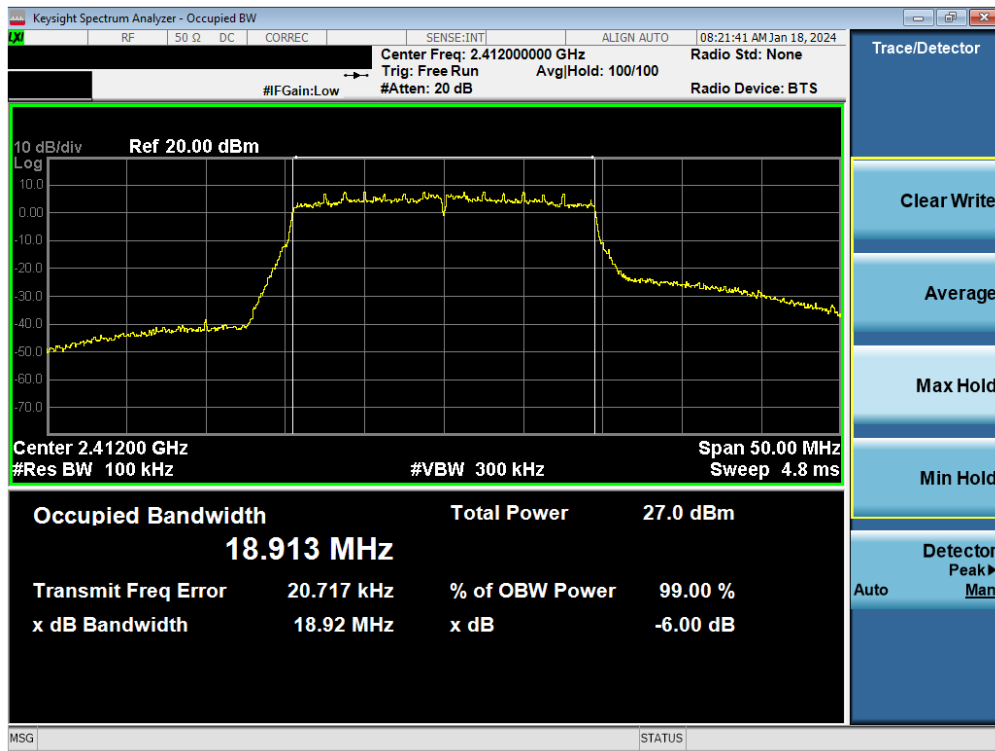
Plot 7-37. 6 dB BW and 99% OBW Plot Antenna WF7 (802.11ax (SU - 2.4GHz) – Ch. 1) – MCS2
