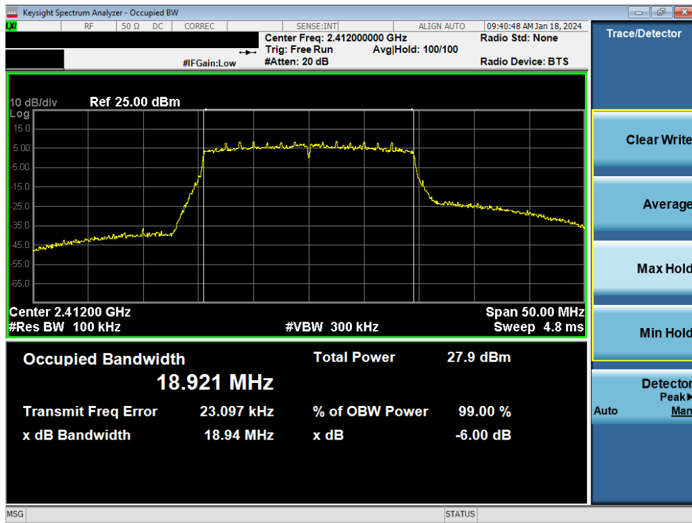
Plot 7-67. 6 dB BW and 99% OBW Plot Antenna WF9 (802.11ax (SU - 2.4GHz) – Ch. 1) – MCS2
