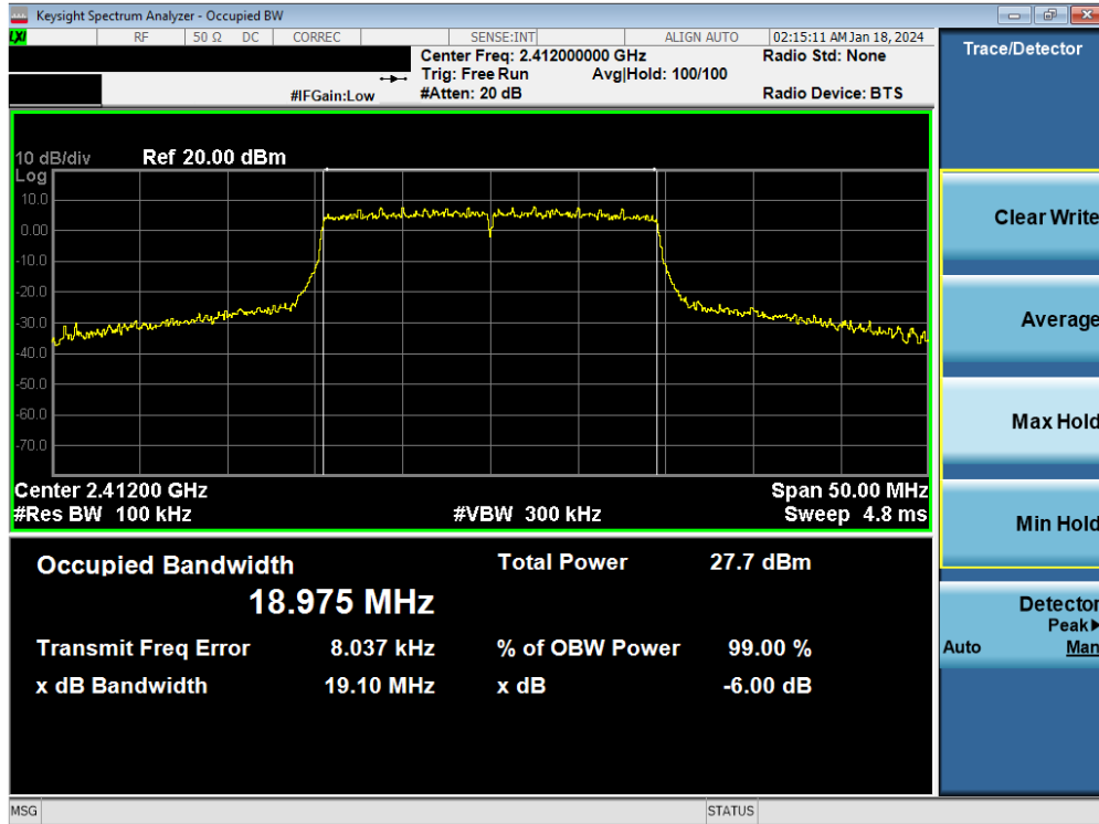
Plot 7-28. 6 dB BW and 99% OBW Plot Antenna WF8 (802.11ax (SU - 2.4GHz) – Ch. 1) – MCS9
