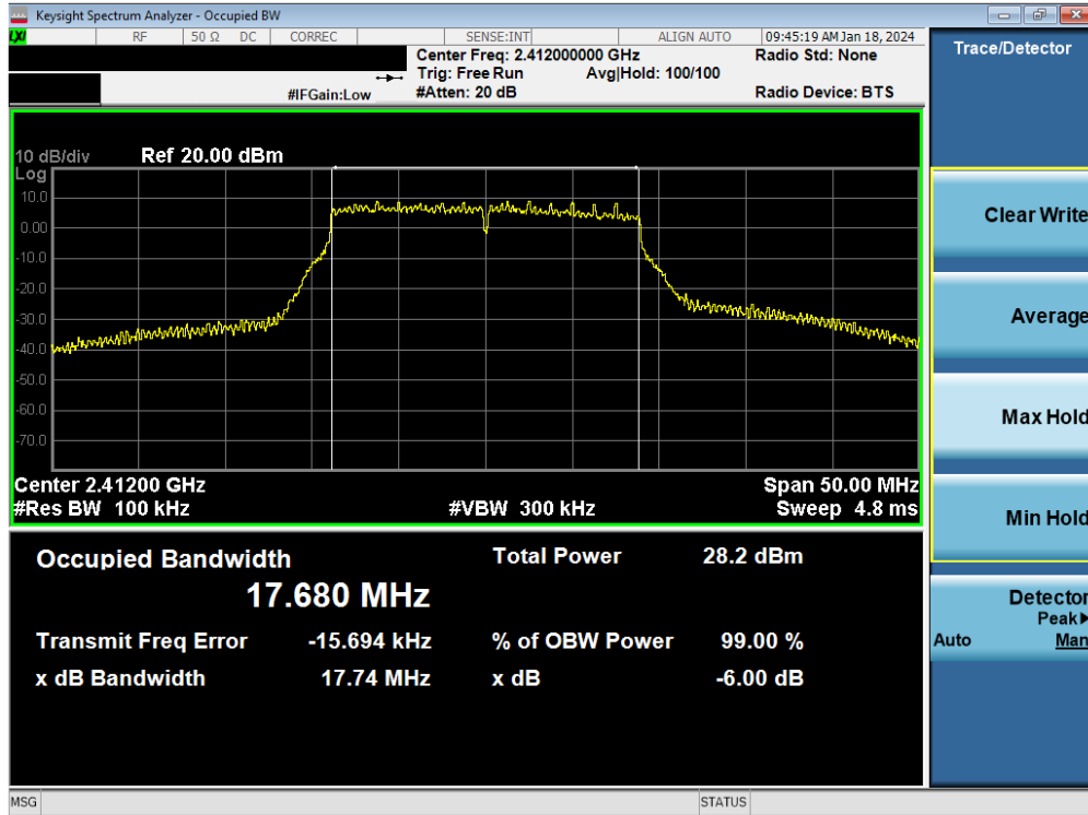
Plot 7-73. 6 dB BW and 99% OBW Plot Antenna WF9 (802.11n (2.4GHz) – Ch. 1) – MCS4
