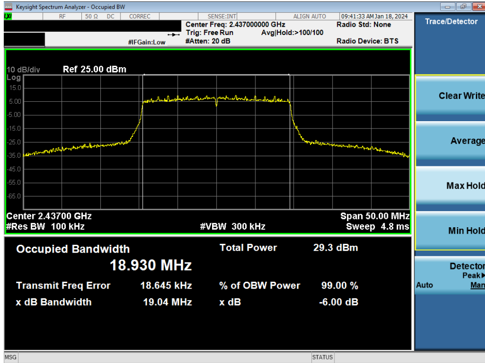
Plot 7-68. 6 dB BW and 99% OBW Plot Antenna WF9 (802.11ax (SU - 2.4GHz) – Ch. 6) – MCS2
