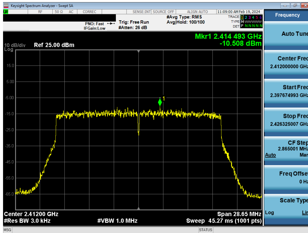
Plot 7-118. Power Spectral Density Plot Antenna WF8 (802.11ax (SU - 2.4GHz) – Ch. 1) – MCS9
