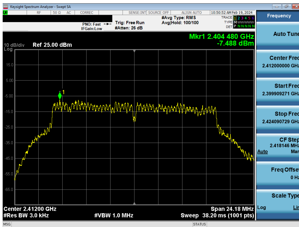
Plot 7-91. Power Spectral Density Plot Antenna WF8 (802.11g – Ch. 1) – 12Mbps
