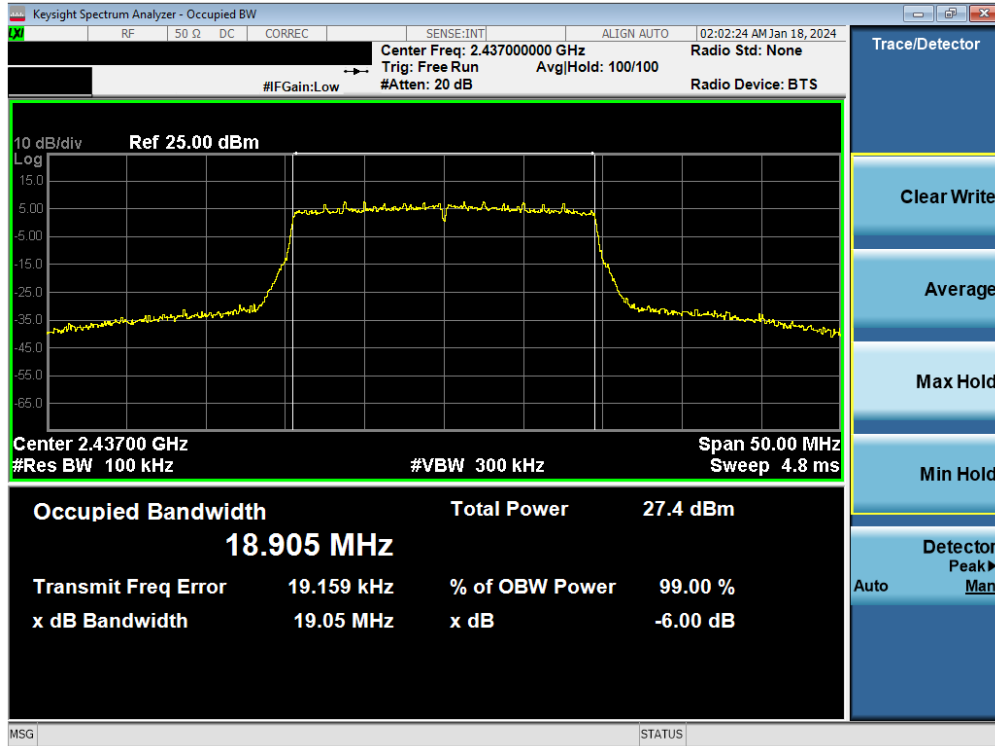
Plot 7-8. 6 dB BW and 99% OBW Plot Antenna WF8 (802.11ax (SU - 2.4GHz) – Ch. 6) – MCS2
