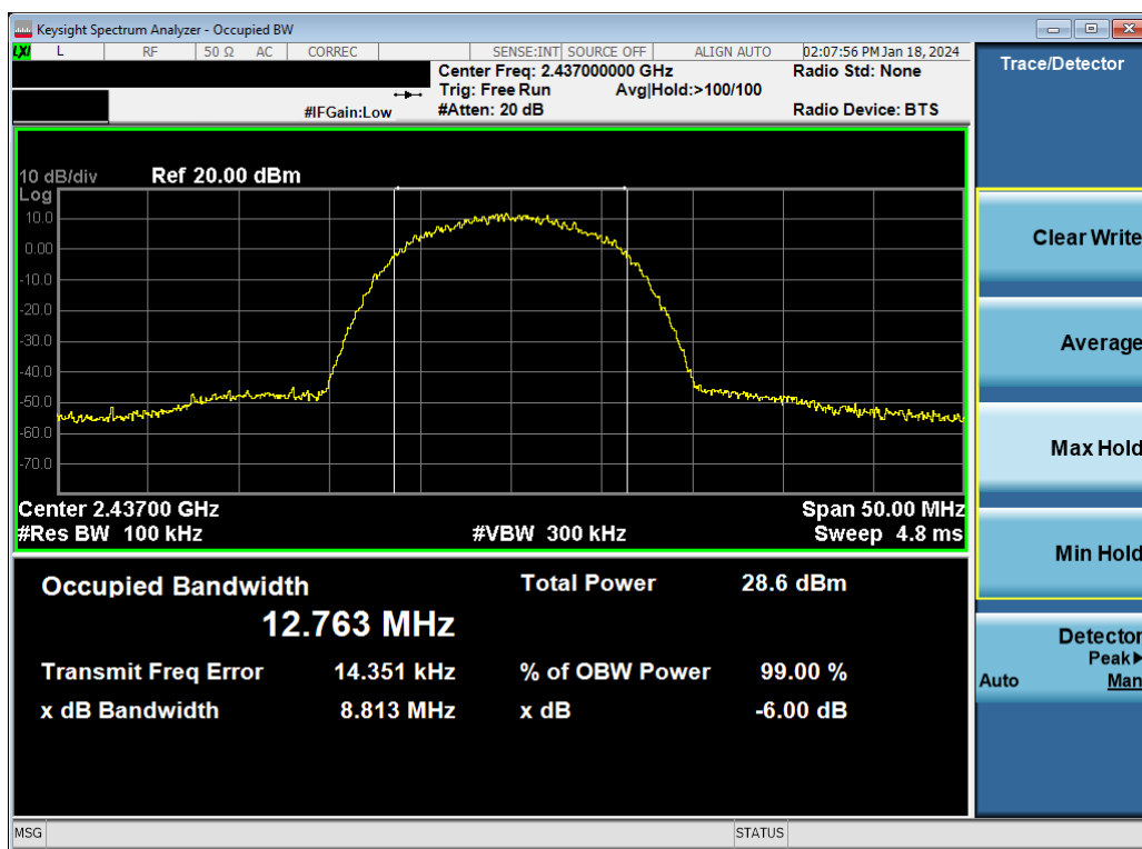
Plot 7-20. 6 dB BW and 99% OBW Plot Antenna WF8 (802.11b – Ch. 6) – 11Mbps
