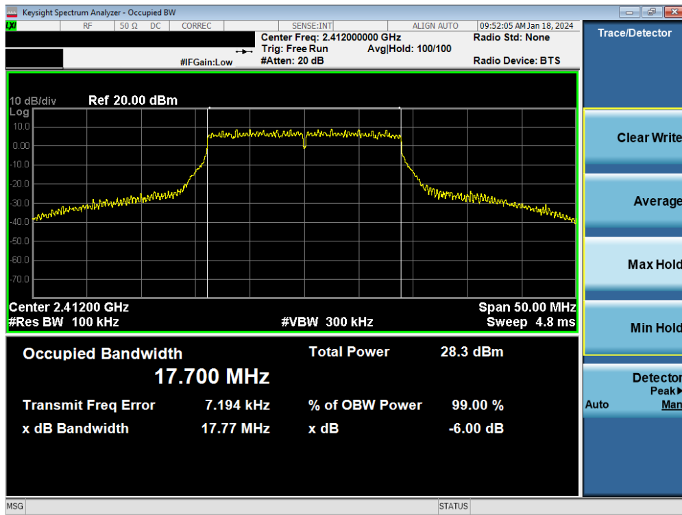
Plot 7-85. 6 dB BW and 99% OBW Plot Antenna WF9 (802.11n (2.4GHz) – Ch. 1) – MCS7
