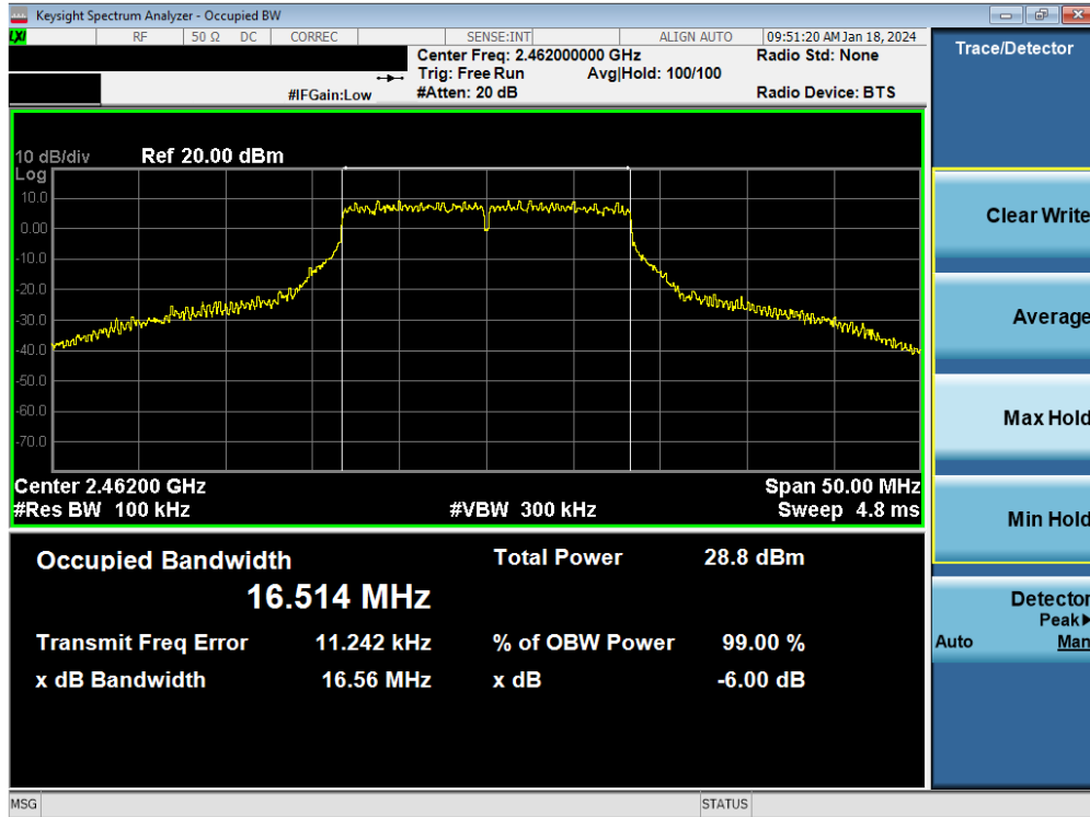
Plot 7-84. 6 dB BW and 99% OBW Plot Antenna WF9 (802.11g – Ch. 11) – 54Mbps
