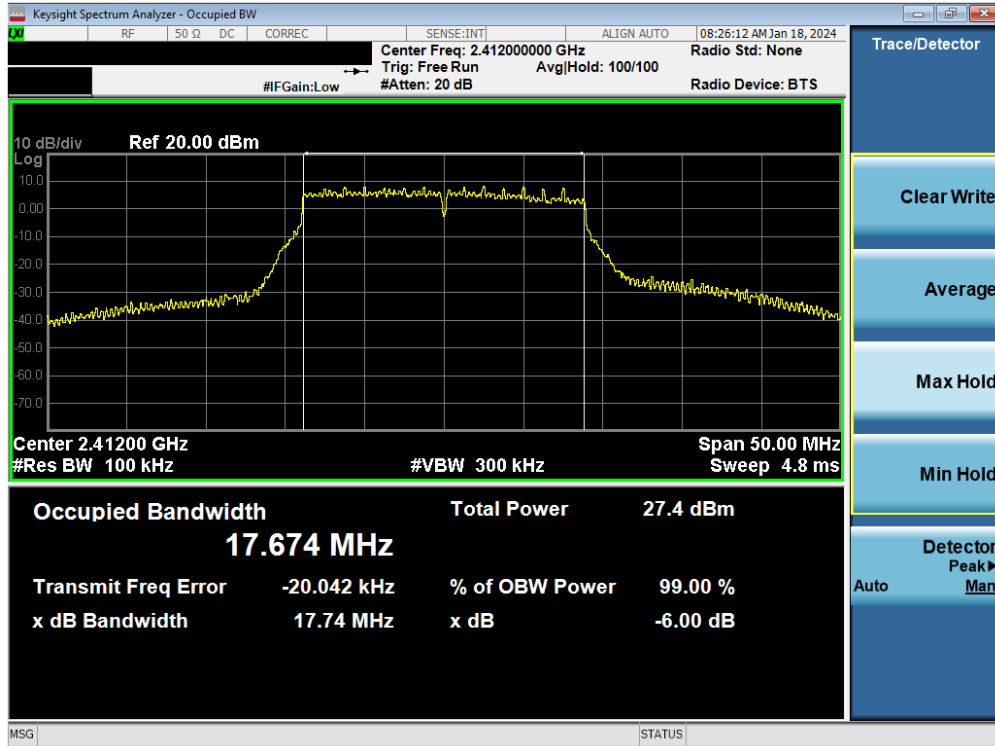
Plot 7-43. 6 dB BW and 99% OBW Plot Antenna WF7 (802.11n (2.4GHz) – Ch. 1) – MCS4
