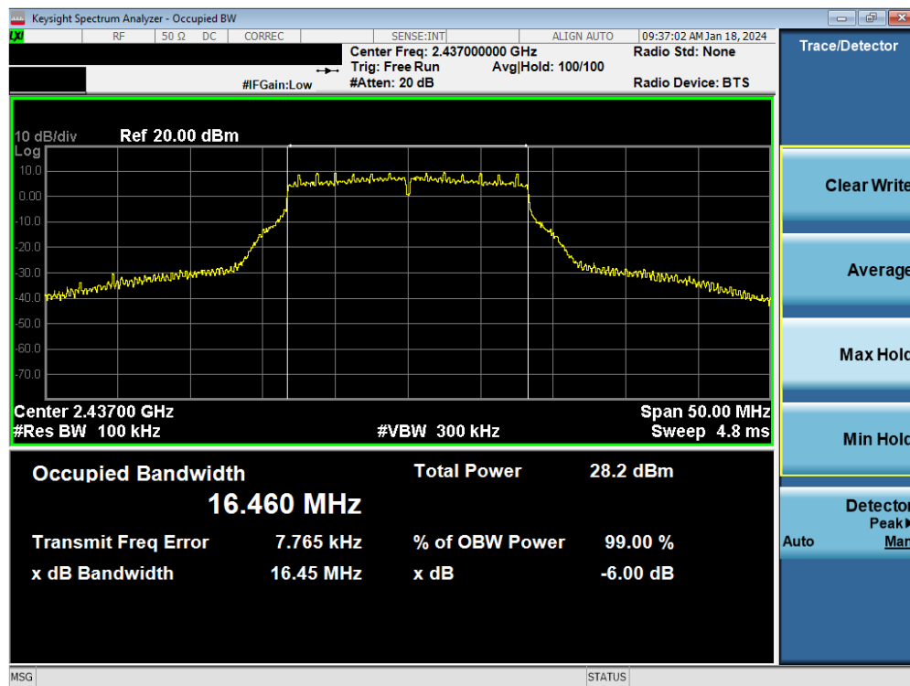
Plot 7-62. 6 dB BW and 99% OBW Plot Antenna WF9 (802.11g – Ch. 6) – 12Mbps
