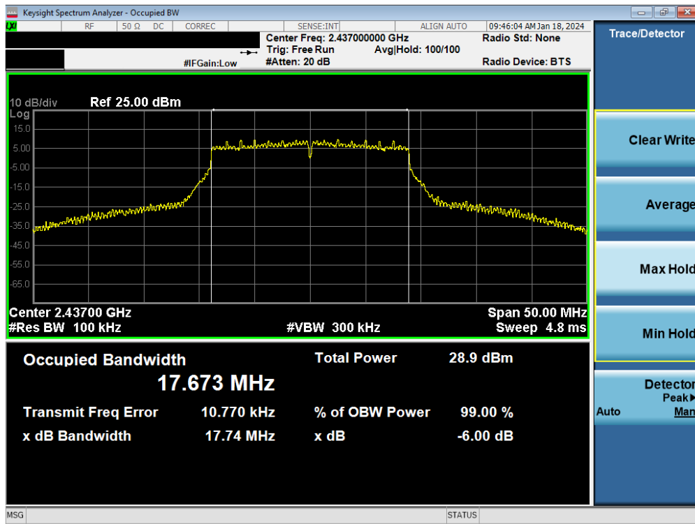
Plot 7-74. 6 dB BW and 99% OBW Plot Antenna WF9 (802.11n (2.4GHz) – Ch. 6) – MCS4
