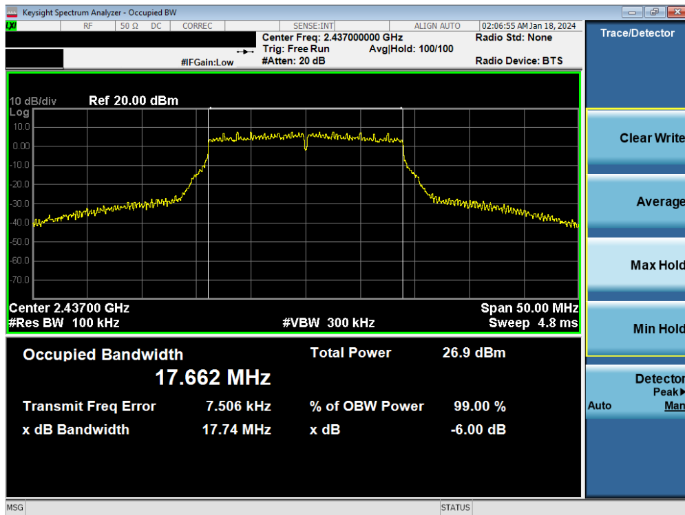
Plot 7-14. 6 dB BW and 99% OBW Plot Antenna WF8 (802.11n (2.4GHz) – Ch. 6) – MCS4
