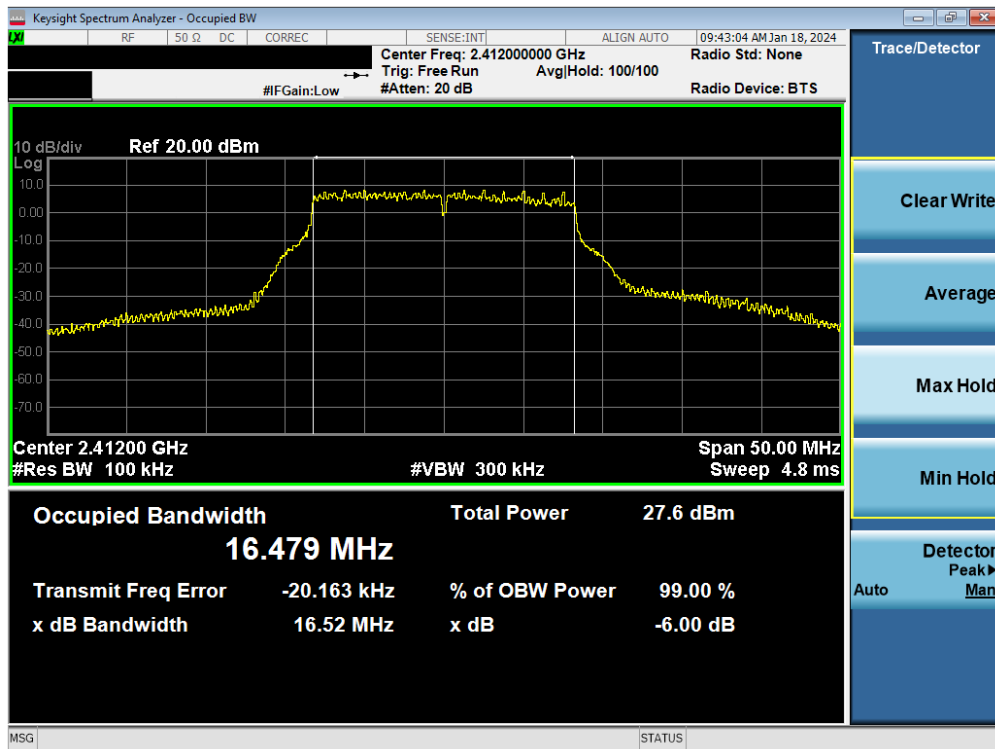
Plot 7-70. 6 dB BW and 99% OBW Plot Antenna WF9 (802.11g – Ch. 1) – 24Mbps
