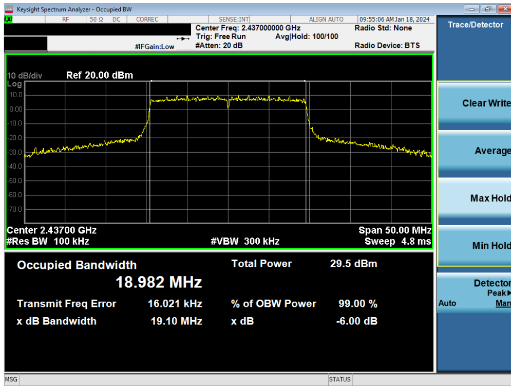
Plot 7-89. 6 dB BW and 99% OBW Plot Antenna WF9 (802.11ax (SU - 2.4GHz) – Ch. 6) – MCS9
