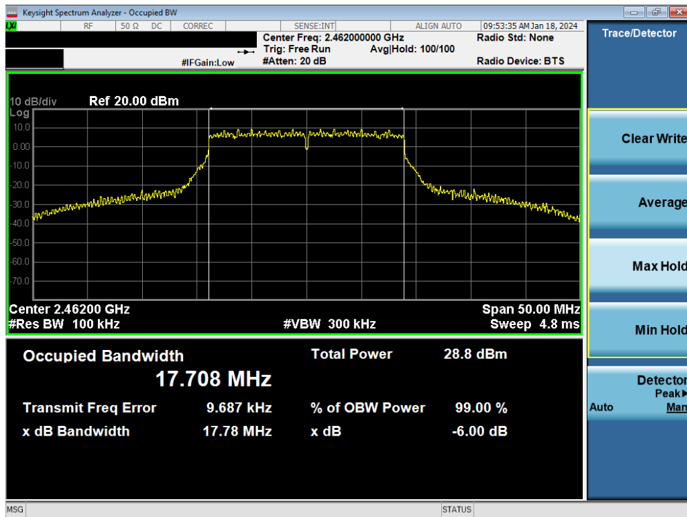
Plot 7-87. 6 dB BW and 99% OBW Plot Antenna WF9 (802.11n (2.4GHz) – Ch. 11) – MCS7
