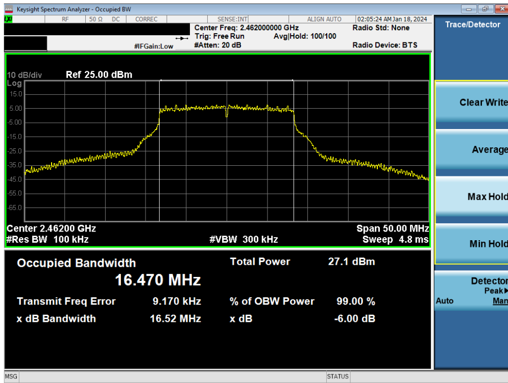
Plot 7-12. 6 dB BW and 99% OBW Plot Antenna WF8 (802.11g – Ch. 11) – 24Mbps
