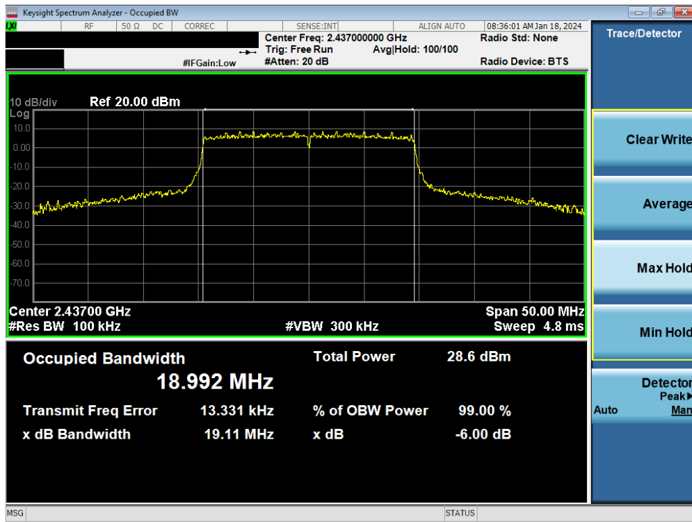
Plot 7-59. 6 dB BW and 99% OBW Plot Antenna WF7 (802.11ax (SU - 2.4GHz) – Ch. 6) – MCS9
