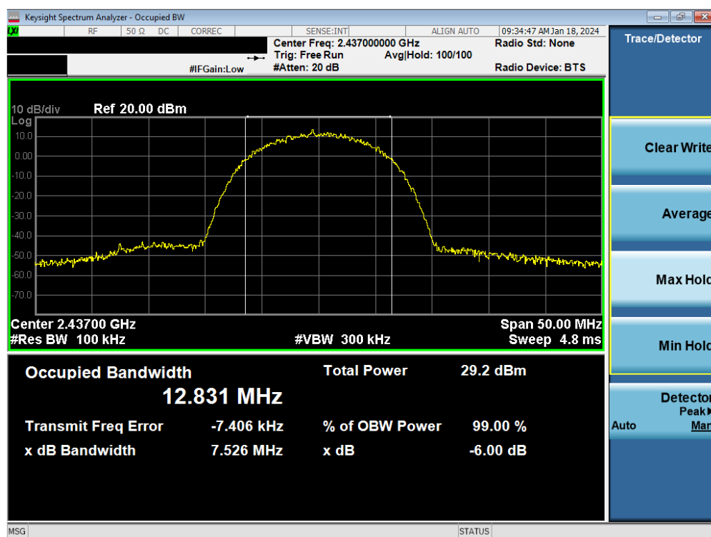
Plot 7-80. 6 dB BW and 99% OBW Plot Antenna WF9 (802.11b – Ch. 6) – 11Mbps
