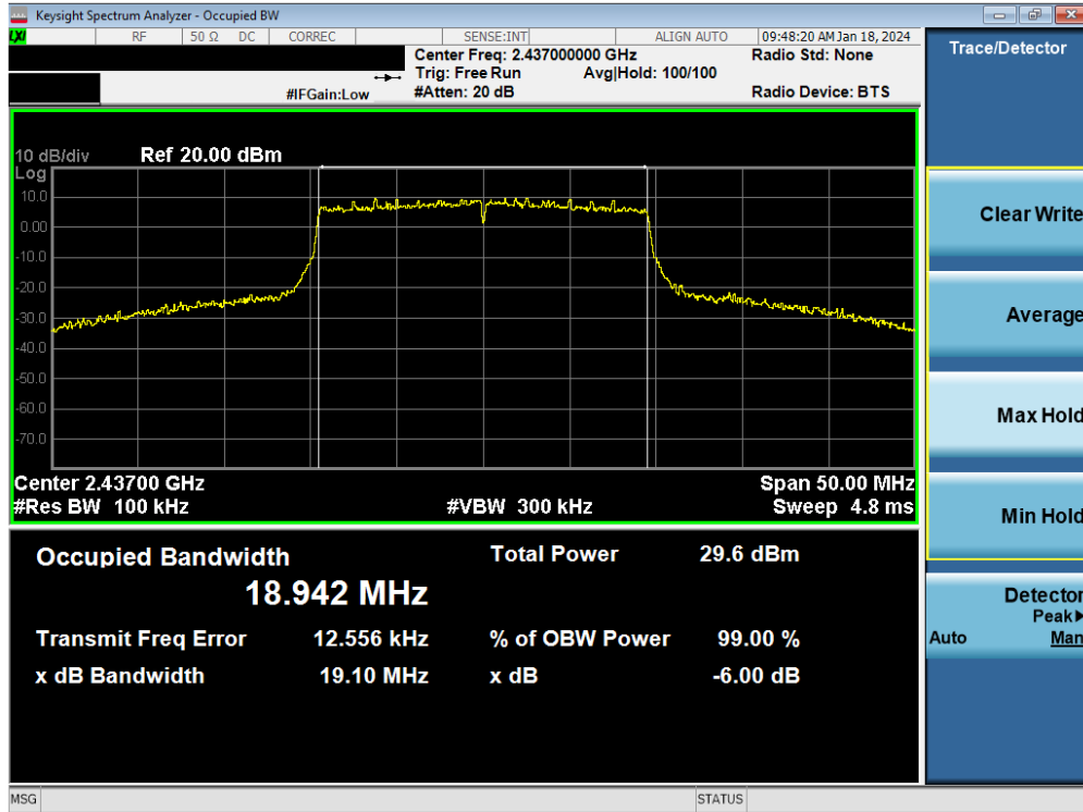
Plot 7-77. 6 dB BW and 99% OBW Plot Antenna WF9 (802.11ax (SU - 2.4GHz) – Ch. 6) – MCS4
