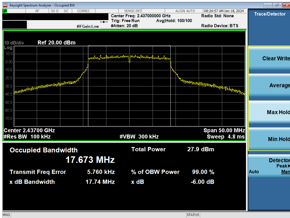
Plot 7-44. 6 dB BW and 99% OBW Plot Antenna WF7 (802.11n (2.4GHz) – Ch. 6) – MCS4
