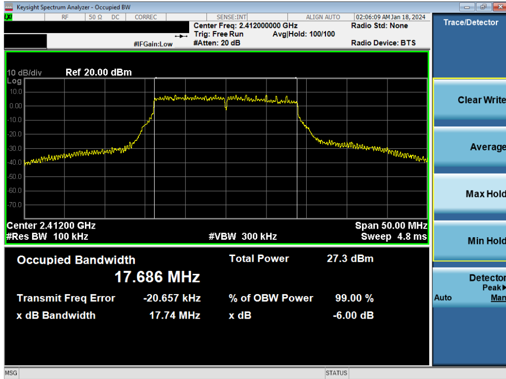
Plot 7-13. 6 dB BW and 99% OBW Plot Antenna WF8 (802.11n (2.4GHz) – Ch. 1) – MCS4
