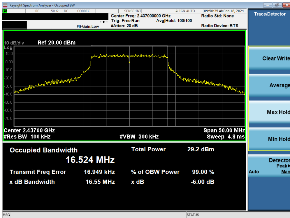
Plot 7-83. 6 dB BW and 99% OBW Plot Antenna WF9 (802.11g – Ch. 6) – 54Mbps
