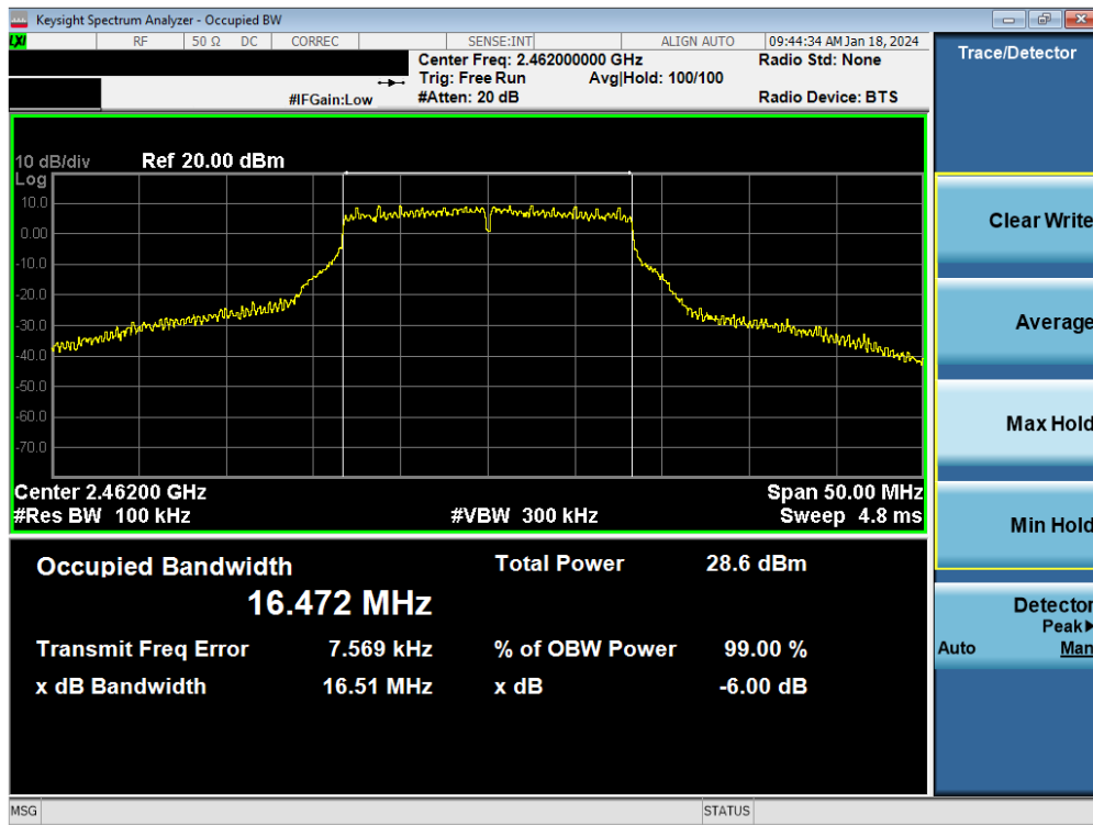
Plot 7-72. 6 dB BW and 99% OBW Plot Antenna WF9 (802.11g – Ch. 11) – 24Mbps
