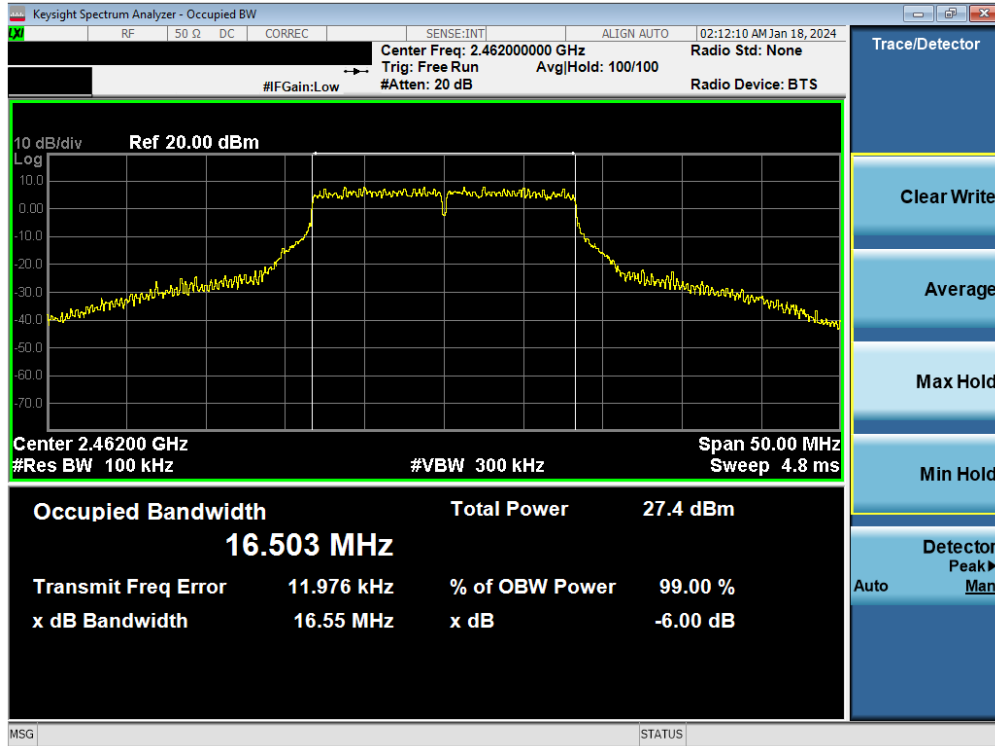
Plot 7-24. 6 dB BW and 99% OBW Plot Antenna WF8 (802.11g – Ch. 11) – 54Mbps
