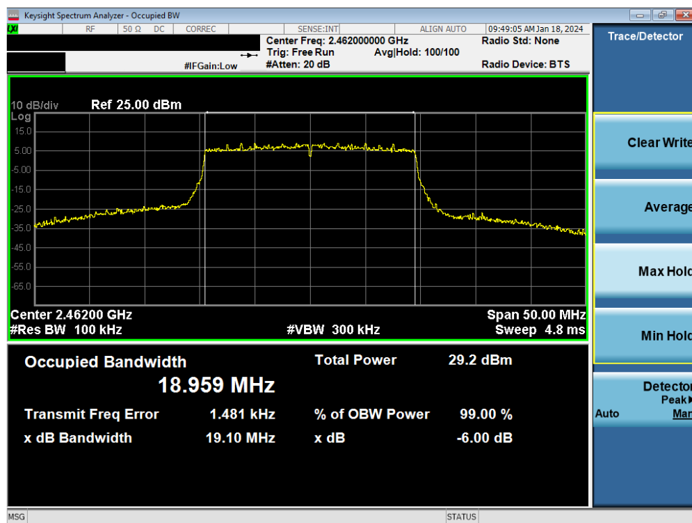
Plot 7-78. 6 dB BW and 99% OBW Plot Antenna WF9 (802.11ax (SU - 2.4GHz) – Ch. 11) – MCS4
