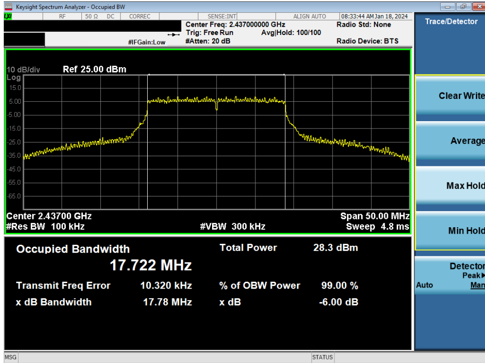
Plot 7-56. 6 dB BW and 99% OBW Plot Antenna WF7 (802.11n (2.4GHz) – Ch. 6) – MCS7
