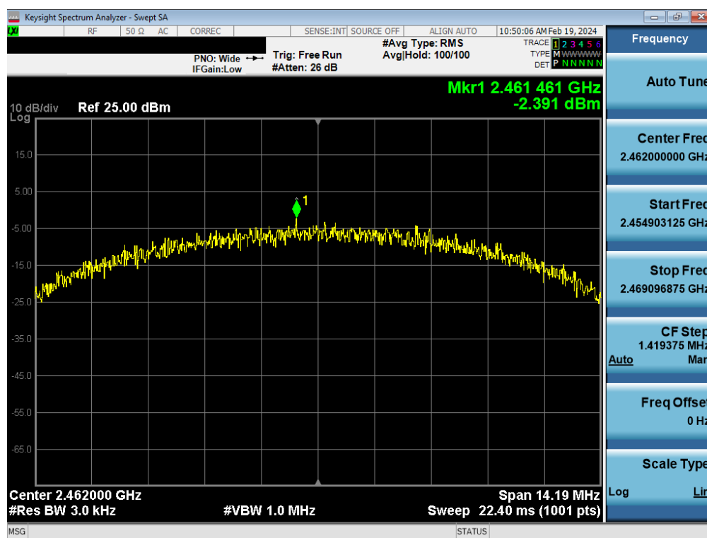
Plot 7-111. Power Spectral Density Plot Antenna WF8 (802.11b – Ch. 11) – 11Mbps
