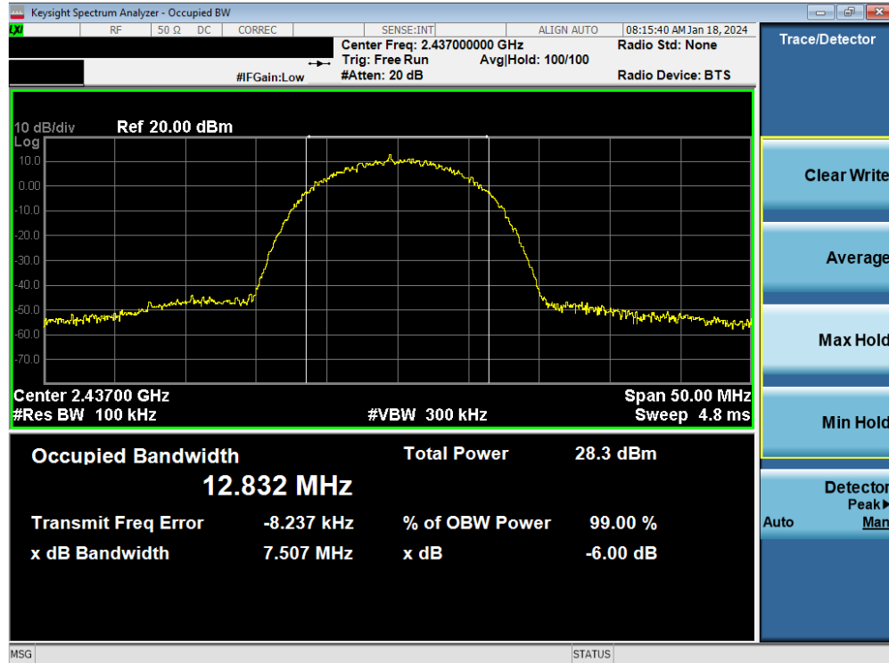
Plot 7-50. 6 dB BW and 99% OBW Plot Antenna WF7 (802.11b – Ch. 6) – 11Mbps
