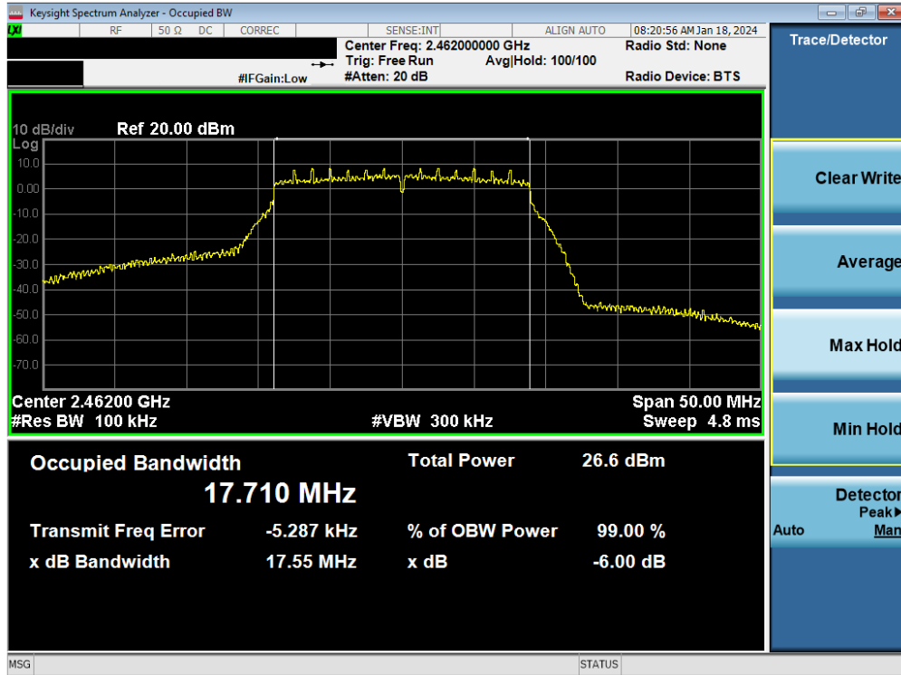
Plot 7-36. 6 dB BW and 99% OBW Plot Antenna WF7 (802.11n (2.4GHz) – Ch. 11) – MCS2
