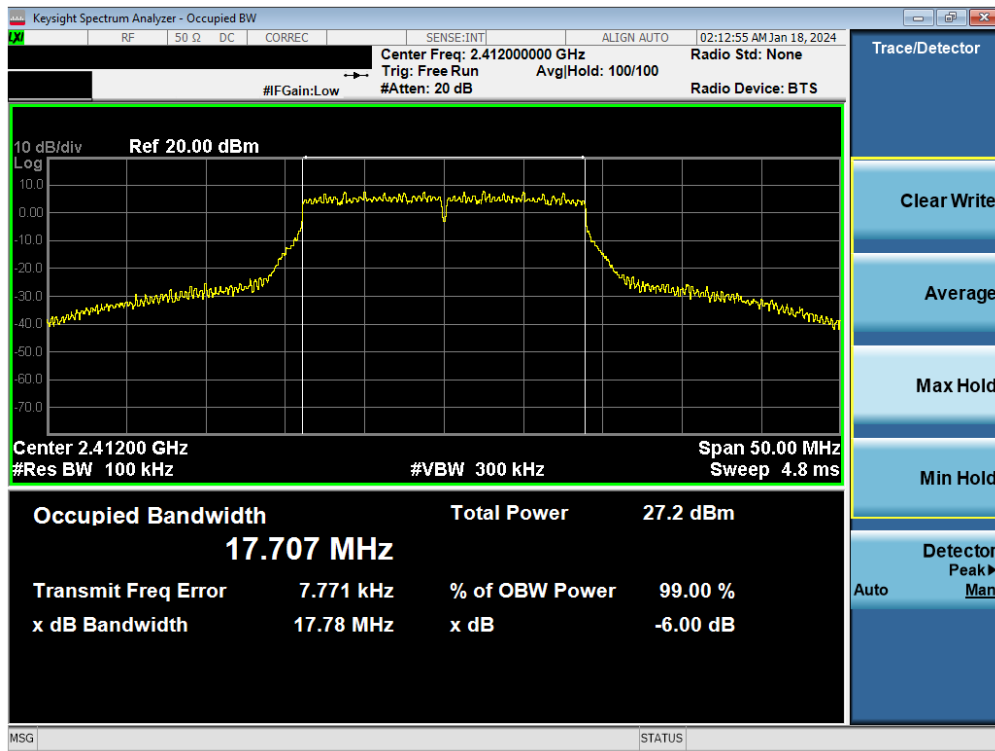
Plot 7-25. 6 dB BW and 99% OBW Plot Antenna WF8 (802.11n (2.4GHz) – Ch. 1) – MCS7
