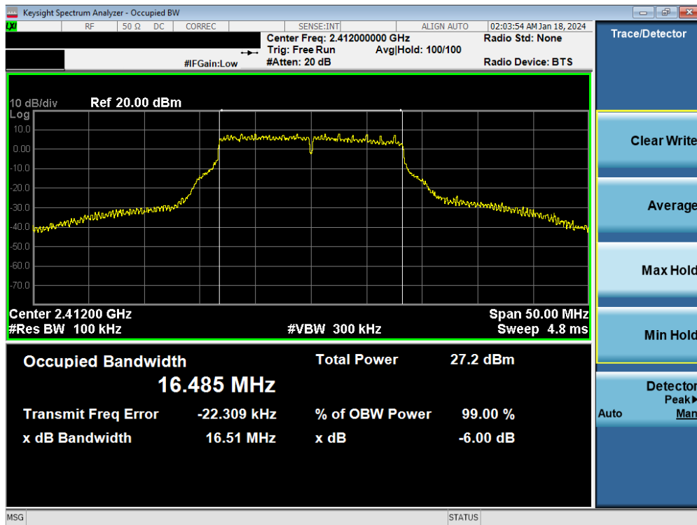
Plot 7-10. 6 dB BW and 99% OBW Plot Antenna WF8 (802.11g – Ch. 1) – 24Mbps
