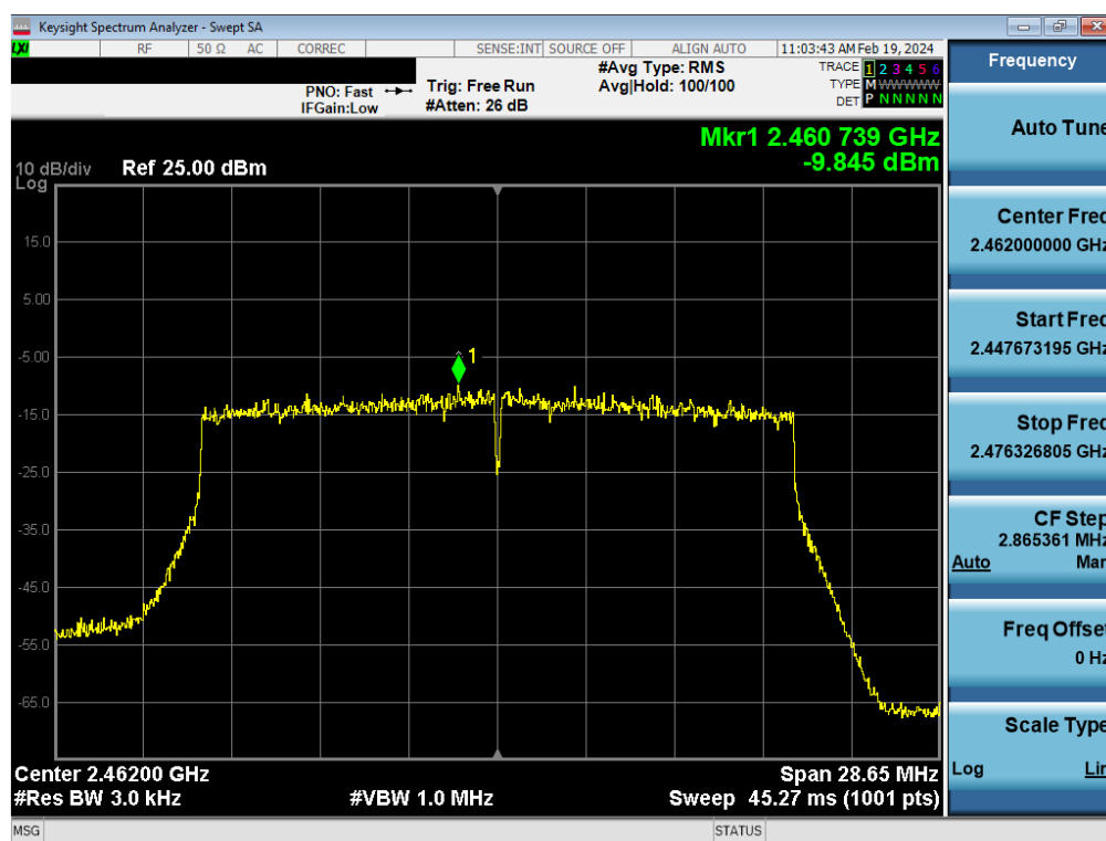
Plot 7-108. Power Spectral Density Plot Antenna WF8 (802.11ax (SU - 2.4GHz) – Ch. 11) – MCS4
