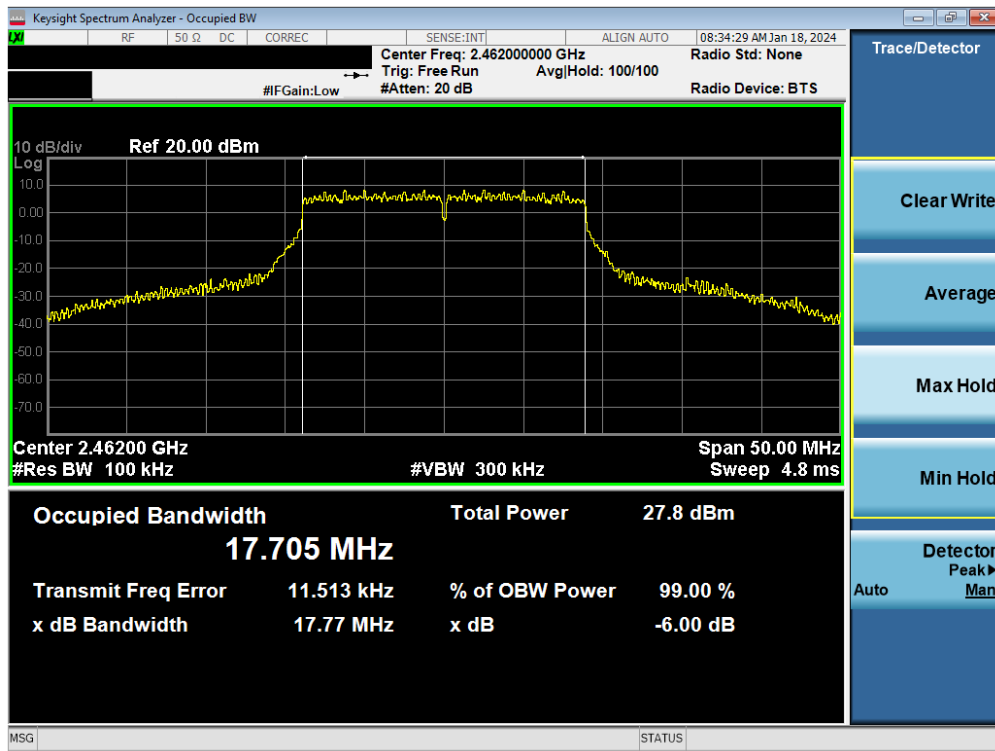
Plot 7-57. 6 dB BW and 99% OBW Plot Antenna WF7 (802.11n (2.4GHz) – Ch. 11) – MCS7
