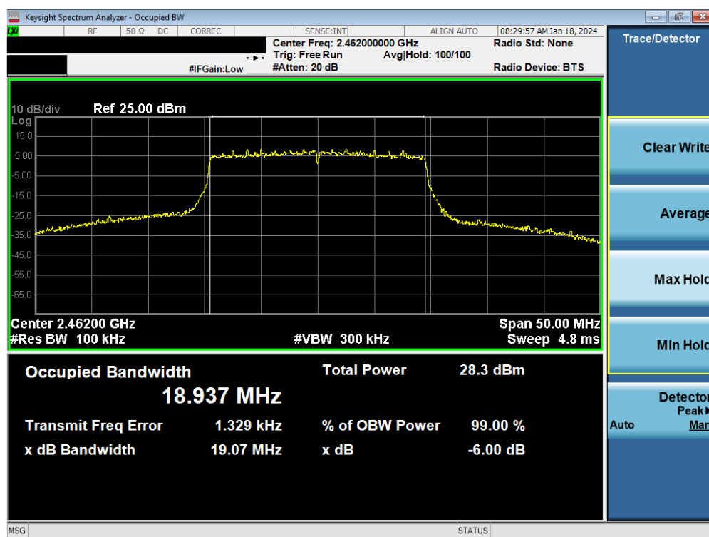
Plot 7-48. 6 dB BW and 99% OBW Plot Antenna WF7 (802.11ax (SU - 2.4GHz) – Ch. 11) – MCS4
