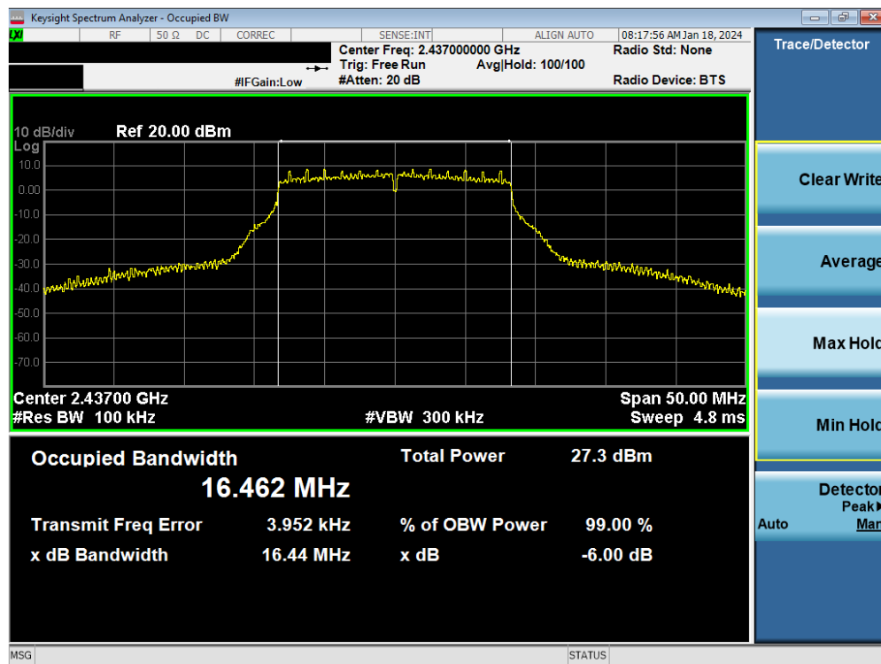
Plot 7-32. 6 dB BW and 99% OBW Plot Antenna WF7 (802.11g – Ch. 6) – 12Mbps
