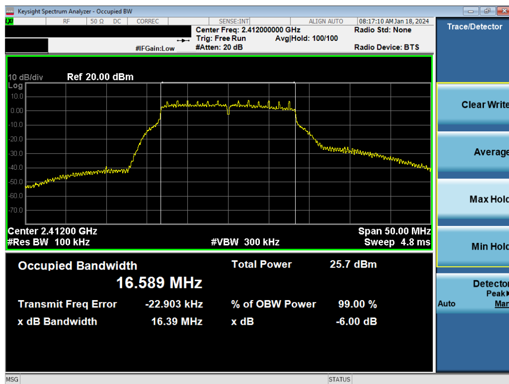
Plot 7-31. 6 dB BW and 99% OBW Plot Antenna WF7 (802.11g – Ch. 1) – 12Mbps
