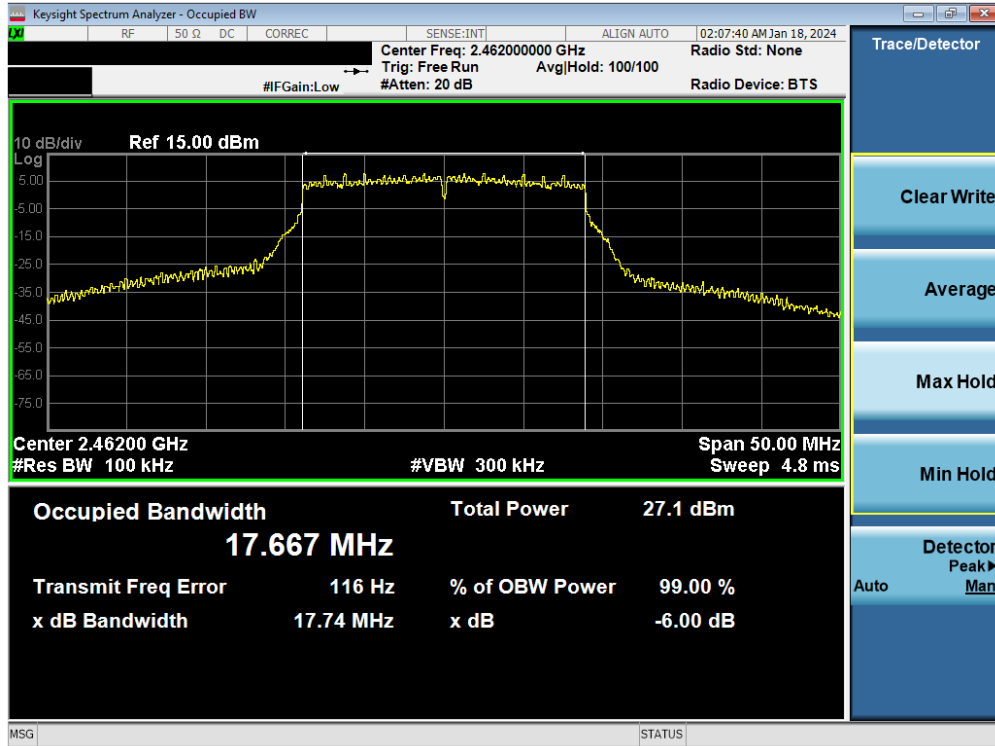
Plot 7-15. 6 dB BW and 99% OBW Plot Antenna WF8 (802.11n (2.4GHz) – Ch. 11) – MCS4
