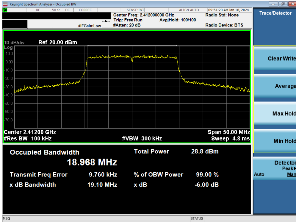
Plot 7-88. 6 dB BW and 99% OBW Plot Antenna WF9 (802.11ax (SU - 2.4GHz) – Ch. 1) – MCS9
