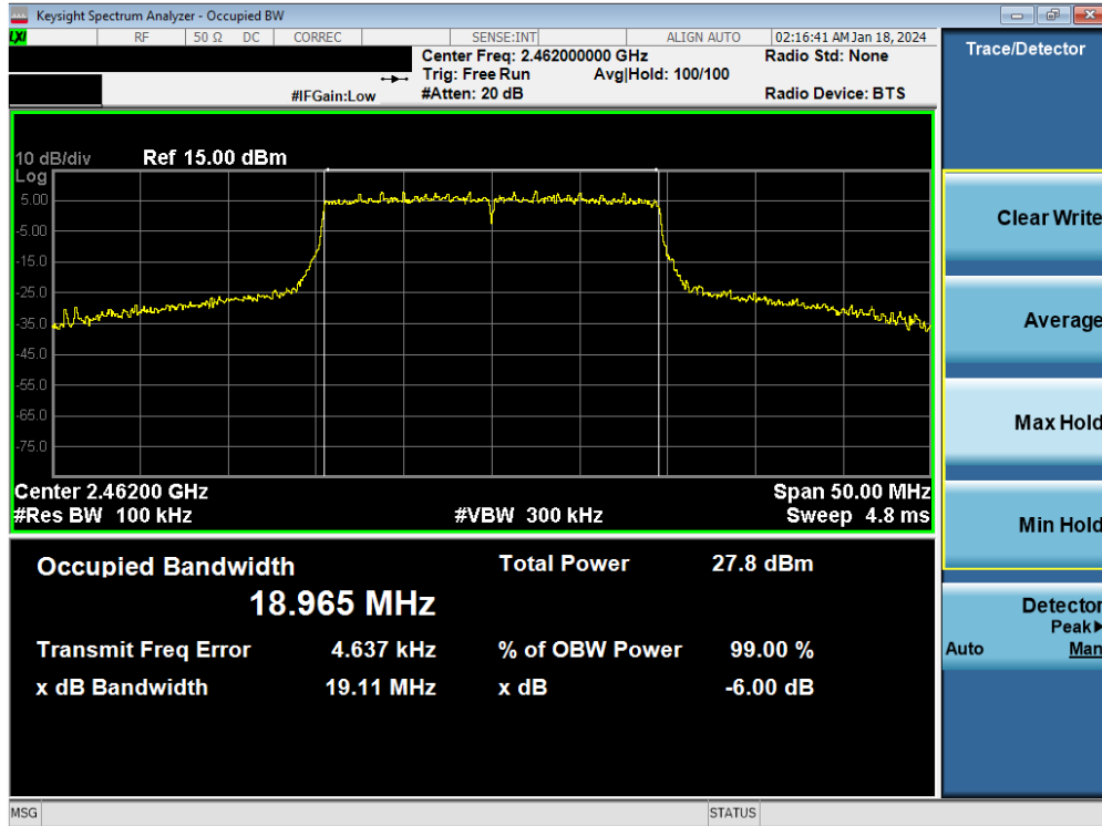
Plot 7-30. 6 dB BW and 99% OBW Plot Antenna WF8 (802.11ax (SU - 2.4GHz) – Ch. 11) – MCS9
