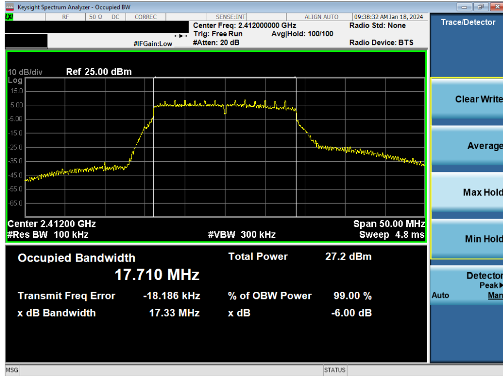
Plot 7-64. 6 dB BW and 99% OBW Plot Antenna WF9 (802.11n (2.4GHz) – Ch. 1) – MCS2
