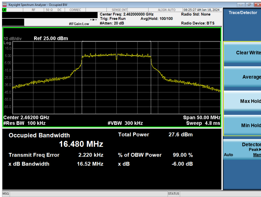
Plot 7-42. 6 dB BW and 99% OBW Plot Antenna WF7 (802.11g – Ch. 11) – 24Mbps
