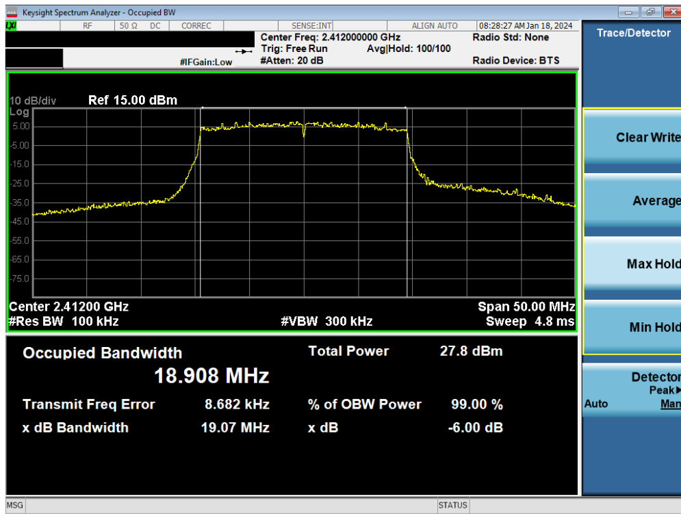
Plot 7-46. 6 dB BW and 99% OBW Plot Antenna WF7 (802.11ax (SU - 2.4GHz) – Ch. 1) – MCS4
