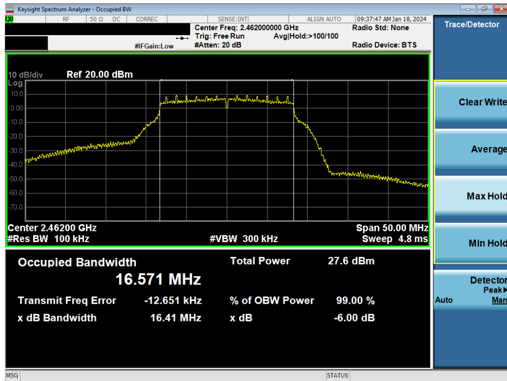
Plot 7-63. 6 dB BW and 99% OBW Plot Antenna WF9 (802.11g – Ch. 11) – 12Mbps
