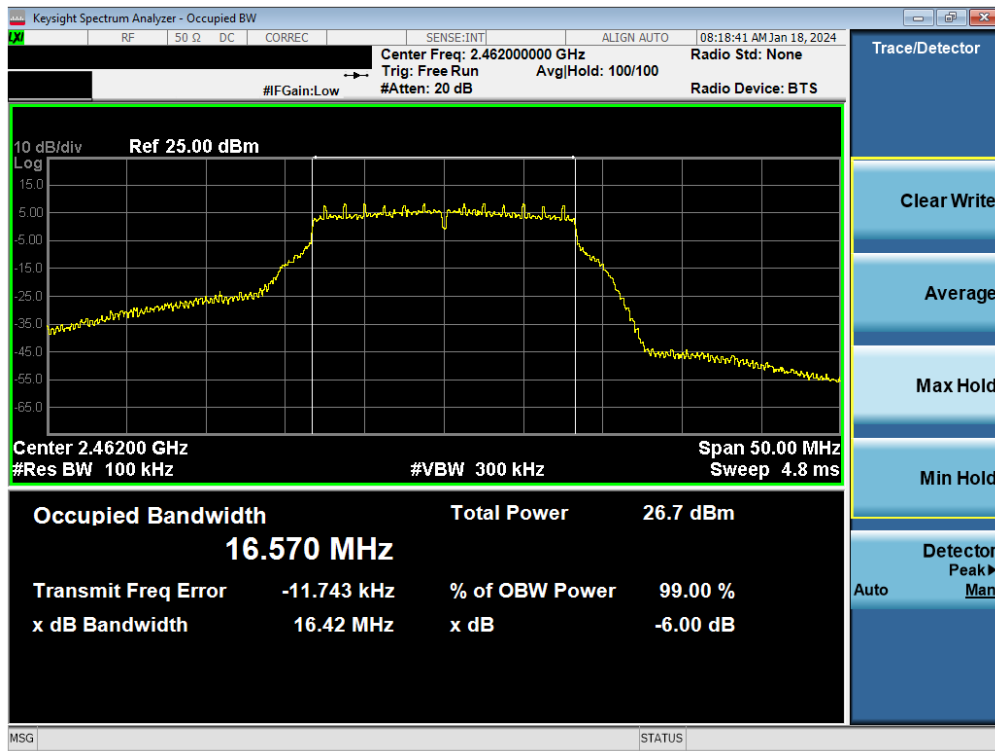
Plot 7-33. 6 dB BW and 99% OBW Plot Antenna WF7 (802.11g – Ch. 11) – 12Mbps
