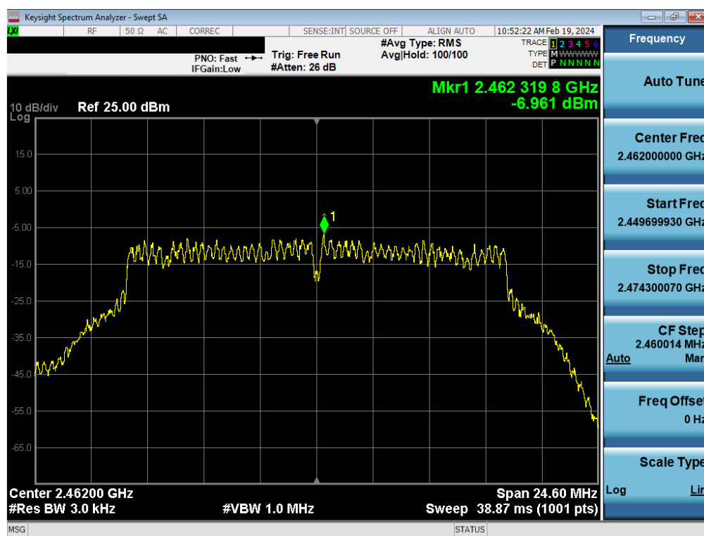
Plot 7-93. Power Spectral Density Plot Antenna WF8 (802.11g – Ch. 11) – 12Mbps
