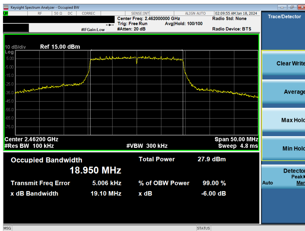
Plot 7-18. 6 dB BW and 99% OBW Plot Antenna WF8 (802.11ax (SU - 2.4GHz) – Ch. 11) – MCS4
