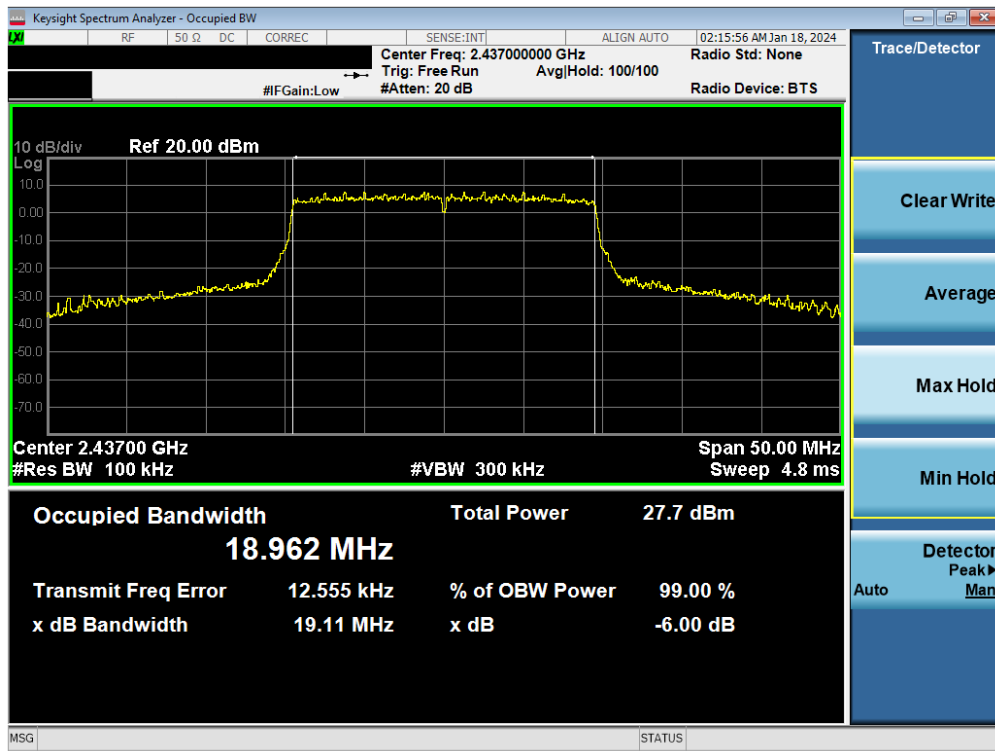
Plot 7-29. 6 dB BW and 99% OBW Plot Antenna WF8 (802.11ax (SU - 2.4GHz) – Ch. 6) – MCS9
