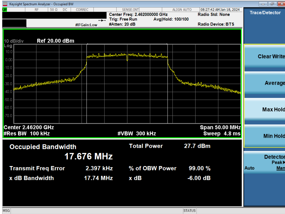
Plot 7-45. 6 dB BW and 99% OBW Plot Antenna WF7 (802.11n (2.4GHz) – Ch. 11) – MCS4
