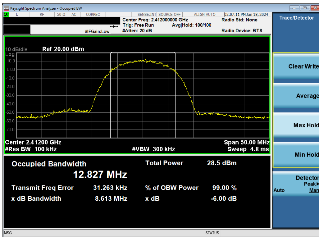
Plot 7-19. 6 dB BW and 99% OBW Plot Antenna WF8 (802.11b – Ch. 1) – 11Mbps
