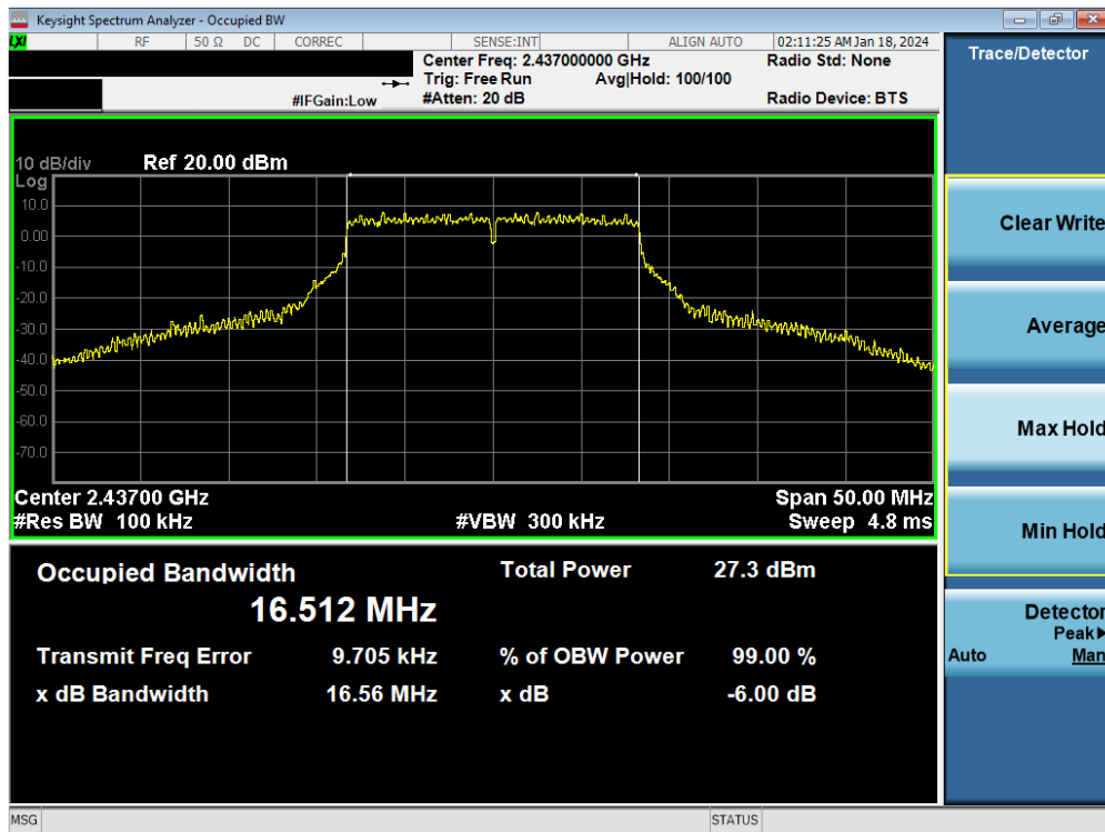
Plot 7-23. 6 dB BW and 99% OBW Plot Antenna WF8 (802.11g – Ch. 6) – 54Mbps
