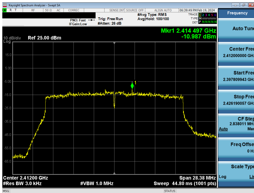
Plot 7-194. Power Spectral Density Plot CDD Primary Antenna WF7 (802.11ax (SU - 2.4GHz) – Ch. 1) – MCS2
