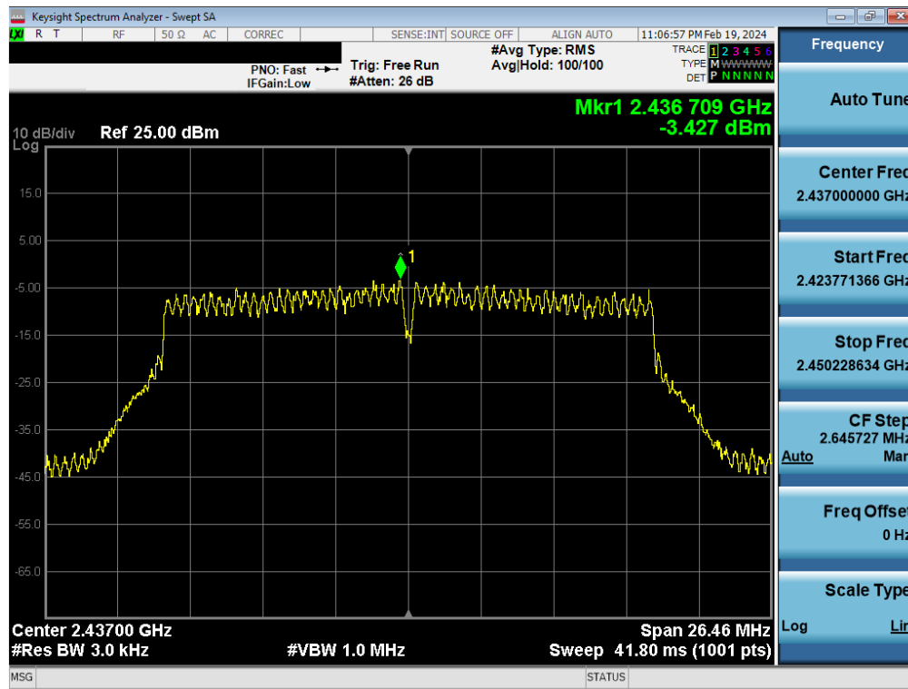
Plot 7-155. Power Spectral Density Plot Antenna WF9 (802.11n (2.4GHz) – Ch. 6) – MCS2
