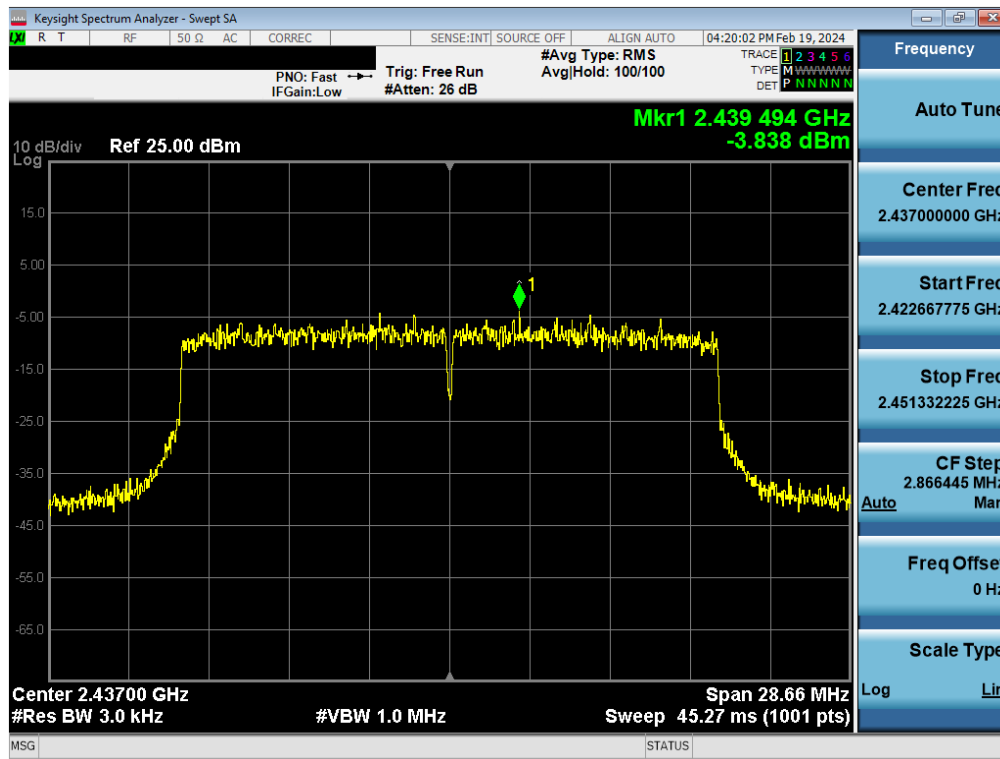
Plot 7-149. Power Spectral Density Plot Antenna WF7 (802.11ax (SU - 2.4GHz) - Ch. 6) - MCS9
