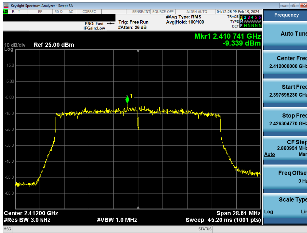
Plot 7-136. Power Spectral Density Plot Antenna WF7 (802.11ax (SU - 2.4GHz) - Ch. 1) - MCS4
