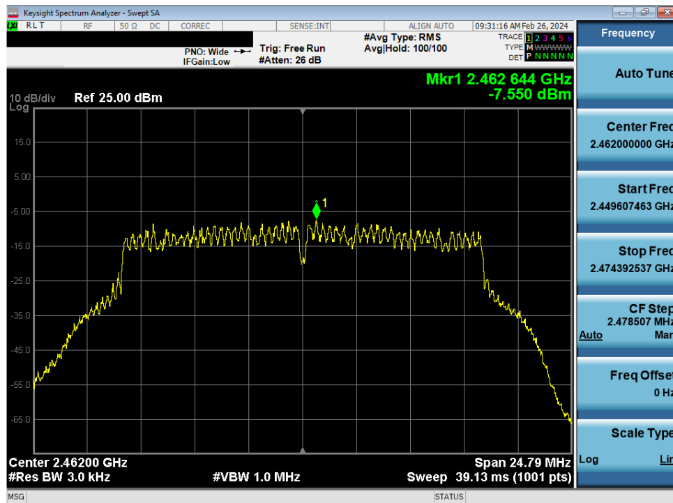
Plot 7-204. Power Spectral Density Plot CDD Primary Antenna WF7 (802.11g- Ch. 11) – 24Mbps
