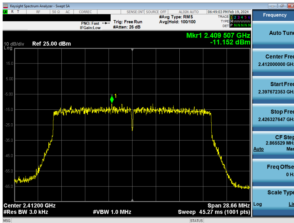
Plot 7-230. Power Spectral Density Plot CDD Primary Antenna WF7 (802.11ax (SU - 2.4GHz) – Ch. 1) – MCS9
