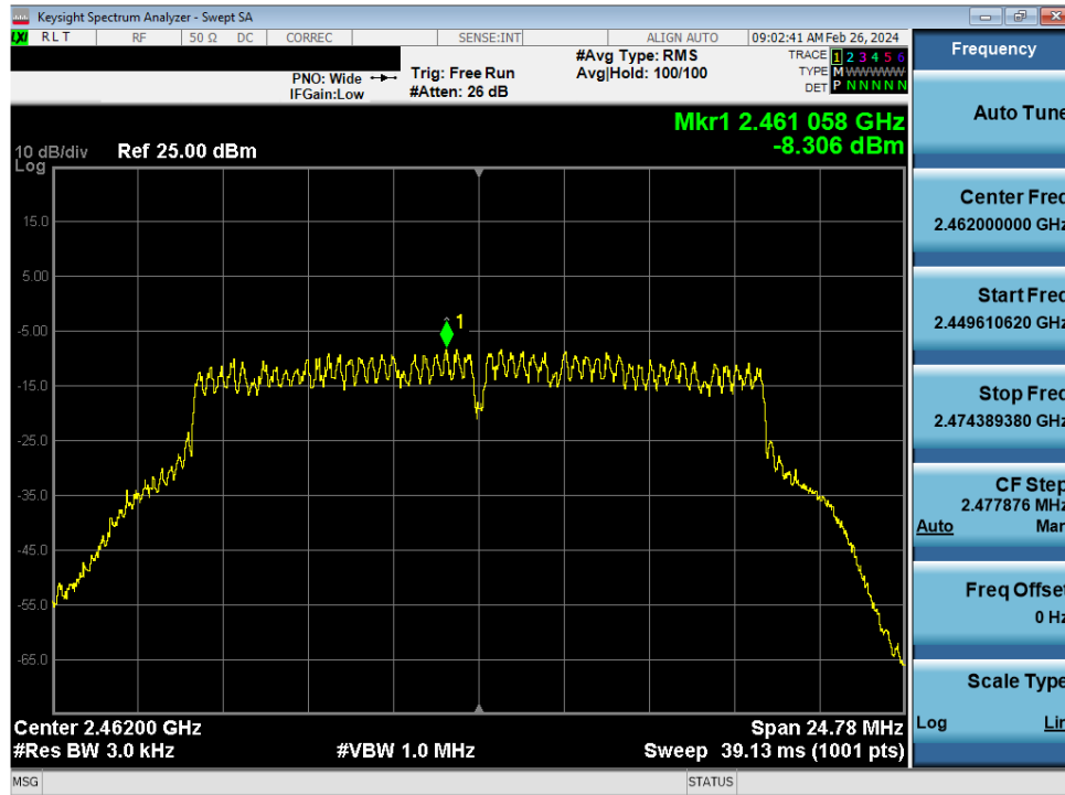
Plot 7-203. Power Spectral Density Plot CDD Primary Antenna WF8 (802.11g- Ch. 11) – 24Mbps
