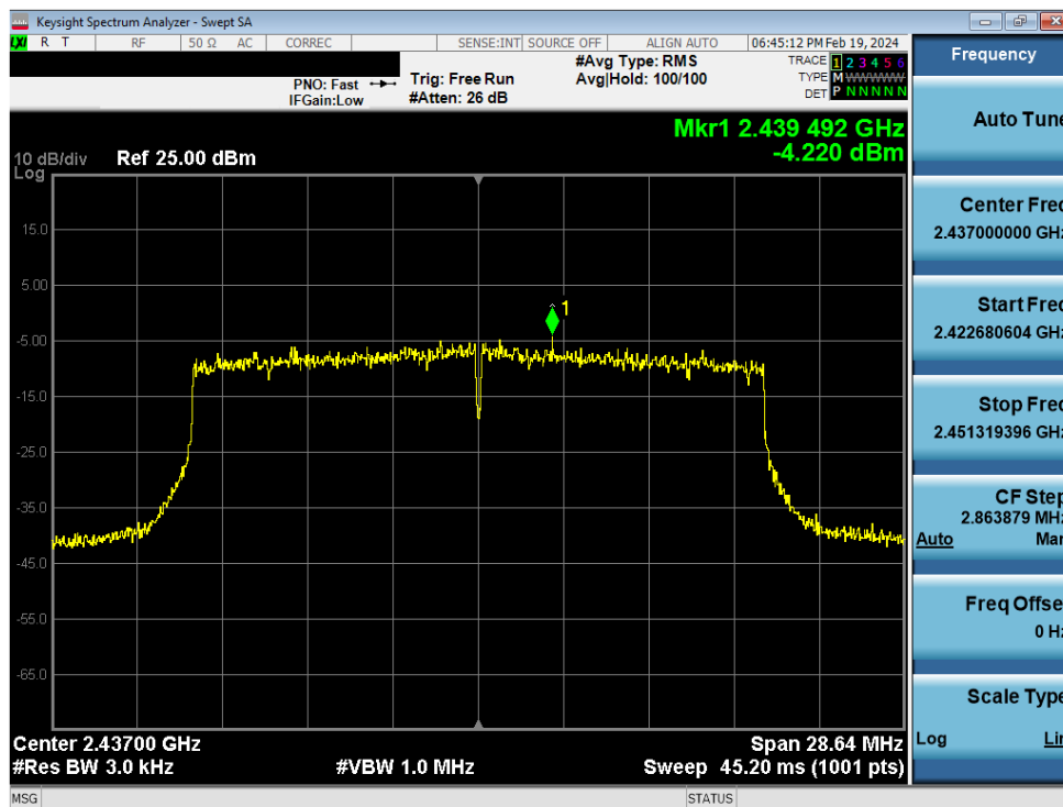
Plot 7-214. Power Spectral Density Plot CDD Primary Antenna WF7 (802.11ax (SU - 2.4GHz) – Ch. 6) – MCS4
