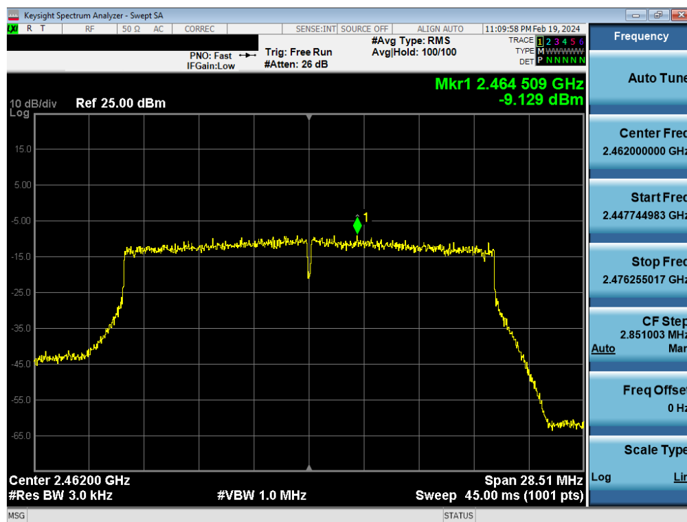
Plot 7-159. Power Spectral Density Plot Antenna WF9 (802.11ax (SU - 2.4GHz) – Ch. 11) – MCS2
