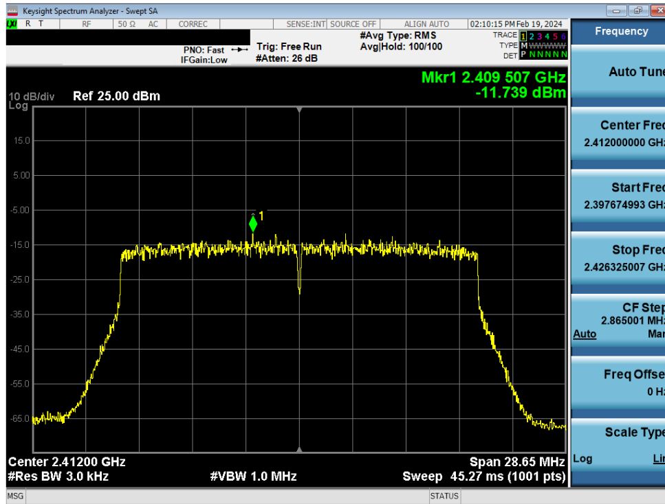
Plot 7-229. Power Spectral Density Plot CDD Primary Antenna WF8 (802.11ax (SU - 2.4GHz) – Ch. 1) – MCS9
