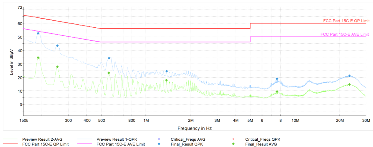
Plot 7-966. AC Line Conducted Plot with CDD Diversity 11ax - SU Ch.6 (N, with Laptop)
