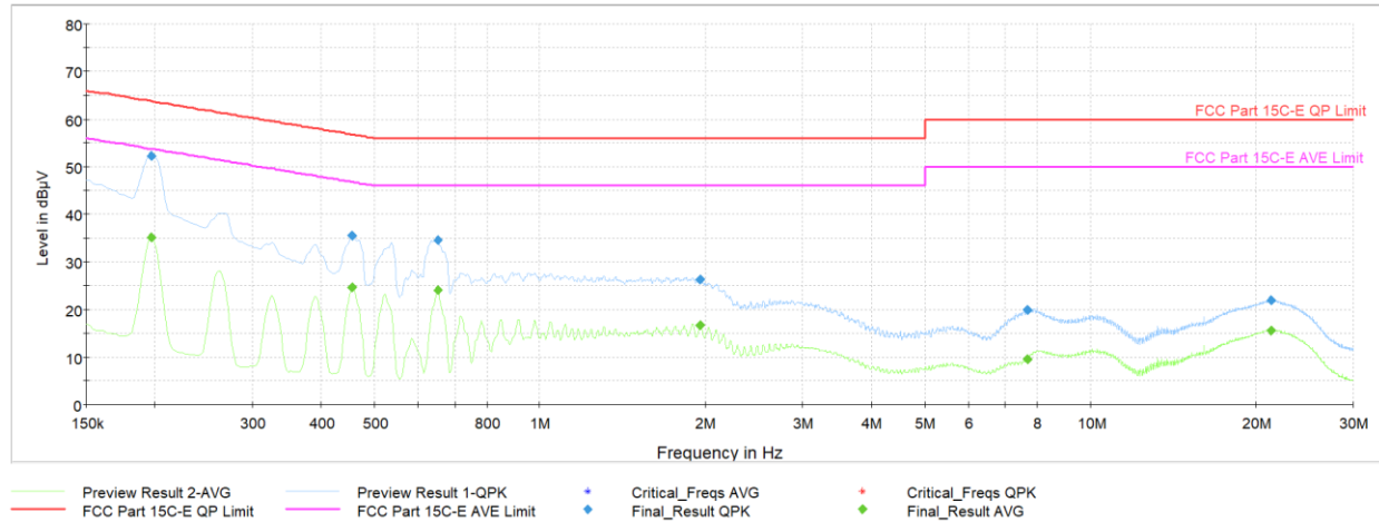
Plot 7-965. AC Line Conducted Plot with CDD Diversity 11ax - SU Ch.6 (L1, with Laptop)
