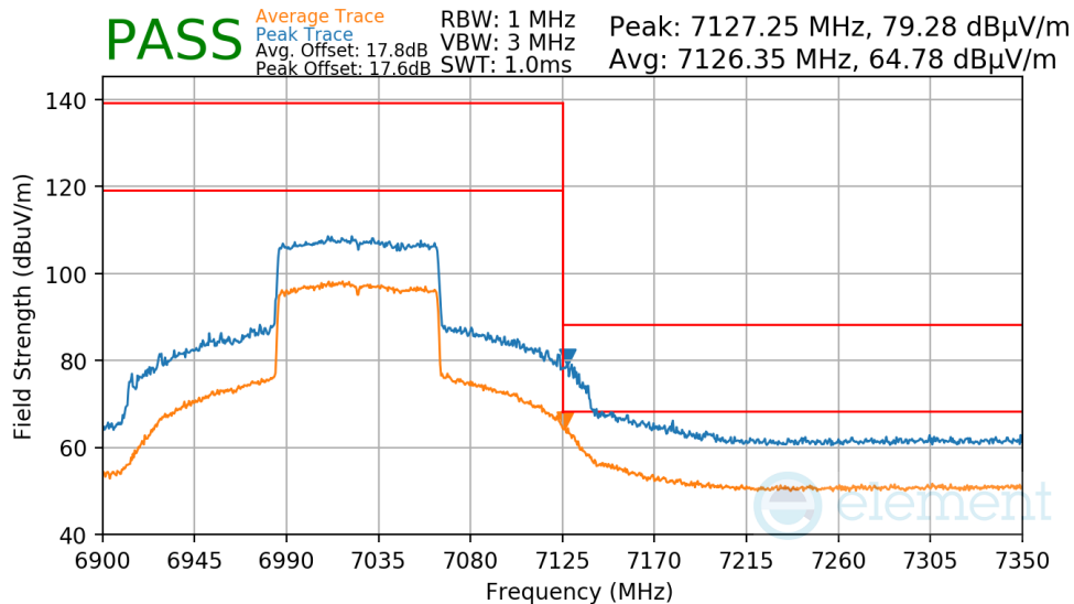
Plot 7-1370. Antenna 2a Radiated Upper Band Edge (Peak & Average – UNII Band 8)
