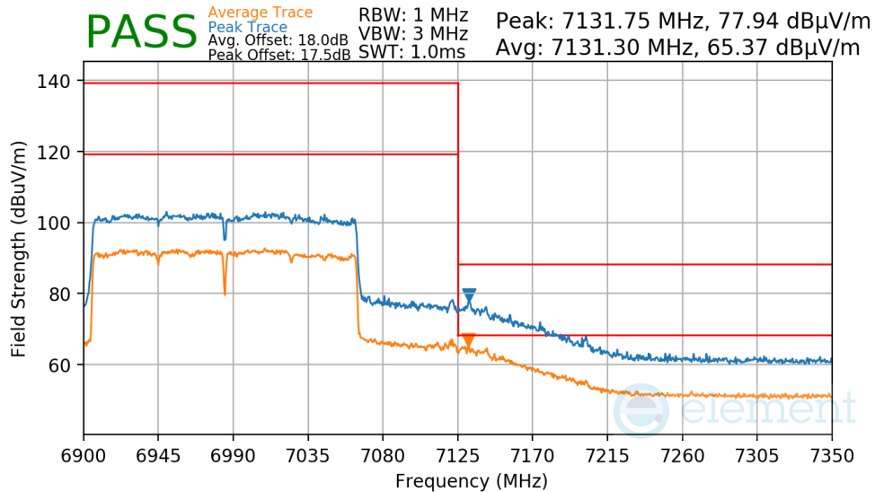
Plot 7-1377. Antenna 2a Radiated Upper Band Edge (Peak & Average – UNII Band 8)
