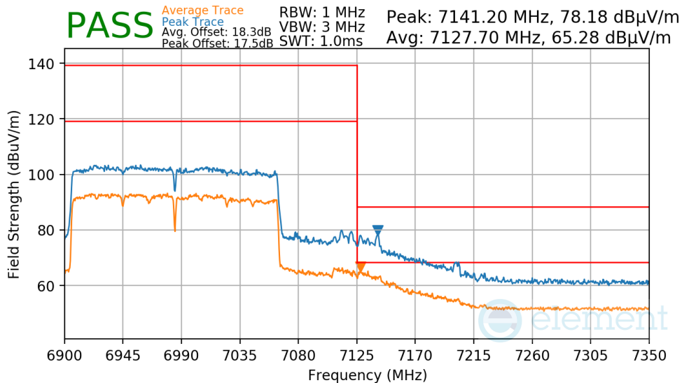
Plot 7-1378. Antenna 2a Radiated Upper Band Edge (Peak & Average – UNII Band 8)
