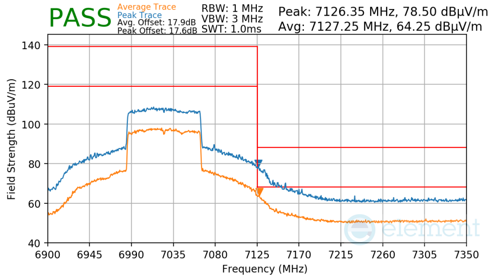
Plot 7-1371. Antenna 2a Radiated Upper Band Edge (Peak & Average – UNII Band 8)
