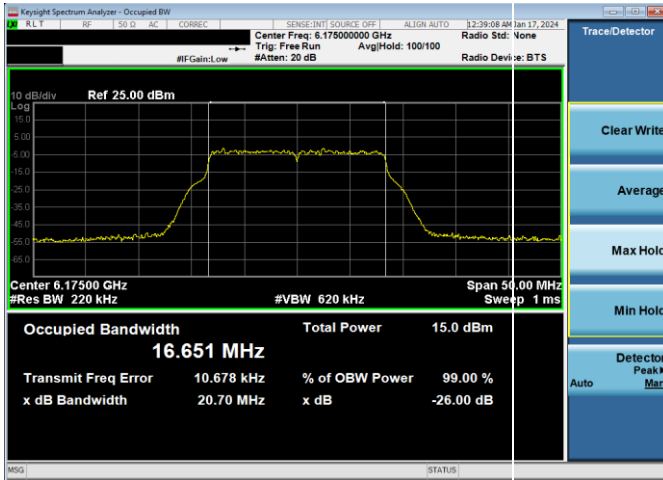
Plot 7-161. 26dB & 99% Bandwidth Plot Antenna 2a (20MHz 802.11a (UNII Band 5) – Ch. 45, 54Mbps)
