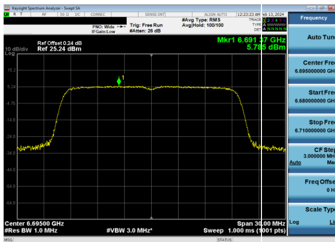
Plot 7-327. SP Power Spectral Density Plot SDM Primary Antenna WF5B (20MHz 802.11ax RU242 (UNII Band 7) – Ch. 149)
