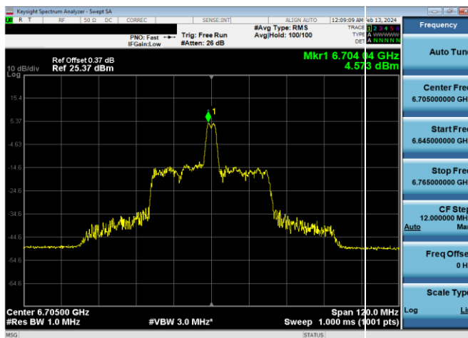
Plot 7-339. SP Power Spectral Density Plot SDM Primary Antenna WF5B (80MHz 802.11ax RU26 (UNII Band 7) – Ch. 151)
