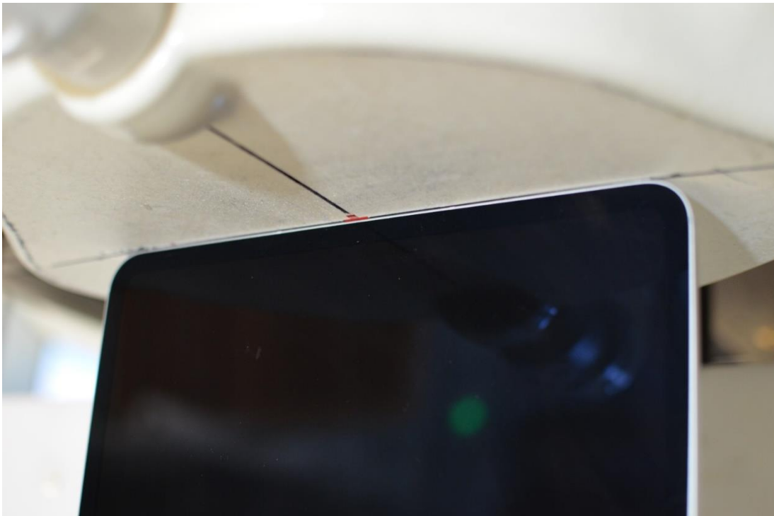
SAR Test Setup Photo 4: Body, Bottom Edge at 0mm
