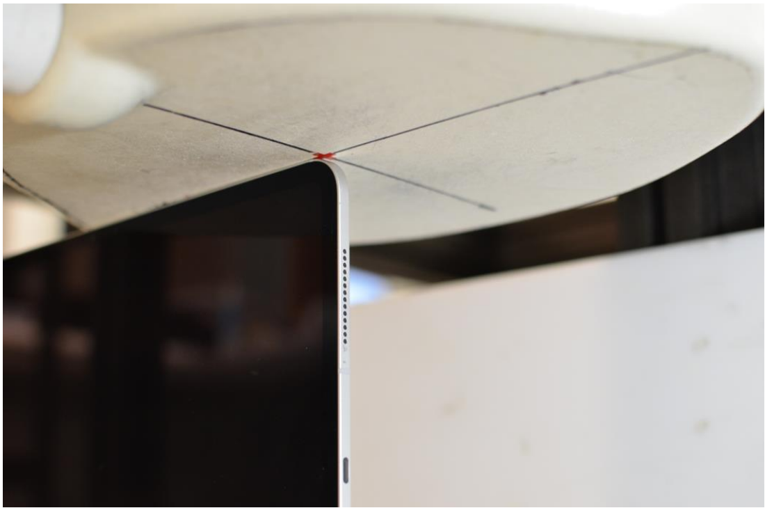
SAR Test Setup Photo 6: Body, Right Edge at 0mm – Antenna 1/2a/2b/WF5B
