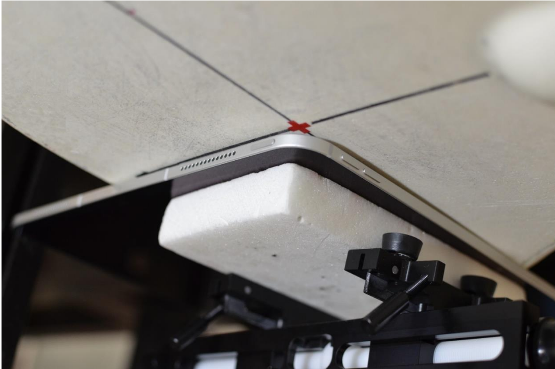
SAR Test Setup Photo 1: Body, Back Side at 0mm – Antenna 3/4a/4b
