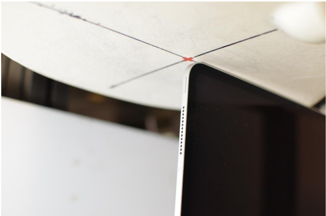
SAR Test Setup Photo 5: Body, Right Edge at 0mm – Antenna 3/4a/4b
