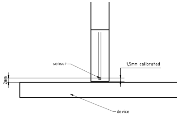
Figure I-2 EUMmWVx Probe
