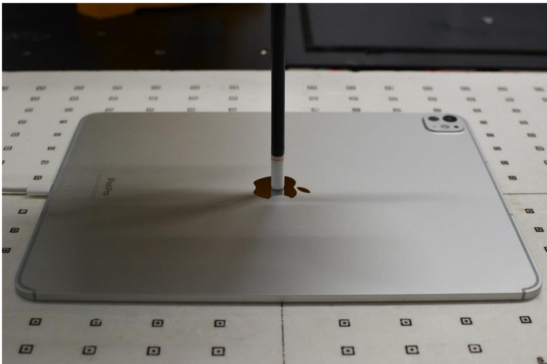
Near Field Power Density Test Setup 9: Back Side at 2mm – Antenna 2a/4a/WF5B
