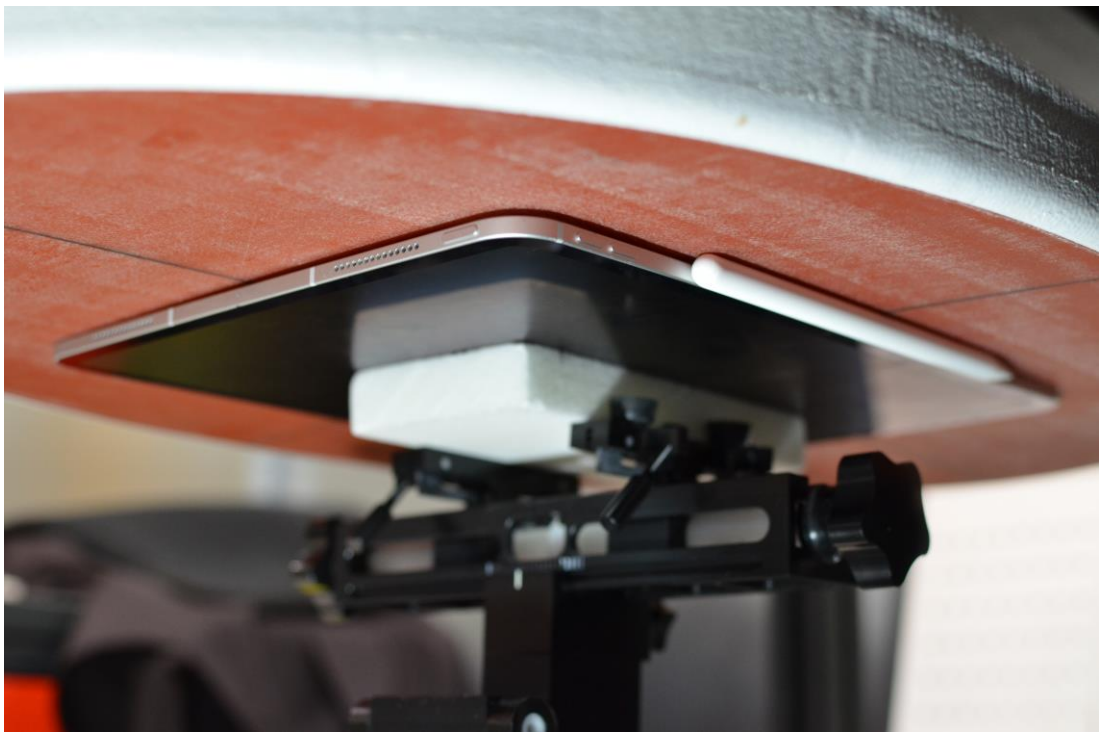
Wireless Power Transfer (wPT) Test Setup Photo 15: Back Side at 0mm
