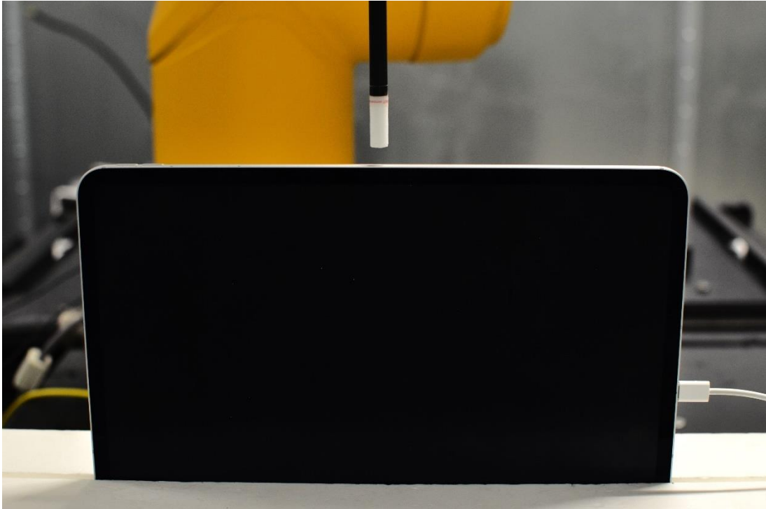
Near Field Power Density Test Setup 13: Right Edge at 9.95mm – Antenna WF5B
