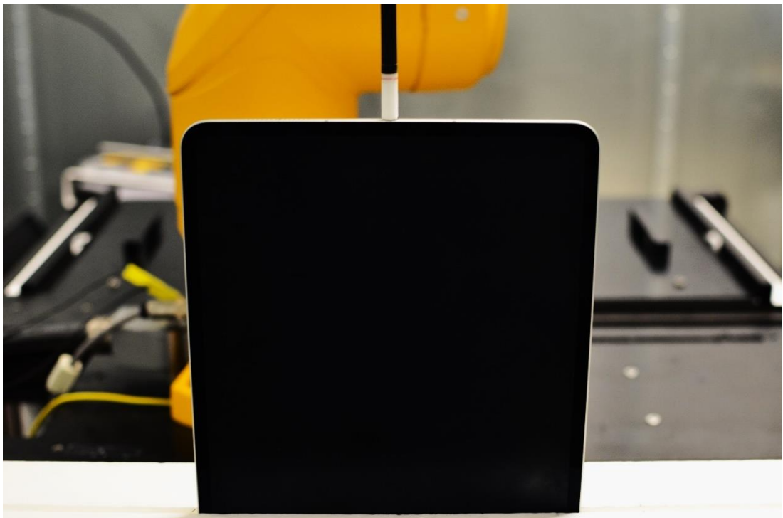
Near Field Power Density Test Setup 11: Bottom Edge at 2mm – Antenna 2a/4a/WF5B
