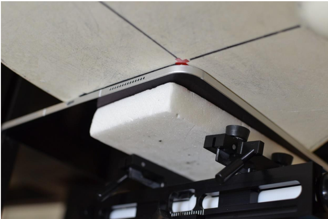
SAR Test Setup Photo 2: Body, Back Side at 0mm– Antenna 1/2a/2b/WF5B
