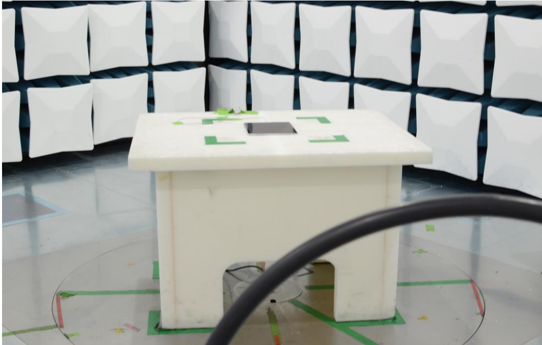
Figure 23: 9kHz-30MHz Test Setup (Front View)
