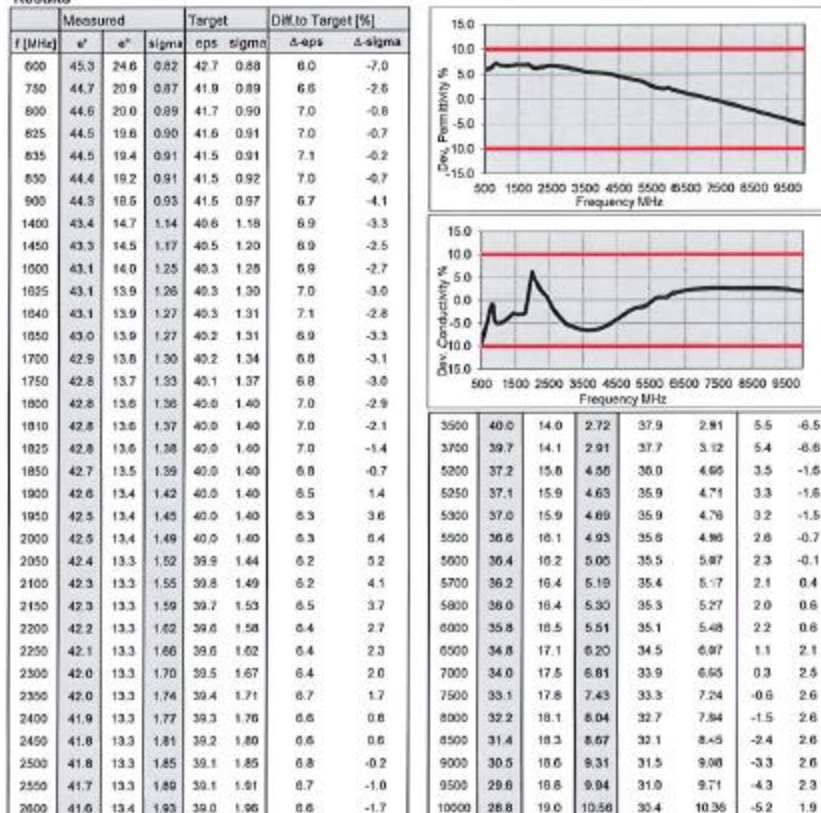
Figure D-2 600 –10000 MHz Head Tissue Equivalent Matte
