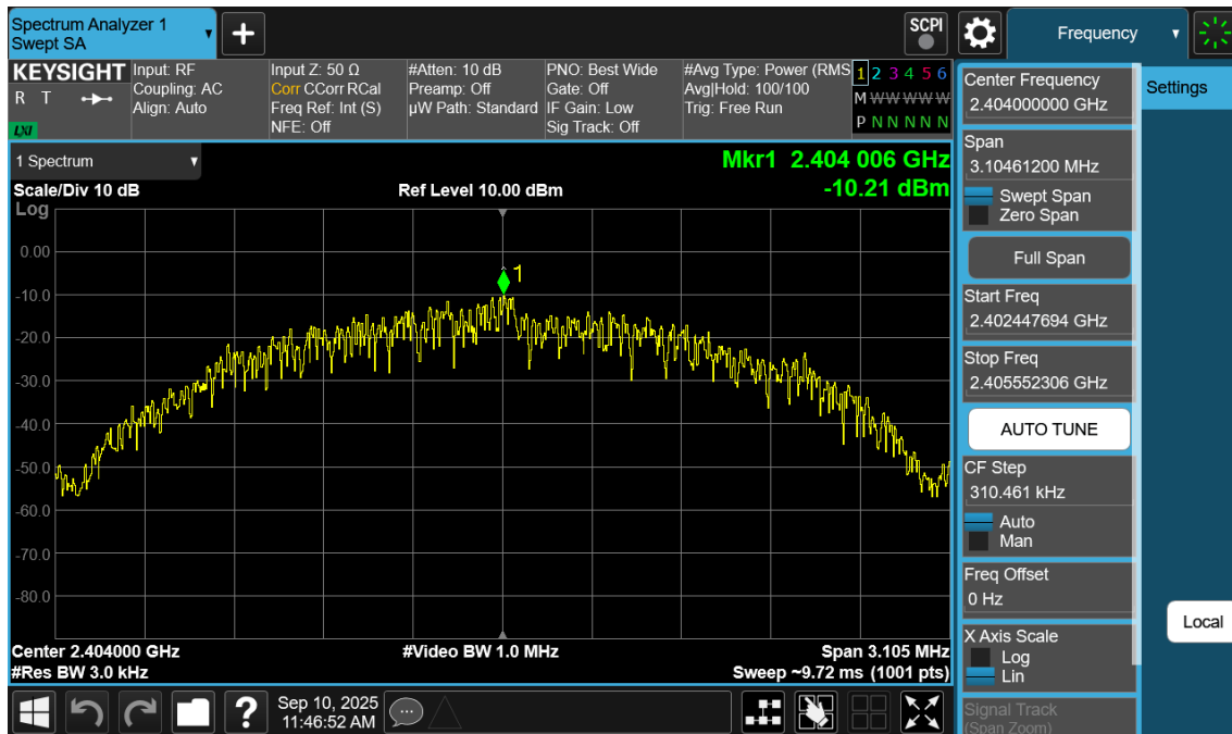
Plot 7-16. Power Spectral Density Plot (Bluetooth (LE), 2Mbps – Ch. 1)
