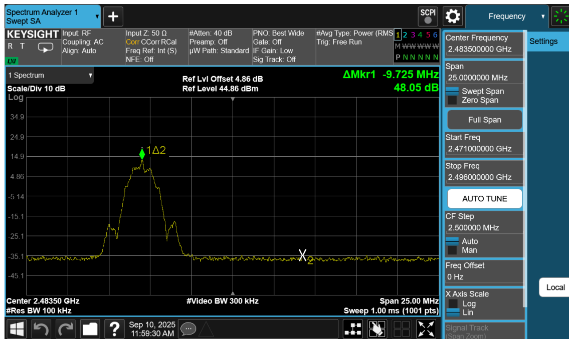
Plot 7-22. Band Edge Plot (Bluetooth (LE), 2Mbps – Ch. 38)
