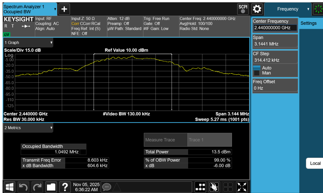
Plot 7-2. 99% OBW Plot (Bluetooth (LE), 1Mbps, ePA – Ch. 19)
