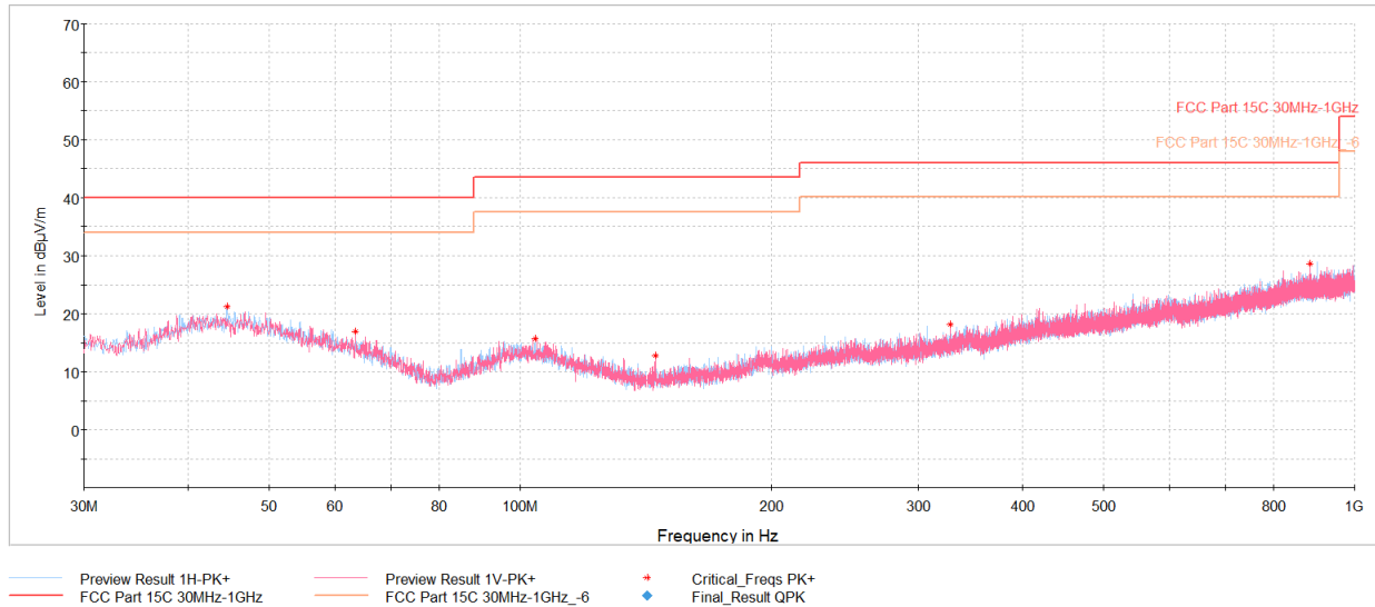
Plot 7-37. Radiated Spurious Emissions Below 1GHz (1Mbps – Ch.19, Pol. H & V)
