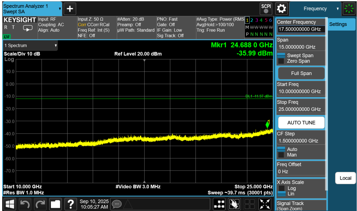
Plot 7-26. Conducted Spurious Plot (Bluetooth (LE), 1Mbps – Ch. 19)
