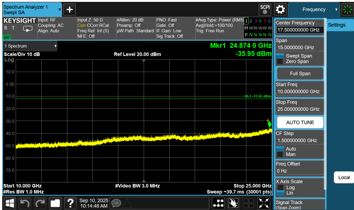
Plot 7-28. Conducted Spurious Plot (Bluetooth (LE), 1Mbps – Ch. 39)
