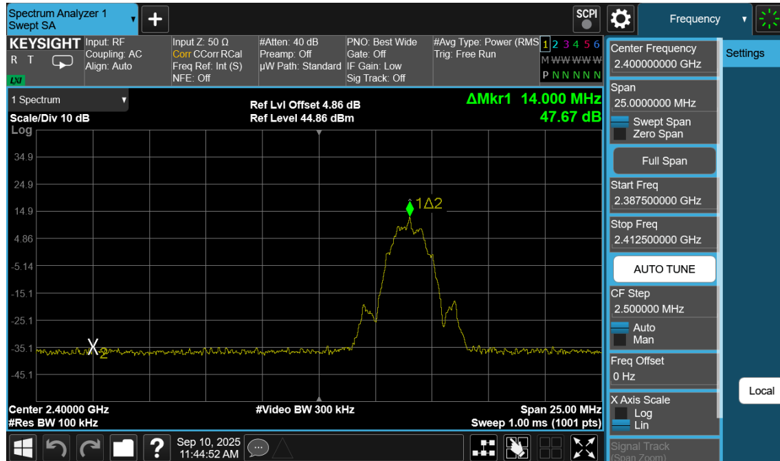
Plot 7-21. Band Edge Plot (Bluetooth (LE), 2Mbps – Ch. 1)
