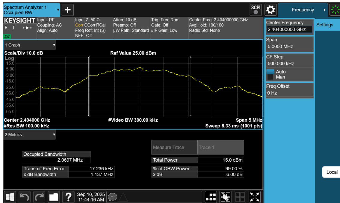
Plot 7-10. 6dB BW OBW Plot (Bluetooth (LE), 2Mbps – Ch. 1)
