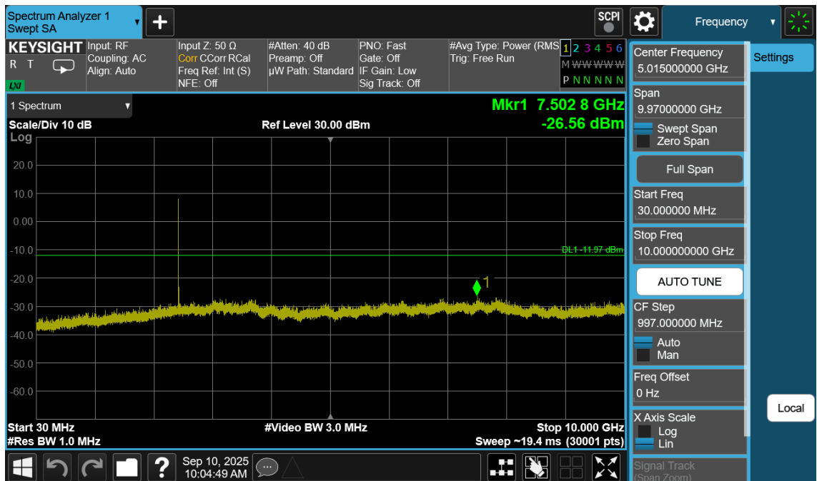
Plot 7-25. Conducted Spurious Plot (Bluetooth (LE), 1Mbps – Ch. 19)
