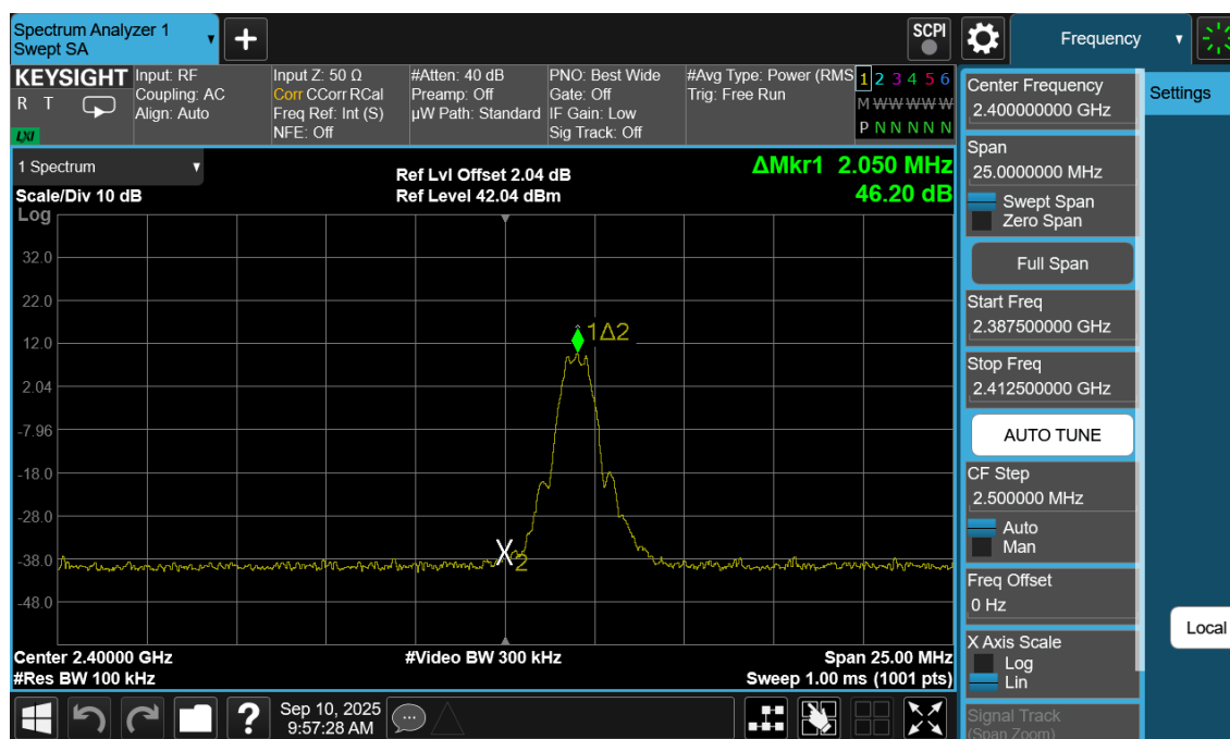
Plot 7-19. Band Edge Plot (Bluetooth (LE), 1Mbps – Ch.0)
