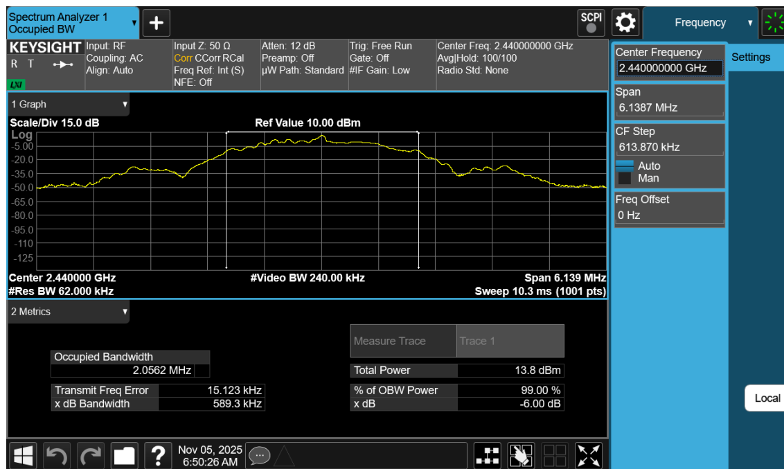
Plot 7-5. 99% OBW Plot (Bluetooth (LE), 2Mbps, ePA – Ch. 19)
