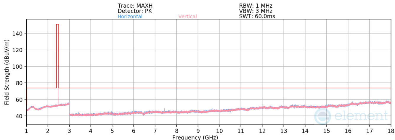
Plot 7-32. Radiated Spurious Emissions 1-18GHz (1Mbps – Ch. 39)
