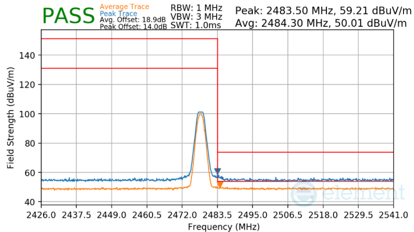
Plot 7-36. Radiated Restricted Upper Band Edge Measurement (Average & Peak)
