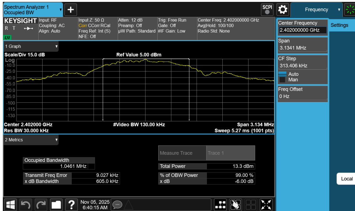
Plot 7-1. 99% OBW Plot (Bluetooth (LE), 1Mbps, ePA – Ch. 0)
