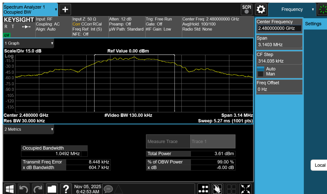
Plot 7-3. 99% OBW Plot (Bluetooth (LE), 1Mbps, ePA – Ch. 39)
