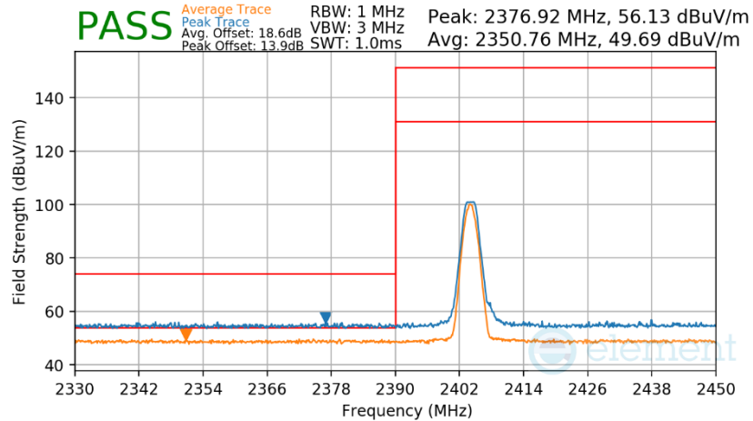
Plot 7-35. Radiated Restricted Lower Band Edge Measurement (Average & Peak)
