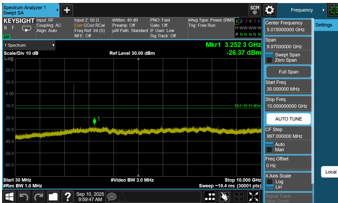
Plot 7-23. Conducted Spurious Plot (Bluetooth (LE), 1Mbps – Ch. 0)
