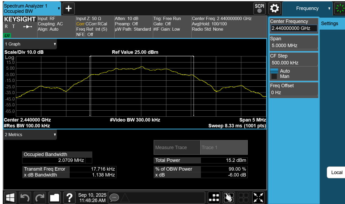
Plot 7-11. 6dB BW OBW Plot (Bluetooth (LE), 2Mbps – Ch. 19)
