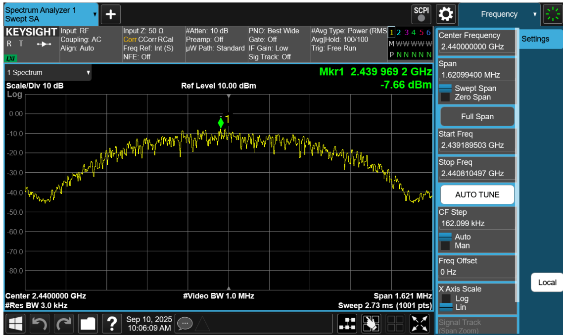
Plot 7-14. Power Spectral Density Plot (Bluetooth (LE), 1Mbps – Ch. 19)
