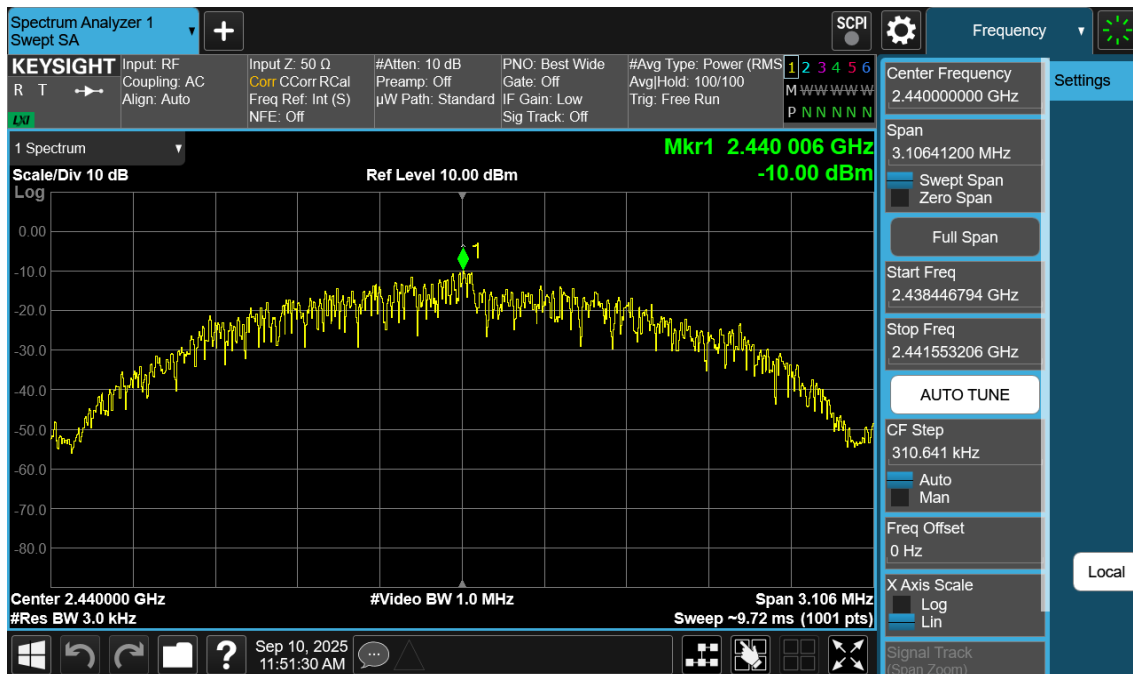
Plot 7-17. Power Spectral Density Plot (Bluetooth (LE), 2Mbps – Ch. 19)
