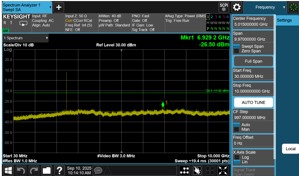
Plot 7-27. Conducted Spurious Plot (Bluetooth (LE), 1Mbps – Ch. 39)
