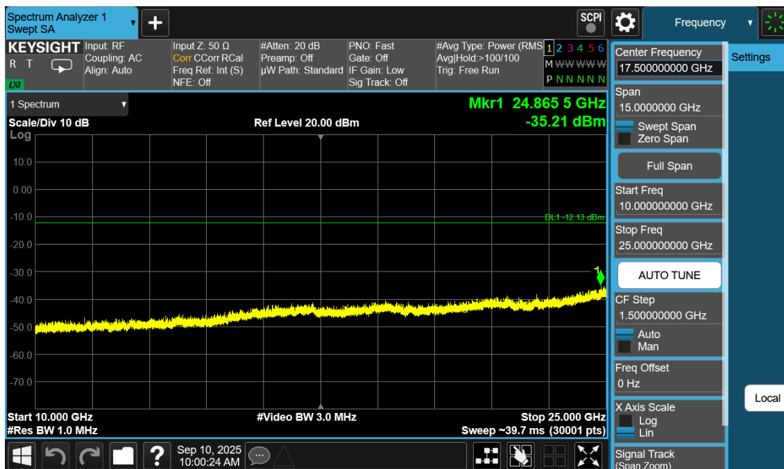
Plot 7-24. Conducted Spurious Plot (Bluetooth (LE), 1Mbps – Ch. 0)
