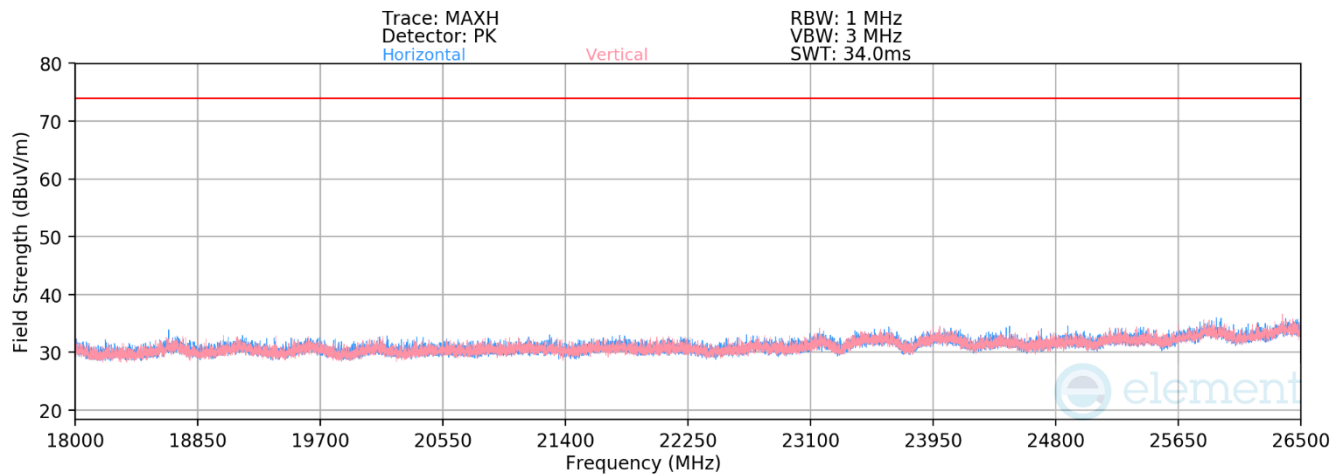
Plot 7-31. Radiated Spurious Emissions Above 18GHz (1Mbps – Ch. 19)
