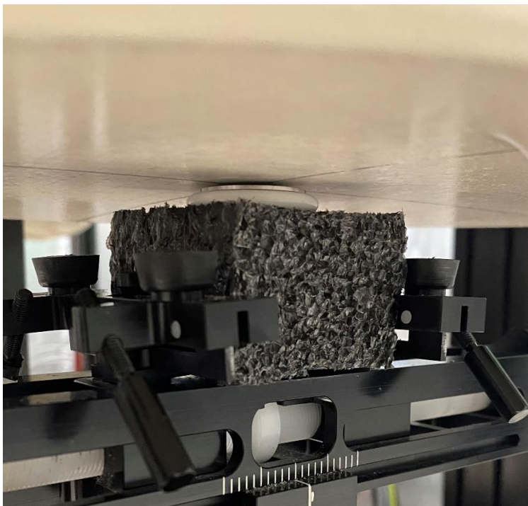
SAR Test Setup Photo 2: Body-worn and Extremity, Back Side at 0.0 cm
