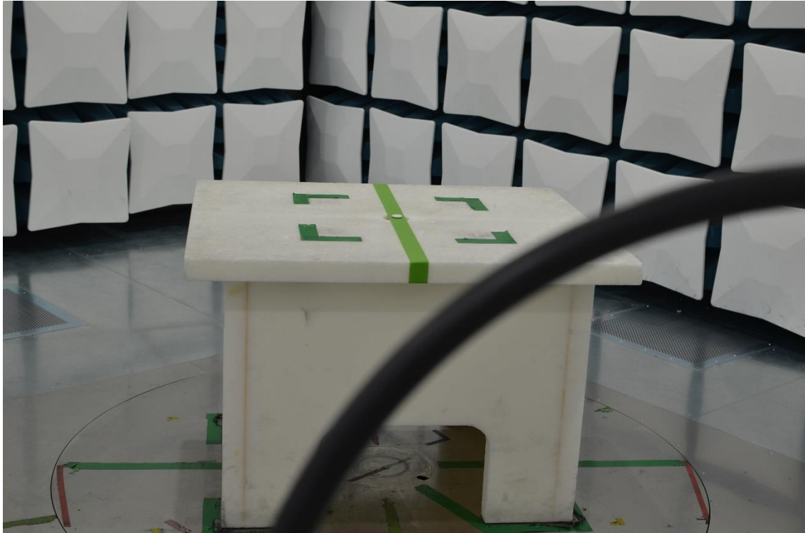
Figure 13: 9kHz-30MHz Test Setup (Front View)
