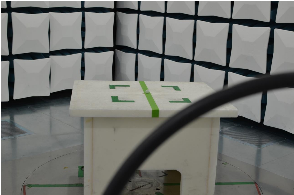
Figure 14: 9kHz-30MHz Test Setup (Front View)
