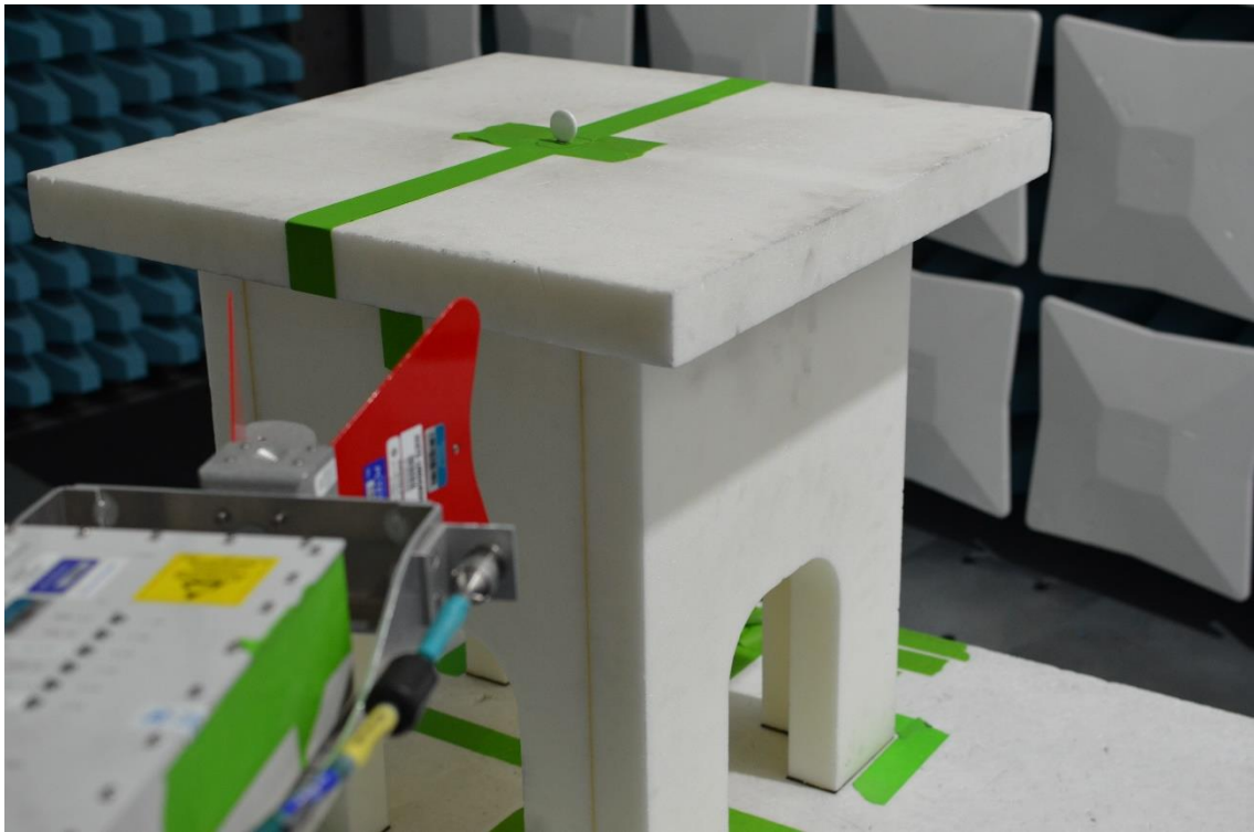
Figure 2: Above 960MHz Test Setup
