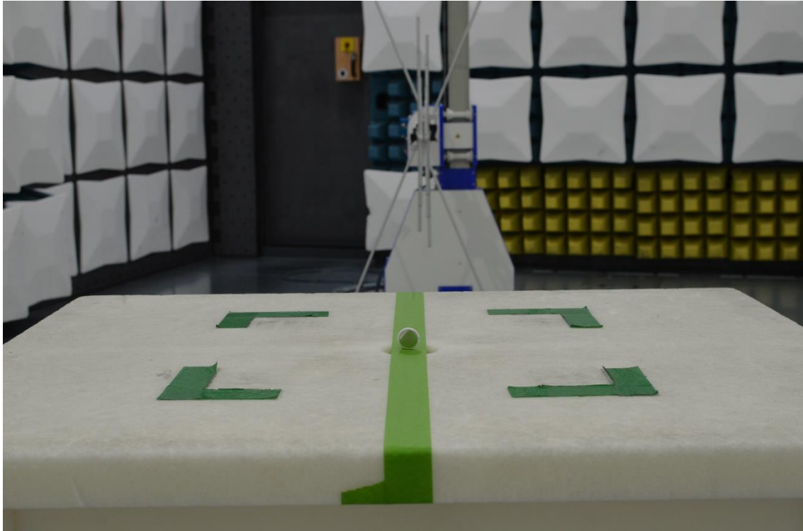
Figure 7: 30MHz-1GHz Test Setup (Rear View)
