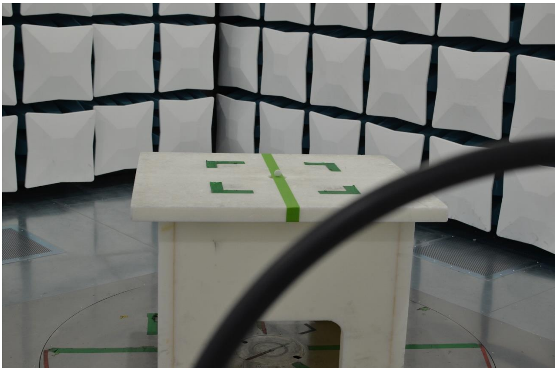
Figure 11: 9kHz-30MHz Test Setup (Front View)
