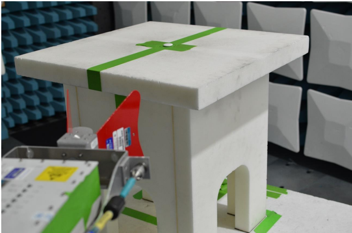
Figure 1: Above 960MHz Test Setup
