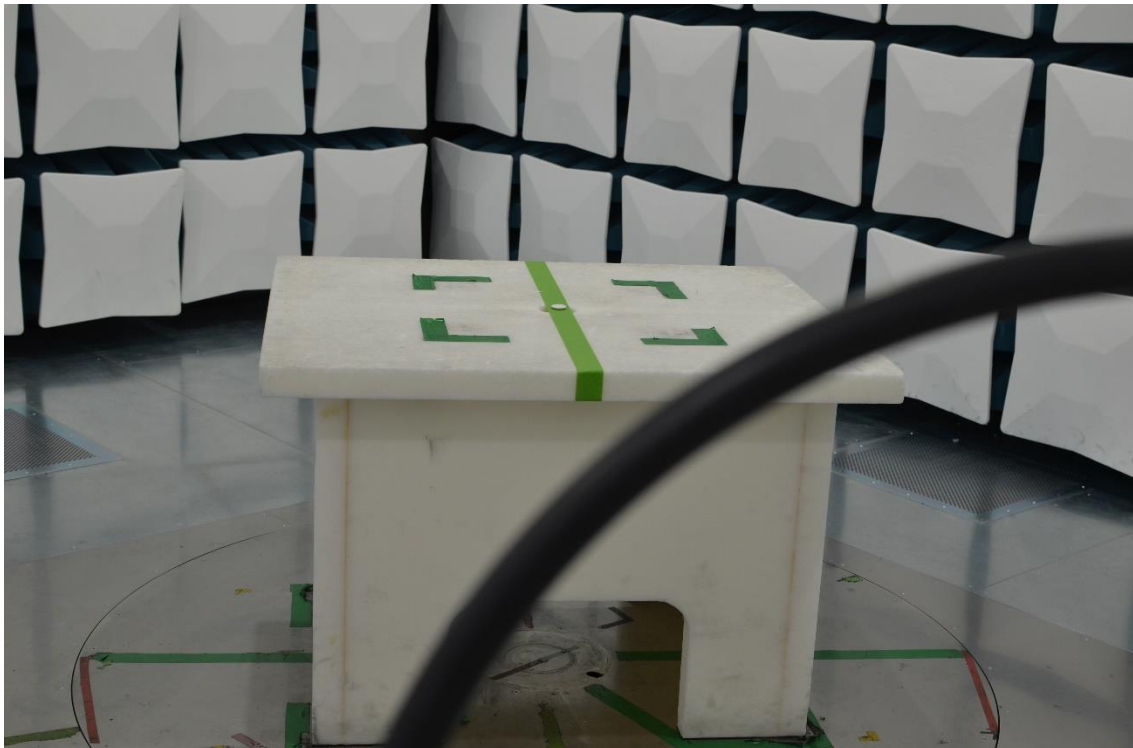
Figure 10: 9kHz-30MHz Test Setup (Front View)
