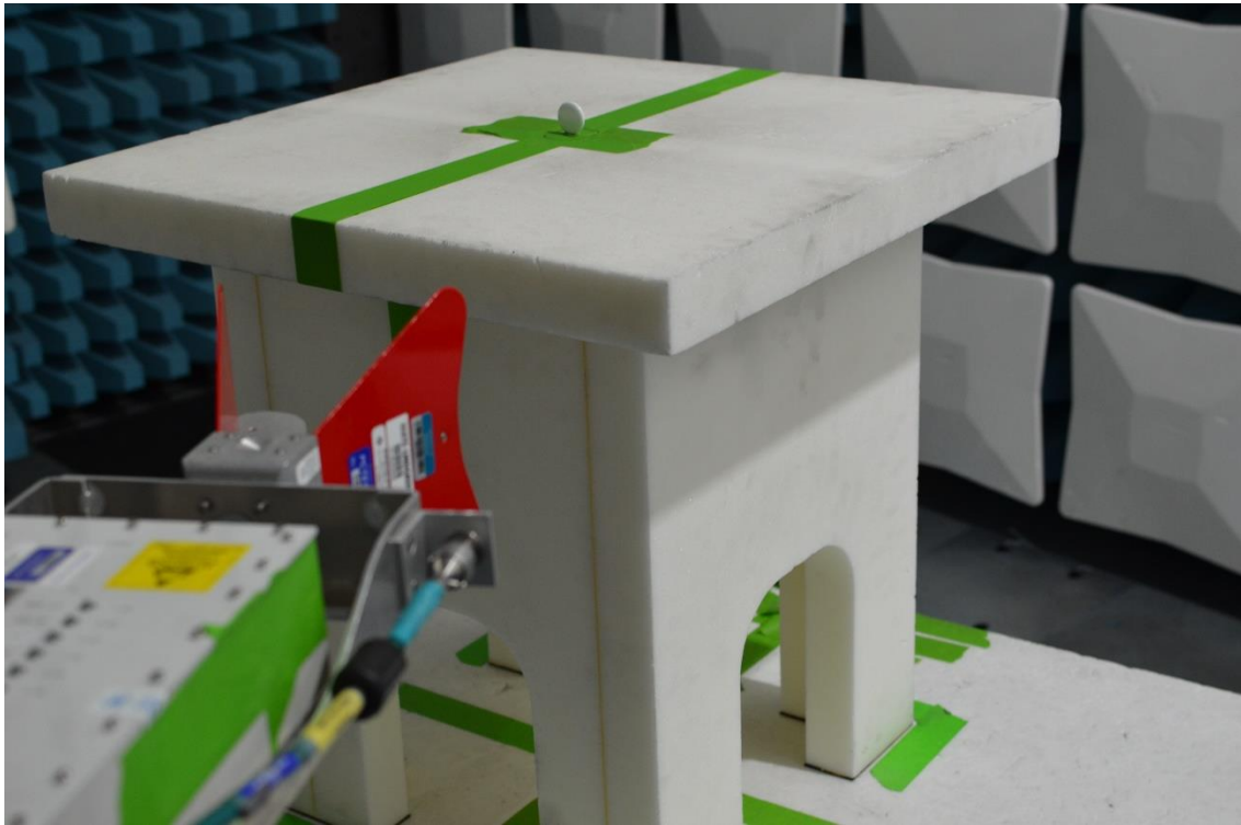
Figure 3: Above 960MHz Test Setup
