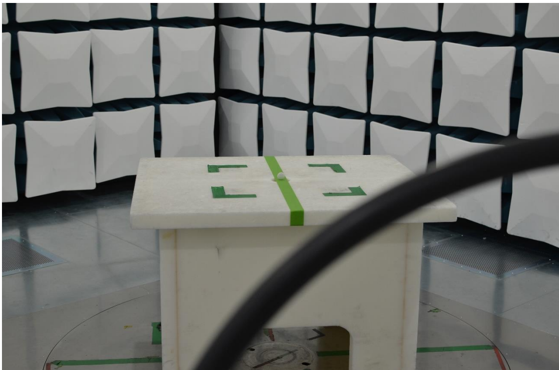
Figure 12: 9kHz-30MHz Test Setup (Front View)
