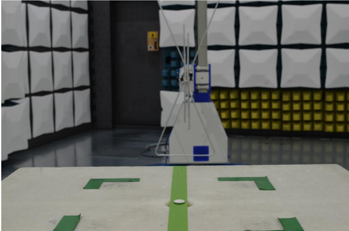
Figure 5: 30MHz-1GHz Test Setup (Rear View)
