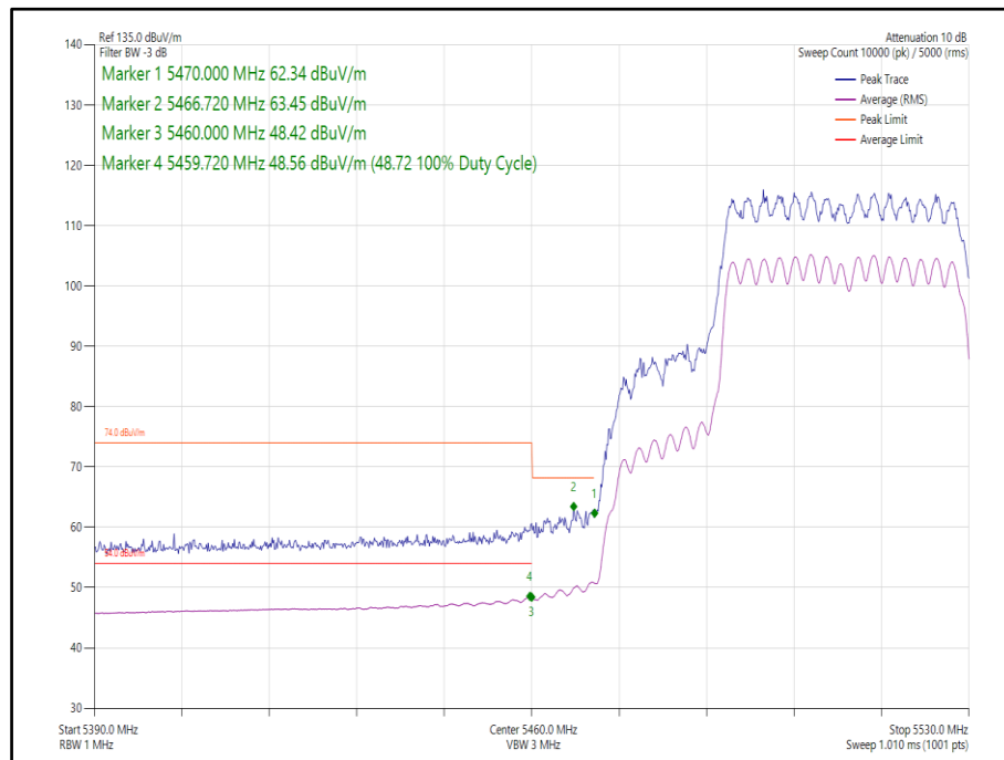
Figure 412 - 802.11ax, HE40, SU, CDD, Core 0-1 - 5510 MHz, Band Edge Frequency 5470 MHz
