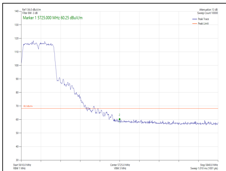
Figure 440 - 802.11n, HT40, SDM, Core 0-1 - 5630 MHz, Band Edge Frequency 5725 MHz
