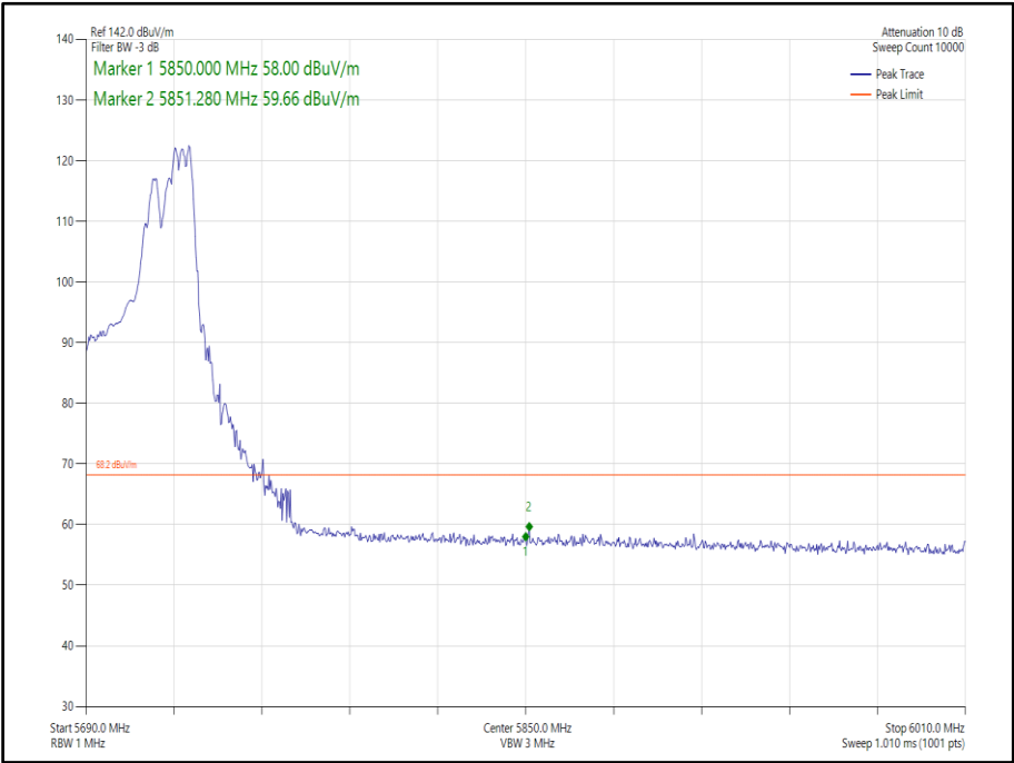
Figure 428 - 802.11ax, HE40, RU 106-56, CDD, Core 0-1 - 5710 MHz, Band Edge Frequency 5850 MHz
