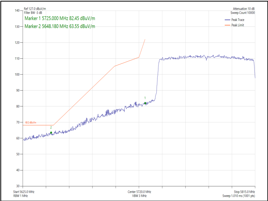
Figure 460 - 802.11ax, HE80, SU, SISO, Core 0 - 5775 MHz, Band Edge Frequency 5725 MHz
