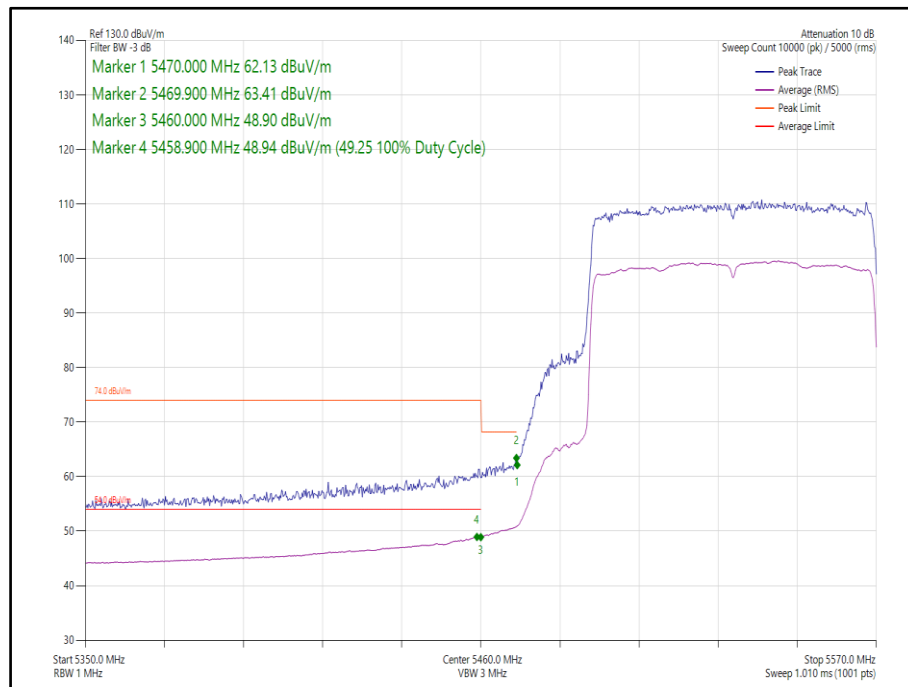
Figure 472 - 802.11ax, HE80, SU, SISO, Core 1 - 5530 MHz, Band Edge Frequency 5470 MHz
