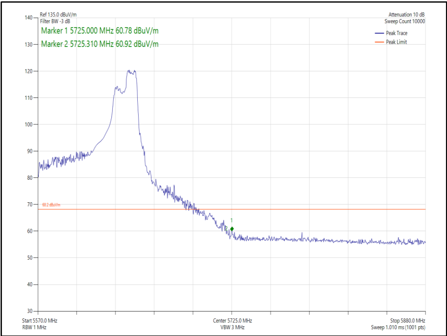
Figure 464 - 802.11ax, HE80, RU 106-60, SISO, Core 0 - 5610 MHz, Band Edge Frequency 5725 MHz
