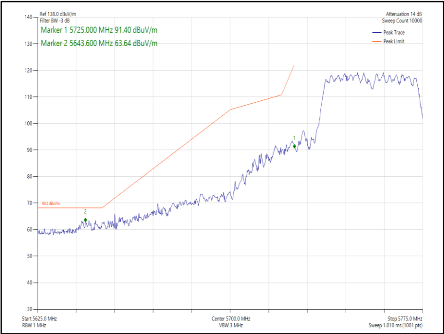
Figure 416 - 802.11n, HT40, CDD, Core 0-1 - 5755 MHz, Band Edge Frequency 5725 MHz
