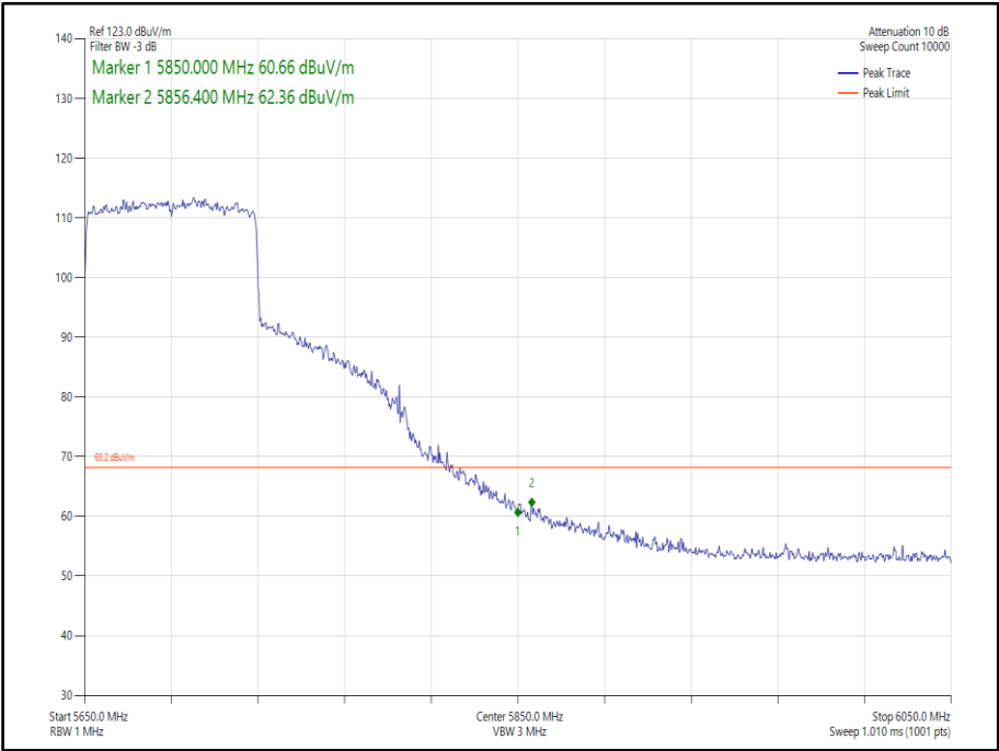
Figure 467 - 802.11ax, HE80, SU, SISO, Core 0 - 5690 MHz, Band Edge Frequency 5850 MHz
