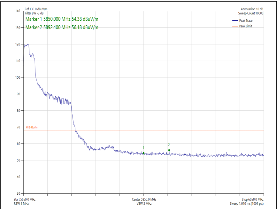
Figure 468 - 802.11ax, HE80, RU 106-53, SISO, Core 0 - 5690 MHz, Band Edge Frequency 5850 MHz
