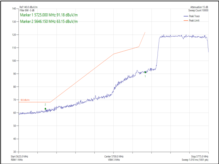
Figure 438 - 802.11ax, HE40, SU, SDM, Core 0-1 - 5755 MHz, Band Edge Frequency 5725 MHz
