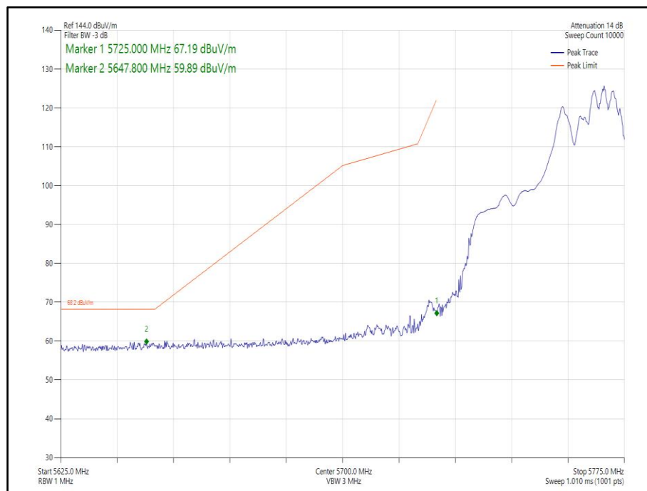
Figure 439 - 802.11ax, HE40, RU 106-56, SDM, Core 0-1 - 5755 MHz, Band Edge Frequency 5725 MHz
