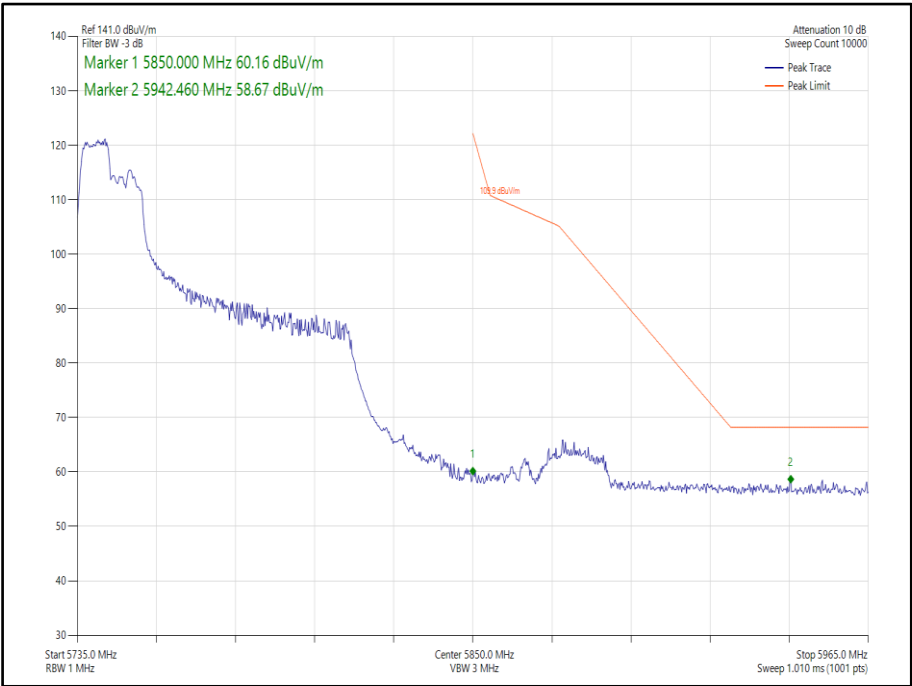
Figure 470 - 802.11ax, HE80, RU 106-53, SISO, Core 0 - 5775 MHz, Band Edge Frequency 5850 MHz
