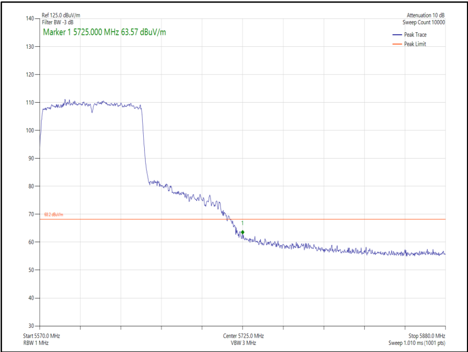
Figure 462 - 802.11ac, VHT80, SISO, Core 0 - 5610 MHz, Band Edge Frequency 5725 MHz
