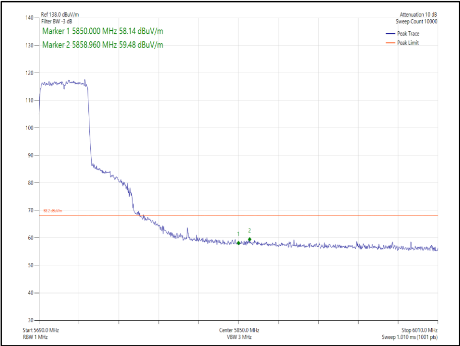
Figure 447 - 802.11ax, HE40, SU, SDM, Core 0-1 - 5710 MHz, Band Edge Frequency 5850 MHz
