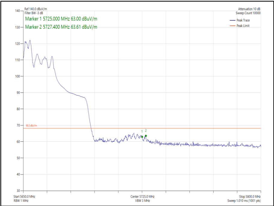
Figure 444 - 802.11ax, HE40, RU 52-37, SDM, Core 0-1 - 5670 MHz, Band Edge Frequency 5725 MHz
