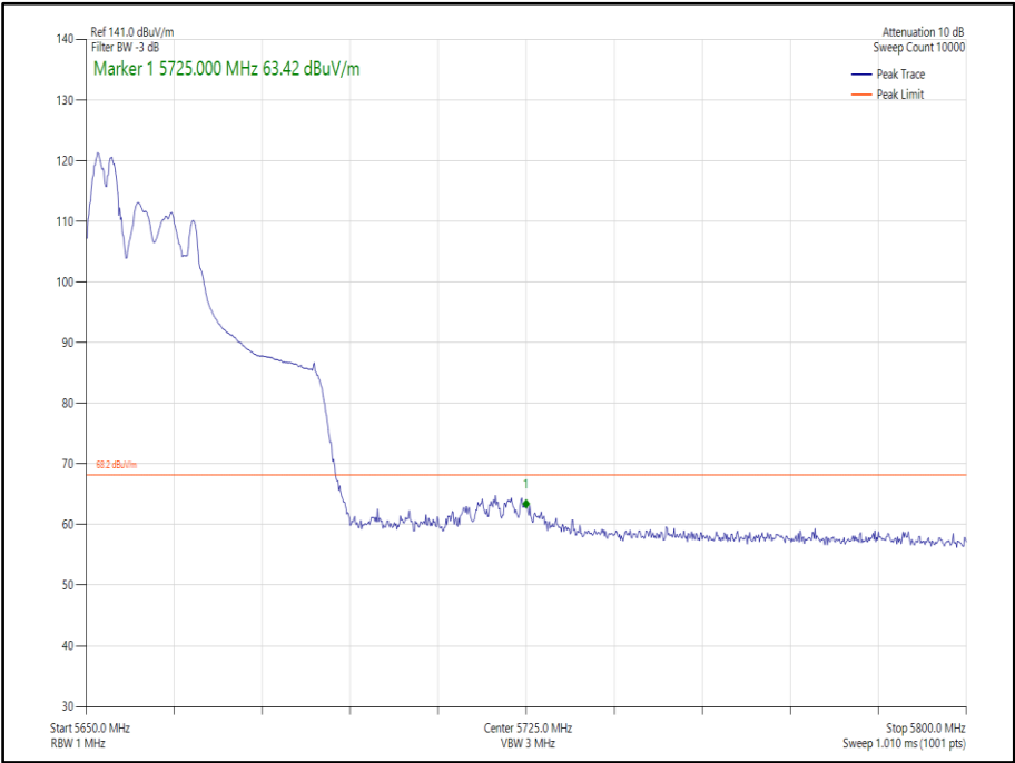
Figure 424 - 802.11ax, HE40, RU 52-37, CDD, Core 0-1 - 5670 MHz, Band Edge Frequency 5725 MHz
