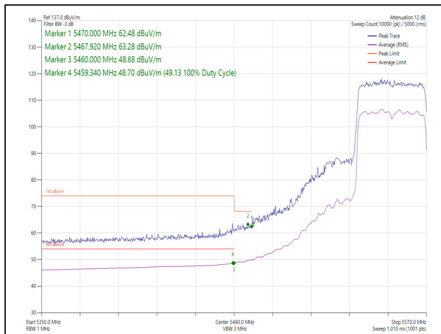
Figure 435 - 802.11ax, HE40, SU, SDM, Core 0-1 - 5550 MHz, Band Edge Frequency 5470 MHz
