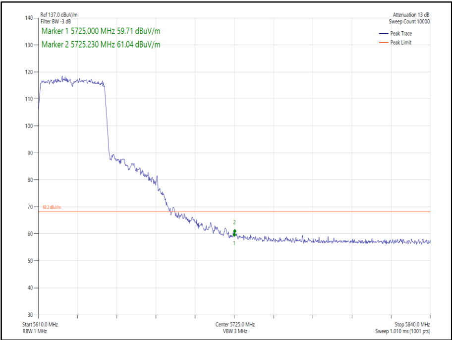
Figure 442 - 802.11ax, HE40, SU SDM, Core 0-1 - 5630 MHz, Band Edge Frequency 5725 MHz
