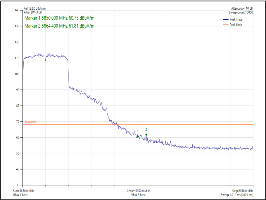
Figure 465 - 802.11ac, VHT80, SISO, Core 0 - 5690 MHz, Band Edge Frequency 5850 MHz
