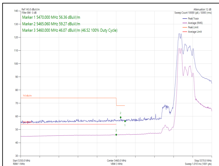
Figure 436 - 802.11ax, HE40, RU 52-37, SDM, Core 0-1 - 5550 MHz, Band Edge Frequency 5470 MHz
