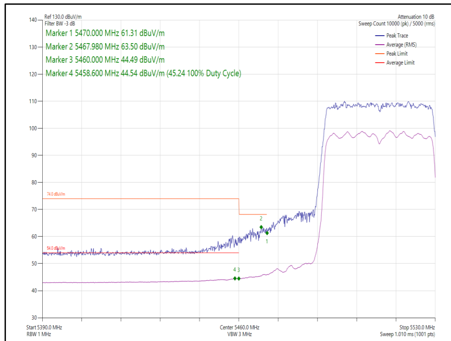
Figure 433 - 802.11ax, HE40, SU, SDM, Core 0-1 - 5510 MHz, Band Edge Frequency 5470 MHz
