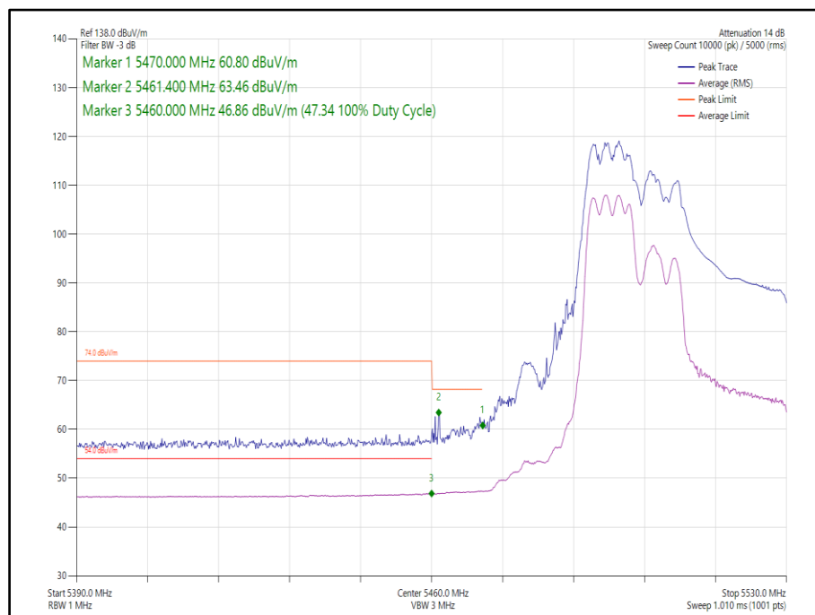
Figure 434 - 802.11ax, HE40, RU 106-53, SDM, Core 0-1 - 5510 MHz, Band Edge Frequency 5470 MHz
