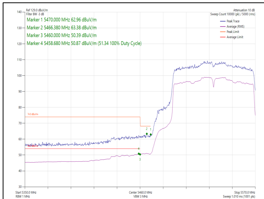
Figure 456 - 802.11ac, VHT80, SISO, Core 0 - 5530 MHz, Band Edge Frequency 5470 MHz
