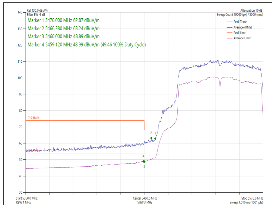
Figure 471 - 802.11ac, VHT80, SISO, Core 1 - 5530 MHz, Band Edge Frequency 5470 MHz
