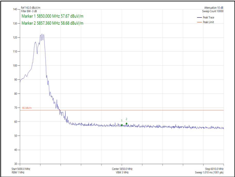
Figure 448 - 802.11ax, HE40, RU 106-56, SDM, Core 0-1 - 5710 MHz, Band Edge Frequency 5850 MHz
