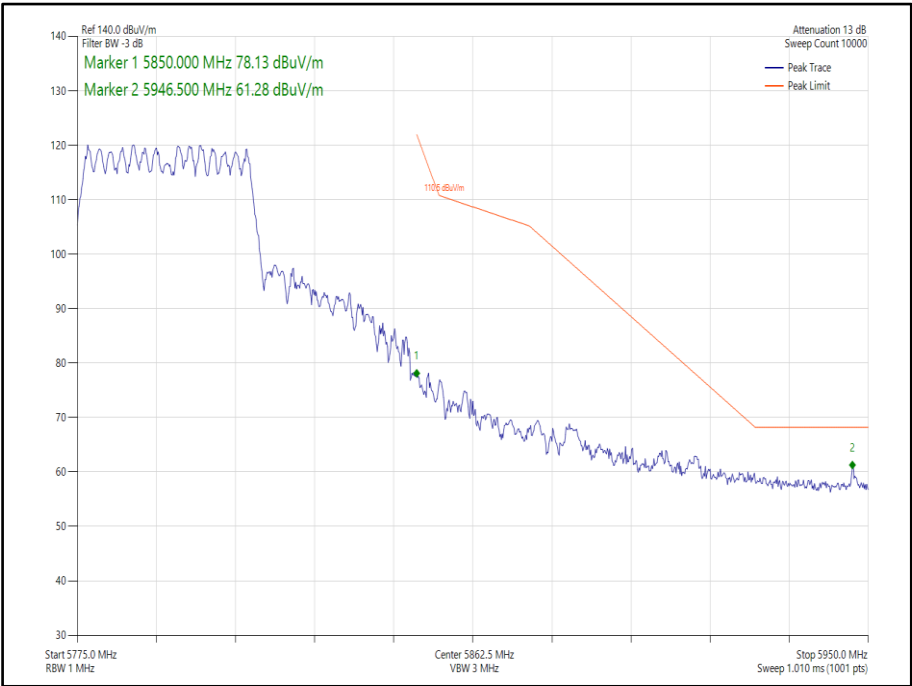
Figure 429 - 802.11ax, HE40, SU, CDD, Core 0-1 - 5795 MHz, Band Edge Frequency 5850 MHz
