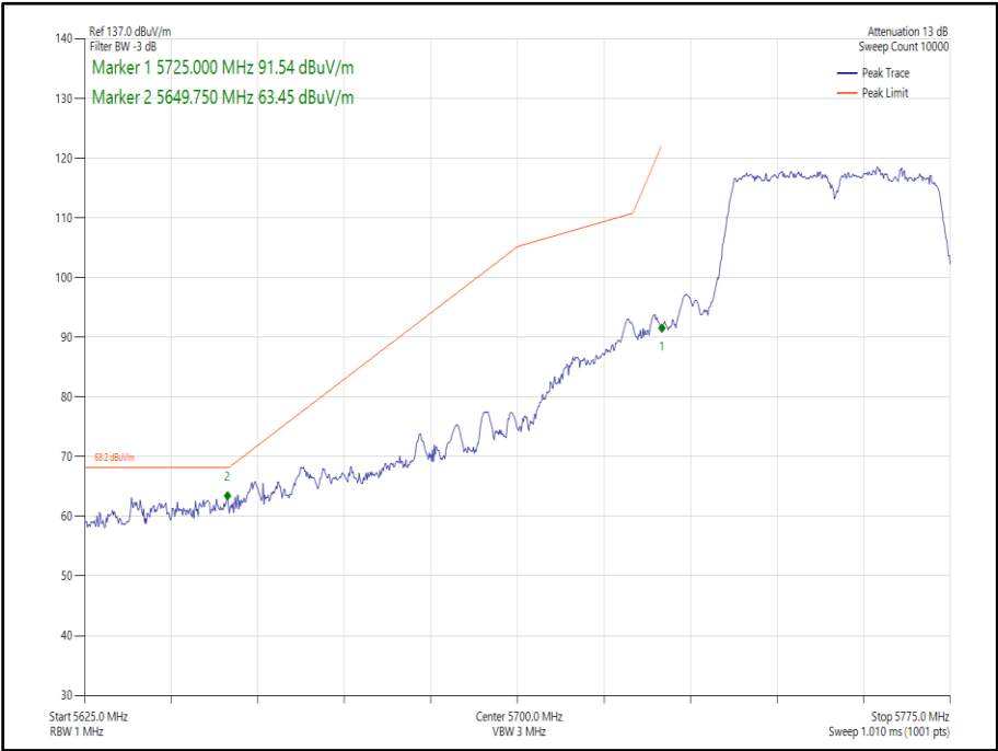
Figure 437 - 802.11n, HT40, SDM, Core 0-1 - 5755 MHz, Band Edge Frequency 5725 MHz
