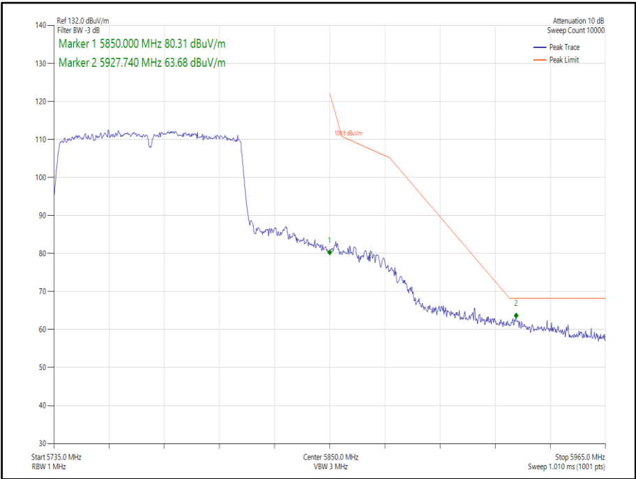
Figure 466 - 802.11ac, VHT80, SISO, Core 0 - 5775 MHz, Band Edge Frequency 5850 MHz
