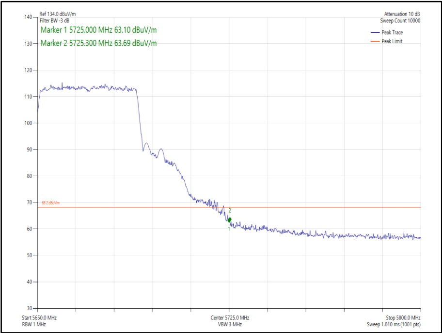
Figure 443 - 802.11ax, HE40, SU, SDM, Core 0-1 - 5670 MHz, Band Edge Frequency 5725 MHz
