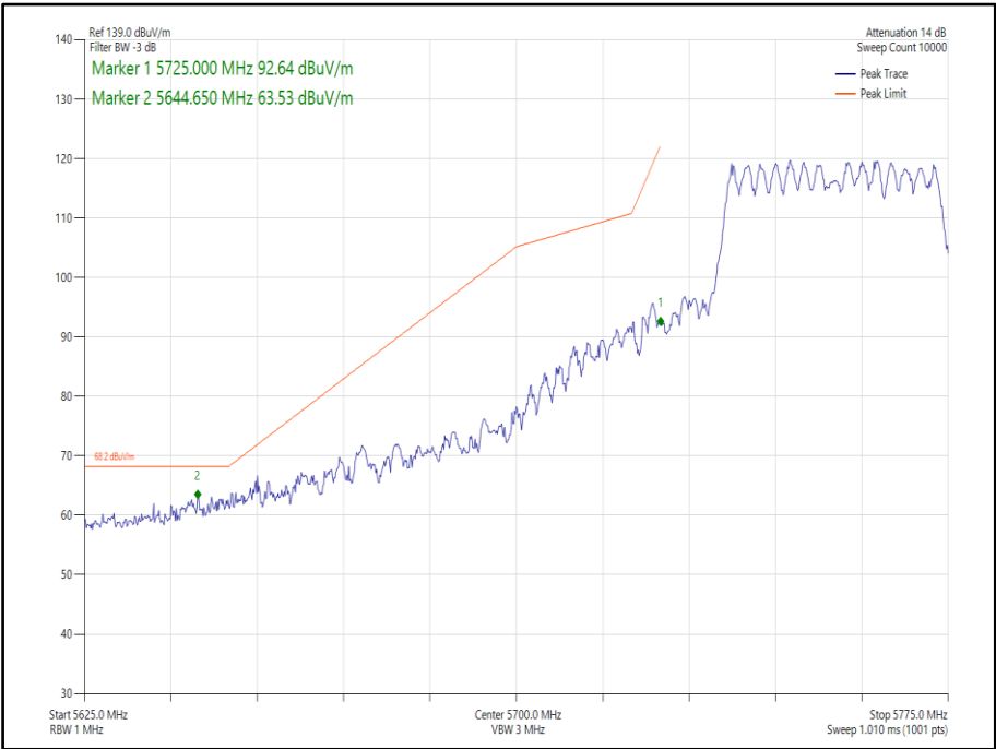
Figure 417 - 802.11ax, HE40, SU, CDD, Core 0-1 - 5755 MHz, Band Edge Frequency 5725 MHz
