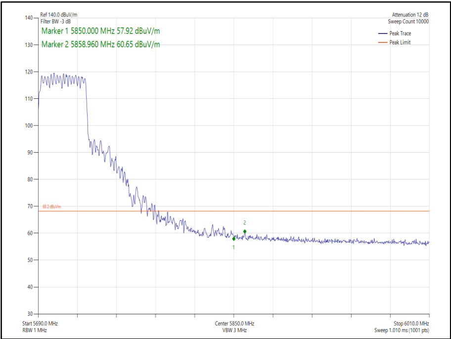
Figure 427 - 802.11ax, HE40, SU, CDD, Core 0-1 - 5710 MHz, Band Edge Frequency 5850 MHz
