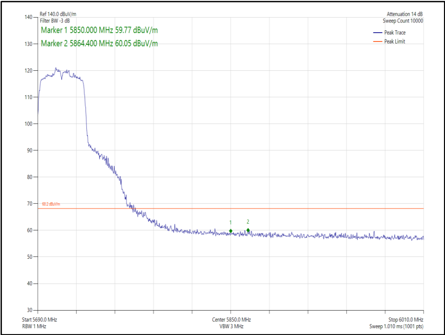
Figure 454 - 802.11ac, VHT40, TxBF, Core 0-1 - 5710 MHz, Band Edge Frequency 5850 MHz
