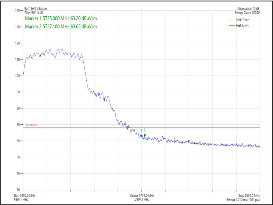
Figure 420 - 802.11n, HT40, CDD, Core 0-1 - 5670 MHz, Band Edge Frequency 5725 MHz
