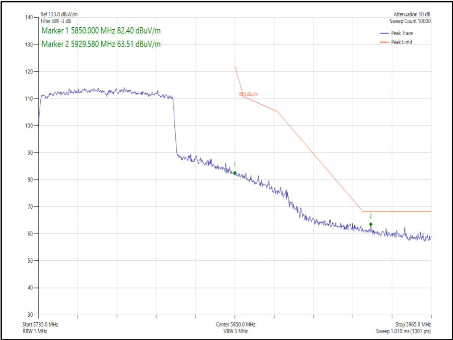
Figure 469 - 802.11ax, HE80, SU, SISO, Core 0 - 5775 MHz, Band Edge Frequency 5850 MHz
