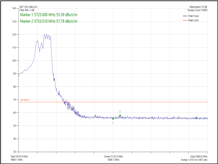
Figure 422 - 802.11ax, HE40, RU 106-56, CDD, Core 0-1 - 5630 MHz, Band Edge Frequency 5725 MHz
