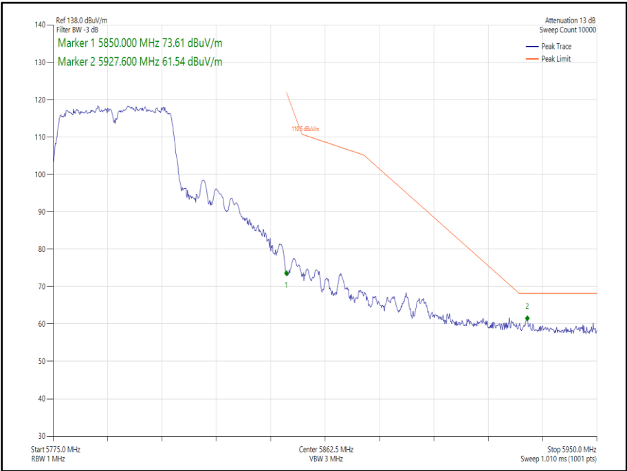
Figure 446 - 802.11n, HT40, SDM, Core 0-1 - 5795 MHz, Band Edge Frequency 5850 MHz
