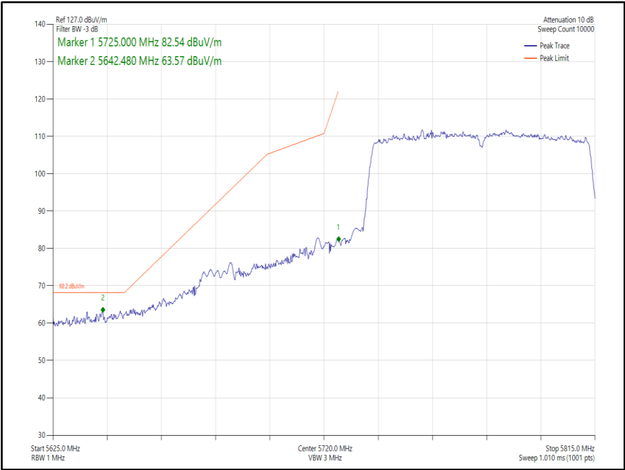
Figure 459 - 802.11ac, VHT80, SISO, Core 0 - 5775 MHz, Band Edge Frequency 5725 MHz
