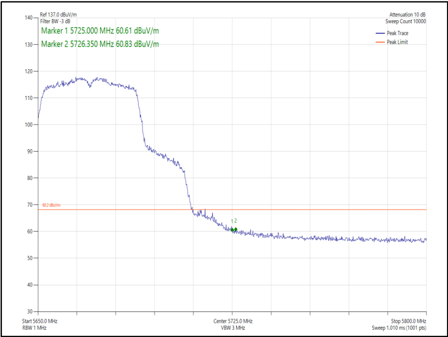
Figure 453 - 802.11ac, VHT40, TxBF, Core 0-1 - 5670 MHz, Band Edge Frequency 5725 MHz
