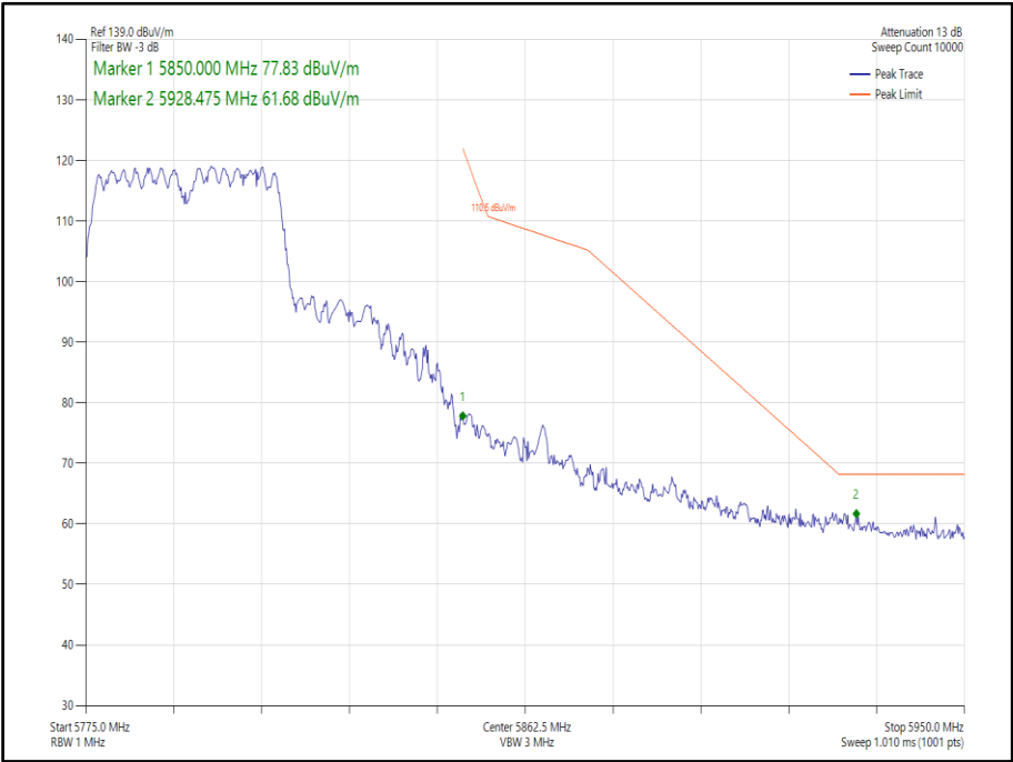
Figure 426 - 802.11n, HT40, CDD, Core 0-1 - 5795 MHz, Band Edge Frequency 5850 MHz
