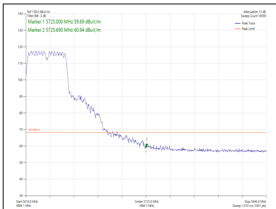
Figure 419 - 802.11n, HT40, CDD, Core 0-1 - 5630 MHz, Band Edge Frequency 5725 MHz
