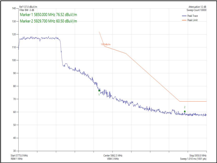
Figure 449 - 802.11ax, HE40, SU, SDM, Core 0-1 - 5795 MHz, Band Edge Frequency 5850 MHz
