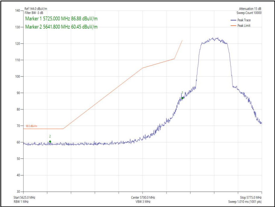
Figure 452 - 802.11ac, VHT40, TxBF, Core 0-1 - 5755 MHz, Band Edge Frequency 5725 MHz
