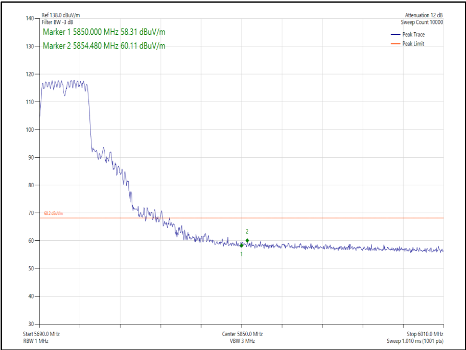
Figure 425 - 802.11n, HT40, CDD, Core 0-1 - 5710 MHz, Band Edge Frequency 5850 MHz
