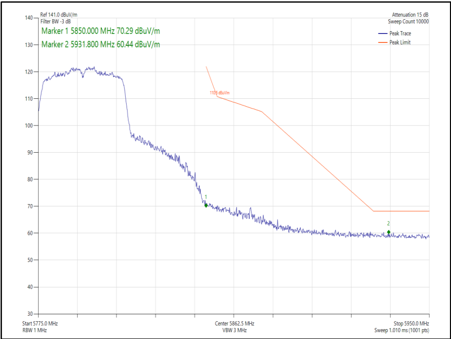
Figure 455 - 802.11ac, VHT40, TxBF, Core 0-1 - 5795 MHz, Band Edge Frequency 5850 MHz
