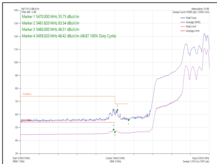
Figure 413 - 802.11ax, HE40, RU 52-44, CDD, Core 0-1 - 5510 MHz, Band Edge Frequency 5470 MHz
