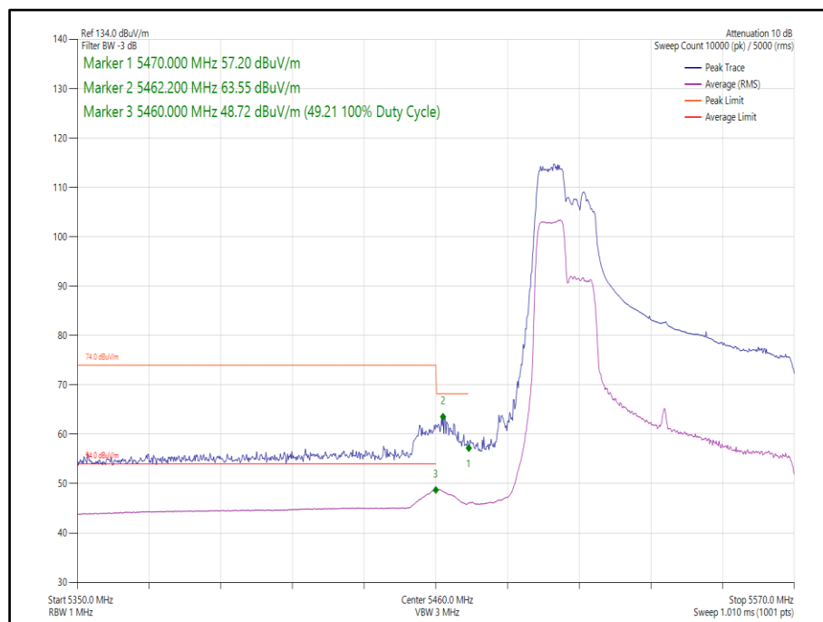
Figure 473 - 802.11ax, HE80, RU 106-53, SISO, Core 1 - 5530 MHz, Band Edge Frequency 5470 MHz
