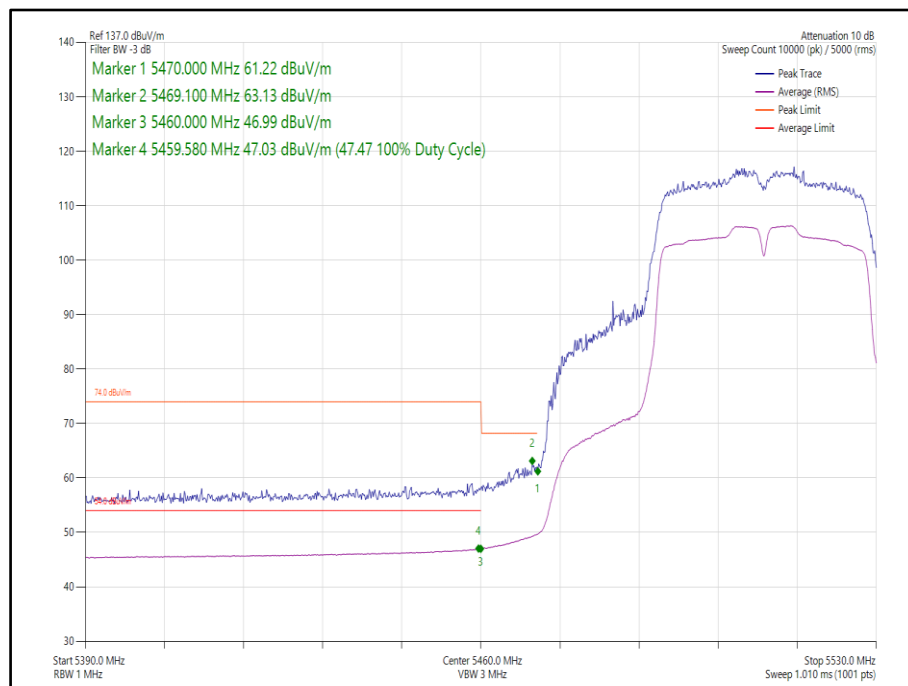
Figure 451 - 802.11ac, VHT40, TxBF, Core 0-1 - 5510 MHz, Band Edge Frequency 5470 MHz
