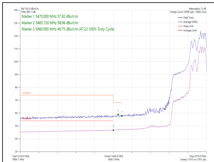
Figure 415 - 802.11ax, HE40, RU 106-56, CDD, Core 0-1 - 5550 MHz, Band Edge Frequency 5470 MHz
