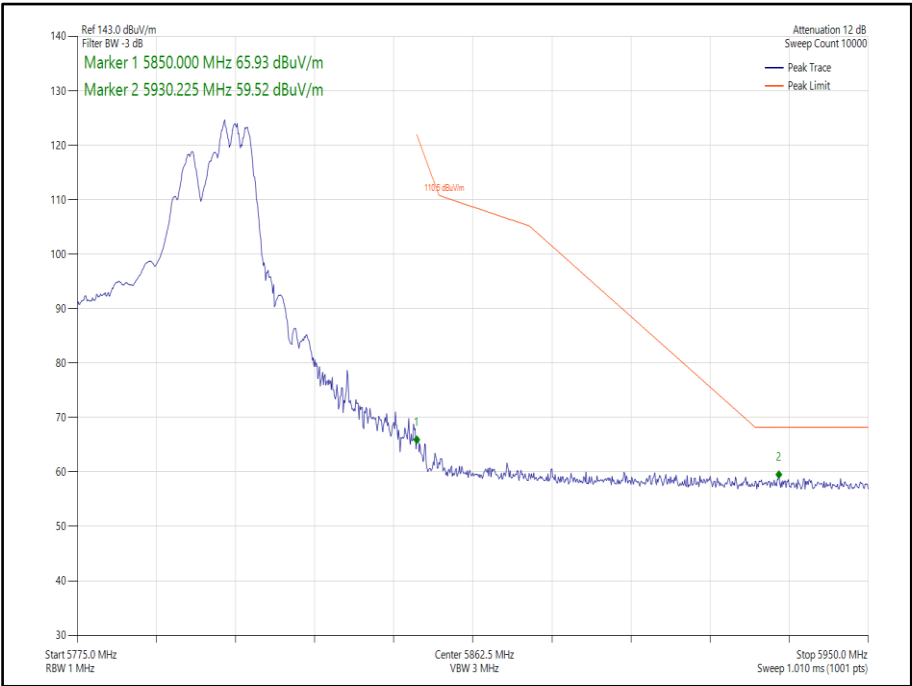
Figure 450 - 802.11ax, HE40, RU 106-56, SDM, Core 0-1 - 5795 MHz, Band Edge Frequency 5850 MHz
