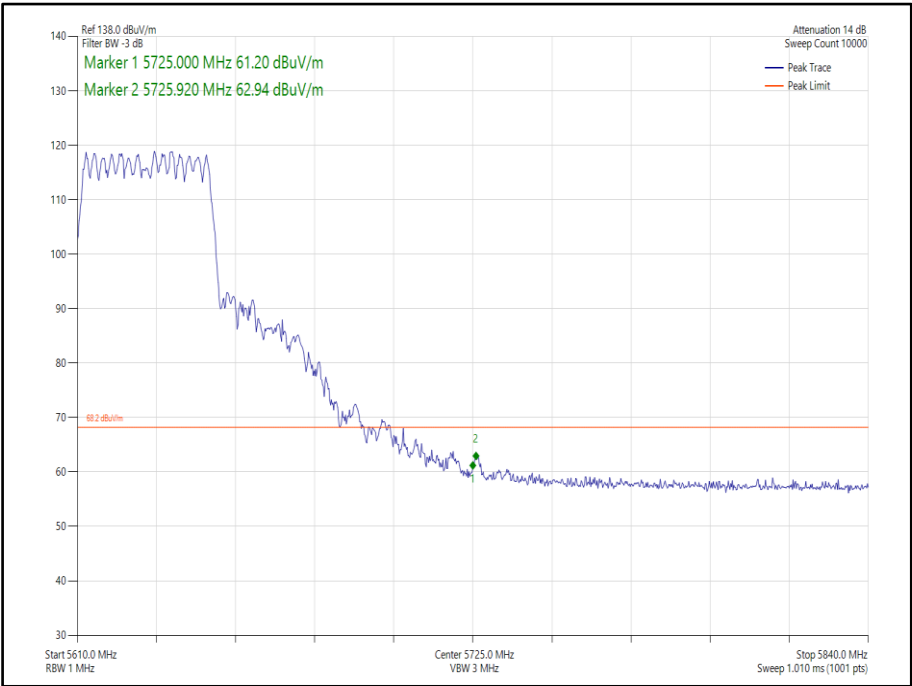
Figure 421 - 802.11ax, HE40, SU, CDD, Core 0-1 - 5630 MHz, Band Edge Frequency 5725 MHz
