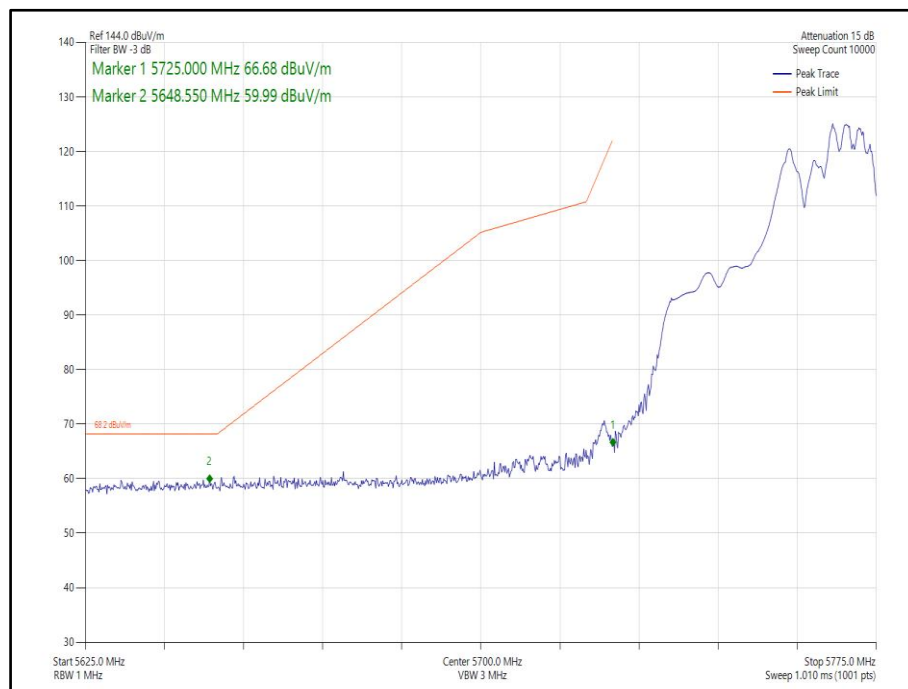
Figure 418 - 802.11ax, HE40, RU 106-56, CDD, Core 0-1 - 5755 MHz, Band Edge Frequency 5725 MHz
