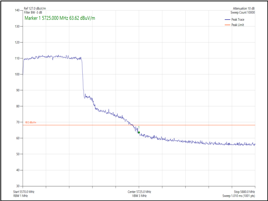
Figure 463 - 802.11ax, HE80, SU, SISO, Core 0 - 5610 MHz, Band Edge Frequency 5725 MHz
