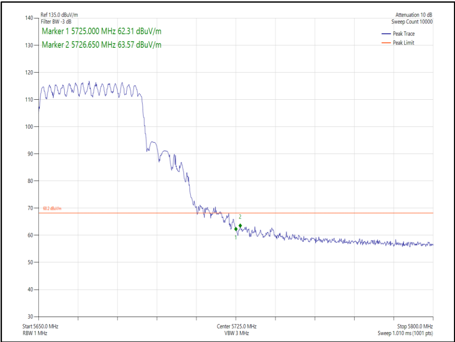
Figure 423 - 802.11ax, HE40, SU, CDD, Core 0-1 - 5670 MHz, Band Edge Frequency 5725 MHz
