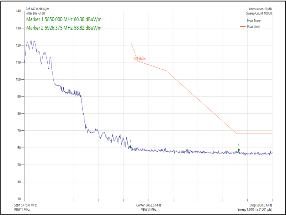
Figure 430 - 802.11ax, HE40, RU 106-53, CDD, Core 0-1 - 5795 MHz, Band Edge Frequency 5850 MHz
