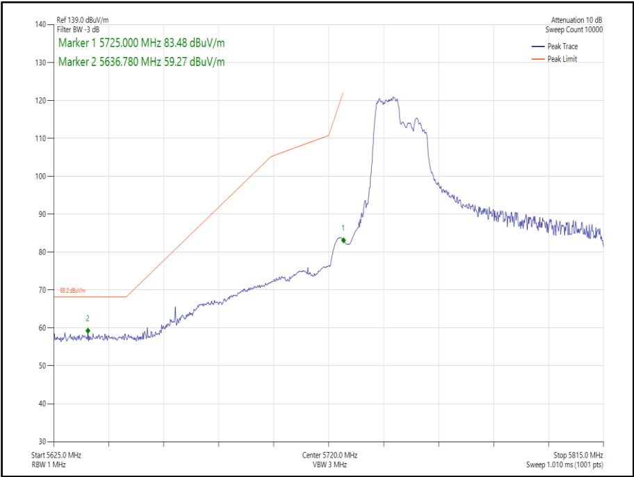
Figure 461 - 802.11ax, HE80, RU 106-53, SISO, Core 0 - 5775 MHz, Band Edge Frequency 5725 MHz
