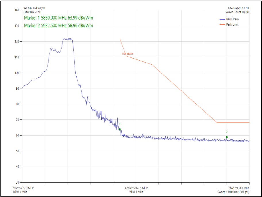
Figure 409 - 802.11ax, HE40, RU 106-56, SISO, Core 1 - 5795 MHz, Band Edge Frequency 5850 MHz
