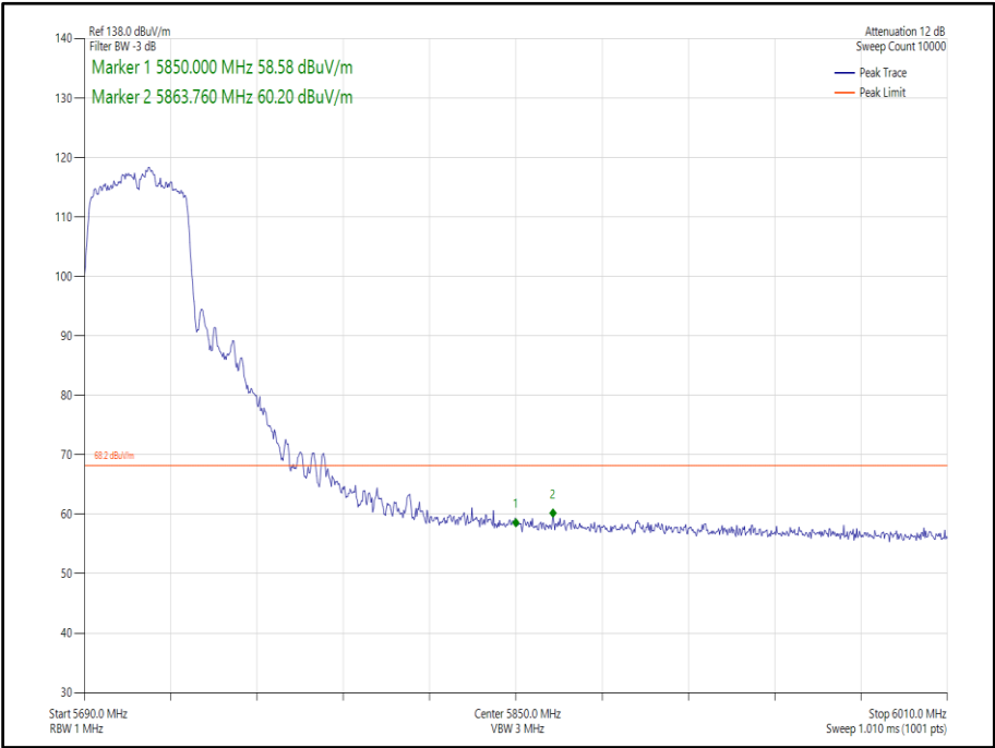
Figure 445 - 802.11n, HT40, SDM, Core 0-1 - 5710 MHz, Band Edge Frequency 5850 MHz
