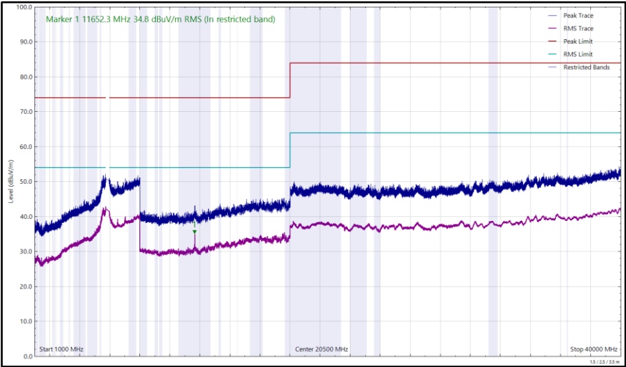
Figure 553 - U-NII-3 - 5825 MHz (CH165), 802.11a, Core 1, 1 GHz to 40 GHz, Vertical
