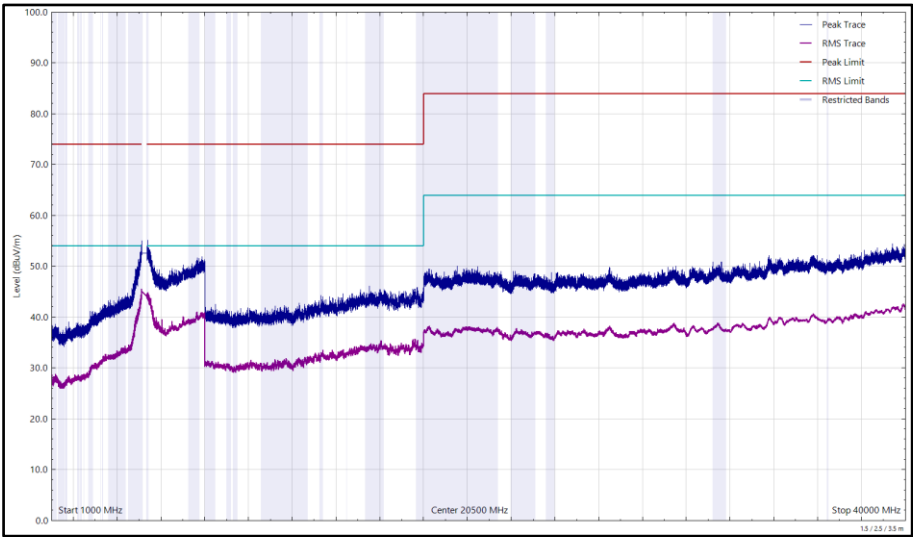
Figure 557 - U-NII-1 - 5180 MHz (CH36), HE20, RU26-0, CDD, Core 0 + Core 1, 1 GHz to 40 GHz, Vertical
