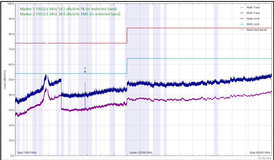
Figure 569 - U-NII-3 - 5825 MHz (CH165), HE20, RU26-0, CDD, Core 0 + Core 1, 1 GHz to 40 GHz, Vertical
