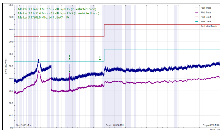
Figure 565 - U-NII-3 - 5745 MHz (CH149), HE20, RU26-0, CDD, Core 0 + Core 1, 1 GHz to 40 GHz, Vertical
