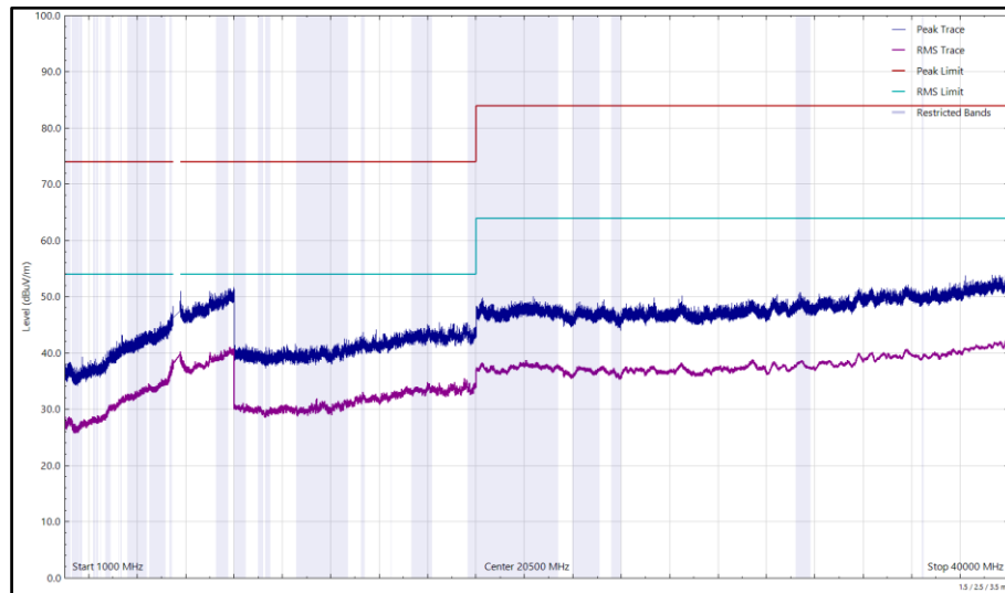
Figure 578 - U-NII-2C - 5700 MHz (CH140), VHT20, CDD, Core 0 + Core 1, 1 GHz to 40 GHz, Horizontal
