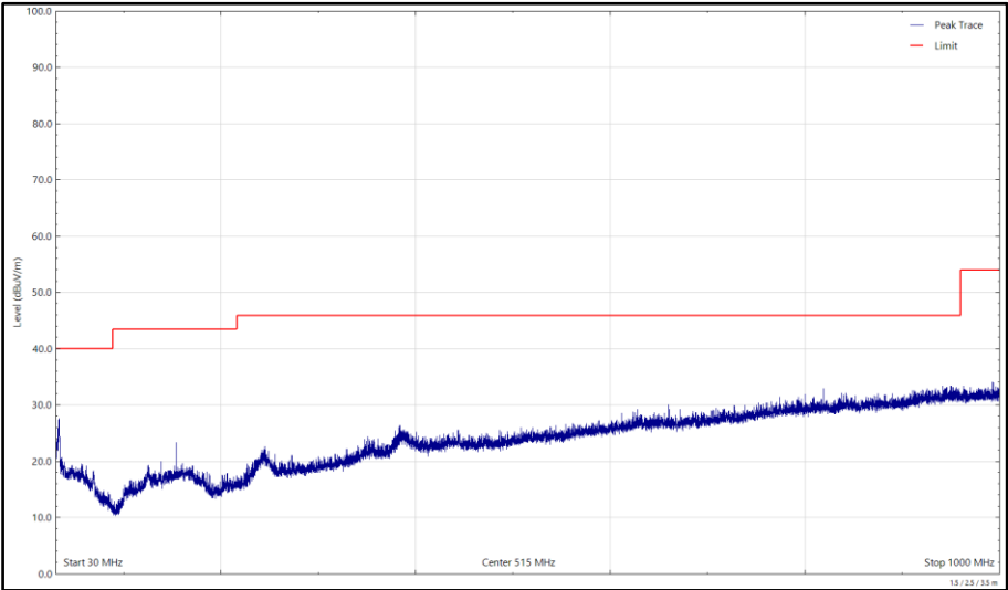
Figure 568 - U-NII-3 - 5825 MHz (CH165), HE20, RU26-0, CDD, Core 0 + Core 1, 30 MHz to 1 GHz, Vertical (Peak)
