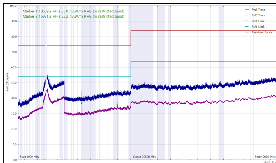
Figure 575 - U-NII-2A - 5320 MHz (CH64), VHT20, CDD, Core 0 + Core 1, 1 GHz to 40 GHz, Vertical
