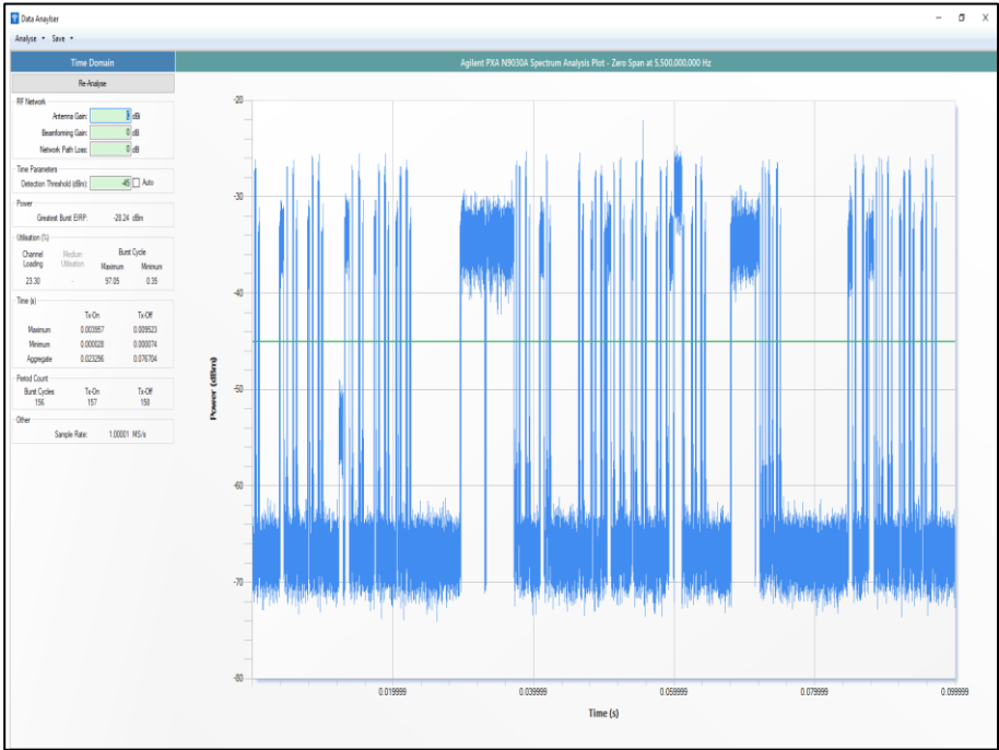
Figure 594 - Channel Loading
