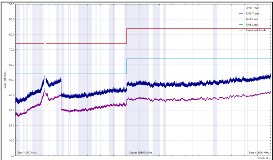
Figure 577 - U-NII-2C - 5500 MHz (CH100), VHT20, CDD, Core 0 + Core 1, 1 GHz to 40 GHz, Vertical
