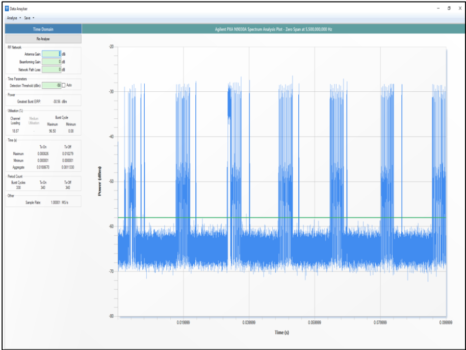
Figure 588 - Channel Loading
