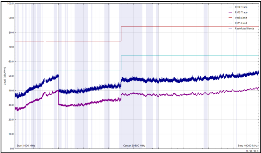
Figure 551 - U-NII-3 - 5825 MHz (CH165), 802.11a, Core 1, 1 GHz to 40 GHz, Horizontal
