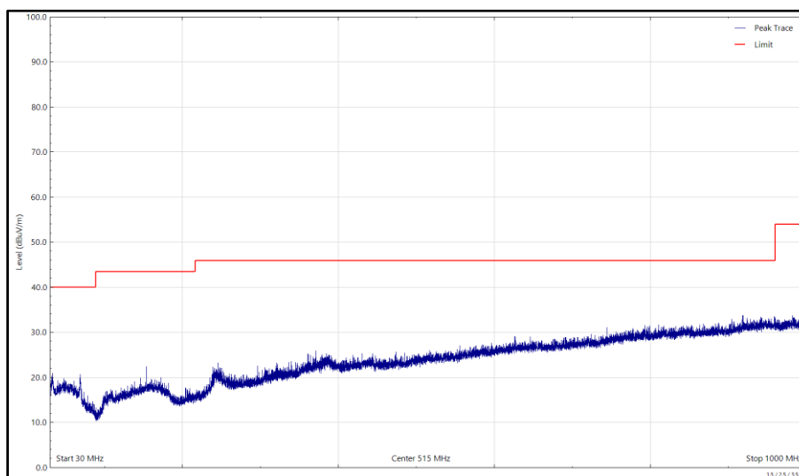
Figure 582 - U-NII-3 - 5825 MHz (CH165), VHT20, CDD, Core 0 + Core 1, 30 MHz to 1 GHz, Horizontal (Peak)
