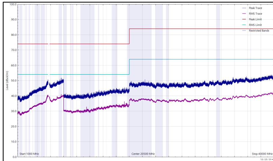
Figure 580 - U-NII-3 - 5745 MHz (CH149), VHT20, CDD, Core 0 + Core 1, 1 GHz to 40 GHz, Horizontal
