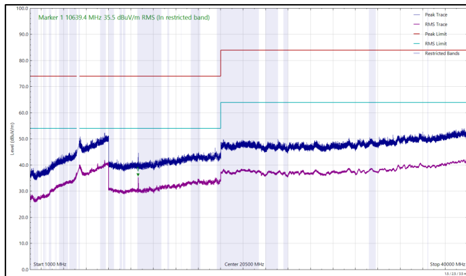
Figure 574 - U-NII-2A - 5320 MHz (CH64), VHT20, CDD, Core 0 + Core 1, 1 GHz to 40 GHz, Horizontal
