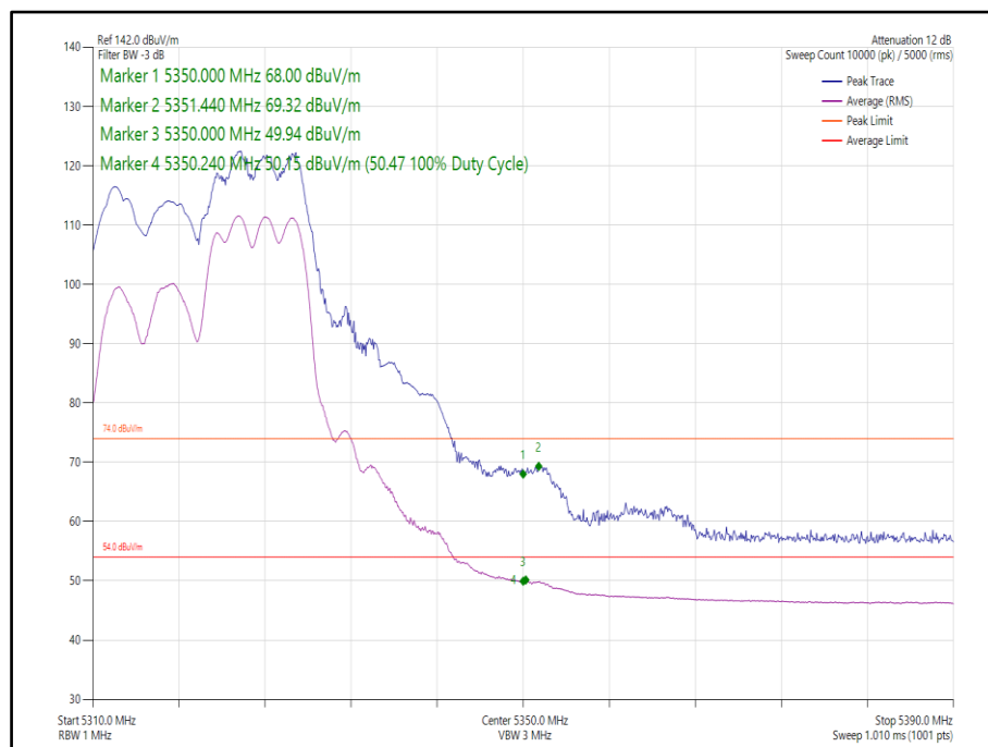
Figure 53 - 802.11ax, HE20, RU 106-54, CDD, Core 0-1 - 5320 MHz, Band Edge Frequency 5350 MHz
