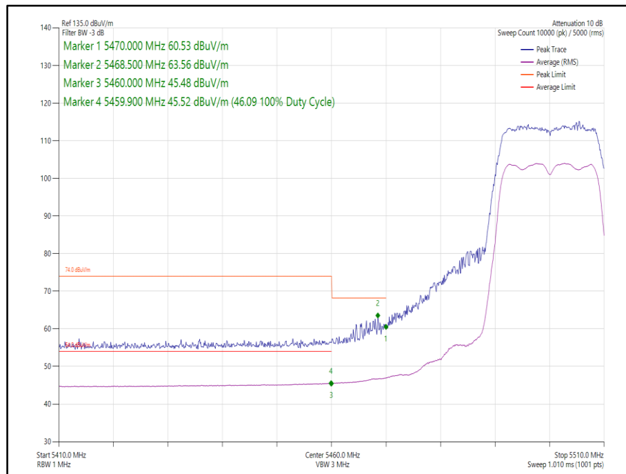
Figure 70 - 802.11n, HT20, SDM, Core 0-1 - 5500 MHz, Band Edge Frequency 5460 MHz
