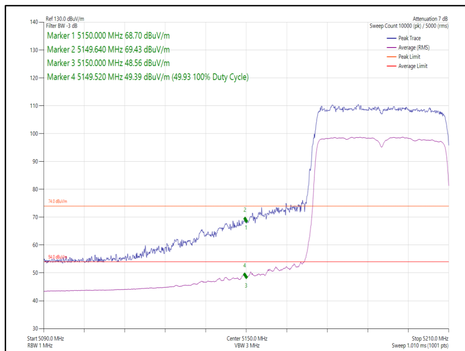
Figure 97 - 802.11ax, HE40, SU, SISO, Core 1 - 5190 MHz, Band Edge Frequency 5150 MHz
