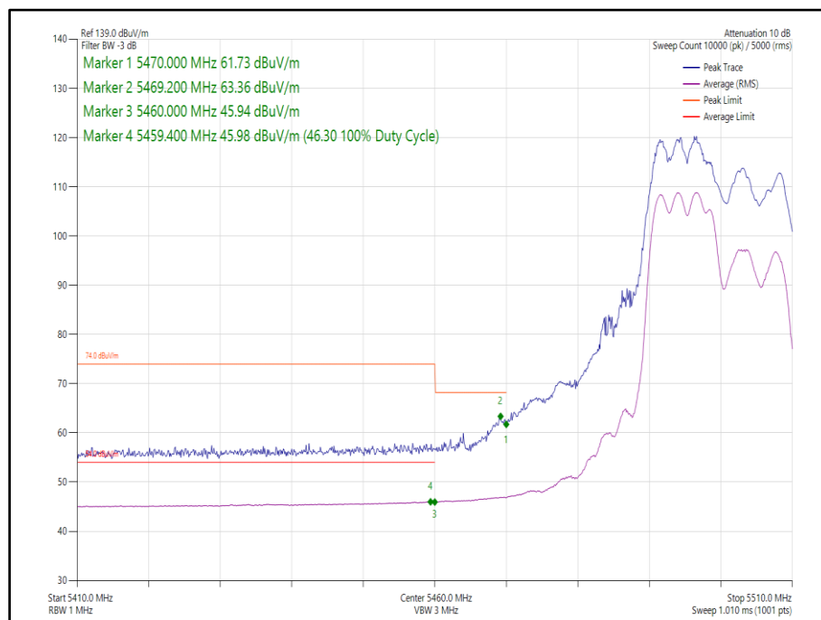
Figure 57 - 802.11ax, HE20, RU 106-53, CDD, Core 0-1 - 5500 MHz, Band Edge Frequency 5460 MHz
