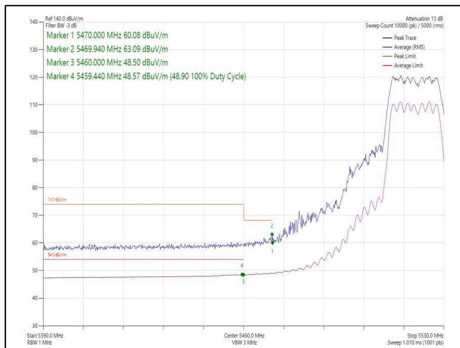
Figure 55 - 802.11n, HT20, CDD, Core 0-1 - 5520 MHz, Band Edge Frequency 5460 MHz
