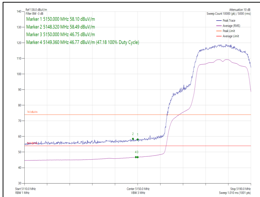
Figure 75 - 802.11ac, VHT20, TxBF, Core 0-1 - 5180 MHz, Band Edge Frequency 5150 MHz
