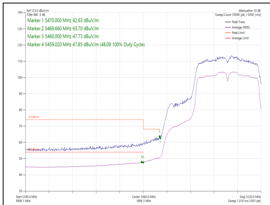
Figure 89 - 802.11n, HT40, SISO, Core 0 - 5510 MHz, Band Edge Frequency 5460 MHz
