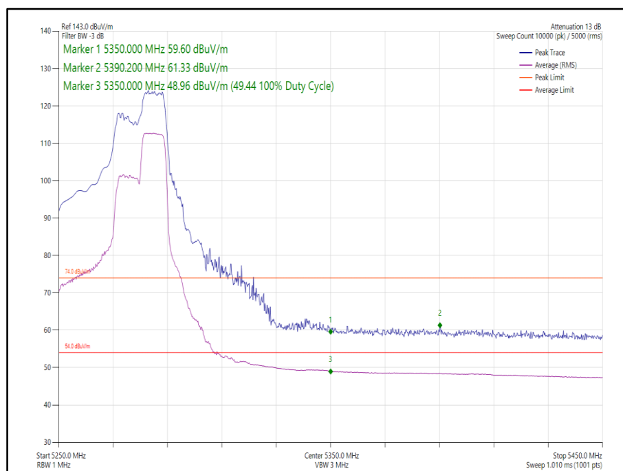
Figure 86 - 802.11ax, HE40, RU 106-56, SISO, Core 0 - 5270 MHz, Band Edge Frequency 5350 MHz
