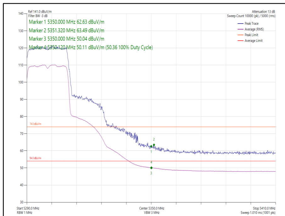
Figure 67 - 802.11ax, HE20, SU, SDM, Core 0-1 - 5300 MHz, Band Edge Frequency 5350 MHz
