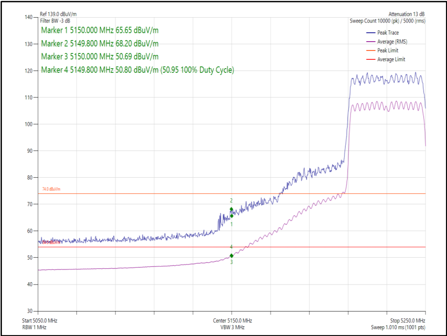
Figure 116 - 802.11ax, HE40, SU, CDD, Core 0-1 - 5230 MHz, Band Edge Frequency 5150 MHz
