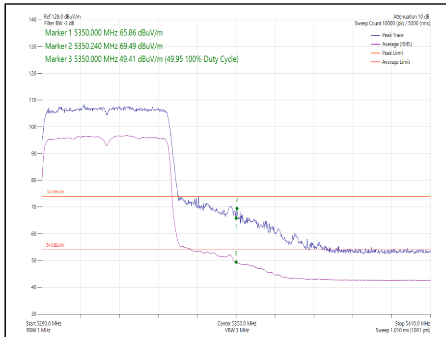
Figure 104 - 802.11ax, HE40, SU, SISO, Core 1 - 5310 MHz, Band Edge Frequency 5350 MHz
