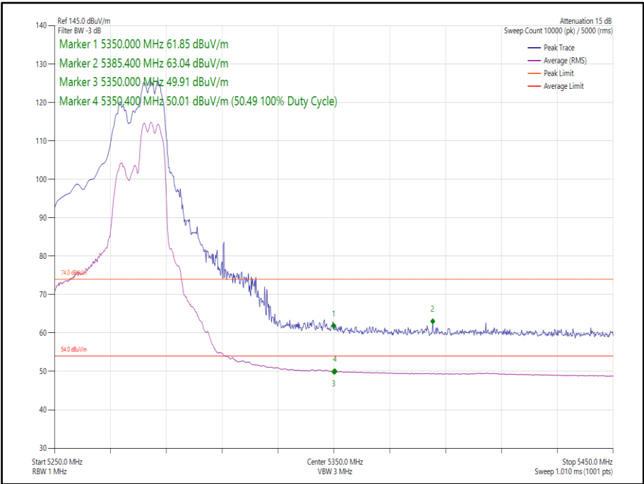
Figure 121 - 802.11ax, HE40, RU 106-56, CDD, Core 0-1 - 5270 MHz, Band Edge Frequency 5350 MHz
