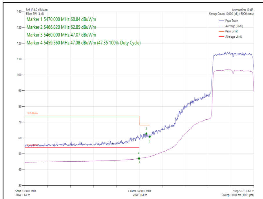
Figure 110 - 802.11ax, HE40, SU, SISO, Core 1 - 5550 MHz, Band Edge Frequency 5460 MHz
