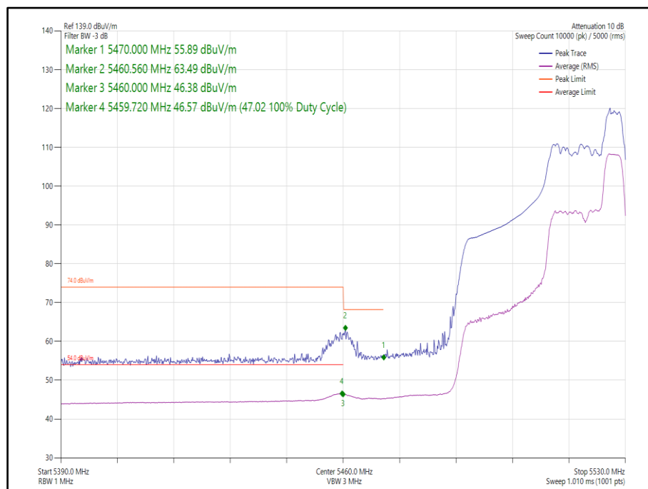
Figure 109 - 802.11ax, HE40, RU 52-44, SISO, Core 1 - 5510 MHz, Band Edge Frequency 5460 MHz
