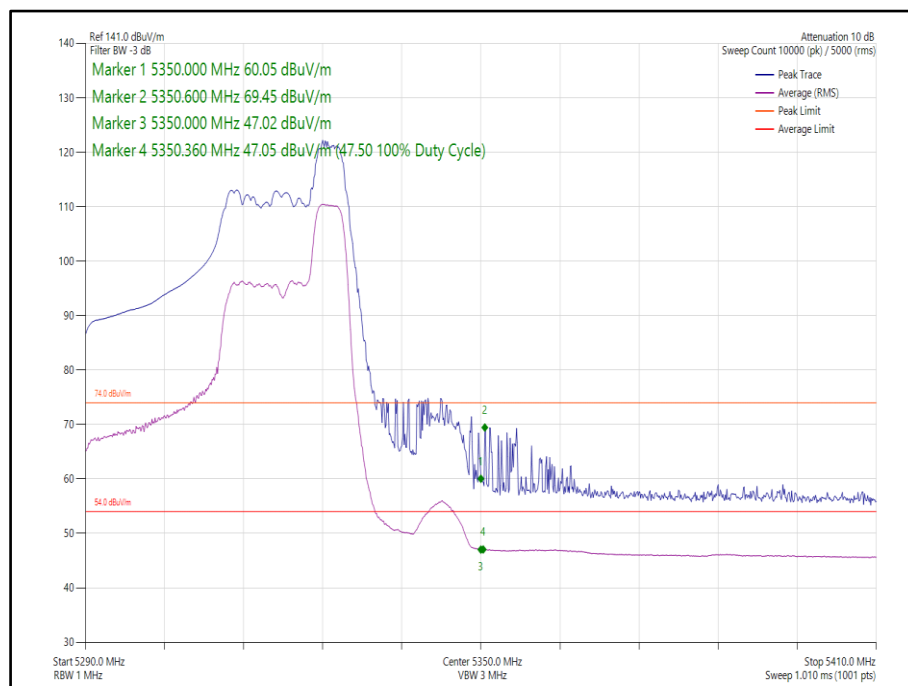
Figure 105 - 802.11ax, HE40, RU 52-44, SISO, Core 1 - 5310 MHz, Band Edge Frequency 5350 MHz
