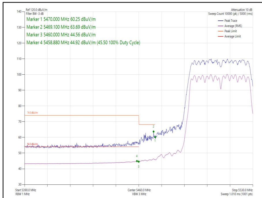
Figure 124 - 802.11n, HT40, CDD, Core 0-1 - 5510 MHz, Band Edge Frequency 5460 MHz
