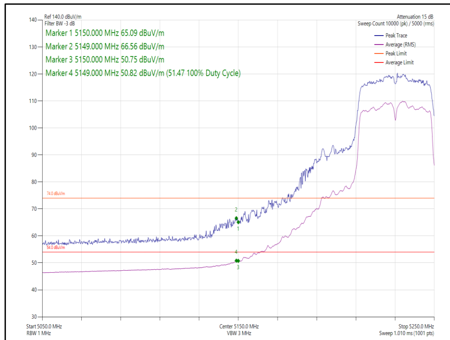
Figure 131 - 802.11n, HT40, SDM, Core 0-1 - 5230 MHz, Band Edge Frequency 5150 MHz
