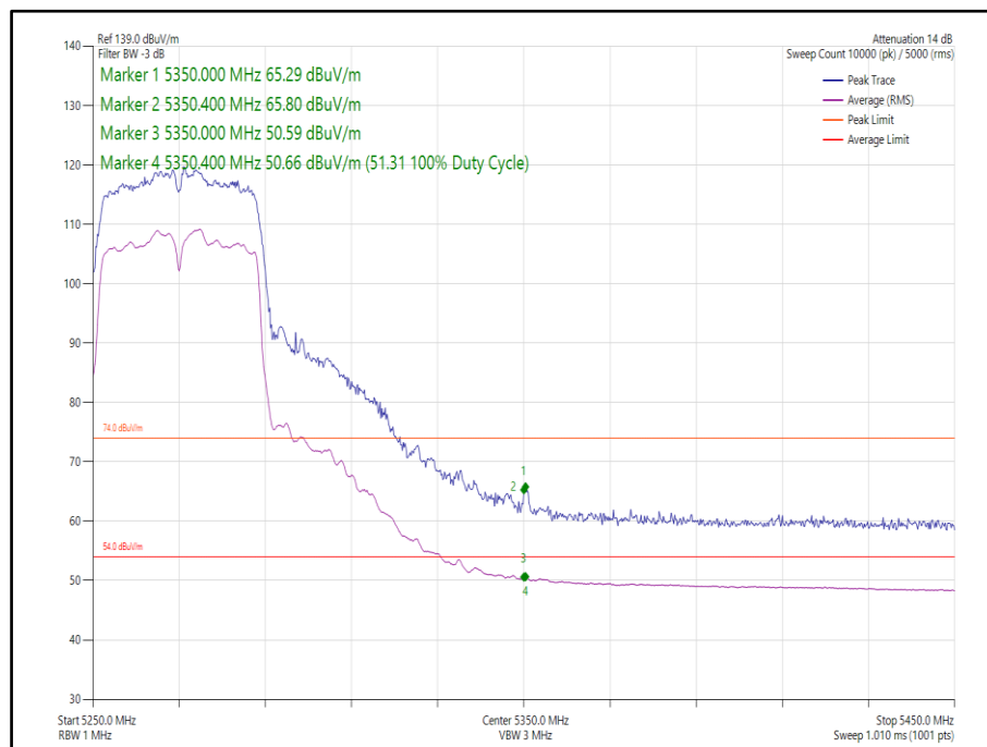
Figure 135 - 802.11n HT40, SDM, Core 0-1 - 5270 MHz, Band Edge Frequency 5350 MHz
