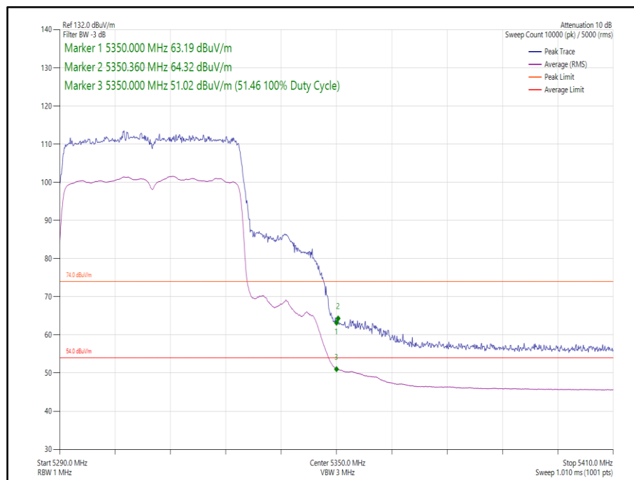
Figure 139 - 802.11ax, HE40, SU, SDM, Core 0-1 - 5310 MHz, Band Edge Frequency 5350 MHz
