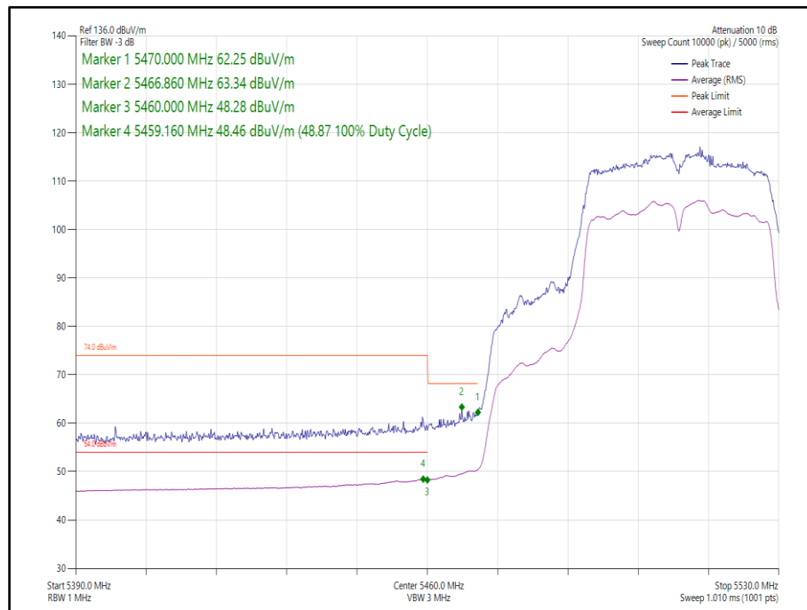
Figure 141 - 802.11n, HT40, SDM, Core 0-1 - 5510 MHz, Band Edge Frequency 5460 MHz
