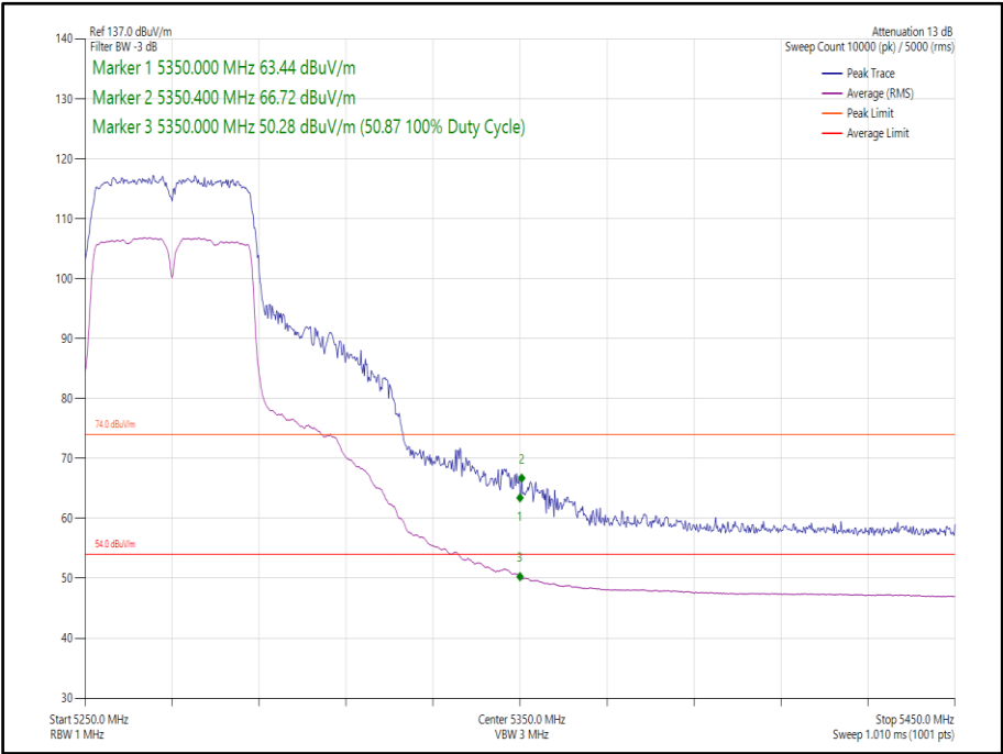
Figure 100 - 802.11n, HT40, SISO, Core 1 - 5270 MHz, Band Edge Frequency 5350 MHz
