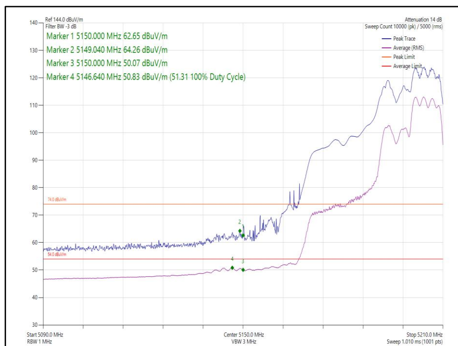
Figure 115 - 802.11ax, HE40, RU 106-56, CDD, Core 0-1 - 5190 MHz, Band Edge Frequency 5150 MHz
