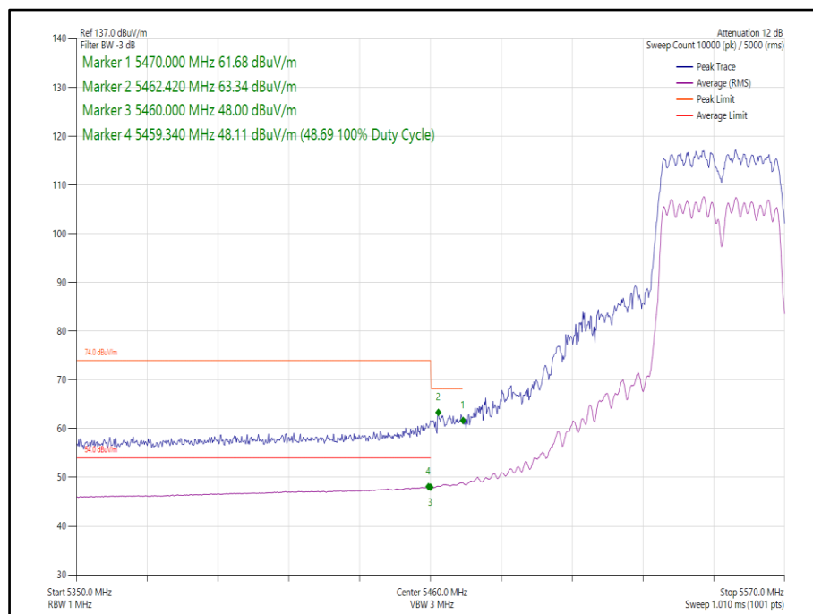
Figure 125 - 802.11n, HT40, CDD, Core 0-1 - 5550 MHz, Band Edge Frequency 5460 MHz
