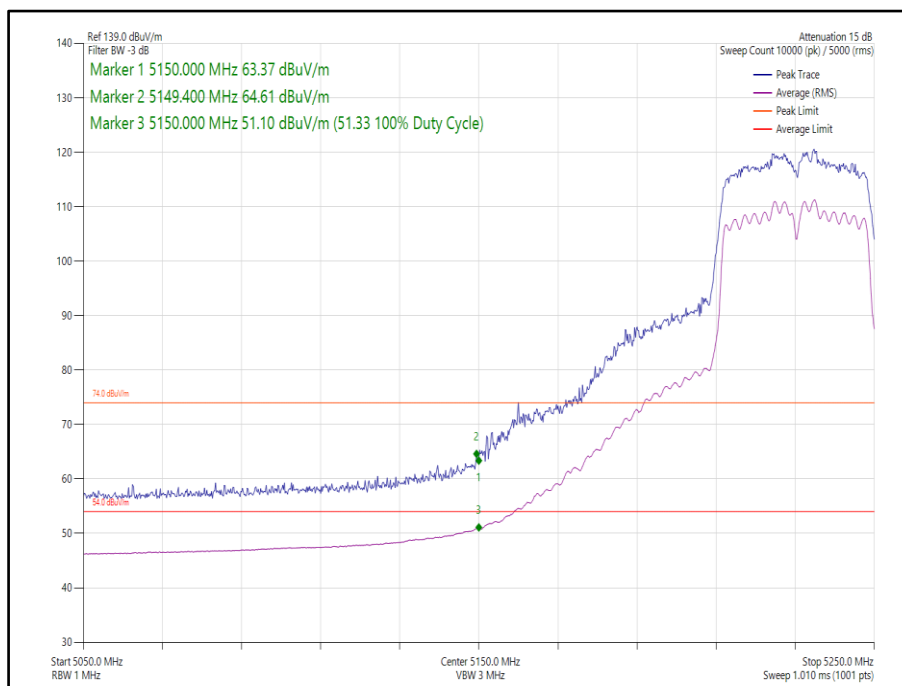
Figure 113 - 802.11n, HT40, CDD, Core 0-1 - 5230 MHz, Band Edge Frequency 5150 MHz
