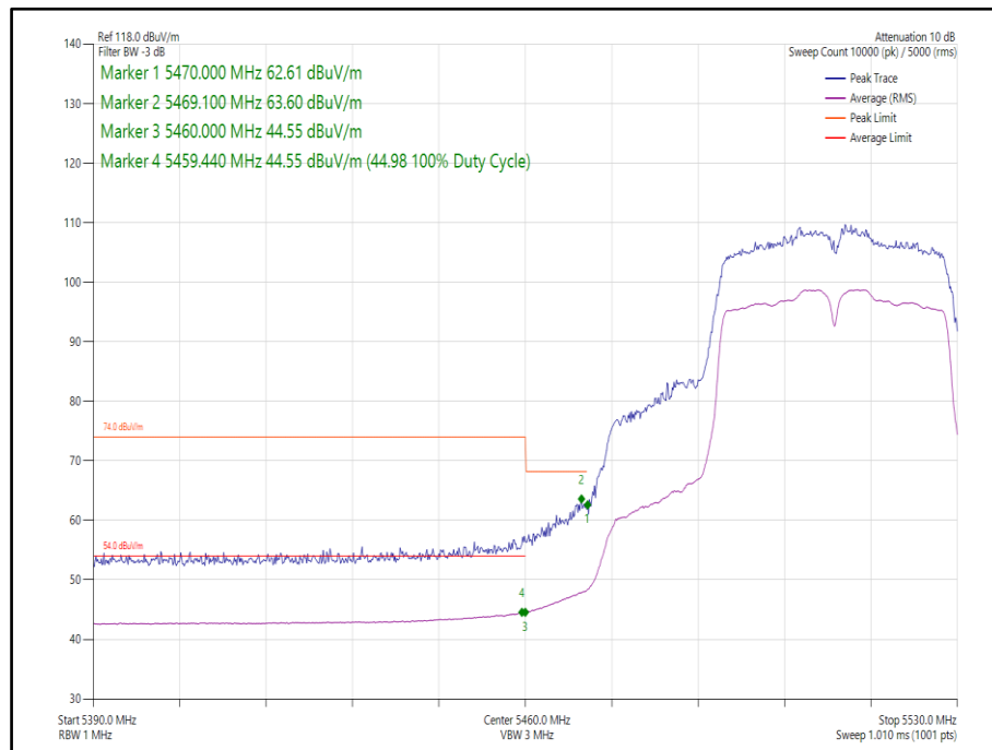
Figure 106 - 802.11n, HT40, SISO, Core 1 - 5510 MHz, Band Edge Frequency 5460 MHz
