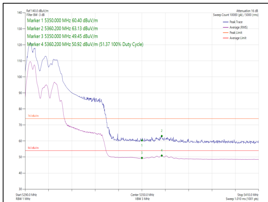
Figure 123 - 802.11ax, HE40, RU 52-37, CDD, Core 0-1 - 5310 MHz, Band Edge Frequency 5350 MHz
