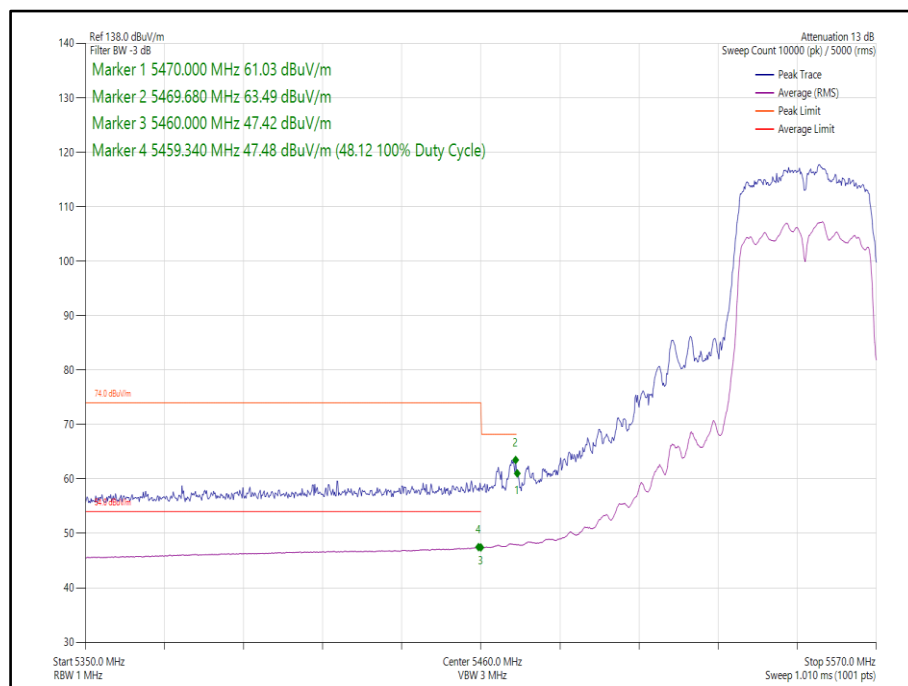
Figure 142 - 802.11n, HT40, SDM, Core 0-1 - 5550 MHz, Band Edge Frequency 5460 MHz
