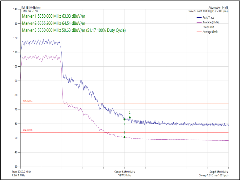
Figure 120 - 802.11ax, HE40, SU, CDD, Core 0-1 - 5270 MHz, Band Edge Frequency 5350 MHz
