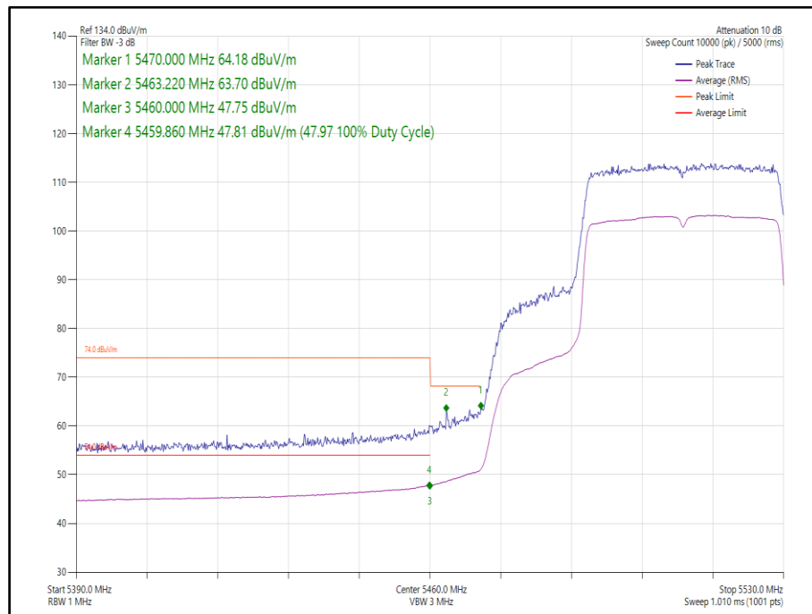
Figure 108 - 802.11ax, HE40, SU, SISO, Core 1 - 5510 MHz, Band Edge Frequency 5460 MHz
