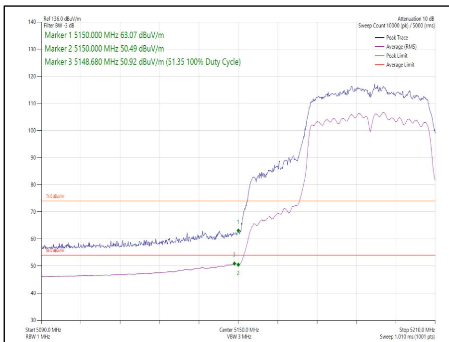
Figure 112 - 802.11n, HT40, CDD, Core 0-1 - 5190 MHz, Band Edge Frequency 5150 MHz
