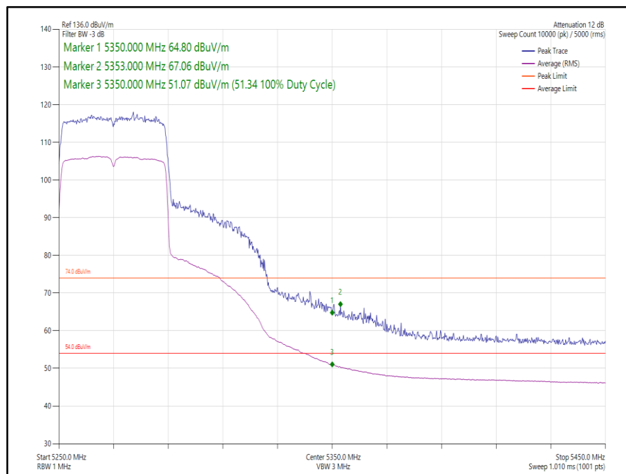
Figure 102 - 802.11ax, HE40, SU, SISO, Core 1 - 5270 MHz, Band Edge Frequency 5350 MHz
