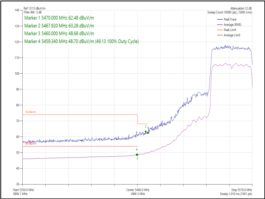
Figure 145 - 802.11ax, HE40, SU, SDM, Core 0-1 - 5550 MHz, Band Edge Frequency 5460 MHz
