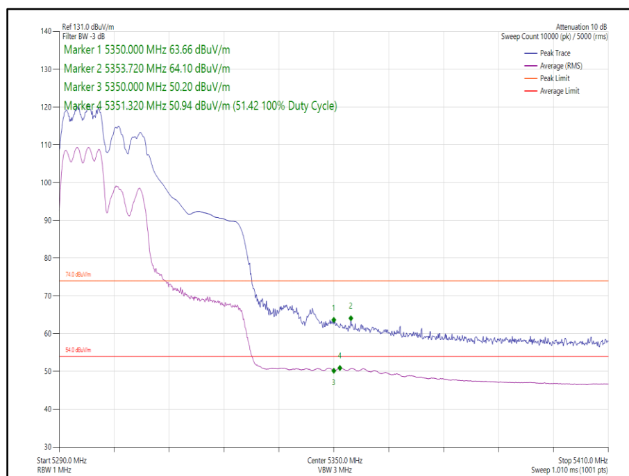
Figure 140 - 802.11ax, HE40, RU 106-53, SDM, Core 0-1 - 5310 MHz, Band Edge Frequency 5350 MHz
