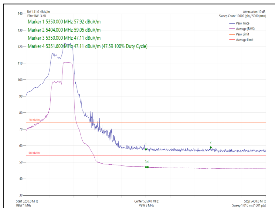
Figure 103 - 802.11ax, HE40, RU 106-56, SISO, Core 1 - 5270 MHz, Band Edge Frequency 5350 MHz
