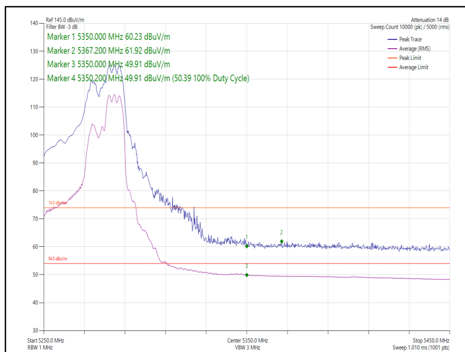
Figure 138 - 802.11ax, HE40, RU 106-56, SDM, Core 0-1 - 5270 MHz, Band Edge Frequency 5350 MHz
