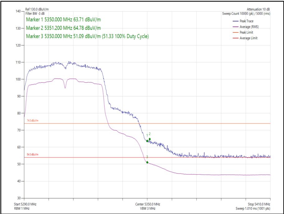
Figure 101 - 802.11n, HT40, SISO, Core 1 - 5310 MHz, Band Edge Frequency 5350 MHz
