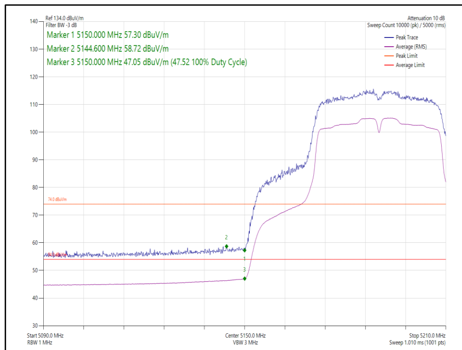
Figure 147 - 802.11ac, VHT40, TxBF, Core 0-1 - 5190 MHz, Band Edge Frequency 5150 MHz
