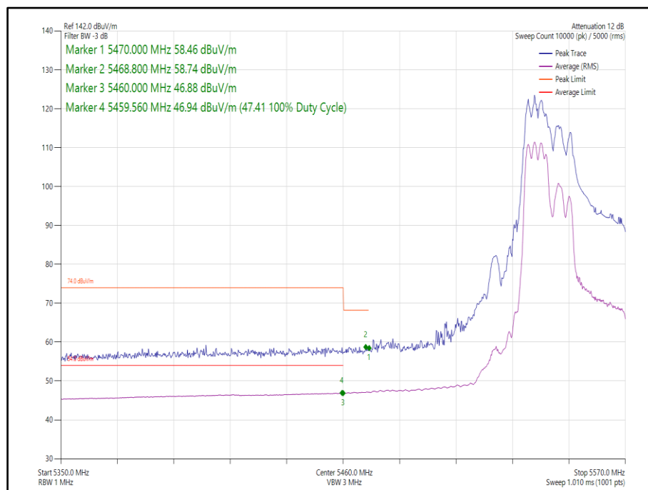
Figure 129 - 802.11ax, HE40, RU 106-53, CDD, Core 0-1 - 5550 MHz, Band Edge Frequency 5460 MHz
