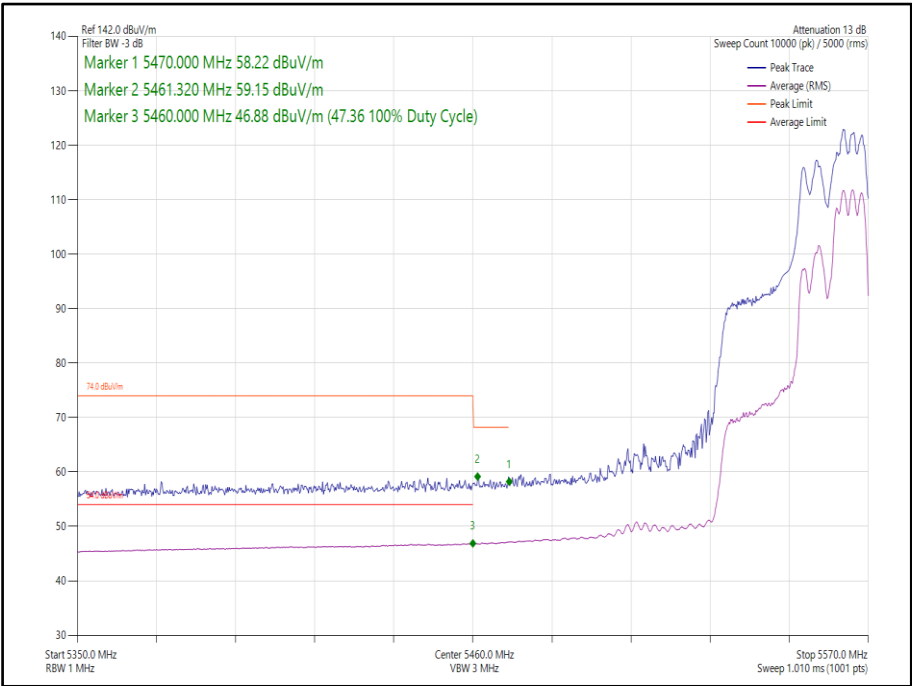
Figure 146 - 802.11ax, HE40, RU 106-56, SDM, Core 0-1 - 5550 MHz, Band Edge Frequency 5460 MHz
