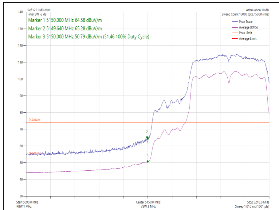
Figure 130 - 802.11n, HT40, SDM, Core 0-1 - 5190 MHz, Band Edge Frequency 5150 MHz
