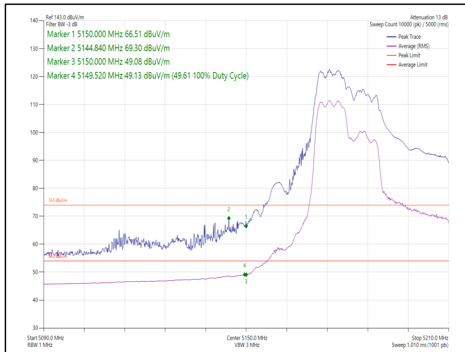
Figure 133 - 802.11ax, HE40, RU 106-53, SDM, Core 0-1 - 5190 MHz, Band Edge Frequency 5150 MHz
