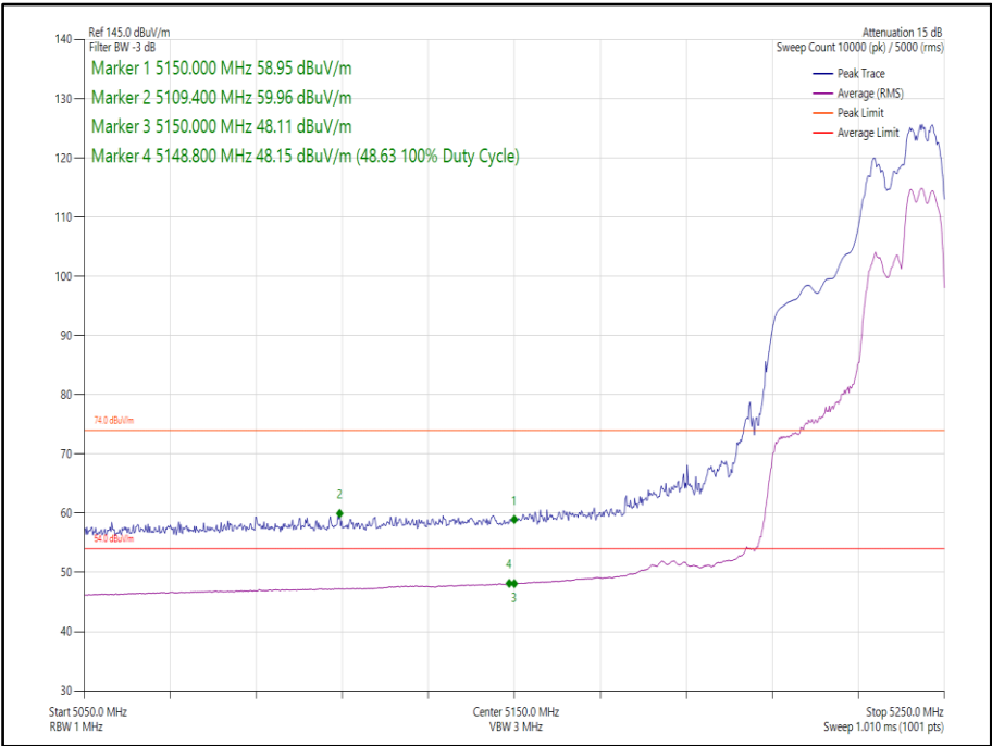
Figure 117 - 802.11ax, HE40, RU 106-56, CDD, Core 0-1 - 5230 MHz, Band Edge Frequency 5150 MHz
