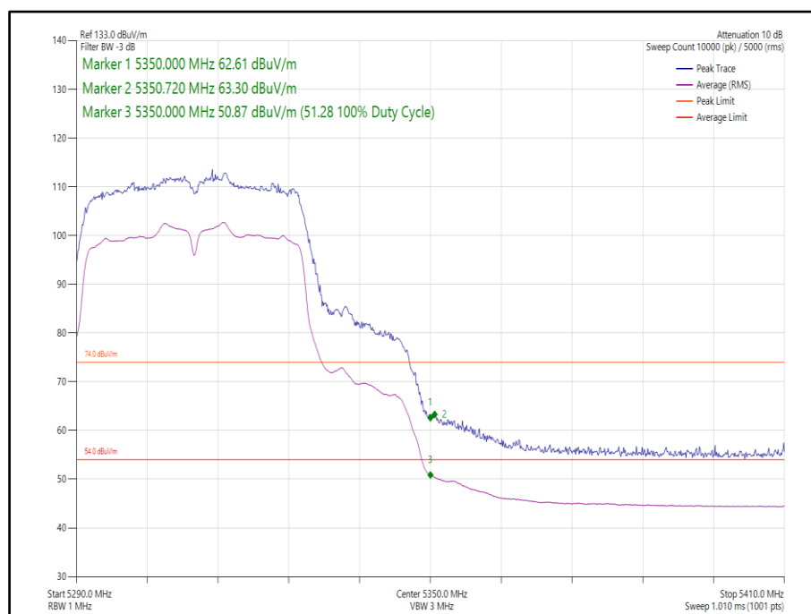
Figure 136 - 802.11n, HT40, SDM, Core 0-1 - 5310 MHz, Band Edge Frequency 5350 MHz
