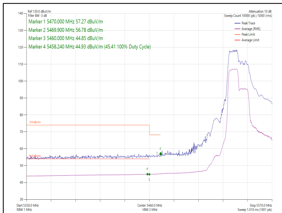
Figure 111 - 802.11ax, HE40, RU 106-53, SISO, Core 1 - 5550 MHz, Band Edge Frequency 5460 MHz
