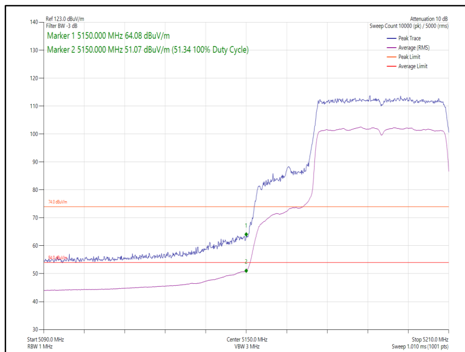
Figure 132 - 802.11ax, HE40, SU, SDM, Core 0-1 - 5190 MHz, Band Edge Frequency 5150 MHz
