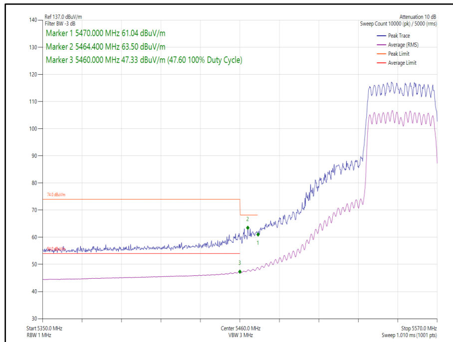
Figure 128 - 802.11ax, HE40, SU, CDD, Core 0-1 - 5550 MHz, Band Edge Frequency 5460 MHz
