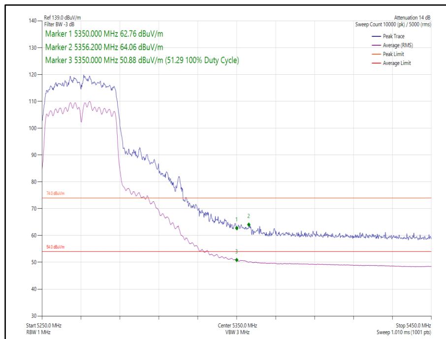
Figure 118 - 802.11n, HT40, CDD, Core 0-1 - 5270 MHz, Band Edge Frequency 5350 MHz
