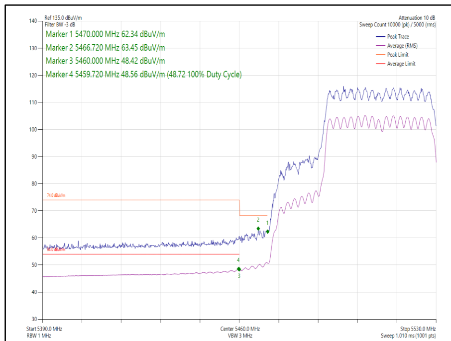
Figure 126 - 802.11ax, HE40, SU, CDD, Core 0-1 - 5510 MHz, Band Edge Frequency 5460 MHz
