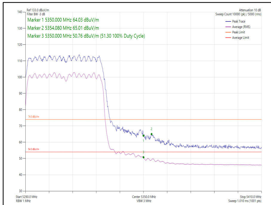
Figure 122 - 802.11ax, HE40, SU, CDD, Core 0-1 - 5310 MHz, Band Edge Frequency 5350 MHz
