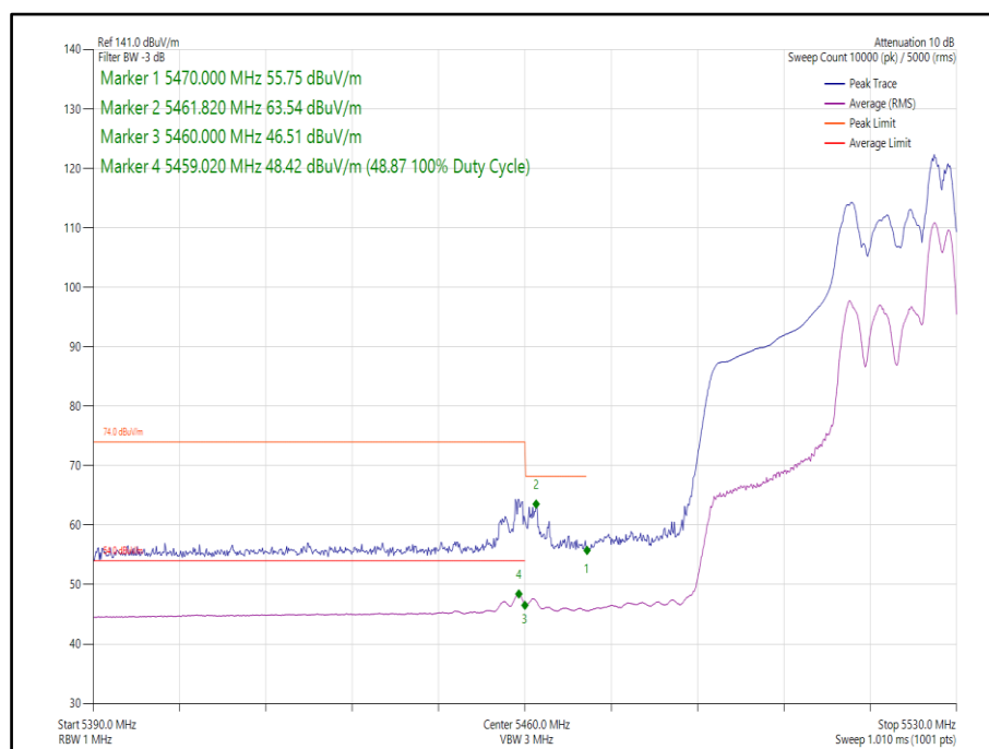
Figure 127 - 802.11ax, HE40, RU 52-44, CDD, Core 0-1 - 5510 MHz, Band Edge Frequency 5460 MHz
