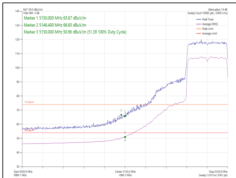
Figure 134 - 802.11ax, HE40, SU, SDM, Core 0-1 - 5230 MHz, Band Edge Frequency 5150 MHz
