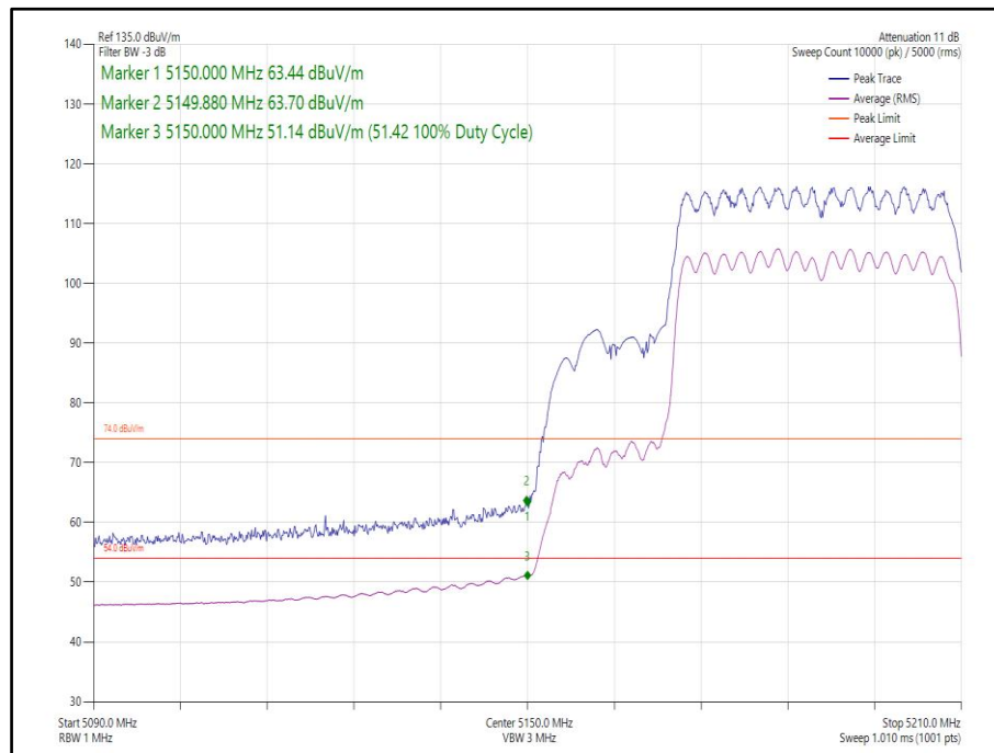
Figure 114 - 802.11ax, HE40, SU, CDD, Core 0-1 - 5190 MHz, Band Edge Frequency 5150 MHz
