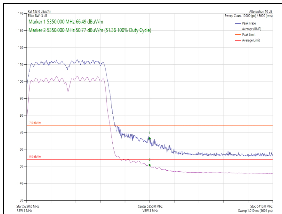
Figure 119 - 802.11n, HT40, CDD, Core 0-1 - 5310 MHz, Band Edge Frequency 5350 MHz
