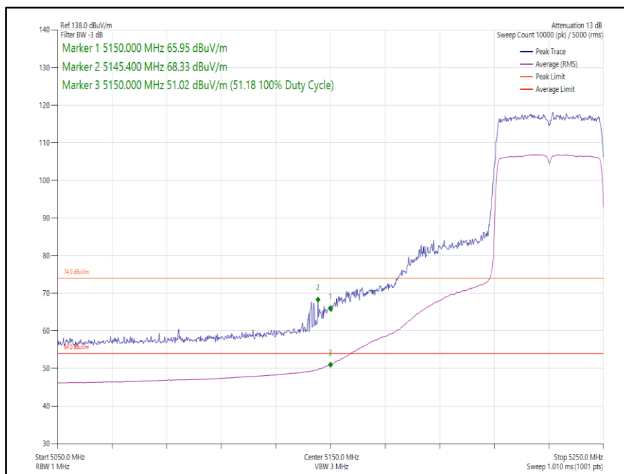
Figure 99 - 802.11ax, HE40, SU, SISO, Core 1 - 5230 MHz, Band Edge Frequency 5150 MHz
