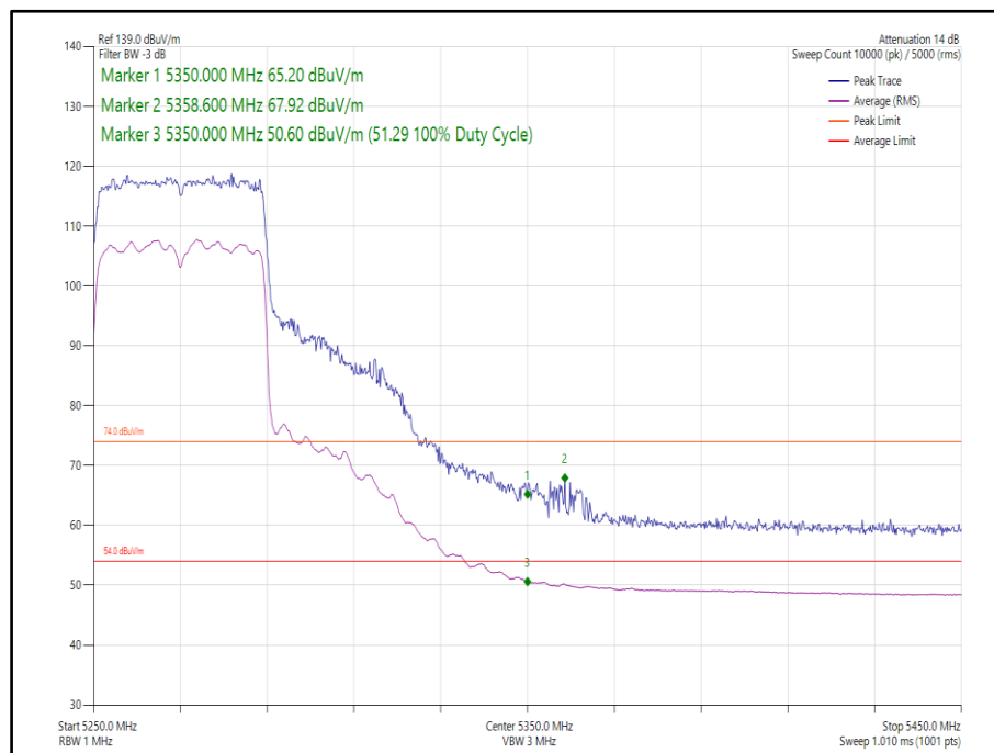
Figure 137 - 802.11ax, HE40, SU, SDM, Core 0-1 - 5270 MHz, Band Edge Frequency 5350 MHz
