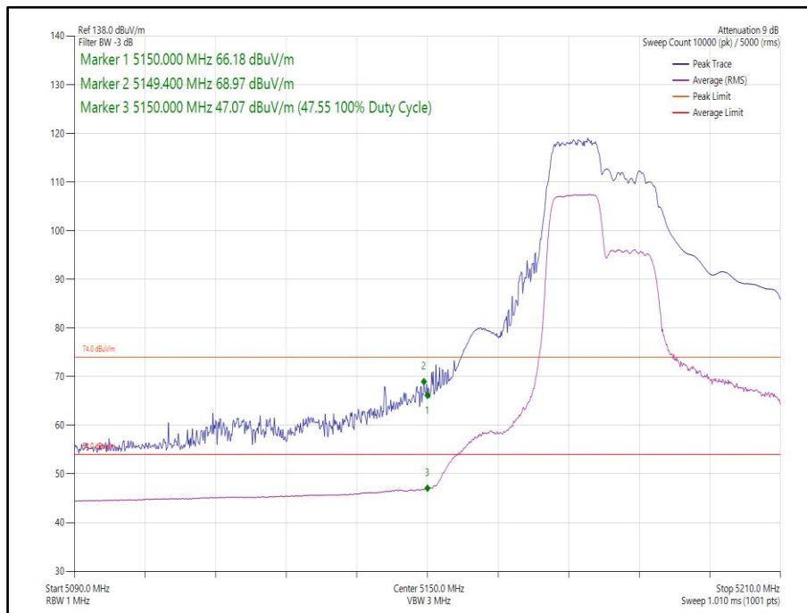
Figure 98 - 802.11ax, HE40, RU 106-53, SISO, Core 1 - 5190 MHz, Band Edge Frequency 5150 MHz
