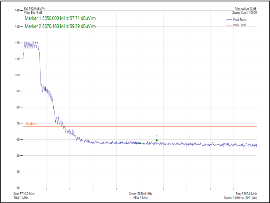
Figure 343 - 802.11ax, HE20, SU, CDD, Core 0-1 - 5720 MHz, Band Edge Frequency 5850 MHz
