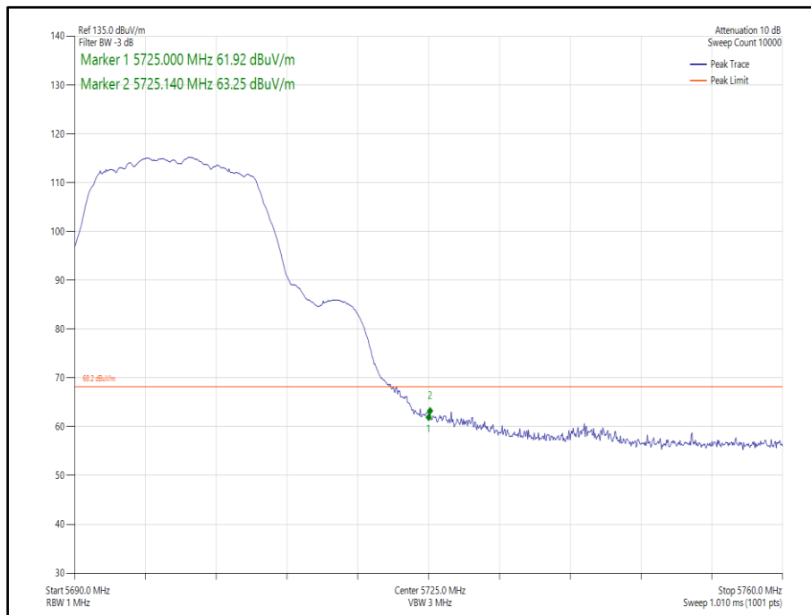
Figure 289 - 802.11a, SISO, Core 0 - 5700 MHz, Band Edge Frequency 5725 MHz
