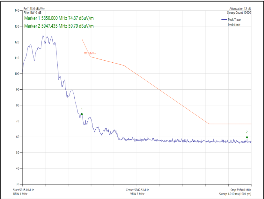
Figure 346 - 802.11ax, HE20, RU 106-54, CDD, Core 0-1 - 5825 MHz, Band Edge Frequency 5850 MHz
