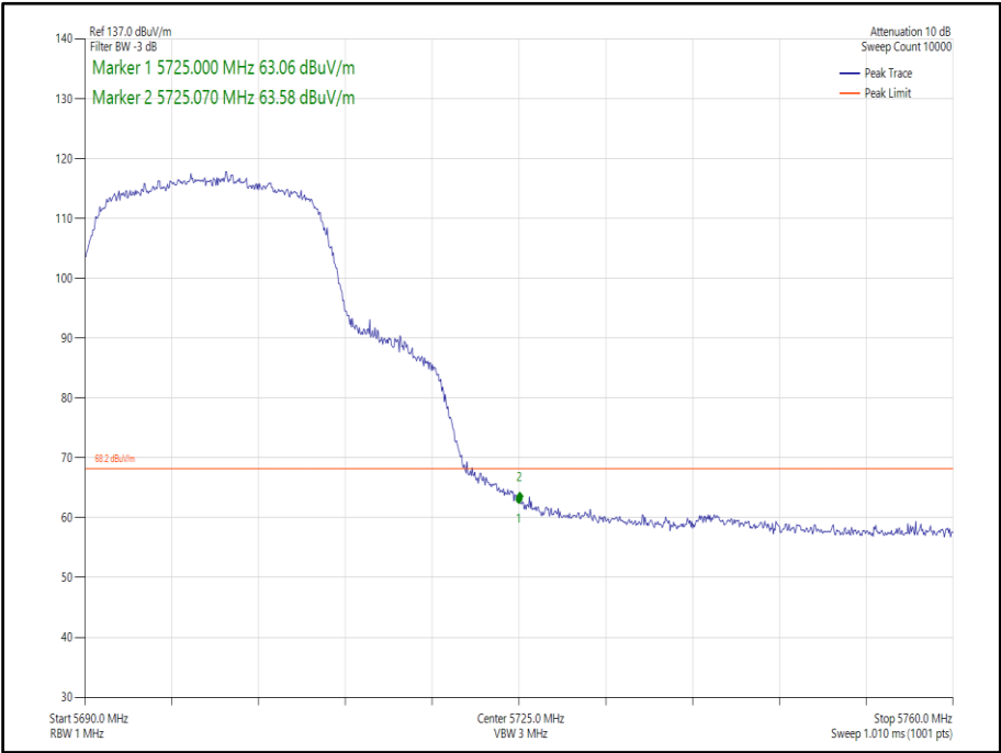
Figure 316 - 802.11n, HT20, SISO, Core 1 - 5700 MHz, Band Edge Frequency 5725 MHz
