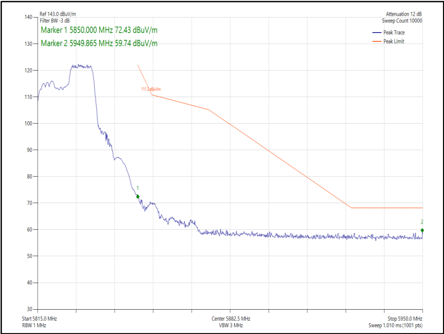
Figure 326 - 802.11ax, HE20, RU 106-54, SISO, Core 1 - 5825 MHz, Band Edge Frequency 5850 MHz
