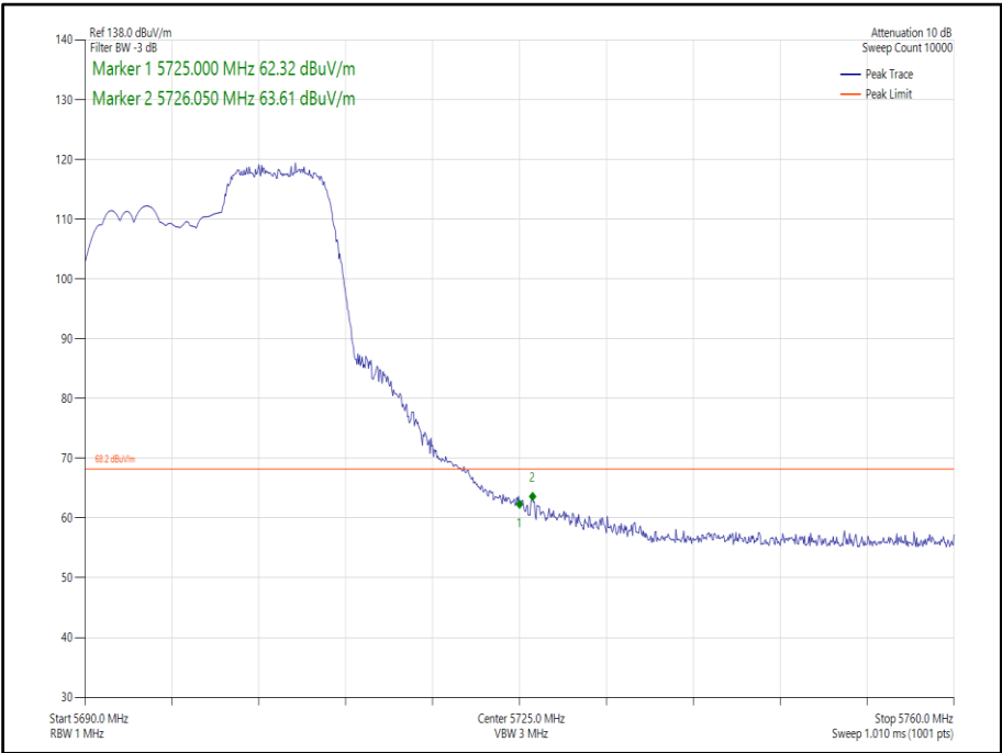
Figure 294 - 802.11ax, HE20, RU 106-54, SISO, Core 0 - 5700 MHz, Band Edge Frequency 5725 MHz
