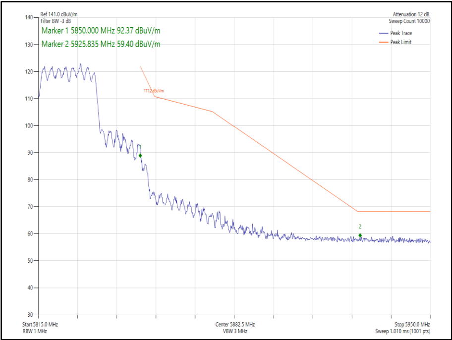
Figure 345 - 802.11ax, HE20, SU, CDD, Core 0-1 - 5825 MHz, Band Edge Frequency 5850 MHz
