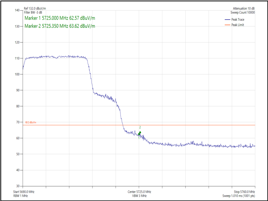
Figure 293 - 802.11ax, HE20, SU, SISO, Core 0 - 5700 MHz, Band Edge Frequency 5725 MHz
