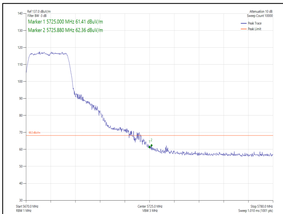
Figure 290 - 802.11n, HT20, SISO, Core 0 - 5680 MHz, Band Edge Frequency 5725 MHz
