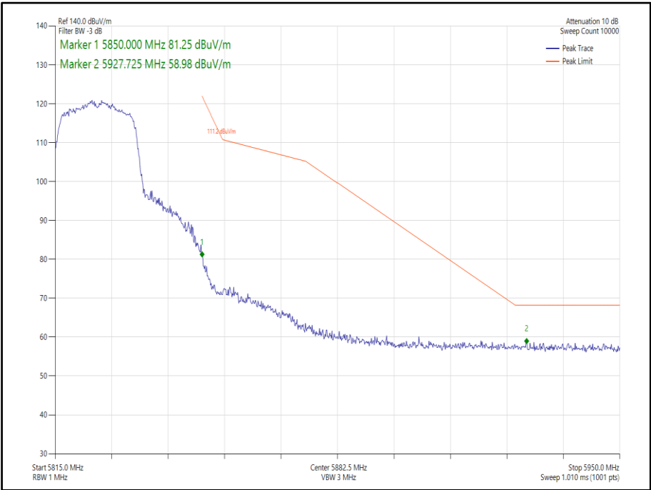
Figure 323 - 802.11n, HT20, SISO, Core 1 - 5825 MHz, Band Edge Frequency 5850 MHz
