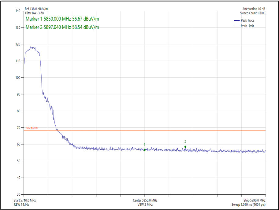
Figure 322 - 802.11n, HT20, SISO, Core 1 - 5720 MHz, Band Edge Frequency 5850 MHz
