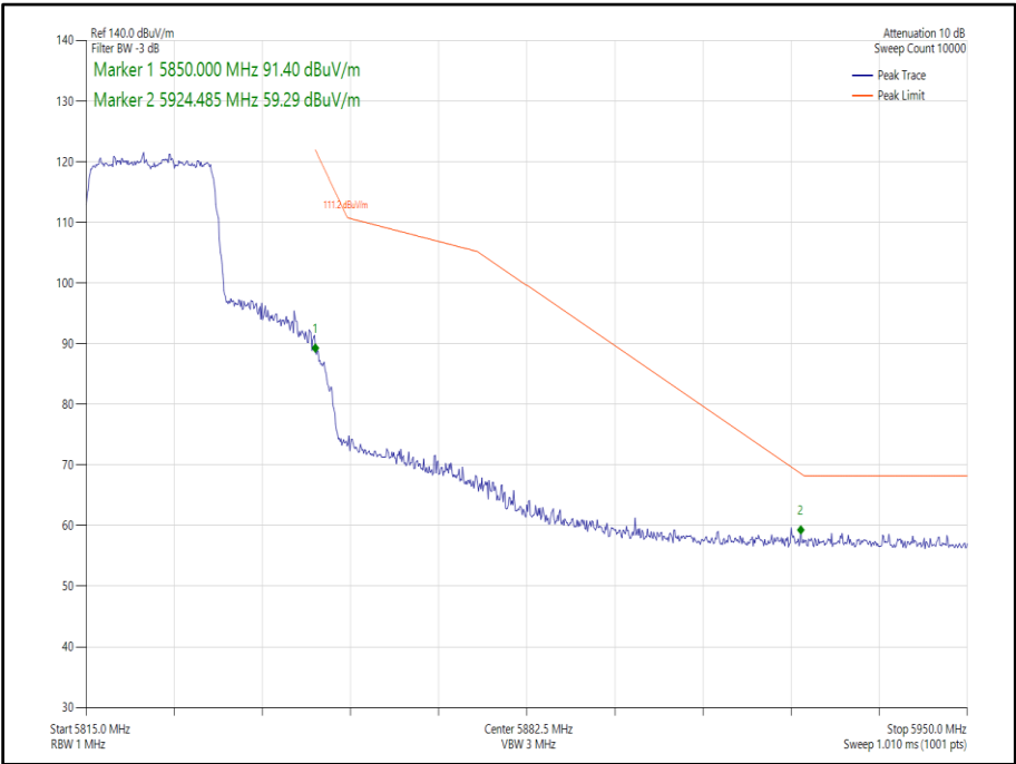
Figure 325 - 802.11ax, HE20, SU, SISO, Core 1 - 5825 MHz, Band Edge Frequency 5850 MHz
