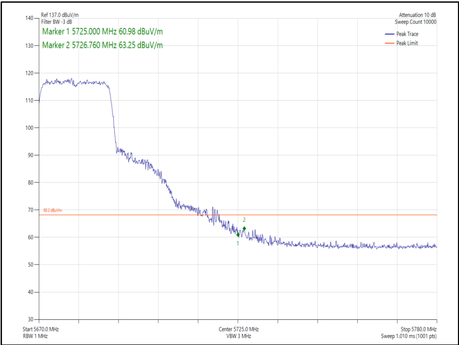
Figure 292 - 802.11ax, HE20, SU, SISO, Core 0 - 5680 MHz, Band Edge Frequency 5725 MHz
