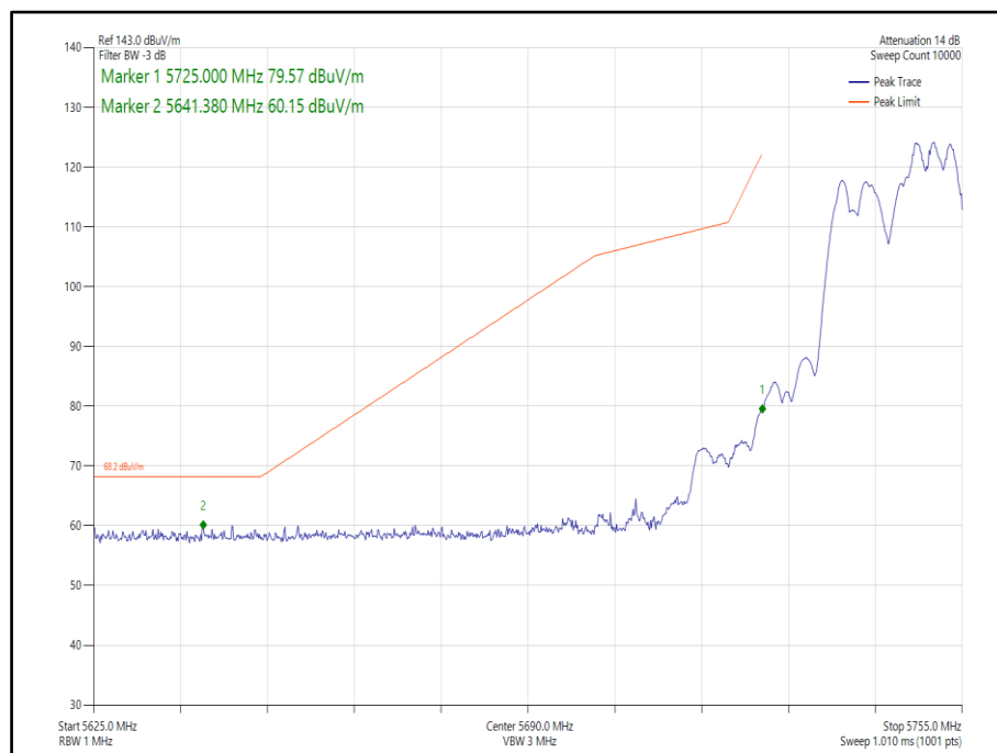
Figure 334 - 802.11ax, HE20, RU 106-54, CDD, Core 0-1 - 5745 MHz, Band Edge Frequency 5725 MHz
