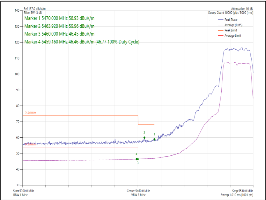
Figure 303 - 802.11a, SISO, Core 1 - 5520 MHz, Band Edge Frequency 5470 MHz
