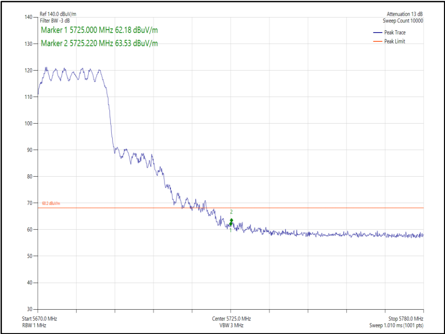
Figure 337 - 802.11ax, HE20, SU, CDD, Core 0-1 - 5680 MHz, Band Edge Frequency 5725 MHz
