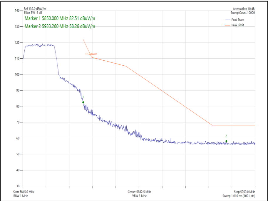
Figure 298 - 802.11n, HT20, SISO, Core 0 - 5825 MHz, Band Edge Frequency 5850 MHz
