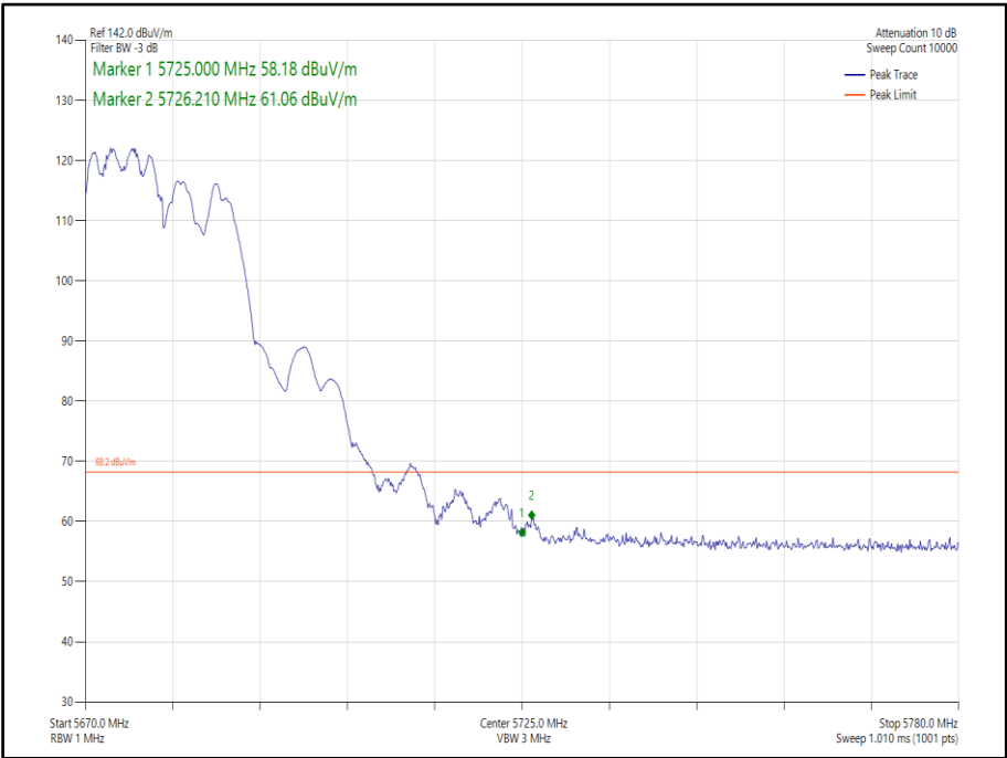
Figure 338 - 802.11ax, HE20, RU 106-53, CDD, Core 0-1 - 5680 MHz, Band Edge Frequency 5725 MHz
