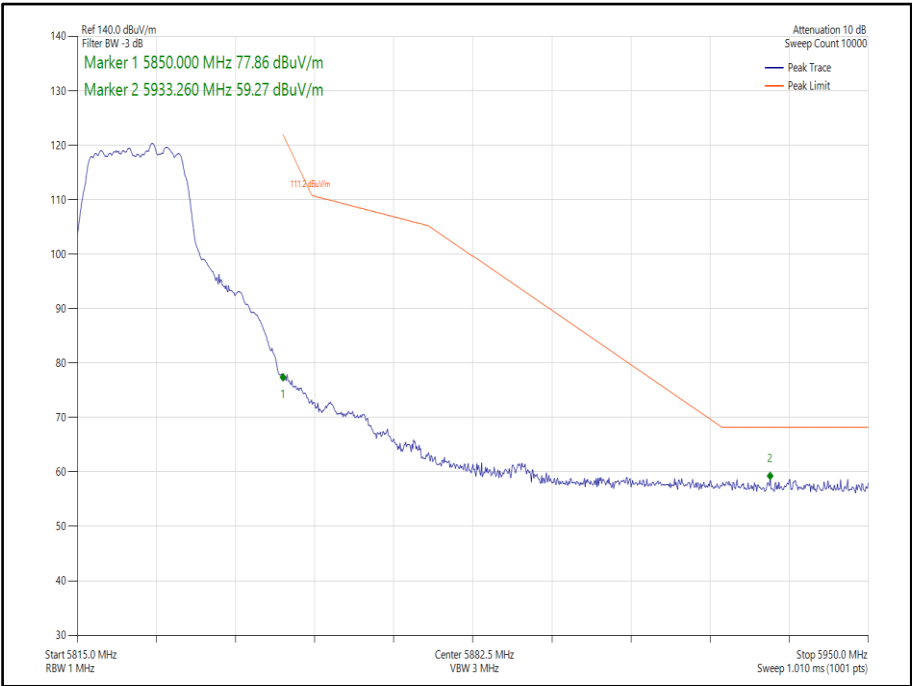
Figure 321 - 802.11a, SISO, Core 1 - 5825 MHz, Band Edge Frequency 5850 MHz
