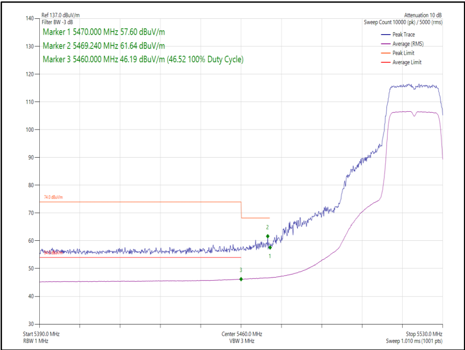
Figure 305 - 802.11n, HT20, SISO, Core 1 - 5520 MHz, Band Edge Frequency 5470 MHz
