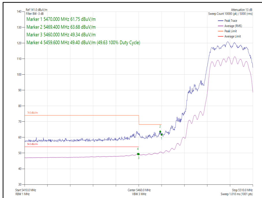
Figure 327 - 802.11n, HT20, CDD, Core 0-1 - 5500 MHz, Band Edge Frequency 5470 MHz
