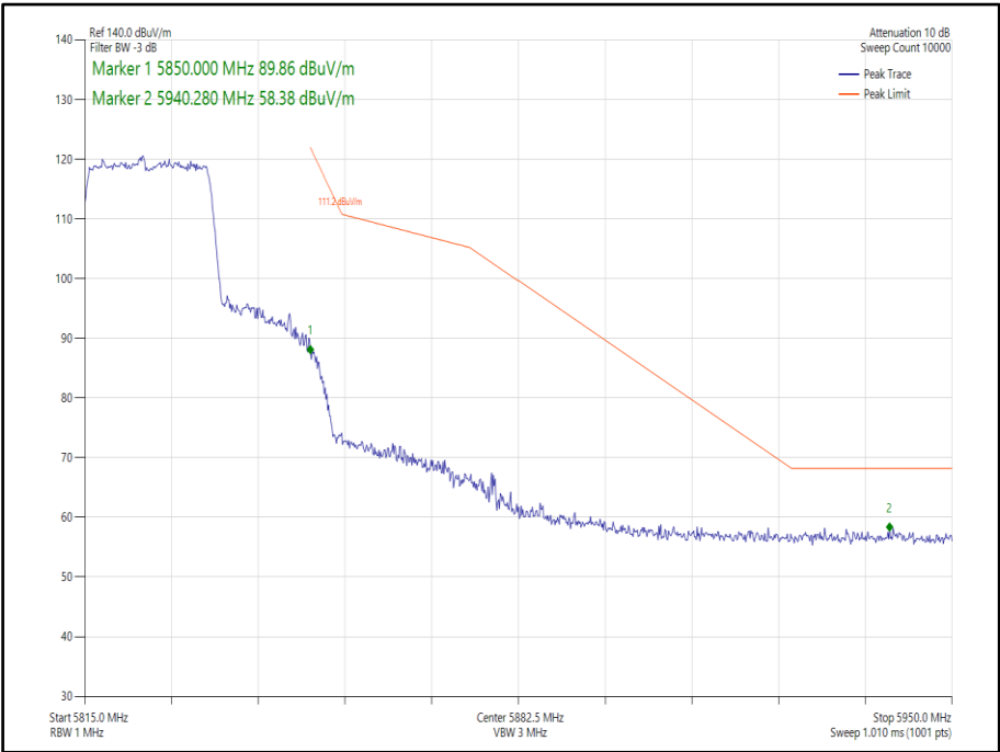
Figure 300 - 802.11ax, HE20, SU, SISO, Core 0 - 5825 MHz, Band Edge Frequency 5850 MHz
