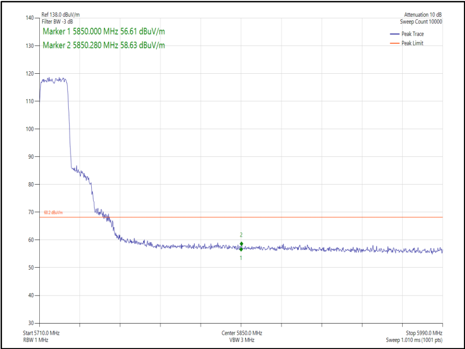
Figure 324 - 802.11ax, HE20, SU, SISO, Core 1 - 5720 MHz, Band Edge Frequency 5850 MHz
