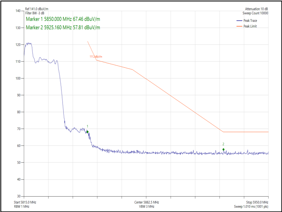
Figure 301 - 802.11ax, HE20, RU 52-37, SISO, Core 0 - 5825 MHz, Band Edge Frequency 5850 MHz
