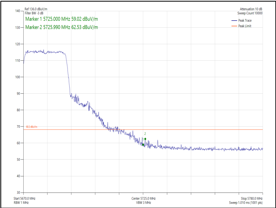
Figure 317 - 802.11ax, HE20, SU, SISO, Core 1 - 5680 MHz, Band Edge Frequency 5725 MHz
