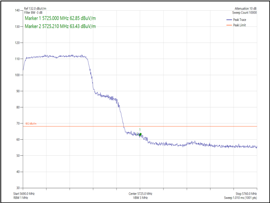
Figure 318 - 802.11ax, HE20, SU, SISO, Core 1 - 5700 MHz, Band Edge Frequency 5725 MHz
