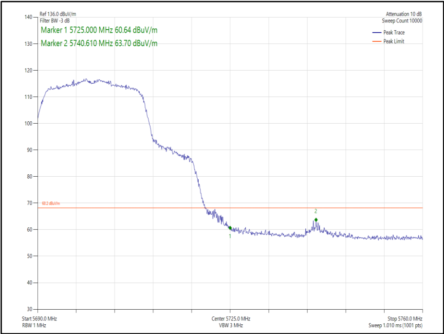
Figure 291 - 802.11n, HT20, SISO, Core 0 - 5700 MHz, Band Edge Frequency 5725 MHz
