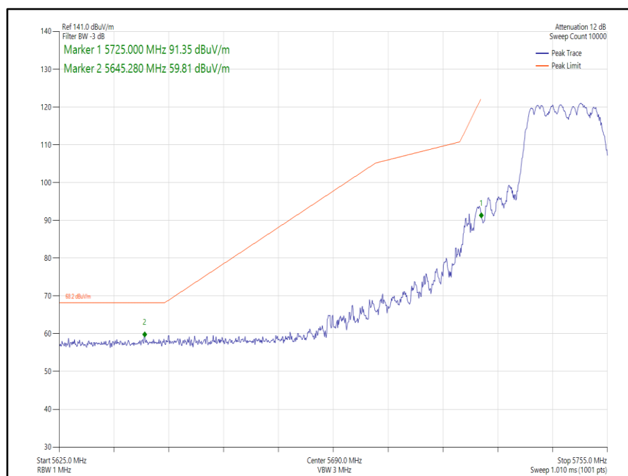
Figure 332 - 802.11n, HT20, CDD, Core 0-1 - 5745 MHz, Band Edge Frequency 5725 MHz
