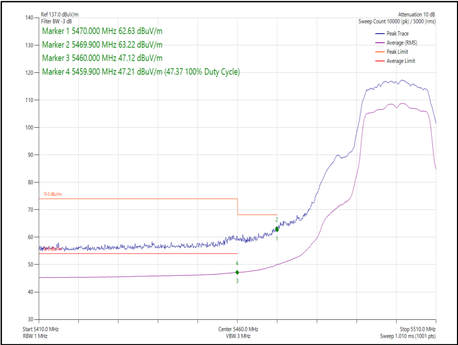
Figure 302 - 802.11a, SISO, Core 1 - 5500 MHz, Band Edge Frequency 5470 MHz
