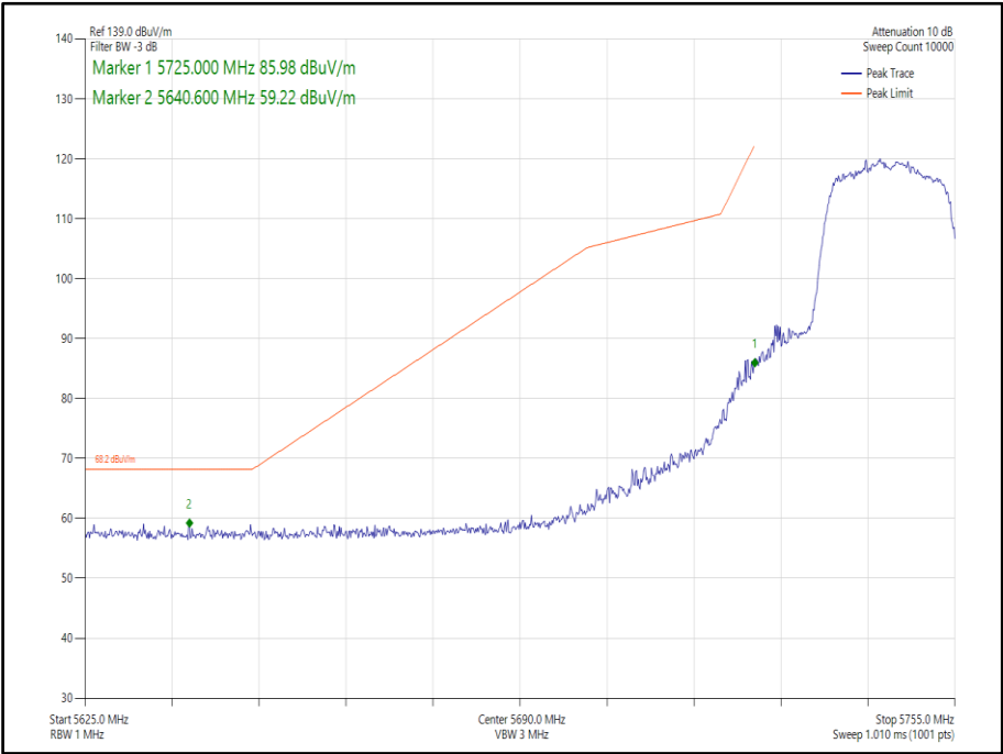
Figure 310 - 802.11n, HT20, SISO, Core 1 - 5745 MHz, Band Edge Frequency 5725 MHz
