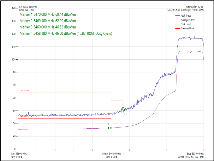
Figure 308 - 802.11ax, HE20, SU, SISO, Core 1 - 5520 MHz, Band Edge Frequency 5470 MHz
