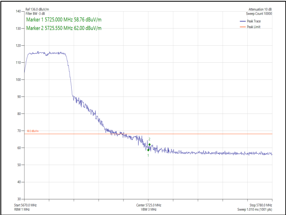
Figure 315 - 802.11n, HT20, SISO, Core 1 - 5680 MHz, Band Edge Frequency 5725 MHz
