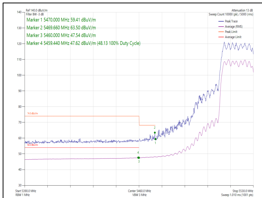
Figure 331 - 802.11ax, HE20, SU, CDD, Core 0-1 - 5520 MHz, Band Edge Frequency 5470 MHz
