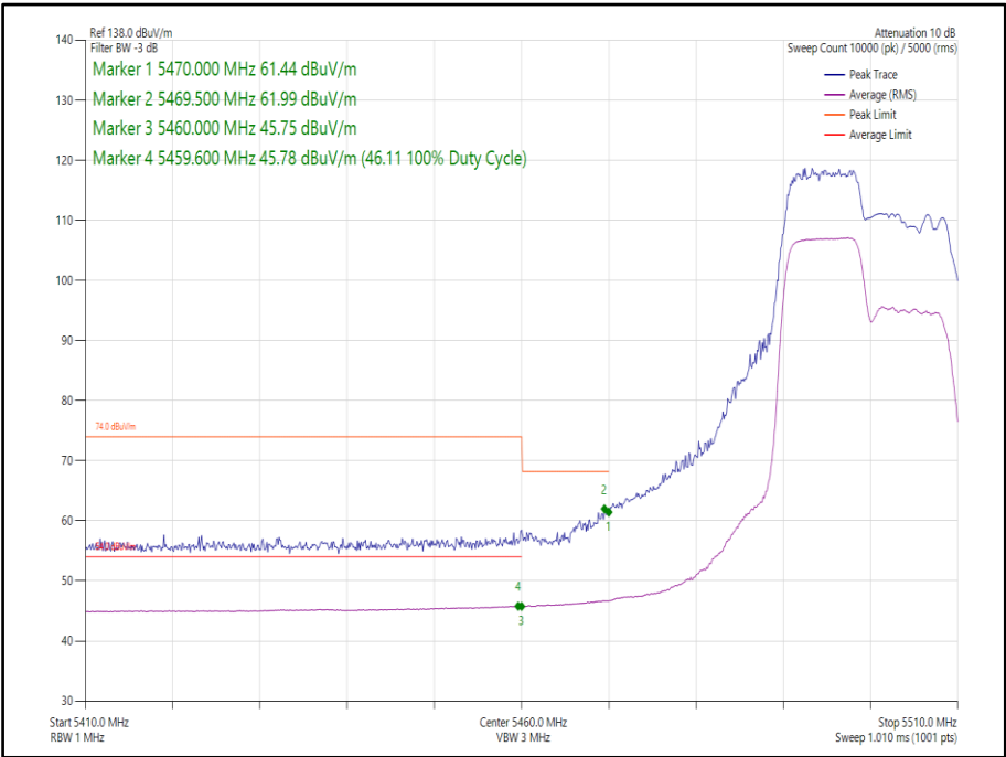
Figure 307 - 802.11ax, HE20, RU 106-53, SISO, Core 1 - 5500 MHz, Band Edge Frequency 5470 MHz
