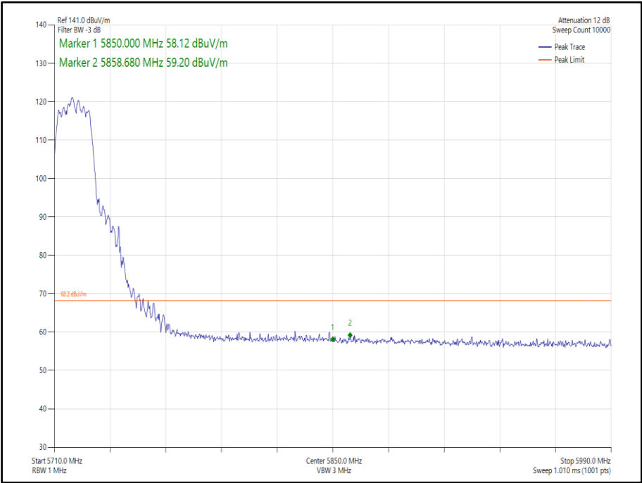
Figure 341 - 802.11n, HT20, CDD, Core 0-1 - 5720 MHz, Band Edge Frequency 5850 MHz
