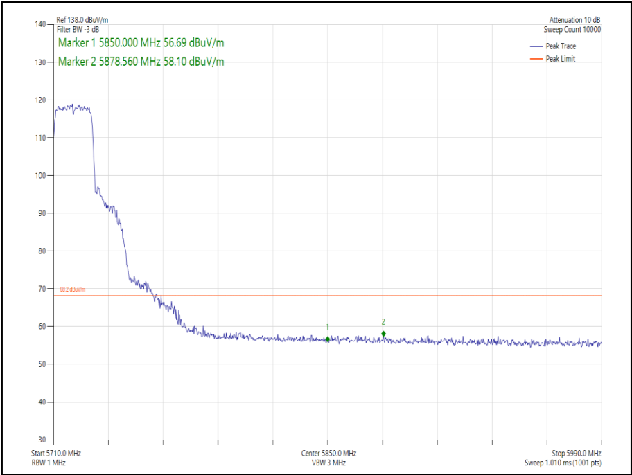
Figure 299 - 802.11ax, HE20, SU, SISO, Core 0 - 5720 MHz, Band Edge Frequency 5850 MHz
