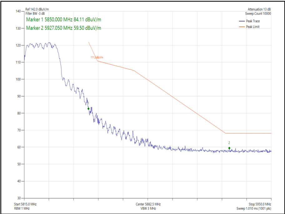
Figure 342 - 802.11n, HT20, CDD, Core 0-1 - 5825 MHz, Band Edge Frequency 5850 MHz
