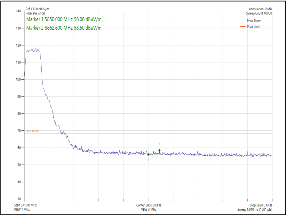
Figure 295 - 802.11a, SISO, Core 0 - 5720 MHz, Band Edge Frequency 5850 MHz
