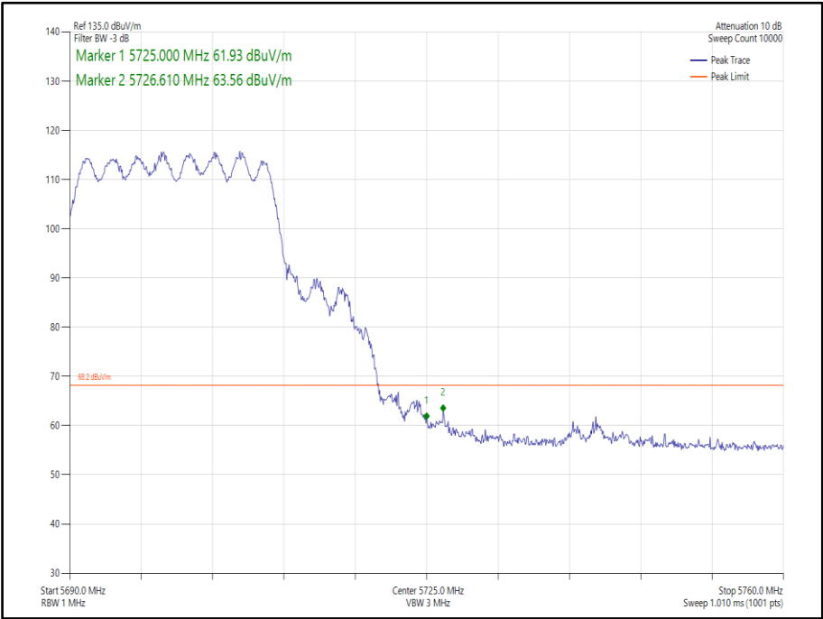
Figure 339 - 802.11ax, HE20, SU, CDD, Core 0-1 - 5700 MHz, Band Edge Frequency 5725 MHz
