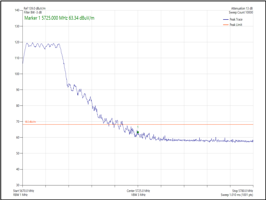
Figure 335 - 802.11n, HT20, CDD, Core 0-1 - 5680 MHz, Band Edge Frequency 5725 MHz
