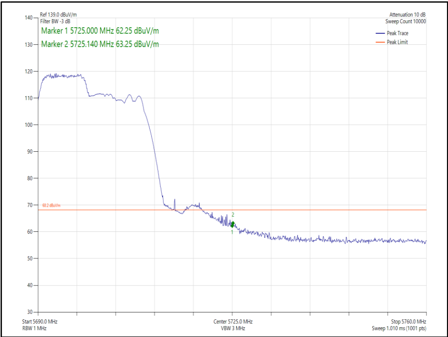
Figure 319 - 802.11ax, HE20, RU 106-53, SISO, Core 1 - 5700 MHz, Band Edge Frequency 5725 MHz
