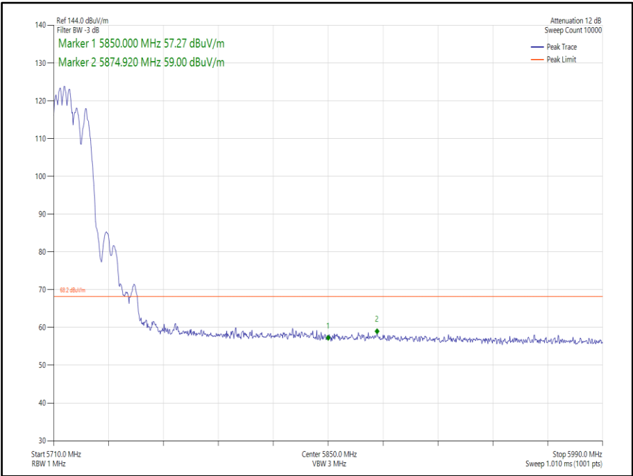
Figure 344 - 802.11ax, HE20, RU 106-53, CDD, Core 0-1 - 5720 MHz, Band Edge Frequency 5850 MHz
