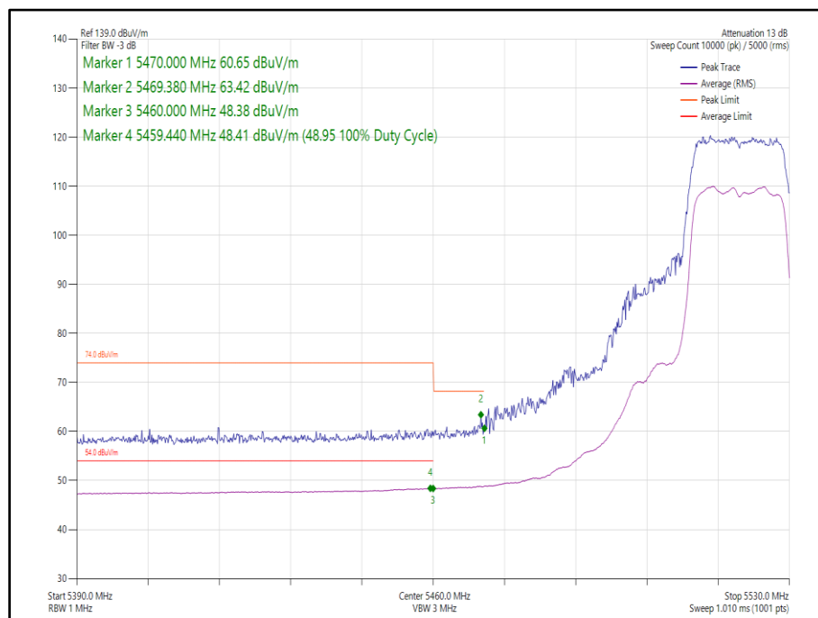
Figure 348 - 802.11n, HT20, SDM, Core 0-1 - 5520 MHz, Band Edge Frequency 5470 MHz
