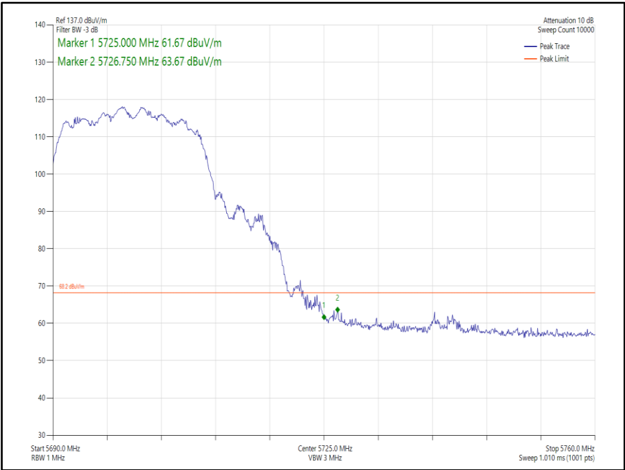
Figure 336 - 802.11n, HT20, CDD, Core 0-1 - 5700 MHz, Band Edge Frequency 5725 MHz
