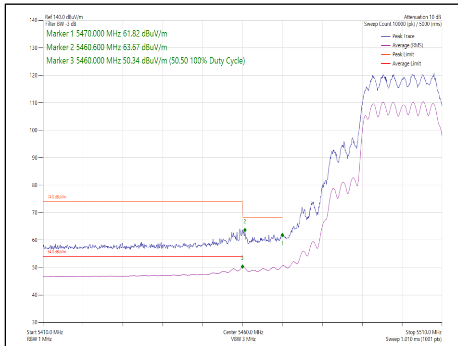
Figure 329 - 802.11ax, HE20, SU, CDD, Core 0-1 - 5500 MHz, Band Edge Frequency 5470 MHz
