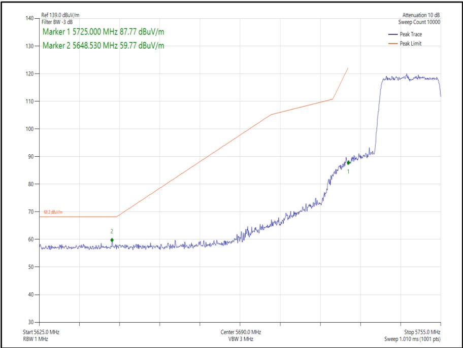
Figure 311 - 802.11ax, HE20, SU, SISO, Core 1 - 5745 MHz, Band Edge Frequency 5725 MHz
