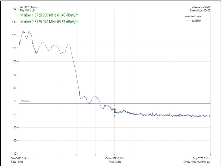
Figure 340 - 802.11ax, HE20, RU 52-37, CDD, Core 0-1 - 5700 MHz, Band Edge Frequency 5725 MHz
