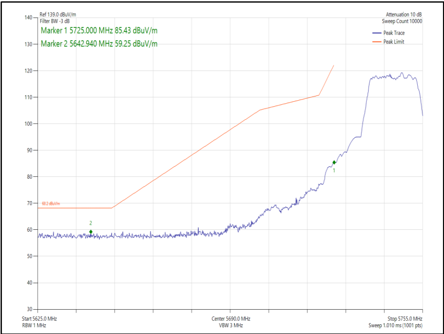
Figure 309 - 802.11a, SISO, Core 1 - 5745 MHz, Band Edge Frequency 5725 MHz
