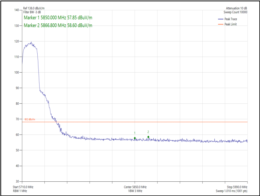
Figure 297 - 802.11n, HT20, SISO, Core 0 - 5720 MHz, Band Edge Frequency 5850 MHz
