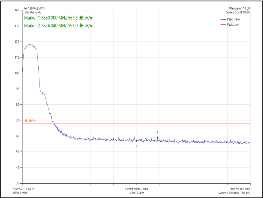
Figure 320 - 802.11a, SISO, Core 1 - 5720 MHz, Band Edge Frequency 5850 MHz
