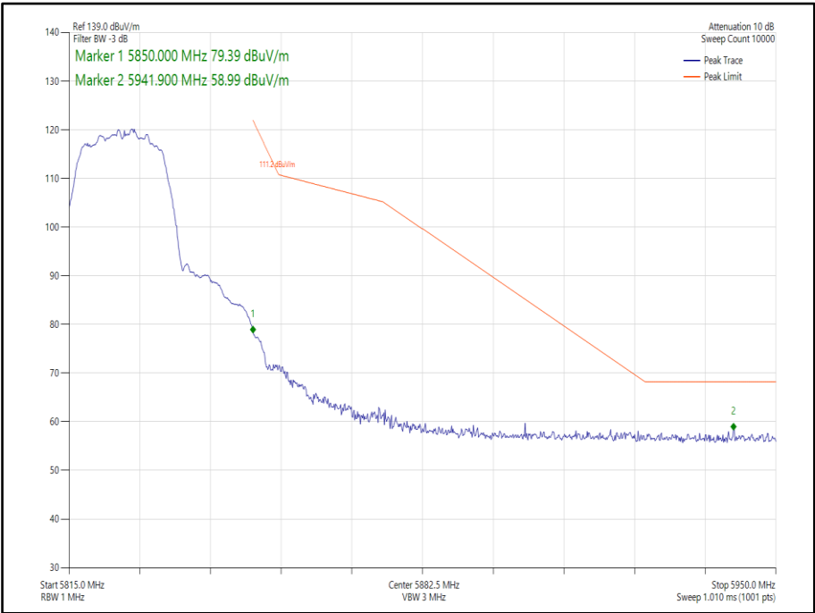
Figure 296 - 802.11a, SISO, Core 0 - 5825 MHz, Band Edge Frequency 5850 MHz
