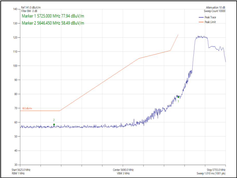
Figure 312 - 802.11ax, HE20, RU 106-53, SISO, Core 1 - 5745 MHz, Band Edge Frequency 5725 MHz
