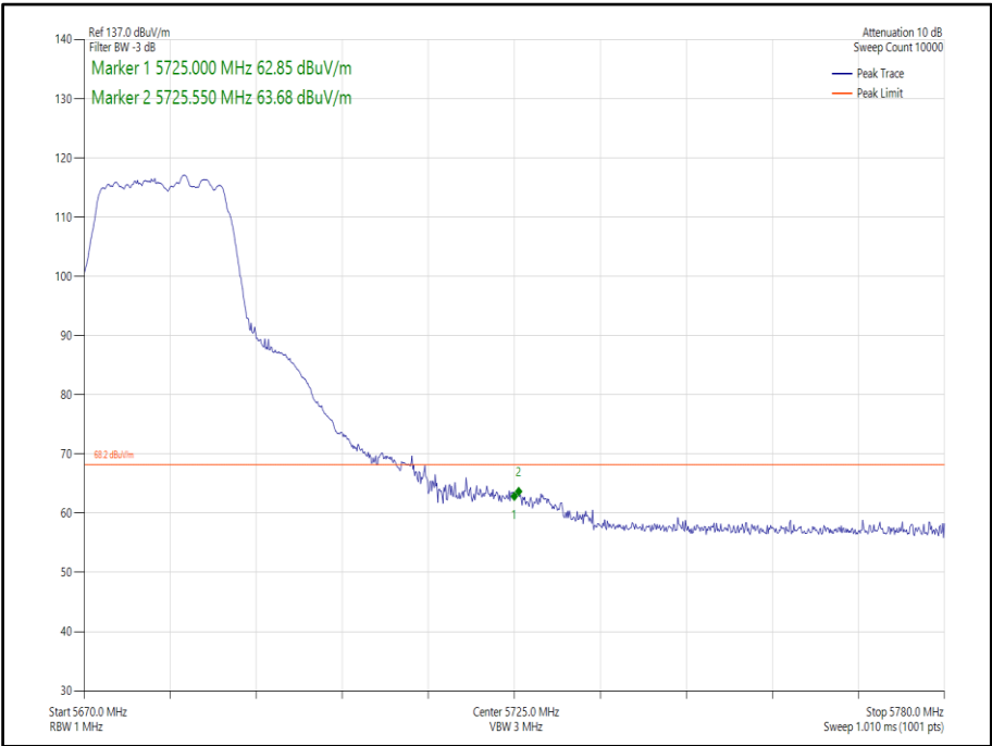
Figure 313 - 802.11a, SISO, Core 1 - 5680 MHz, Band Edge Frequency 5725 MHz
