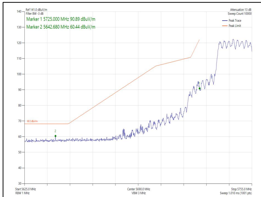
Figure 333 - 802.11ax, HE20, SU, CDD, Core 0-1 - 5745 MHz, Band Edge Frequency 5725 MHz
