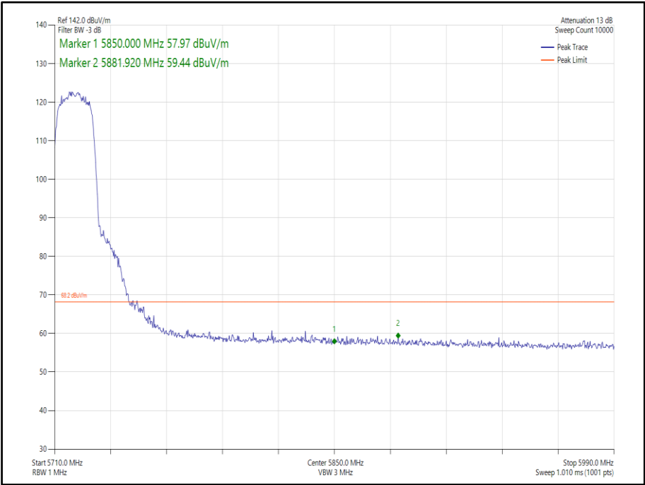
Figure 370 - 802.11ac, VHT20, TxBF, Core 0-1 - 5720 MHz, Band Edge Frequency 5850 MHz
