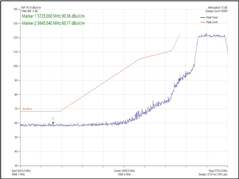
Figure 368 - 802.11ac, VHT20, TxBF, Core 0-1 - 5745 MHz, Band Edge Frequency 5725 MHz
