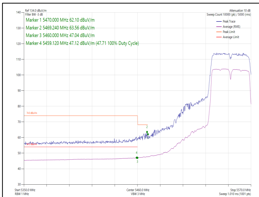
Figure 373 - 802.11n, HT40, SISO, Core 0 - 5550 MHz, Band Edge Frequency 5470 MHz
