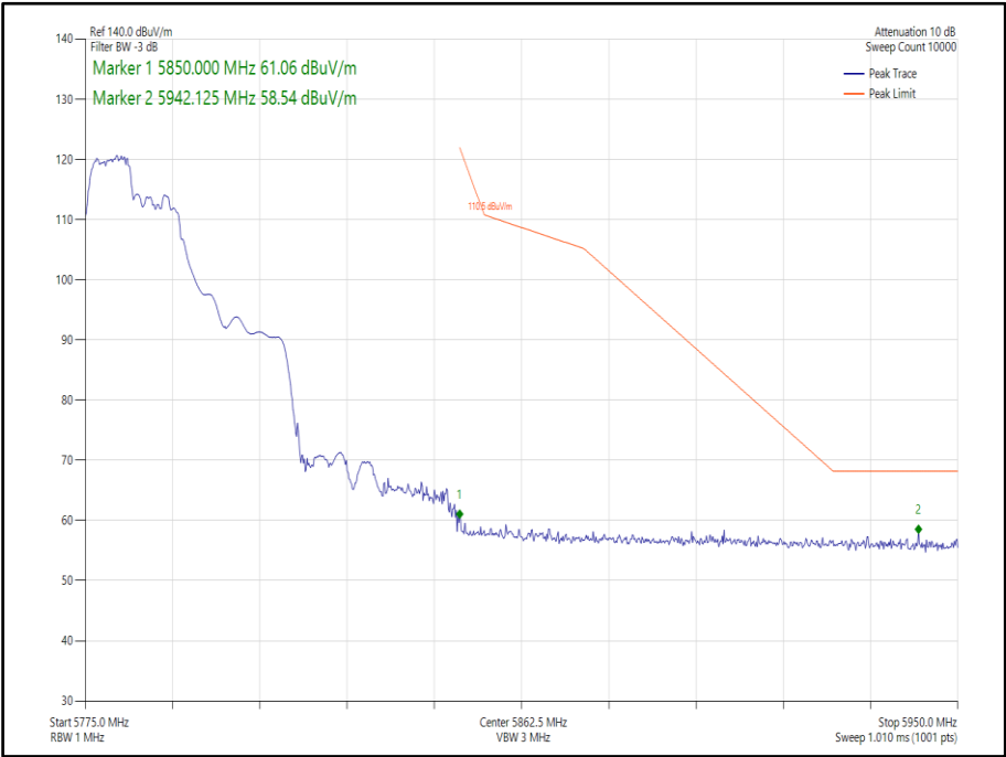
Figure 390 - 802.11ax, HE40, RU 106-53, SISO, Core 0 - 5795 MHz, Band Edge Frequency 5850 MHz
