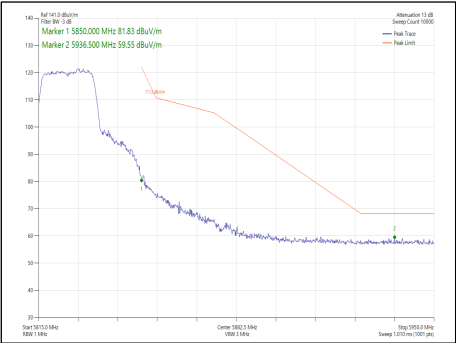
Figure 362 - 802.11n, HT20, SDM, Core 0-1 - 5825 MHz, Band Edge Frequency 5850 MHz
