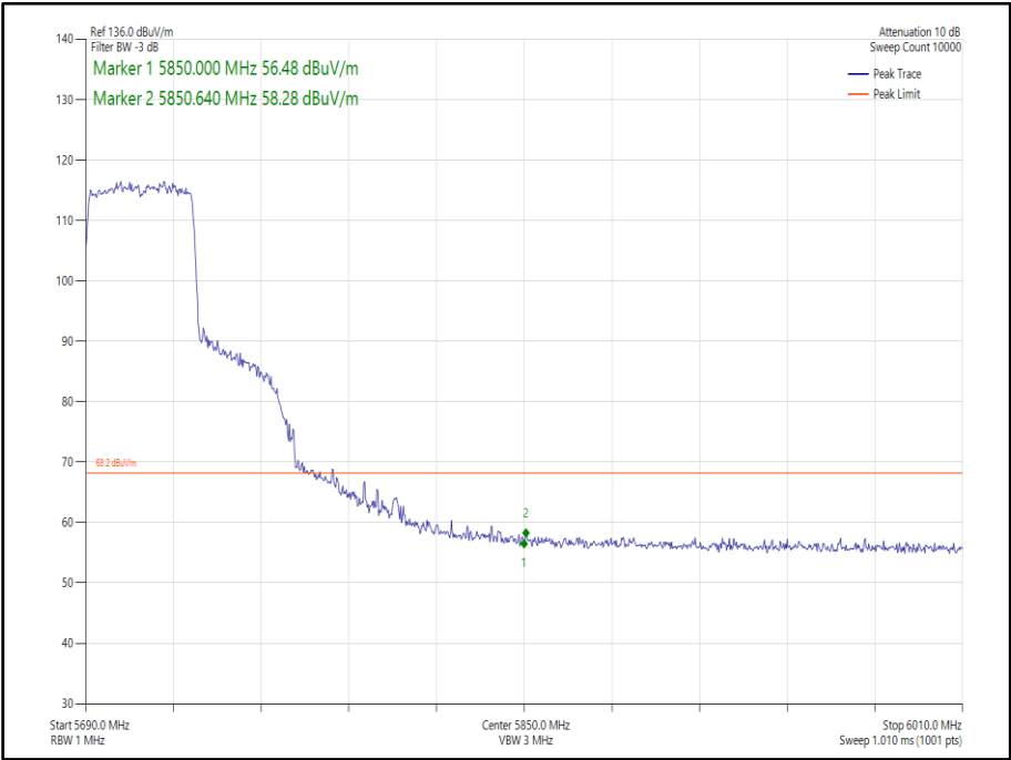
Figure 388 - 802.11ax, HE40, SU, SISO, Core 0 - 5710 MHz, Band Edge Frequency 5850 MHz
