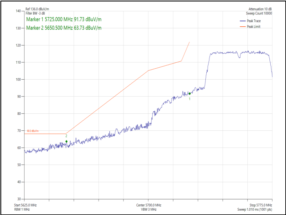
Figure 378 - 802.11n, HT40, SISO, Core 0 - 5755 MHz, Band Edge Frequency 5725 MHz
