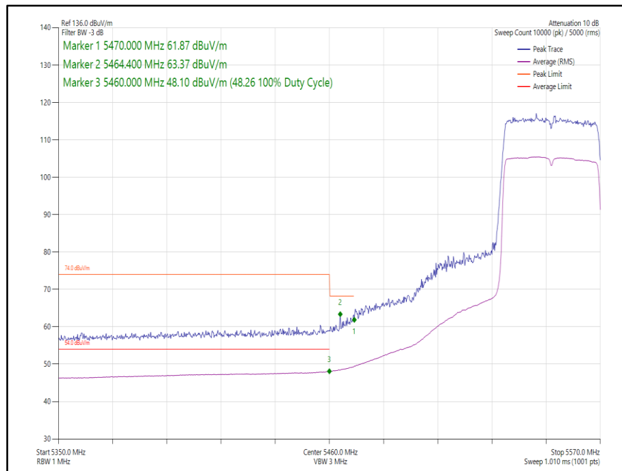
Figure 376 - 802.11ax, HE40, SU, SISO, Core 0 - 5550 MHz, Band Edge Frequency 5470 MHz
