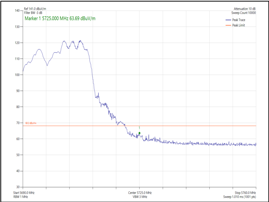
Figure 360 - 802.11ax, HE20, RU 106-54, SDM, Core 0-1 - 5700 MHz, Band Edge Frequency 5725 MHz
