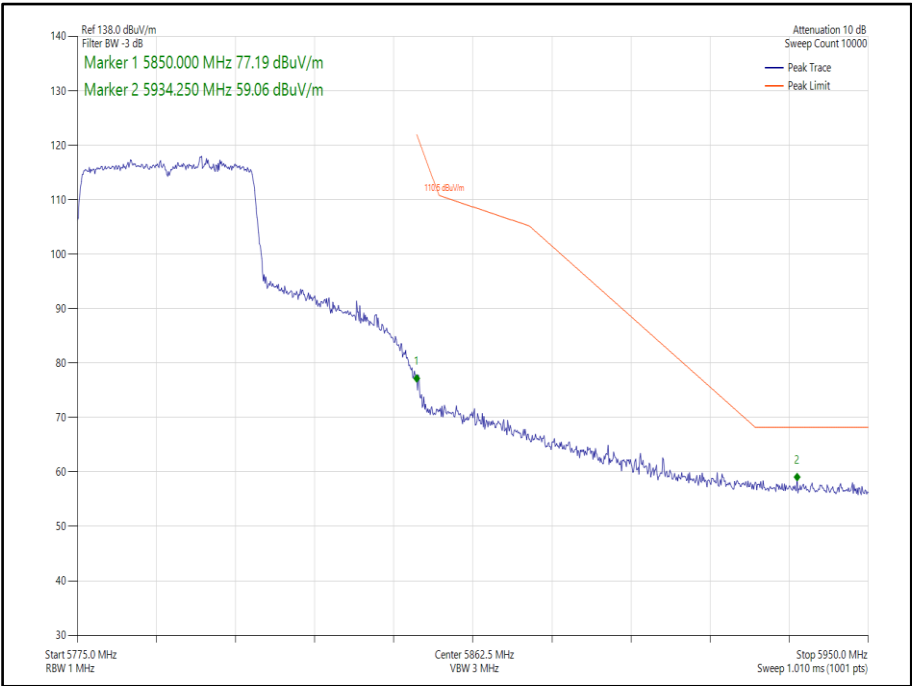
Figure 389 - 802.11ax, HE40, SU, SISO, Core 0 - 5795 MHz, Band Edge Frequency 5850 MHz
