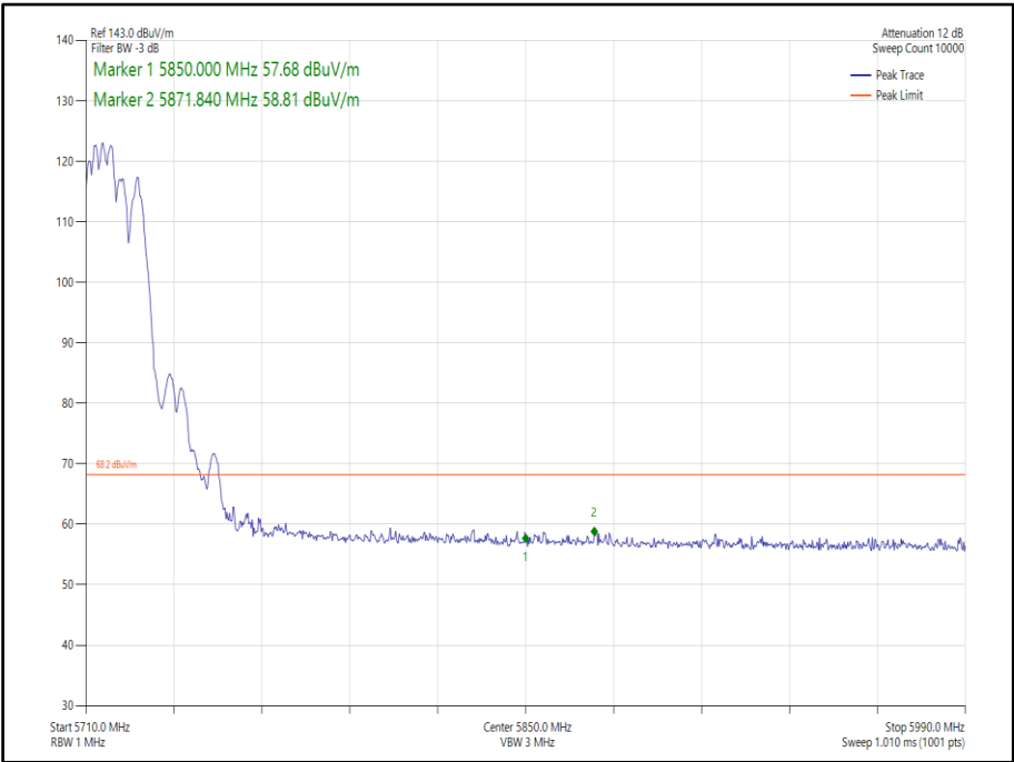
Figure 364 - 802.11ax, HE20, RU 106-53, SDM, Core 0-1 - 5720 MHz, Band Edge Frequency 5850 MHz
