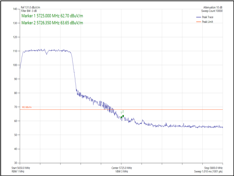
Figure 401 - 802.11n, HT40, SISO, Core 1 - 5670 MHz, Band Edge Frequency 5725 MHz
