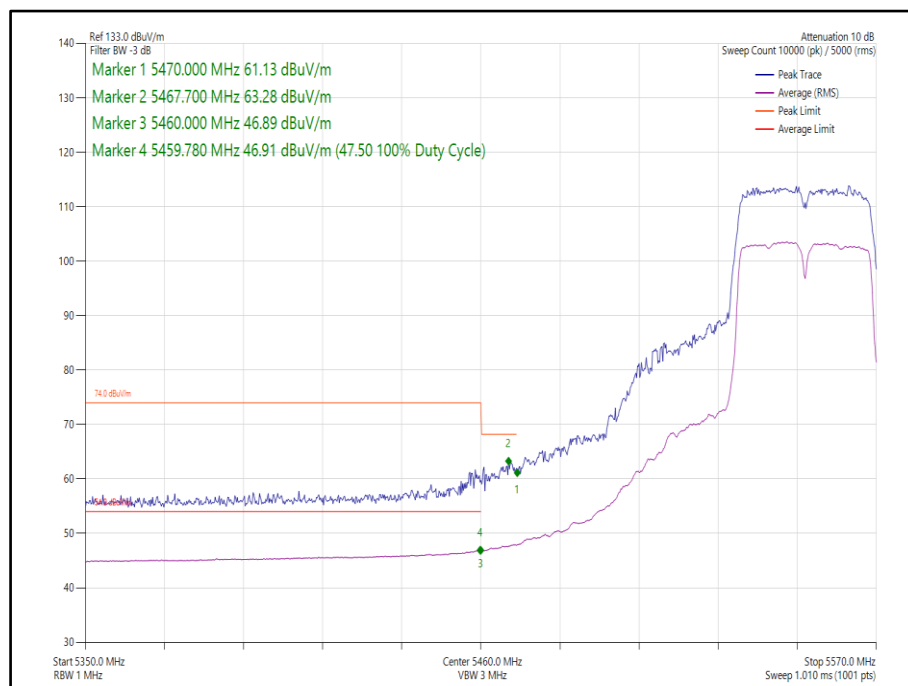
Figure 392 - 802.11n, HT40, SISO, Core 1 - 5550 MHz, Band Edge Frequency 5470 MHz
