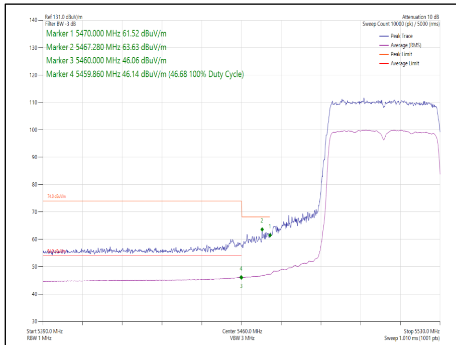
Figure 374 - 802.11ax, HE40, SU, SISO, Core 0 - 5510 MHz, Band Edge Frequency 5470 MHz
