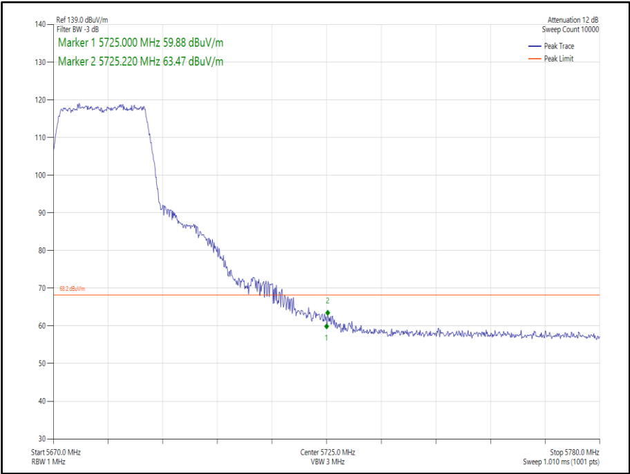
Figure 355 - 802.11n, HT20, SDM, Core 0-1 - 5680 MHz, Band Edge Frequency 5725 MHz
