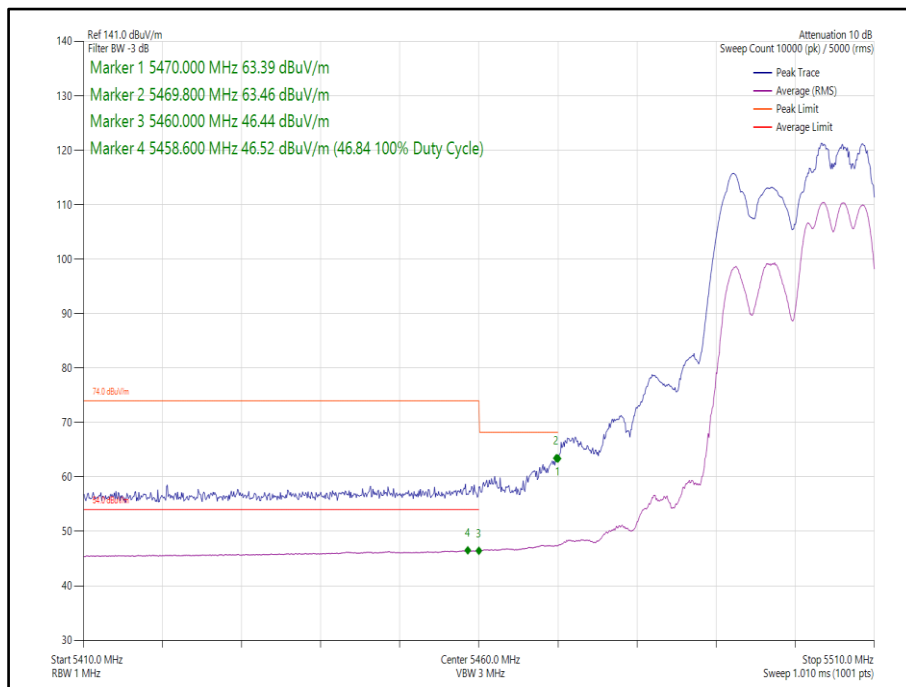
Figure 350 - 802.11ax, HE20, RU 106-54, SDM, Core 0-1 - 5500 MHz, Band Edge Frequency 5470 MHz
