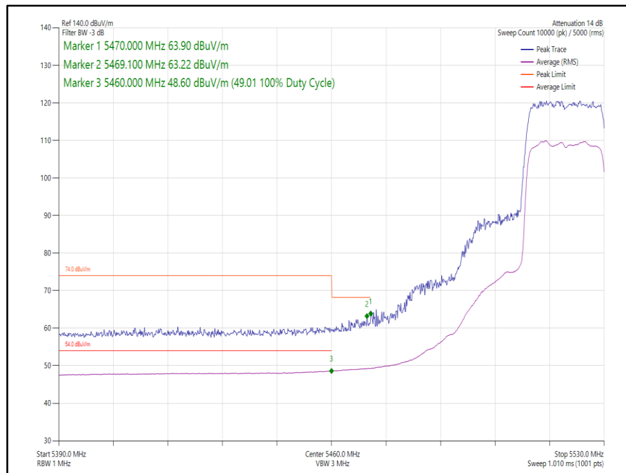
Figure 351 - 802.11ax, HE20, SU, SDM, Core 0-1 - 5520 MHz, Band Edge Frequency 5470 MHz
