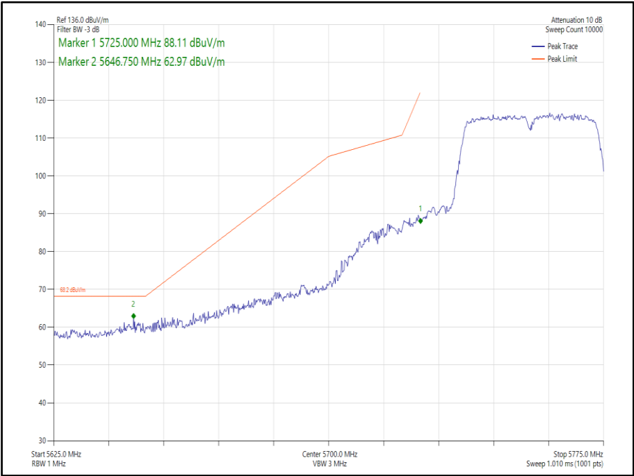
Figure 397 - 802.11n, HT40, SISO, Core 1 - 5755 MHz, Band Edge Frequency 5725 MHz
