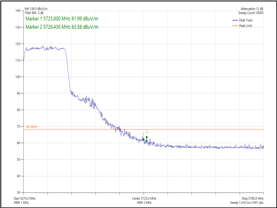
Figure 357 - 802.11ax, HE20, SU, SDM, Core 0-1 - 5680 MHz, Band Edge Frequency 5725 MHz
