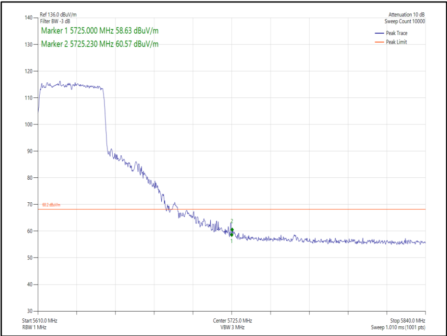
Figure 383 - 802.11ax, HE40, SU, SISO, Core 0 - 5630 MHz, Band Edge Frequency 5725 MHz
