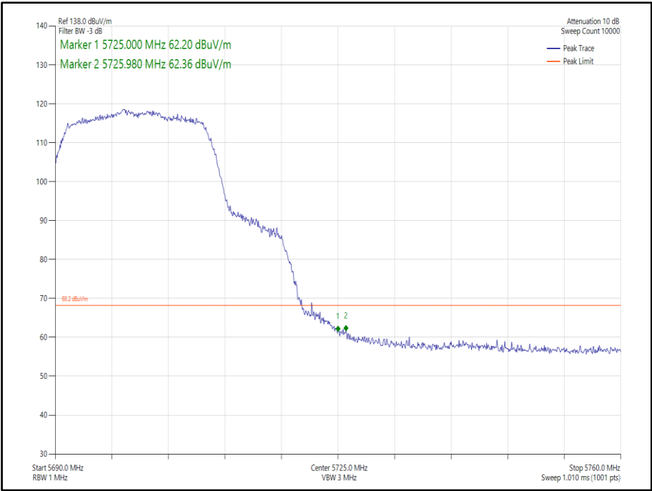
Figure 369 - 802.11ac, VHT20, TxBF, Core 0-1 - 5700 MHz, Band Edge Frequency 5725 MHz
