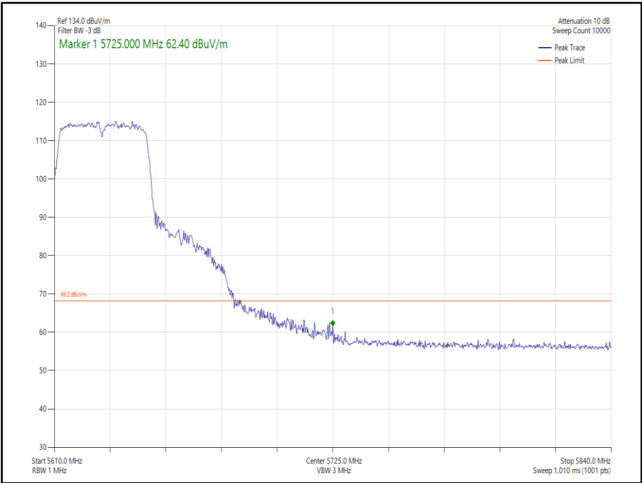
Figure 400 - 802.11n, HT40, SISO, Core 1 - 5630 MHz, Band Edge Frequency 5725 MHz
