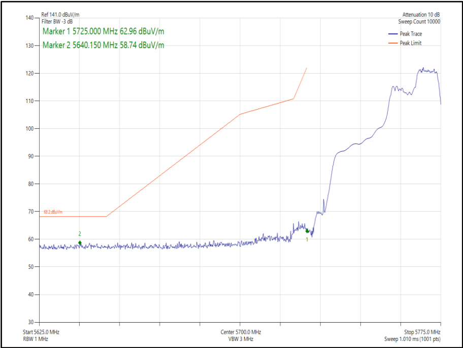
Figure 399 - 802.11ax, HE40, RU 106-56, SISO, Core 1 - 5755 MHz, Band Edge Frequency 5725 MHz
