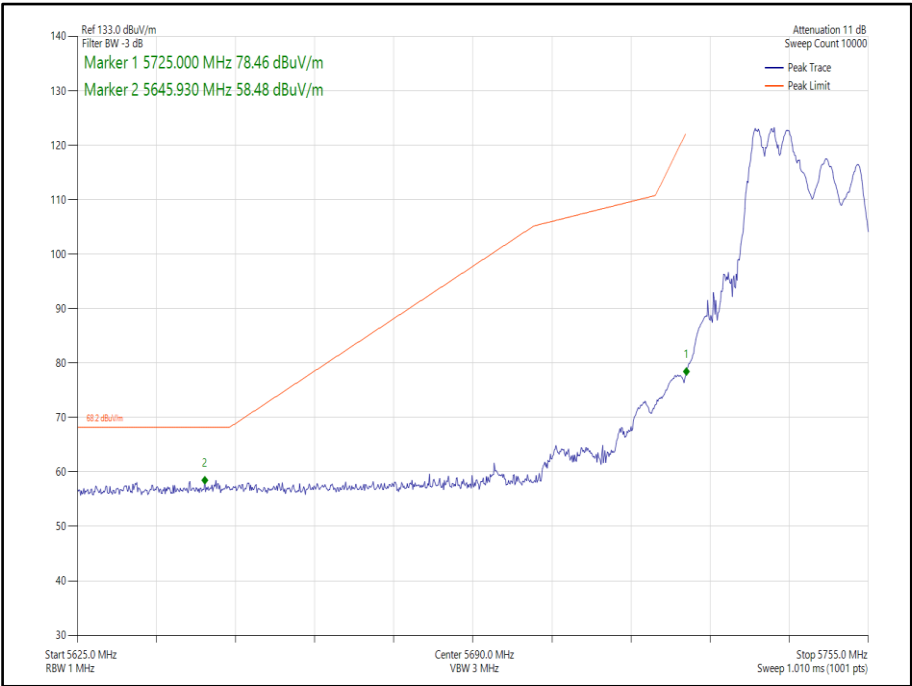
Figure 354 - 802.11ax, HE20, RU 106-53, SDM, Core 0-1 - 5745 MHz, Band Edge Frequency 5725 MHz
