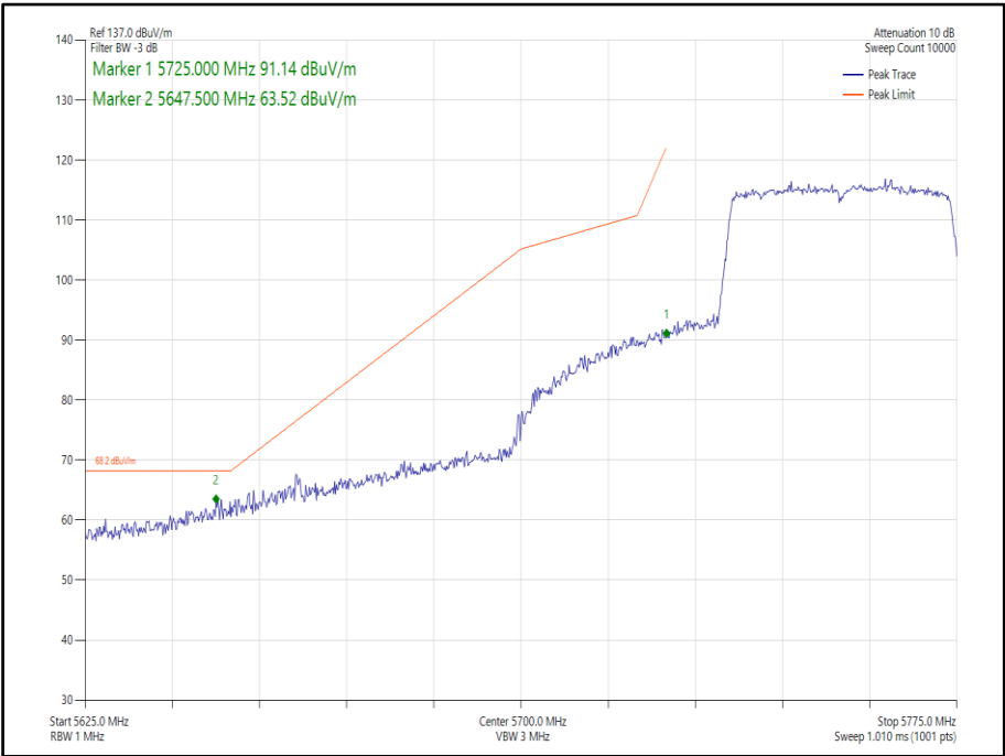
Figure 379 - 802.11ax, HE40, SU, SISO, Core 0 - 5755 MHz, Band Edge Frequency 5725 MHz
