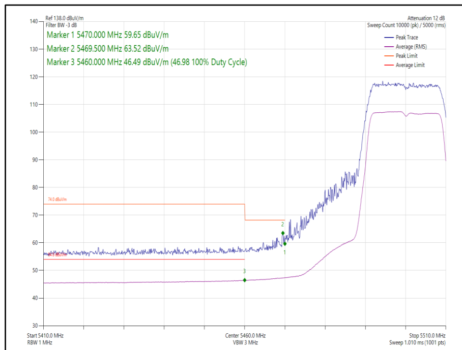
Figure 367 - 802.11ac, VHT20, TxBF, Core 0-1 - 5500 MHz, Band Edge Frequency 5470 MHz
