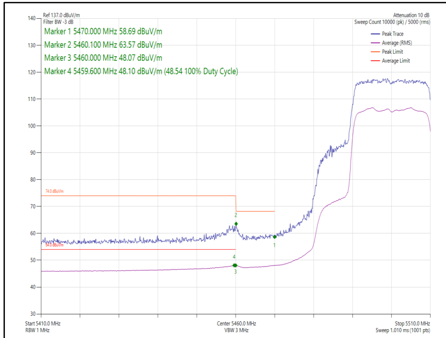
Figure 349 - 802.11ax, HE20, SU, SDM, Core 0-1 - 5500 MHz, Band Edge Frequency 5470 MHz
