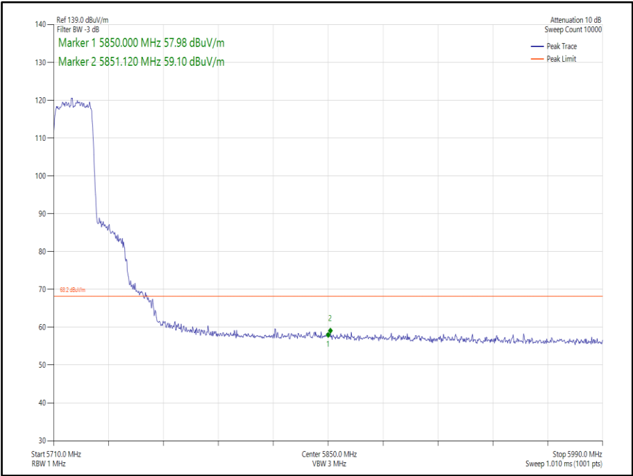
Figure 363 - 802.11ax, HE20, SU, SDM, Core 0-1 - 5720 MHz, Band Edge Frequency 5850 MHz
