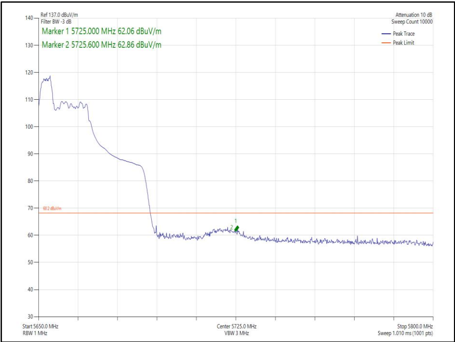
Figure 404 - 802.11ax, HE40, RU 52-37, SISO, Core 1 - 5670 MHz, Band Edge Frequency 5725 MHz
