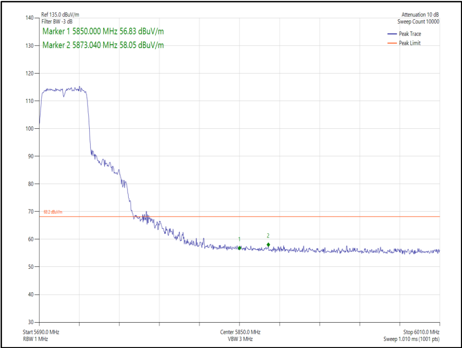
Figure 386 - 802.11n, HT40, SISO, Core 0 - 5710 MHz, Band Edge Frequency 5850 MHz
