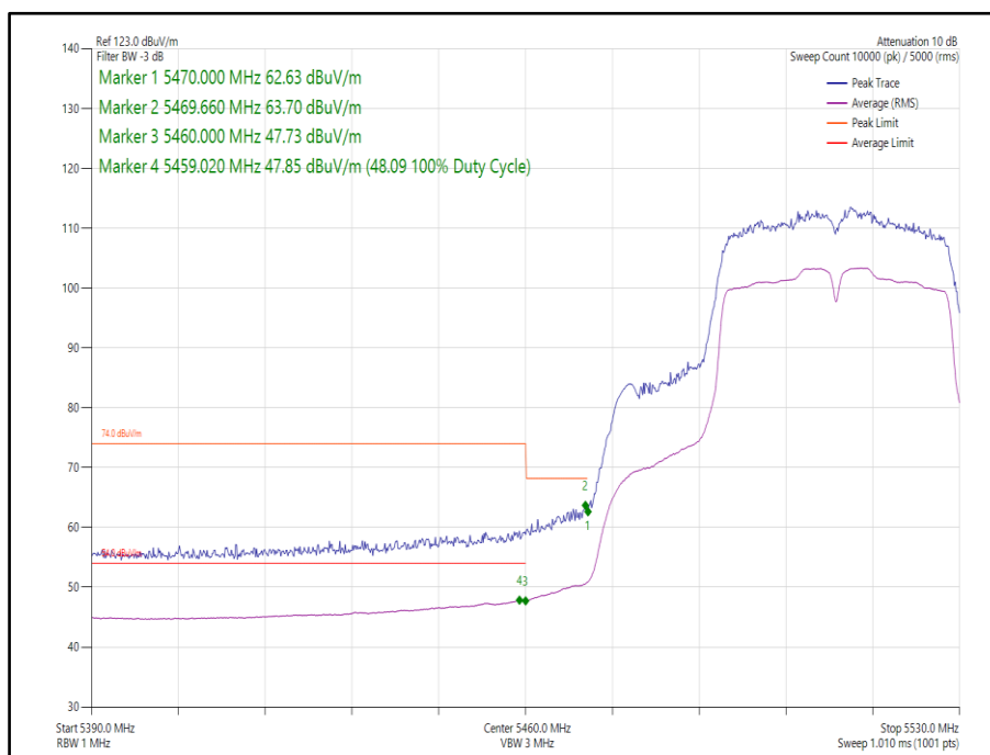
Figure 372 - 802.11n, HT40, SISO, Core 0 - 5510 MHz, Band Edge Frequency 5470 MHz
