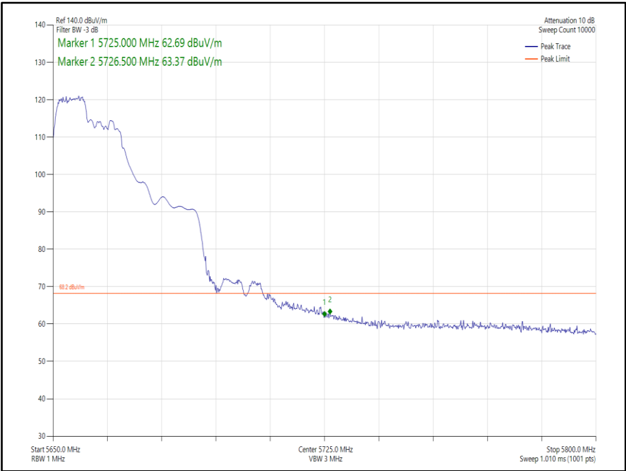
Figure 385 - 802.11ax, HE40, RU 106-53, SISO, Core 0 - 5670 MHz, Band Edge Frequency 5725 MHz
