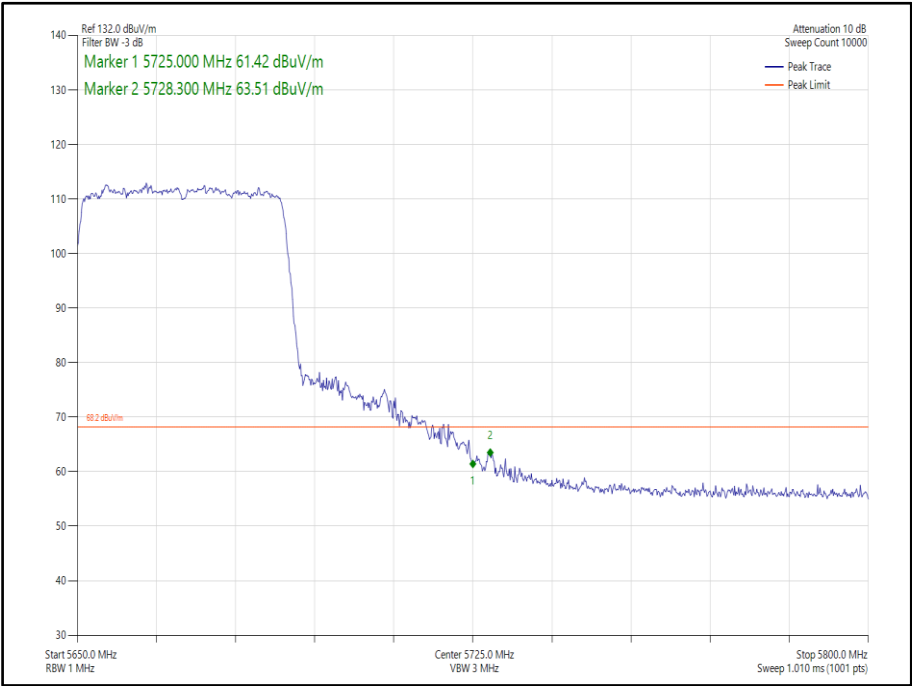
Figure 403 - 802.11ax, HE40, SU, SISO, Core 1 - 5670 MHz, Band Edge Frequency 5725 MHz
