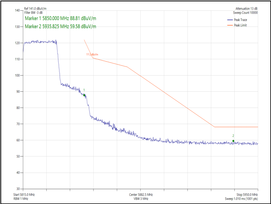
Figure 365 - 802.11ax, HE20, SU, SDM, Core 0-1 - 5825 MHz, Band Edge Frequency 5850 MHz
