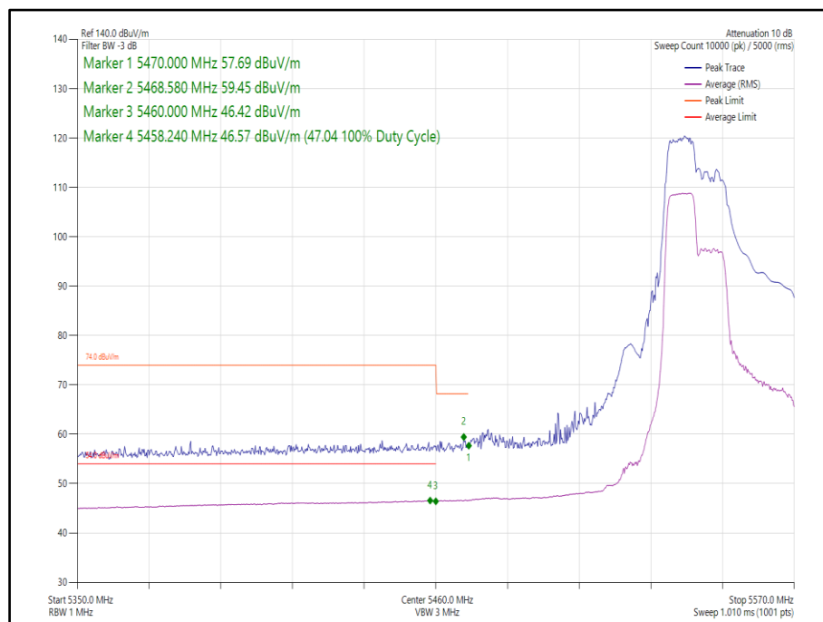
Figure 377 - 802.11ax, HE40, RU 106-53, SISO, Core 0 - 5550 MHz, Band Edge Frequency 5470 MHz
