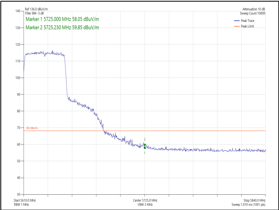
Figure 402 - 802.11ax, HE40, SU, SISO, Core 1 - 5630 MHz, Band Edge Frequency 5725 MHz
