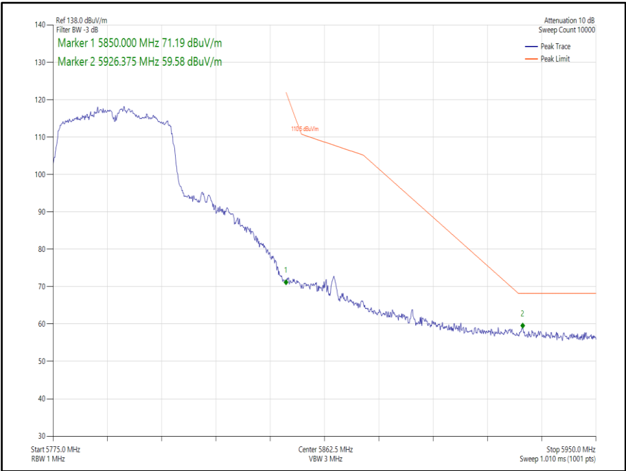
Figure 387 - 802.11n, HT40, SISO, Core 0 - 5795 MHz, Band Edge Frequency 5850 MHz
