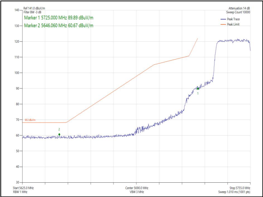
Figure 353 - 802.11ax, HE20, SU, SDM, Core 0-1 - 5745 MHz, Band Edge Frequency 5725 MHz
