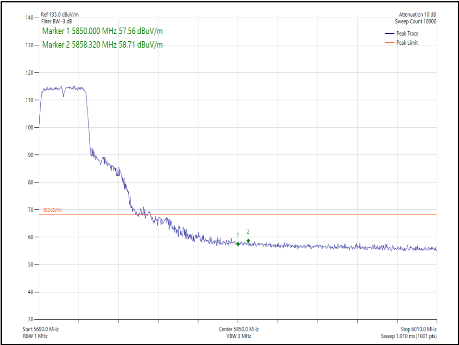
Figure 405 - 802.11n, HT40, SISO, Core 1 - 5710 MHz, Band Edge Frequency 5850 MHz
