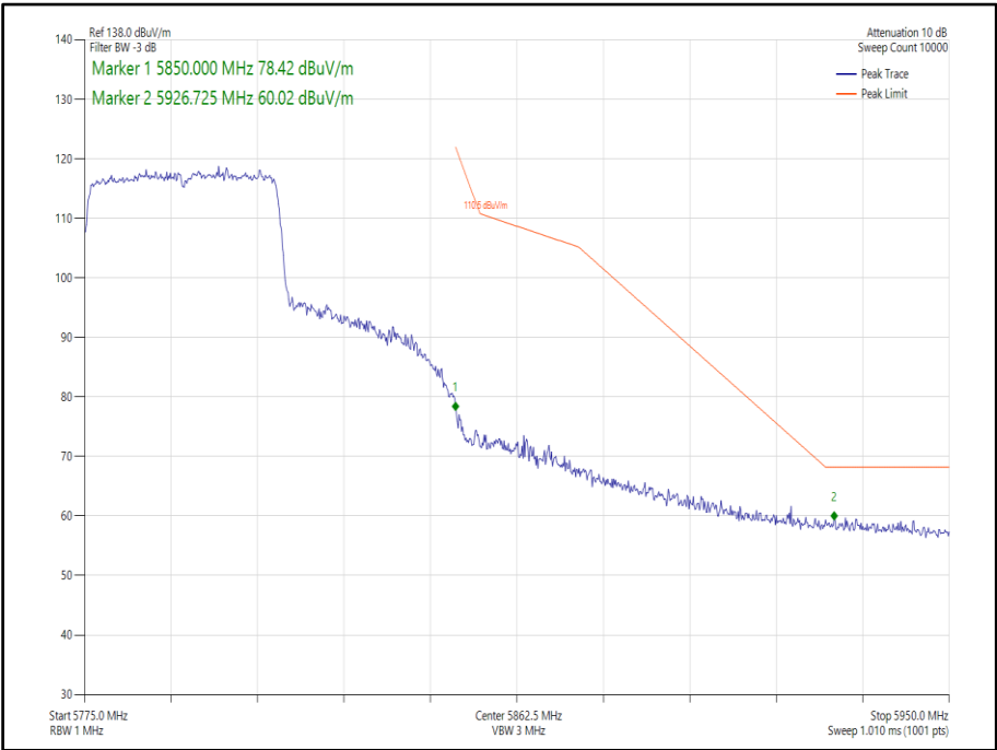
Figure 408 - 802.11ax, HE40, SU, SISO, Core 1 - 5795 MHz, Band Edge Frequency 5850 MHz
