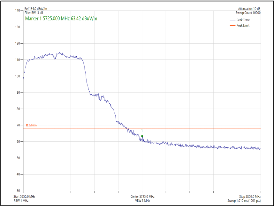
Figure 382 - 802.11n, HT40, SISO, Core 0 - 5670 MHz, Band Edge Frequency 5725 MHz
