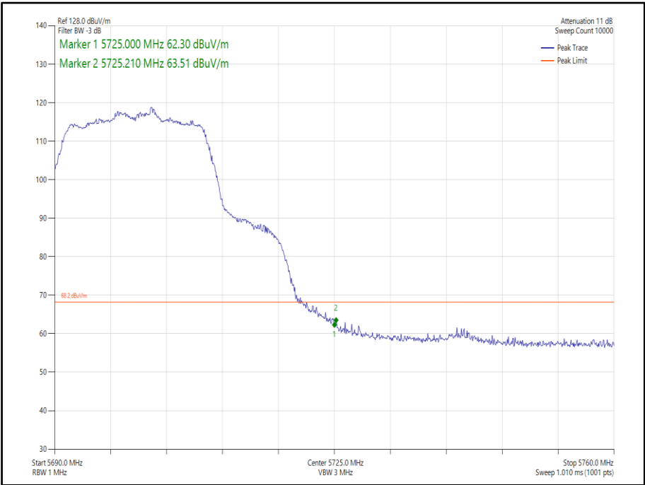
Figure 356 - 802.11n, HT20, SDM, Core 0-1 - 5700 MHz, Band Edge Frequency 5725 MHz
