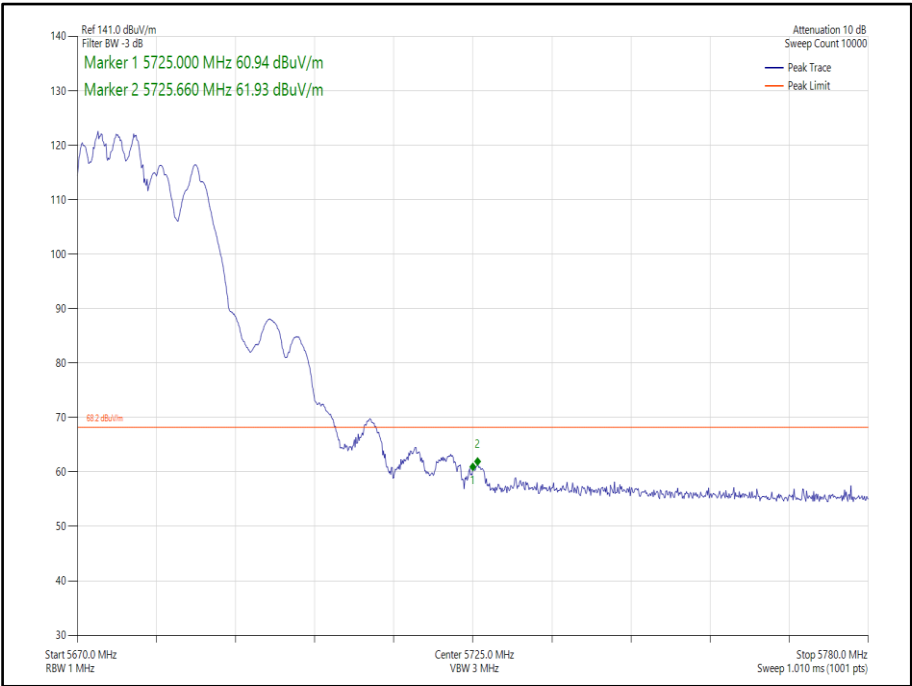
Figure 358 - 802.11ax, HE20, RU 106-53, SDM, Core 0-1 - 5680 MHz, Band Edge Frequency 5725 MHz
