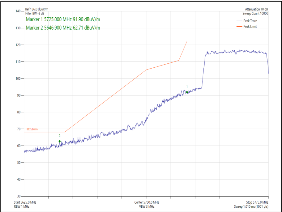
Figure 398 - 802.11ax, HE40, SU, SISO, Core 1 - 5755 MHz, Band Edge Frequency 5725 MHz
