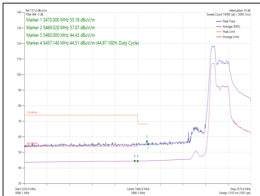
Figure 396 - 802.11ax, HE40, RU 52-37, SISO, Core 1 - 5550 MHz, Band Edge Frequency 5470 MHz
