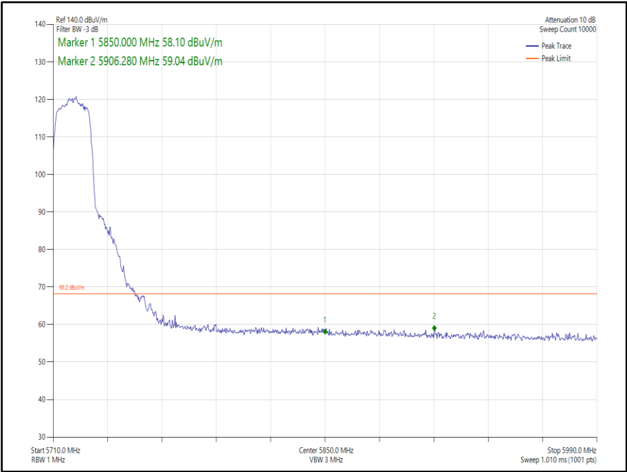
Figure 361 - 802.11n, HT20, SDM, Core 0-1 - 5720 MHz, Band Edge Frequency 5850 MHz
