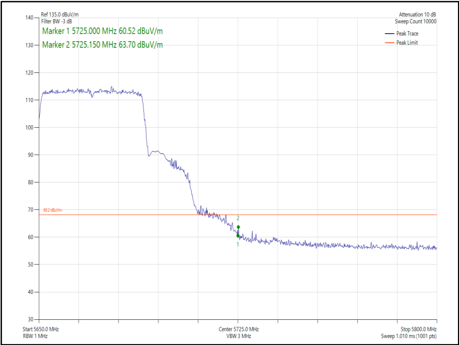
Figure 384 - 802.11ax, HE40, SU, SISO, Core 0 - 5670 MHz, Band Edge Frequency 5725 MHz
