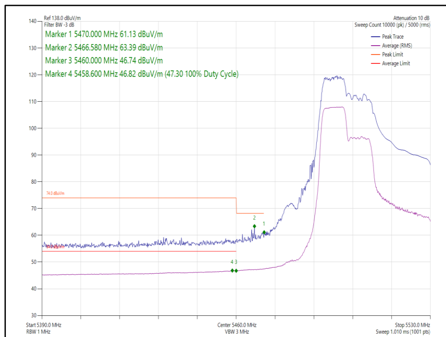
Figure 375 - 802.11ax, HE40, RU 106-53, SISO, Core 0 - 5510 MHz, Band Edge Frequency 5470 MHz
