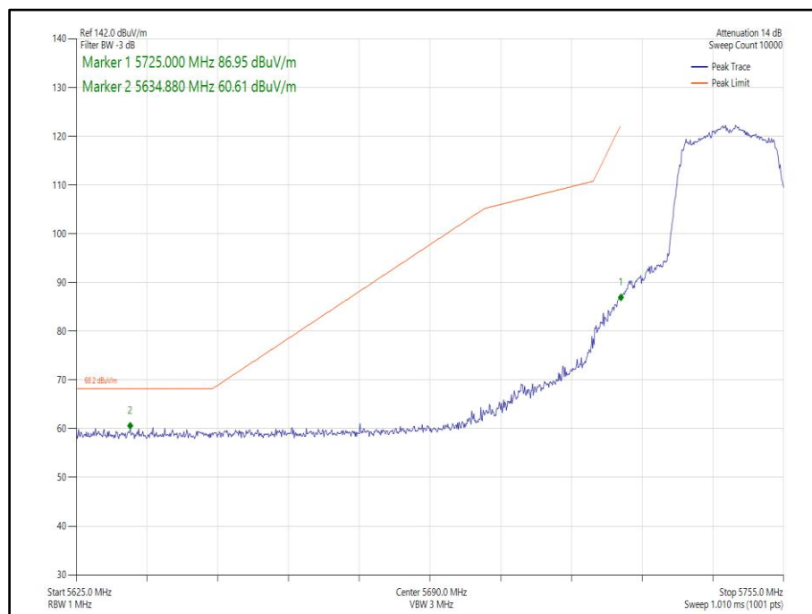
Figure 352 - 802.11n, HT20, SDM, Core 0-1 - 5745 MHz, Band Edge Frequency 5725 MHz
