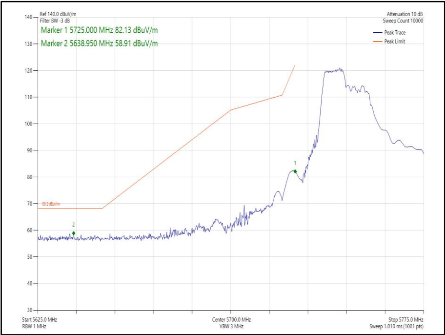
Figure 380 - 802.11ax, HE40, RU 106-53, SISO, Core 0 - 5755 MHz, Band Edge Frequency 5725 MHz
