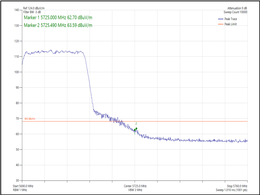
Figure 359 - 802.11ax, HE20, SU, SDM, Core 0-1 - 5700 MHz, Band Edge Frequency 5725 MHz
