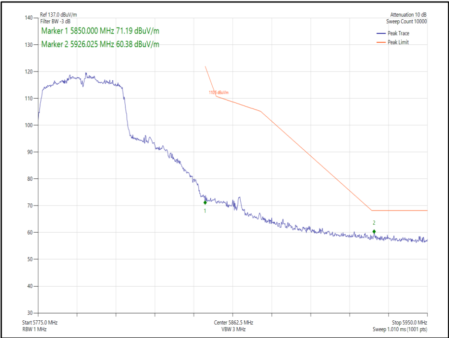
Figure 406 - 802.11n, HT40, SISO, Core 1 - 5795 MHz, Band Edge Frequency 5850 MHz
