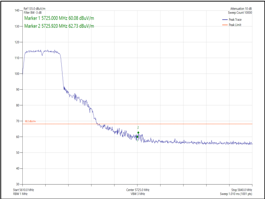
Figure 381 - 802.11n, HT40, SISO, Core 0 - 5630 MHz, Band Edge Frequency 5725 MHz
