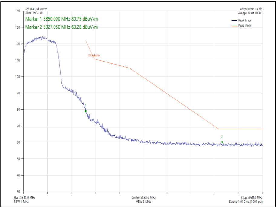
Figure 371 - 802.11ac, VHT20, TxBF, Core 0-1 - 5825 MHz, Band Edge Frequency 5850 MHz
