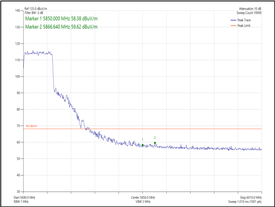
Figure 407 - 802.11ax, HE40, SU, SISO, Core 1 - 5710 MHz, Band Edge Frequency 5850 MHz
