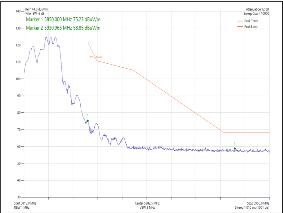
Figure 366 - 802.11ax, HE20, RU 106-54, SDM, Core 0-1 - 5825 MHz, Band Edge Frequency 5850 MHz
