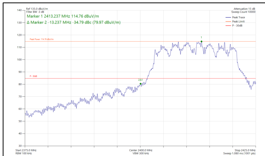
Figure 87 - 802.11n HT20, CDD, Core 0 + Core 1 - 2412 MHz Band Edge Frequency 2400 MHz
