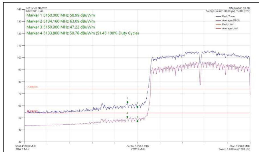
Figure 206 - 802.11ac VHT160, CDD, Core 0 + Core 1 - 5250 MHz Band Edge Frequency 5150 MHz
