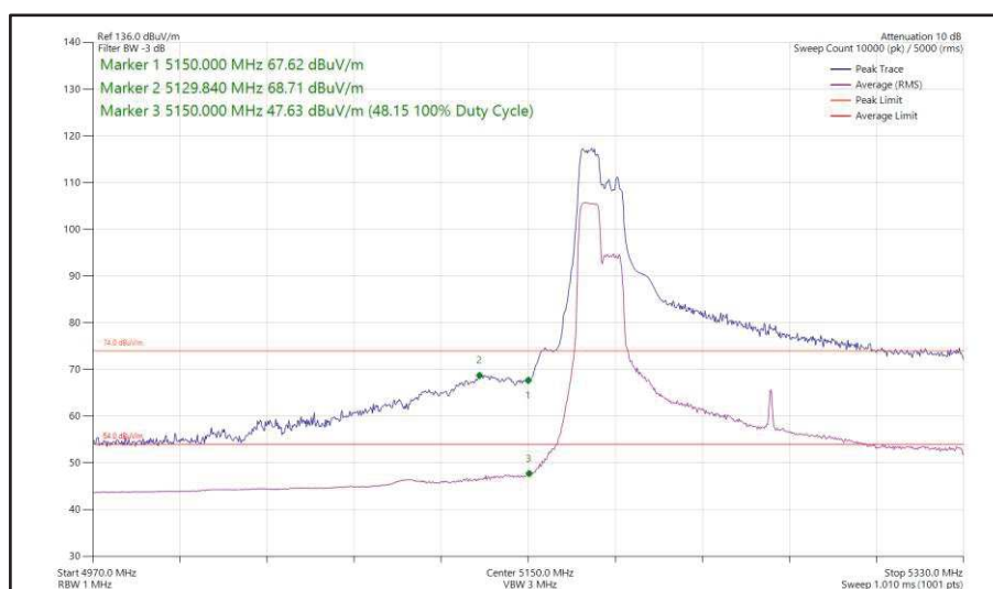
Figure 190 - 802.11ax HE160, RU 106-53, SISO, Core 0 - 5250 MHz Band Edge Frequency 5150 MHz
