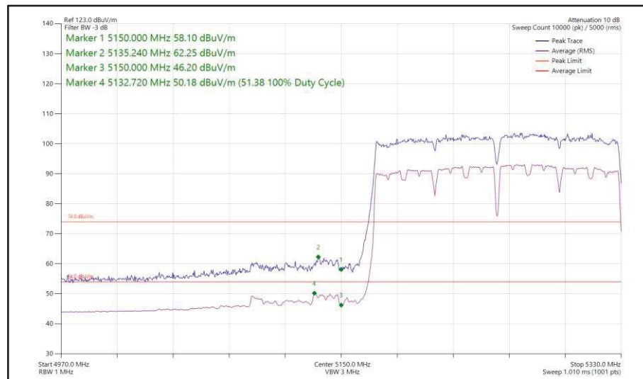
Figure 197 - 802.11ac VHT160, SISO, Core 1 - 5250 MHz Band Edge Frequency 5150 MHz
