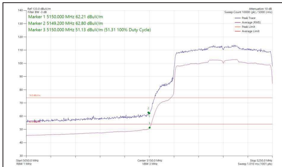
Figure 159 - 802.11ax HE80, SU, SISO, Core 1 - 5210 MHz Band Edge Frequency 5150 MHz
