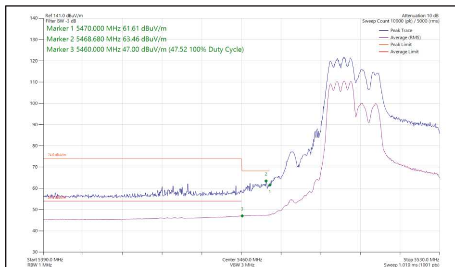
Figure 141 - 802.11ax HE40, RU 106-53, SDM, Core 0 + Core 1 - 5510 MHz Band Edge Frequency 5460 MHz
