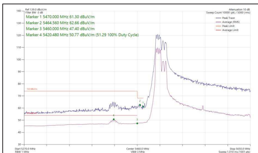
Figure 223 - 802.11ax HE160, RU 106-53, SDM, Core 0 + Core 1 - 5570 MHz Band Edge Frequency 5460 MHz
