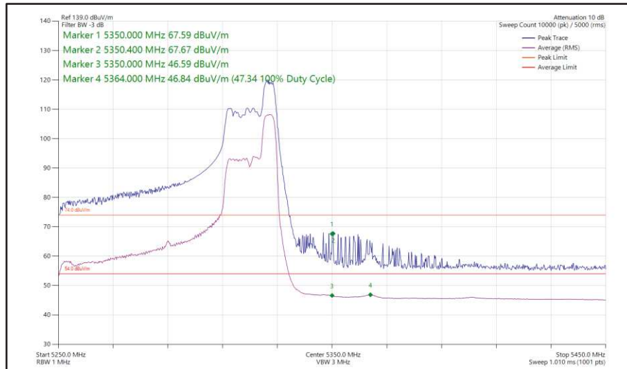
Figure 154 - 802.11ax HE80, RU 52-52, SISO, Core 0 - 5290 MHz Band Edge Frequency 5350 MHz
