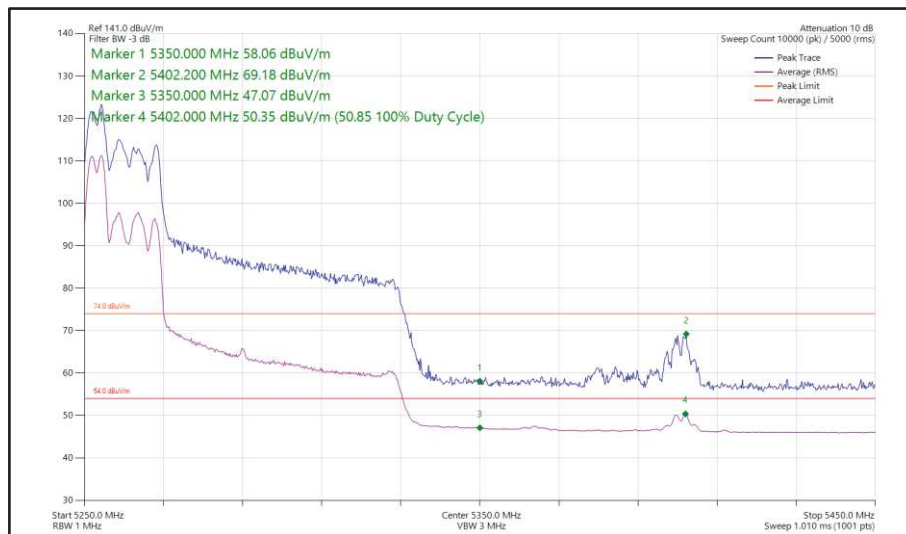
Figure 181 - 802.11ax HE80, RU 52-37, SDM, Core 0 + Core 1 - 5290 MHz Band Edge Frequency 5350 MHz
