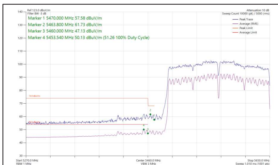
Figure 221 - 802.11ac VHT160, SDM, Core 0 + Core 1 - 5570 MHz Band Edge Frequency 5460 MHz
