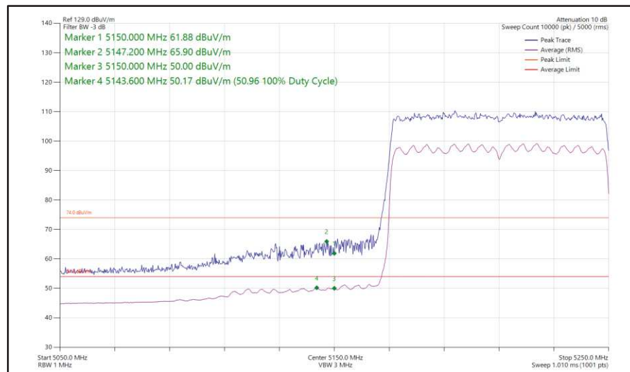
Figure 177 - 802.11ax HE80, SU, SDM, Core 0 + Core 1 - 5210 MHz Band Edge Frequency 5150 MHz
