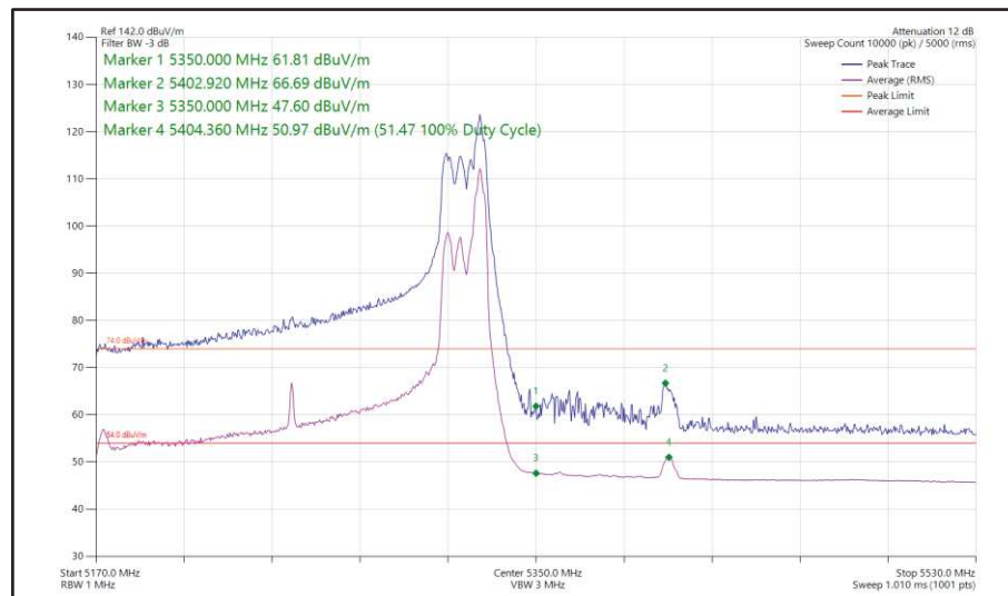
Figure 211 - 802.11ax HE160, RU 52-52, CDD, Core 0 + Core 1 - 5250 MHz Band Edge Frequency 5350 MHz
