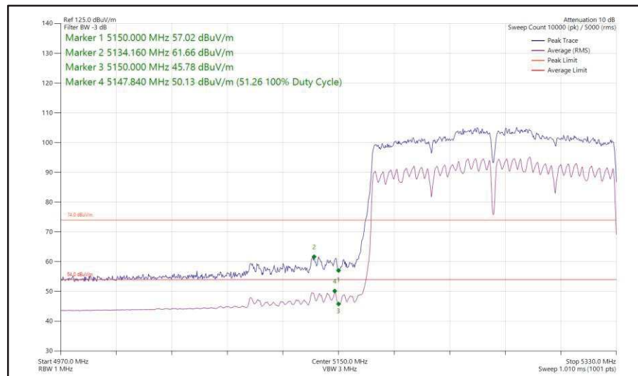
Figure 215 - 802.11ac VHT160, SDM, Core 0 + Core 1 - 5250 MHz Band Edge Frequency 5150 MHz
