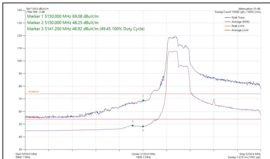
Figure 160 - 802.11ax HE80, RU 106-53, SISO, Core 1 - 5210 MHz Band Edge Frequency 5150 MHz
