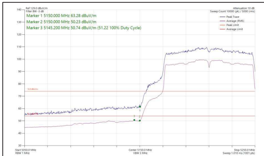
Figure 149 - 802.11ac VHT80, SISO, Core 0 - 5210 MHz Band Edge Frequency 5150 MHz
