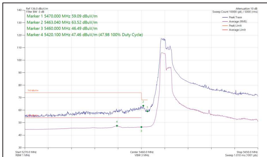
Figure 196 - 802.11ax HE160, RU 106-53, SISO, Core 0 - 5570 MHz Band Edge Frequency 5460 MHz
