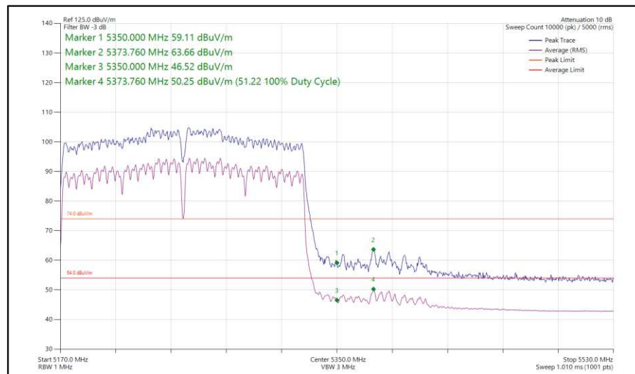
Figure 209 - 802.11ac VHT160, CDD, Core 0 + Core 1 - 5250 MHz Band Edge Frequency 5350 MHz
