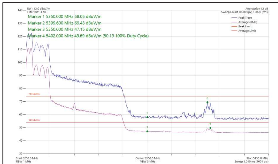
Figure 172 - 802.11ax HE80, RU 52-37, CDD, Core 0 + Core 1 - 5290 MHz Band Edge Frequency 5350 MHz
