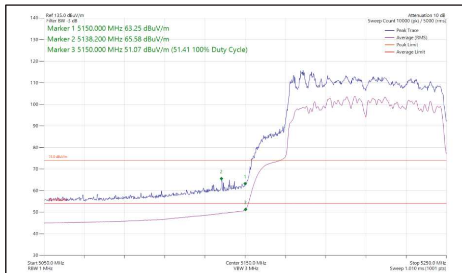
Figure 185 - 802.11ac VHT80, TxBF, Core 0 + Core 1 - 5210 MHz Band Edge Frequency 5150 MHz
