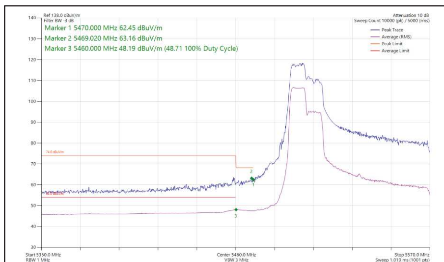
Figure 157 - 802.11ax HE80, RU 106-53, SISO, Core 0 - 5530 MHz Band Edge Frequency 5460 MHz
