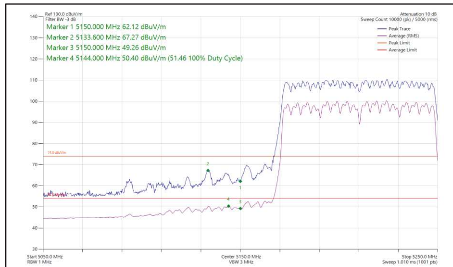
Figure 167 - 802.11ac VHT80, CDD, Core 0 + Core 1 - 5210 MHz Band Edge Frequency 5150 MHz
