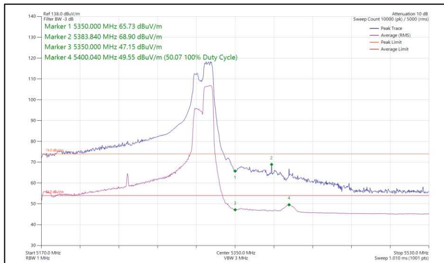
Figure 202 - 802.11ax HE160, RU 106-60, SISO, Core 1 - 5250 MHz Band Edge Frequency 5350 MHz
