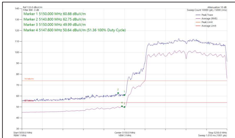
Figure 176 - 802.11ac VHT80, SDM, Core 0 + Core 1 - 5210 MHz Band Edge Frequency 5150 MHz
