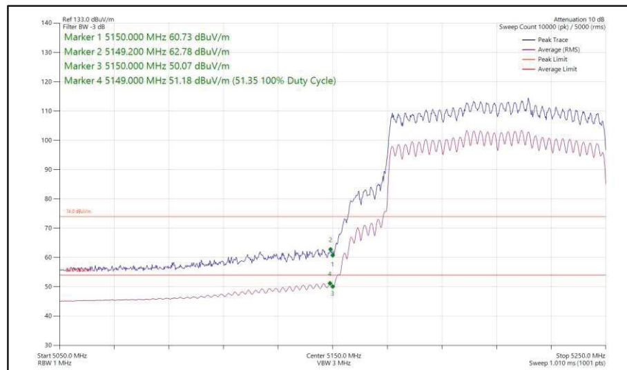
Figure 168 - 802.11ax HE80, SU, CDD, Core 0 + Core 1 - 5210 MHz Band Edge Frequency 5150 MHz
