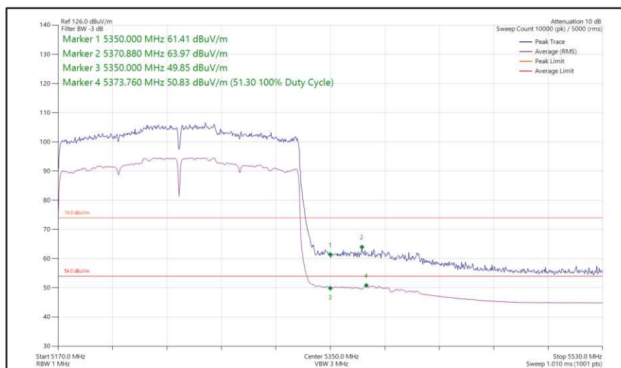
Figure 201 - 802.11ax HE160, SU, SISO, Core 1 - 5250 MHz Band Edge Frequency 5350 MHz
