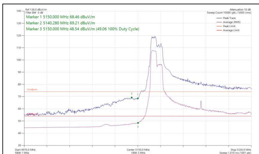
Figure 199 - 802.11ax HE160, RU 106-53, SISO, Core 1 - 5250 MHz Band Edge Frequency 5150 MHz
