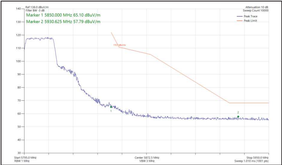
Figure 427 - 802.11n HT20, SDM, Core 0 + Core 1 - 5805 MHz Band Edge Frequency 5850 MHz
