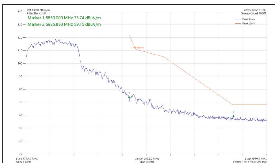
Figure 495 - 802.11n HT40, CDD, Core 0 + Core 1 - 5795 MHz Band Edge Frequency 5850 MHz
