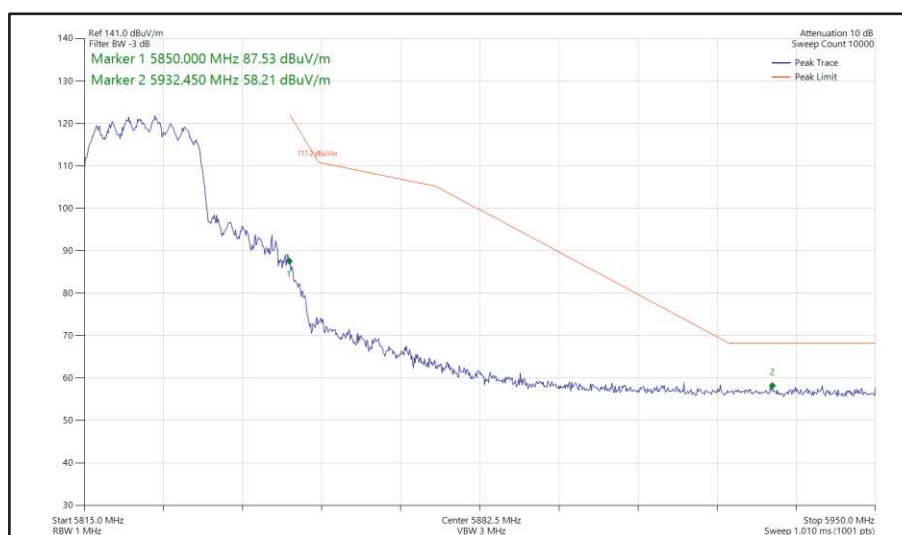
Figure 409 - 802.11ax HE20, SU, CDD, Core 0 + Core 1 - 5825 MHz Band Edge Frequency 5850 MHz
