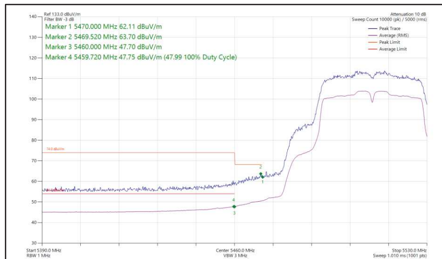
Figure 443 - 802.11n HT40, SISO, Core 0 - 5510 MHz Band Edge Frequency 5470 MHz
