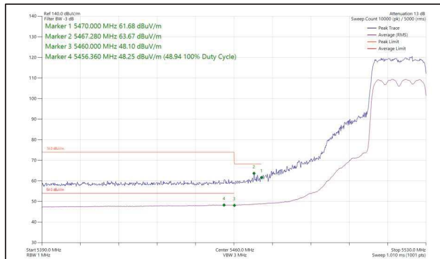
Figure 415 - 802.11ax HE20, SU, SDM, Core 0 + Core 1 - 5520 MHz Band Edge Frequency 5470 MHz
