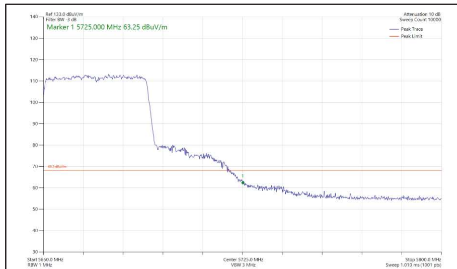
Figure 511 - 802.11ax HE40, SU, SDM, Core 0 + Core 1 - 5670 MHz Band Edge Frequency 5725 MHz
