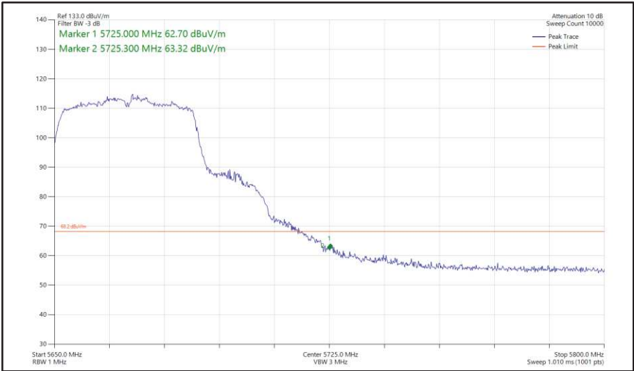
Figure 471 - 802.11n HT40, SISO, Core 1 - 5670 MHz Band Edge Frequency 5725 MHz
