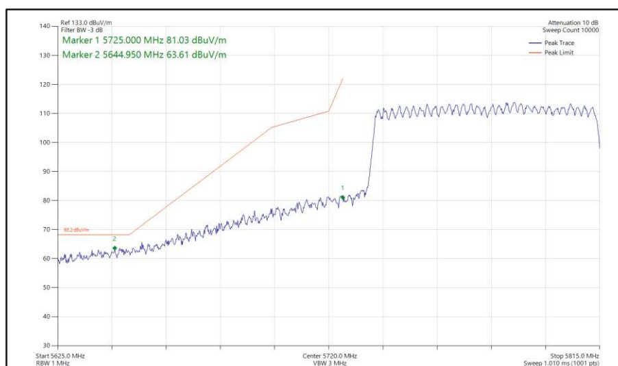
Figure 560 - 802.11ax HE80, SU, CDD, Core 0 + Core 1 - 5775 MHz Band Edge Frequency 5725 MHz
