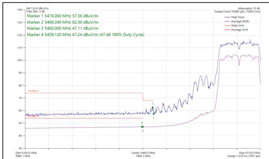
Figure 520 - 802.11ac VHT40, TxBF, Core 0 + Core 1 - 5550 MHz Band Edge Frequency 5470 MHz
