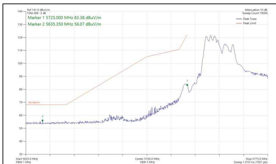
Figure 507 - 802.11ax HE40, RU 106-53, SDM, Core 0 + Core 1 - 5755 MHz Band Edge Frequency 5725 MHz
