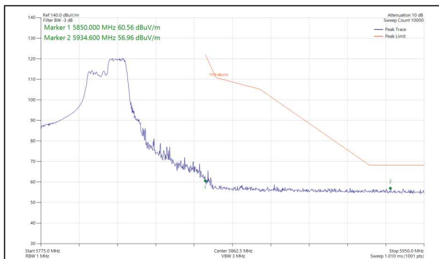
Figure 480 - 802.11ax HE40, RU 106-56, SISO, Core 1 - 5795 MHz Band Edge Frequency 5850 MHz
