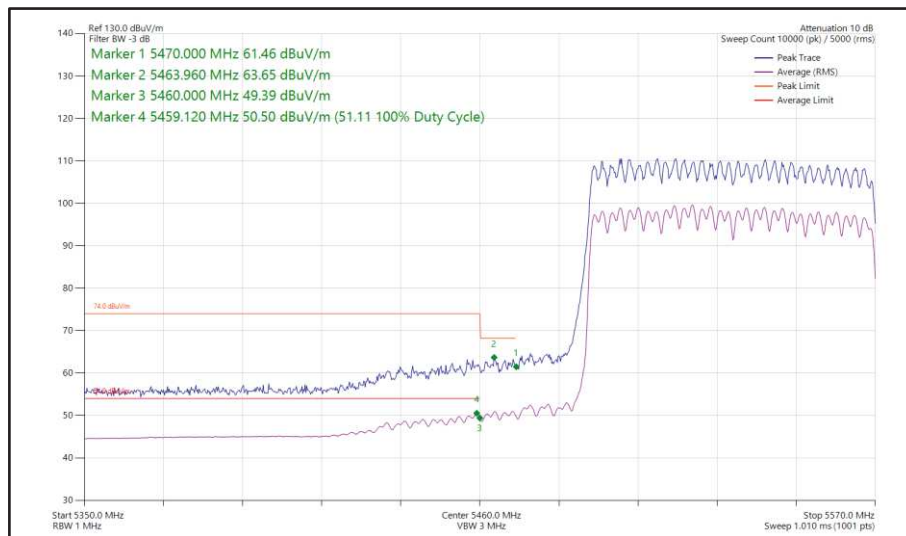
Figure 557 - 802.11ax HE80, SU, CDD, Core 0 + Core 1 - 5530 MHz Band Edge Frequency 5470 MHz
