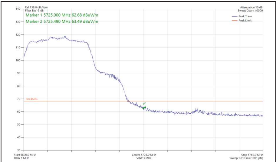
Figure 422 - 802.11n HT20, SDM, Core 0 + Core 1 - 5700 MHz Band Edge Frequency 5725 MHz
