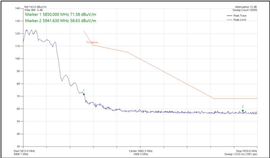
Figure 410 - 802.11ax HE20, RU 106-53, CDD, Core 0 + Core 1 - 5825 MHz Band Edge Frequency 5850 MHz
