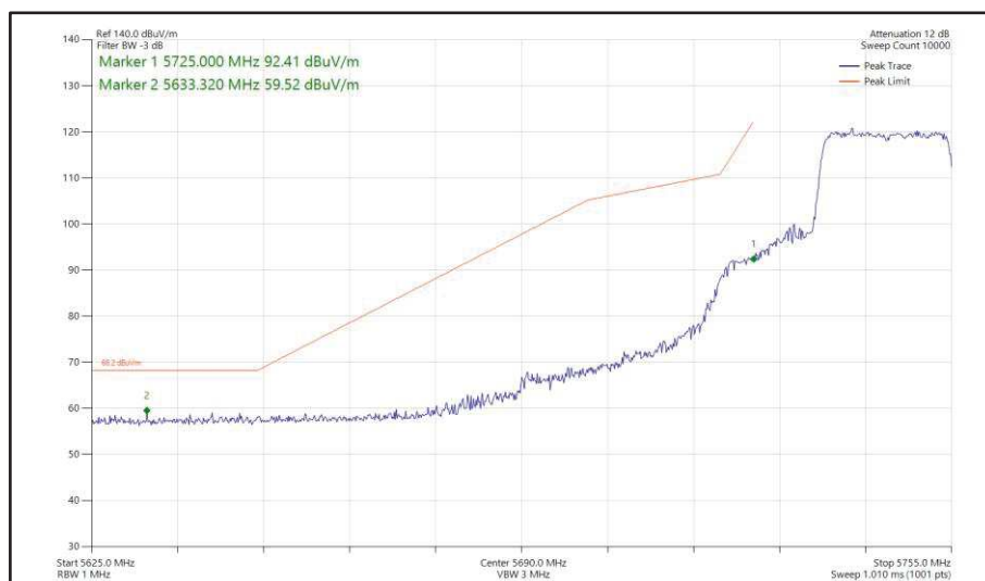
Figure 418 - 802.11ax HE20, SU, SDM, Core 0 + Core 1 - 5745 MHz Band Edge Frequency 5725 MHz
