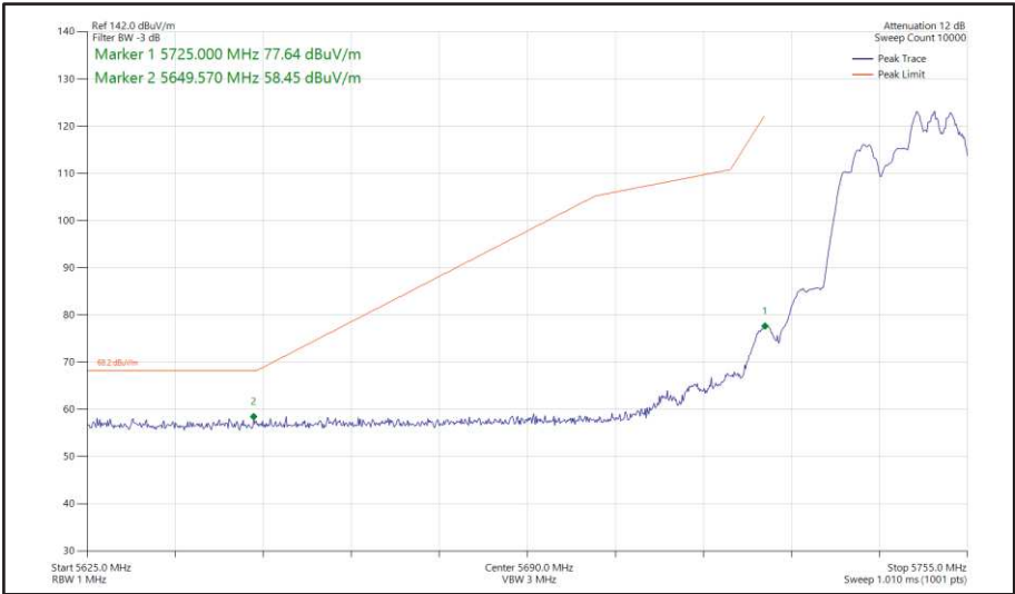
Figure 419 - 802.11ax HE20, RU 106-54, SDM, Core 0 + Core 1 - 5745 MHz Band Edge Frequency 5725 MHz
