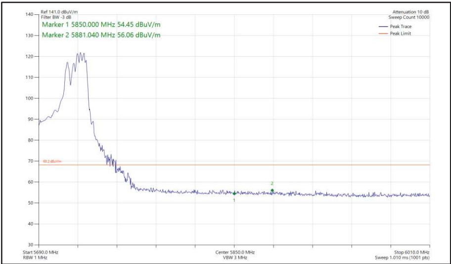
Figure 516 - 802.11ax HE40, RU 106-56, SDM, Core 0 + Core 1 - 5710 MHz Band Edge Frequency 5850 MHz
