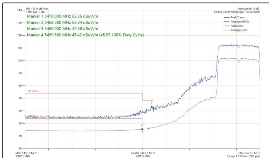
Figure 466 - 802.11ax HE40, SU, SISO, Core 1 - 5550 MHz Band Edge Frequency 5470 MHz
