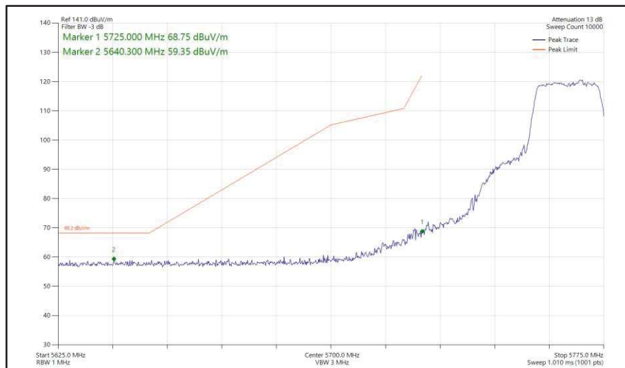
Figure 417 - 802.11n HT20, SDM, Core 0 + Core 1 - 5765 MHz Band Edge Frequency 5725 MHz
