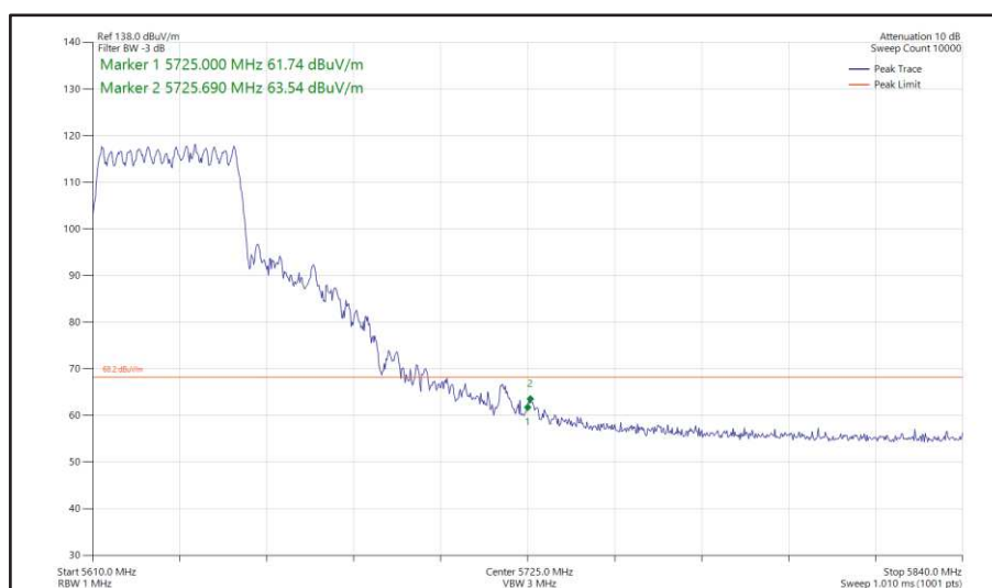
Figure 491 - 802.11ax HE40, SU, CDD, Core 0 + Core 1 - 5630 MHz Band Edge Frequency 5725 MHz
