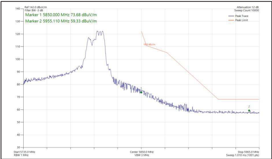
Figure 570 - 802.11ax HE80, RU 106-60, CDD, Core 0 + Core 1 - 5775 MHz Band Edge Frequency 5850 MHz
