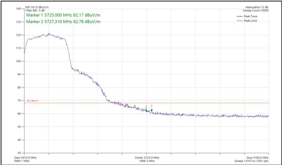
Figure 421 - 802.11n HT20, SDM, Core 0 + Core 1 - 5680 MHz Band Edge Frequency 5725 MHz
