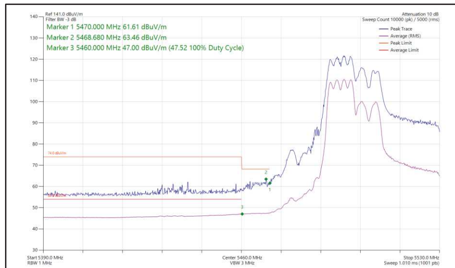
Figure 503 - 802.11ax HE40, RU 106-53, SDM, Core 0 + Core 1 - 5510 MHz Band Edge Frequency 5470 MHz
