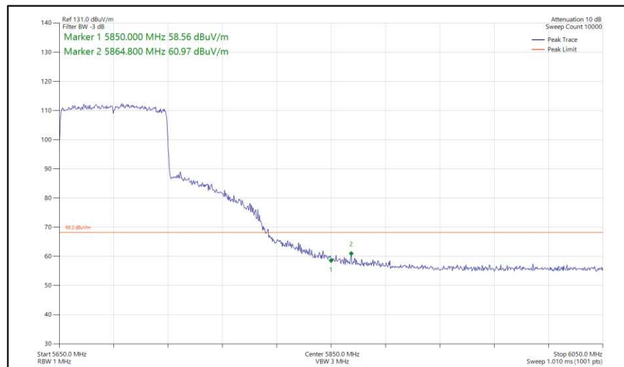
Figure 537 - 802.11ax HE80, SU, SISO, Core 0 - 5690 MHz Band Edge Frequency 5850 MHz
