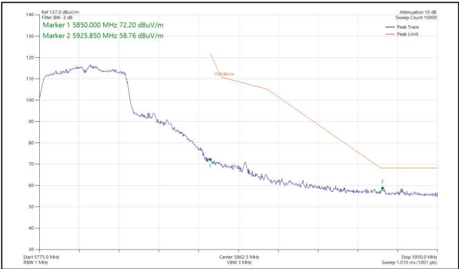
Figure 476 - 802.11n HT40, SISO, Core 1 - 5795 MHz Band Edge Frequency 5850 MHz
