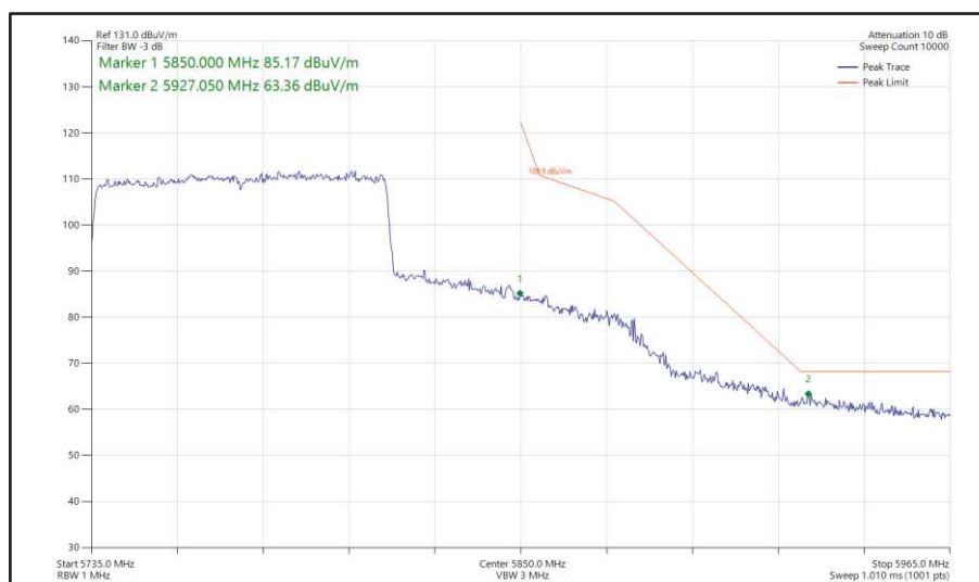
Figure 539 - 802.11ax HE80, SU, SISO, Core 0 - 5775 MHz Band Edge Frequency 5850 MHz
