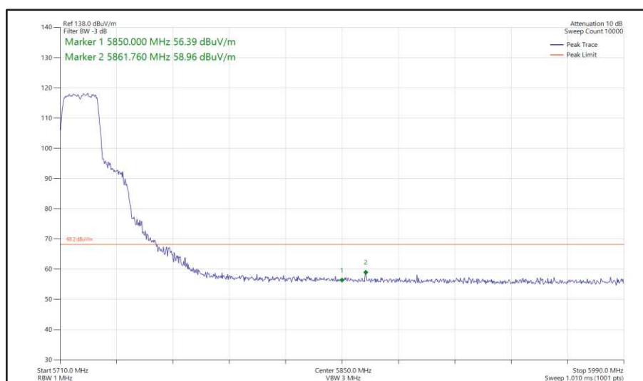
Figure 426 - 802.11n HT20, SDM, Core 0 + Core 1 - 5720 MHz Band Edge Frequency 5850 MHz
