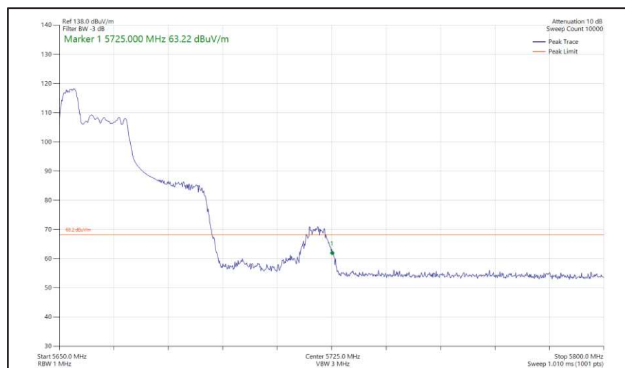
Figure 474 - 802.11ax HE40, RU 52-37, SISO, Core 1 - 5670 MHz Band Edge Frequency 5725 MHz
