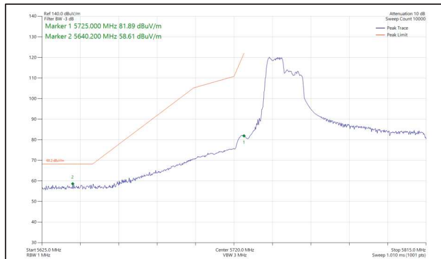
Figure 546 - 802.11ax HE80, RU 106-53, SISO, Core 1 - 5775 MHz Band Edge Frequency 5725 MHz
