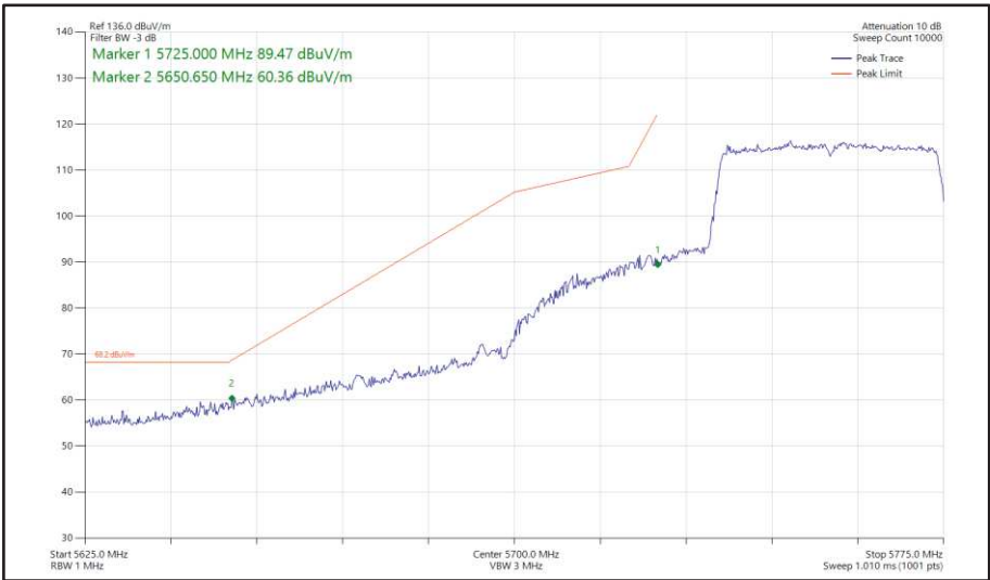
Figure 468 - 802.11ax HE40, SU, SISO, Core 1 - 5755 MHz Band Edge Frequency 5725 MHz
