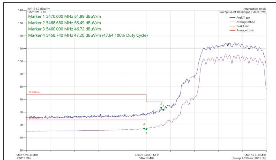
Figure 481 - 802.11n HT40, CDD, Core 0 + Core 1 - 5510 MHz Band Edge Frequency 5470 MHz
