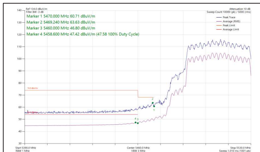
Figure 483 - 802.11ax HE40, SU, CDD, Core 0 + Core 1 - 5510 MHz Band Edge Frequency 5470 MHz
