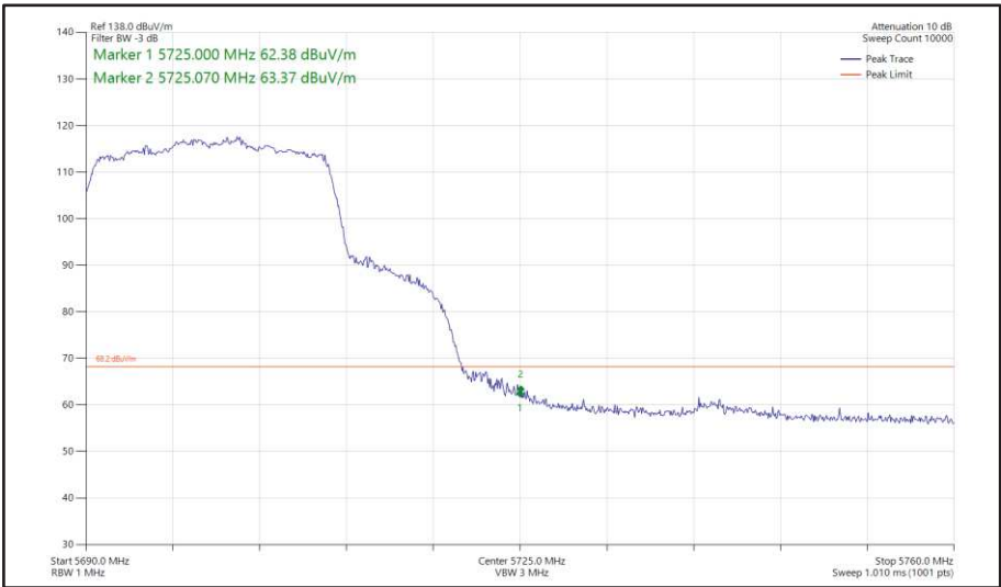
Figure 424 - 802.11ax HE20, SU, SDM, Core 0 + Core 1 - 5700 MHz Band Edge Frequency 5725 MHz
