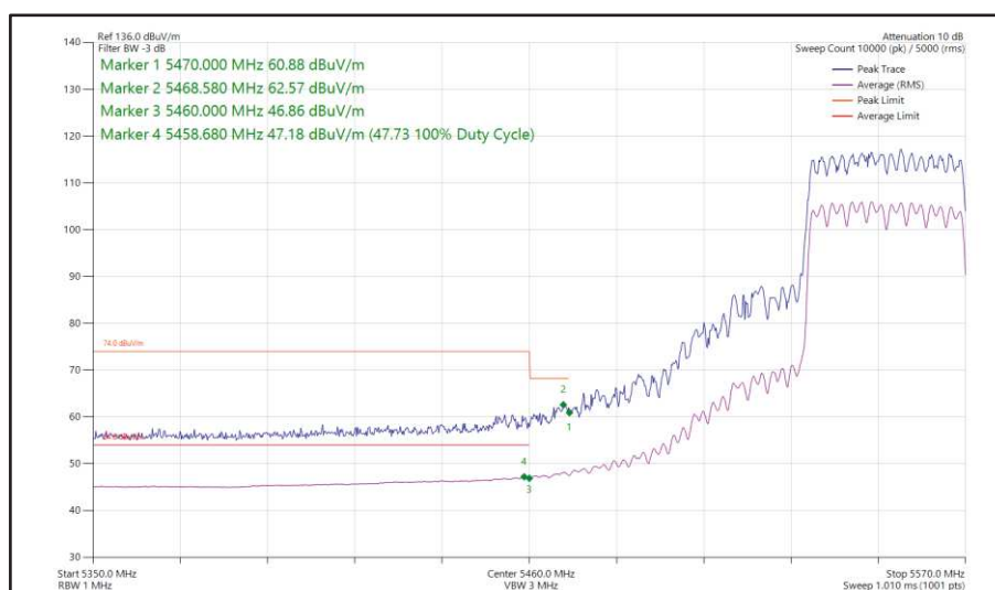
Figure 485 - 802.11ax HE40, SU, CDD, Core 0 + Core 1 - 5550 MHz Band Edge Frequency 5470 MHz
