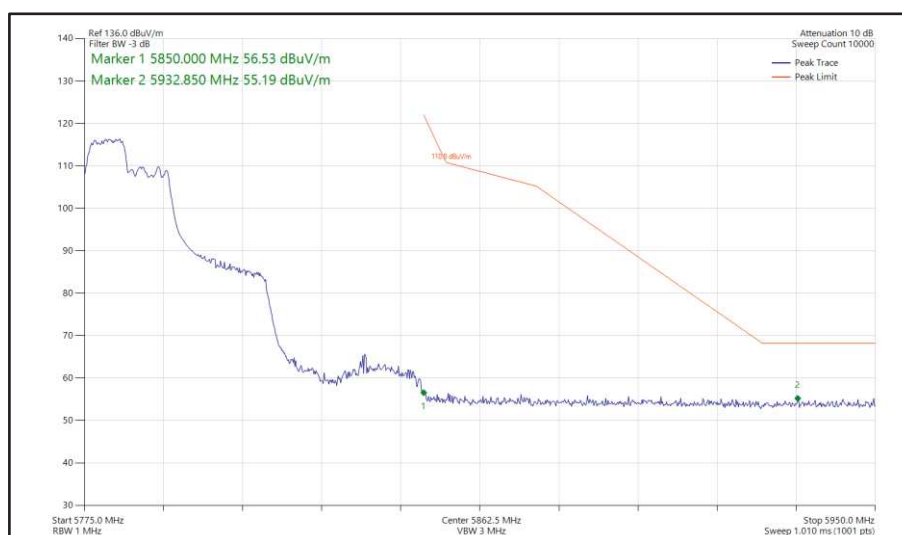
Figure 461 - 802.11ax HE40, RU 106-53, SISO, Core 0 - 5795 MHz Band Edge Frequency 5850 MHz
