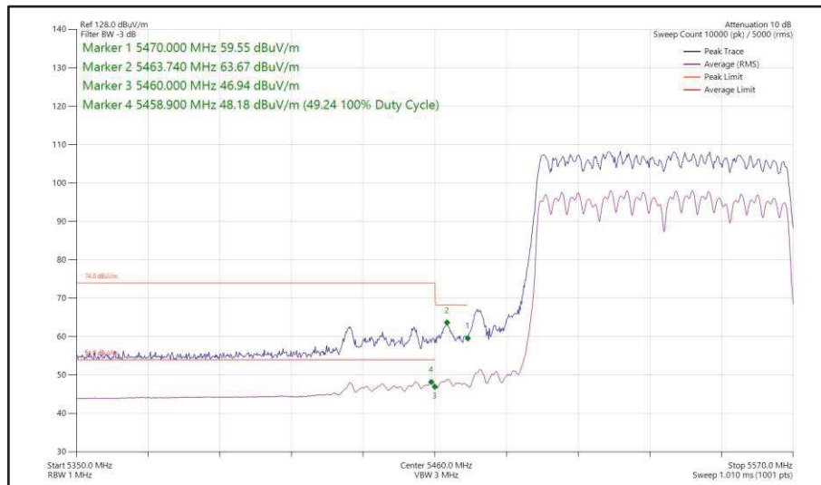
Figure 556 - 802.11ac VHT80, CDD, Core 0 + Core 1 - 5530 MHz Band Edge Frequency 5470 MHz
