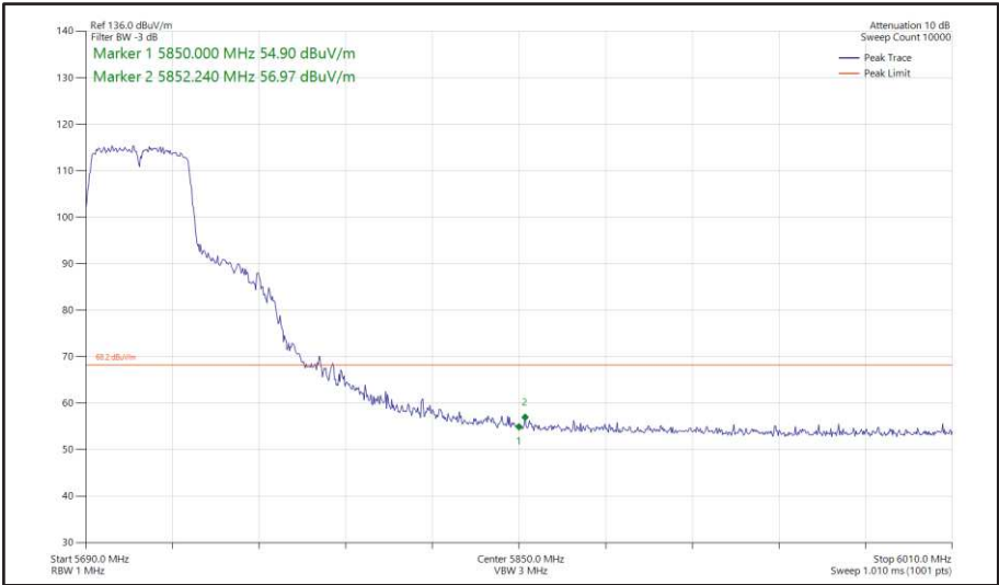
Figure 456 - 802.11n HT40, SISO, Core 0 - 5710 MHz Band Edge Frequency 5850 MHz
