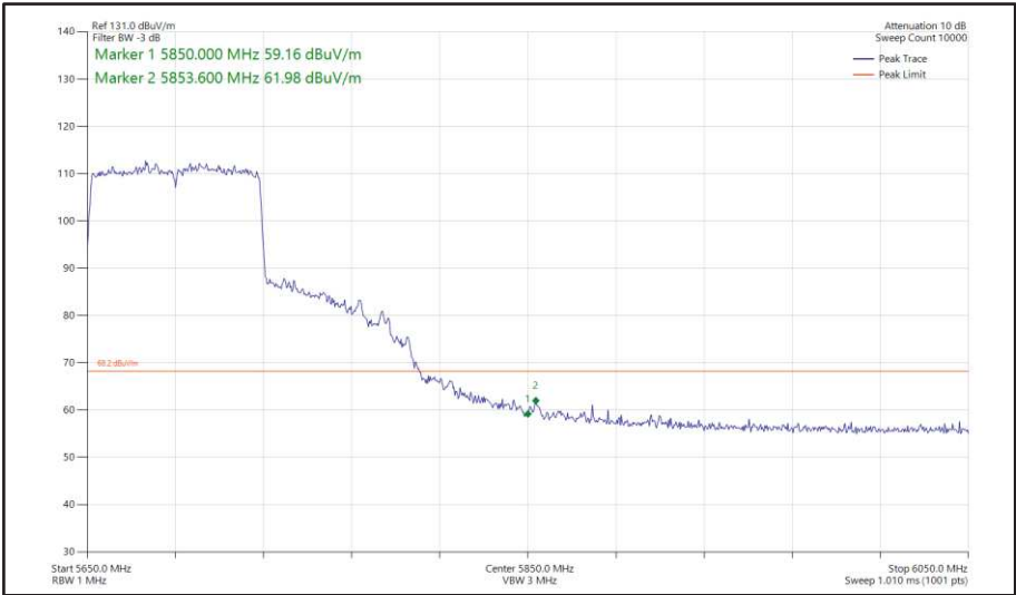
Figure 535 - 802.11ac VHT80, SISO, Core 0 - 5690 MHz Band Edge Frequency 5850 MHz
