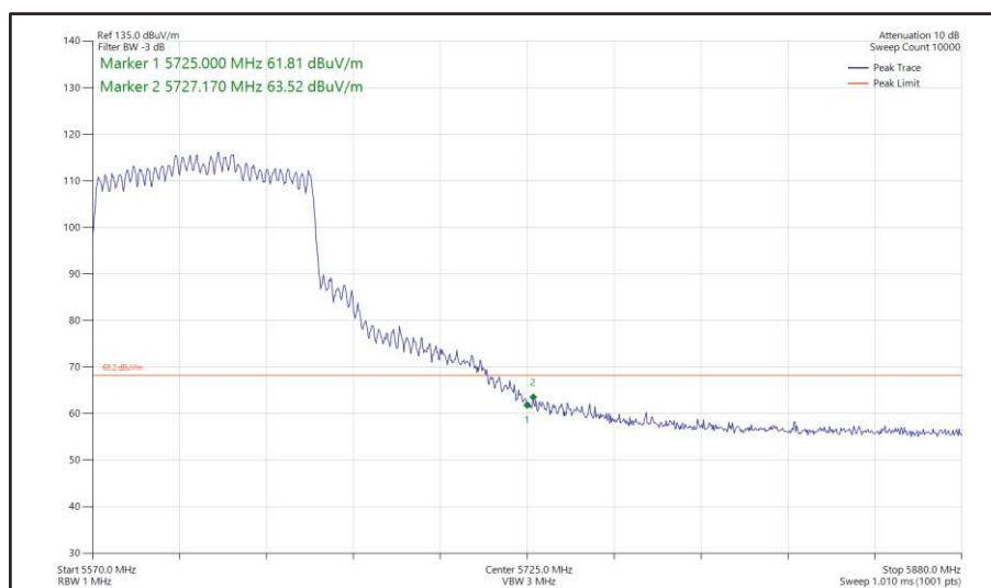
Figure 563 - 802.11ax HE80, SU, CDD, Core 0 + Core 1 - 5610 MHz Band Edge Frequency 5725 MHz
