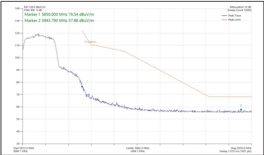
Figure 428 - 802.11n HT20, SDM, Core 0 + Core 1 - 5825 MHz Band Edge Frequency 5850 MHz
