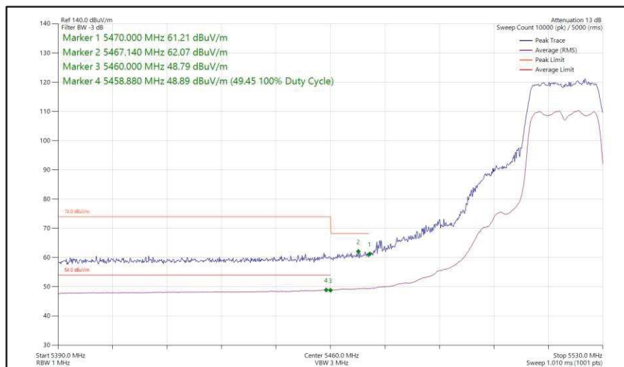
Figure 412 - 802.11n HT20, SDM, Core 0 + Core 1 - 5520 MHz Band Edge Frequency 5470 MHz
