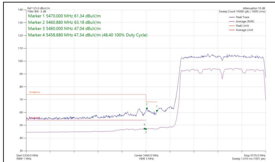
Figure 541 - 802.11ac VHT80, SISO, Core 1 - 5530 MHz Band Edge Frequency 5470 MHz
