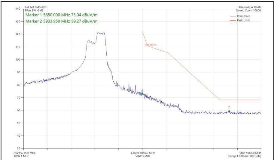
Figure 555 - 802.11ax HE80, RU 106-60, SISO, Core 1 - 5775 MHz Band Edge Frequency 5850 MHz
