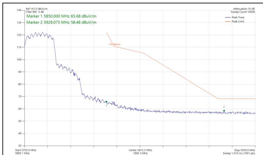
Figure 408 - 802.11ax HE20, SU, CDD, Core 0 + Core 1 - 5805 MHz Band Edge Frequency 5850 MHz
