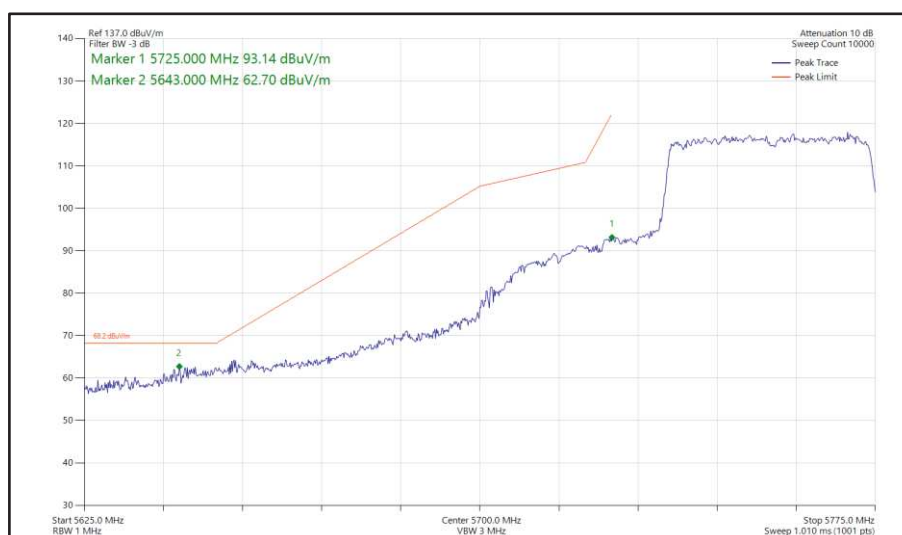
Figure 506 - 802.11ax HE40, SU, SDM, Core 0 + Core 1 - 5755 MHz Band Edge Frequency 5725 MHz
