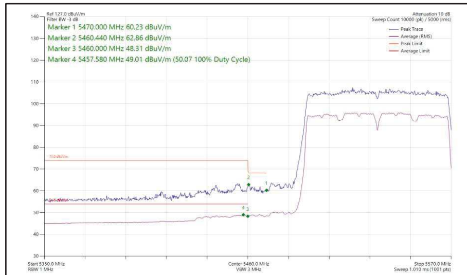
Figure 526 - 802.11ac VHT80, SISO, Core 0 - 5530 MHz Band Edge Frequency 5470 MHz
