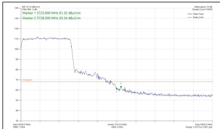
Figure 473 - 802.11ax HE40, SU, SISO, Core 1 - 5670 MHz Band Edge Frequency 5725 MHz
