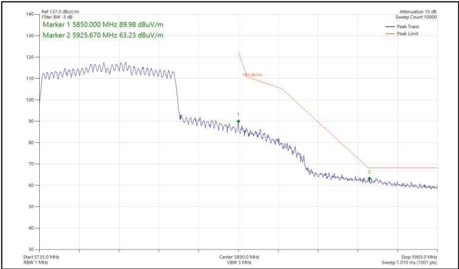
Figure 569 - 802.11ax HE80, SU, CDD, Core 0 + Core 1 - 5775 MHz Band Edge Frequency 5850 MHz
