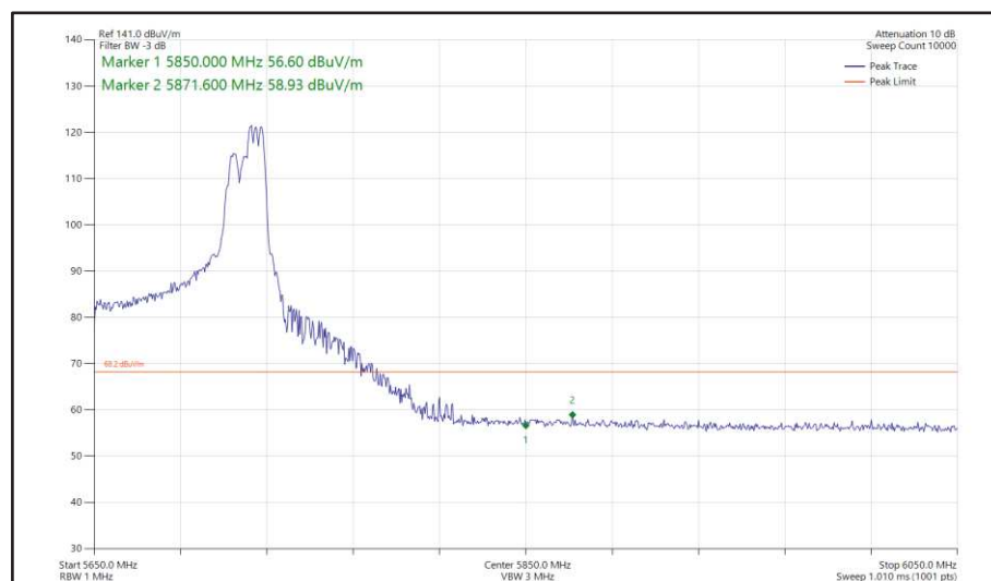
Figure 568 - 802.11ax HE80, RU 106-60, CDD, Core 0 + Core 1 - 5690 MHz Band Edge Frequency 5850 MHz
