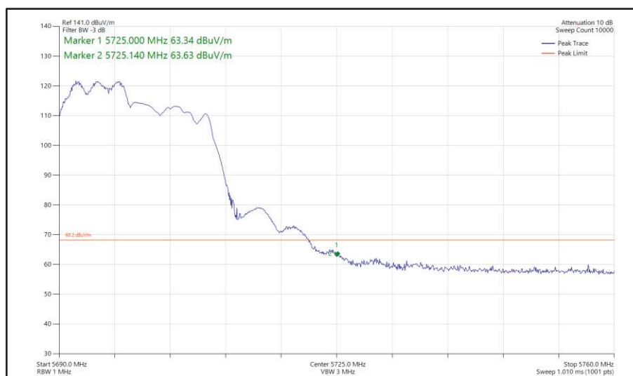
Figure 425 - 802.11ax HE20, RU 106-53, SDM, Core 0 + Core 1 - 5700 MHz Band Edge Frequency 5725 MHz
