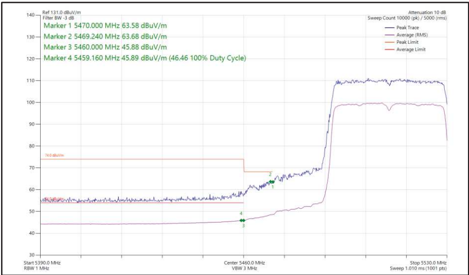
Figure 445 - 802.11ax HE40, SU, SISO, Core 0 - 5510 MHz Band Edge Frequency 5470 MHz
