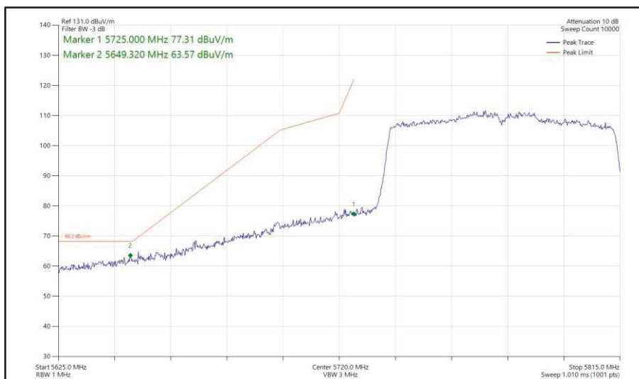
Figure 529 - 802.11ac VHT80, SISO, Core 0 - 5775 MHz Band Edge Frequency 5725 MHz
