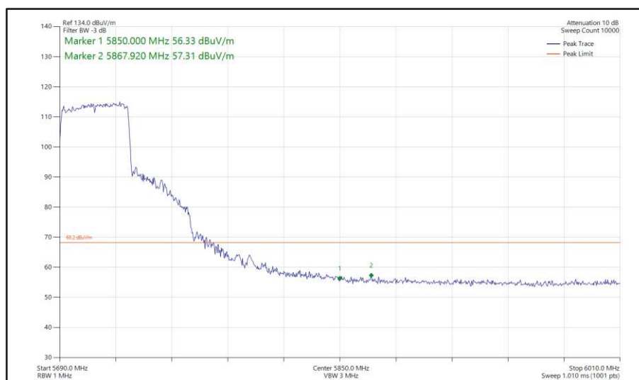
Figure 477 - 802.11ax HE40, SU, SISO, Core 1 - 5710 MHz Band Edge Frequency 5850 MHz
