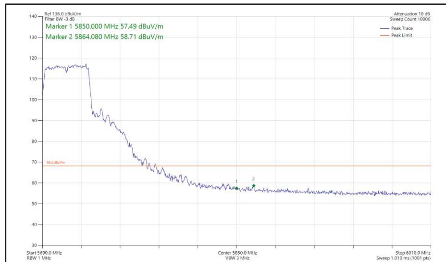
Figure 513 - 802.11n HT40, SDM, Core 0 + Core 1 - 5710 MHz Band Edge Frequency 5850 MHz
