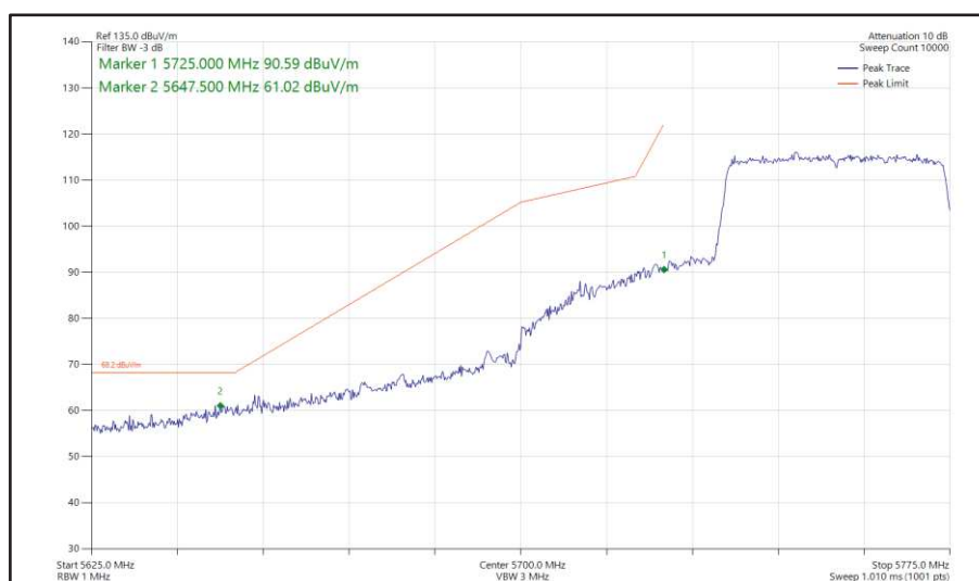
Figure 449 - 802.11ax HE40, SU, SISO, Core 0 - 5755 MHz Band Edge Frequency 5725 MHz
