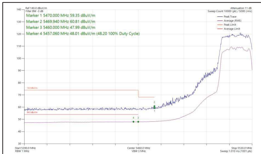
Figure 435 - 802.11ac VHT20, TxBF, Core 0 + Core 1 - 5520 MHz Band Edge Frequency 5470 MHz
