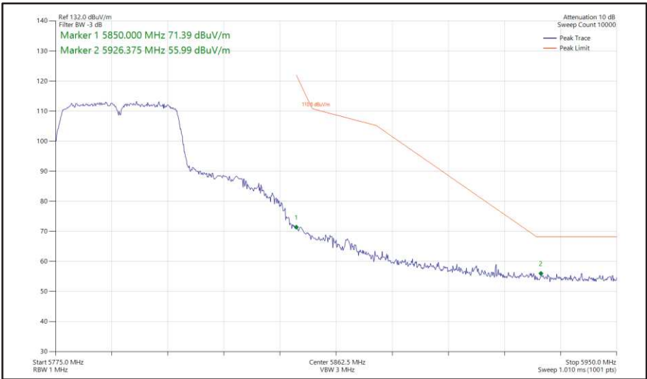
Figure 457 - 802.11n HT40, SISO, Core 0 - 5795 MHz Band Edge Frequency 5850 MHz
