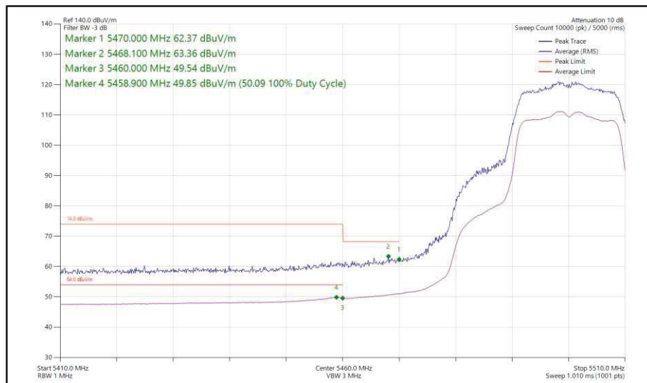
Figure 411 - 802.11n HT20, SDM, Core 0 + Core 1 - 5500 MHz Band Edge Frequency 5470 MHz
