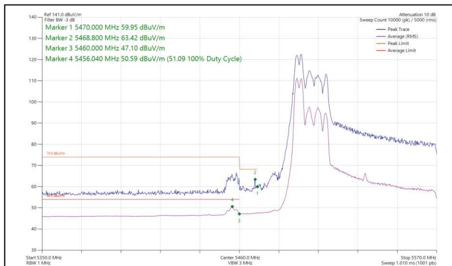
Figure 558 - 802.11ax HE80, RU 52-37, CDD, Core 0 + Core 1 - 5530 MHz Band Edge Frequency 5470 MHz
