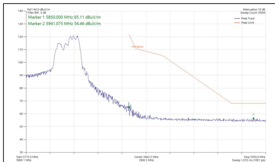
Figure 518 - 802.11ax HE40, RU 106-56, SDM, Core 0 + Core 1 - 5795 MHz Band Edge Frequency 5850 MHz
