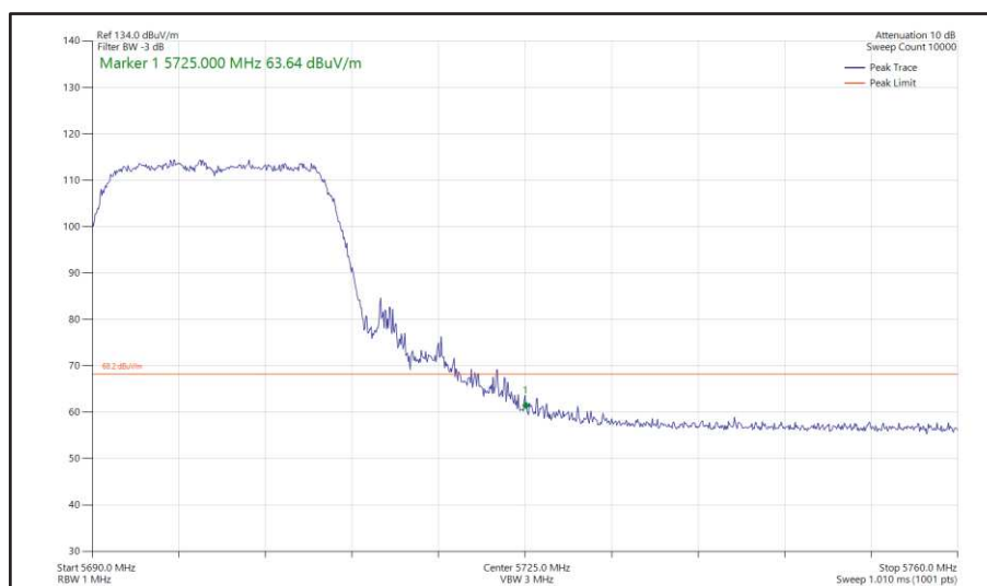
Figure 439 - 802.11ac VHT20, TxBF, Core 0 + Core 1 - 5700 MHz Band Edge Frequency 5725 MHz
