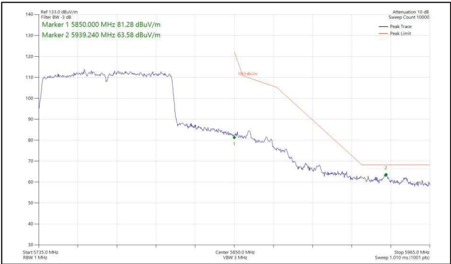
Figure 551 - 802.11ac VHT80, SISO, Core 1 - 5775 MHz Band Edge Frequency 5850 MHz
