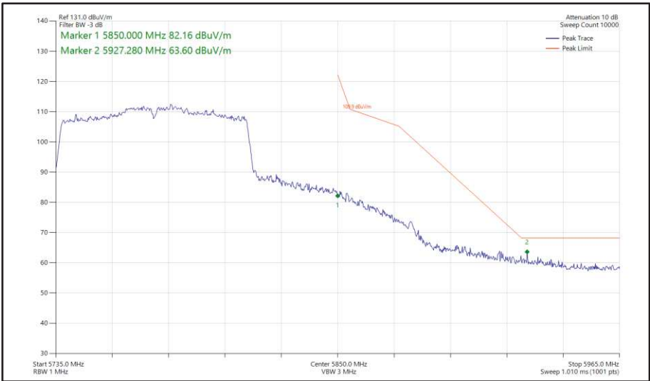
Figure 536 - 802.11ac VHT80, SISO, Core 0 - 5775 MHz Band Edge Frequency 5850 MHz
