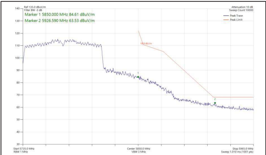
Figure 566 - 802.11ac VHT80, CDD, Core 0 + Core 1 - 5775 MHz Band Edge Frequency 5850 MHz
