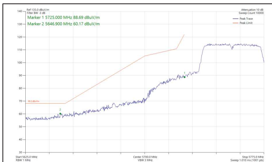
Figure 448 - 802.11n HT40, SISO, Core 0 - 5755 MHz Band Edge Frequency 5725 MHz
