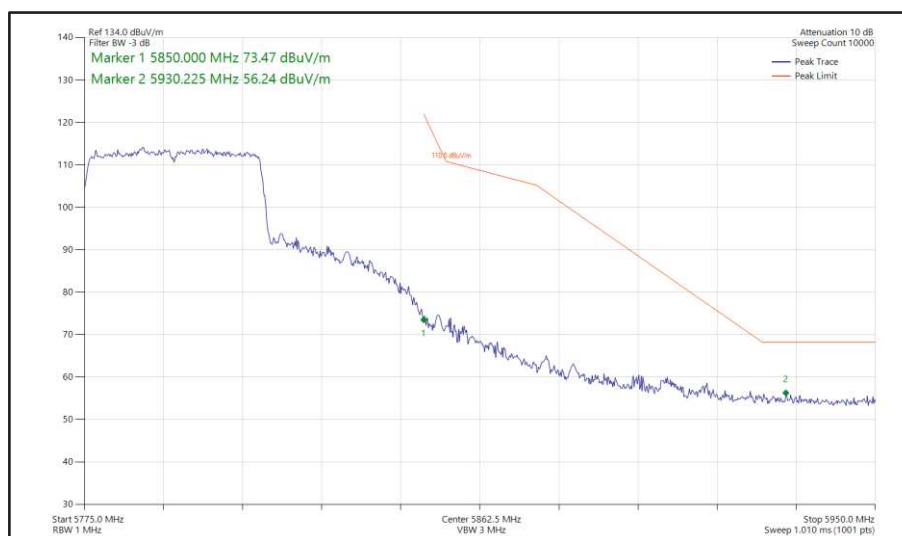
Figure 460 - 802.11ax HE40, SU, SISO, Core 0 - 5795 MHz Band Edge Frequency 5850 MHz
