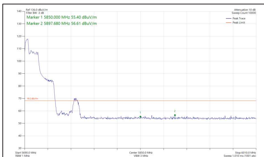
Figure 478 - 802.11ax HE40, RU 52-37, SISO, Core 1 - 5710 MHz Band Edge Frequency 5850 MHz
