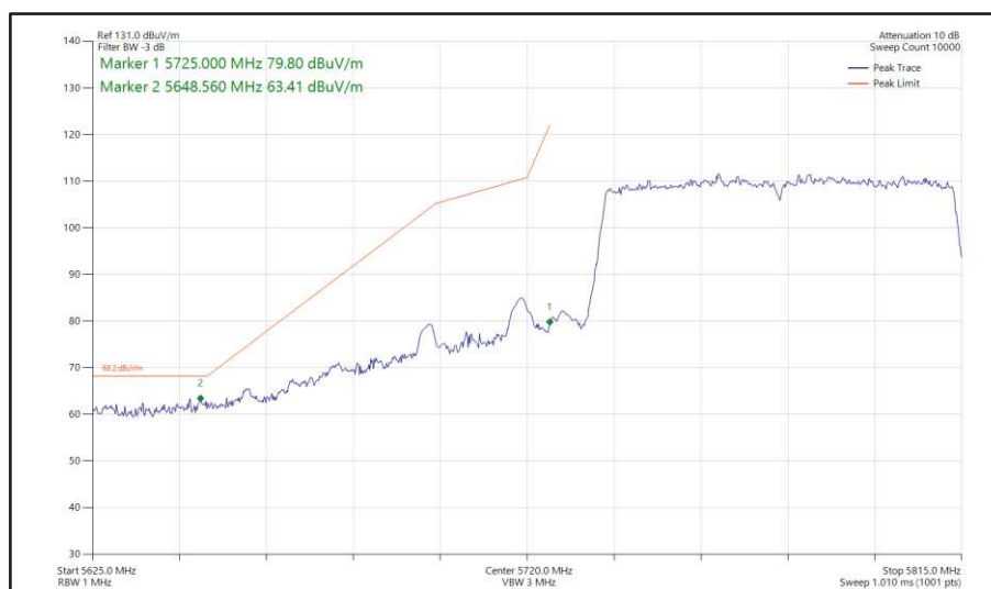
Figure 544 - 802.11ac VHT80, SISO, Core 1 - 5775 MHz Band Edge Frequency 5725 MHz
