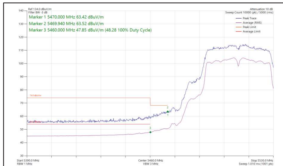
Figure 500 - 802.11n HT40, SDM, Core 0 + Core 1 - 5510 MHz Band Edge Frequency 5470 MHz
