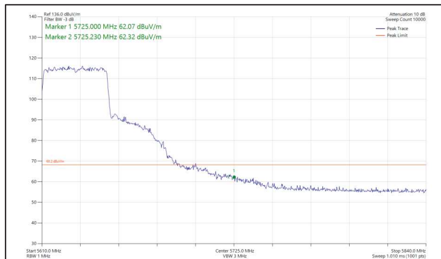
Figure 510 - 802.11ax HE40, SU, SDM, Core 0 + Core 1 - 5630 MHz Band Edge Frequency 5725 MHz
