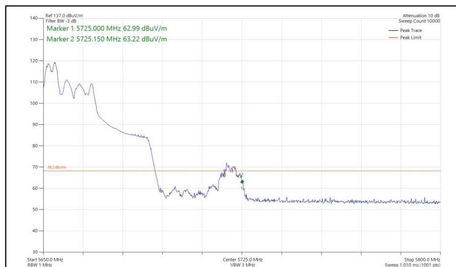
Figure 512 - 802.11ax HE40, RU 52-37, SDM, Core 0 + Core 1 - 5670 MHz Band Edge Frequency 5725 MHz
