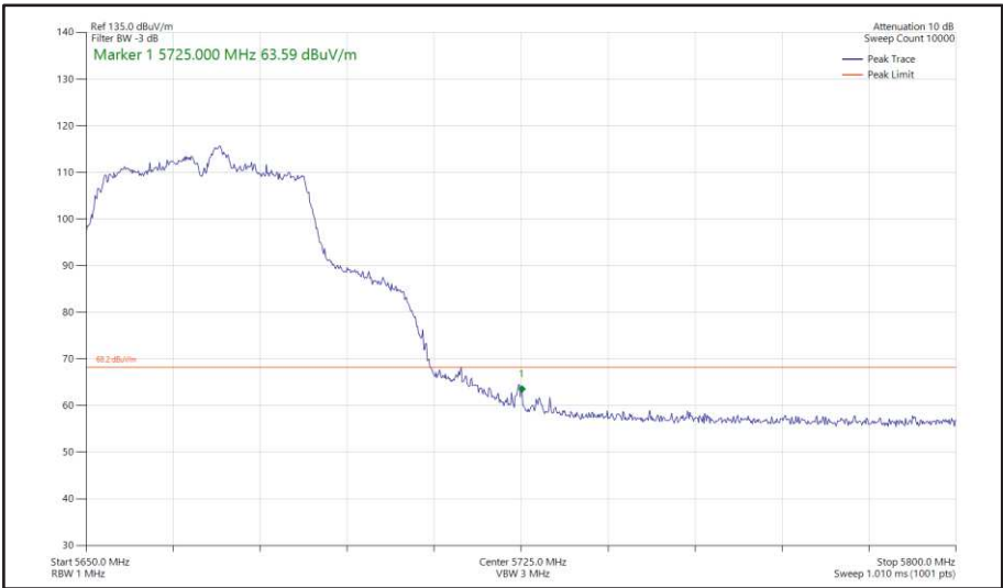
Figure 523 - 802.11ac VHT40, TxBF, Core 0 + Core 1 - 5670 MHz Band Edge Frequency 5725 MHz
