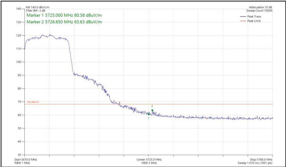
Figure 423 - 802.11ax HE20, SU, SDM, Core 0 + Core 1 - 5680 MHz Band Edge Frequency 5725 MHz
