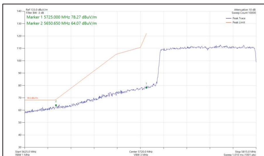
Figure 545 - 802.11ax HE80, SU, SISO, Core 1 - 5775 MHz Band Edge Frequency 5725 MHz
