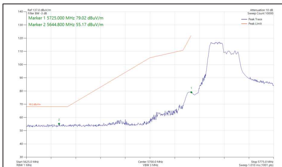
Figure 450 - 802.11ax HE40, RU 106-53, SISO, Core 0 - 5755 MHz Band Edge Frequency 5725 MHz
