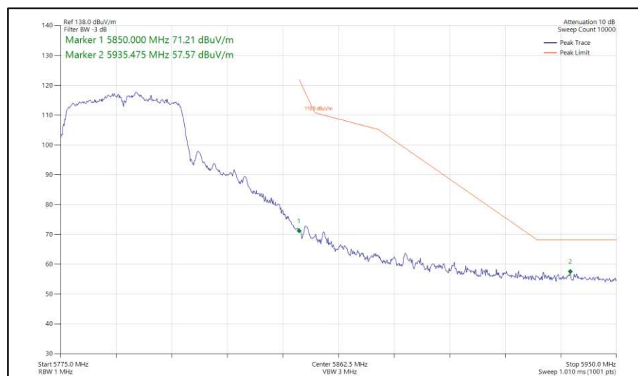
Figure 514 - 802.11n HT40, SDM, Core 0 + Core 1 - 5795 MHz Band Edge Frequency 5850 MHz
