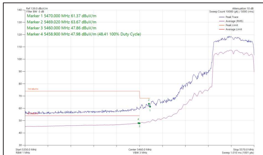
Figure 504 - 802.11ax HE40, SU, SDM, Core 0 + Core 1 - 5550 MHz Band Edge Frequency 5470 MHz
