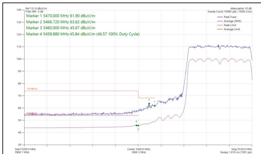
Figure 502 - 802.11ax HE40, SU, SDM, Core 0 + Core 1 - 5510 MHz Band Edge Frequency 5470 MHz
