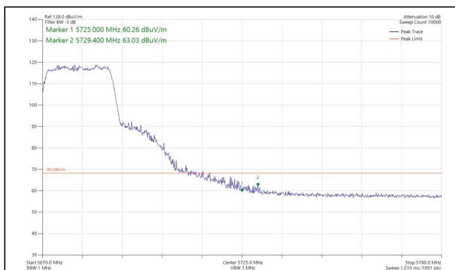
Figure 438 - 802.11ac VHT20, TxBF, Core 0 + Core 1 - 5680 MHz Band Edge Frequency 5725 MHz
