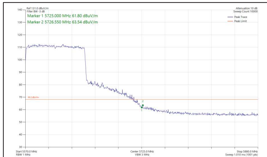
Figure 533 - 802.11ax HE80, SU, SISO, Core 0 - 5610 MHz Band Edge Frequency 5725 MHz
