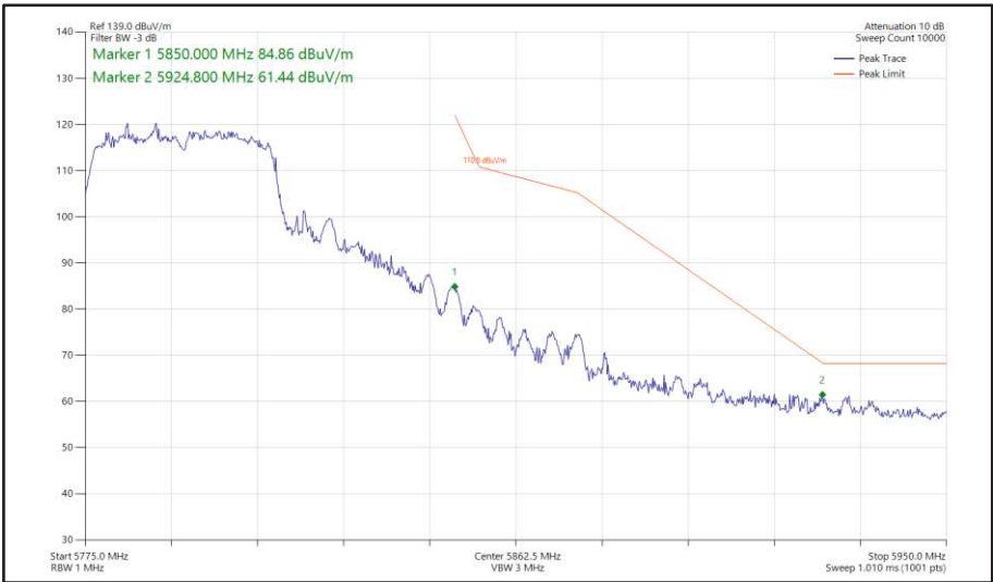
Figure 525 - 802.11ac VHT40, TxBF, Core 0 + Core 1 - 5795 MHz Band Edge Frequency 5850 MHz
