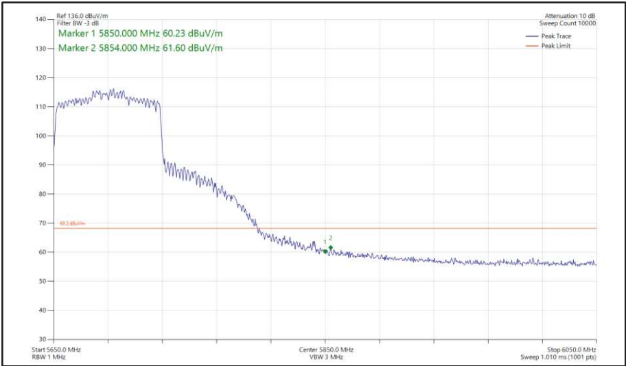
Figure 565 - 802.11ac VHT80, CDD, Core 0 + Core 1 - 5690 MHz Band Edge Frequency 5850 MHz
