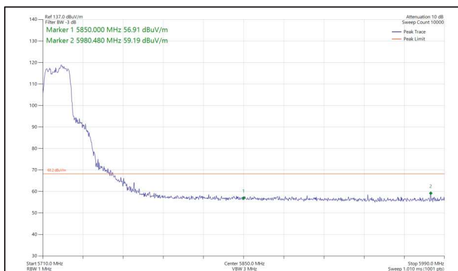
Figure 440 - 802.11ac VHT20, TxBF, Core 0 + Core 1 - 5720 MHz Band Edge Frequency 5850 MHz
