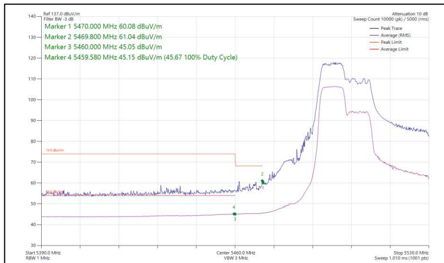
Figure 465 - 802.11ax HE40, RU 106-53, SISO, Core 1 - 5510 MHz Band Edge Frequency 5470 MHz
