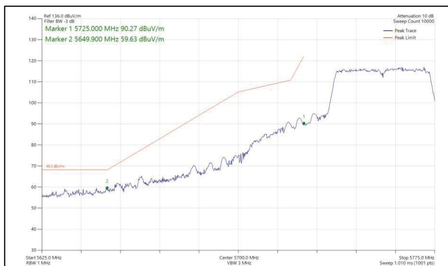
Figure 505 - 802.11n HT40, SDM, Core 0 + Core 1 - 5755 MHz Band Edge Frequency 5725 MHz
