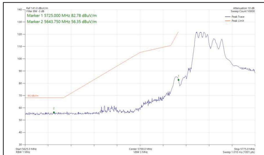
Figure 488 - 802.11ax HE40, RU 106-53, CDD, Core 0 + Core 1 - 5755 MHz Band Edge Frequency 5725 MHz
