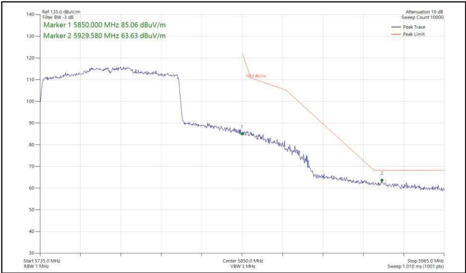
Figure 554 - 802.11ax HE80, SU, SISO, Core 1 - 5775 MHz Band Edge Frequency 5850 MHz
