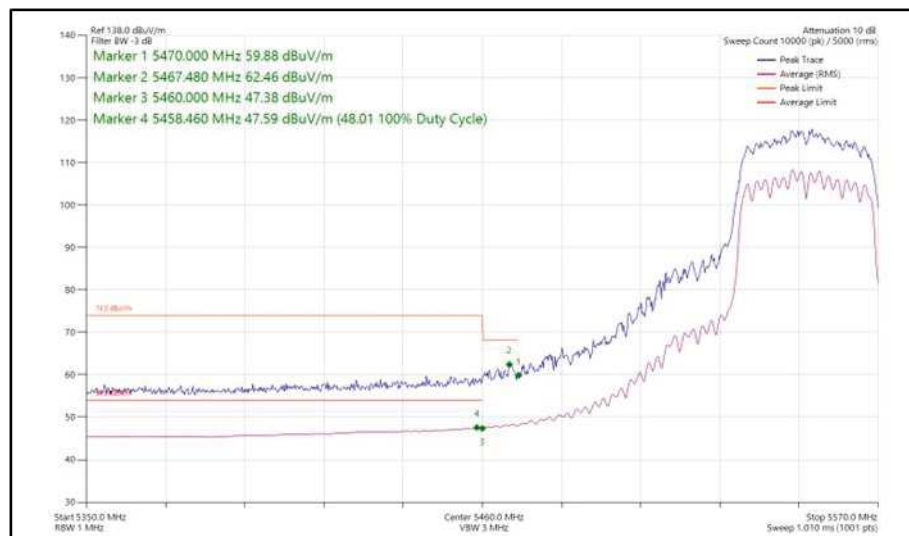
Figure 482 - 802.11n HT40, CDD, Core 0 + Core 1 - 5550 MHz Band Edge Frequency 5470 MHz
