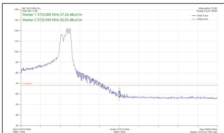
Figure 564 - 802.11ax HE80, RU 106-60, CDD, Core 0 + Core 1 - 5610 MHz Band Edge Frequency 5725 MHz
