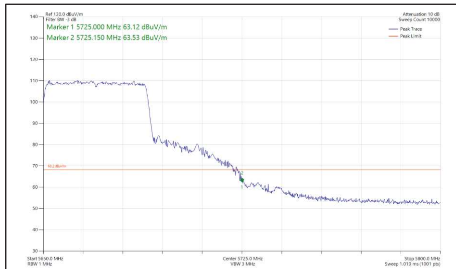
Figure 454 - 802.11ax HE40, SU, SISO, Core 0 - 5670 MHz Band Edge Frequency 5725 MHz
