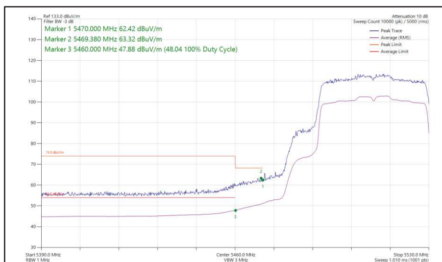
Figure 464 - 802.11ax HE40, SU, SISO, Core 1 - 5510 MHz Band Edge Frequency 5470 MHz
