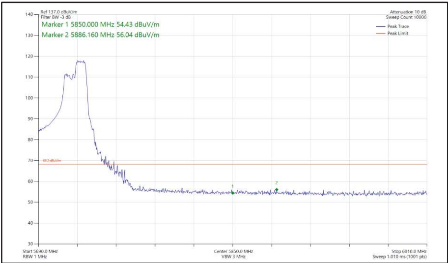
Figure 459 - 802.11ax HE40, RU 106-56, SISO, Core 0 - 5710 MHz Band Edge Frequency 5850 MHz
