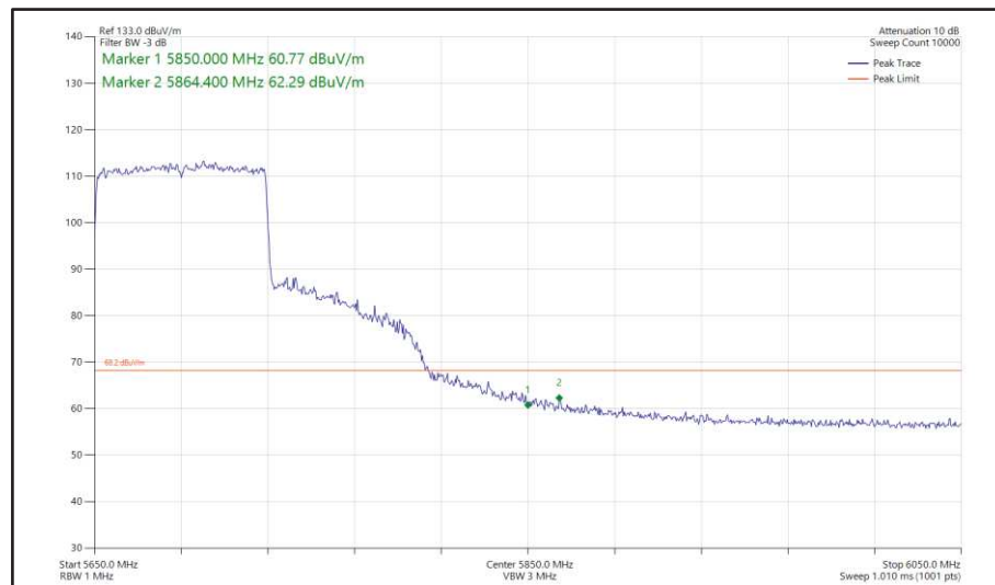
Figure 552 - 802.11ax HE80, SU, SISO, Core 1 - 5690 MHz Band Edge Frequency 5850 MHz
