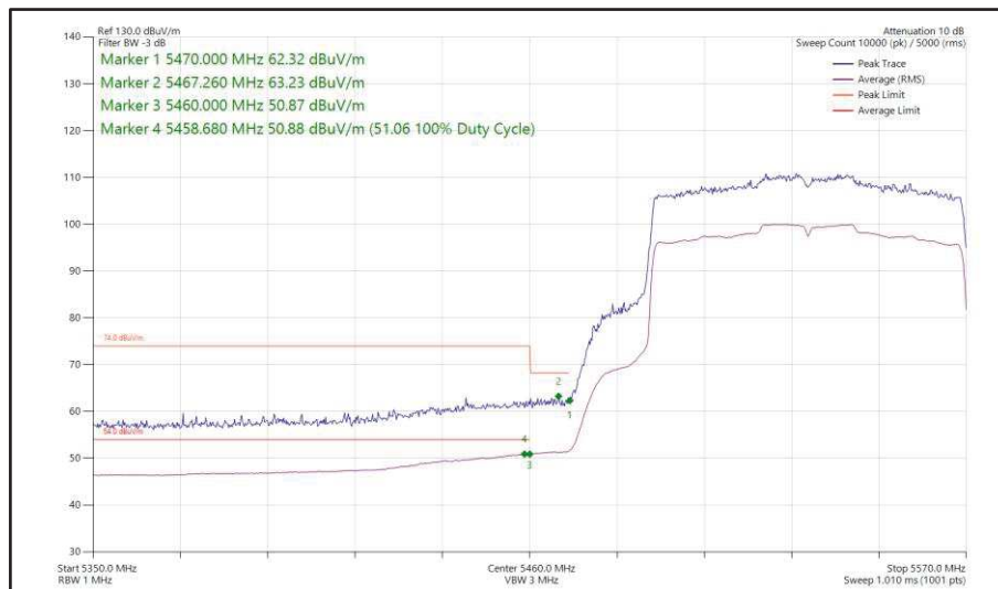
Figure 527 - 802.11ax HE80, SU, SISO, Core 0 - 5530 MHz Band Edge Frequency 5470 MHz
