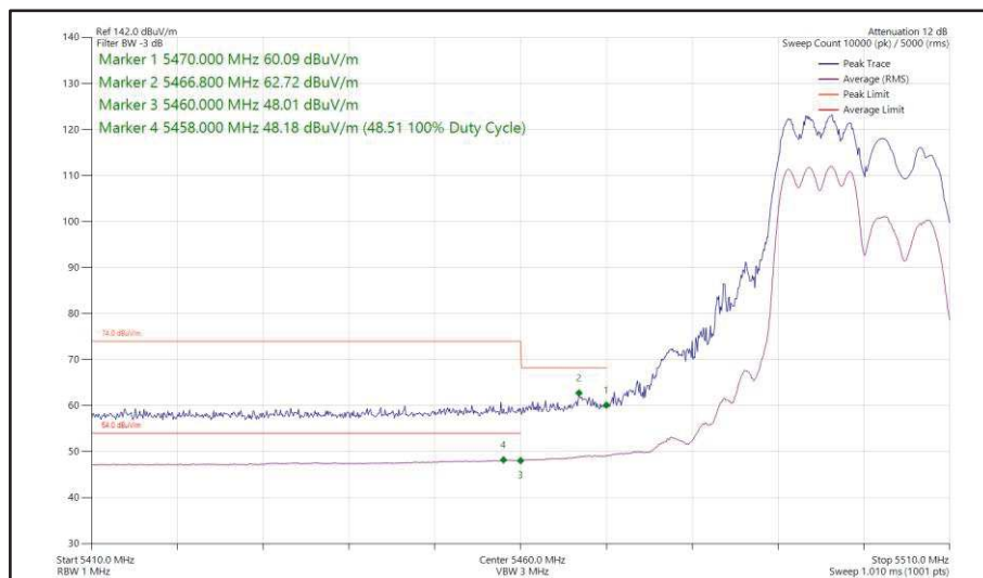
Figure 414 - 802.11ax HE20, RU 106-53, SDM, Core 0 + Core 1 - 5500 MHz Band Edge Frequency 5470 MHz
