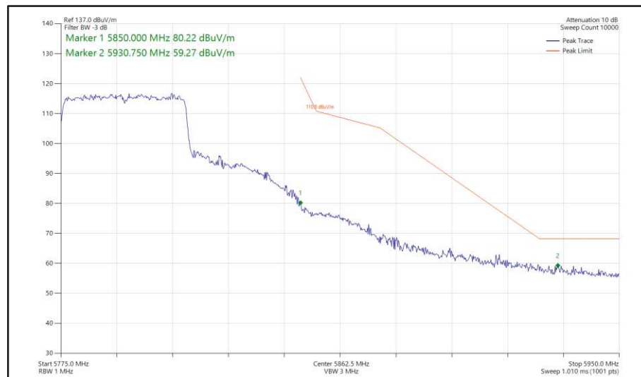
Figure 517 - 802.11ax HE40, SU, SDM, Core 0 + Core 1 - 5795 MHz Band Edge Frequency 5850 MHz
