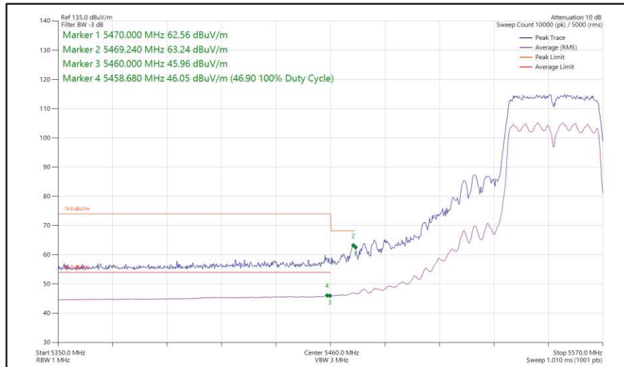
Figure 501 - 802.11n HT40, SDM, Core 0 + Core 1 - 5550 MHz Band Edge Frequency 5470 MHz
