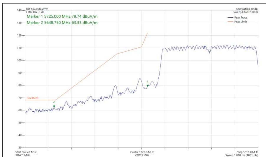
Figure 559 - 802.11ac VHT80, CDD, Core 0 + Core 1 - 5775 MHz Band Edge Frequency 5725 MHz
