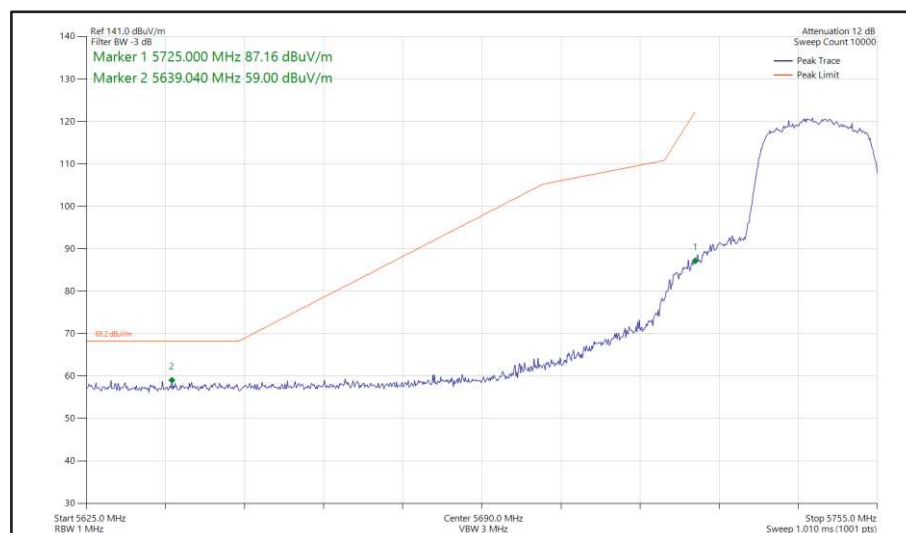
Figure 416 - 802.11n HT20, SDM, Core 0 + Core 1 - 5745 MHz Band Edge Frequency 5725 MHz
