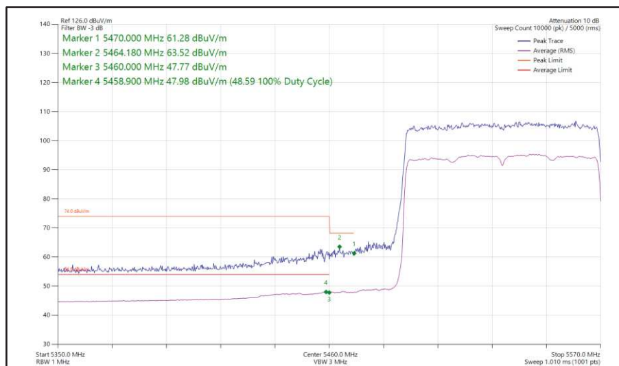
Figure 542 - 802.11ax HE80, SU, SISO, Core 1 - 5530 MHz Band Edge Frequency 5470 MHz
