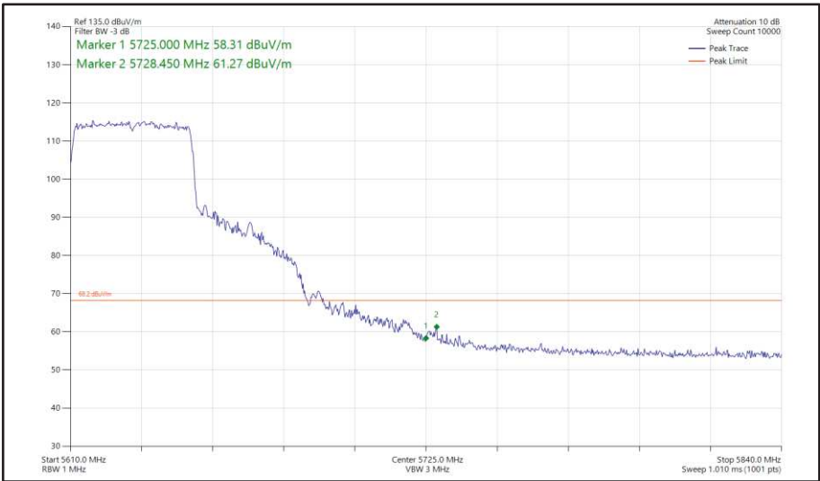
Figure 453 - 802.11ax HE40, SU, SISO, Core 0 - 5630 MHz Band Edge Frequency 5725 MHz
