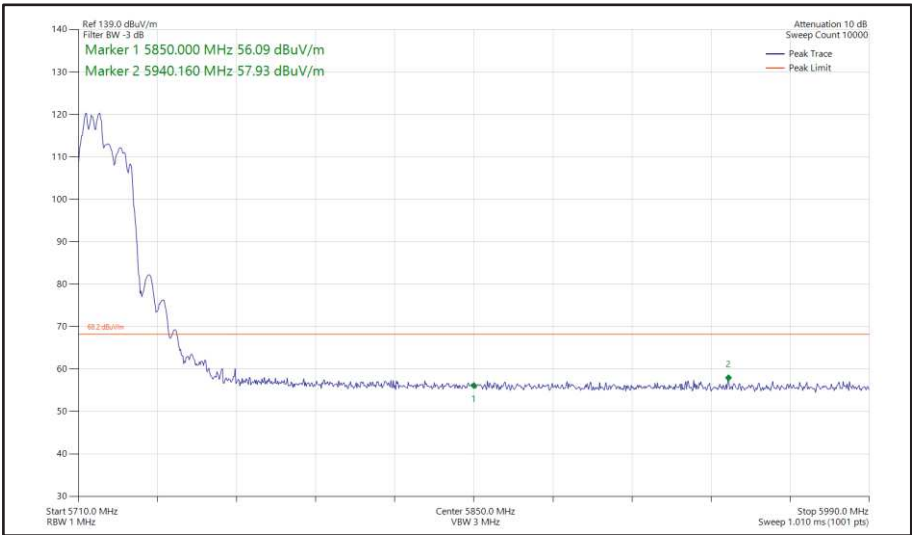
Figure 430 - 802.11ax HE20, RU 106-53, SDM, Core 0 + Core 1 - 5720 MHz Band Edge Frequency 5850 MHz
