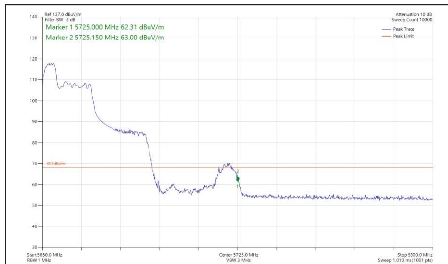
Figure 455 - 802.11ax HE40, RU 52-37, SISO, Core 0 - 5670 MHz Band Edge Frequency 5725 MHz
