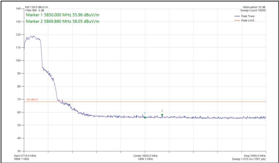
Figure 429 - 802.11ax HE20, SU, SDM, Core 0 + Core 1 - 5720 MHz Band Edge Frequency 5850 MHz
