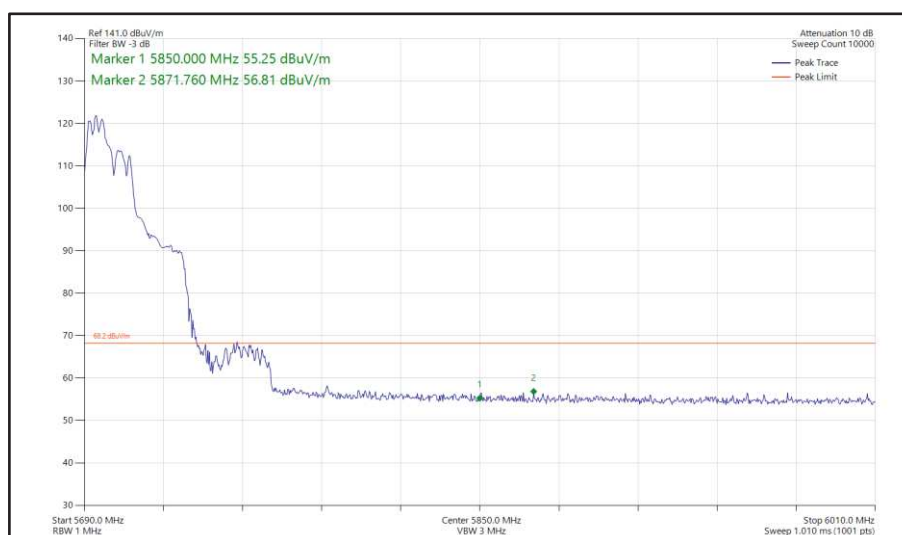
Figure 497 - 802.11ax HE40, RU 106-53, CDD, Core 0 + Core 1 - 5710 MHz Band Edge Frequency 5850 MHz
