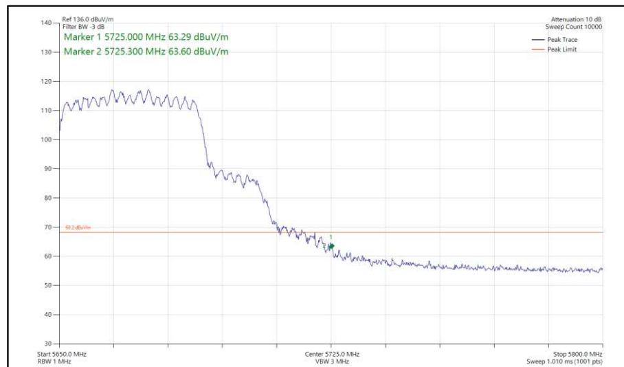
Figure 492 - 802.11ax HE40, SU, CDD, Core 0 + Core 1 - 5670 MHz Band Edge Frequency 5725 MHz
