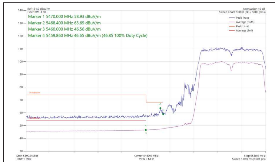
Figure 519 - 802.11ac VHT40, TxBF, Core 0 + Core 1 - 5510 MHz Band Edge Frequency 5470 MHz
