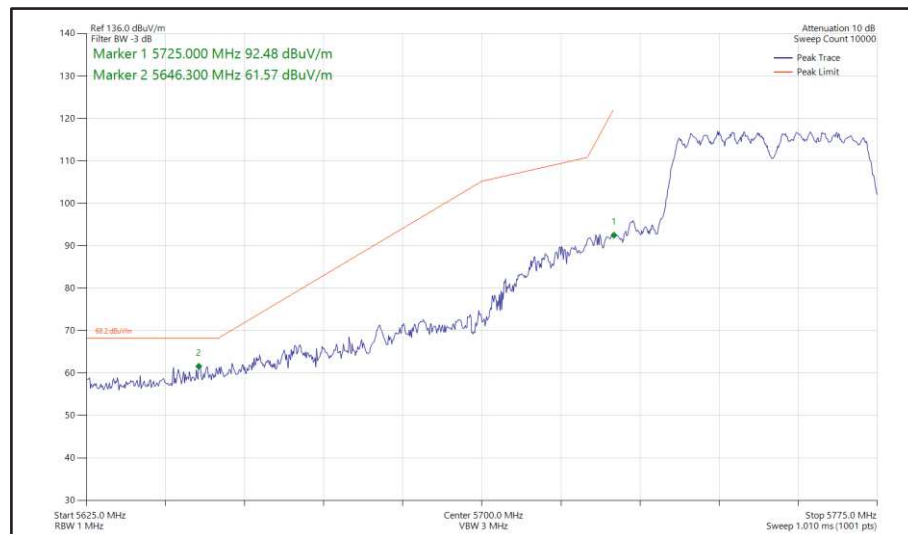
Figure 486 - 802.11n HT40, CDD, Core 0 + Core 1 - 5755 MHz Band Edge Frequency 5725 MHz
