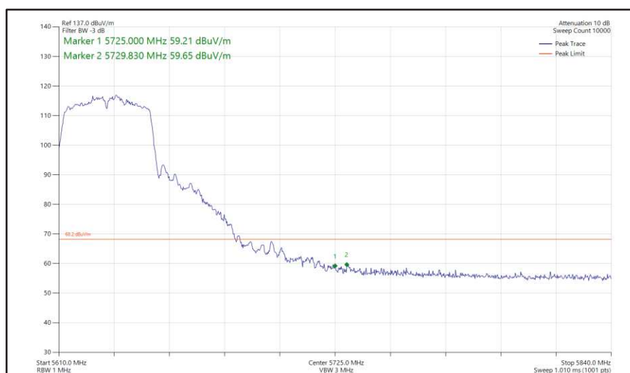
Figure 508 - 802.11n HT40, SDM, Core 0 + Core 1 - 5630 MHz Band Edge Frequency 5725 MHz
