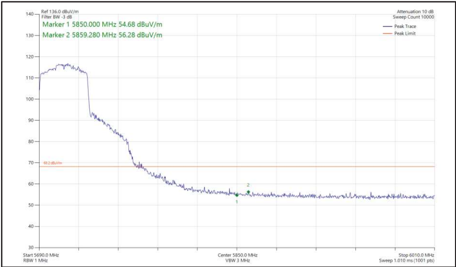
Figure 458 - 802.11ax HE40, SU, SISO, Core 0 - 5710 MHz Band Edge Frequency 5850 MHz
