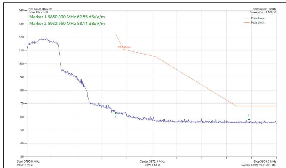
Figure 431 - 802.11ax HE20, SU, SDM, Core 0 + Core 1 - 5805 MHz Band Edge Frequency 5850 MHz
