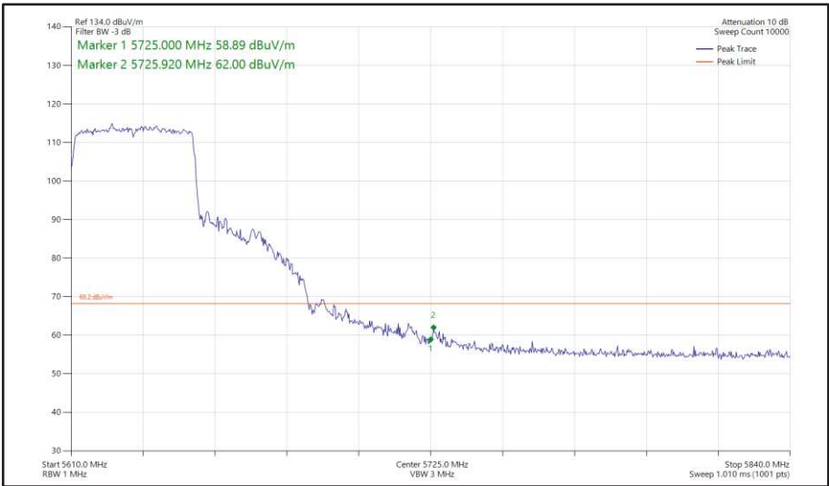
Figure 472 - 802.11ax HE40, SU, SISO, Core 1 - 5630 MHz Band Edge Frequency 5725 MHz
