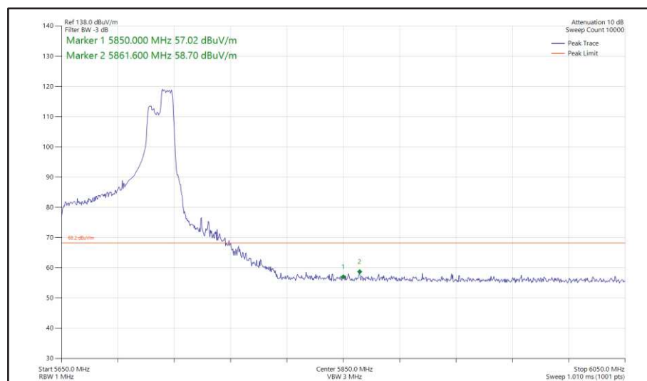
Figure 538 - 802.11ax HE80, RU 106-60, SISO, Core 0 - 5690 MHz Band Edge Frequency 5850 MHz
