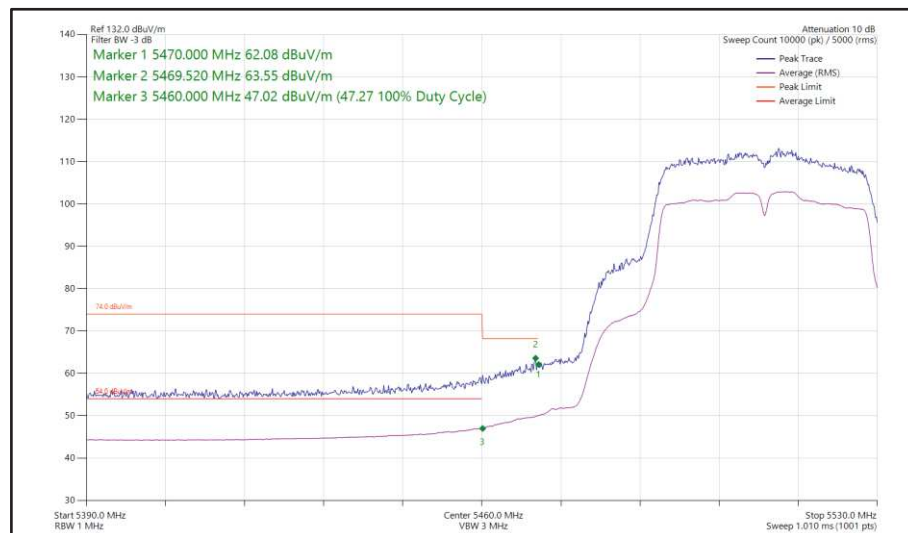
Figure 462 - 802.11n HT40, SISO, Core 1 - 5510 MHz Band Edge Frequency 5470 MHz
