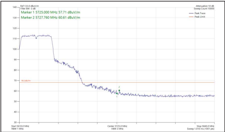
Figure 470 - 802.11n HT40, SISO, Core 1 - 5630 MHz Band Edge Frequency 5725 MHz
