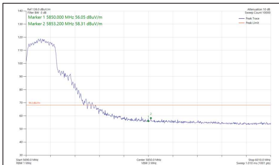
Figure 494 - 802.11n HT40, CDD, Core 0 + Core 1 - 5710 MHz Band Edge Frequency 5850 MHz
