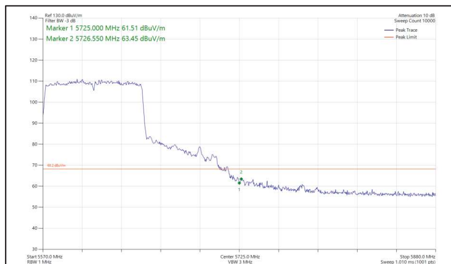
Figure 547 - 802.11ac VHT80, SISO, Core 1 - 5610 MHz Band Edge Frequency 5725 MHz
