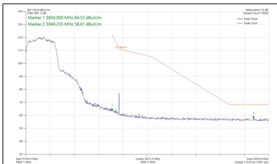
Figure 441 - 802.11ac VHT20, TxBF, Core 0 + Core 1 - 5805 MHz Band Edge Frequency 5850 MHz
