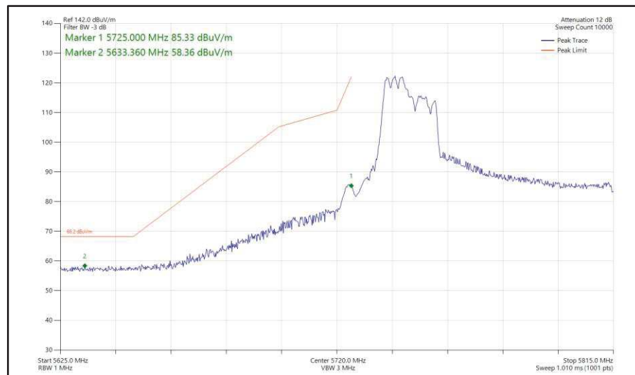
Figure 561 - 802.11ax HE80, RU 106-53, CDD, Core 0 + Core 1 - 5775 MHz Band Edge Frequency 5725 MHz
