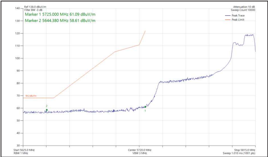
Figure 531 - 802.11ax HE80, RU 106-60, SISO, Core 0 - 5775 MHz Band Edge Frequency 5725 MHz
