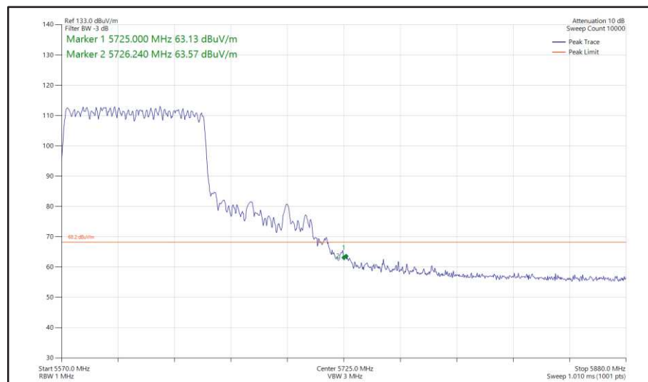
Figure 562 - 802.11ac VHT80, CDD, Core 0 + Core 1 - 5610 MHz Band Edge Frequency 5725 MHz
