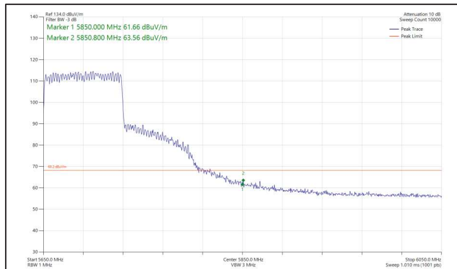
Figure 567 - 802.11ax HE80, SU, CDD, Core 0 + Core 1 - 5690 MHz Band Edge Frequency 5850 MHz
