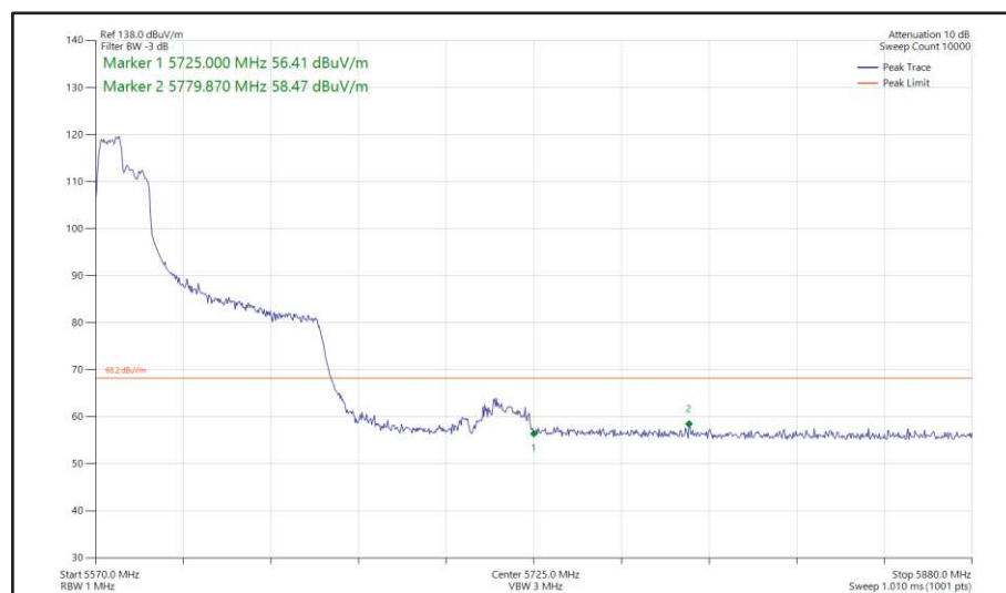
Figure 534 - 802.11ax HE80, RU 106-53, SISO, Core 0 - 5610 MHz Band Edge Frequency 5725 MHz
