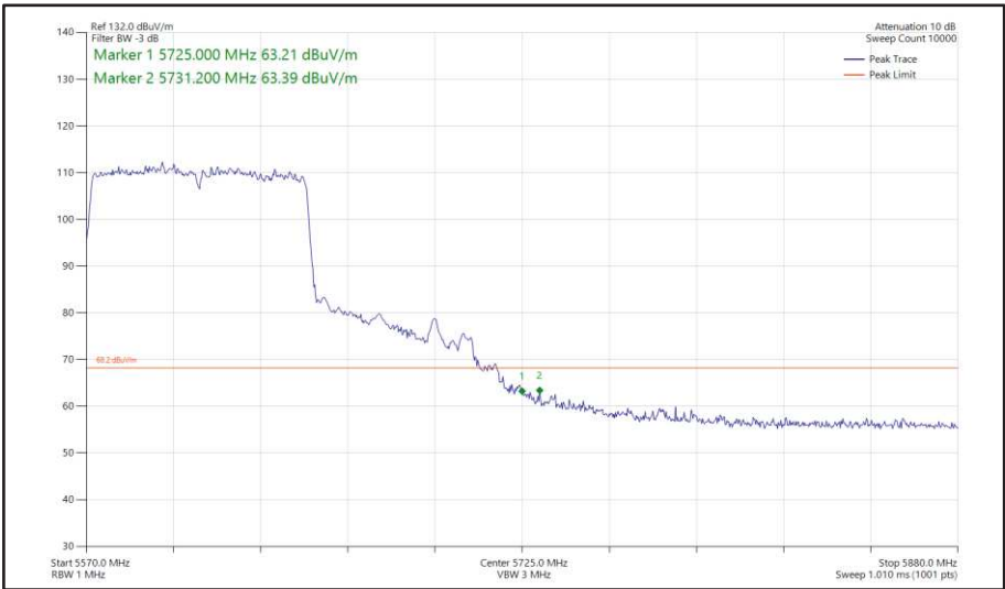
Figure 532 - 802.11ac VHT80, SISO, Core 0 - 5610 MHz Band Edge Frequency 5725 MHz
