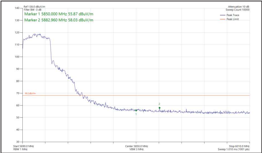
Figure 515 - 802.11ax HE40, SU, SDM, Core 0 + Core 1 - 5710 MHz Band Edge Frequency 5850 MHz
