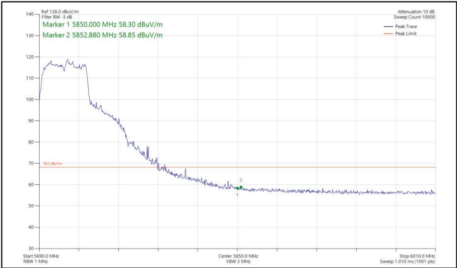
Figure 524 - 802.11ac VHT40, TxBF, Core 0 + Core 1 - 5710 MHz Band Edge Frequency 5850 MHz
