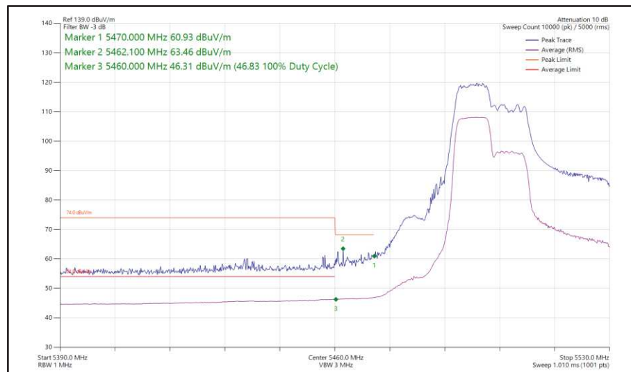
Figure 446 - 802.11ax HE40, RU 106-53, SISO, Core 0 - 5510 MHz Band Edge Frequency 5470 MHz
