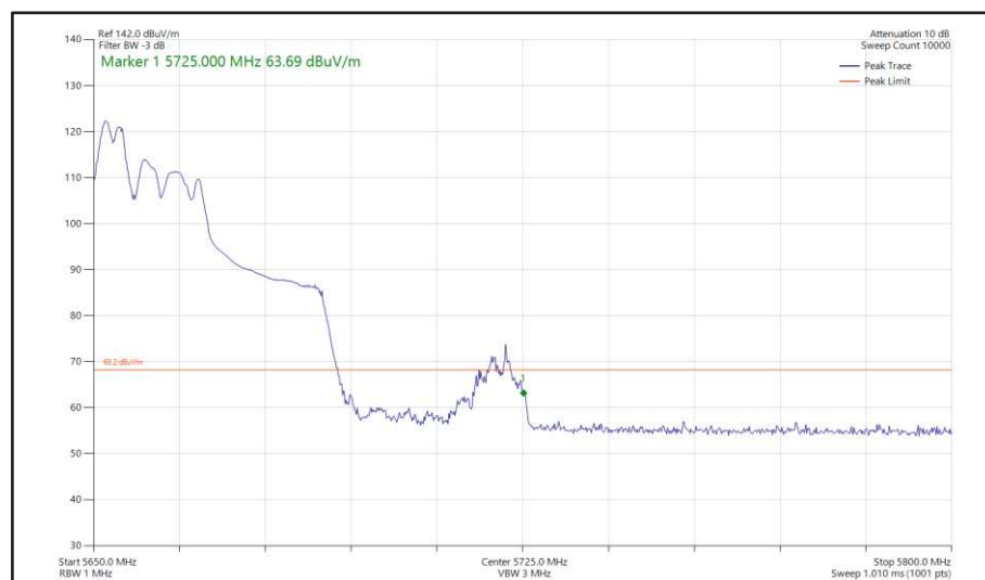
Figure 493 - 802.11ax HE40, RU 52-37, CDD, Core 0 + Core 1 - 5670 MHz Band Edge Frequency 5725 MHz
