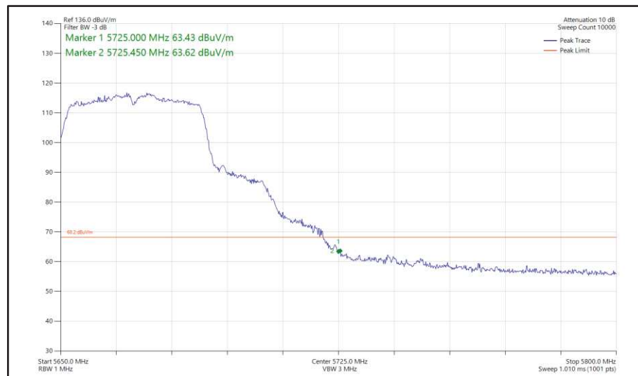
Figure 509 - 802.11n HT40, SDM, Core 0 + Core 1 - 5670 MHz Band Edge Frequency 5725 MHz
