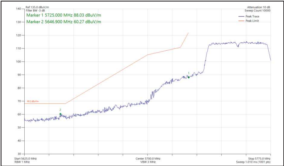
Figure 467 - 802.11n HT40, SISO, Core 1 - 5755 MHz Band Edge Frequency 5725 MHz
