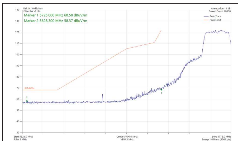
Figure 437 - 802.11ac VHT20, TxBF, Core 0 + Core 1 - 5765 MHz Band Edge Frequency 5725 MHz
