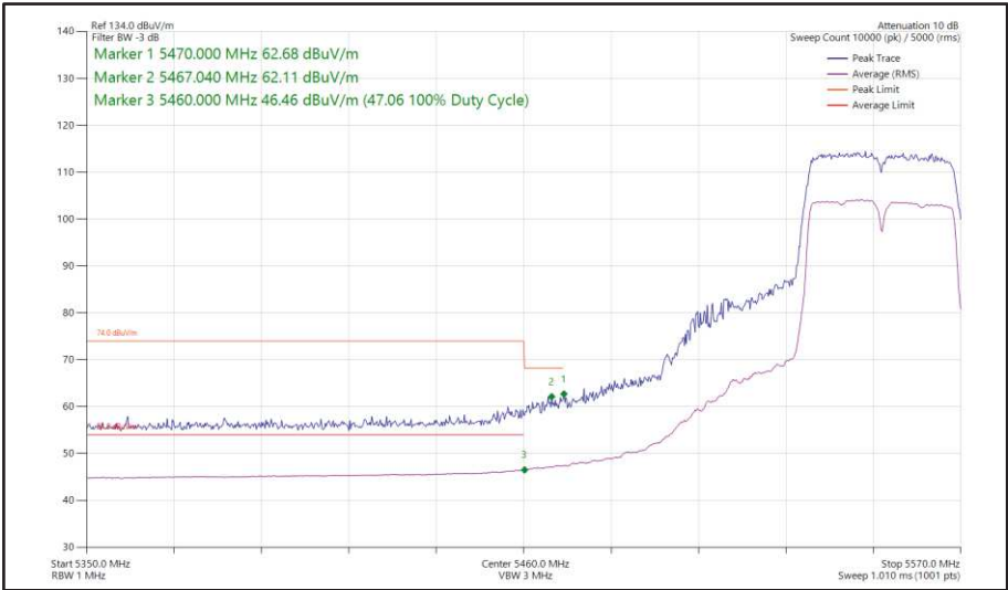
Figure 444 - 802.11n HT40, SISO, Core 0 - 5550 MHz Band Edge Frequency 5470 MHz
