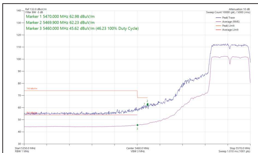
Figure 463 - 802.11n HT40, SISO, Core 1 - 5550 MHz Band Edge Frequency 5470 MHz
