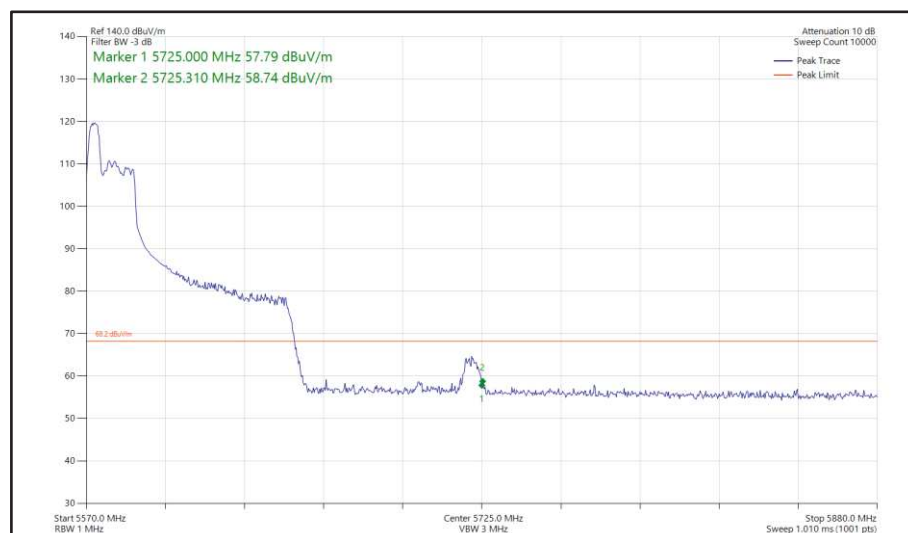
Figure 549 - 802.11ax HE80, RU 52-37, SISO, Core 1 - 5610 MHz Band Edge Frequency 5725 MHz
