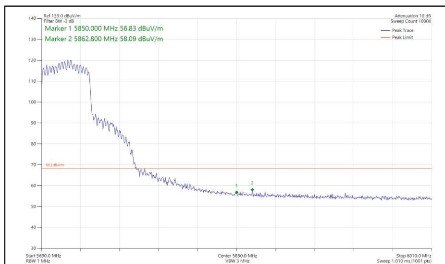
Figure 496 - 802.11ax HE40, SU, CDD, Core 0 + Core 1 - 5710 MHz Band Edge Frequency 5850 MHz
