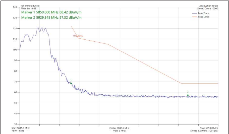
Figure 433 - 802.11ax HE20, RU 106-54, SDM, Core 0 + Core 1 - 5825 MHz Band Edge Frequency 5850 MHz
