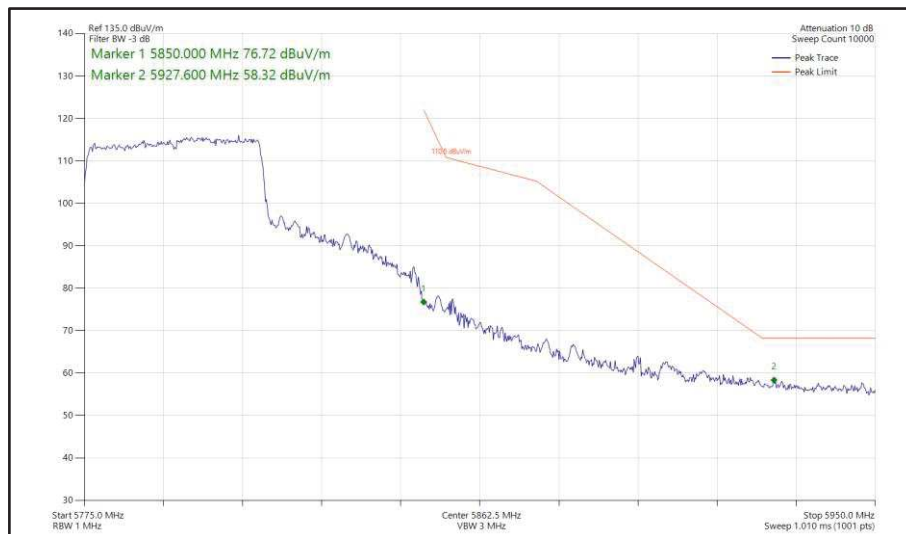
Figure 479 - 802.11ax HE40, SU, SISO, Core 1 - 5795 MHz Band Edge Frequency 5850 MHz
