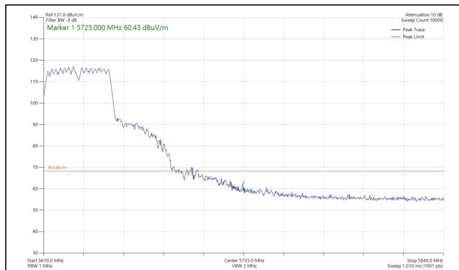
Figure 489 - 802.11n HT40, CDD, Core 0 + Core 1 - 5630 MHz Band Edge Frequency 5725 MHz
