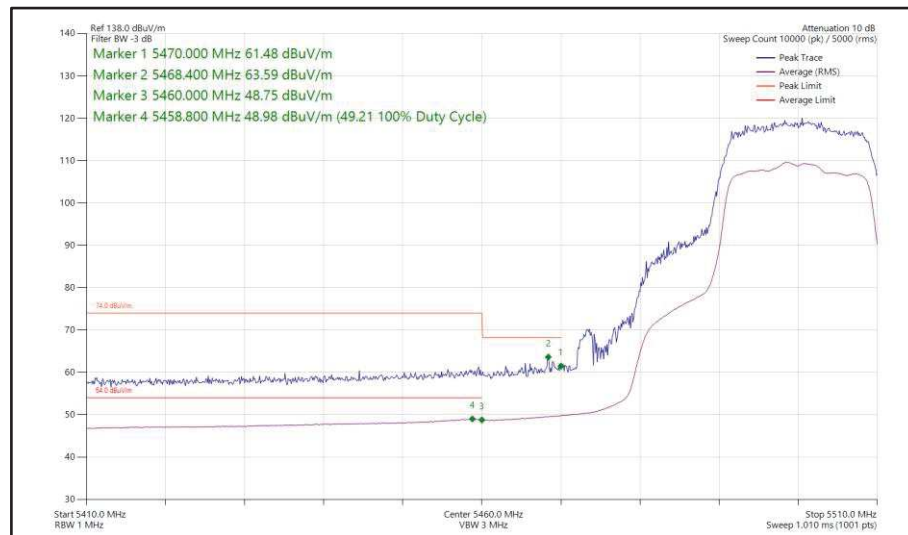
Figure 434 - 802.11ac VHT20, TxBF, Core 0 + Core 1 - 5500 MHz Band Edge Frequency 5470 MHz
