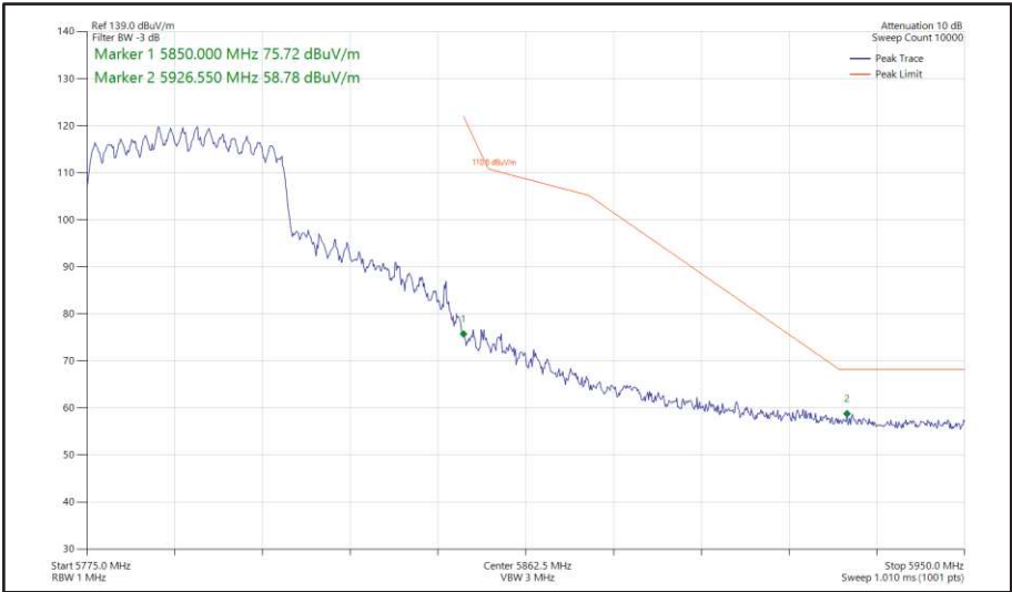
Figure 498 - 802.11ax HE40, SU, CDD, Core 0 + Core 1 - 5795 MHz Band Edge Frequency 5850 MHz
