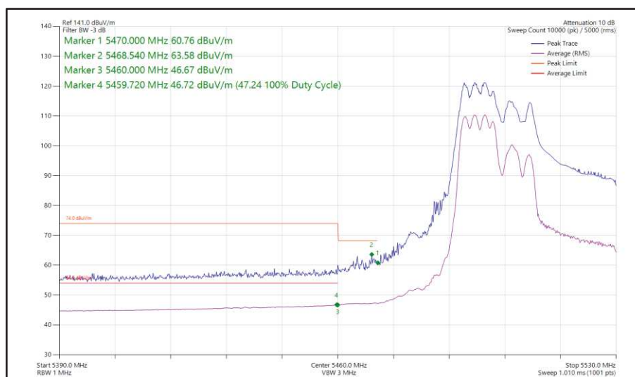
Figure 484 - 802.11ax HE40, RU 106-53, CDD, Core 0 + Core 1 - 5510 MHz Band Edge Frequency 5470 MHz
