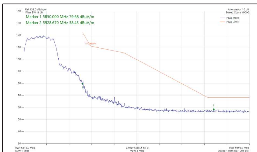
Figure 442 - 802.11ac VHT20, TxBF, Core 0 + Core 1 - 5825 MHz Band Edge Frequency 5850 MHz
