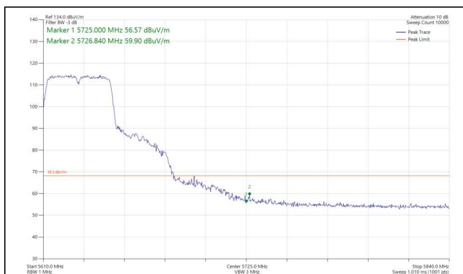
Figure 451 - 802.11n HT40, SISO, Core 0 - 5630 MHz Band Edge Frequency 5725 MHz
