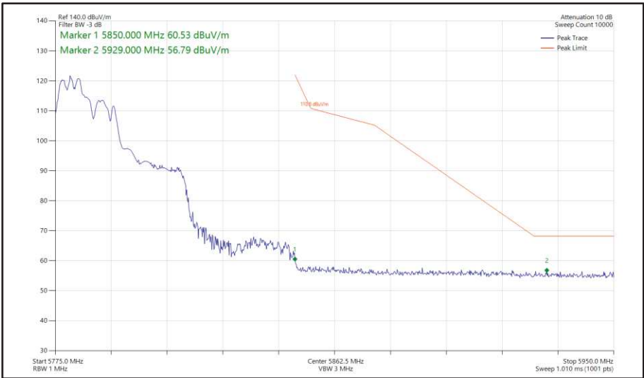
Figure 499 - 802.11ax HE40, RU 106-53, CDD, Core 0 + Core 1 - 5795 MHz Band Edge Frequency 5850 MHz
