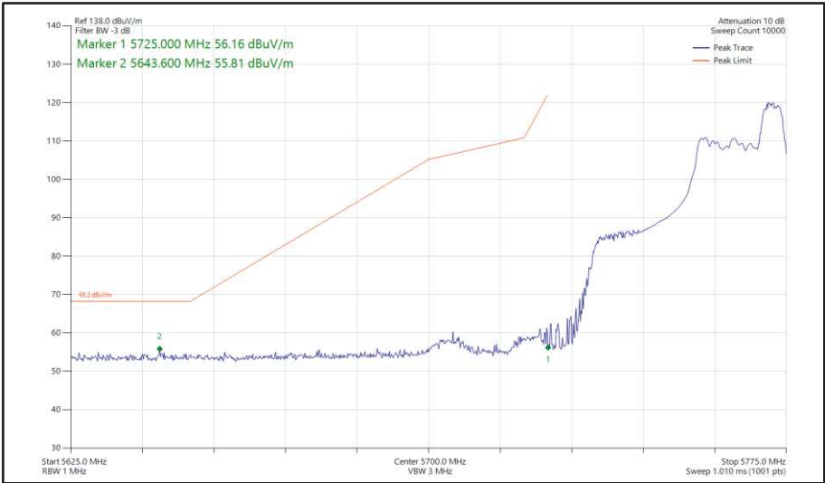
Figure 469 - 802.11ax HE40, RU 52-44, SISO, Core 1 - 5755 MHz Band Edge Frequency 5725 MHz
