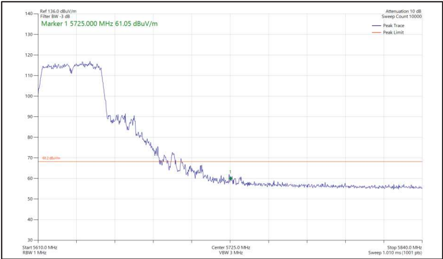
Figure 522 - 802.11ac VHT40, TxBF, Core 0 + Core 1 - 5630 MHz Band Edge Frequency 5725 MHz
