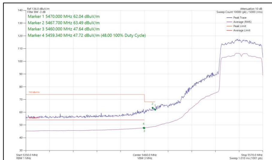
Figure 447 - 802.11ax HE40, SU, SISO, Core 0 - 5550 MHz Band Edge Frequency 5470 MHz
