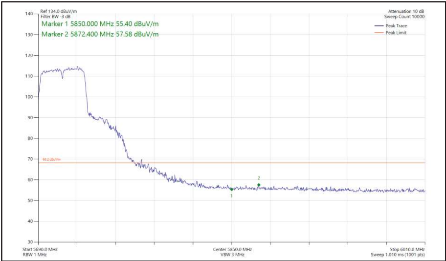
Figure 475 - 802.11n HT40, SISO, Core 1 - 5710 MHz Band Edge Frequency 5850 MHz
