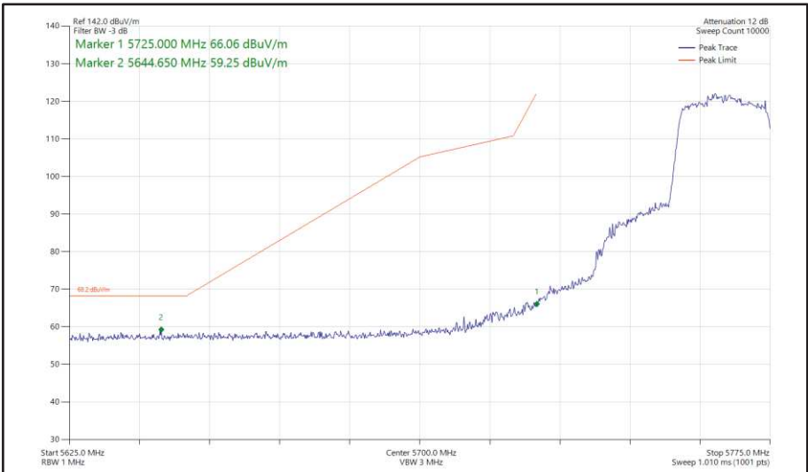
Figure 420 - 802.11ax HE20, SU, SDM, Core 0 + Core 1 - 5765 MHz Band Edge Frequency 5725 MHz
