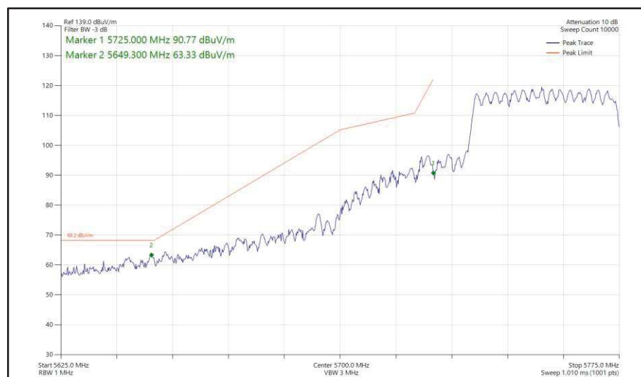
Figure 487 - 802.11ax HE40, SU, CDD, Core 0 + Core 1 - 5755 MHz Band Edge Frequency 5725 MHz
