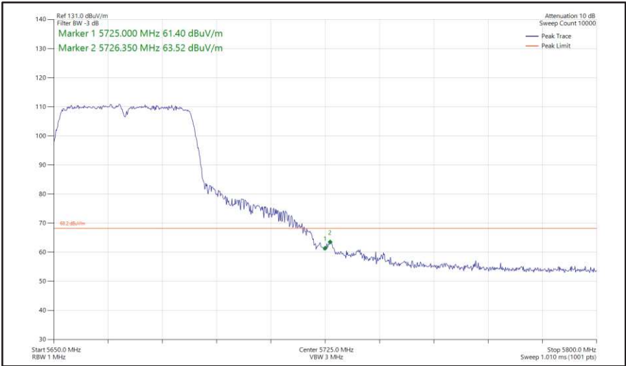
Figure 452 - 802.11n HT40, SISO, Core 0 - 5670 MHz Band Edge Frequency 5725 MHz
