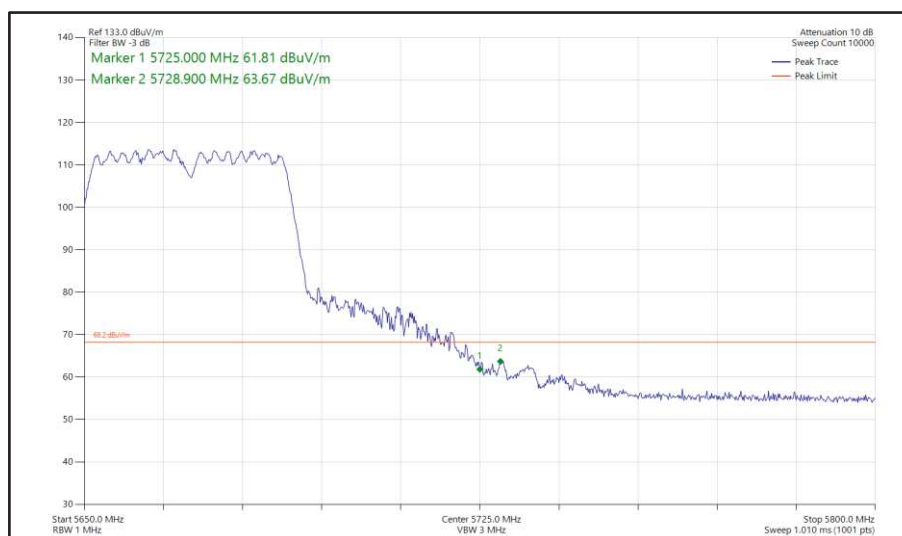
Figure 490 - 802.11n HT40, CDD, Core 0 + Core 1 - 5670 MHz Band Edge Frequency 5725 MHz
