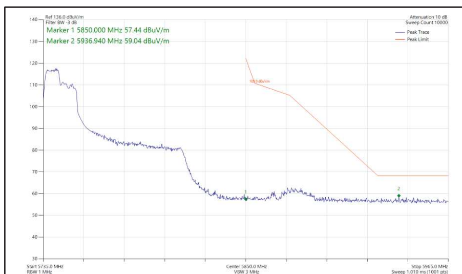
Figure 540 - 802.11ax HE80, RU 106-53, SISO, Core 0 - 5775 MHz Band Edge Frequency 5850 MHz
