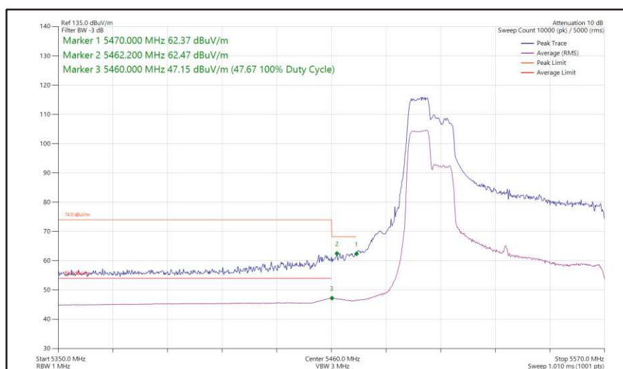
Figure 543 - 802.11ax HE80, RU 106-53, SISO, Core 1 - 5530 MHz Band Edge Frequency 5470 MHz
