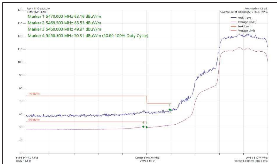
Figure 413 - 802.11ax HE20, SU, SDM, Core 0 + Core 1 - 5500 MHz Band Edge Frequency 5470 MHz
