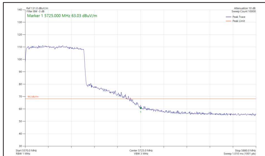
Figure 548 - 802.11ax HE80, SU, SISO, Core 1 - 5610 MHz Band Edge Frequency 5725 MHz
