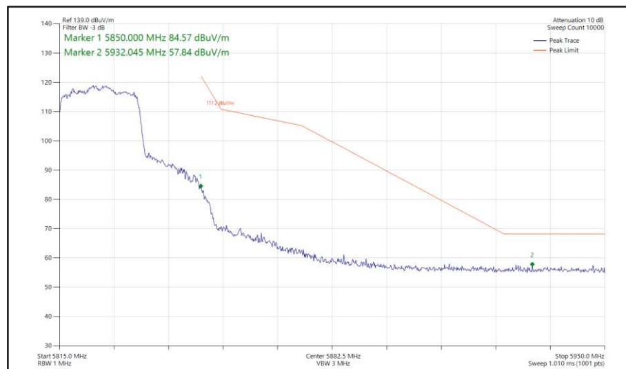
Figure 432 - 802.11ax HE20, SU, SDM, Core 0 + Core 1 - 5825 MHz Band Edge Frequency 5850 MHz
