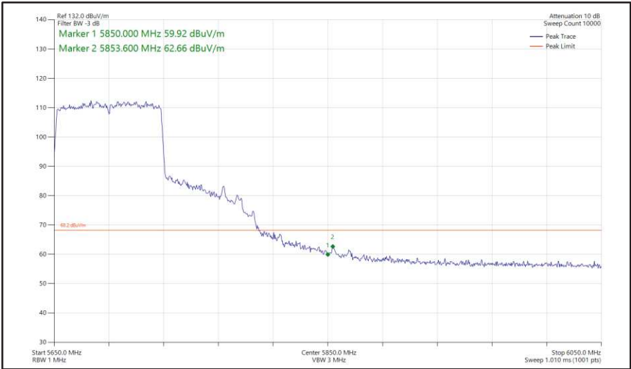
Figure 550 - 802.11ac VHT80, SISO, Core 1 - 5690 MHz Band Edge Frequency 5850 MHz
