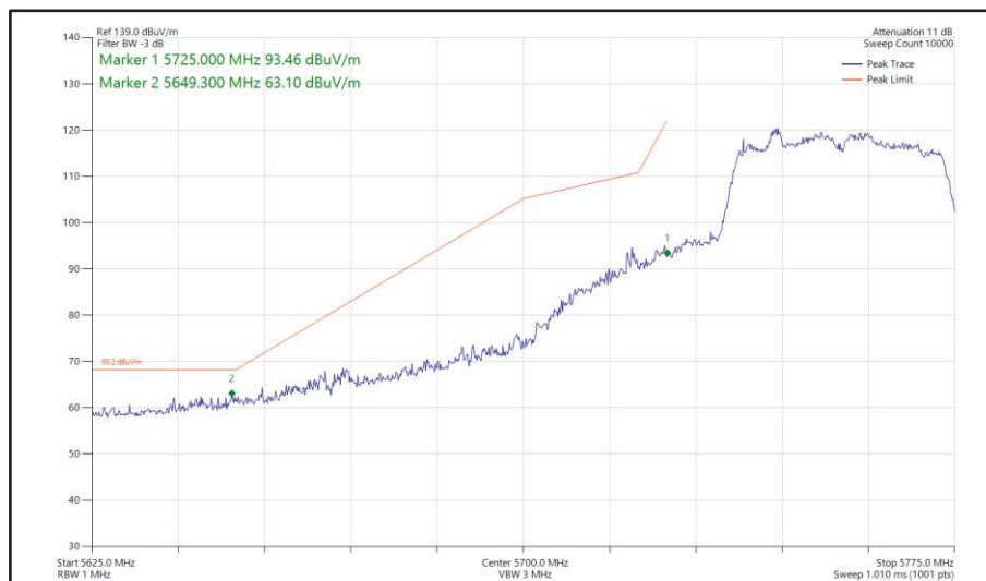
Figure 521 - 802.11ac VHT40, TxBF, Core 0 + Core 1 - 5755 MHz Band Edge Frequency 5725 MHz
