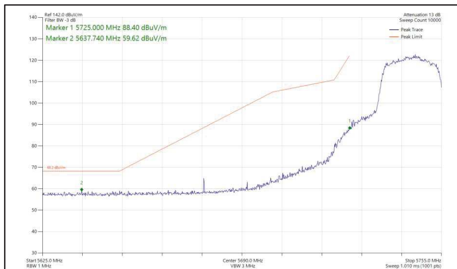
Figure 436 - 802.11ac VHT20, TxBF, Core 0 + Core 1 - 5745 MHz Band Edge Frequency 5725 MHz
