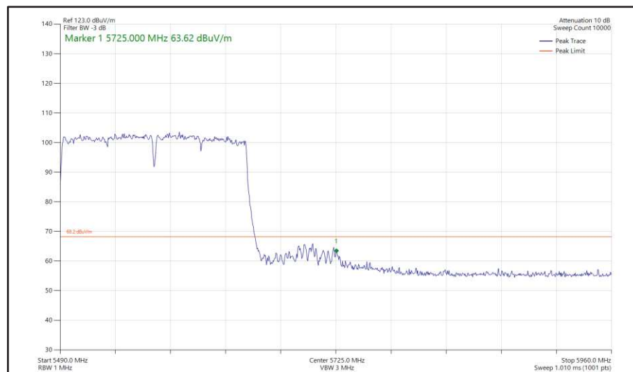
Figure 612 - 802.11ac VHT160, SDM, Core 0 + Core 1 - 5570 MHz Band Edge Frequency 5725 MHz
