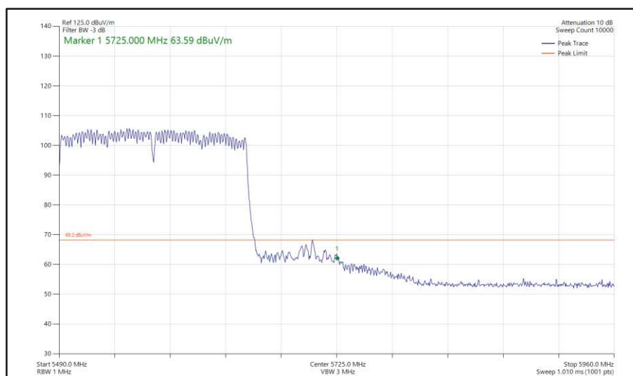
Figure 607 - 802.11ax HE160, SU, CDD, Core 0 + Core 1 - 5570 MHz Band Edge Frequency 5725 MHz
