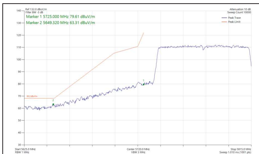
Figure 574 - 802.11ac VHT80, SDM, Core 0 + Core 1 - 5775 MHz Band Edge Frequency 5725 MHz
