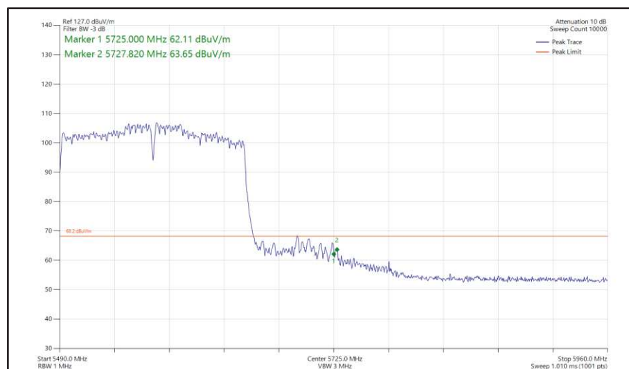
Figure 606 - 802.11ac VHT160, CDD, Core 0 + Core 1 - 5570 MHz Band Edge Frequency 5725 MHz
