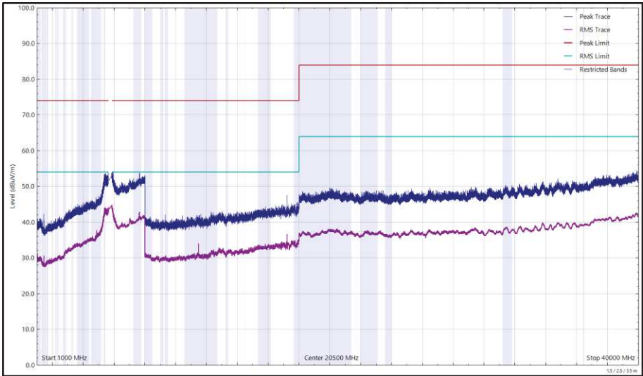
Figure 643 - U-NII-3 - 5745 MHz (CH149), HE20, RU26-0, CDD, Core 0 + Core 1, 1 GHz to 40 GHz, Vertical
