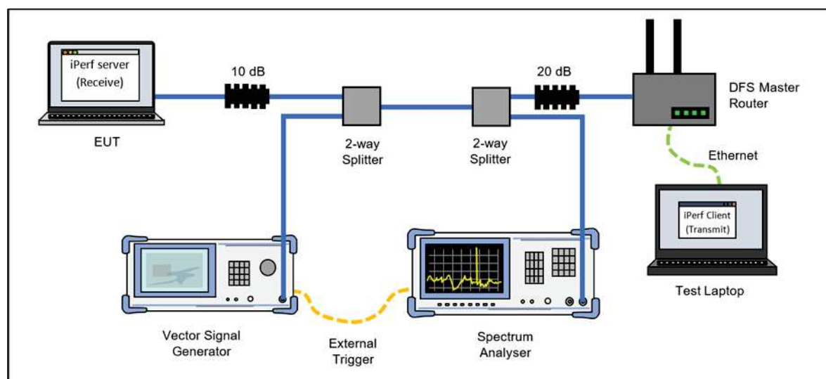
Figure 680 - Test Equipment Setup Diagram for Client without Radar Detection with Injection at the Master
