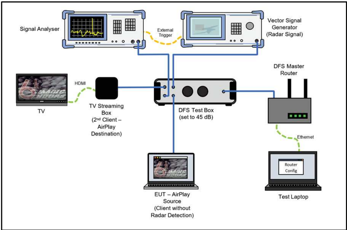
Figure 686- Test Equipment Setup Diagram for Client without Radar Detection with Injection at the Master
