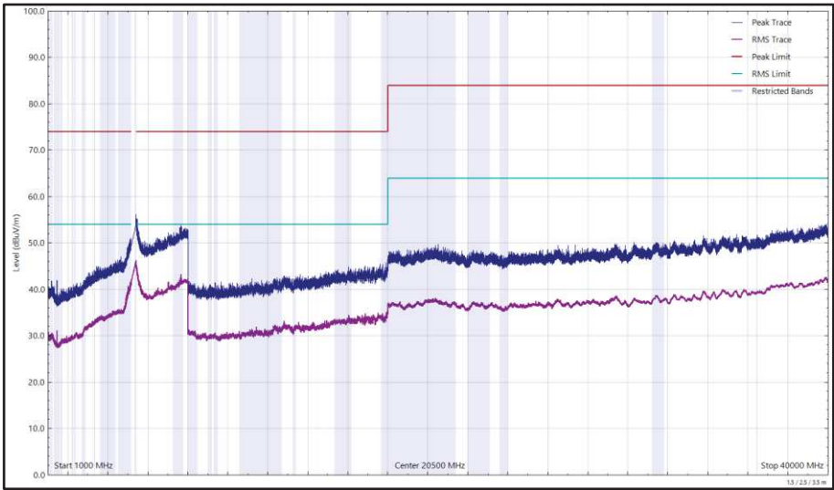
Figure 653 - U-NII-2A - 5320 MHz (CH64), 802.11a, Core 0, 1 GHz to 40 GHz, Vertical
