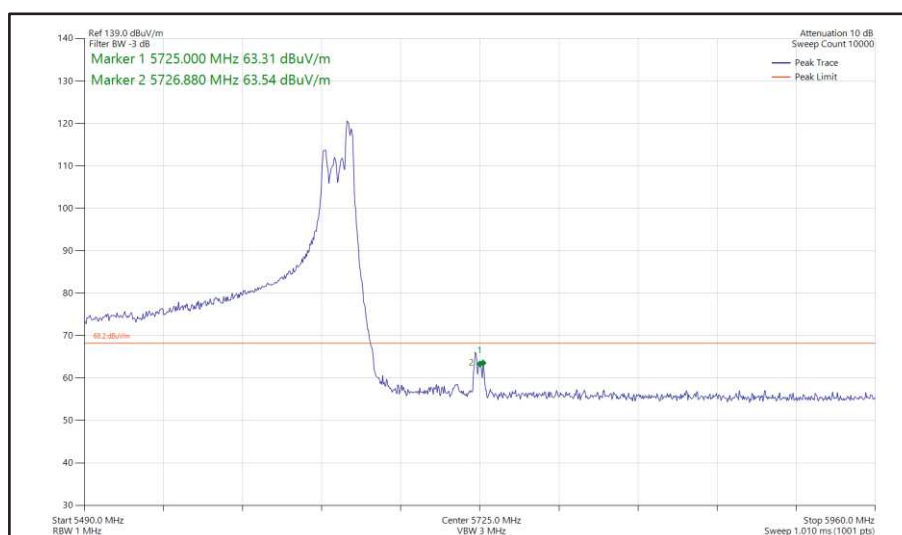
Figure 608 - 802.11ax HE160, RU 52-52, CDD, Core 0 + Core 1 - 5570 MHz Band Edge Frequency 5725 MHz
