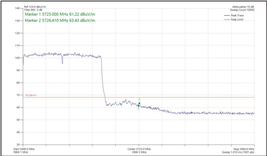
Figure 595 - 802.11ax HE160, SU, SISO, Core 0 - 5570 MHz Band Edge Frequency 5725 MHz
