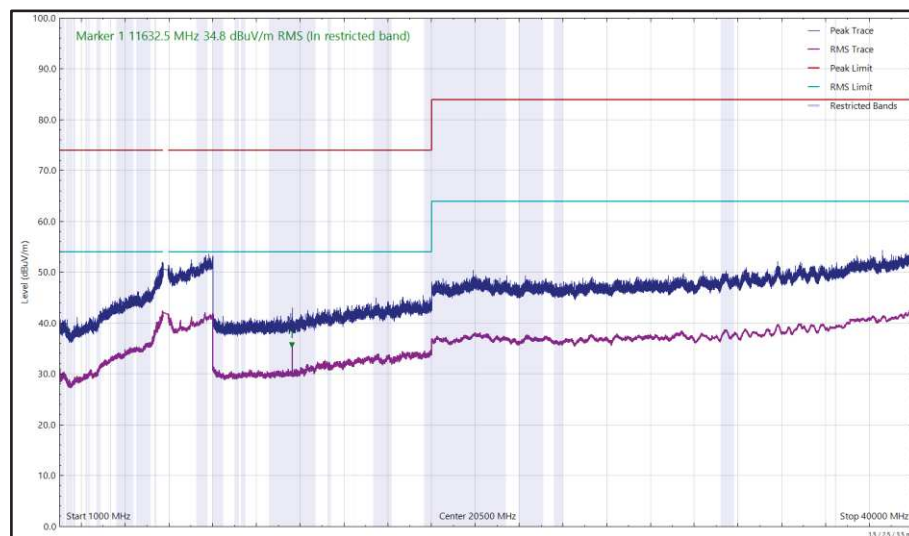
Figure 645 - U-NII-3 - 5825 MHz (CH165), HE20, RU26-0, CDD, Core 0 + Core 1, 1 GHz to 40 GHz, Horizontal
