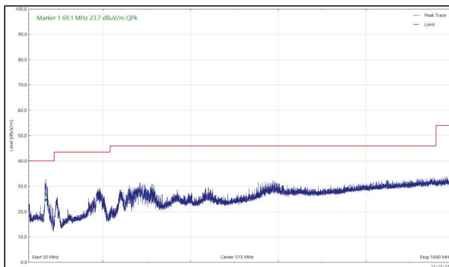
Figure 660 - U-NII-3 - 5825 MHz (CH165), 802.11a, Core 0, 30 MHz to 1 GHz, Horizontal (Peak)
