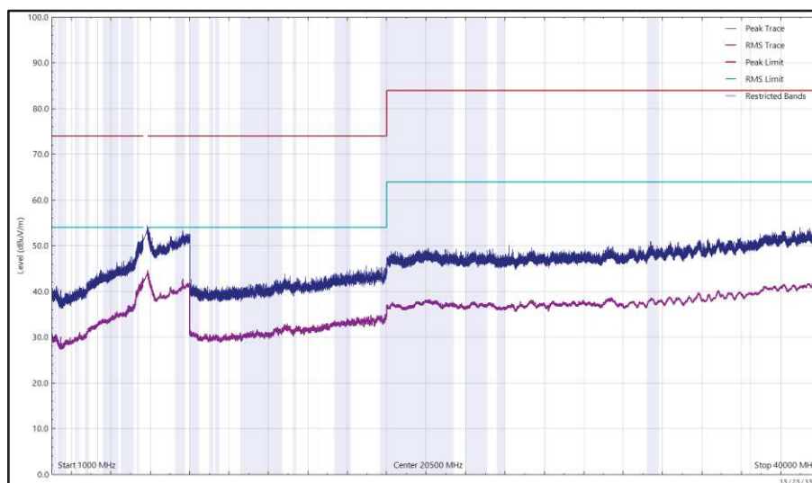
Figure 675 - U-NII-3 - 5745 MHz (CH149), 802.11a, Core 1, 1 GHz to 40 GHz, Vertical
