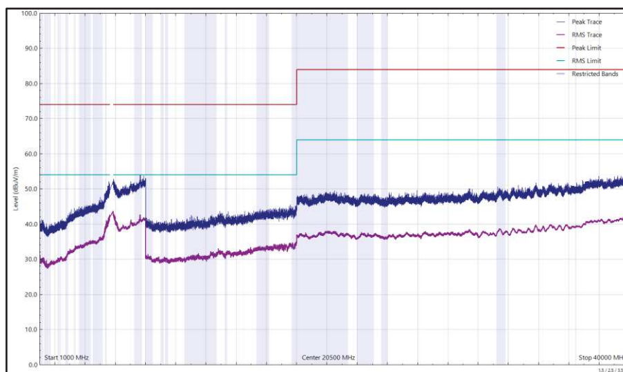
Figure 626 - U-NII-3 - 5745 MHz (CH149), HT20, CDD, Core 0 + Core 1, 1 GHz to 40 GHz, Horizontal
