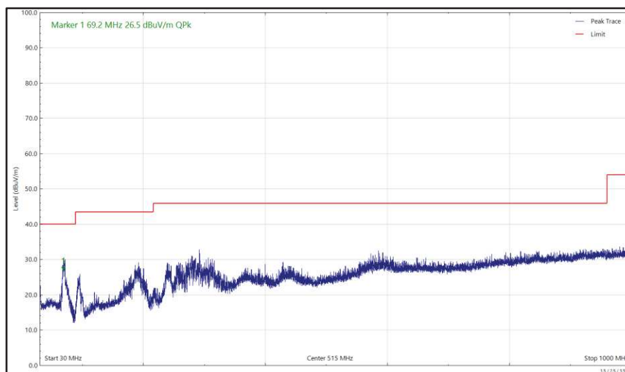
Figure 648 - U-NII-1 - 5180 MHz (CH36), 802.11a, Core 0, 30 MHz to 1 GHz, Horizontal (Peak)
