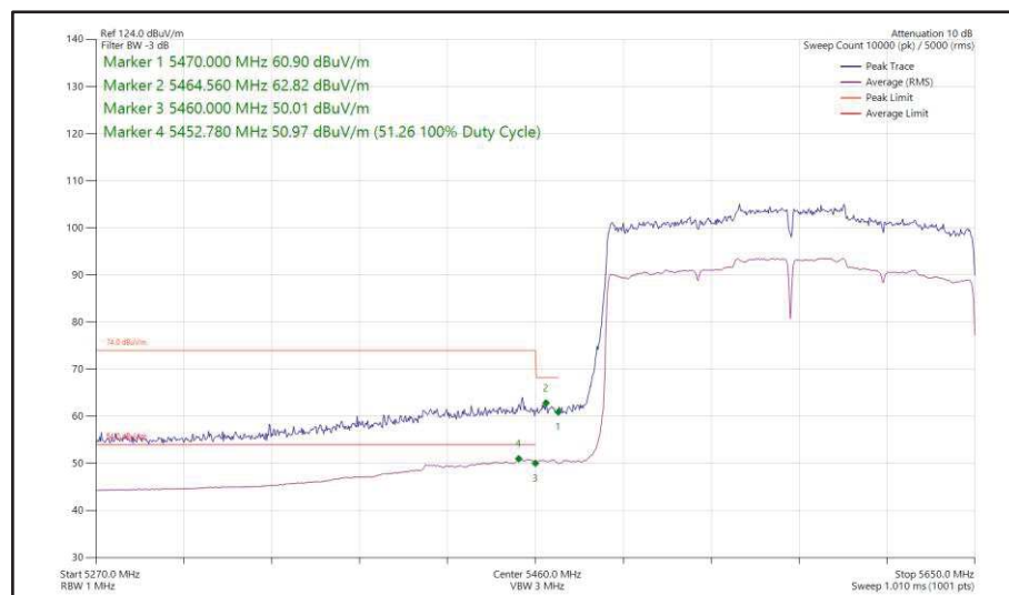
Figure 592 - 802.11ax HE160, SU, SISO, Core 0 - 5570 MHz Band Edge Frequency 5470 MHz
