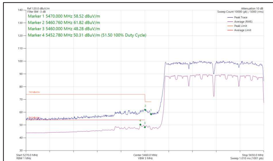
Figure 591 - 802.11ac VHT160, SISO, Core 0 - 5570 MHz Band Edge Frequency 5470 MHz
