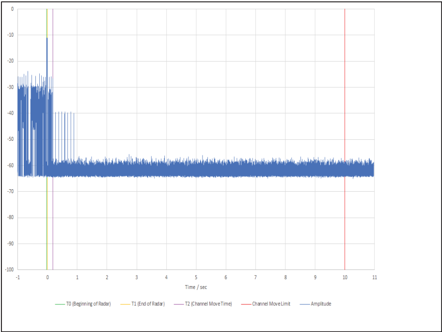
Figure 690 - First 12 s of Channel Shutdown Period
