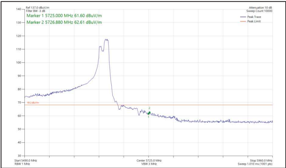
Figure 596 - 802.11ax HE160, RU 106-60, SISO, Core 0 - 5570 MHz Band Edge Frequency 5725 MHz
