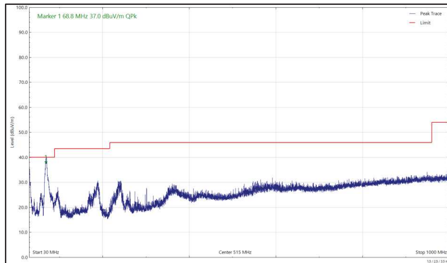
Figure 618 - U-NII-1 - 5180 MHz (CH36), HT20, CDD, Core 0 + Core 1, 30 MHz to 1 GHz, Vertical (Peak)
