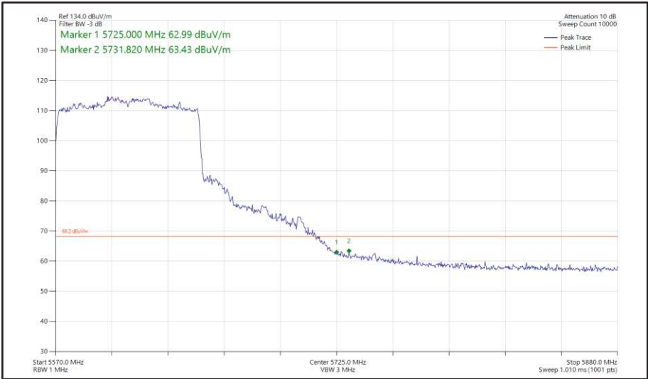
Figure 578 - 802.11ax HE80, SU, SDM, Core 0 + Core 1 - 5610 MHz Band Edge Frequency 5725 MHz
