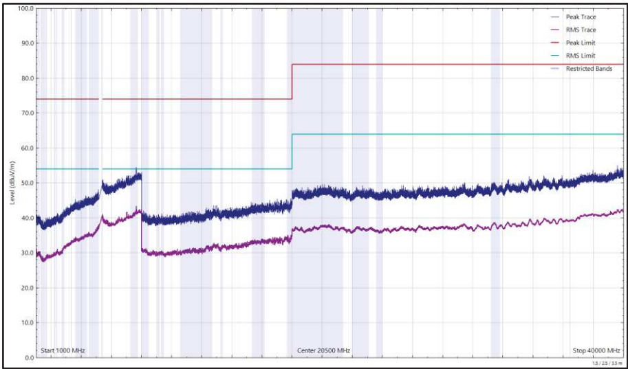
Figure 652 - U-NII-2A - 5320 MHz (CH64), 802.11a, Core 0, 1 GHz to 40 GHz, Horizontal
