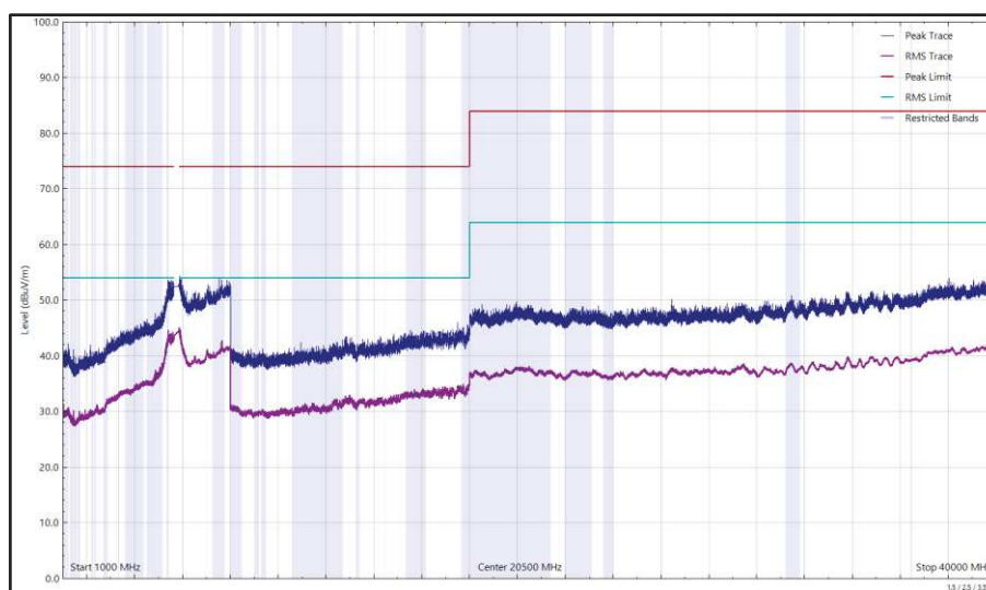
Figure 627 - U-NII-3 - 5745 MHz (CH149), HT20, CDD, Core 0 + Core 1, 1 GHz to 40 GHz, Vertical
