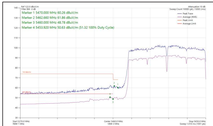
Figure 597 - 802.11ac VHT160, SISO, Core 1 - 5570 MHz Band Edge Frequency 5470 MHz
