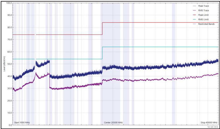
Figure 620 - U-NII-2A - 5320 MHz (CH64), HT20, CDD, Core 0 + Core 1, 1 GHz to 40 GHz, Horizontal
