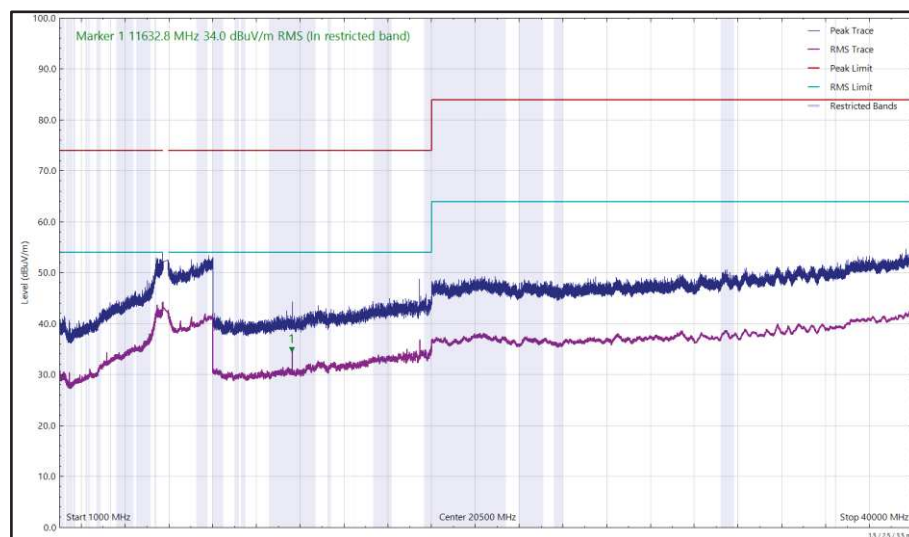
Figure 647 - U-NII-3 - 5825 MHz (CH165), HE20, RU26-0, CDD, Core 0 + Core 1, 1 GHz to 40 GHz, Vertical
