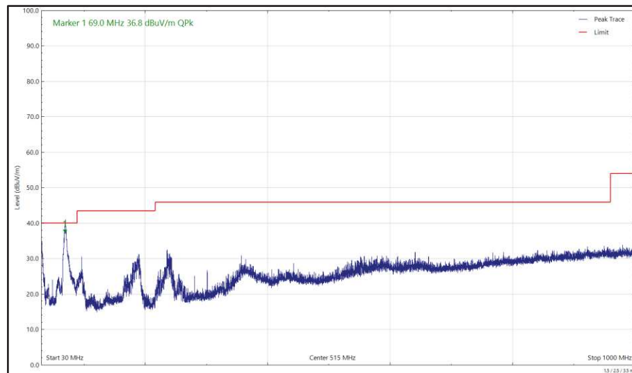
Figure 662 - U-NII-3 - 5825 MHz (CH165), 802.11a, Core 0, 30 MHz to 1 GHz, Vertical (Peak)
