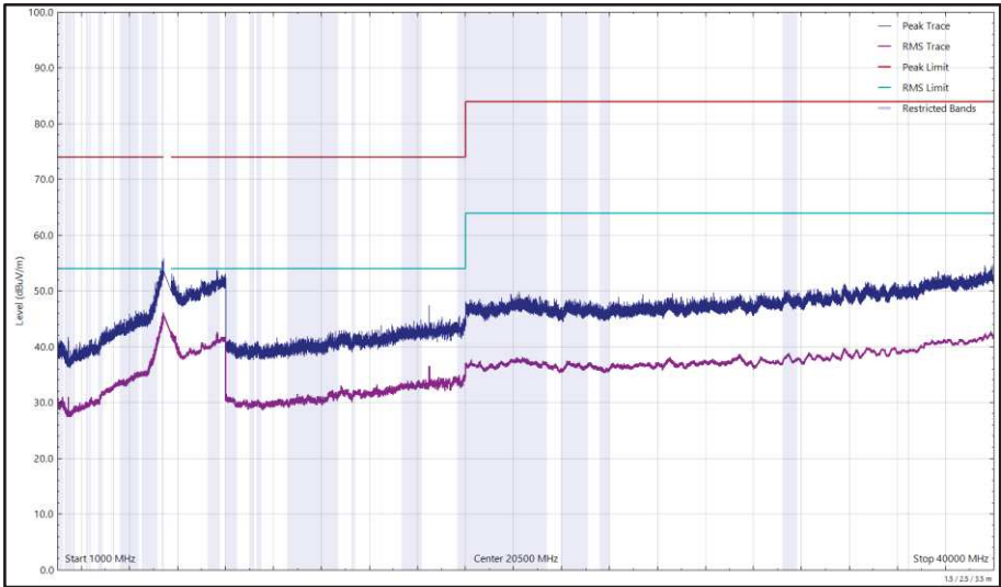
Figure 639 - U-NII-2C - 5500 MHz (CH100), HE20, RU52-37, CDD, Core 0 + Core 1, 1 GHz to 40 GHz, Vertical
