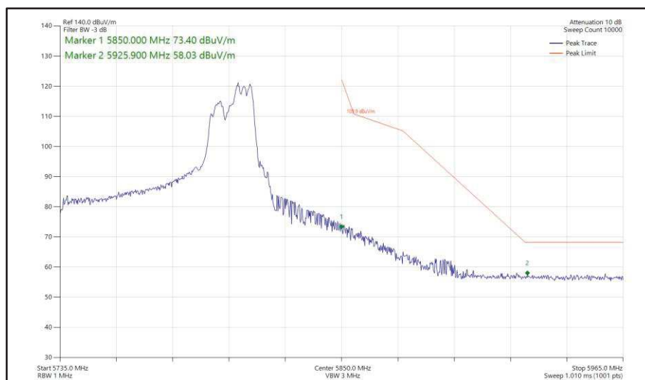
Figure 585 - 802.11ax HE80, RU 106-60, SDM, Core 0 + Core 1 - 5775 MHz Band Edge Frequency 5850 MHz
