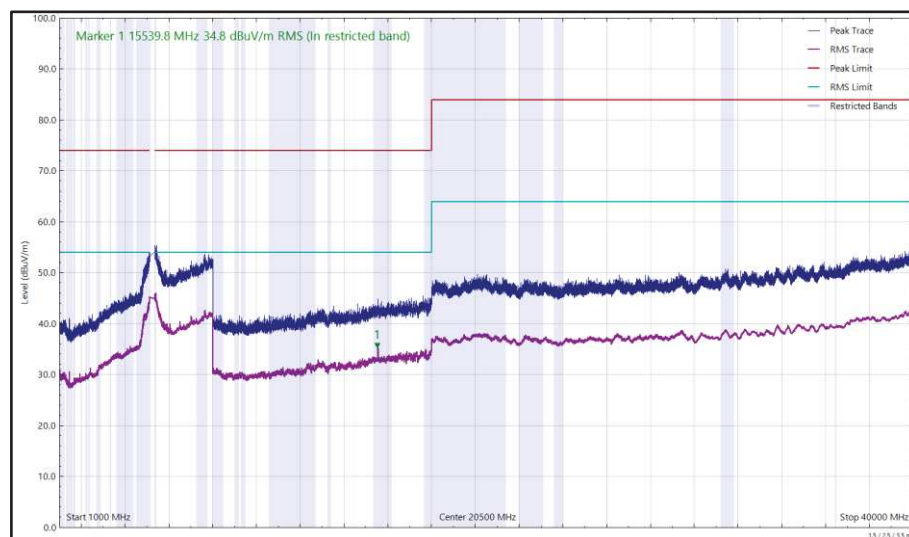
Figure 619 - U-NII-1 - 5180 MHz (CH36), HT20, CDD, Core 0 + Core 1, 1 GHz to 40 GHz, Vertical
