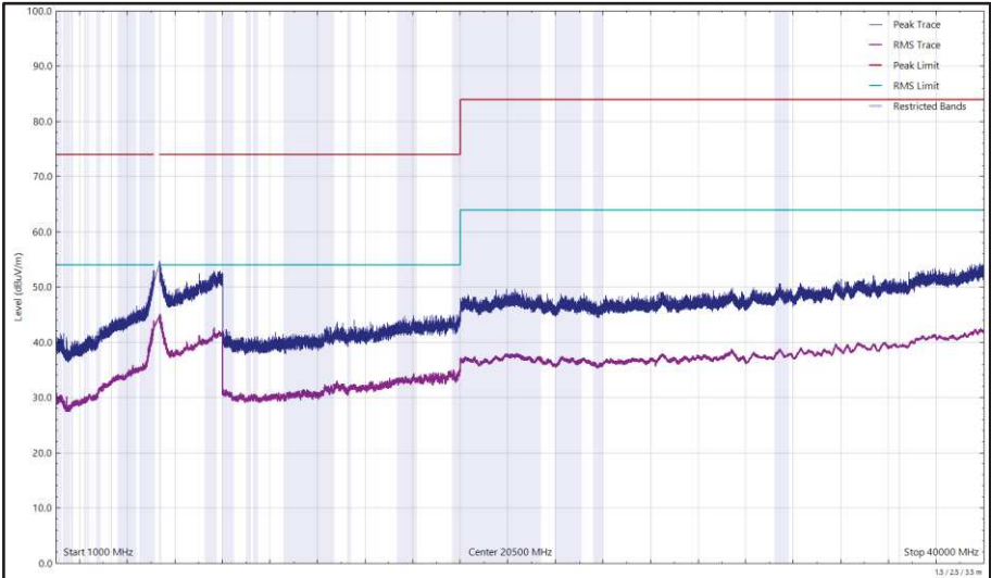
Figure 651 - U-NII-1 - 5180 MHz (CH36), 802.11a, Core 0, 1 GHz to 40 GHz, Vertical
