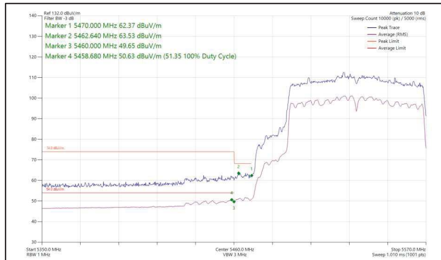
Figure 571 - 802.11ac VHT80, SDM, Core 0 + Core 1 - 5530 MHz Band Edge Frequency 5470 MHz
