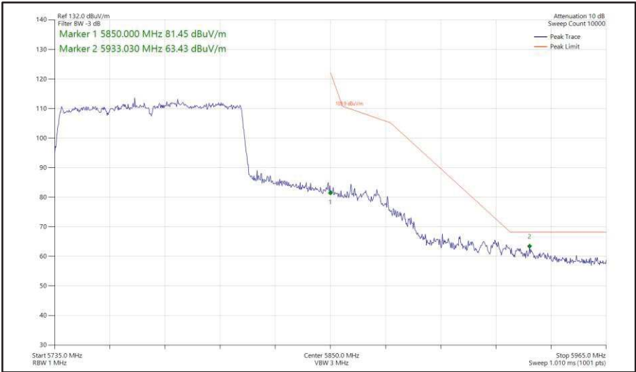
Figure 590 - 802.11ac VHT80, TxBF, Core 0 + Core 1 - 5775 MHz Band Edge Frequency 5850 MHz
