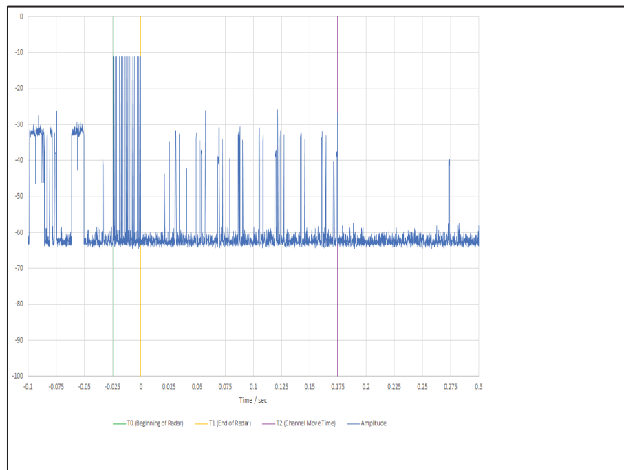
Figure 689 - First 200 ms of Channel Shutdown Period
