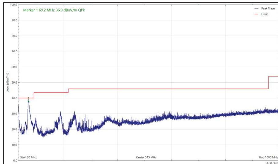
Figure 630 - U-NII-3 - 5825 MHz (CH165), HT20, CDD, Core 0 + Core 1, 30 MHz to 1 GHz, Vertical (Peak)
