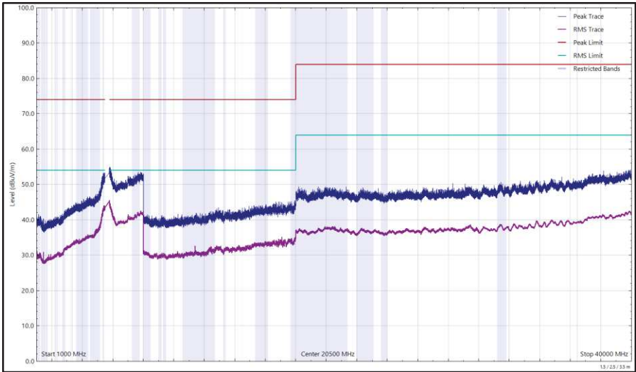
Figure 641 - U-NII-2C - 5700 MHz (CH140), HE20, RU52-37, CDD, Core 0 + Core 1, 1 GHz to 40 GHz, Vertical
