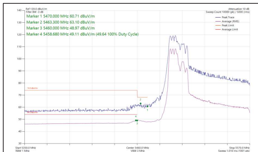
Figure 573 - 802.11ax HE80, RU 106-53, SDM, Core 0 + Core 1 - 5530 MHz Band Edge Frequency 5470 MHz
