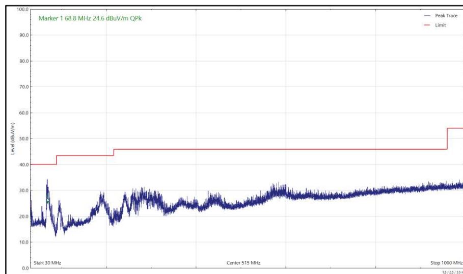
Figure 632 - U-NII-1 - 5180 MHz (CH36), HE20, RU26-0, CDD, Core 0 + Core 1, 30 MHz to 1 GHz, Horizontal (Peak)
