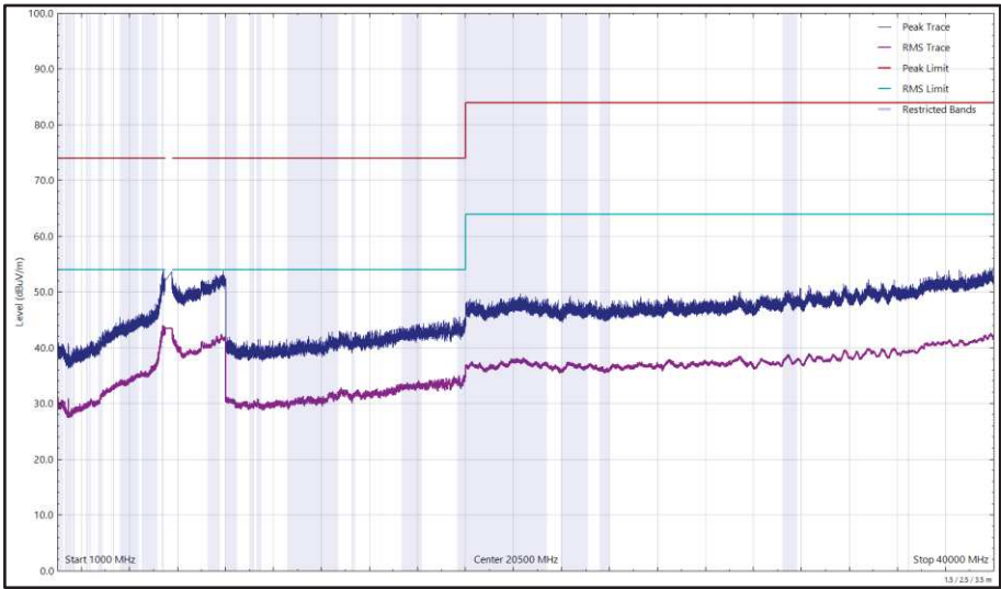
Figure 657 - U-NII-2C - 5700 MHz (CH140), 802.11a, Core 0, 1 GHz to 40 GHz, Vertical
