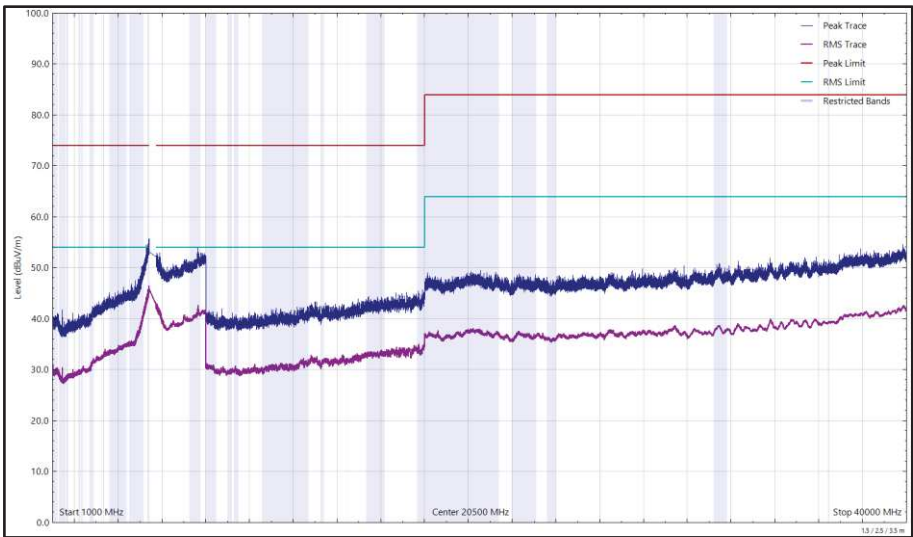
Figure 623 - U-NII-2C - 5500 MHz (CH100), HT20, CDD, Core 0 + Core 1, 1 GHz to 40 GHz, Vertical
