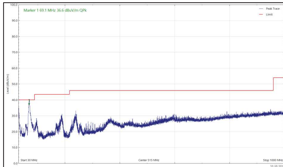
Figure 678 - U-NII-3 - 5825 MHz (CH165), 802.11a, Core 1, 30 MHz to 1 GHz, Vertical (Peak)
