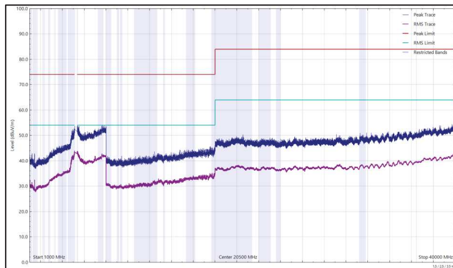
Figure 667 - U-NII-1 - 5180 MHz (CH36), 802.11a, Core 1, 1 GHz to 40 GHz, Vertical
