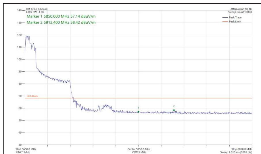
Figure 583 - 802.11ax HE80, RU 106-53, SDM, Core 0 + Core 1 - 5690 MHz Band Edge Frequency 5850 MHz
