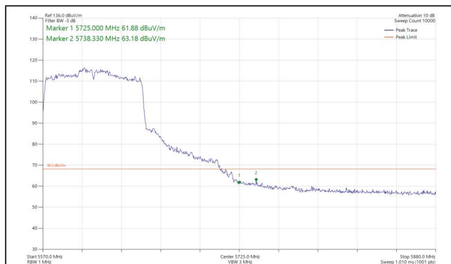
Figure 577 - 802.11ac VHT80, SDM, Core 0 + Core 1 - 5610 MHz Band Edge Frequency 5725 MHz
