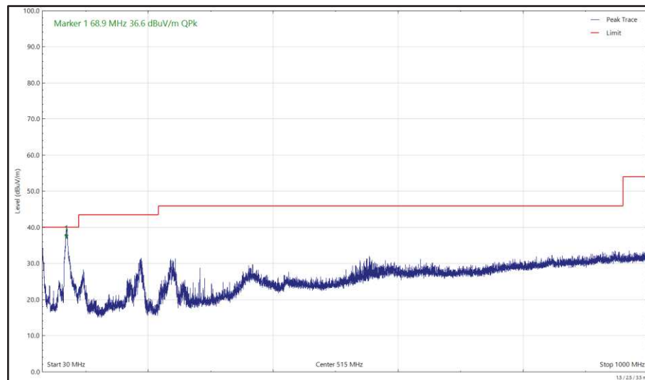
Figure 666 - U-NII-1 - 5180 MHz (CH36), 802.11a, Core 1, 30 MHz to 1 GHz, Vertical (Peak)
