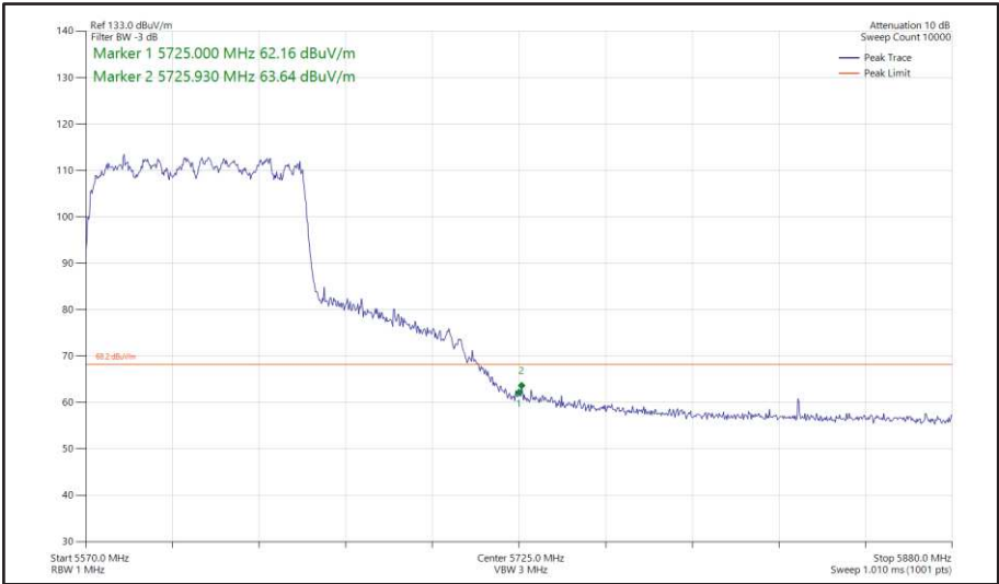
Figure 588 - 802.11ac VHT80, TxBF, Core 0 + Core 1 - 5610 MHz Band Edge Frequency 5725 MHz
