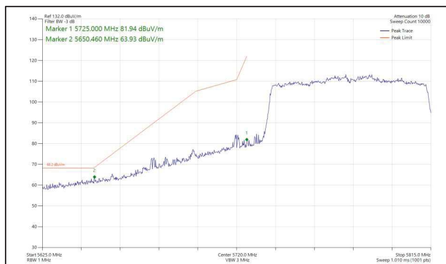
Figure 587 - 802.11ac VHT80, TxBF, Core 0 + Core 1 - 5775 MHz Band Edge Frequency 5725 MHz
