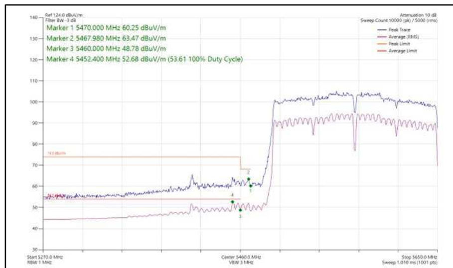
Figure 609 - 802.11ac VHT160, SDM, Core 0 + Core 1 - 5570 MHz Band Edge Frequency 5470 MHz
