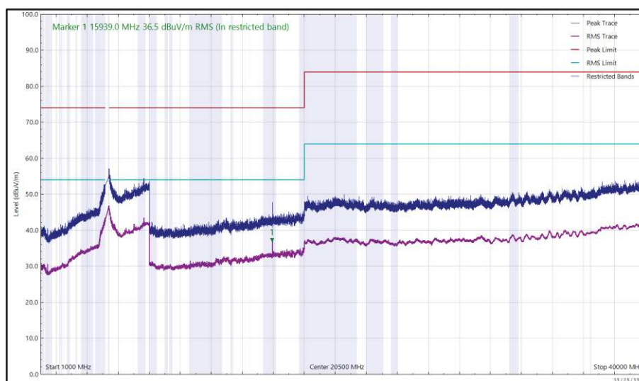
Figure 637 - U-NII-2A - 5320 MHz (CH64), HE20, RU52-37, CDD, Core 0 + Core 1, 1 GHz to 40 GHz, Vertical
