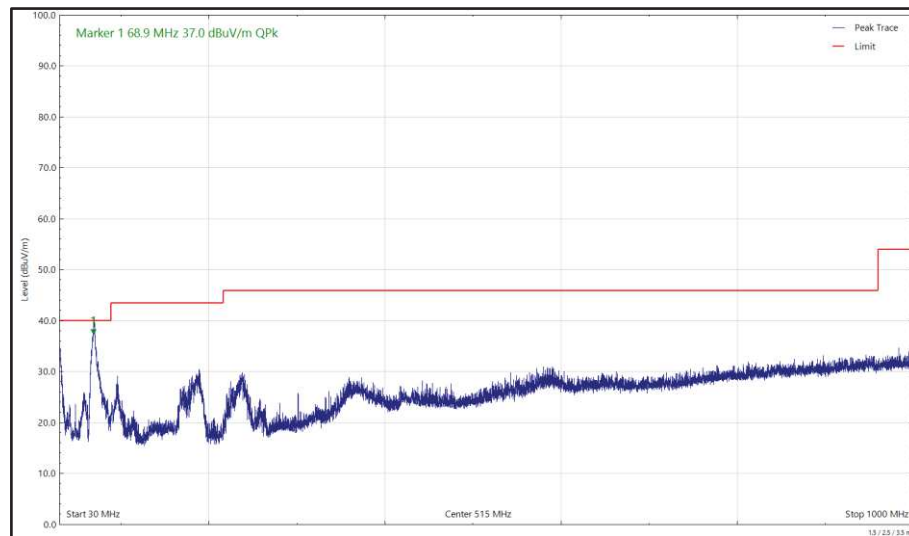
Figure 646 - U-NII-3 - 5825 MHz (CH165), HE20, RU26-0, CDD, Core 0 + Core 1, 30 MHz to 1 GHz, Vertical (Peak)
