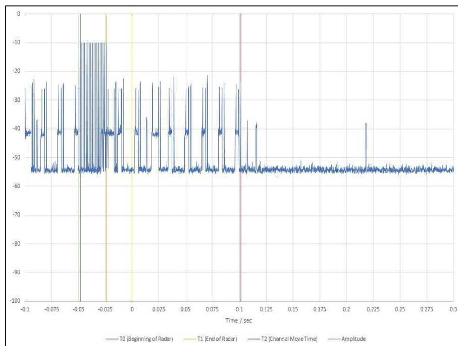
Figure 683 - First 200 ms of Channel Shutdown Period
