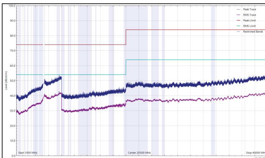
Figure 665 - U-NII-1 - 5180 MHz (CH36), 802.11a, Core 1, 1 GHz to 40 GHz, Horizontal
