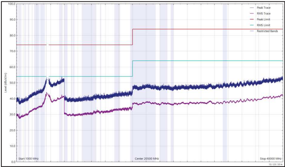
Figure 671 - U-NII-2C - 5500 MHz (CH100), 802.11a, Core 1, 1 GHz to 40 GHz, Vertical
