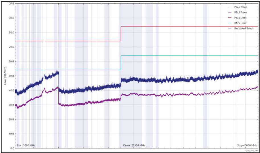
Figure 656 - U-NII-2C - 5700 MHz (CH140), 802.11a, Core 0, 1 GHz to 40 GHz, Horizontal
