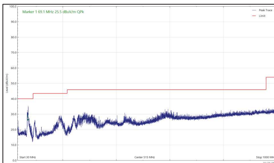
Figure 616 - U-NII-1 - 5180 MHz (CH36), HT20, CDD, Core 0 + Core 1, 30 MHz to 1 GHz, Horizontal (Peak)
