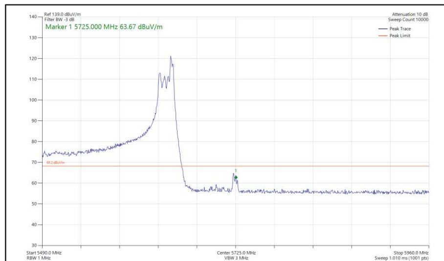
Figure 614 - 802.11ax HE160, RU 52-52, SDM, Core 0 + Core 1 - 5570 MHz Band Edge Frequency 5725 MHz
