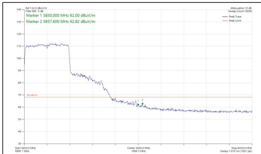
Figure 580 - 802.11ac VHT80, SDM, Core 0 + Core 1 - 5690 MHz Band Edge Frequency 5850 MHz
