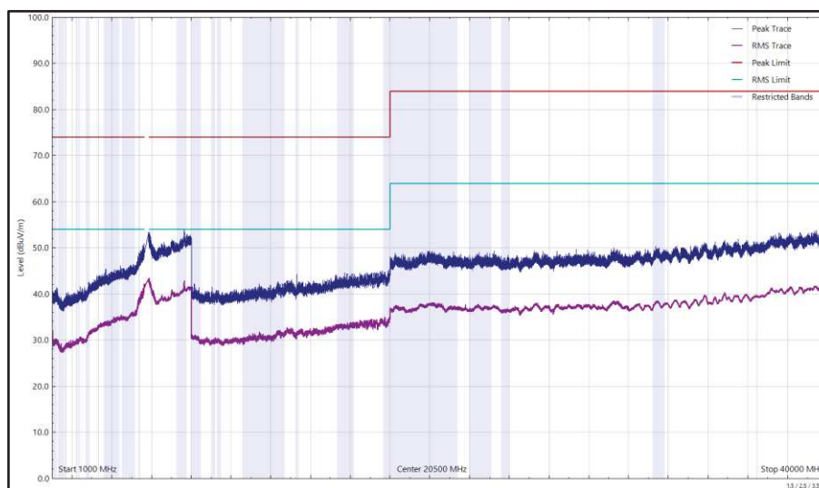
Figure 674 - U-NII-3 - 5745 MHz (CH149), 802.11a, Core 1, 1 GHz to 40 GHz, Horizontal
