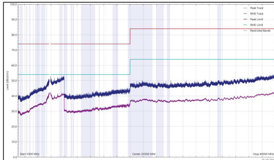
Figure 677 - U-NII-3 - 5825 MHz (CH165), 802.11a, Core 1, 1 GHz to 40 GHz, Horizontal
