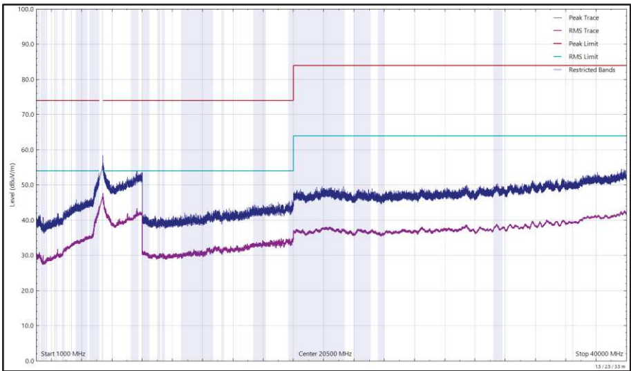
Figure 621 - U-NII-2A - 5320 MHz (CH64), HT20, CDD, Core 0 + Core 1, 1 GHz to 40 GHz, Vertical
