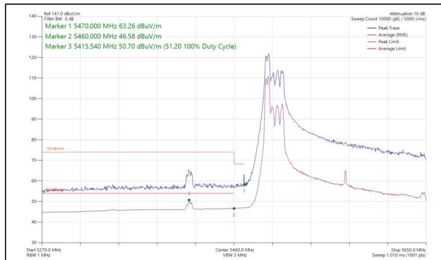
Figure 611 - 802.11ax HE160, RU 52-37, SDM, Core 0 + Core 1 - 5570 MHz Band Edge Frequency 5470 MHz
