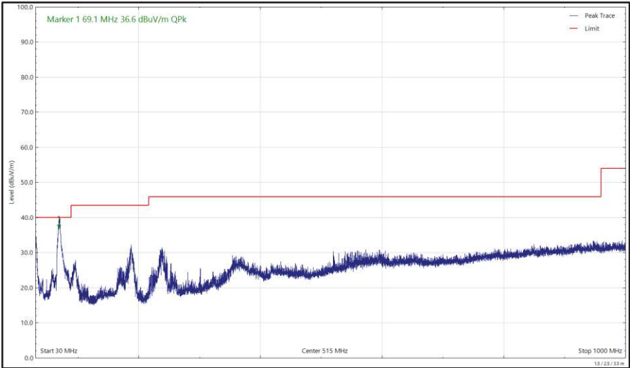
Figure 650 - U-NII-1 - 5180 MHz (CH36), 802.11a, Core 0, 30 MHz to 1 GHz, Vertical (Peak)
