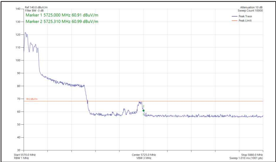
Figure 579 - 802.11ax HE80, RU 52-37, SDM, Core 0 + Core 1 - 5610 MHz Band Edge Frequency 5725 MHz
