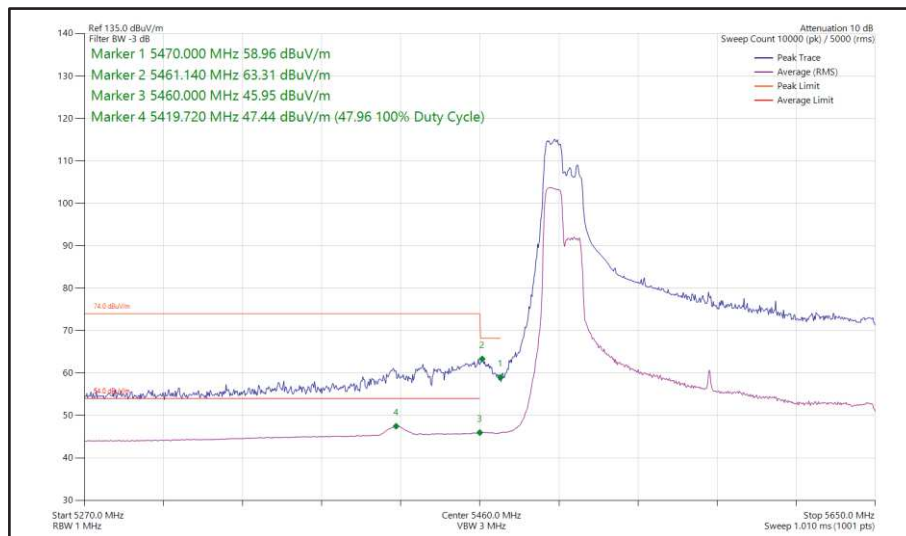
Figure 599 - 802.11ax HE160, RU 106-53, SISO, Core 1 - 5570 MHz Band Edge Frequency 5470 MHz
