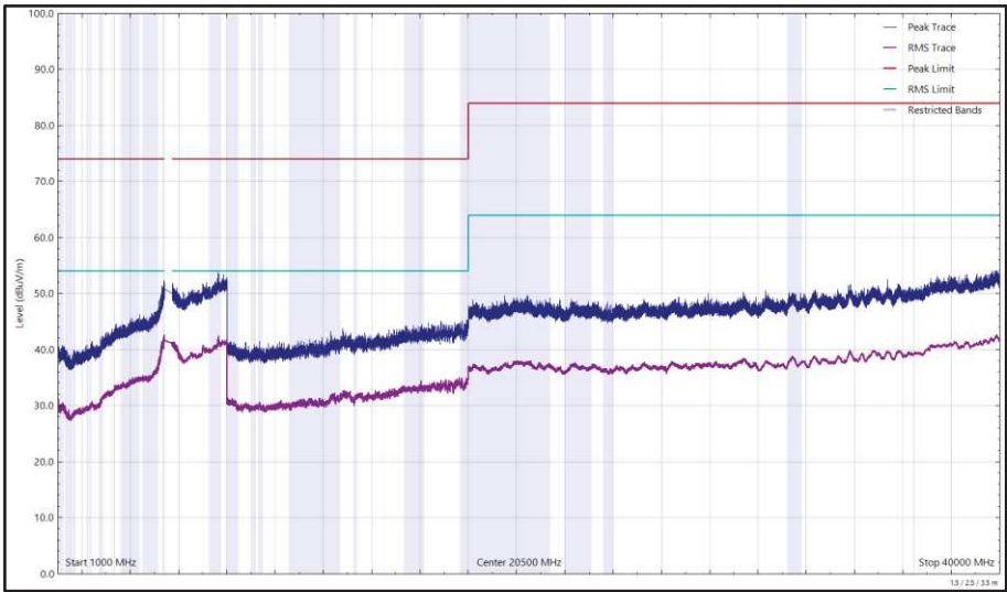
Figure 622 - U-NII-2C - 5500 MHz (CH100), HT20, CDD, Core 0 + Core 1, 1 GHz to 40 GHz, Horizontal
