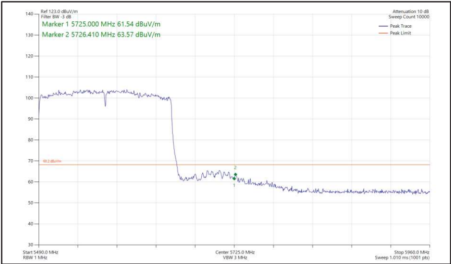
Figure 601 - 802.11ax HE160, SU, SISO, Core 1 - 5570 MHz Band Edge Frequency 5725 MHz
