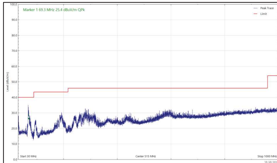
Figure 628 - U-NII-3 - 5825 MHz (CH165), HT20, CDD, Core 0 + Core 1, 30 MHz to 1 GHz, Horizontal (Peak)
