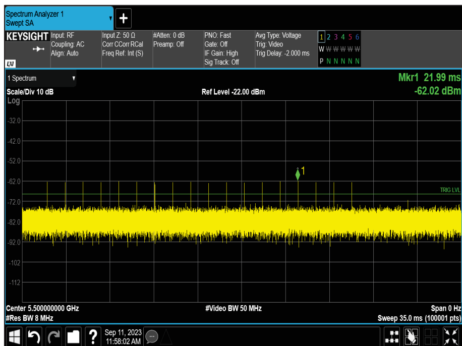
Figure 687- Verification of Radar Type 0
