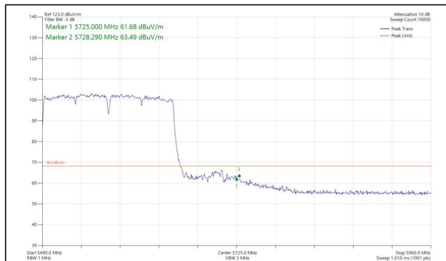
Figure 594 - 802.11ac VHT160, SISO, Core 0 - 5570 MHz Band Edge Frequency 5725 MHz
