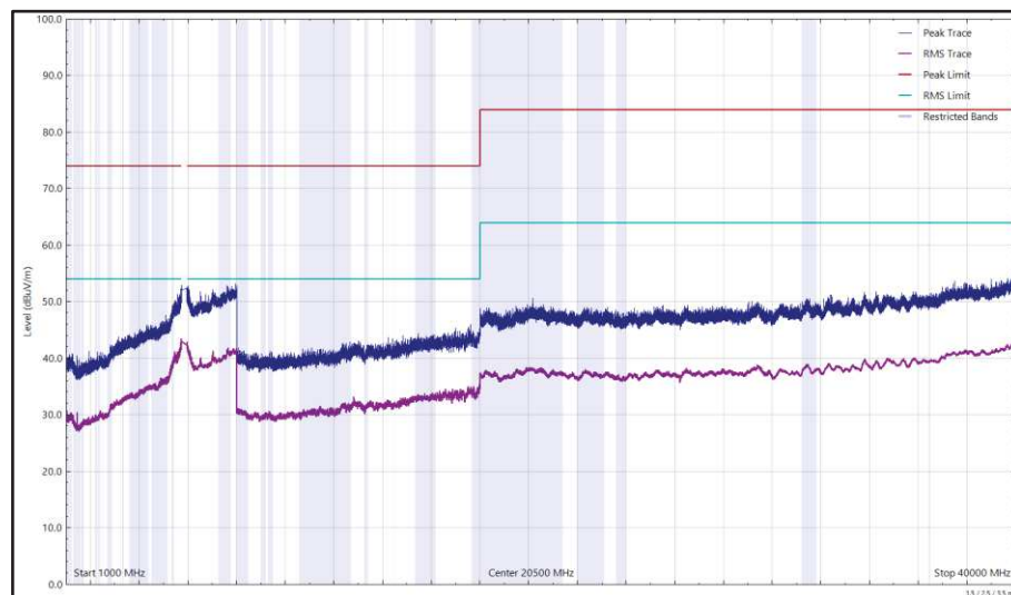
Figure 679 - U-NII-3 - 5825 MHz (CH165), 802.11a, Core 1, 1 GHz to 40 GHz, Vertical
