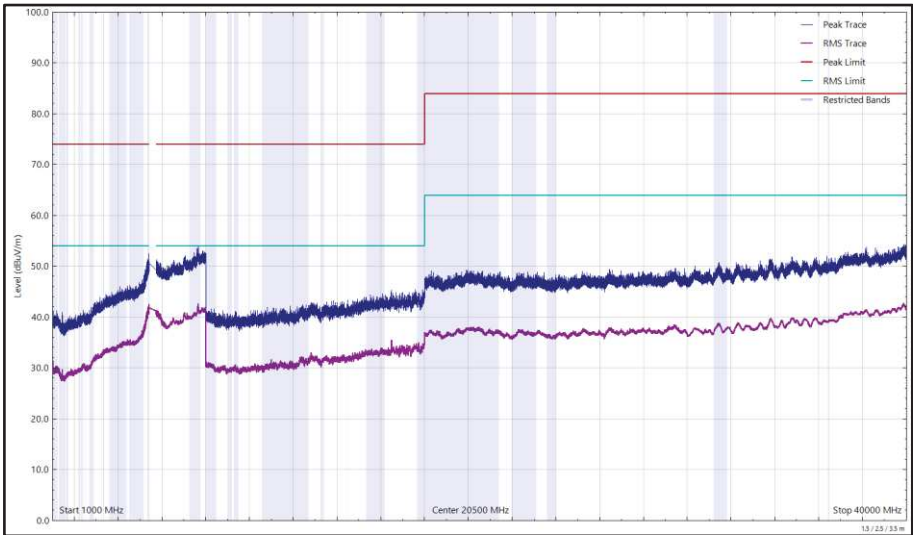
Figure 638 - U-NII-2C - 5500 MHz (CH100), HE20, RU52-37, CDD, Core 0 + Core 1, 1 GHz to 40 GHz, Horizontal
