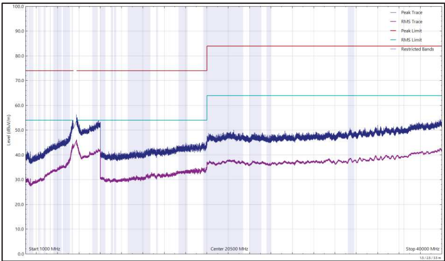
Figure 625 - U-NII-2C - 5700 MHz (CH140), HT20, CDD, Core 0 + Core 1, 1 GHz to 40 GHz, Vertical
