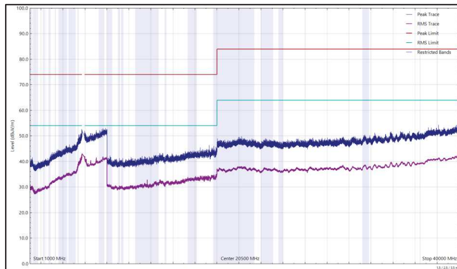
Figure 629 - U-NII-3 - 5825 MHz (CH165), HT20, CDD, Core 0 + Core 1, 1 GHz to 40 GHz, Horizontal
