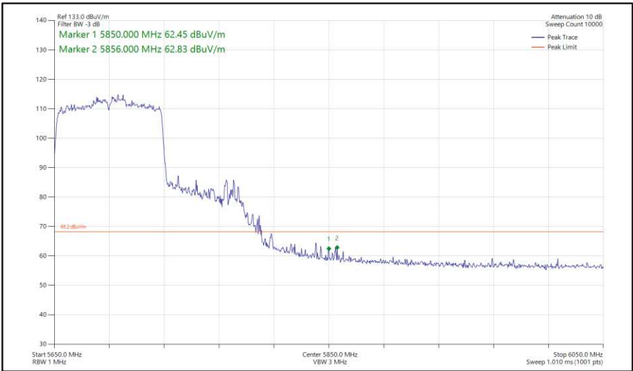
Figure 589 - 802.11ac VHT80, TxBF, Core 0 + Core 1 - 5690 MHz Band Edge Frequency 5850 MHz
