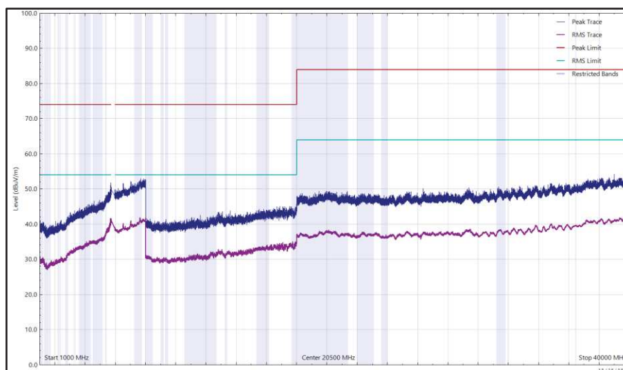
Figure 661 - U-NII-3 - 5825 MHz (CH165), 802.11a, Core 0, 1 GHz to 40 GHz, Horizontal
