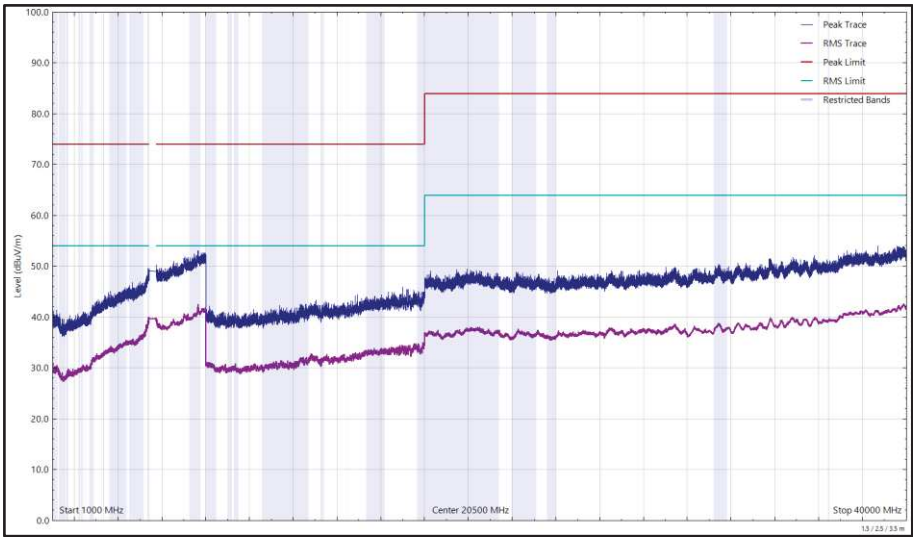
Figure 654 - U-NII-2C - 5500 MHz (CH100), 802.11a, Core 0, 1 GHz to 40 GHz, Horizontal
