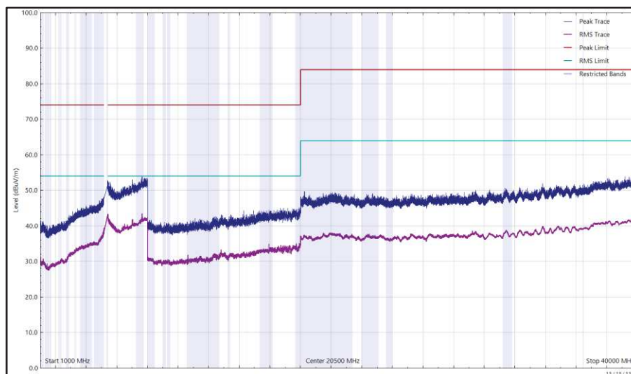
Figure 636 - U-NII-2A - 5320 MHz (CH64), HE20, RU52-37, CDD, Core 0 + Core 1, 1 GHz to 40 GHz, Horizontal
