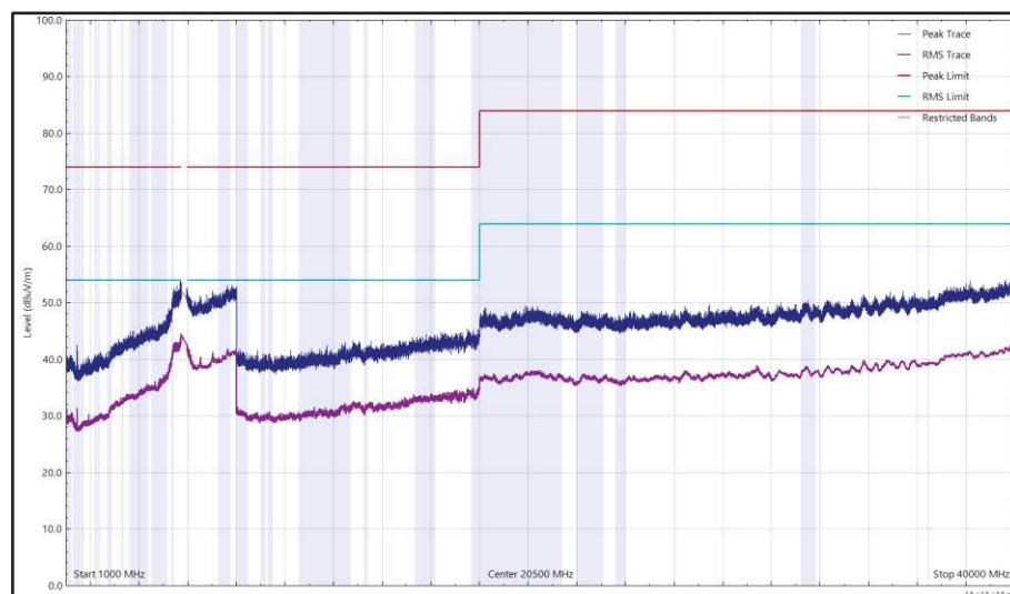
Figure 631 - U-NII-3 - 5825 MHz (CH165), HT20, CDD, Core 0 + Core 1, 1 GHz to 40 GHz, Vertical
