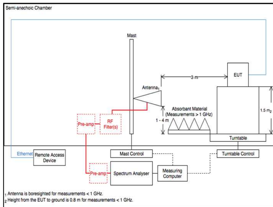
Figure 615 - Radiated Emissions Test Setup Diagram
