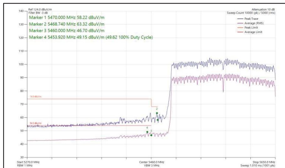
Figure 604 - 802.11ax HE160, SU, CDD, Core 0 + Core 1 - 5570 MHz Band Edge Frequency 5470 MHz
