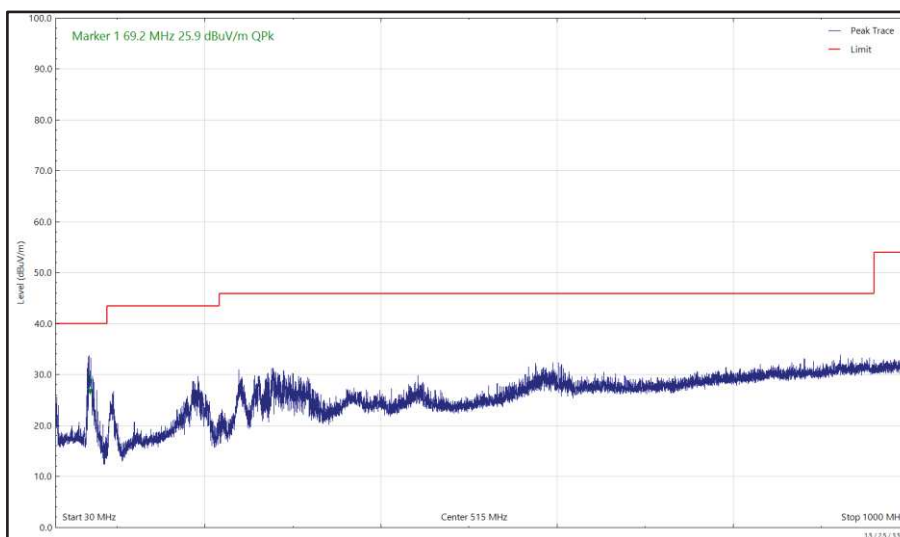
Figure 664 - U-NII-1 - 5180 MHz (CH36), 802.11a, Core 1, 30 MHz to 1 GHz, Horizontal (Peak)
