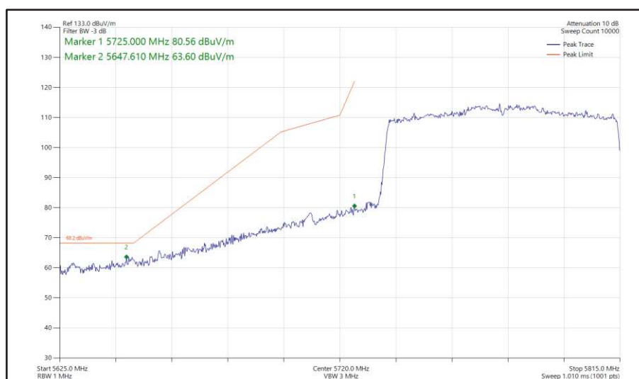
Figure 575 - 802.11ax HE80, SU, SDM, Core 0 + Core 1 - 5775 MHz Band Edge Frequency 5725 MHz
