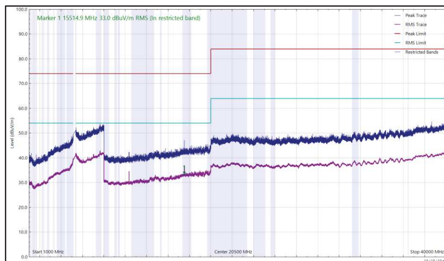
Figure 633 - U-NII-1 - 5180 MHz (CH36), HE20, RU26-0, CDD, Core 0 + Core 1, 1 GHz to 40 GHz, Horizontal
