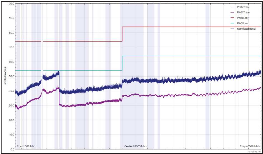
Figure 668 - U-NII-2A - 5320 MHz (CH64), 802.11a, Core 1, 1 GHz to 40 GHz, Horizontal
