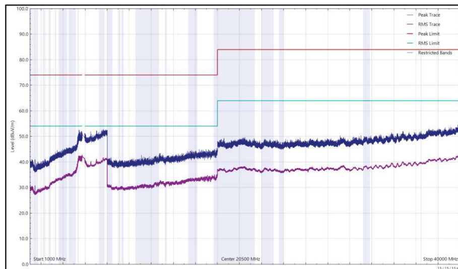
Figure 663 - U-NII-3 - 5825 MHz (CH165), 802.11a, Core 0, 1 GHz to 40 GHz, Vertical
