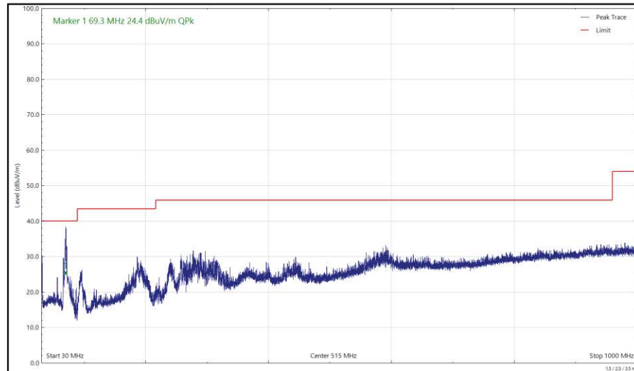
Figure 676 - U-NII-3 - 5825 MHz (CH165), 802.11a, Core 1, 30 MHz to 1 GHz, Horizontal (Peak)
