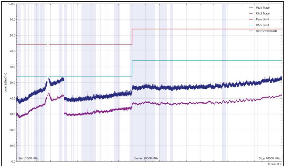
Figure 640 - U-NII-2C - 5700 MHz (CH140), HE20, RU52-37, CDD, Core 0 + Core 1, 1 GHz to 40 GHz, Horizontal
