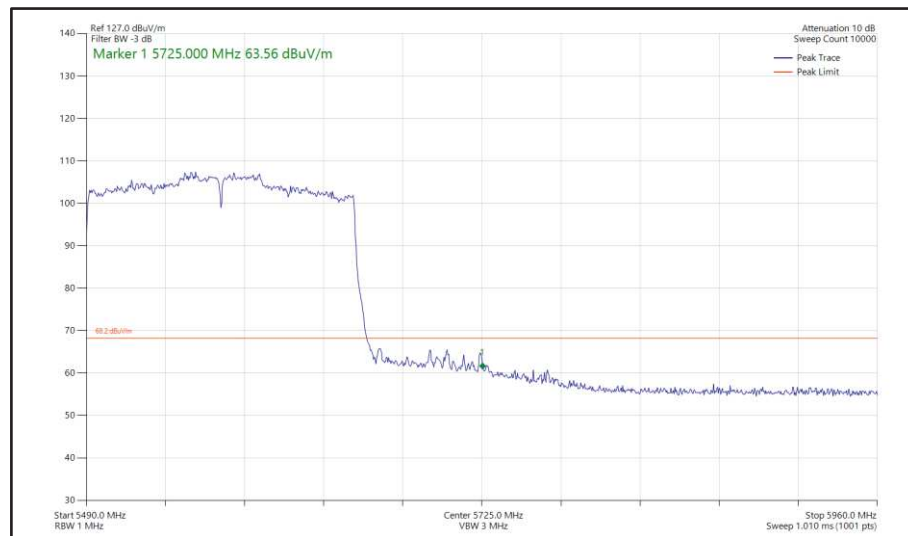
Figure 613 - 802.11ax HE160, SU, SDM, Core 0 + Core 1 - 5570 MHz Band Edge Frequency 5725 MHz
