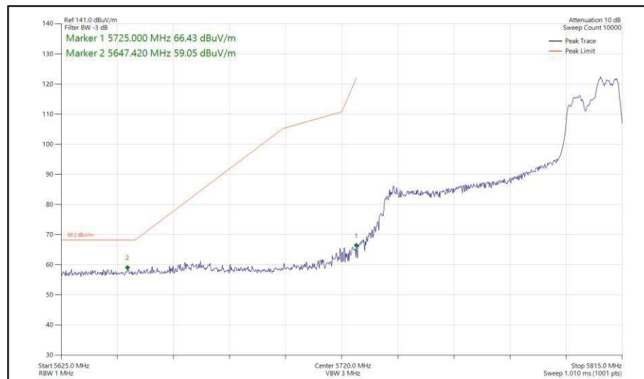
Figure 576 - 802.11ax HE80, RU 106-60, SDM, Core 0 + Core 1 - 5775 MHz Band Edge Frequency 5725 MHz
