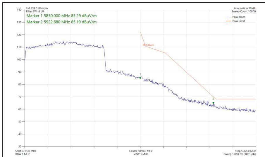
Figure 584 - 802.11ax HE80, SU, SDM, Core 0 + Core 1 - 5775 MHz Band Edge Frequency 5850 MHz
