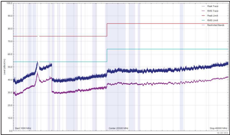
Figure 655 - U-NII-2C - 5500 MHz (CH100), 802.11a, Core 0, 1 GHz to 40 GHz, Vertical
