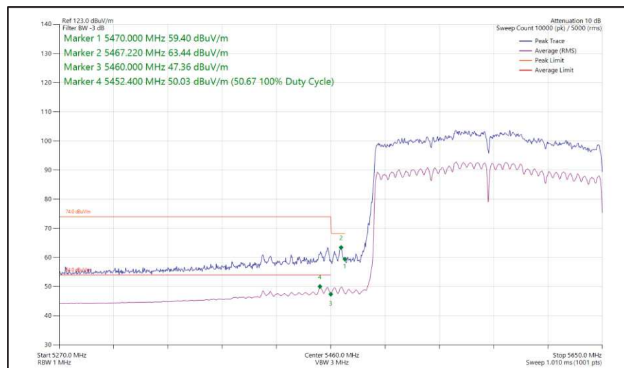
Figure 610 - 802.11ax HE160, SU, SDM, Core 0 + Core 1 - 5570 MHz Band Edge Frequency 5470 MHz
