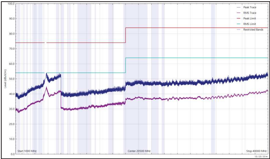
Figure 672 - U-NII-2C - 5700 MHz (CH140), 802.11a, Core 1, 1 GHz to 40 GHz, Horizontal
