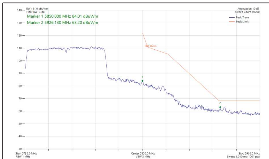
Figure 581 - 802.11ac VHT80, SDM, Core 0 + Core 1 - 5775 MHz Band Edge Frequency 5850 MHz
