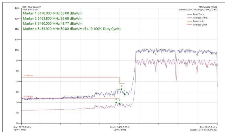
Figure 603 - 802.11ac VHT160, CDD, Core 0 + Core 1 - 5570 MHz Band Edge Frequency 5470 MHz
