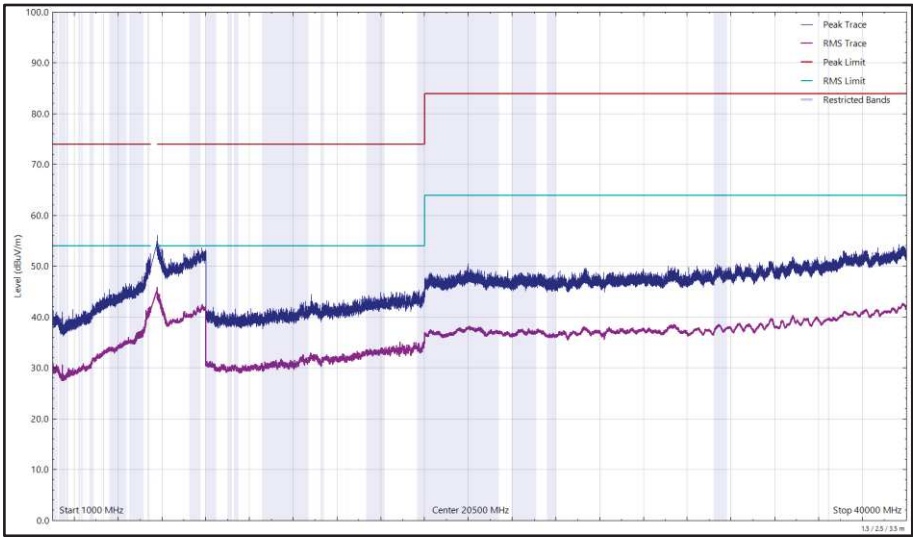
Figure 673 - U-NII-2C - 5700 MHz (CH140), 802.11a, Core 1, 1 GHz to 40 GHz, Vertical
