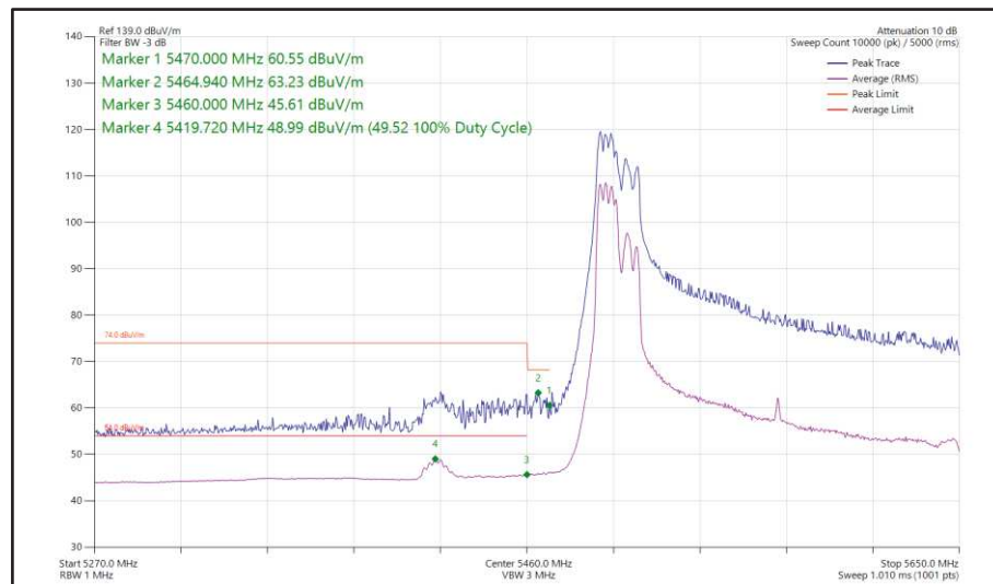
Figure 605 - 802.11ax HE160, RU 106-53, CDD, Core 0 + Core 1 - 5570 MHz Band Edge Frequency 5470 MHz
