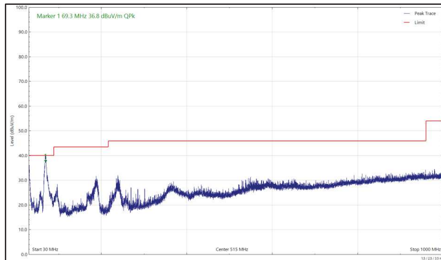
Figure 634 - U-NII-1 - 5180 MHz (CH36), HE20, RU26-0, CDD, Core 0 + Core 1, 30 MHz to 1 GHz, Vertical (Peak)
