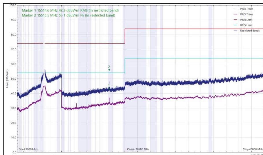
Figure 635 - U-NII-1 - 5180 MHz (CH36), HE20, RU26-0, CDD, Core 0 + Core 1, 1 GHz to 40 GHz, Vertical
