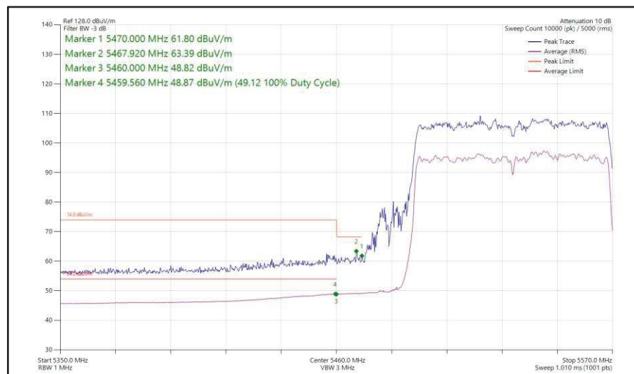
Figure 586 - 802.11ac VHT80, TxBF, Core 0 + Core 1 - 5530 MHz Band Edge Frequency 5470 MHz
