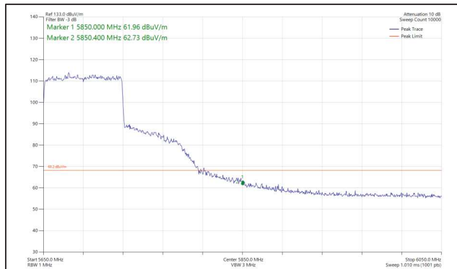
Figure 582 - 802.11ax HE80, SU, SDM, Core 0 + Core 1 - 5690 MHz Band Edge Frequency 5850 MHz
