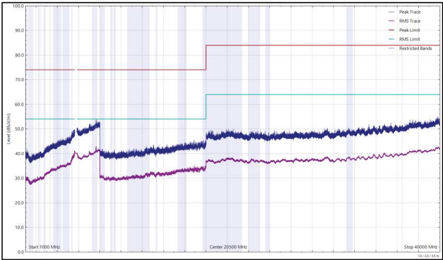
Figure 658 - U-NII-3 - 5745 MHz (CH149), 802.11a, Core 0, 1 GHz to 40 GHz, Horizontal
