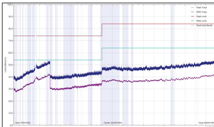
Figure 649 - U-NII-1 - 5180 MHz (CH36), 802.11a, Core 0, 1 GHz to 40 GHz, Horizontal
