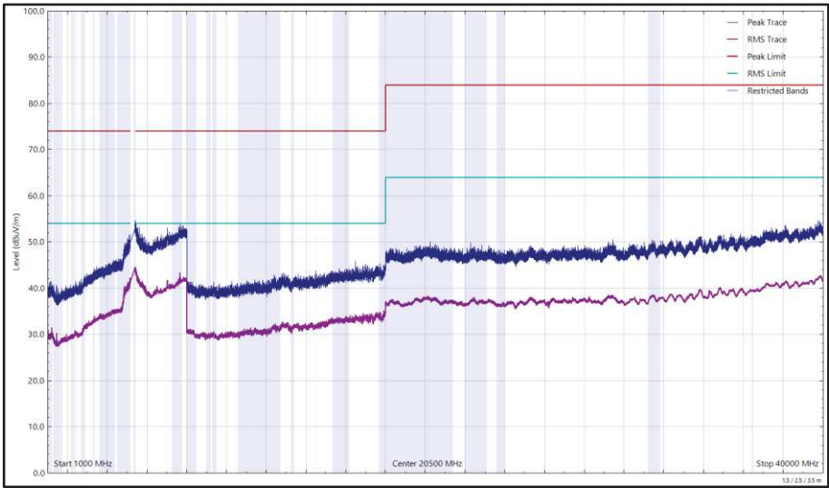
Figure 669 - U-NII-2A - 5320 MHz (CH64), 802.11a, Core 1, 1 GHz to 40 GHz, Vertical
