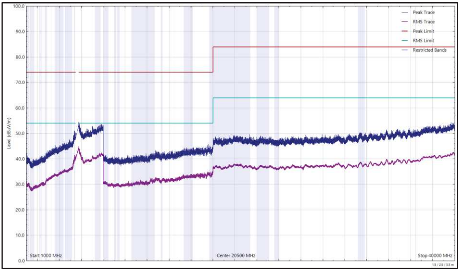
Figure 624 - U-NII-2C - 5700 MHz (CH140), HT20, CDD, Core 0 + Core 1, 1 GHz to 40 GHz, Horizontal
