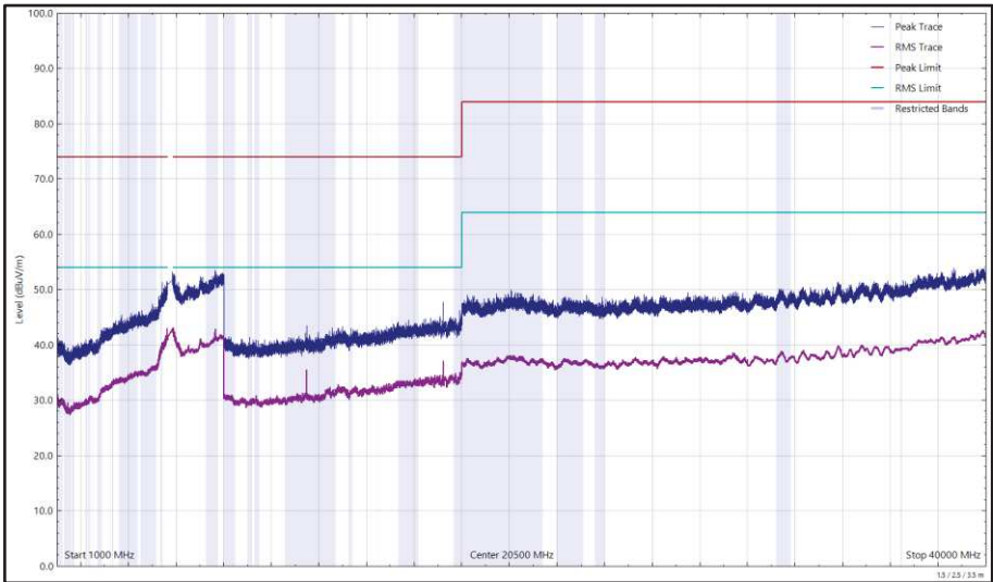
Figure 642 - U-NII-3 - 5745 MHz (CH149), HE20, RU26-0, CDD, Core 0 + Core 1, 1 GHz to 40 GHz, Horizontal
