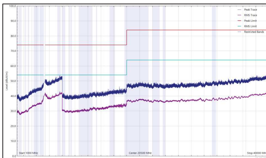
Figure 617 - U-NII-1 - 5180 MHz (CH36), HT20, CDD, Core 0 + Core 1, 1 GHz to 40 GHz, Horizontal
