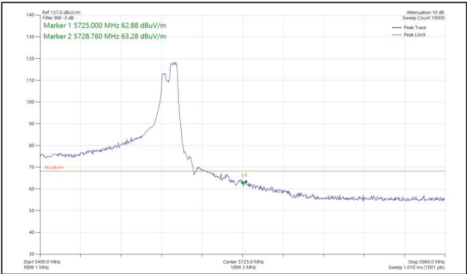
Figure 602 - 802.11ax HE160, RU 106-60, SISO, Core 1 - 5570 MHz Band Edge Frequency 5725 MHz
