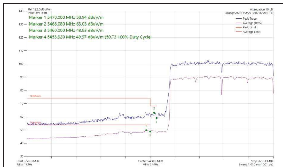
Figure 598 - 802.11ax HE160, SU, SISO, Core 1 - 5570 MHz Band Edge Frequency 5470 MHz
