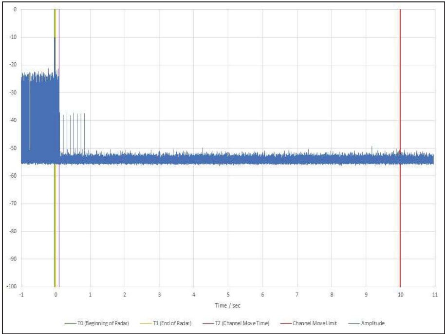
Figure 684 - First 12 s of Channel Shutdown Period
