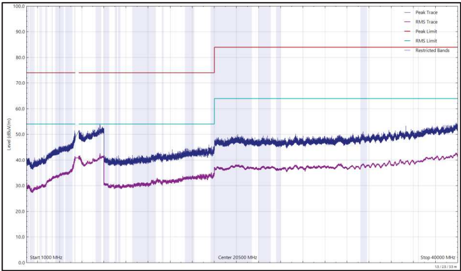
Figure 670 - U-NII-2C - 5500 MHz (CH100), 802.11a, Core 1, 1 GHz to 40 GHz, Horizontal
