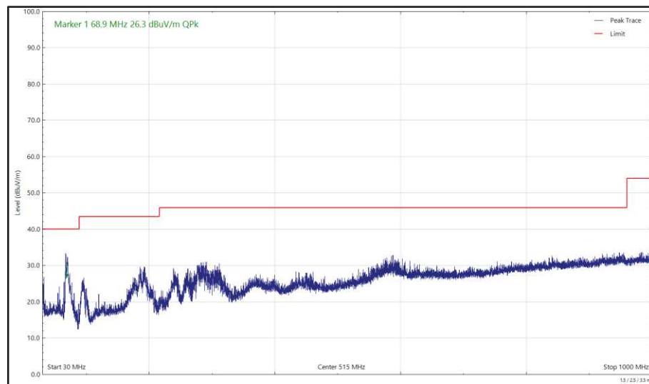
Figure 644 - U-NII-3 - 5825 MHz (CH165), HE20, RU26-0, CDD, Core 0 + Core 1, 30 MHz to 1 GHz, Horizontal (Peak)
