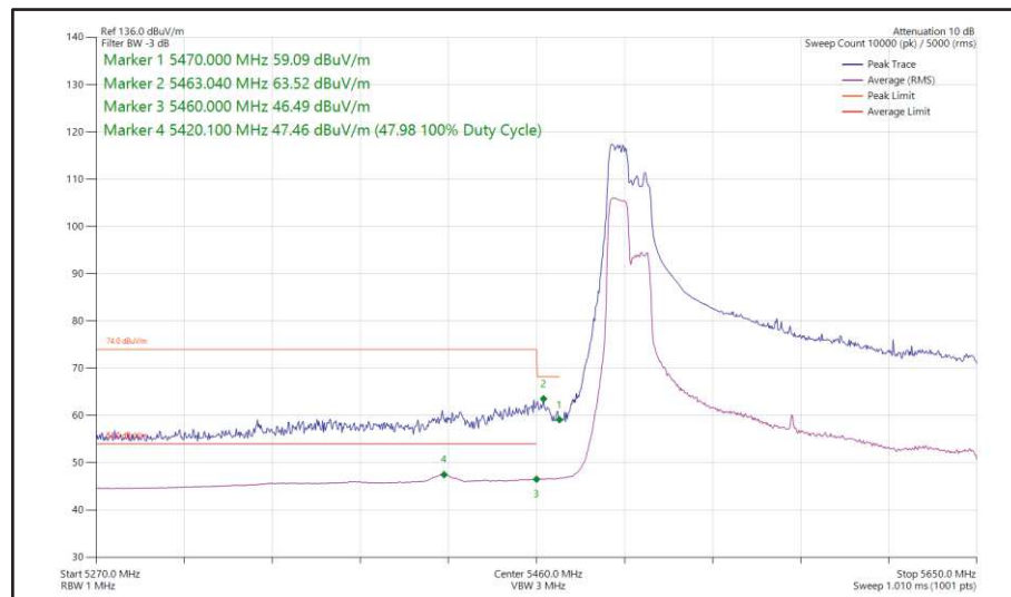
Figure 593 - 802.11ax HE160, RU 106-53, SISO, Core 0 - 5570 MHz Band Edge Frequency 5470 MHz
