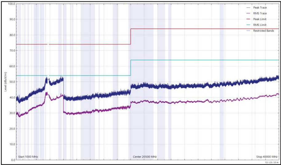
Figure 659 - U-NII-3 - 5745 MHz (CH149), 802.11a, Core 0, 1 GHz to 40 GHz, Vertical
