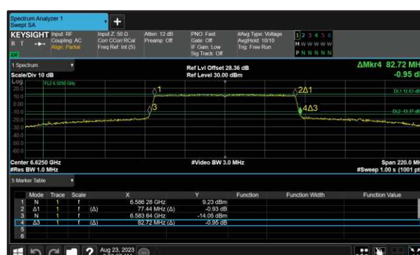
Figure 34 - 802.11ax HE80 SU SP Maximum 99% OBW
