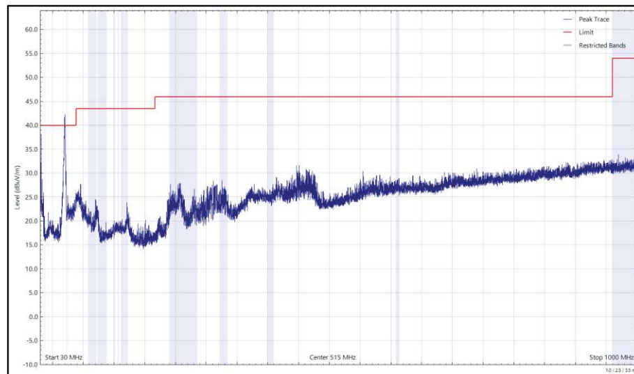
Figure 14 - 2441 MHz (CH39), DH5, ePA, Core 0 + Core 1 and U-NII-5 - 5955 MHz (CH1), HE20, SU, CDD, Core 0 + Core 1, 30 MHz to 1 GHz, Horizontal (Peak)
