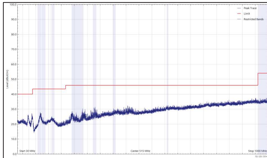
Figure 38 - 2440 MHz (CH18), Thread, ePA, Core 0 and U-NII-1 - 5240 MHz (CH48), VHT20, CDD, Core 0 + Core 1, 30 MHz to 1 GHz, Horizontal (Peak)
