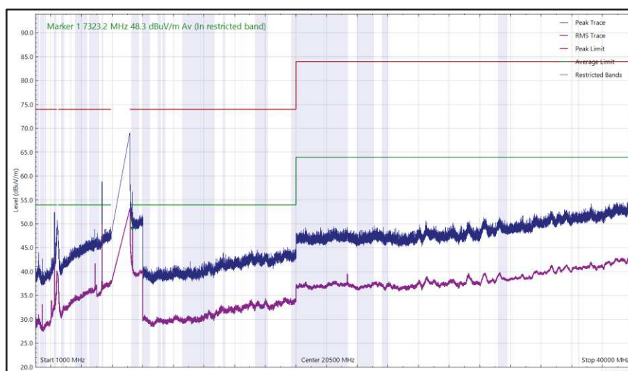
Figure 21 - 2441 MHz (CH39), DH5, ePA, Core 0 + Core 1 and U-NII-8 - 7115 MHz (CH233), HE20, SU, CDD, Core 0 + Core 1, 1 GHz to 40 GHz, Vertical
