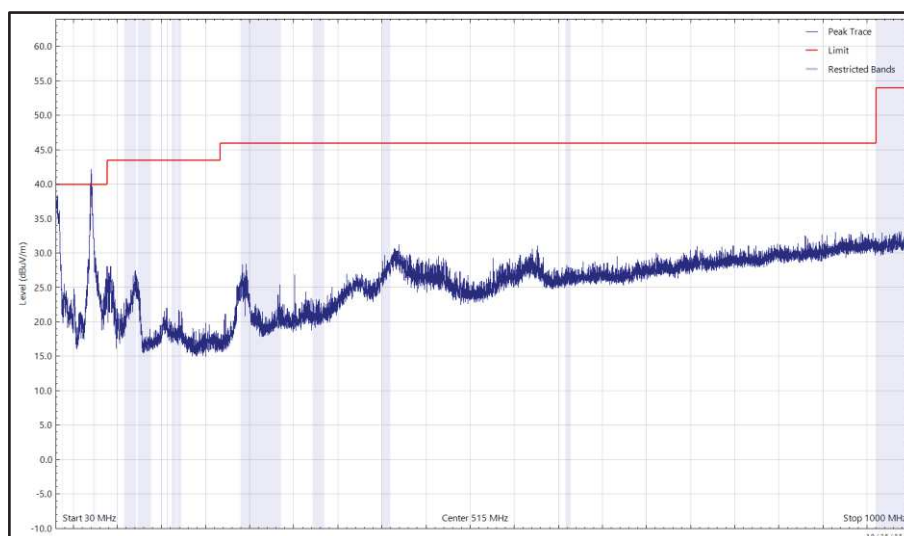
Figure 20 - 2441 MHz (CH39), DH5, ePA, Core 0 + Core 1 and U-NII-8 - 7115 MHz (CH233), HE20, SU, CDD, Core 0 + Core 1, 30 MHz to 1 GHz, Vertical (Peak)
