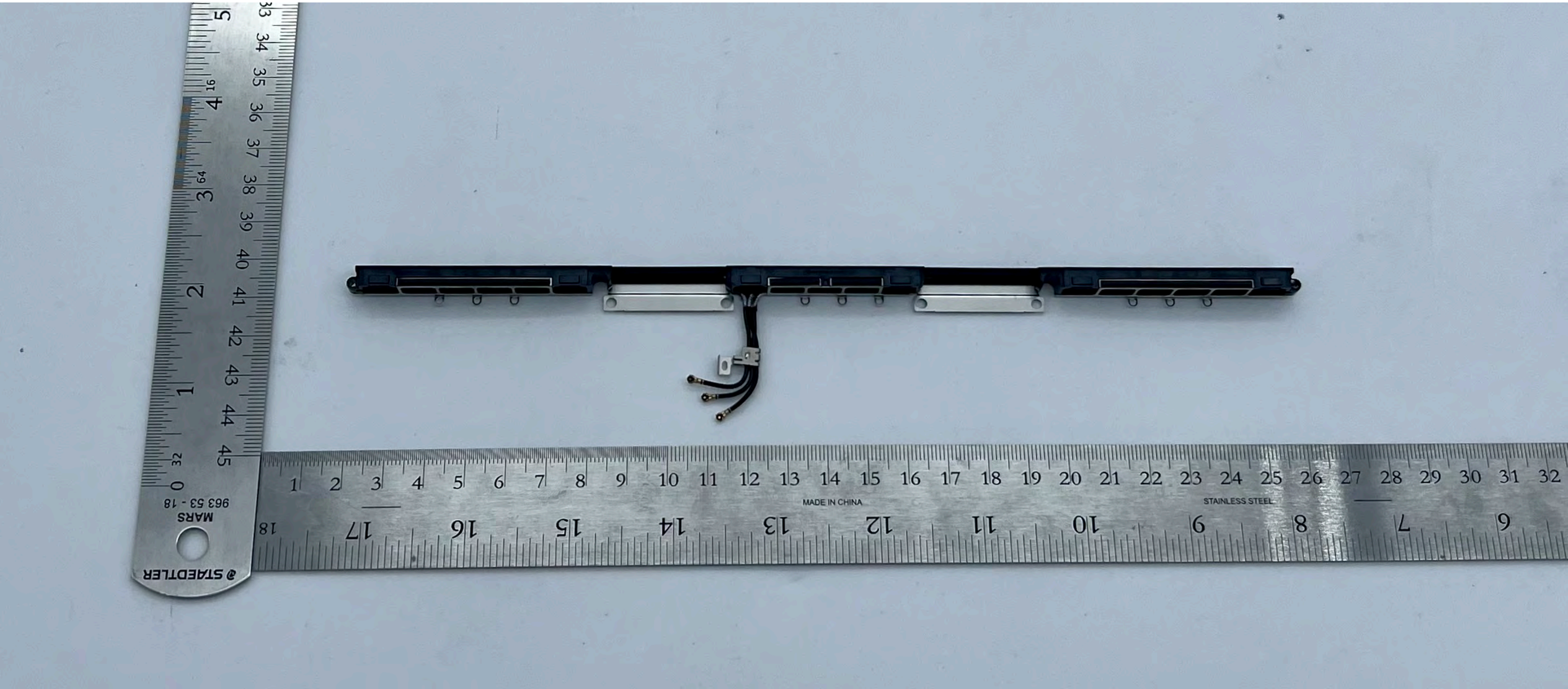
A2992 WF1/BT, WF2/BT, WF3 (BT) antenna structure and feed - Back
