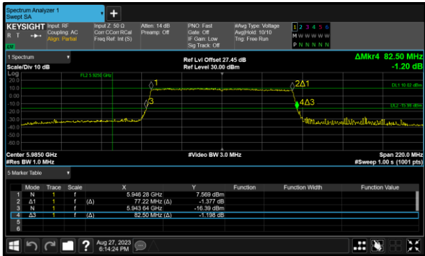
Figure 61 - 802.11ax HE80 SU SP Minimum 99% OBW
