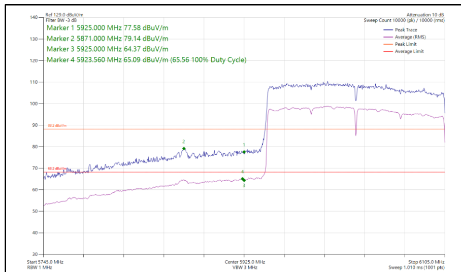
Figure 122 - 802.11ax HE160, SU, SISO, Core 1 - 6025 MHz Band Edge Frequency 5925 MHz
