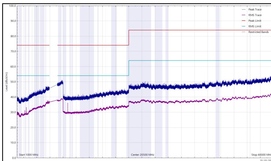
Figure 151 - U-NII-7 - 6535 MHz (CH117), HE20, SU, CDD, Core 0 + Core 1, 1 GHz to 40 GHz, Horizontal
