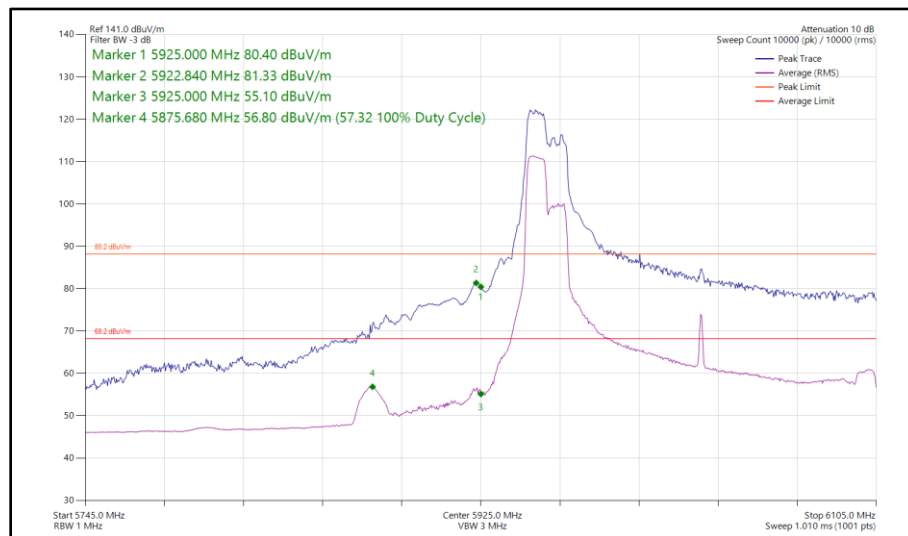
Figure 119 - 802.11ax HE160, RU 106-53, SISO, Core 0 - 6025 MHz Band Edge Frequency 5925 MHz
