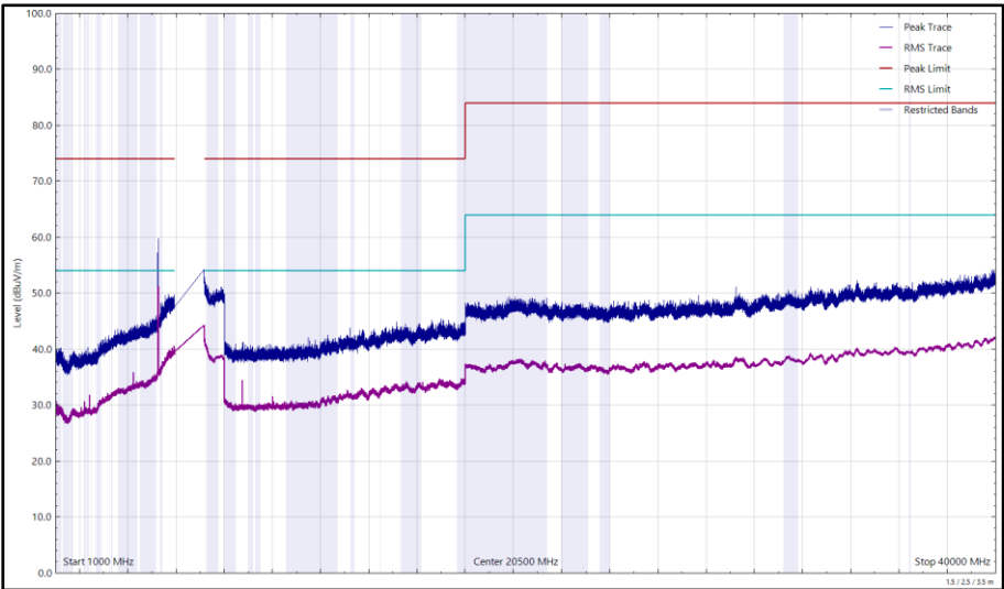
Figure 164 - U-NII-8 - 6995 MHz (CH209), HE20, SU, CDD, Core 0 + Core 1, 1 GHz to 40 GHz, Vertical
