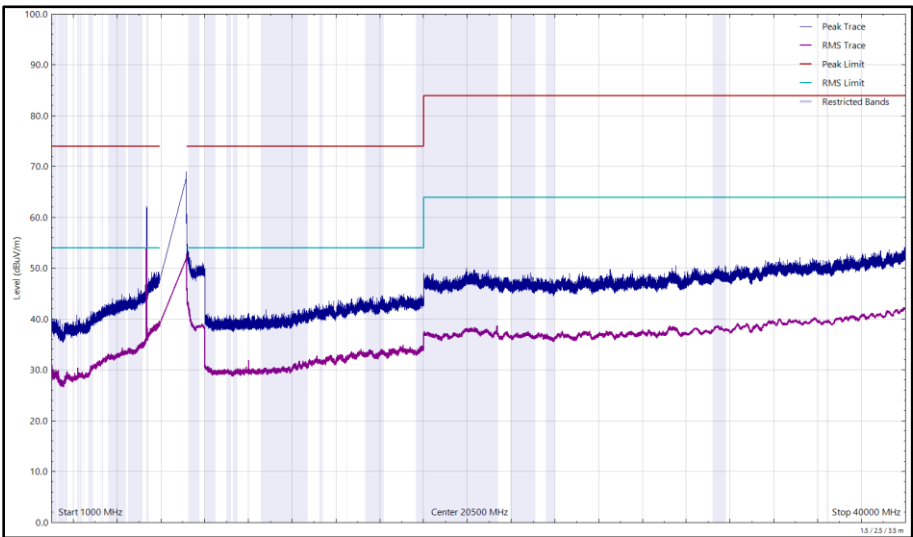
Figure 166 - U-NII-8 - 7115 MHz (CH233), HE20, SU, CDD, Core 0 + Core 1, 1 GHz to 40 GHz, Vertical
