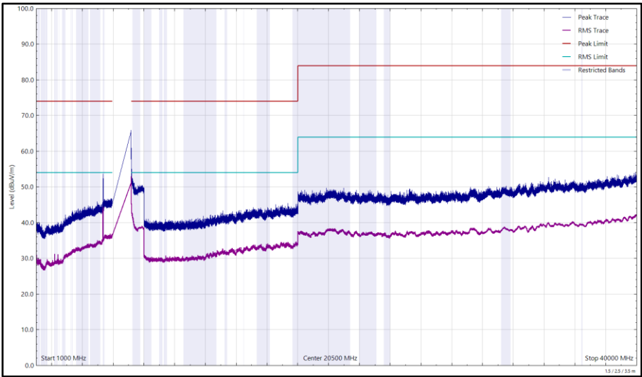
Figure 165 - U-NII-8 - 7115 MHz (CH233), HE20, SU, CDD, Core 0 + Core 1, 1 GHz to 40 GHz, Horizontal
