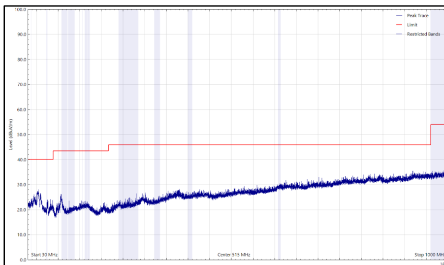
Figure 153 - U-NII-7 - 6695 MHz (CH149), HE20, SU, CDD, Core 0 + Core 1, 30 MHz to 1 GHz, Horizontal (Peak)
