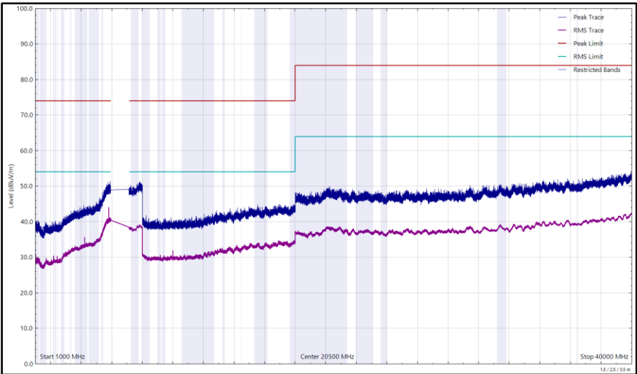
Figure 156 - U-NII-7 - 6695 MHz (CH149), HE20, SU, CDD, Core 0 + Core 1, 1 GHz to 40 GHz, Vertical
