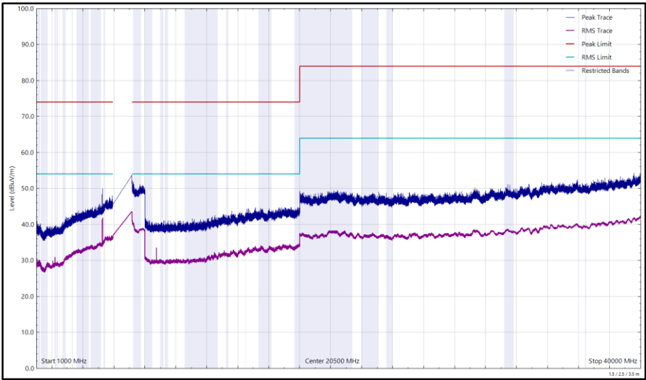
Figure 162 - U-NII-8 - 6995 MHz (CH209), HE20, SU, CDD, Core 0 + Core 1, 1 GHz to 40 GHz, Horizontal
