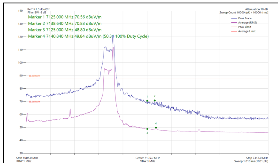
Figure 125 - 802.11ax HE160, RU 26-36, SISO, Core 1 - 6985 MHz Band Edge Frequency 7125 MHz
