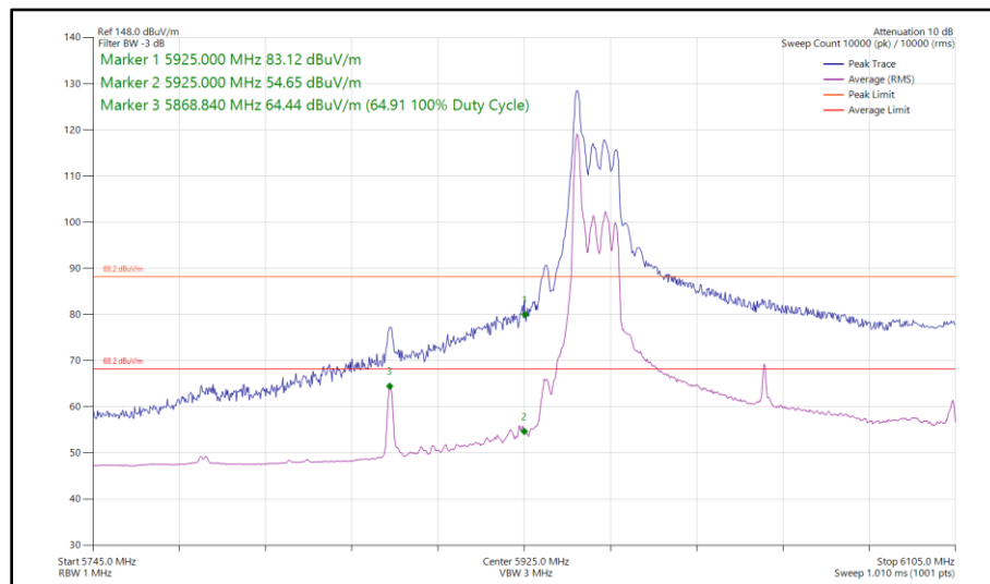
Figure 131 - 802.11ax HE160, RU 26-0, SDM, Core 0 + Core 1 - 6025 MHz Band Edge Frequency 5925 MHz
