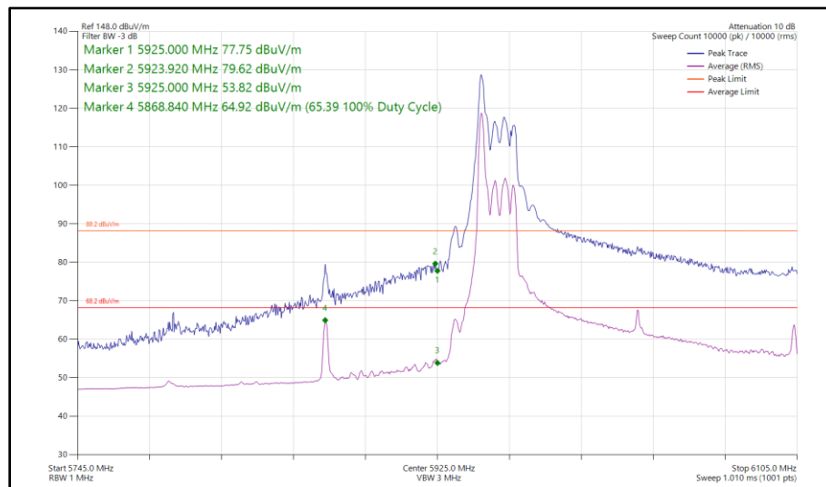
Figure 127 - 802.11ax HE160, RU 26-0, CDD, Core 0 + Core 1 - 6025 MHz Band Edge Frequency 5925 MHz
