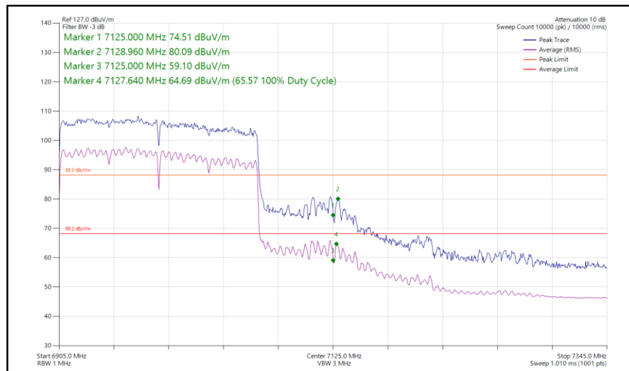
Figure 132 - 802.11ax HE160, SU, SDM, Core 0 + Core 1 - 6985 MHz Band Edge Frequency 7125 MHz
