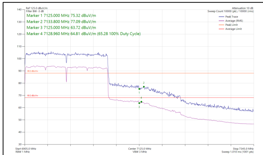
Figure 124 - 802.11ax HE160, SU, SISO, Core 1 - 6985 MHz Band Edge Frequency 7125 MHz
