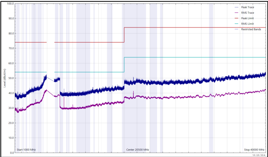
Figure 148 - U-NII-6 - 6475 MHz (CH105), HE20, SU, CDD, Core 0 + Core 1, 1 GHz to 40 GHz, Vertical
