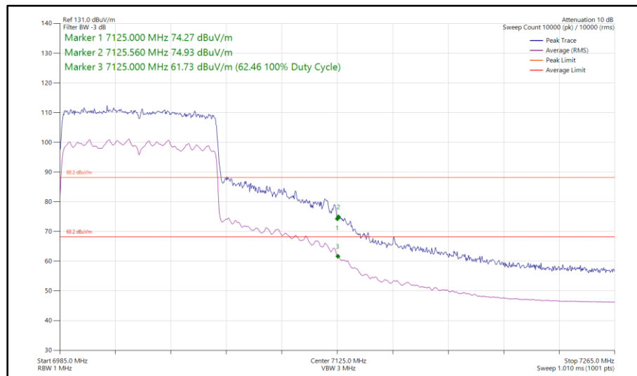
Figure 114 - 802.11ax HE80, SU, SDM, Core 0 + Core 1 - 7025 MHz Band Edge Frequency 7125 MHz
