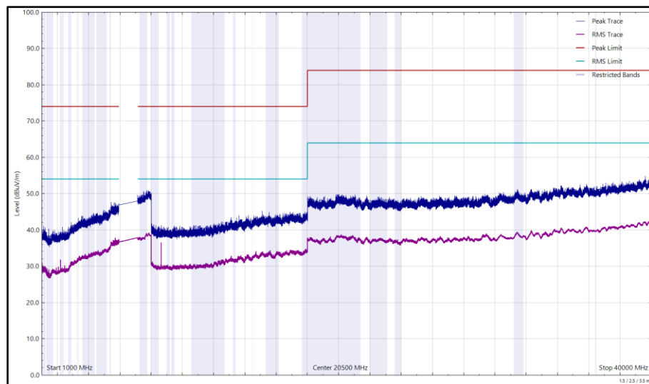
Figure 146 - U-NII-6 - 6475 MHz (CH105), HE20, SU, CDD, Core 0 + Core 1, 1 GHz to 40 GHz, Horizontal
