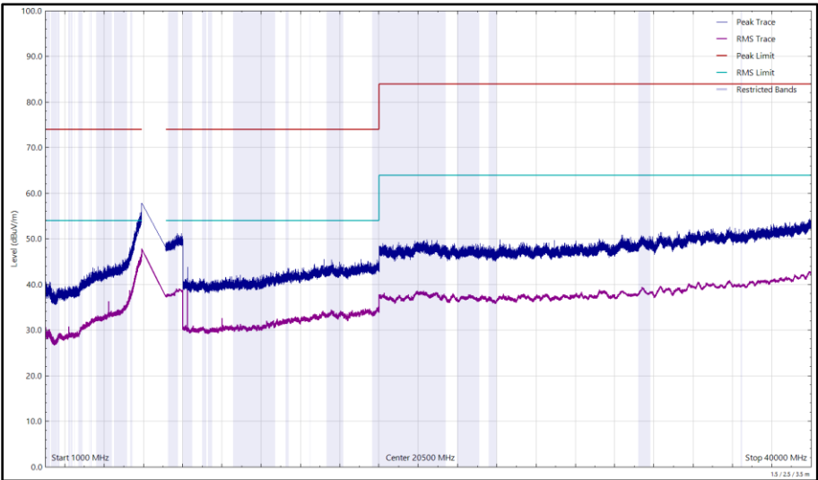
Figure 140 - U-NII-5 - 6175 MHz (CH45), HE20, SU, CDD, Core 0 + Core 1, 1 GHz to 40 GHz, Vertical
