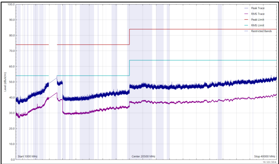
Figure 158 - U-NII-7 - 6855 MHz (CH181), HE20, SU, CDD, Core 0 + Core 1, 1 GHz to 40 GHz, Vertical
