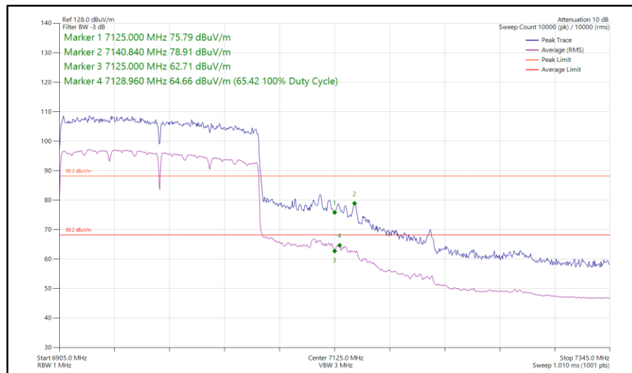
Figure 120 - 802.11ax HE160, SU, SISO, Core 0 - 6985 MHz Band Edge Frequency 7125 MHz
