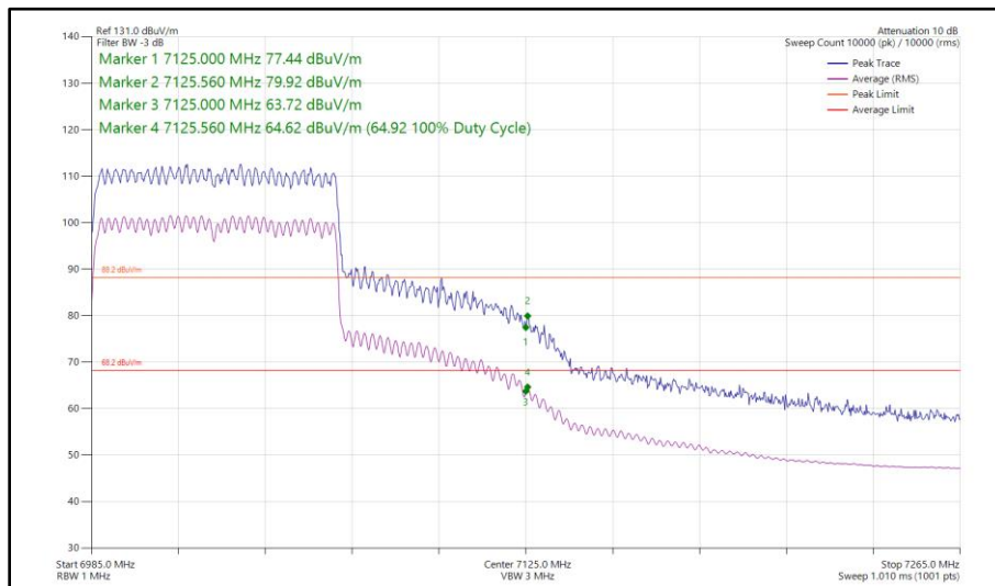
Figure 110 - 802.11ax HE80, SU, CDD, Core 0 + Core 1 - 7025 MHz Band Edge Frequency 7125 MHz
