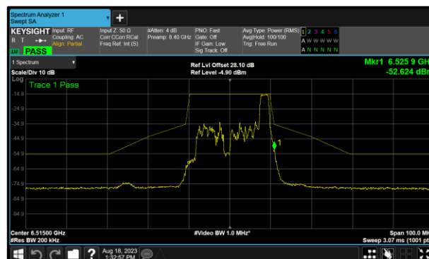
Figure 173 - A (Core 0) 802.11ax HE20 RU26 LPI 6515 MHz (CH113)
