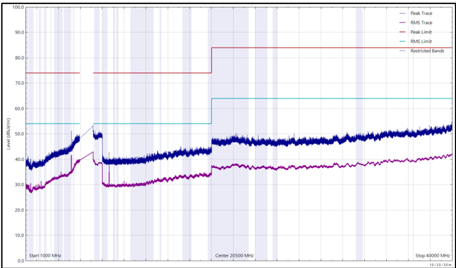
Figure 160 - U-NII-8 - 6895 MHz (CH189), HE20, SU, CDD, Core 0 + Core 1, 1 GHz to 40 GHz, Vertical
