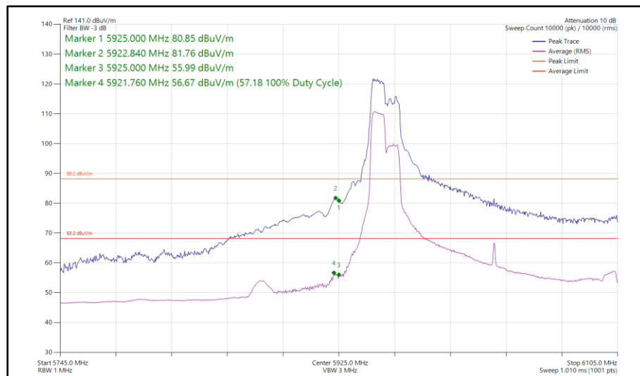
Figure 123 - 802.11ax HE160, RU 106-53, SISO, Core 1 - 6025 MHz Band Edge Frequency 5925 MHz
