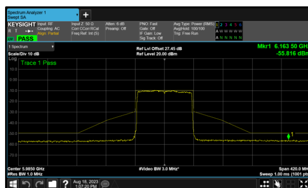
Figure 170 - A (Core 0) 802.11ax HE80 SU LPI 5985 MHz (CH7)
