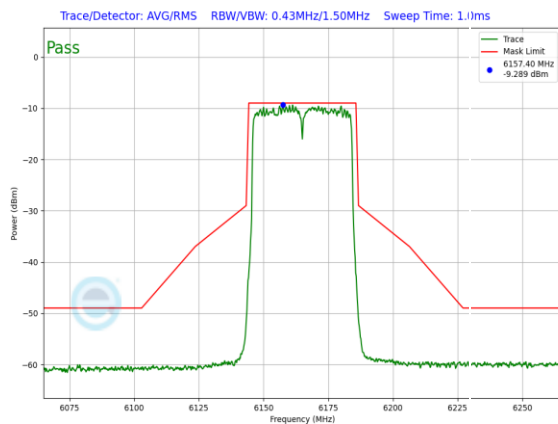
Plot 7-267. In-Band Emission Plot Antenna WF2 LPI (40MHz 802.11ax (UNII Band 5) – Ch. 43, MCS11)
