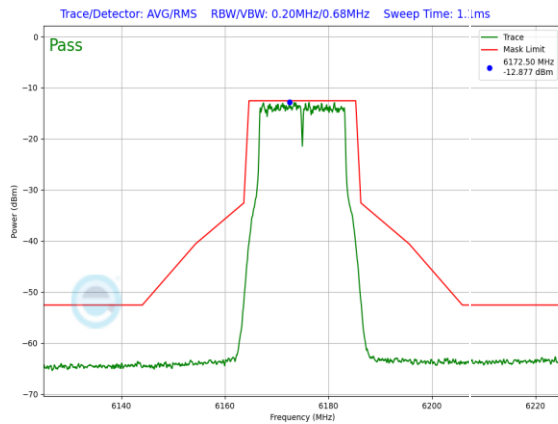
Plot 7-265. In-Band Emission Plot Antenna WF2 LPI (20MHz 802.11a (UNII Band 5) – Ch. 45, 54Mbps)
