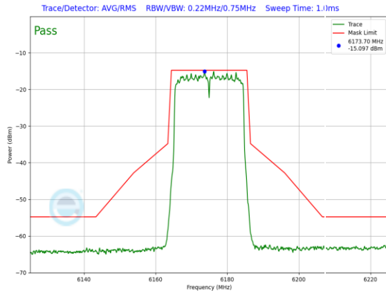
Plot 7-305. In-Band Emission Plot SDM Antenna WF5T LPI (20MHz 802.11ax (UNII Band 5) – Ch. 45, MCS11)
