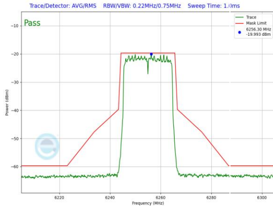
Plot 7-354. In-Band Emission Plot SDM Antenna WF2 VLP (20MHz 802.11ax (UNII Band 5) – Ch. 61, MCS11)
