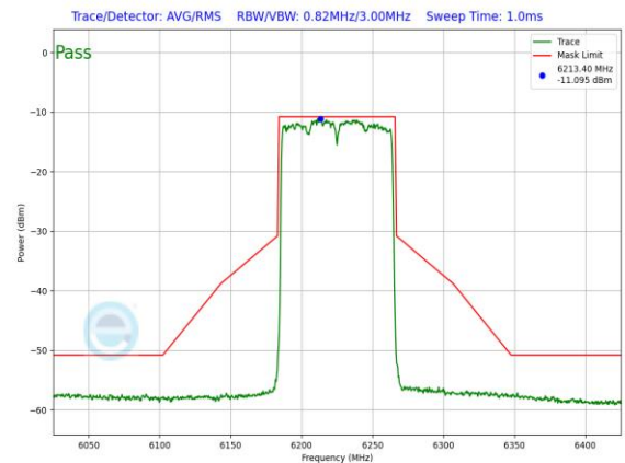
Plot 7-298. In-Band Emission Plot Antenna WF2 VLP (80MHz 802.11ax (UNII Band 5) – Ch. 55, MCS11)
