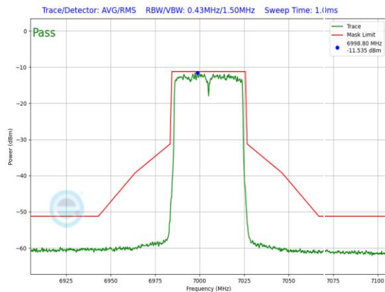
Plot 7-331. In-Band Emission Plot SDM Antenna WF5T LPI (40MHz 802.11ax (UNII Band 8) – Ch. 211, MCS11)
