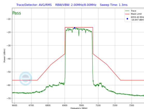
Plot 7-284. In-Band Emission Plot Antenna WF2 LPI (160MHz 802.11ax (UNII Band 8) – Ch. 207, MCS11)
