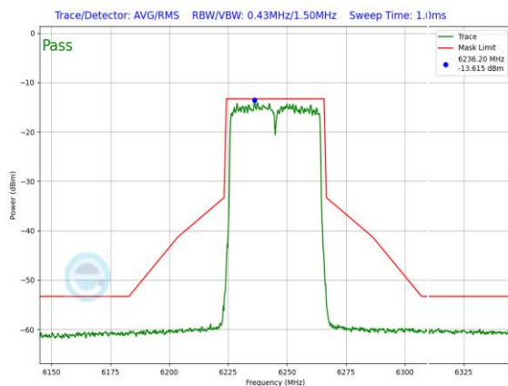
Plot 7-297. In-Band Emission Plot Antenna WF2 VLP (40MHz 802.11ax (UNII Band 5) – Ch. 59, MCS11)
