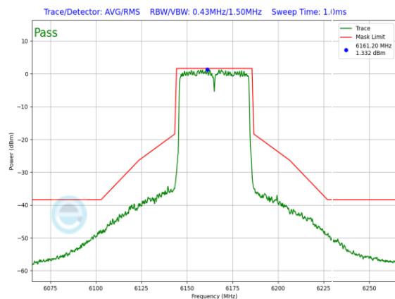
Plot 7-287. In-Band Emission Plot Antenna WF2 SP (40MHz) 802.11ax (UNII Band 5) – Ch. 43, MCS11)
