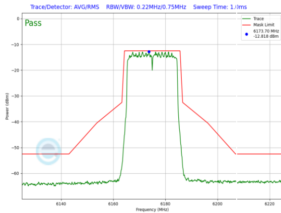
Plot 7-266. In-Band Emission Plot Antenna WF2 LPI (20MHz 802.11ax (UNII Band 5) – Ch. 45, MCS11)
