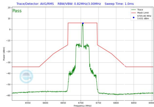
Plot 7-770. SP In-Band Emission Plot Antenna WF5T (80MHz 802.11ax RU26 (UNII Band 7) – Ch. 151)
