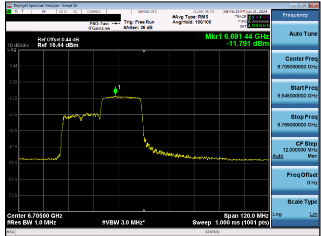
Plot 7-731. VLP Power Spectral Density Plot SDM Antenna WF5T (80MHz 802.11ax RU242 (UNII Band 7) – Ch. 151)
