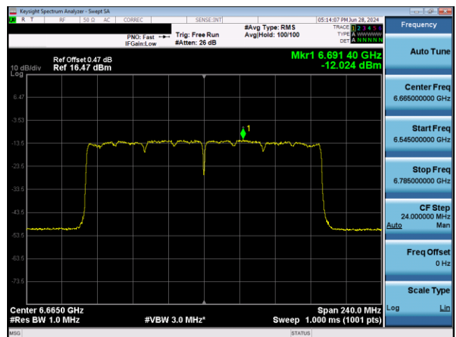
Plot 7-744. VLP Power Spectral Density Plot SDM Antenna WF2 (160MHz 802.11ax RU996x2 (UNII Band 7) – Ch. 143)
