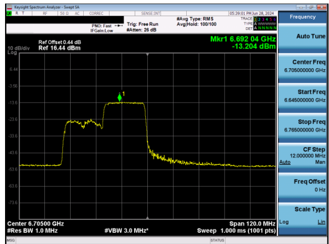
Plot 7-732. VLP Power Spectral Density Plot SDM Antenna WF2 (80MHz 802.11ax RU242 (UNII Band 7) – Ch. 151)
