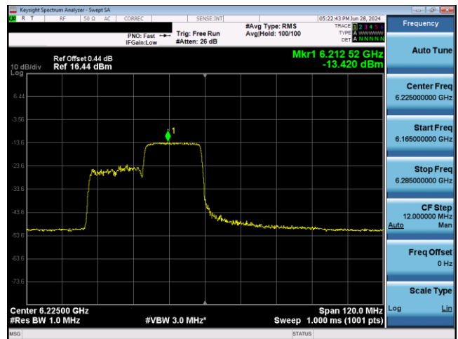
Plot 7-708. VLP Power Spectral Density Plot SDM Antenna WF2 (80MHz 802.11ax RU242 (UNII Band 5) – Ch. 55)
