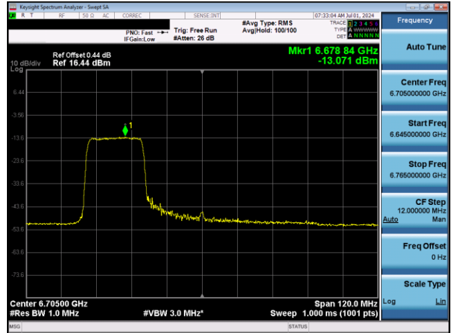
Plot 7-730. VLP Power Spectral Density Plot SDM Antenna WF2 (80MHz 802.11ax RU242 (UNII Band 7) – Ch. 151)
