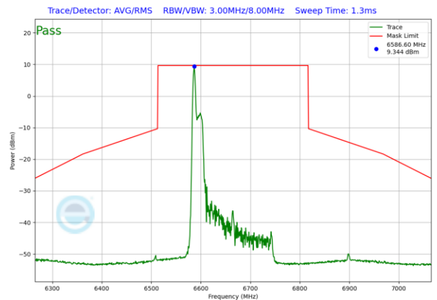
Plot 7-773. SP In-Band Emission Plot Antenna WF5T (160MHz 802.11ax RU26 (UNII Band 7) – Ch. 143)
