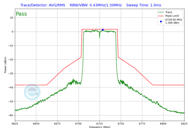
Plot 7-768. SP In-Band Emission Plot Antenna WF5T (40MHz 802.11ax RU484 (UNII Band 7) – Ch. 155)
