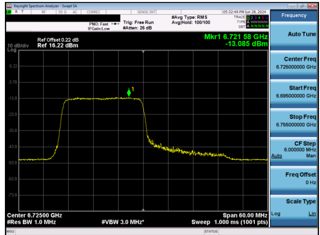
Plot 7-724. VLP Power Spectral Density Plot SDM Antenna WF2 (40MHz 802.11ax RU242 (UNII Band 7) – Ch. 155)
