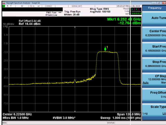
Plot 7-710. VLP Power Spectral Density Plot SDM Antenna WF2 (80MHz 802.11ax RU242 (UNII Band 5) – Ch. 55)
