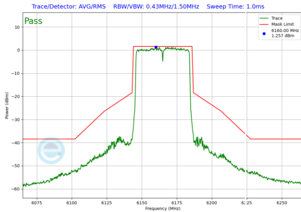
Plot 7-752. SP In-Band Emission Plot Antenna WF5T (40MHz 802.11ax RU484 (UNII Band 5) – Ch. 43)
