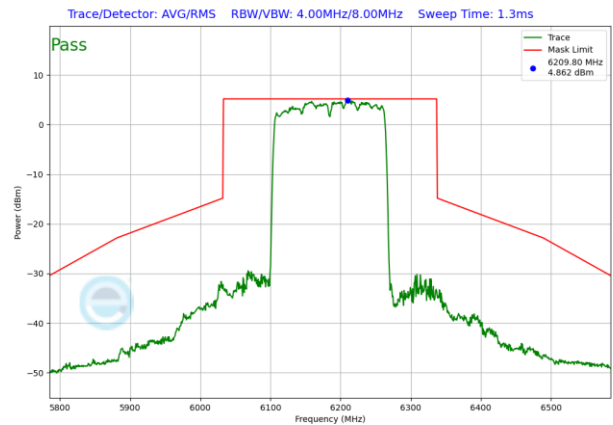
Plot 7-760. SP In-Band Emission Plot Antenna WF5T (160MHz 802.11ax RU996x2 (UNII Band 5) – Ch. 47)
