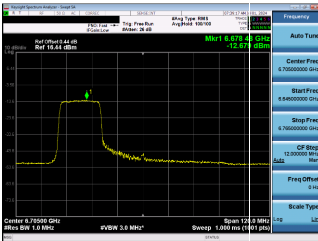
Plot 7-729. VLP Power Spectral Density Plot SDM Antenna WF5T (80MHz 802.11ax RU242 (UNII Band 7) – Ch. 151)
