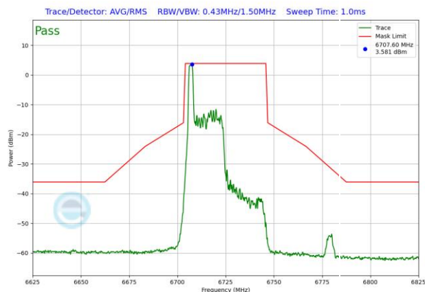
Plot 7-765. SP In-Band Emission Plot Antenna WF5T (40MHz 802.11ax RU26 (UNII Band 7) – Ch. 155)
