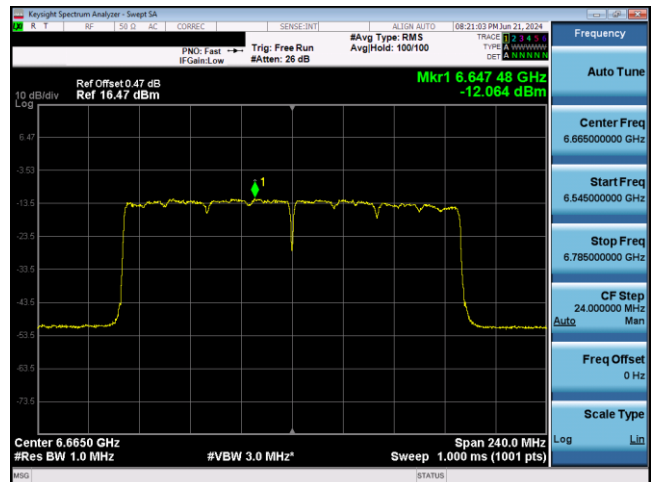
Plot 7-743. VLP Power Spectral Density Plot SDM Antenna WF5T (160MHz 802.11ax RU996x2 (UNII Band 7) – Ch. 143)
