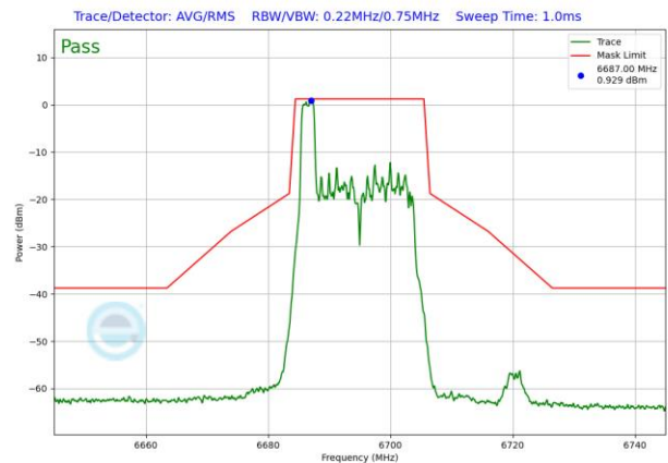
Plot 7-761. SP In-Band Emission Plot Antenna WF5T (20MHz 802.11ax RU26 (UNII Band 7) – Ch. 149)
