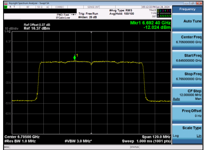
Plot 7-736. VLP Power Spectral Density Plot SDM Antenna WF2 (80MHz 802.11ax RU996 (UNII Band 7) – Ch. 151)
