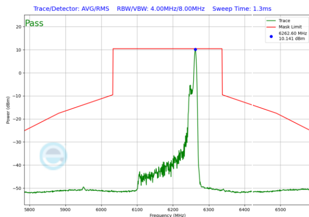
Plot 7-759. SP In-Band Emission Plot Antenna WF5T (160MHz 802.11ax RU26 (UNII Band 5) – Ch. 47)
