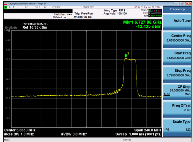
Plot 7-742. VLP Power Spectral Density Plot SDM Antenna WF2 (160MHz 802.11ax RU242 (UNII Band 7) – Ch. 143)
