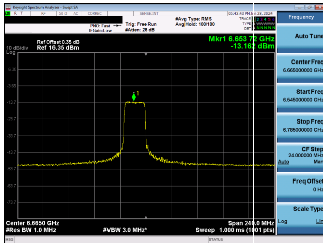
Plot 7-740. VLP Power Spectral Density Plot SDM Antenna WF2 (160MHz 802.11ax RU242 (UNII Band 7) – Ch. 143)
