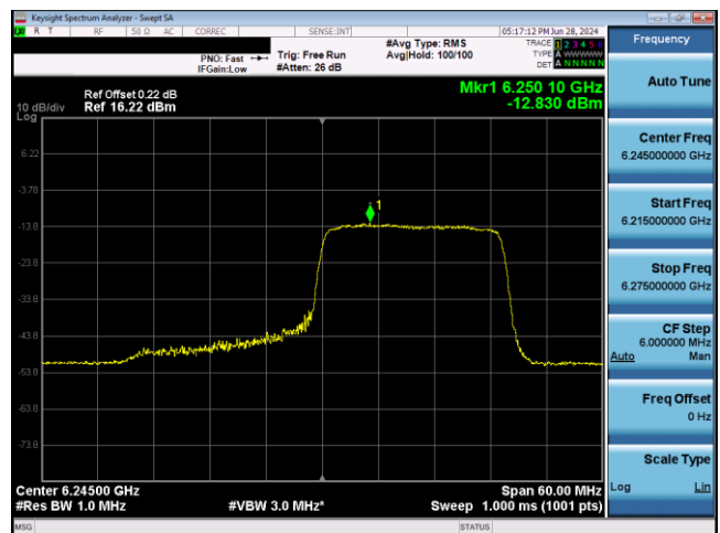
Plot 7-702. VLP Power Spectral Density Plot SDM Antenna WF2 (40MHz) 802.11ax RU242 (UNII Band 5) - Ch. 59
