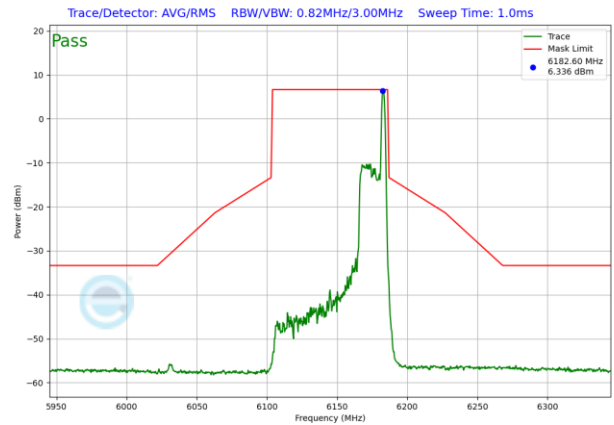
Plot 7-755. SP In-Band Emission Plot Antenna WF5T (80MHz 802.11ax RU26 (UNII Band 5) – Ch. 39)
