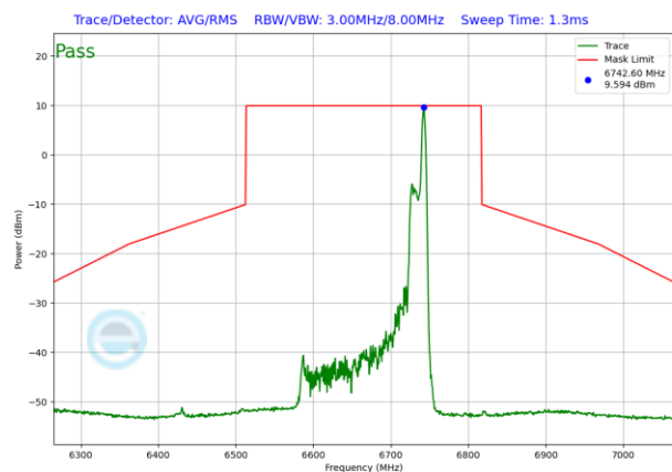
Plot 7-775. SP In-Band Emission Plot Antenna WF5T (160MHz 802.11ax RU26 (UNII Band 7) – Ch. 143)
