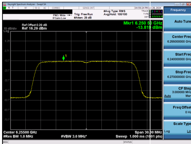
Plot 7-698. VLP Power Spectral Density Plot SDM Antenna WF2 (20MHz) 802.11ax RU242 (UNII Band 5) - Ch. 61
