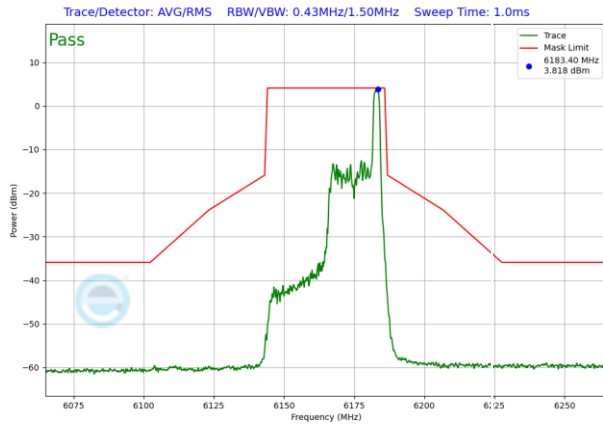
Plot 7-751. SP In-Band Emission Plot Antenna WF5T (40MHz 802.11ax RU26 (UNII Band 5) – Ch. 43)
