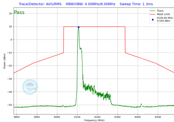
Plot 7-757. SP In-Band Emission Plot Antenna WF5T (160MHz 802.11ax RU26 (UNII Band 5) – Ch. 47)
