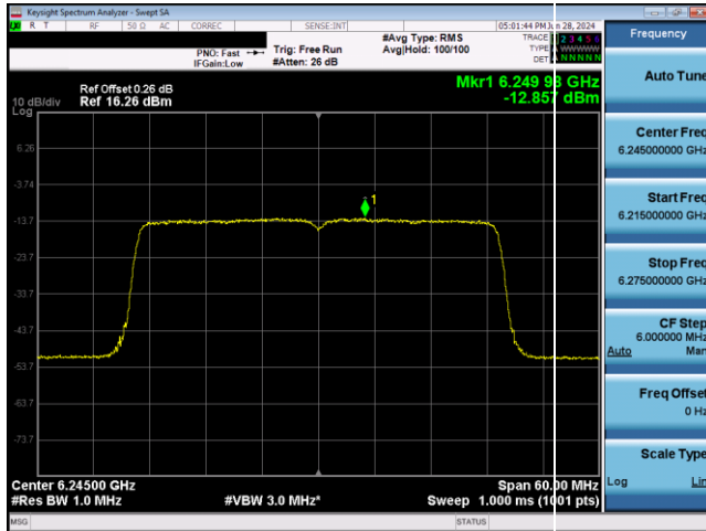
Plot 7-704. VLP Power Spectral Density Plot SDM Antenna WF2 (40MHz 802.11ax RU484 (UNII Band 5) – Ch. 59)
