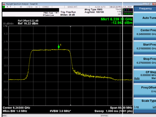
Plot 7-699. VLP Power Spectral Density Plot SDM Antenna WF5T (40MHz) 802.11ax RU242 (UNII Band 5) - Ch. 59
