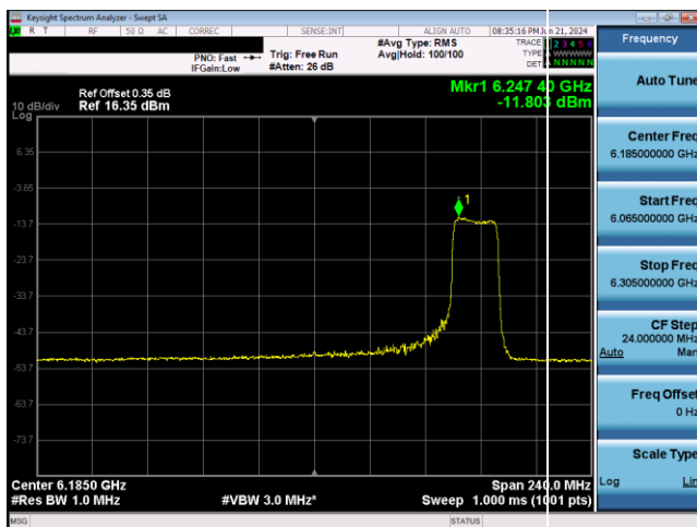
Plot 7-717. VLP Power Spectral Density Plot SDM Antenna WF5T (160MHz 802.11ax RU242 (UNII Band 5) – Ch. 47)
