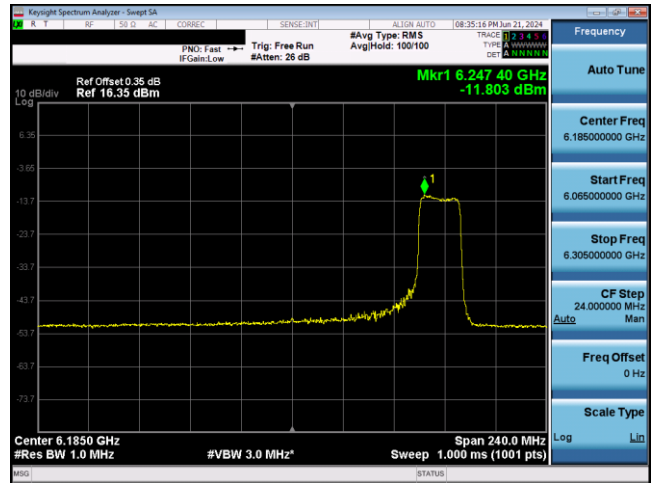
Plot 7-718. VLP Power Spectral Density Plot SDM Antenna WF2 (160MHz 802.11ax RU242 (UNII Band 5) – Ch. 47)
