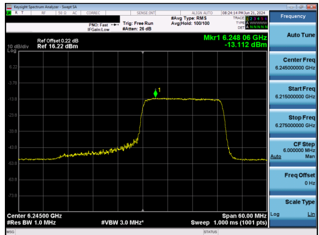
Plot 7-701. VLP Power Spectral Density Plot SDM Antenna WF5T (40MHz) 802.11ax RU242 (UNII Band 5) - Ch. 59
