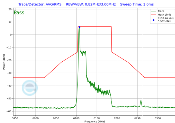
Plot 7-753. SP In-Band Emission Plot Antenna WF5T (80MHz 802.11ax RU26 (UNII Band 5) – Ch. 39)
