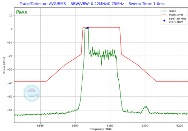
Plot 7-745. SP In-Band Emission Plot Antenna WF5T (20MHz 802.11ax RU26 (UNII Band 5) – Ch. 45)
