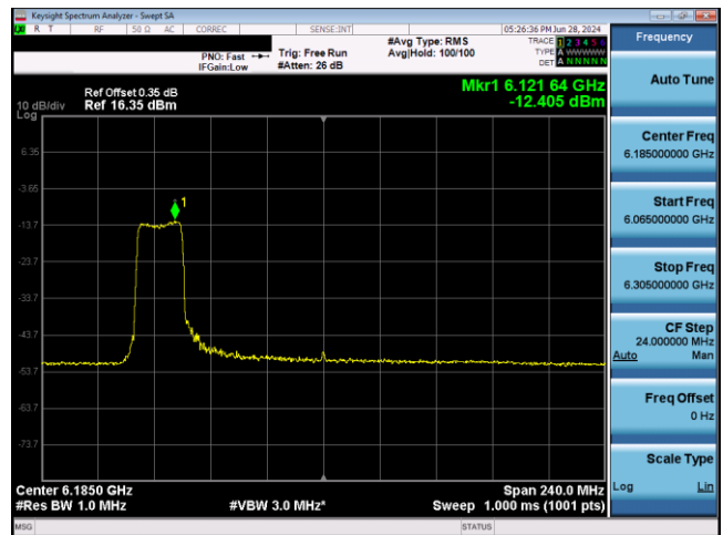
Plot 7-714. VLP Power Spectral Density Plot SDM Antenna WF2 (160MHz 802.11ax RU242 (UNII Band 5) – Ch. 47)
