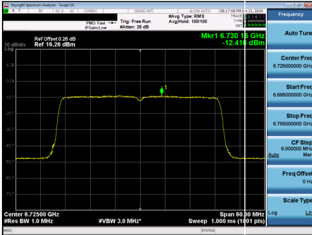
Plot 7-727. VLP Power Spectral Density Plot SDM Antenna WF5T (40MHz 802.11ax RU484 (UNII Band 7) – Ch. 155)
