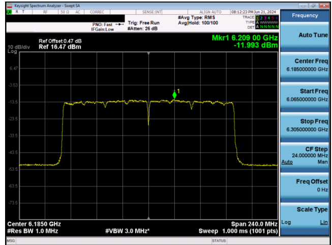
Plot 7-719. VLP Power Spectral Density Plot SDM Antenna WF5T (160MHz 802.11ax RU996x2 (UNII Band 5) – Ch. 47)
