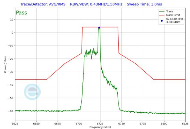
Plot 7-766. SP In-Band Emission Plot Antenna WF5T (40MHz 802.11ax RU26 (UNII Band 7) – Ch. 155)
