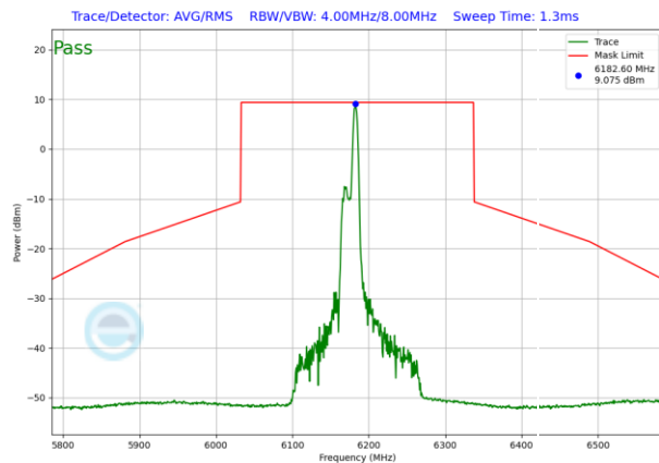
Plot 7-758. SP In-Band Emission Plot Antenna WF5T (160MHz 802.11ax RU26 (UNII Band 5) – Ch. 47)
