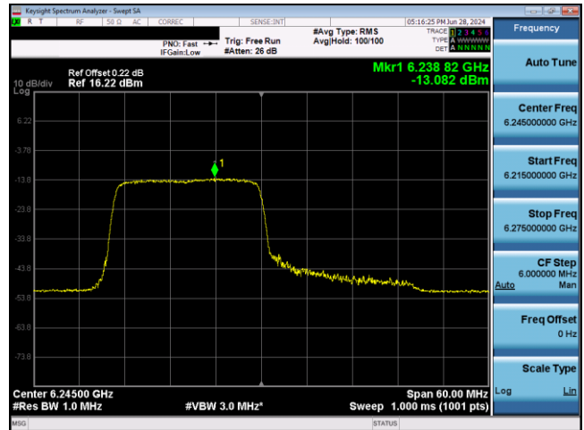
Plot 7-700. VLP Power Spectral Density Plot SDM Antenna WF2 (40MHz) 802.11ax RU242 (UNII Band 5) - Ch. 59
