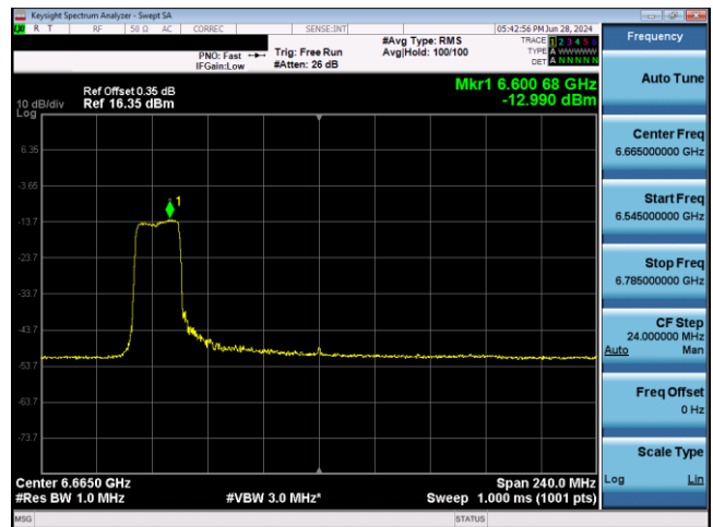
Plot 7-738. VLP Power Spectral Density Plot SDM Antenna WF2 (160MHz 802.11ax RU242 (UNII Band 7) – Ch. 143)
