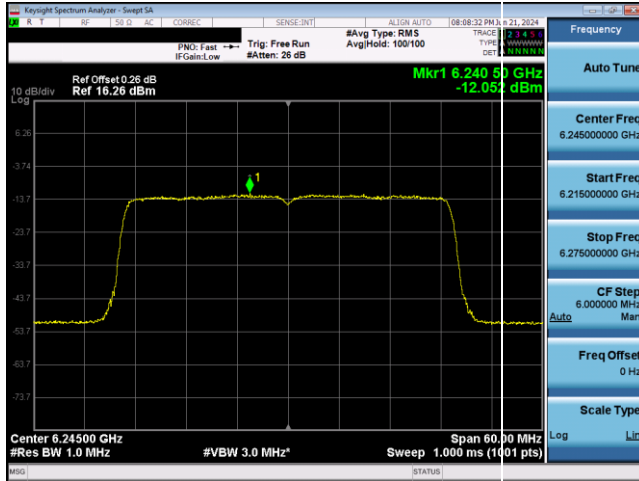
Plot 7-703. VLP Power Spectral Density Plot SDM Antenna WF5T (40MHz 802.11ax RU484 (UNII Band 5) – Ch. 59)
