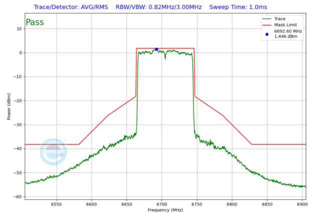
Plot 7-772. SP In-Band Emission Plot Antenna WF5T (80MHz 802.11ax RU996 (UNII Band 7) – Ch. 151)
