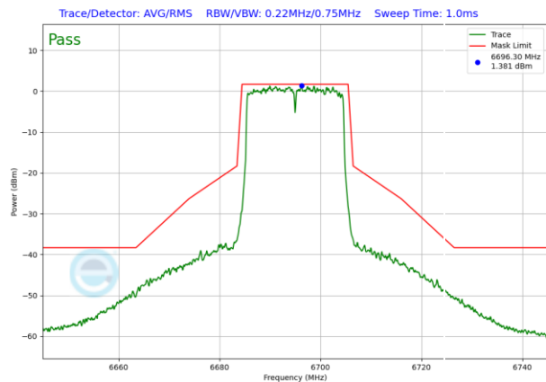
Plot 7-764. SP In-Band Emission Plot Antenna WF5T (20MHz 802.11ax RU242 (UNII Band 7) – Ch. 149)
