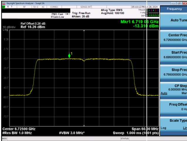
Plot 7-728. VLP Power Spectral Density Plot SDM Antenna WF2 (40MHz 802.11ax RU484 (UNII Band 7) – Ch. 155)
