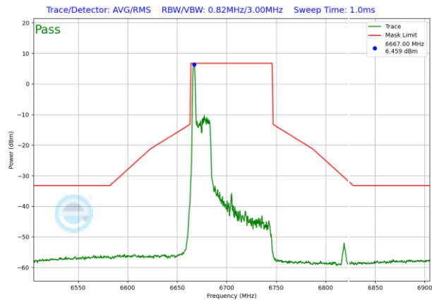
Plot 7-769. SP In-Band Emission Plot Antenna WF5T (80MHz 802.11ax RU26 (UNII Band 7) – Ch. 151)
