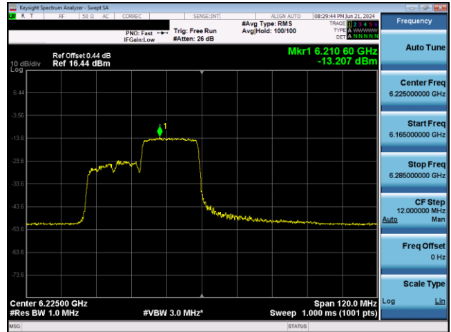
Plot 7-707. VLP Power Spectral Density Plot SDM Antenna WF5T (80MHz 802.11ax RU242 (UNII Band 5) – Ch. 55)
