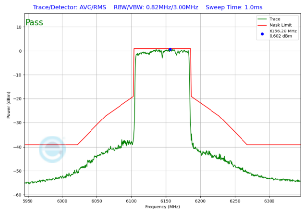
Plot 7-756. SP In-Band Emission Plot Antenna WF5T (80MHz 802.11ax RU996 (UNII Band 5) – Ch. 39)
