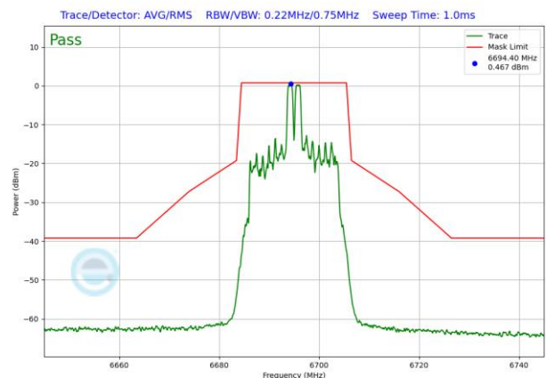
Plot 7-762. SP In-Band Emission Plot Antenna WF5T (20MHz 802.11ax RU26 (UNII Band 7) – Ch. 149)
