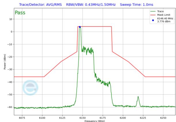
Plot 7-749. SP In-Band Emission Plot Antenna WF5T (40MHz 802.11ax RU26 (UNII Band 5) – Ch. 43)
