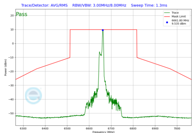
Plot 7-774. SP In-Band Emission Plot Antenna WF5T (160MHz 802.11ax RU26 (UNII Band 7) – Ch. 143)
