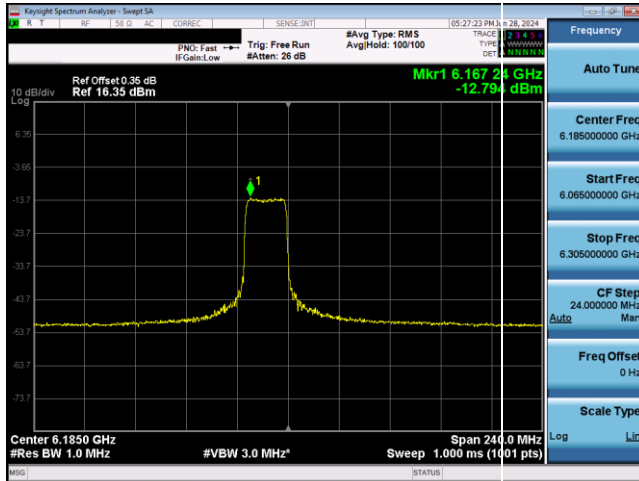
Plot 7-716. VLP Power Spectral Density Plot SDM Antenna WF2 (160MHz 802.11ax RU242 (UNII Band 5) – Ch. 47)
