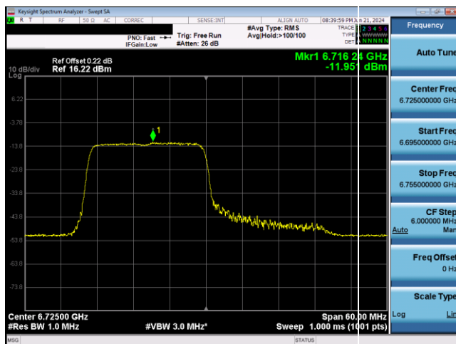
Plot 7-723. VLP Power Spectral Density Plot SDM Antenna WF5T (40MHz 802.11ax RU242 (UNII Band 7) – Ch. 155)
