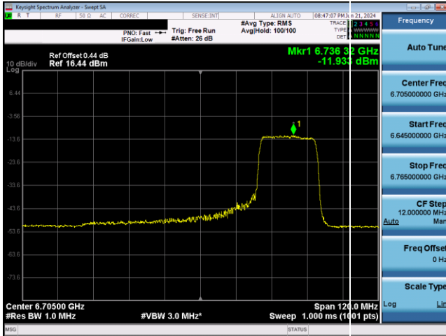
Plot 7-733. VLP Power Spectral Density Plot SDM Antenna WF5T (80MHz 802.11ax RU242 (UNII Band 7) – Ch. 151)
