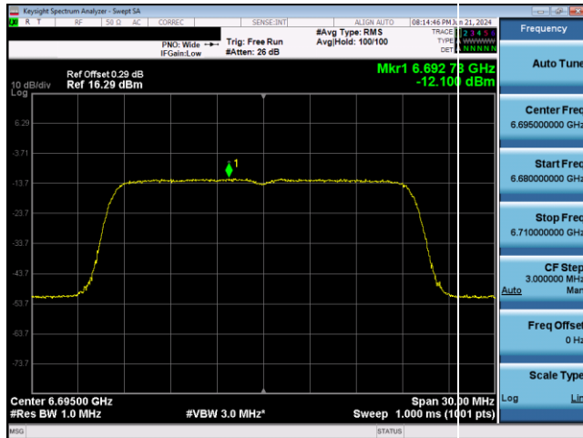
Plot 7-721. VLP Power Spectral Density Plot SDM Antenna WF5T (20MHz 802.11ax RU242 (UNII Band 7) – Ch. 149)
