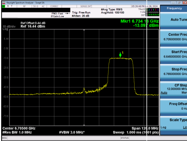
Plot 7-734. VLP Power Spectral Density Plot SDM Antenna WF2 (80MHz 802.11ax RU242 (UNII Band 7) – Ch. 151)
