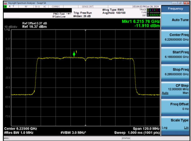
Plot 7-712. VLP Power Spectral Density Plot SDM Antenna WF2 (80MHz 802.11ax RU996 (UNII Band 5) – Ch. 55)
