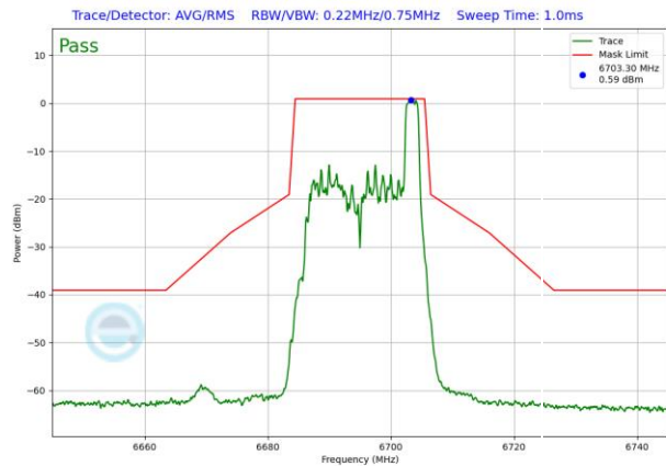
Plot 7-763. SP In-Band Emission Plot Antenna WF5T (20MHz 802.11ax RU26 (UNII Band 7) – Ch. 149)
