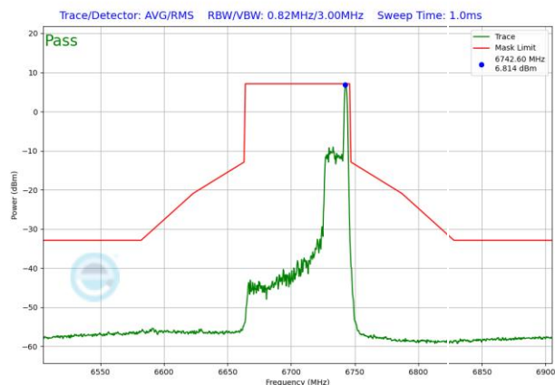
Plot 7-771. SP In-Band Emission Plot Antenna WF5T (80MHz 802.11ax RU26 (UNII Band 7) – Ch. 151)
