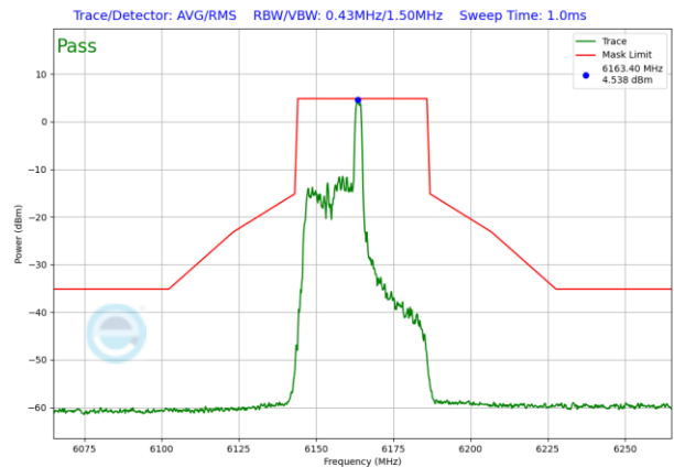
Plot 7-750. SP In-Band Emission Plot Antenna WF5T (40MHz 802.11ax RU26 (UNII Band 5) – Ch. 43)
