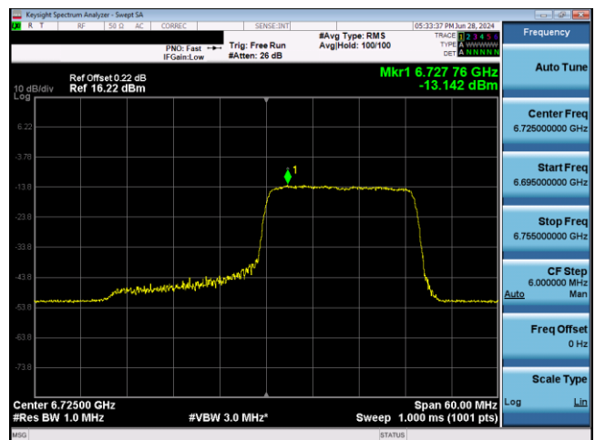
Plot 7-726. VLP Power Spectral Density Plot SDM Antenna WF2 (40MHz 802.11ax RU242 (UNII Band 7) – Ch. 155)
