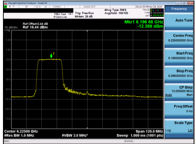
Plot 7-706. VLP Power Spectral Density Plot SDM Antenna WF2 (80MHz 802.11ax RU242 (UNII Band 5) – Ch. 55)
