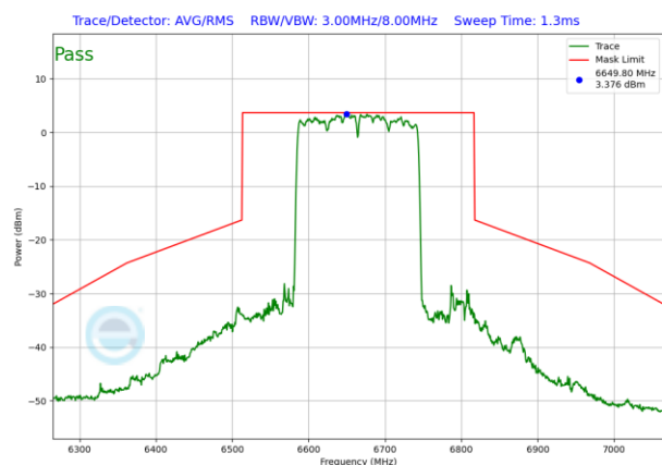
Plot 7-776. SP In-Band Emission Plot Antenna WF5T (160MHz 802.11ax RU996x2 (UNII Band 7) – Ch. 143)
