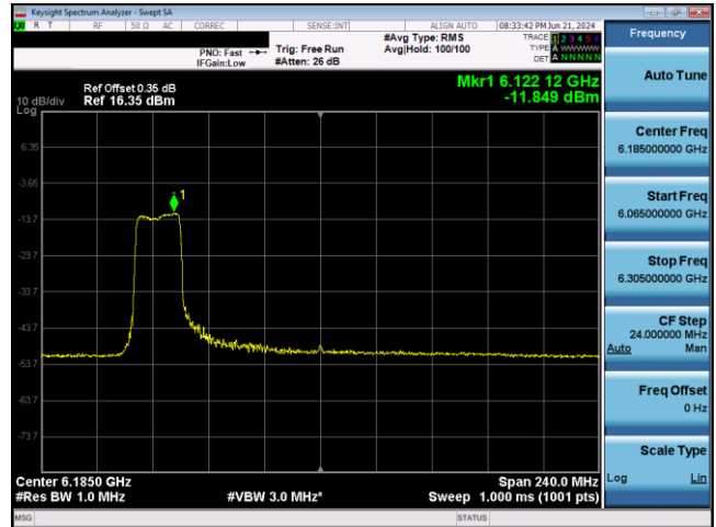
Plot 7-713. VLP Power Spectral Density Plot SDM Antenna WF5T (160MHz 802.11ax RU242 (UNII Band 5) – Ch. 47)
