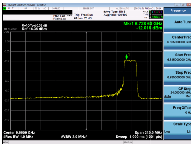
Plot 7-741. VLP Power Spectral Density Plot SDM Antenna WF5T (160MHz 802.11ax RU242 (UNII Band 7) – Ch. 143)
