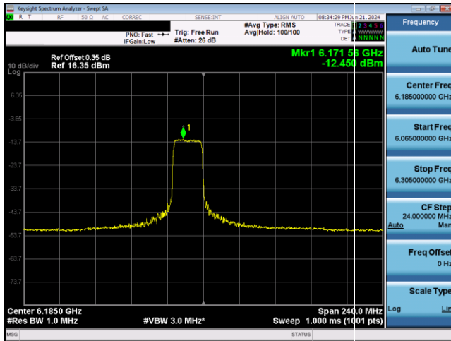
Plot 7-715. VLP Power Spectral Density Plot SDM Antenna WF5T (160MHz 802.11ax RU242 (UNII Band 5) – Ch. 47)
