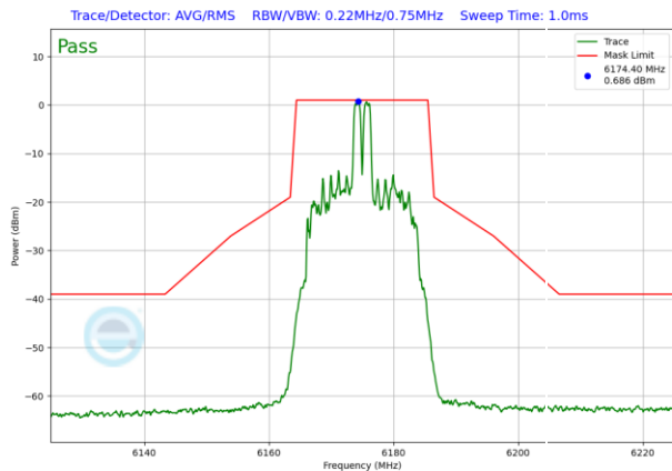
Plot 7-746. SP In-Band Emission Plot Antenna WF5T (20MHz 802.11ax RU26 (UNII Band 5) – Ch. 45)
