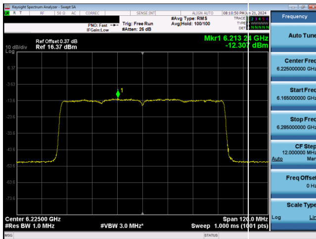
Plot 7-711. VLP Power Spectral Density Plot SDM Antenna WF5T (80MHz 802.11ax RU996 (UNII Band 5) – Ch. 55)
