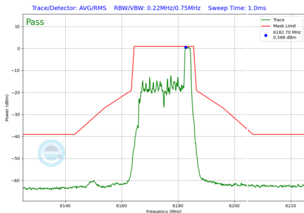
Plot 7-747. SP In-Band Emission Plot Antenna WF5T (20MHz 802.11ax RU26 (UNII Band 5) – Ch. 45)
