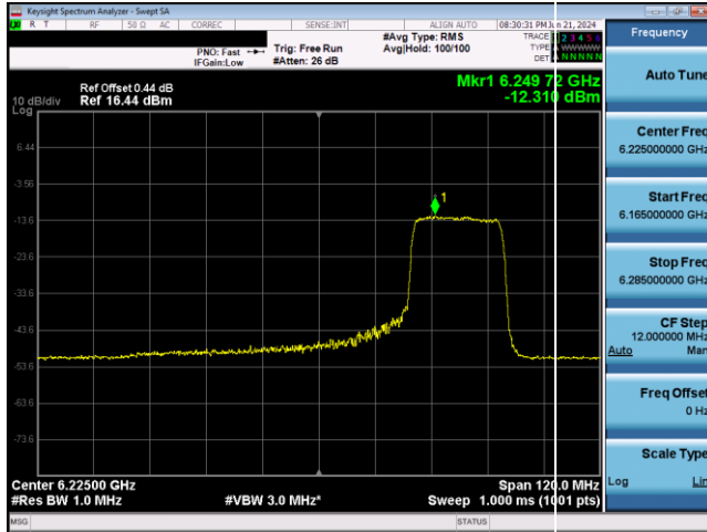
Plot 7-709. VLP Power Spectral Density Plot SDM Antenna WF5T (80MHz 802.11ax RU242 (UNII Band 5) – Ch. 55)
