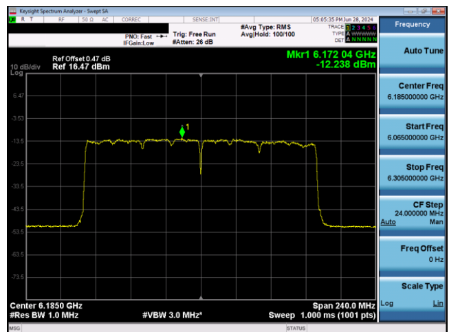
Plot 7-720. VLP Power Spectral Density Plot SDM Antenna WF2 (160MHz 802.11ax RU996x2 (UNII Band 5) – Ch. 47)
