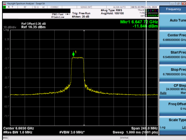
Plot 7-739. VLP Power Spectral Density Plot SDM Antenna WF5T (160MHz 802.11ax RU242 (UNII Band 7) – Ch. 143)
