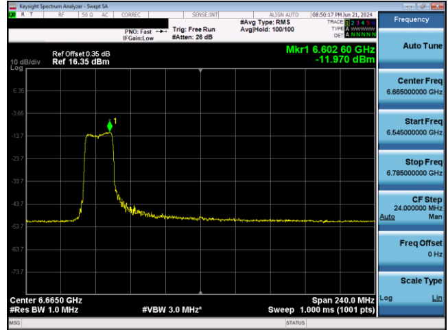
Plot 7-737. VLP Power Spectral Density Plot SDM Antenna WF5T (160MHz 802.11ax RU242 (UNII Band 7) – Ch. 143)
