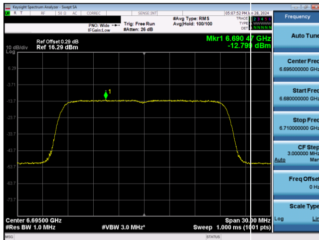
Plot 7-722. VLP Power Spectral Density Plot SDM Antenna WF2 (20MHz 802.11ax RU242 (UNII Band 7) – Ch. 149)
