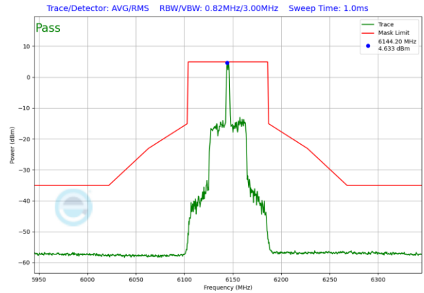
Plot 7-754. SP In-Band Emission Plot Antenna WF5T (80MHz 802.11ax RU26 (UNII Band 5) – Ch. 39)
