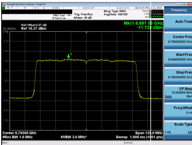
Plot 7-735. VLP Power Spectral Density Plot SDM Antenna WF5T (80MHz 802.11ax RU996 (UNII Band 7) – Ch. 151)
