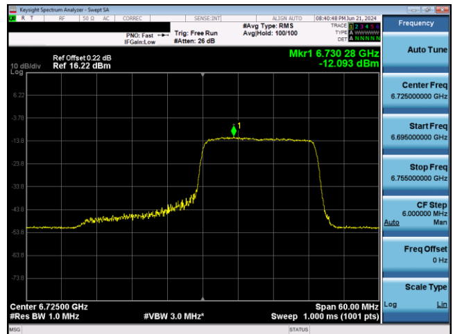
Plot 7-725. VLP Power Spectral Density Plot SDM Antenna WF5T (40MHz 802.11ax RU242 (UNII Band 7) – Ch. 155)
