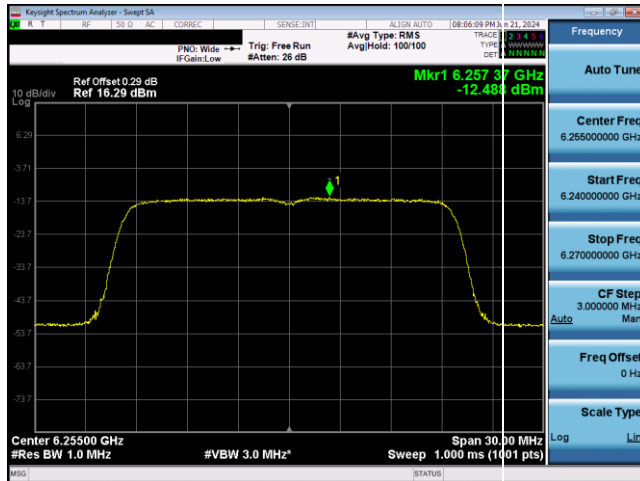
Plot 7-697. VLP Power Spectral Density Plot SDM Antenna WF5T (20MHz) 802.11ax RU242 (UNII Band 5) - Ch. 61
