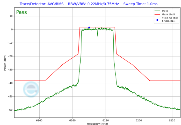
Plot 7-748. SP In-Band Emission Plot Antenna WF5T (20MHz 802.11ax RU242 (UNII Band 5) – Ch. 45)
