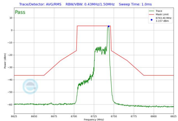
Plot 7-767. SP In-Band Emission Plot Antenna WF5T (40MHz 802.11ax RU26 (UNII Band 7) – Ch. 155)
