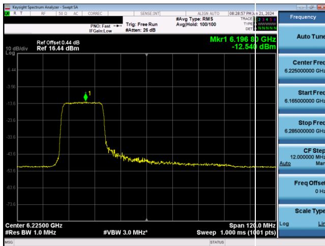
Plot 7-705. VLP Power Spectral Density Plot SDM Antenna WF5T (80MHz 802.11ax RU242 (UNII Band 5) – Ch. 55)
