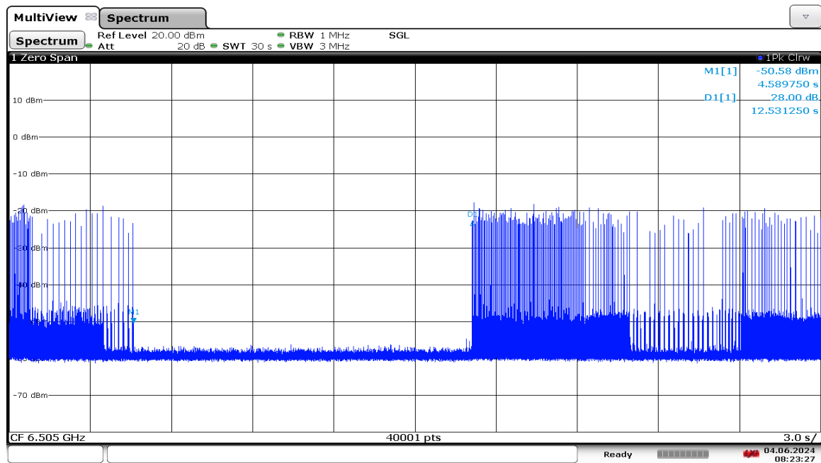
Plot 7-1258. LPI Contention Based Protocol Timing Plot – UNII 6 – 160MHz Channel 111 – Low
