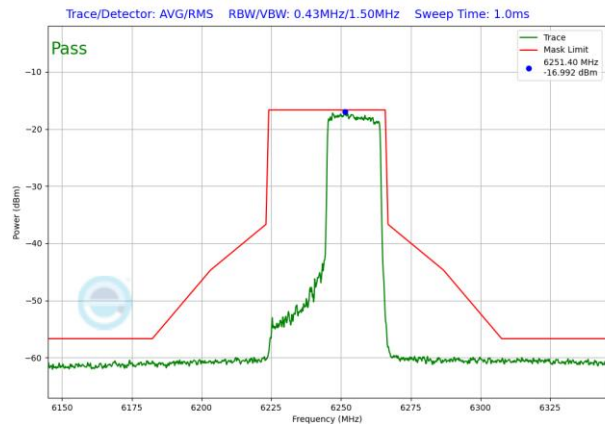
Plot 7-1194. VLP In-Band Emission Plot SDM Antenna WF2 (40MHz) 802.11ax RU242 (UNII Band 5) – Ch. 59)
