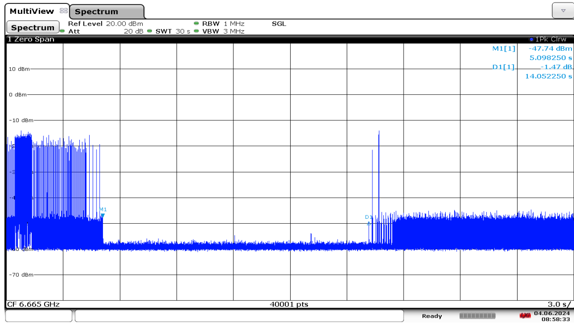
Plot 7-1263. LPI Contention Based Protocol Timing Plot – UNII 7 – 160MHz Channel 143 – Mid
