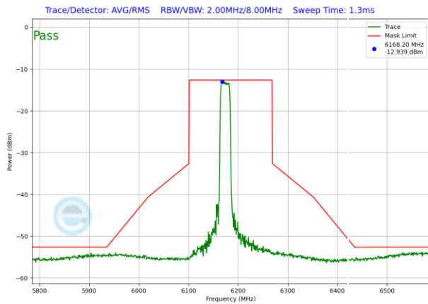
Plot 7-1207. VLP In-Band Emission Plot SDM Antenna WF5T (160MHz 802.11ax RU242 (UNII Band 5) – Ch. 47)
