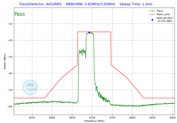
Plot 7-1224. VLP In-Band Emission Plot SDM Antenna WF2 (80MHz 802.11ax RU242 (UNII Band 7) – Ch. 151)
