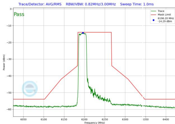
Plot 7-1197. VLP In-Band Emission Plot SDM Antenna WF5T (80MHz) 802.11ax RU242 (UNII Band 5) – Ch. 55
