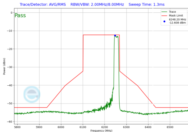
Plot 7-1209. VLP In-Band Emission Plot SDM Antenna WF5T (160MHz 802.11ax RU242 (UNII Band 5) – Ch. 47)
