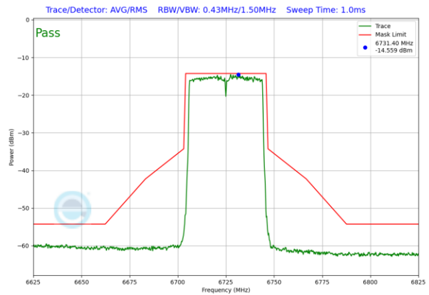
Plot 7-1180. VLP In-Band Emission Plot Antenna WF2 (40MHz 802.11ax RU484 (UNII Band 7) – Ch. 155)
