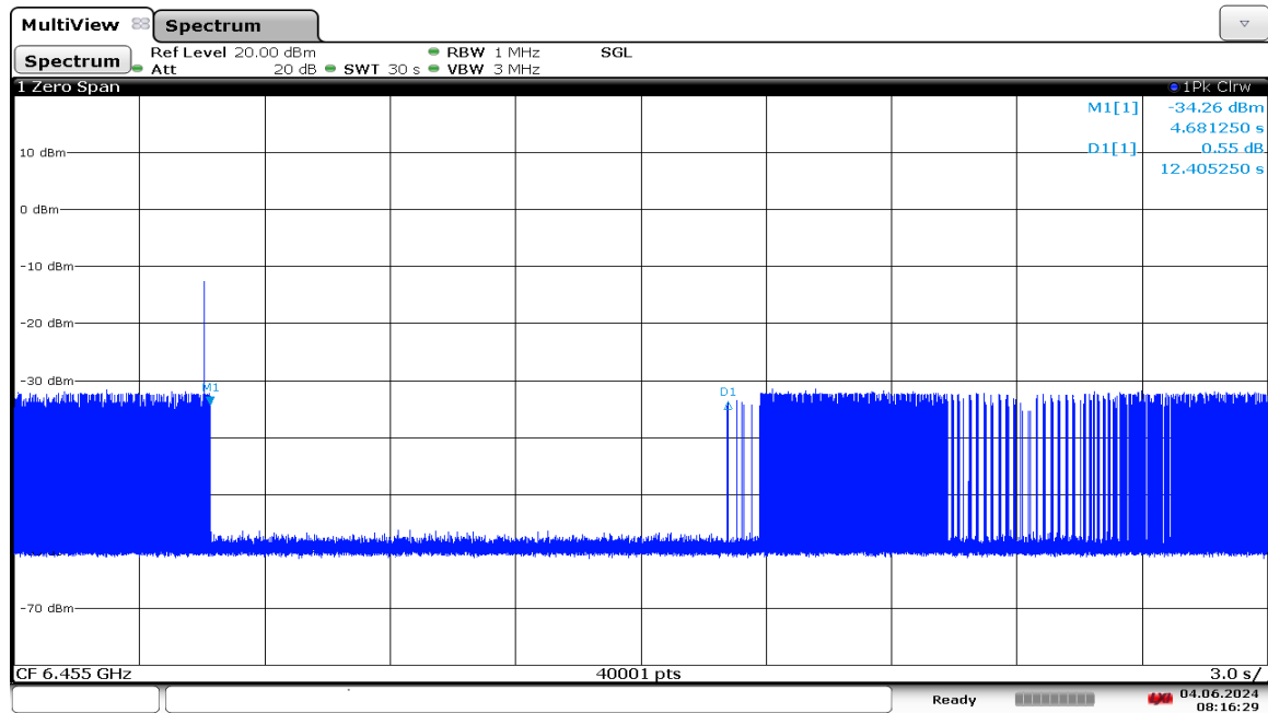
Plot 7-1257. LPI Contention Based Protocol Timing Plot – UNII 6 – 20MHz Channel 101
