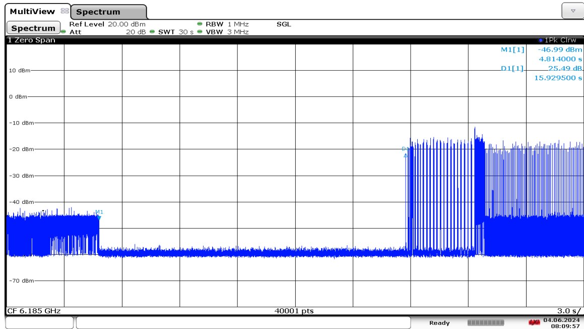
Plot 7-1256. LPI Contention Based Protocol Timing Plot – UNII 5 – 160MHz Channel 47 – High
