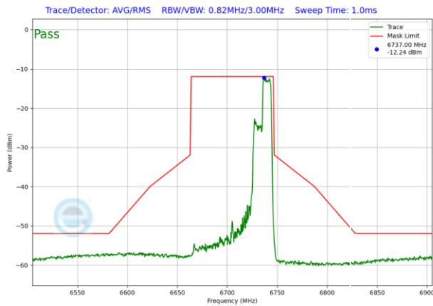
Plot 7-1183. VLP In-Band Emission Plot Antenna WF2 (80MHz 802.11ax RU106 (UNII Band 7) – Ch. 151)
