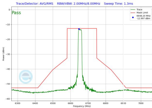
Plot 7-1231. VLP In-Band Emission Plot SDM Antenna WF5T (160MHz 802.11ax RU242 (UNII Band 7) – Ch. 143)
