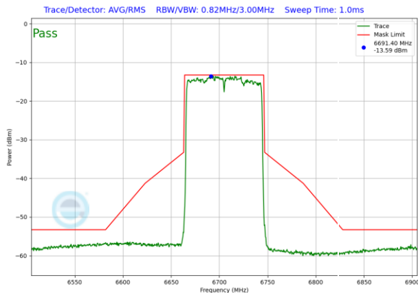
Plot 7-1227. VLP In-Band Emission Plot SDM Antenna WF5T (80MHz 802.11ax RU996 (UNII Band 7) – Ch. 151)
