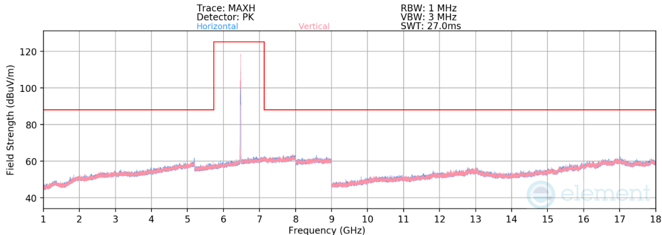
Plot 7-1285. Radiated Spurious Emissions above 1GHz Antenna WF5T (802.11ax – Ch. 105 – RU26)
