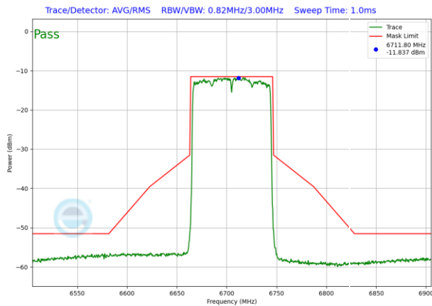
Plot 7-1184. VLP In-Band Emission Plot Antenna WF2 (80MHz 802.11ax RU996 (UNII Band 7) – Ch. 151)
