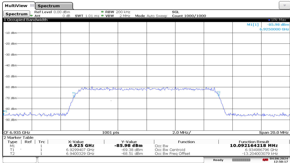
Plot 7-1249. AWGN Signal – UNII 8 – 20MHz
