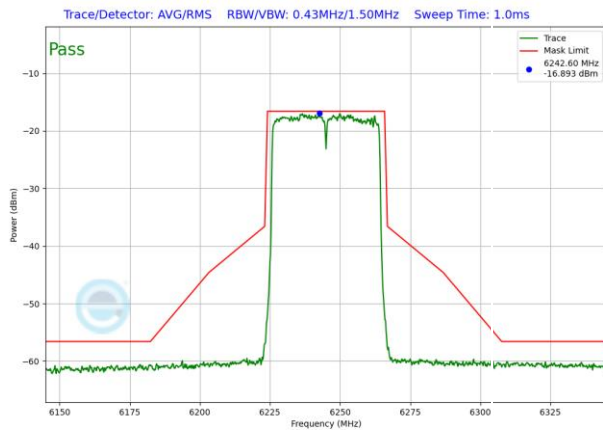
Plot 7-1196. VLP In-Band Emission Plot SDM Antenna WF2 (40MHz) 802.11ax RU484 (UNII Band 5) – Ch. 59
