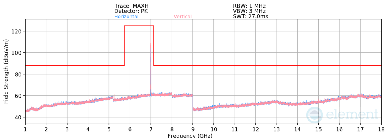
Plot 7-1291. Radiated Spurious Emissions above 1GHz Antenna WF5T (802.11ax – Ch. 209 – RU26)
