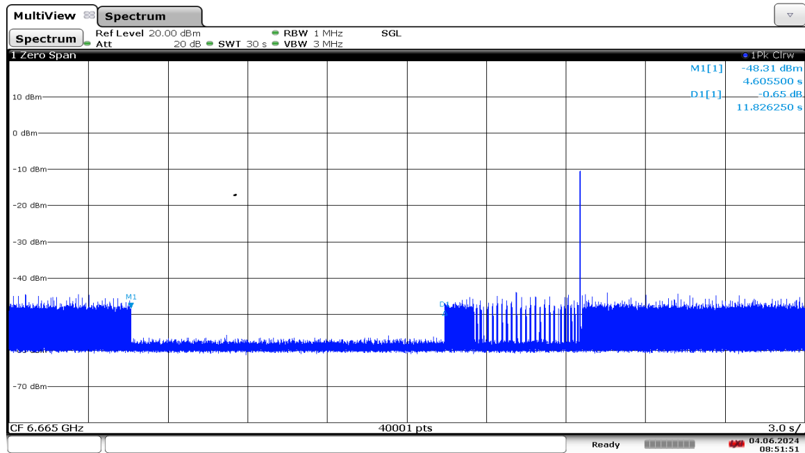
Plot 7-1262. LPI Contention Based Protocol Timing Plot – UNII 7 – 160MHz Channel 143 – Low
