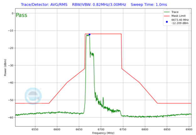
Plot 7-1181. VLP In-Band Emission Plot Antenna WF2 (80MHz 802.11ax RU106 (UNII Band 7) – Ch. 151)
