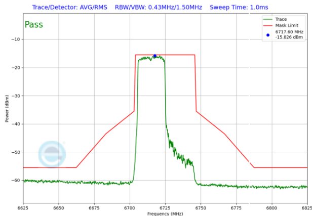
Plot 7-1215. VLP In-Band Emission Plot SDM Antenna WF5T (40MHz) 802.11ax RU242 (UNII Band 7) – Ch. 155
