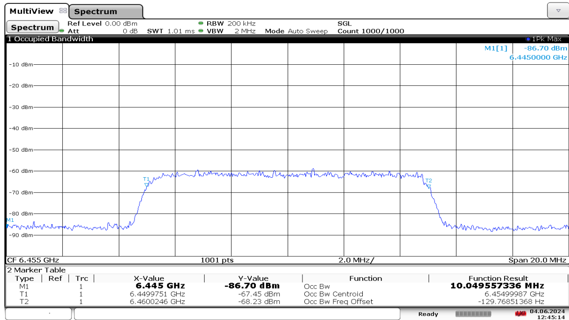
Plot 7-1241. AWGN Signal – UNII 6 – 20MHz
