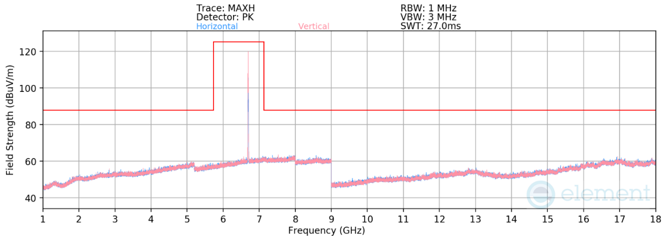
Plot 7-1288. Radiated Spurious Emissions above 1GHz Antenna WF5T (802.11ax – Ch. 149 – RU26)
