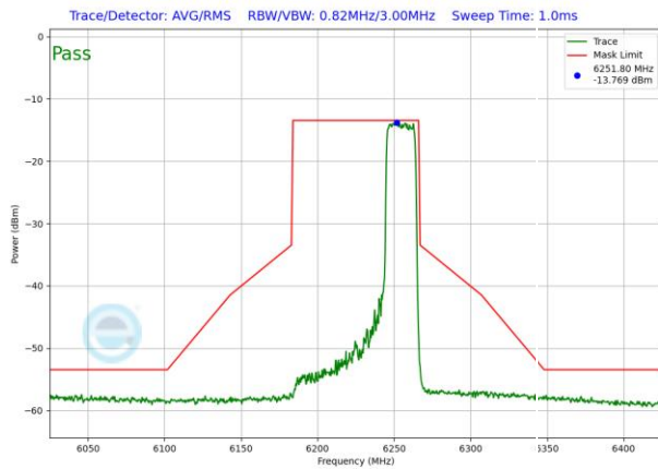
Plot 7-1201. VLP In-Band Emission Plot SDM Antenna WF5T (80MHz) 802.11ax RU242 (UNII Band 5) – Ch. 55)
