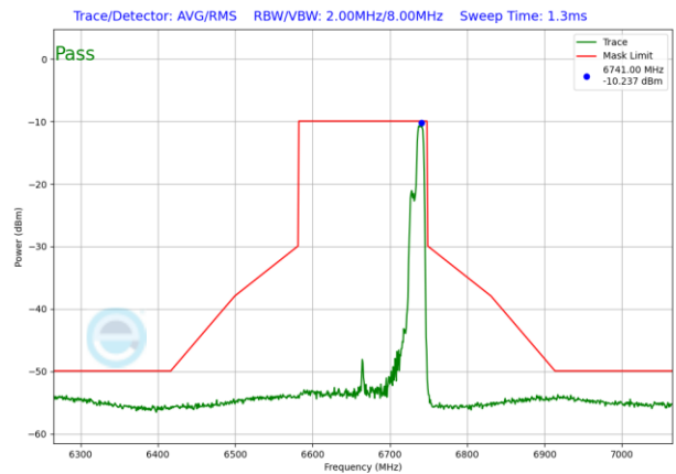
Plot 7-1187. VLP In-Band Emission Plot Antenna WF2 (160MHz 802.11ax RU106 (UNII Band 7) – Ch. 143)
