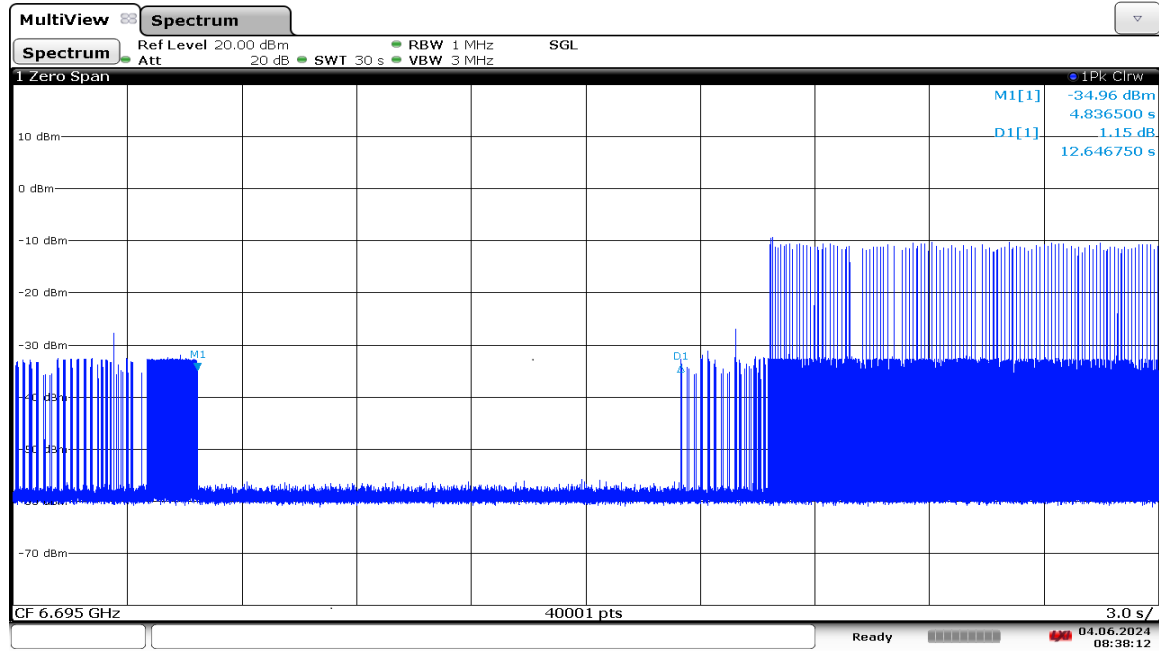
Plot 7-1261. LPI Contention Based Protocol Timing Plot – UNII 7 – 20MHz Channel 149
