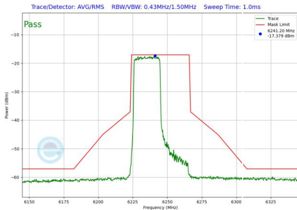
Plot 7-1191. VLP In-Band Emission Plot SDM Antenna WF5T (40MHz) 802.11ax RU242 (UNII Band 5) – Ch. 59)
