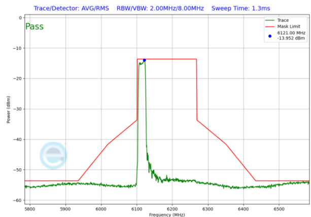
Plot 7-1206. VLP In-Band Emission Plot SDM Antenna WF2 (160MHz) 802.11ax RU242 (UNII Band 5) – Ch. 47)
