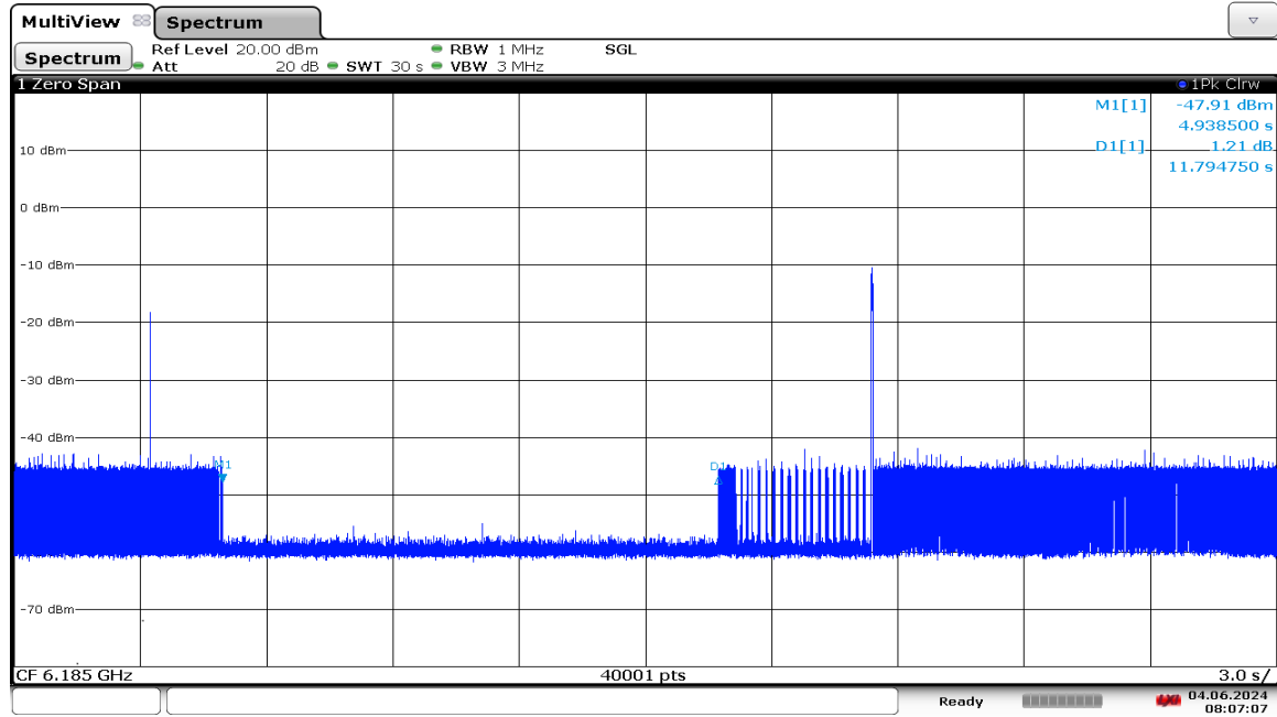
Plot 7-1255. LPI Contention Based Protocol Timing Plot – UNII 5 – 160MHz Channel 47 – Mid
