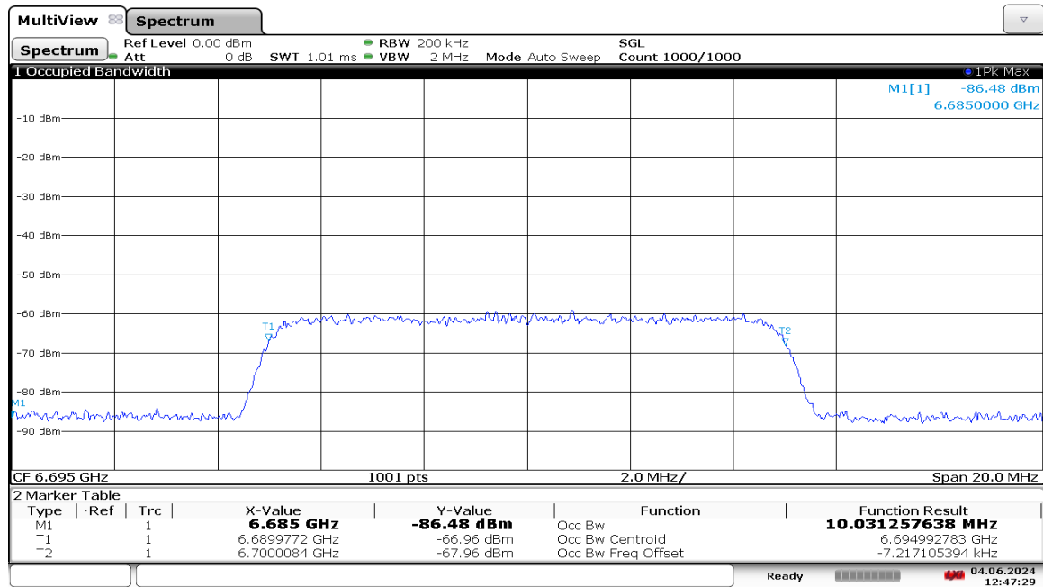
Plot 7-1245. AWGN Signal – UNII 7 – 20MHz
