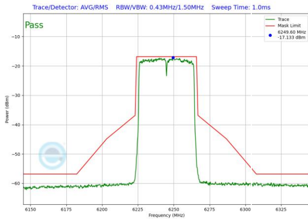
Plot 7-1195. VLP In-Band Emission Plot SDM Antenna WF5T (40MHz) 802.11ax RU484 (UNII Band 5) – Ch. 59
