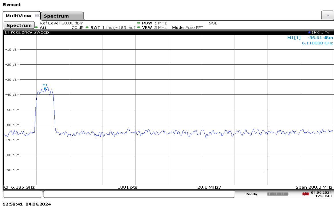
Plot 7-1278. 160MHz Bandwidth – AWGN Signal Injected at Low End – Channel 47
