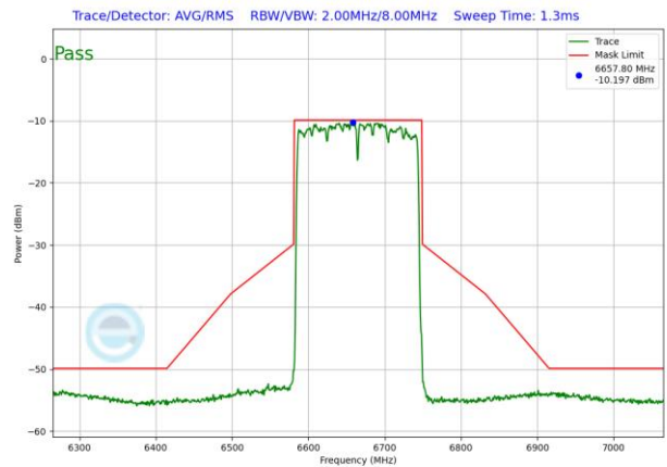
Plot 7-1235. VLP In-Band Emission Plot SDM Antenna WF5T (160MHz 802.11ax RU996x2 (UNII Band 7) – Ch. 143)
