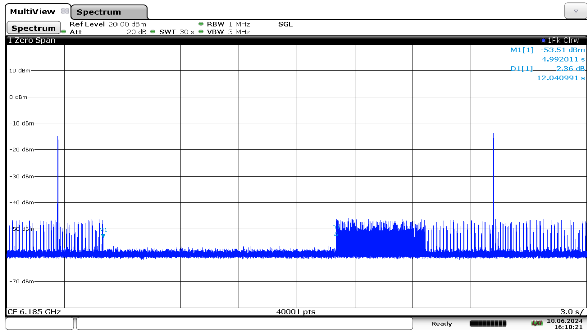
Plot 7-1272. VLP Contention Based Protocol Timing Plot – UNII 5 – 160MHz Channel 47 – High
