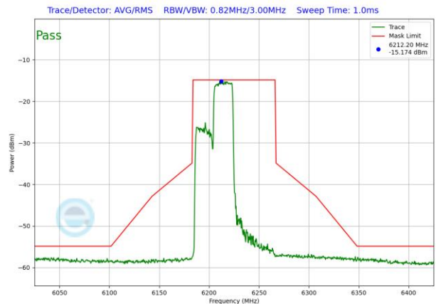
Plot 7-1200. VLP In-Band Emission Plot SDM Antenna WF2 (80MHz) 802.11ax RU242 (UNII Band 5) – Ch. 55
