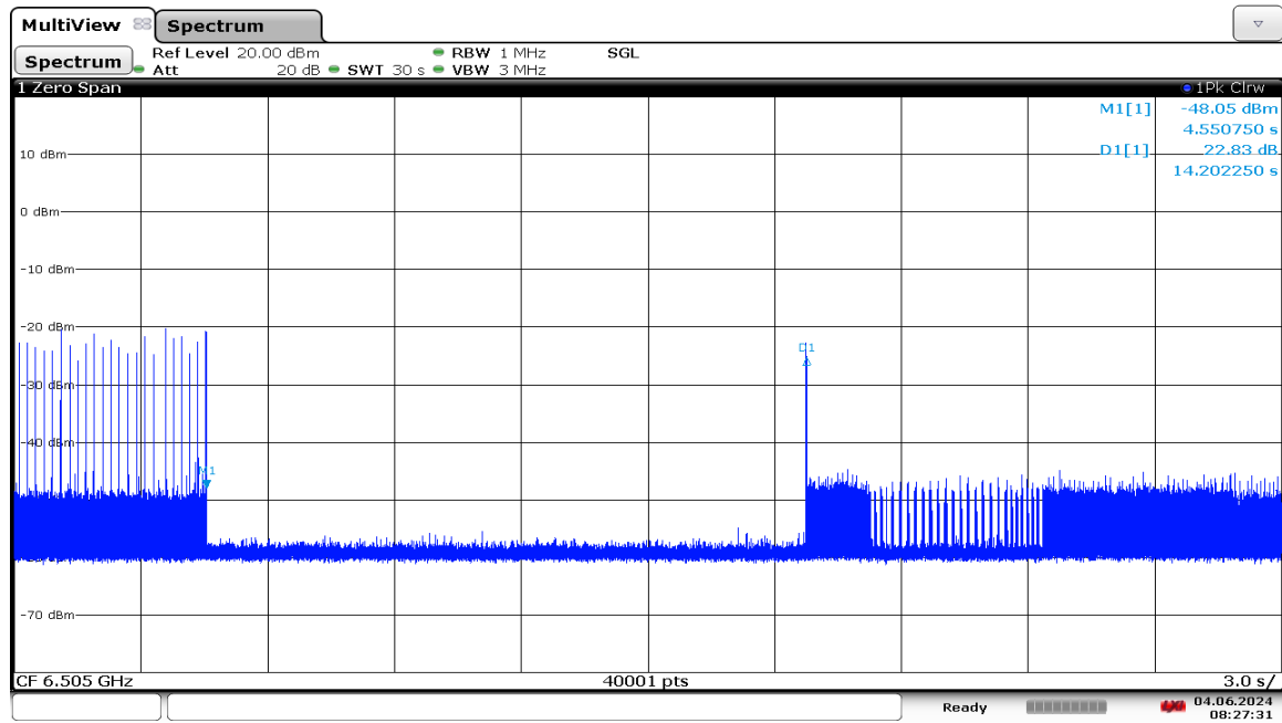
Plot 7-1259. LPI Contention Based Protocol Timing Plot – UNII 6 – 160MHz Channel 111 – Mid
