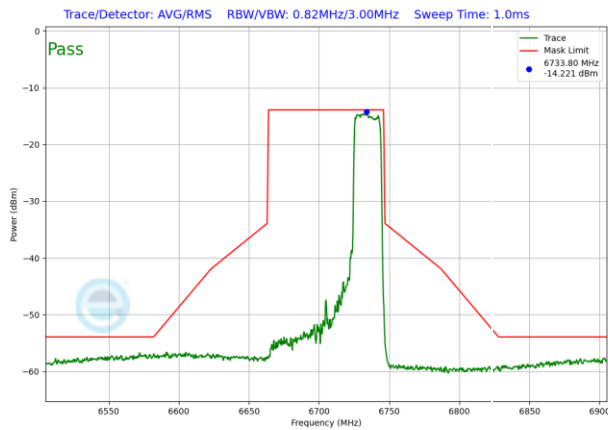
Plot 7-1225. VLP In-Band Emission Plot SDM Antenna WF5T (80MHz 802.11ax RU242 (UNII Band 7) – Ch. 151)
