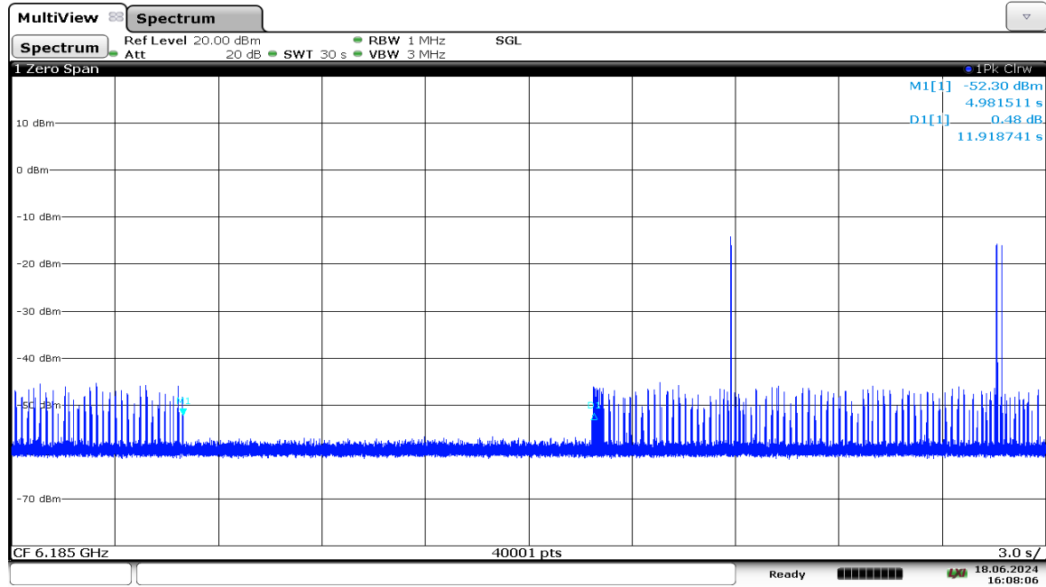
Plot 7-1271. VLP Contention Based Protocol Timing Plot – UNII 5 – 160MHz Channel 47 – Mid
