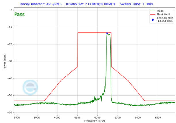
Plot 7-1210. VLP In-Band Emission Plot SDM Antenna WF2 (160MHz 802.11ax RU242 (UNII Band 5) – Ch. 47)
