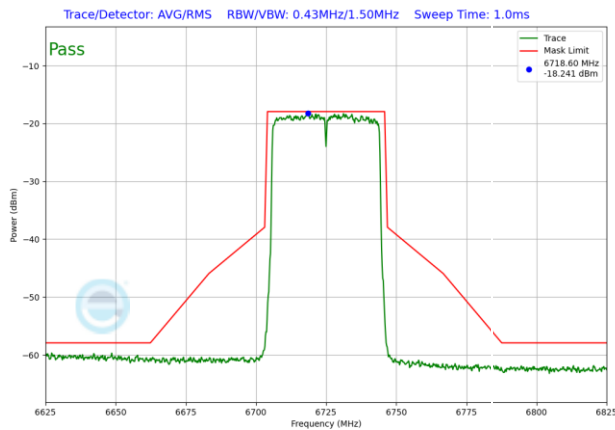
Plot 7-1220. VLP In-Band Emission Plot SDM Antenna WF2 (40MHz 802.11ax RU484 (UNII Band 7) – Ch. 155)
