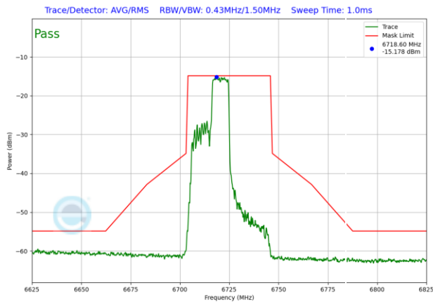
Plot 7-1178. VLP In-Band Emission Plot Antenna WF2 (40MHz 802.11ax RU106 (UNII Band 7) – Ch. 155)
