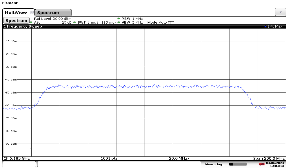
Plot 7-1277. 160MHz Bandwidth – Before AWGN Signal Injected – Channel 47
