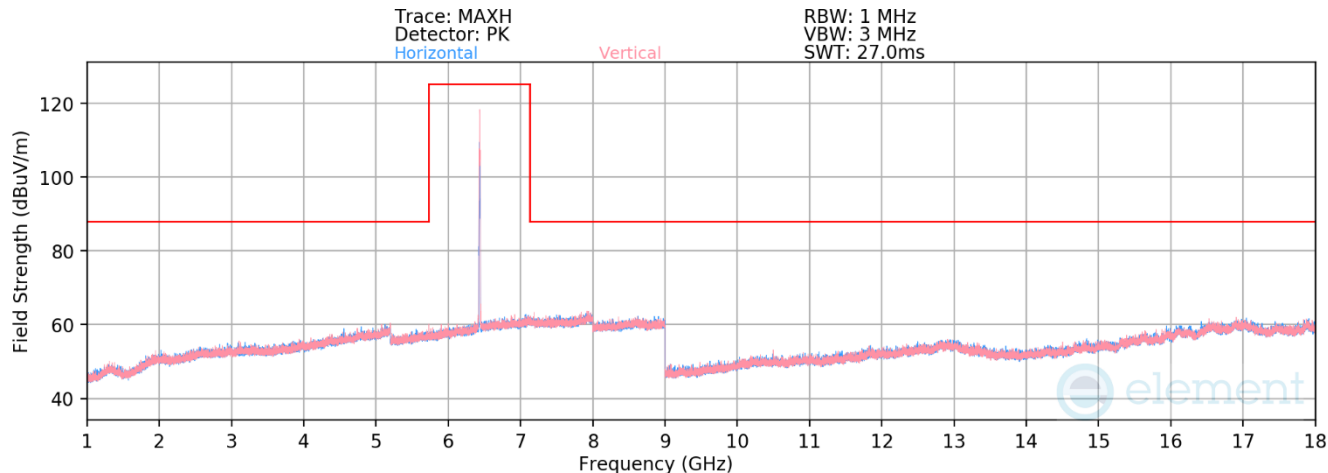
Plot 7-1284. Radiated Spurious Emissions above 1GHz Antenna WF5T (802.11ax – Ch. 97 – RU26)
