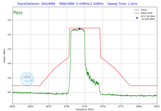
Plot 7-1217. VLP In-Band Emission Plot SDM Antenna WF5T (40MHz) 802.11ax RU242 (UNII Band 7) – Ch. 155
