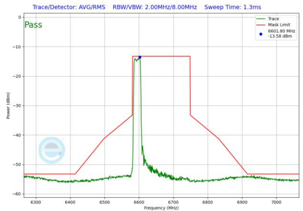
Plot 7-1229. VLP In-Band Emission Plot SDM Antenna WF5T (160MHz 802.11ax RU242 (UNII Band 7) – Ch. 143)
