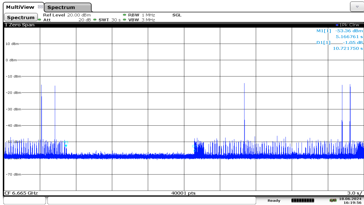
Plot 7-1275. VLP Contention Based Protocol Timing Plot – UNII 7 – 160MHz Channel 143 – Mid
