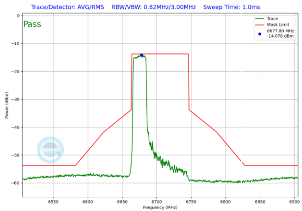
Plot 7-1221. VLP In-Band Emission Plot SDM Antenna WF5T (80MHz 802.11ax RU242 (UNII Band 7) – Ch. 151)
