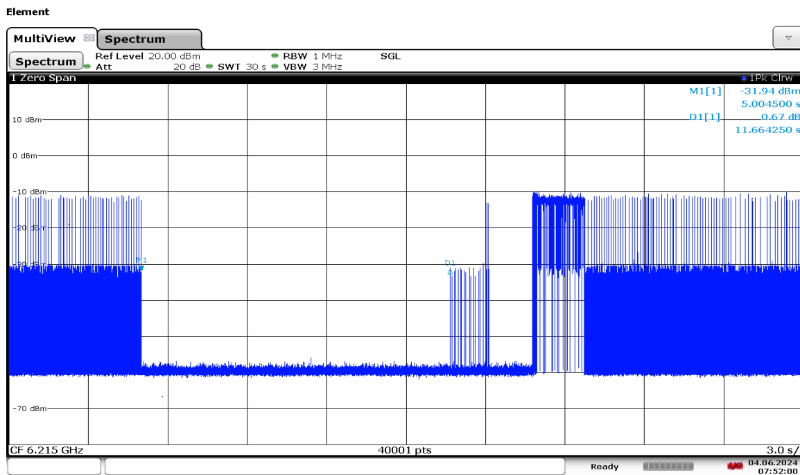
Plot 7-1253. LPI Contention Based Protocol Timing Plot – UNII 5 – 20MHz Channel 53
