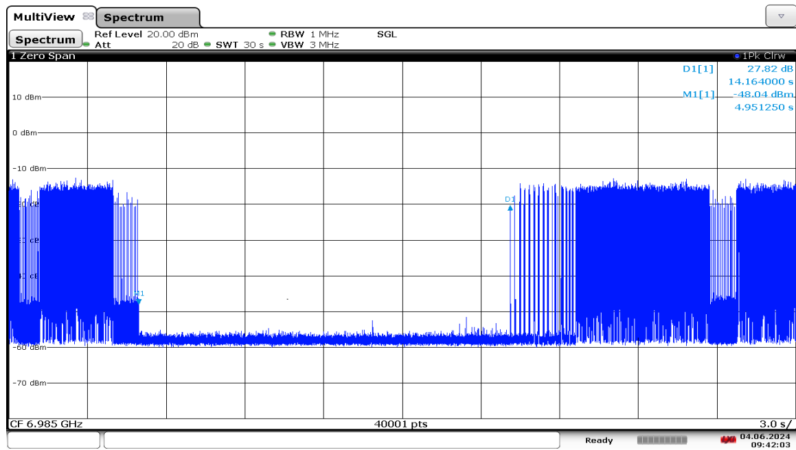
Plot 7-1266. LPI Contention Based Protocol Timing Plot – UNII 8 – 160MHz Channel 207 – Low
