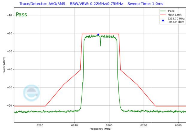
Plot 7-1190. VLP In-Band Emission Plot SDM Antenna WF2 (20MHz) 802.11ax RU242 (UNII Band 5) – Ch. 61)
