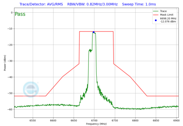
Plot 7-1182. VLP In-Band Emission Plot Antenna WF2 (80MHz 802.11ax RU106 (UNII Band 7) – Ch. 151)
