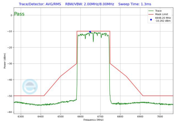
Plot 7-1236. VLP In-Band Emission Plot SDM Antenna WF2 (160MHz 802.11ax RU996x2 (UNII Band 7) – Ch. 143)
