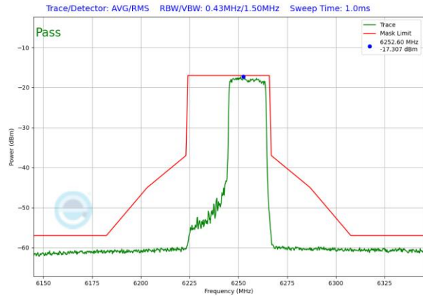
Plot 7-1193. VLP In-Band Emission Plot SDM Antenna WF5T (40MHz) 802.11ax RU242 (UNII Band 5) – Ch. 59)
