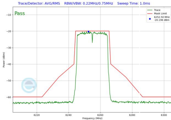
Plot 7-1189. VLP In-Band Emission Plot SDM Antenna WF5T (20MHz) 802.11ax RU242 (UNII Band 5) – Ch. 61)
