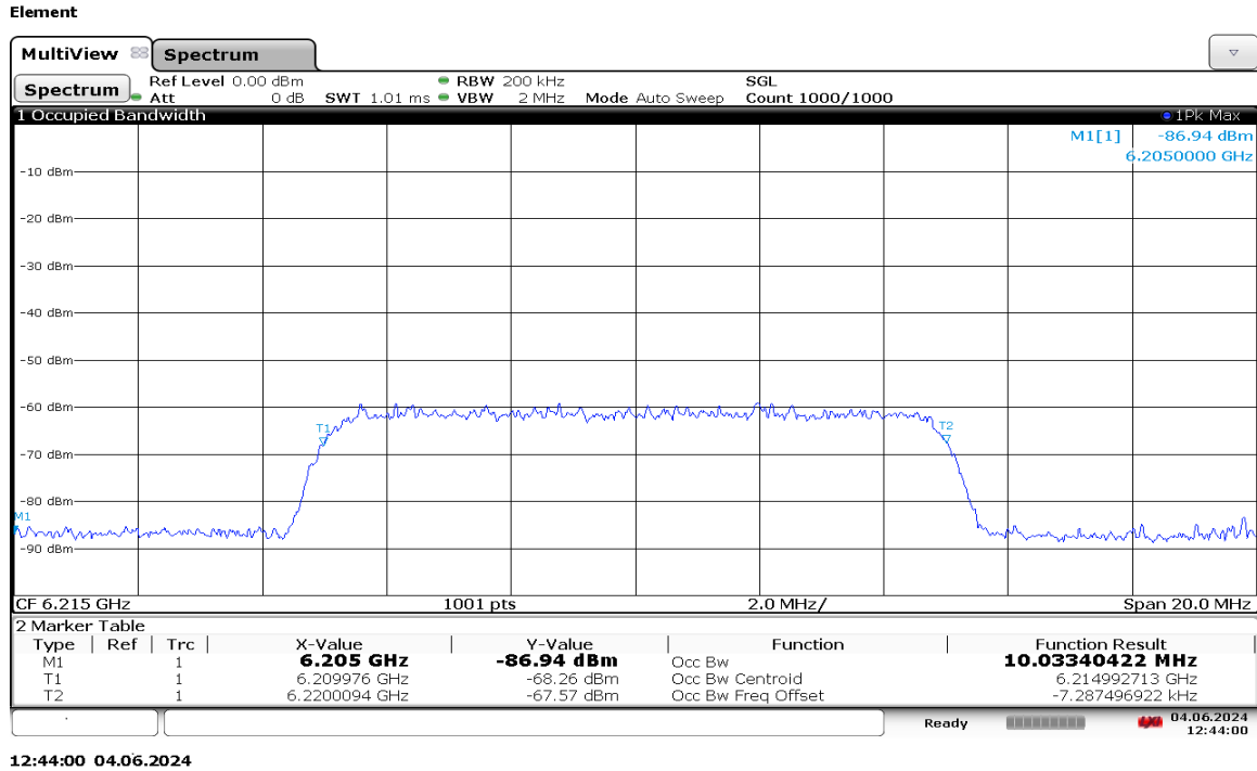
Plot 7-1237. AWGN Signal – UNII 5 – 20MHz
