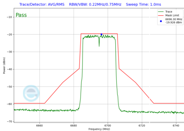
Plot 7-1214. VLP In-Band Emission Plot SDM Antenna WF2 (20MHz) 802.11ax RU242 (UNII Band 7) – Ch. 149
