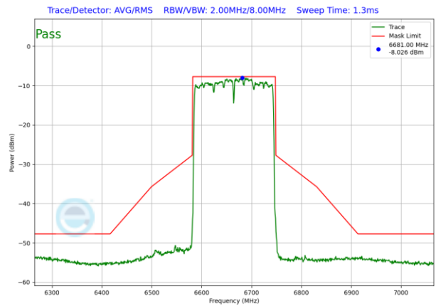
Plot 7-1188. VLP In-Band Emission Plot Antenna WF2 (160MHz 802.11ax RU996x2 (UNII Band 7) – Ch. 143)
