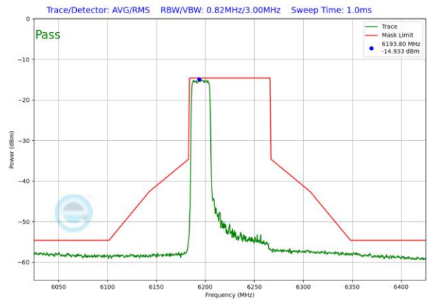
Plot 7-1198. VLP In-Band Emission Plot SDM Antenna WF2 (80MHz) 802.11ax RU242 (UNII Band 5) – Ch. 55
