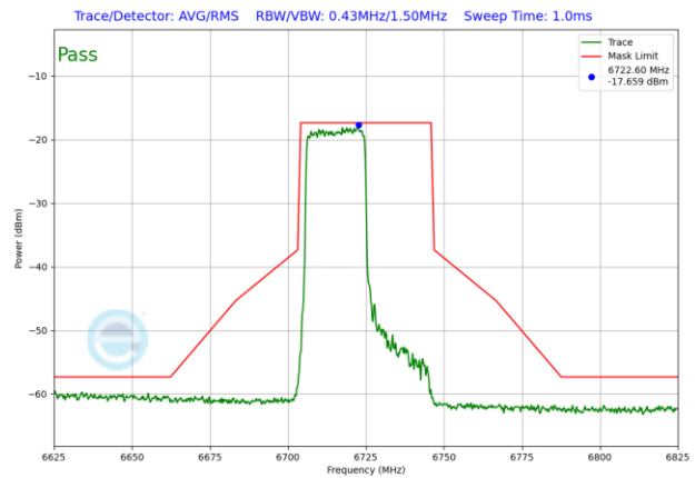
Plot 7-1216. VLP In-Band Emission Plot SDM Antenna WF2 (40MHz) 802.11ax RU242 (UNII Band 7) – Ch. 155
