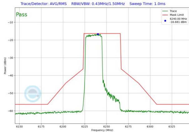
Plot 7-1192. VLP In-Band Emission Plot SDM Antenna WF2 (40MHz) 802.11ax RU242 (UNII Band 5) – Ch. 59)
