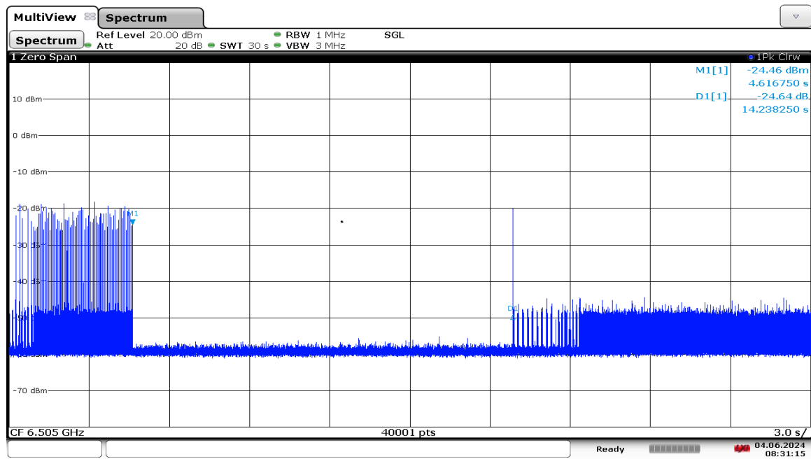
Plot 7-1260. LPI Contention Based Protocol Timing Plot – UNII 6 – 160MHz Channel 111 – High
