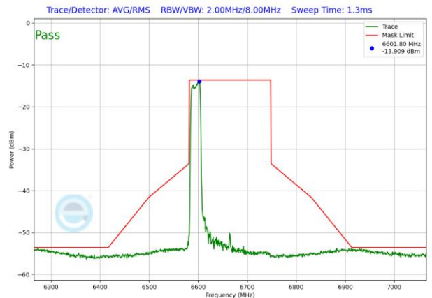
Plot 7-1230. VLP In-Band Emission Plot SDM Antenna WF2 (160MHz 802.11ax RU242 (UNII Band 7) – Ch. 143)
