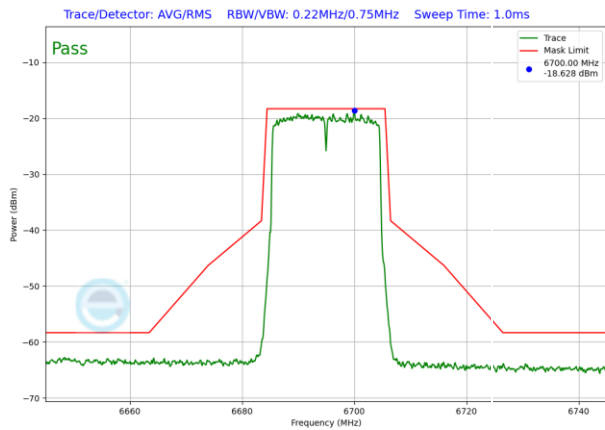
Plot 7-1213. VLP In-Band Emission Plot SDM Antenna WF5T (20MHz) 802.11ax RU242 (UNII Band 7) – Ch. 149
