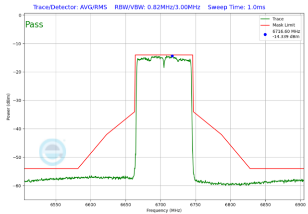
Plot 7-1228. VLP In-Band Emission Plot SDM Antenna WF2 (80MHz 802.11ax RU996 (UNII Band 7) – Ch. 151)
