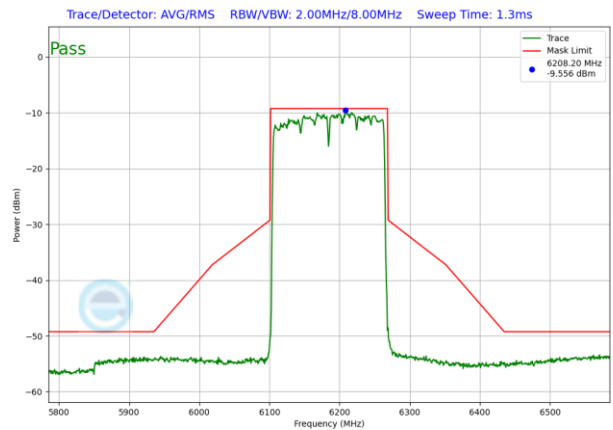
Plot 7-1211. VLP In-Band Emission Plot SDM Antenna WF5T (160MHz 802.11ax RU996x2 (UNII Band 5) – Ch. 47)
