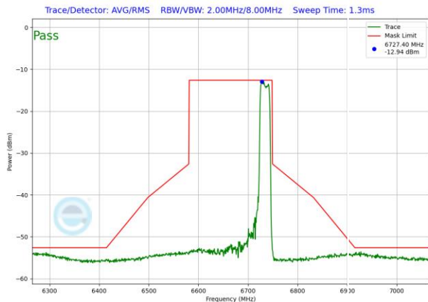
Plot 7-1233. VLP In-Band Emission Plot SDM Antenna WF5T (160MHz 802.11ax RU242 (UNII Band 7) – Ch. 143)
