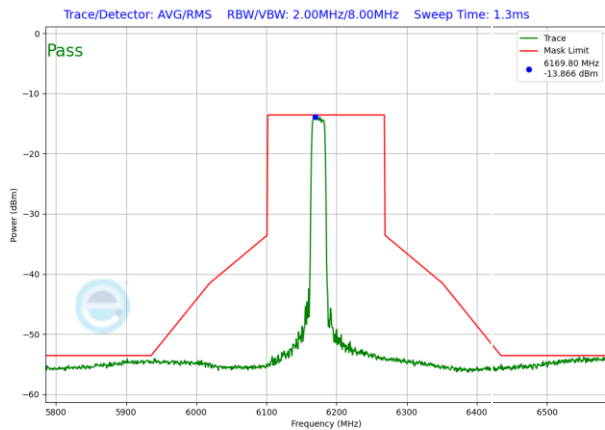
Plot 7-1208. VLP In-Band Emission Plot SDM Antenna WF2 (160MHz 802.11ax RU242 (UNII Band 5) – Ch. 47)
