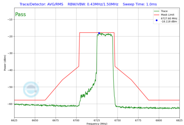
Plot 7-1218. VLP In-Band Emission Plot SDM Antenna WF2 (40MHz) 802.11ax RU242 (UNII Band 7) – Ch. 155
