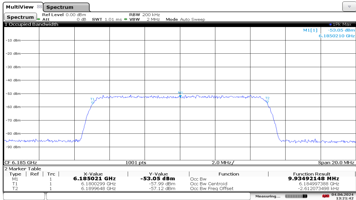
Plot 7-1239. AWGN Signal – UNII 5 – 160MHz – Mid
