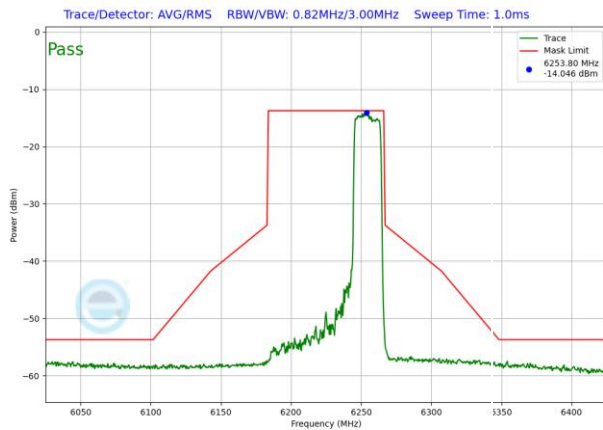
Plot 7-1202. VLP In-Band Emission Plot SDM Antenna WF2 (80MHz) 802.11ax RU242 (UNII Band 5) – Ch. 55)
