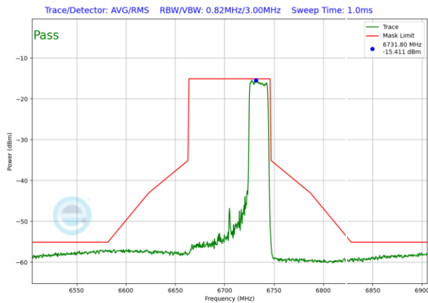
Plot 7-1226. VLP In-Band Emission Plot SDM Antenna WF2 (80MHz 802.11ax RU242 (UNII Band 7) – Ch. 151)
