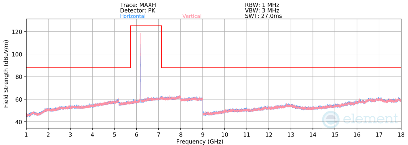
Plot 7-1282. Radiated Spurious Emissions above 1GHz Antenna WF5T (802.11ax – Ch. 45 – RU26)
