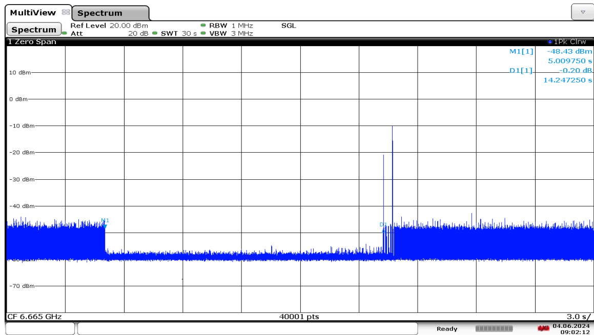
Plot 7-1264. LPI Contention Based Protocol Timing Plot – UNII 7 – 160MHz Channel 143 – High
