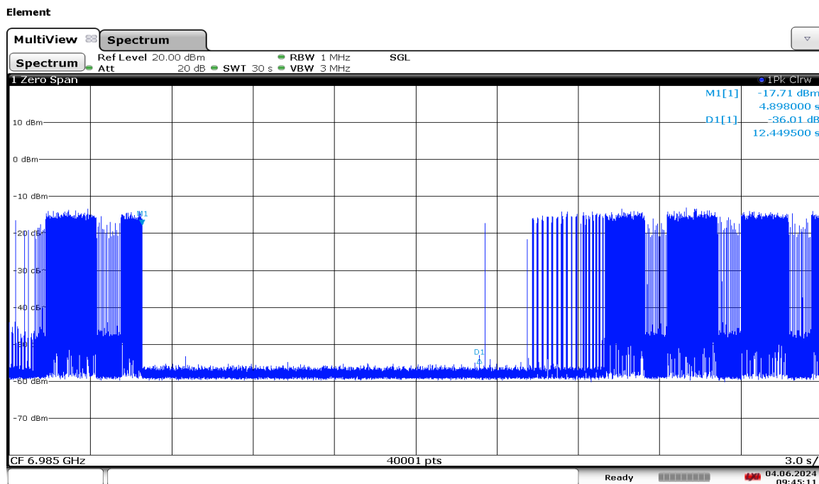
Plot 7-1267. LPI Contention Based Protocol Timing Plot – UNII 8 – 160MHz Channel 207 – Mid
