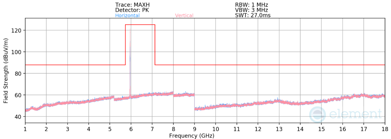
Plot 7-1281. Radiated Spurious Emissions above 1GHz Antenna WF5T (802.11ax – Ch. 1 – RU26)
