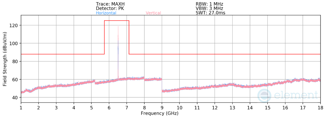
Plot 7-1286. Radiated Spurious Emissions above 1GHz Antenna WF5T (802.11ax – Ch. 113 – RU26)
