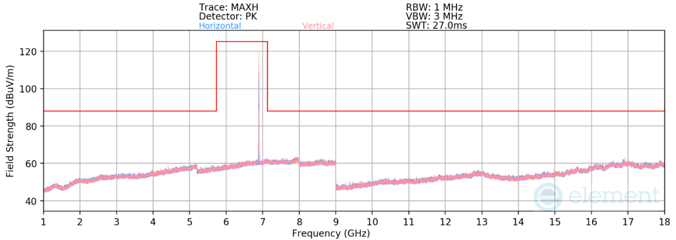
Plot 7-1290. Radiated Spurious Emissions above 1GHz Antenna WF5T (802.11ax – Ch. 189 – RU26)
