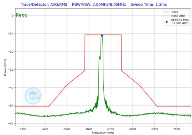
Plot 7-1186. VLP In-Band Emission Plot Antenna WF2 (160MHz 802.11ax RU106 (UNII Band 7) – Ch. 143)
