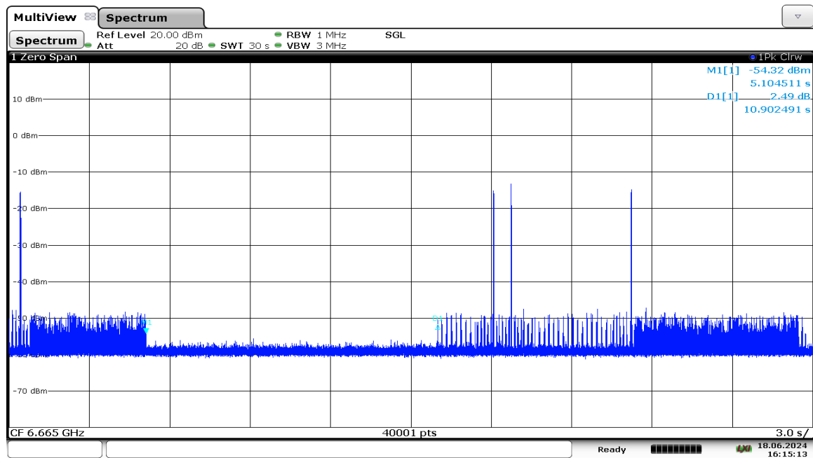
Plot 7-1274. VLP Contention Based Protocol Timing Plot – UNII 7 – 160MHz Channel 143 – Low
