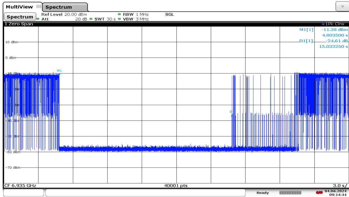
Plot 7-1265. LPI Contention Based Protocol Timing Plot – UNII 8 – 20MHz Channel 197
