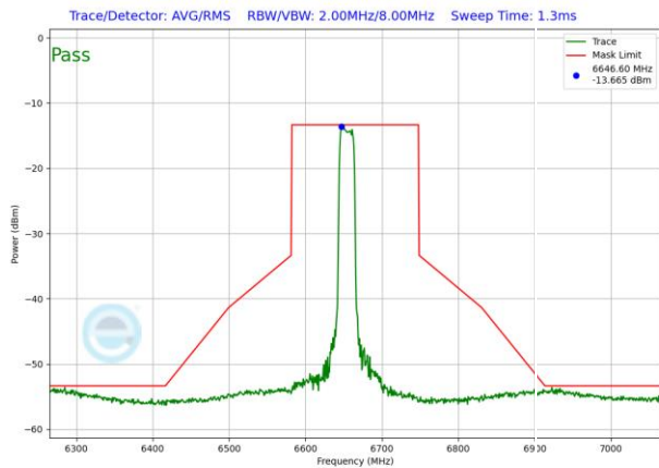
Plot 7-1232. VLP In-Band Emission Plot SDM Antenna WF2 (160MHz 802.11ax RU242 (UNII Band 7) – Ch. 143)
