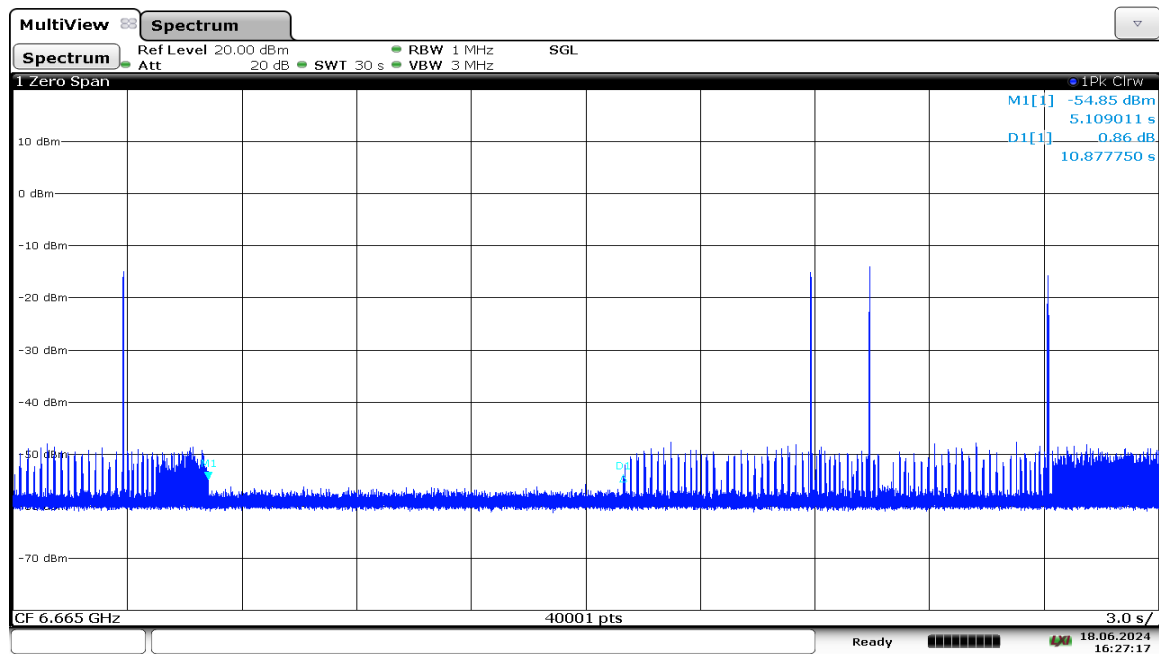
Plot 7-1276. VLP Contention Based Protocol Timing Plot – UNII 7 – 160MHz Channel 143 – High
