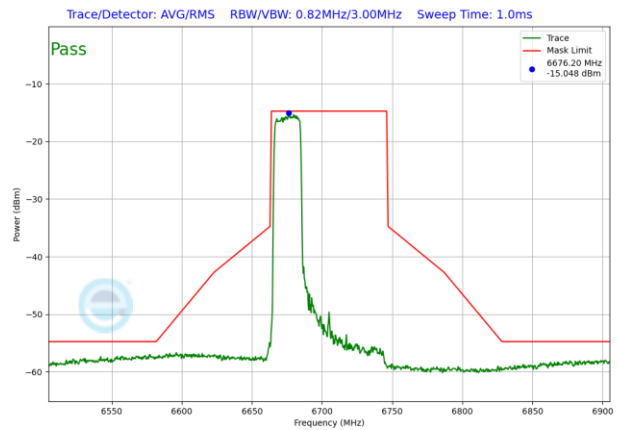
Plot 7-1222. VLP In-Band Emission Plot SDM Antenna WF2 (80MHz 802.11ax RU242 (UNII Band 7) – Ch. 151)
