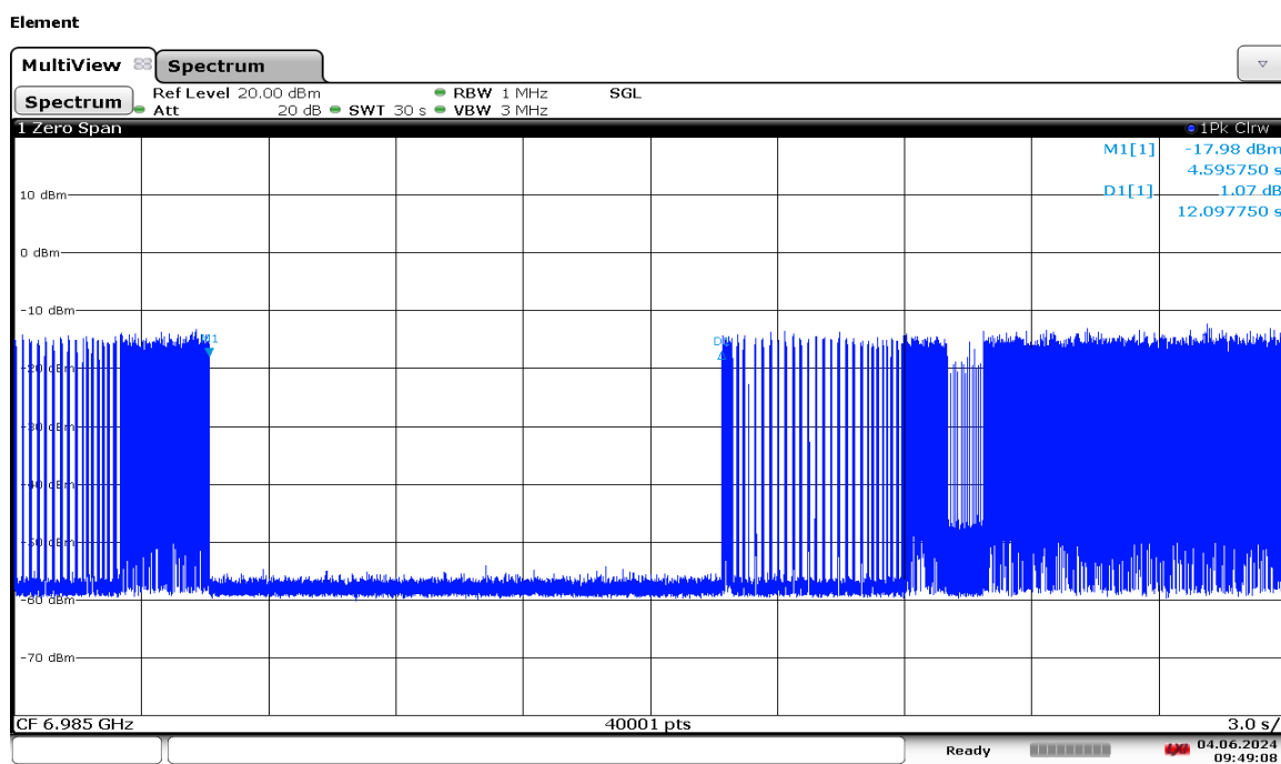
Plot 7-1268. LPI Contention Based Protocol Timing Plot – UNII 8 – 160MHz Channel 207 – High
