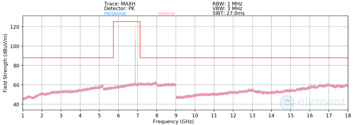
Plot 7-1289. Radiated Spurious Emissions above 1GHz Antenna WF5T (802.11ax – Ch. 185 – RU26)
