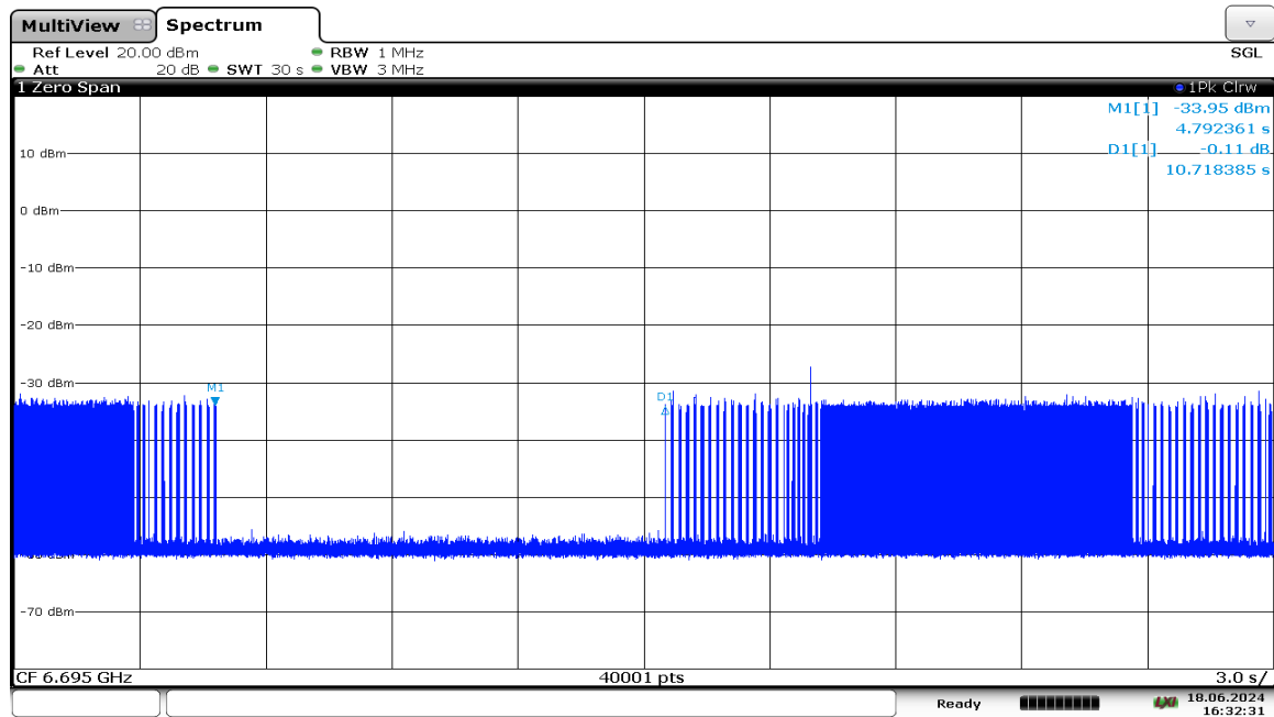
Plot 7-1273. VLP Contention Based Protocol Timing Plot – UNII 7 – 20MHz Channel 149
