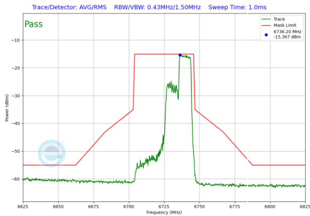
Plot 7-1179. VLP In-Band Emission Plot Antenna WF2 (40MHz 802.11ax RU106 (UNII Band 7) – Ch. 155)
