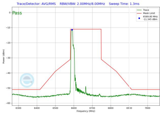
Plot 7-1185. VLP In-Band Emission Plot Antenna WF2 (160MHz 802.11ax RU106 (UNII Band 7) – Ch. 143)
