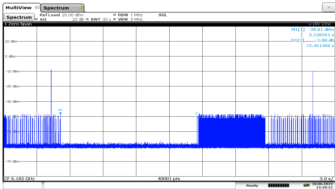
Plot 7-1270. VLP Contention Based Protocol Timing Plot – UNII 5 – 160MHz Channel 47 – Low
