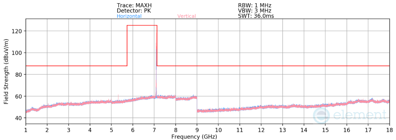
Plot 7-1292. Radiated Spurious Emissions above 1GHz Antenna WF5T (802.11ax – Ch. 229 – RU26)
