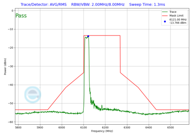
Plot 7-1205. VLP In-Band Emission Plot SDM Antenna WF5T (160MHz) 802.11ax RU242 (UNII Band 5) – Ch. 47)
