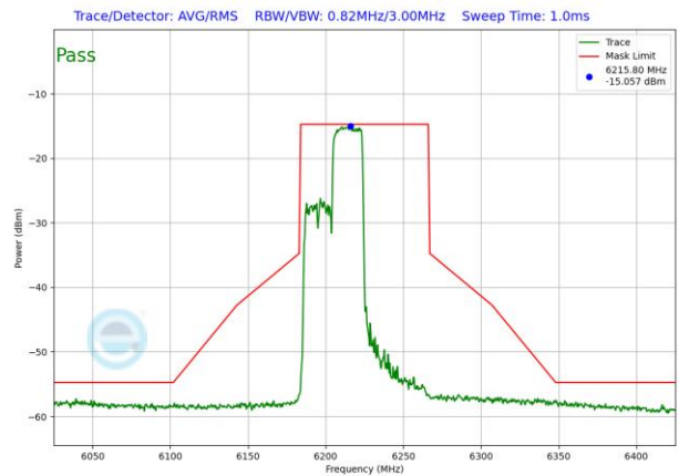
Plot 7-1199. VLP In-Band Emission Plot SDM Antenna WF5T (80MHz) 802.11ax RU242 (UNII Band 5) – Ch. 55
