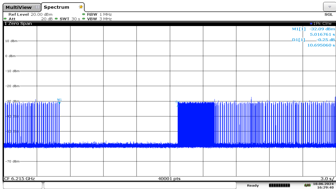
Plot 7-1269. VLP Contention Based Protocol Timing Plot – UNII 5 – 20MHz Channel 53
