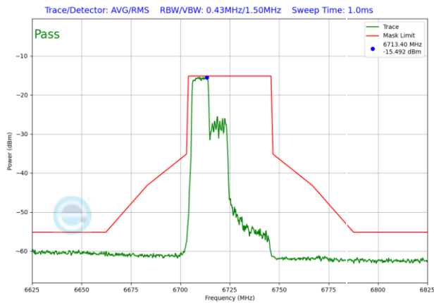
Plot 7-1177. VLP In-Band Emission Plot Antenna WF2 (40MHz 802.11ax RU106 (UNII Band 7) – Ch. 155)
