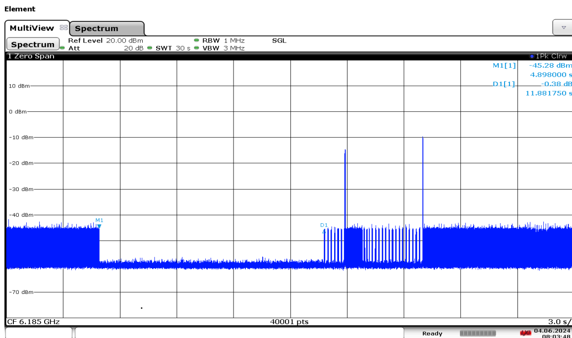
Plot 7-1254. LPI Contention Based Protocol Timing Plot – UNII 5 – 160MHz Channel 47 – Low
