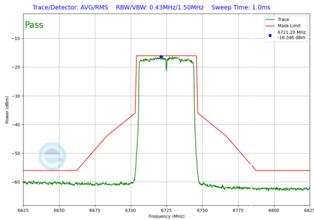
Plot 7-1219. VLP In-Band Emission Plot SDM Antenna WF5T (40MHz 802.11ax RU484 (UNII Band 7) – Ch. 155)
