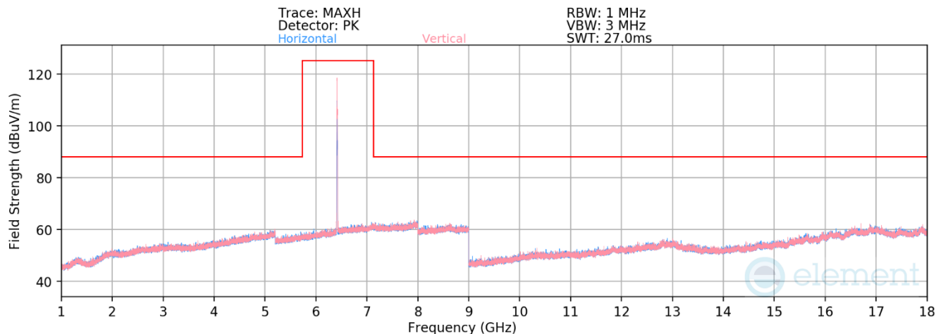
Plot 7-1283. Radiated Spurious Emissions above 1GHz Antenna WF5T (802.11ax – Ch. 93 – RU26)
