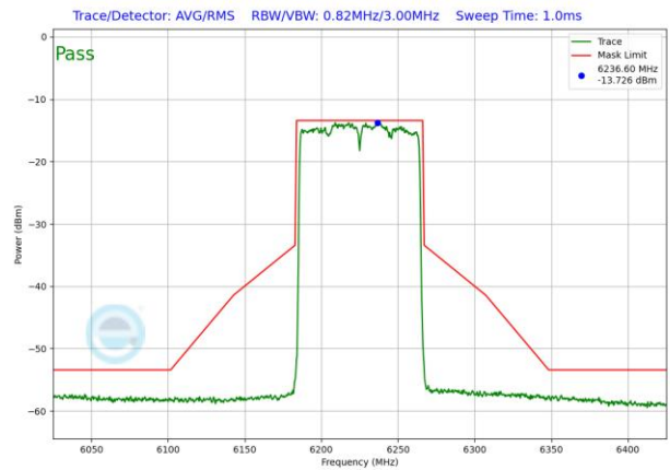
Plot 7-1204. VLP In-Band Emission Plot SDM Antenna WF2 (80MHz) 802.11ax RU996 (UNII Band 5) – Ch. 55)
