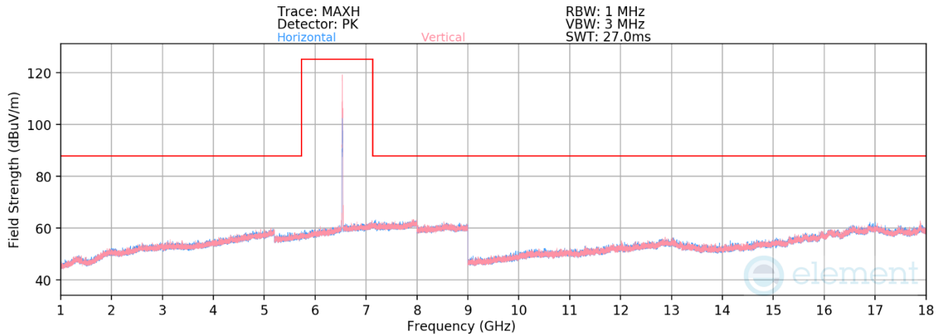
Plot 7-1287. Radiated Spurious Emissions above 1GHz Antenna WF5T (802.11ax – Ch. 117 – RU26)
