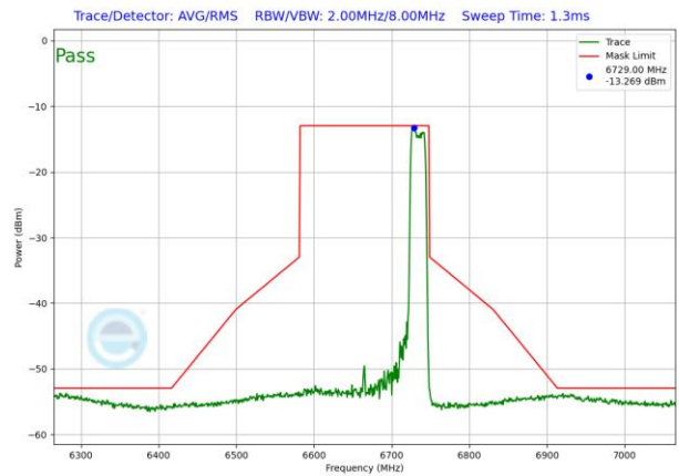
Plot 7-1234. VLP In-Band Emission Plot SDM Antenna WF2 (160MHz 802.11ax RU242 (UNII Band 7) – Ch. 143)
