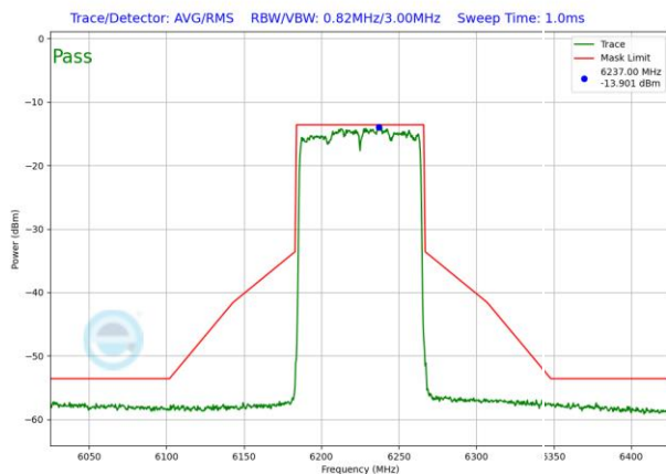
Plot 7-1203. VLP In-Band Emission Plot SDM Antenna WF5T (80MHz) 802.11ax RU996 (UNII Band 5) – Ch. 55)
