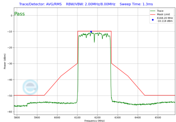
Plot 7-1212. VLP In-Band Emission Plot SDM Antenna WF2 (160MHz 802.11ax RU996x2 (UNII Band 5) – Ch. 47)
