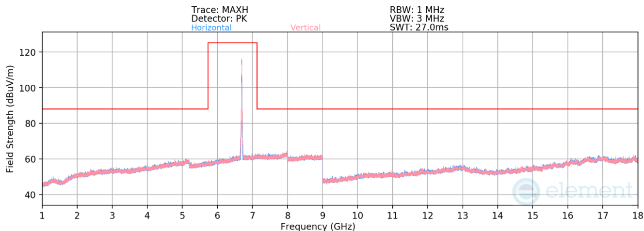
Plot 7-1354. Radiated Spurious Emissions above 1GHz SDM (802.11ax – Ch. 149 – RU242)
