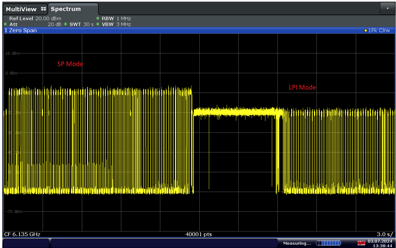
Plot 7-1417. Client device observation from Standard Power AP mode to Low Power Indoor AP mode
