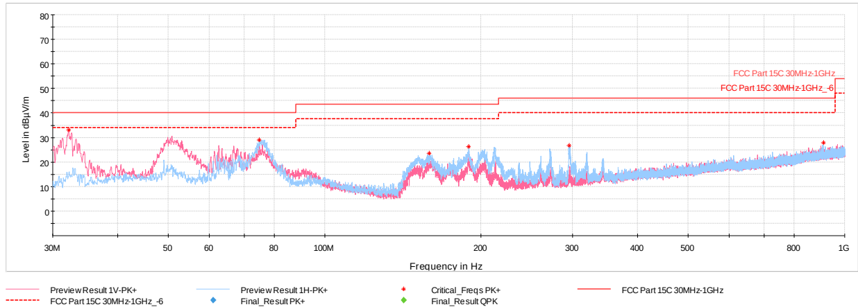
Plot 7-1411. Radiated Spurious Emissions below 1GHz SDM (802.11ax – Ch.1 – RU26) with AC/DC adaptor via USB-C cable with wire charger
