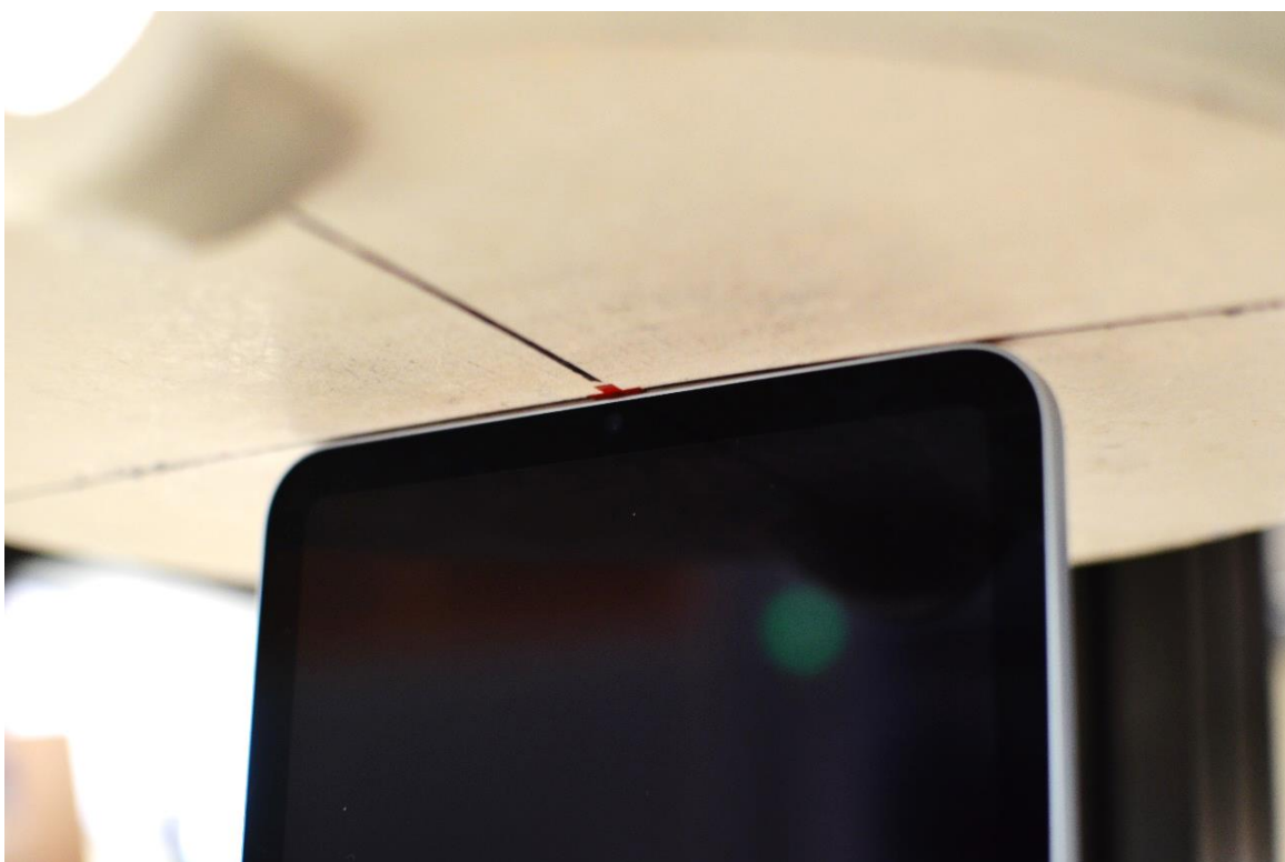
SAR Test Setup Photo 4: Top Edge at 0mm – Ant WF8/WF7/WF5T/WF2
