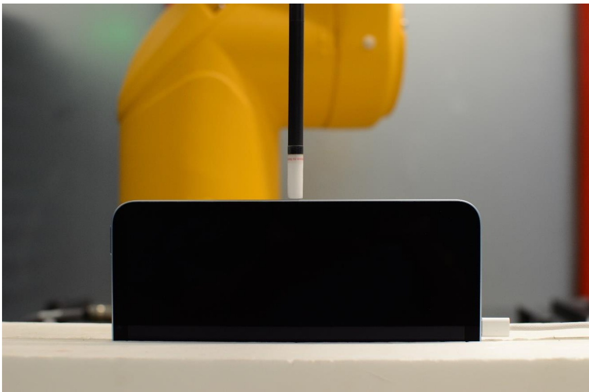
Near Field Power Density Test Setup Photo 18: Right Edge at 2mm – WF5T/WF2
