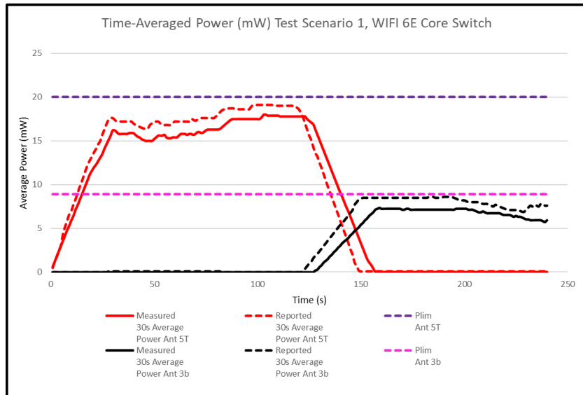
Figure J-6 30s Average Power vs. Time, 6 GHz
