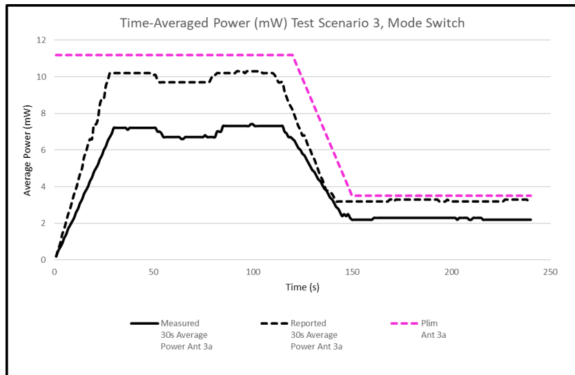
Figure J-10 30s Average Power vs. Time during Mode Switch
